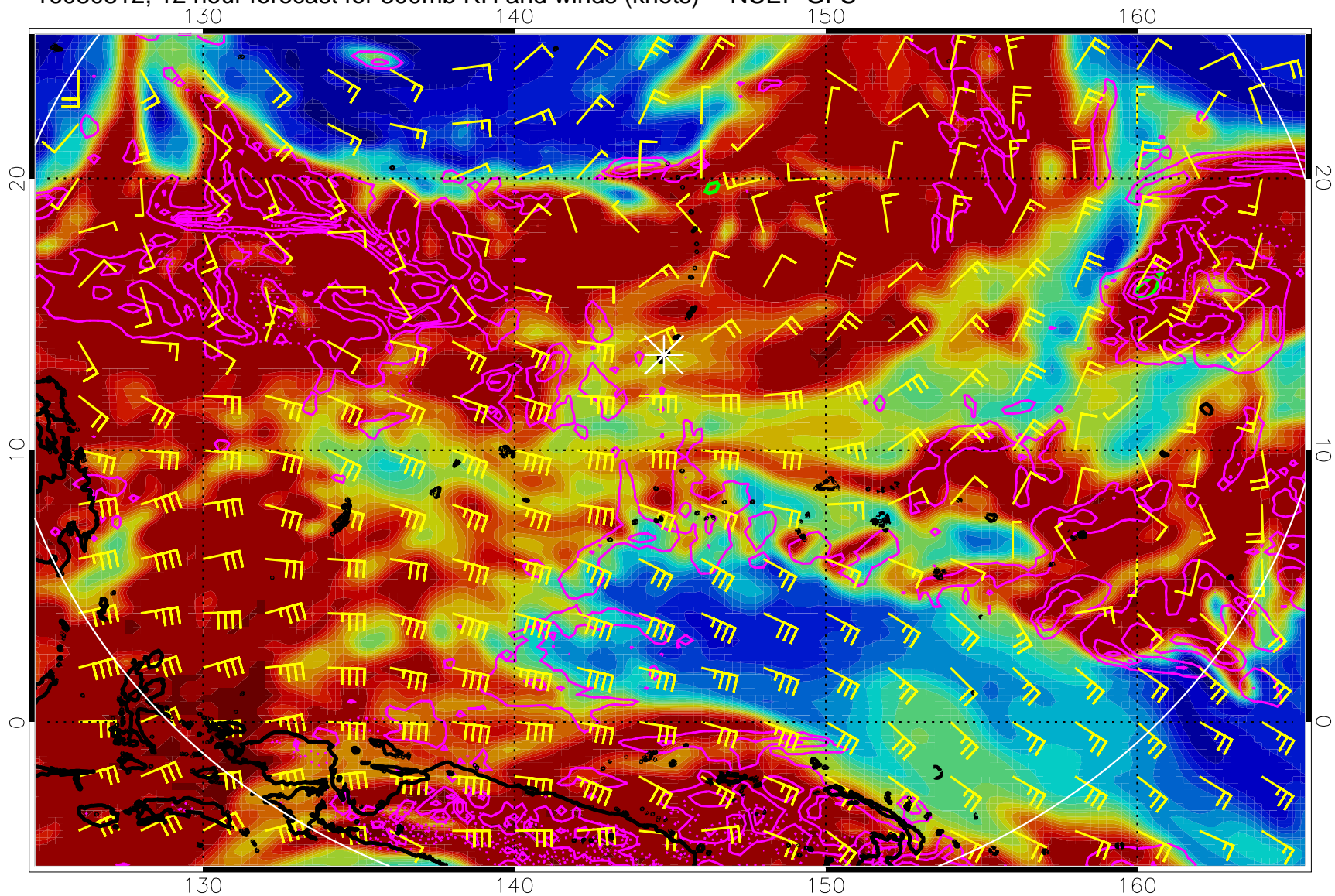
16080812, 12 hour forecast for 300mb RH and winds (knots) -- NCEP GFS
