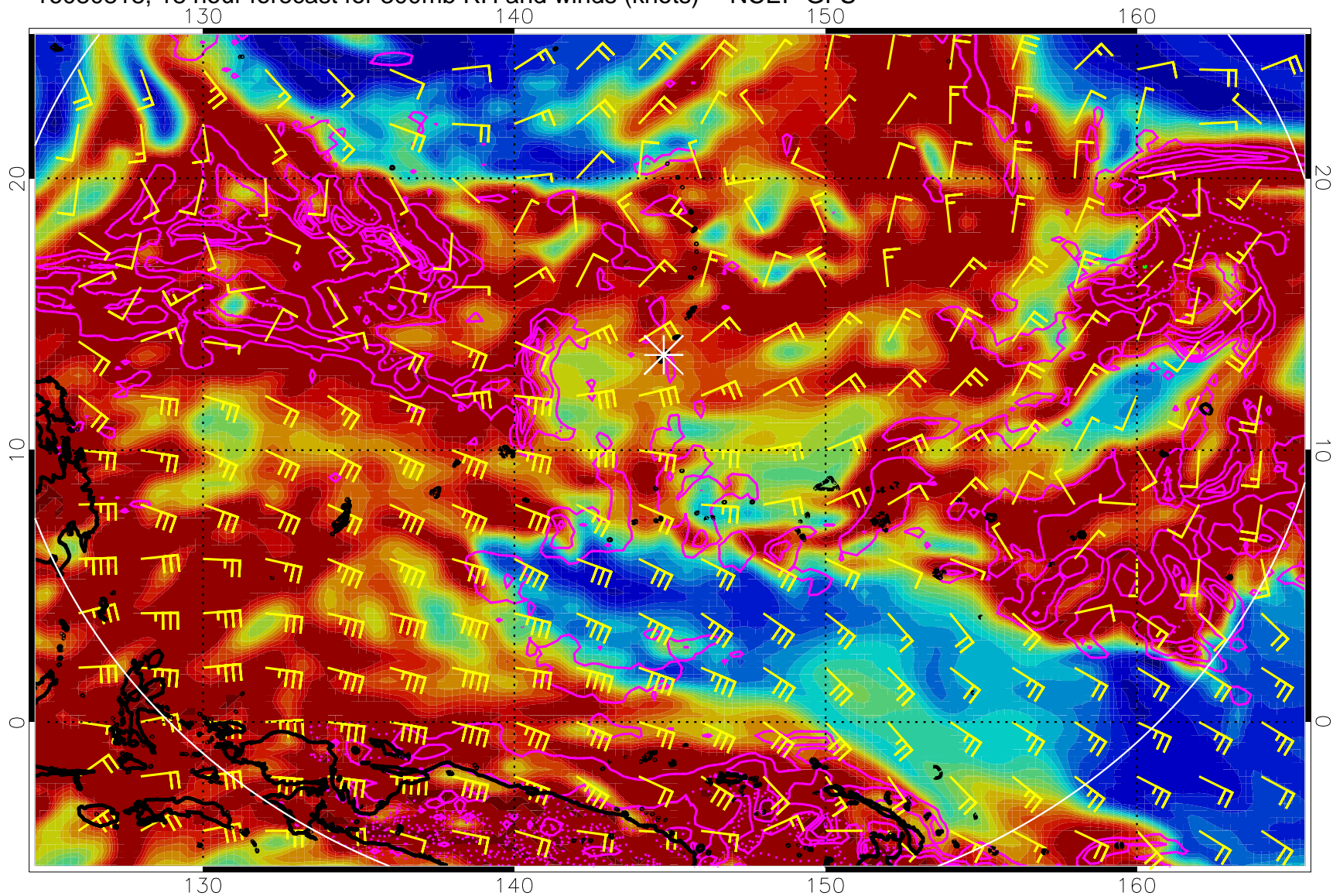
16080818, 18 hour forecast for 300mb RH and winds (knots) -- NCEP GFS
