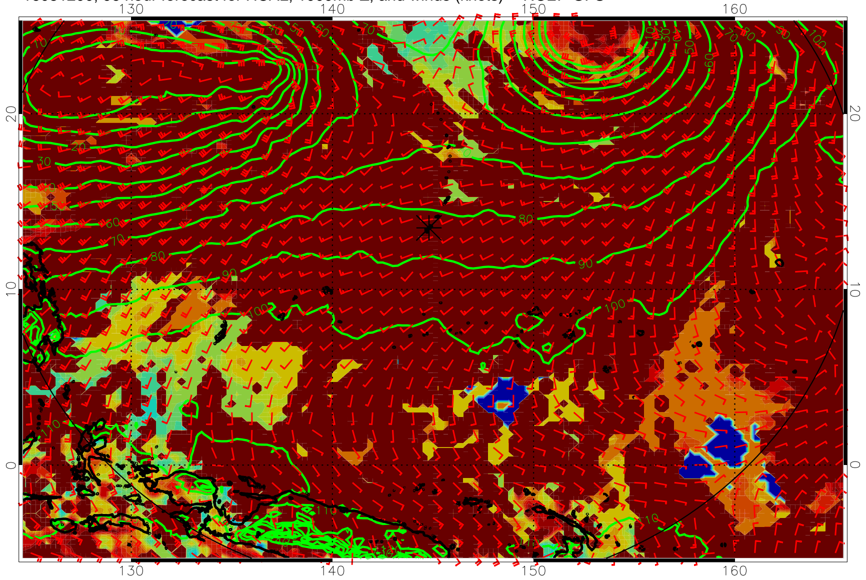
16081200, 96 hour forecast for HCAL, 1000mb Z, and winds (knots) -- NCEP GFS
