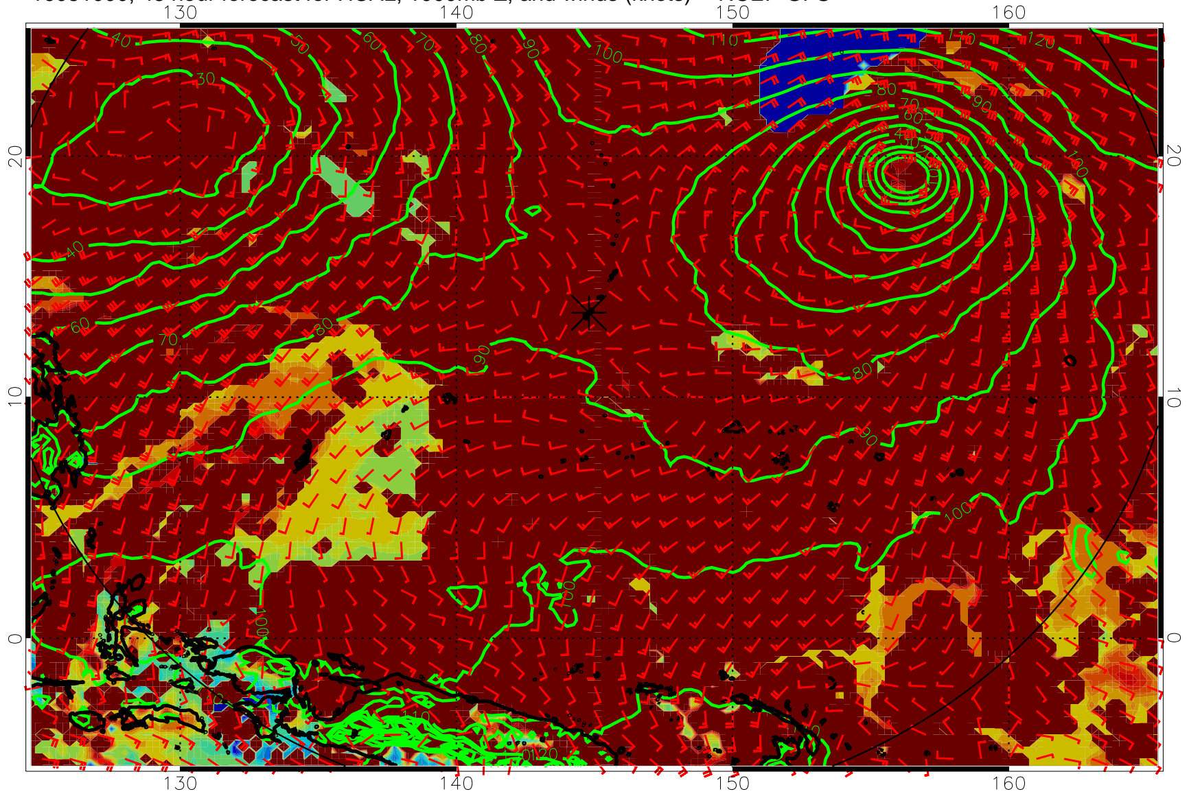
16081000, 48 hour forecast for HCAL, 1000mb Z, and winds (knots) -- NCEP GFS
