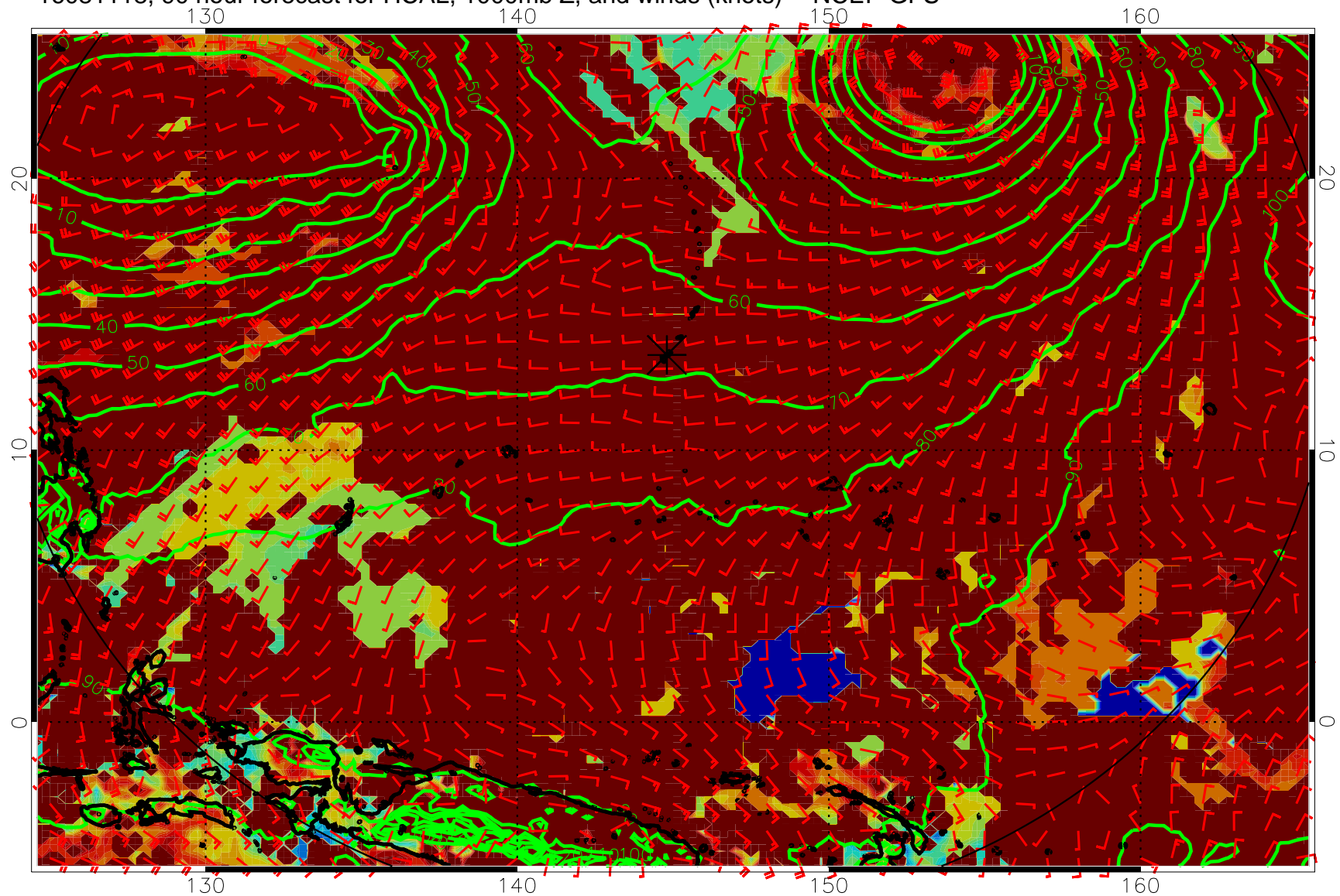
16081118, 90 hour forecast for HCAL, 1000mb Z, and winds (knots) -- NCEP GFS
