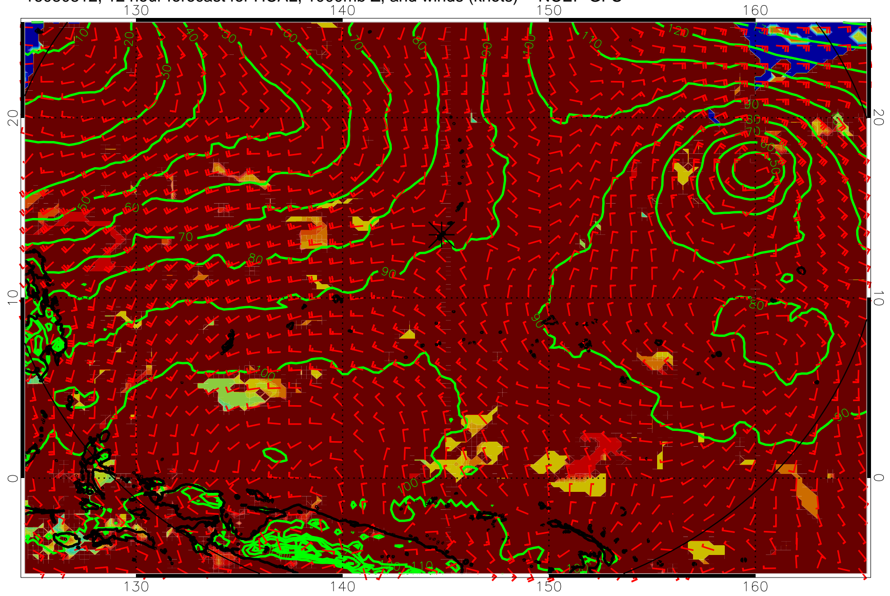
16080812, 12 hour forecast for HCAL, 1000mb Z, and winds (knots) -- NCEP GFS
