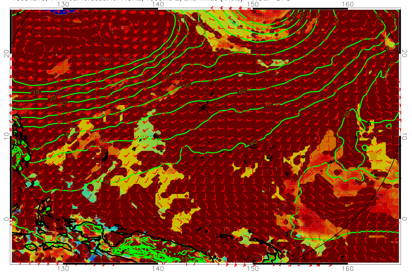
16081218, 114 hour forecast for HCAL, 1000mb Z, and winds (knots) -- NCEP GFS
