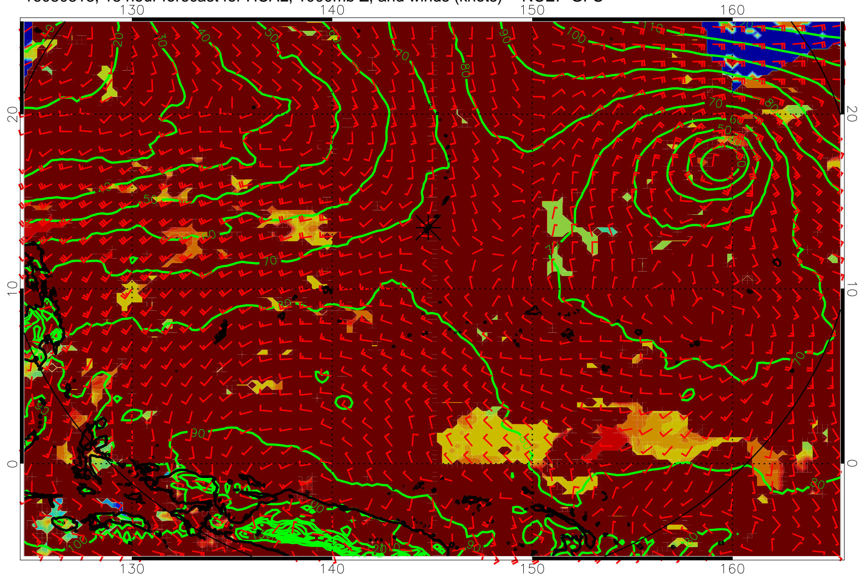
16080818, 18 hour forecast for HCAL, 1000mb Z, and winds (knots) -- NCEP GFS
