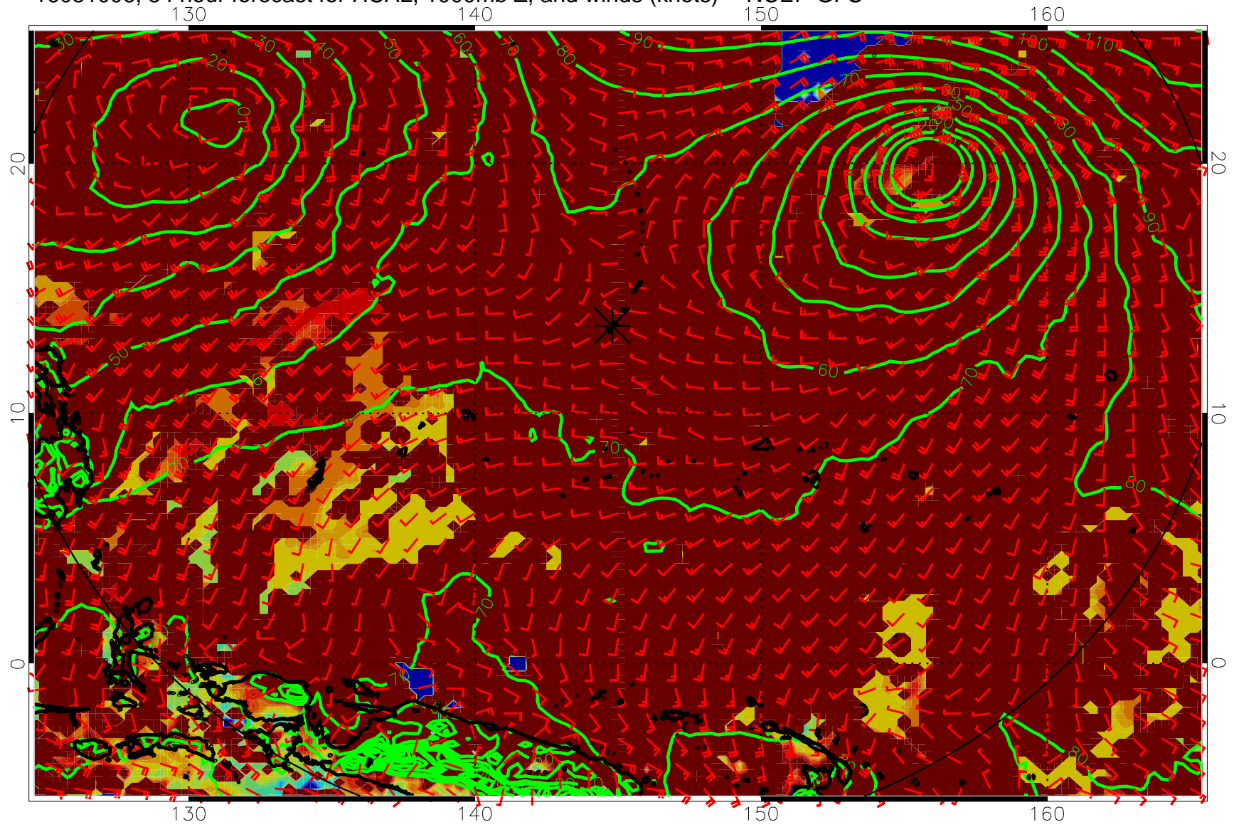
16081006, 54 hour forecast for HCAL, 1000mb Z, and winds (knots) -- NCEP GFS
