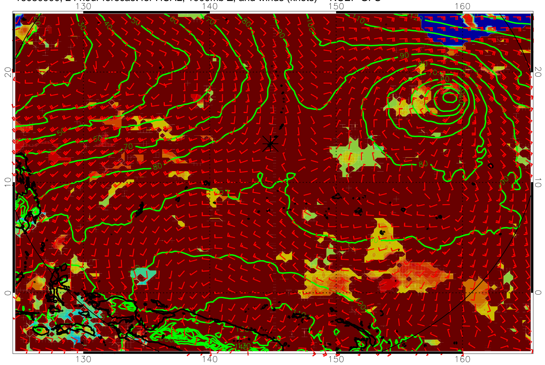
16080900, 24 hour forecast for HCAL, 1000mb Z, and winds (knots) -- NCEP GFS
