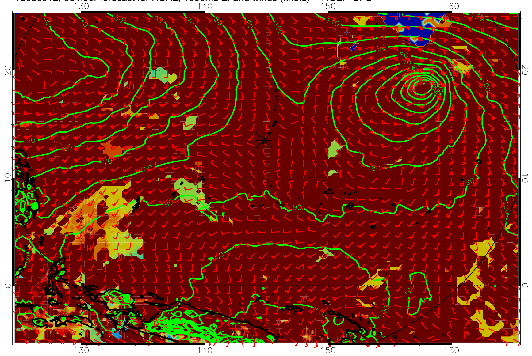
16080912, 36 hour forecast for HCAL, 1000mb Z, and winds (knots) -- NCEP GFS
