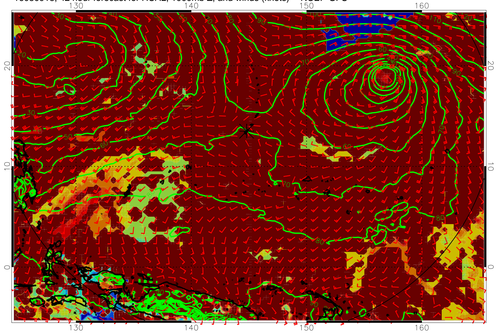
16080918, 42 hour forecast for HCAL, 1000mb Z, and winds (knots) -- NCEP GFS
