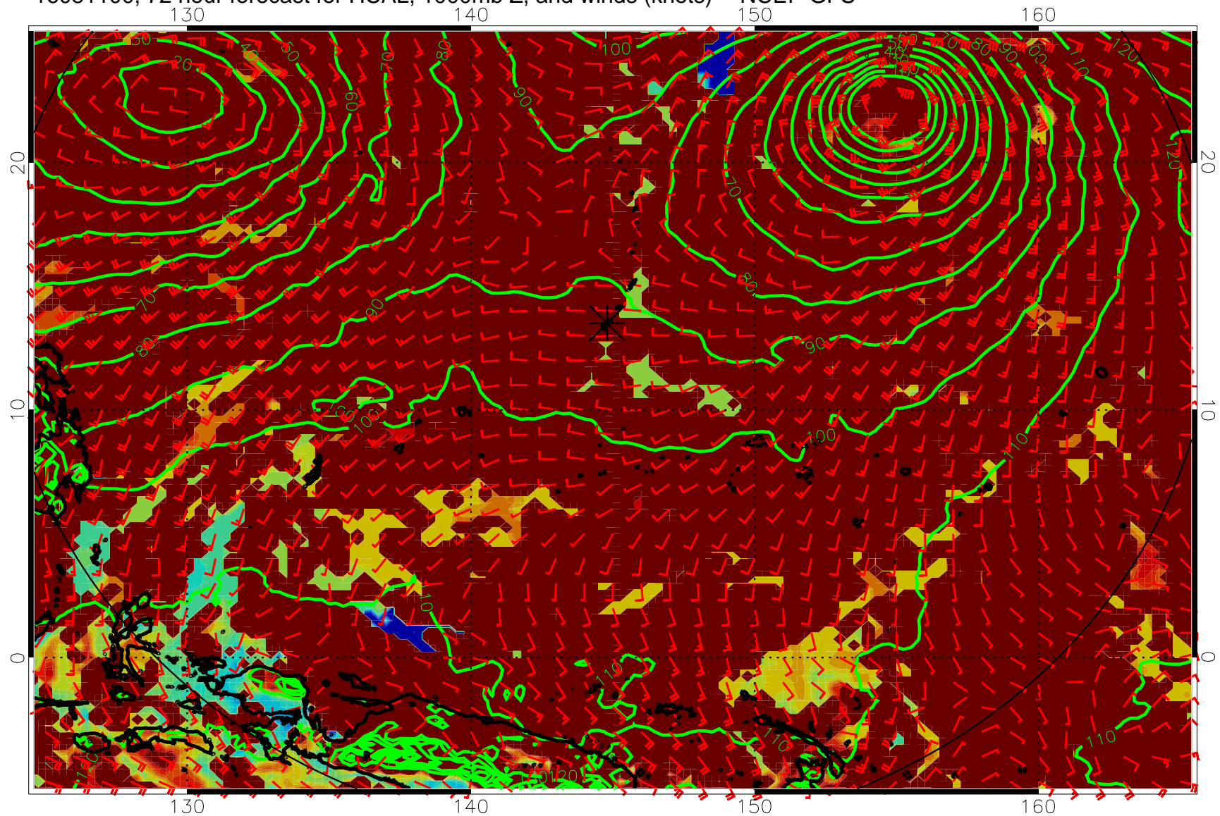
16081100, 72 hour forecast for HCAL, 1000mb Z, and winds (knots) -- NCEP GFS
