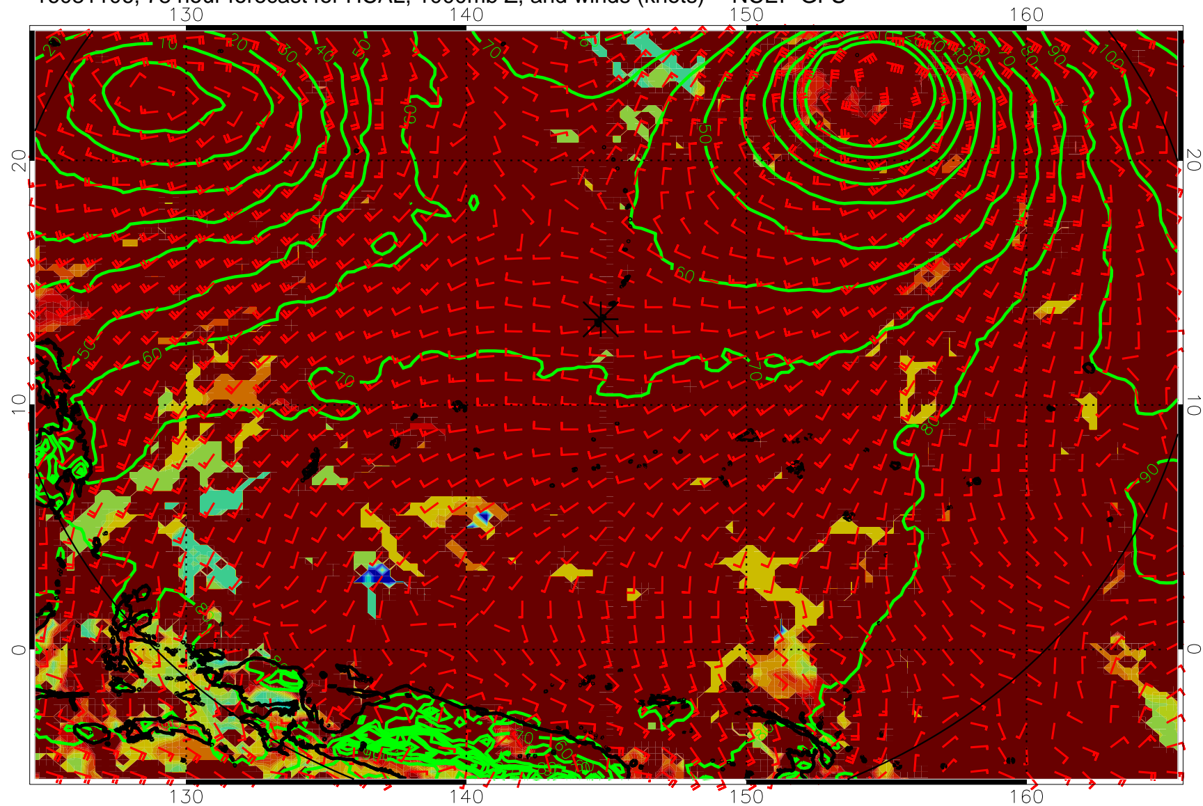
16081106, 78 hour forecast for HCAL, 1000mb Z, and winds (knots) -- NCEP GFS
