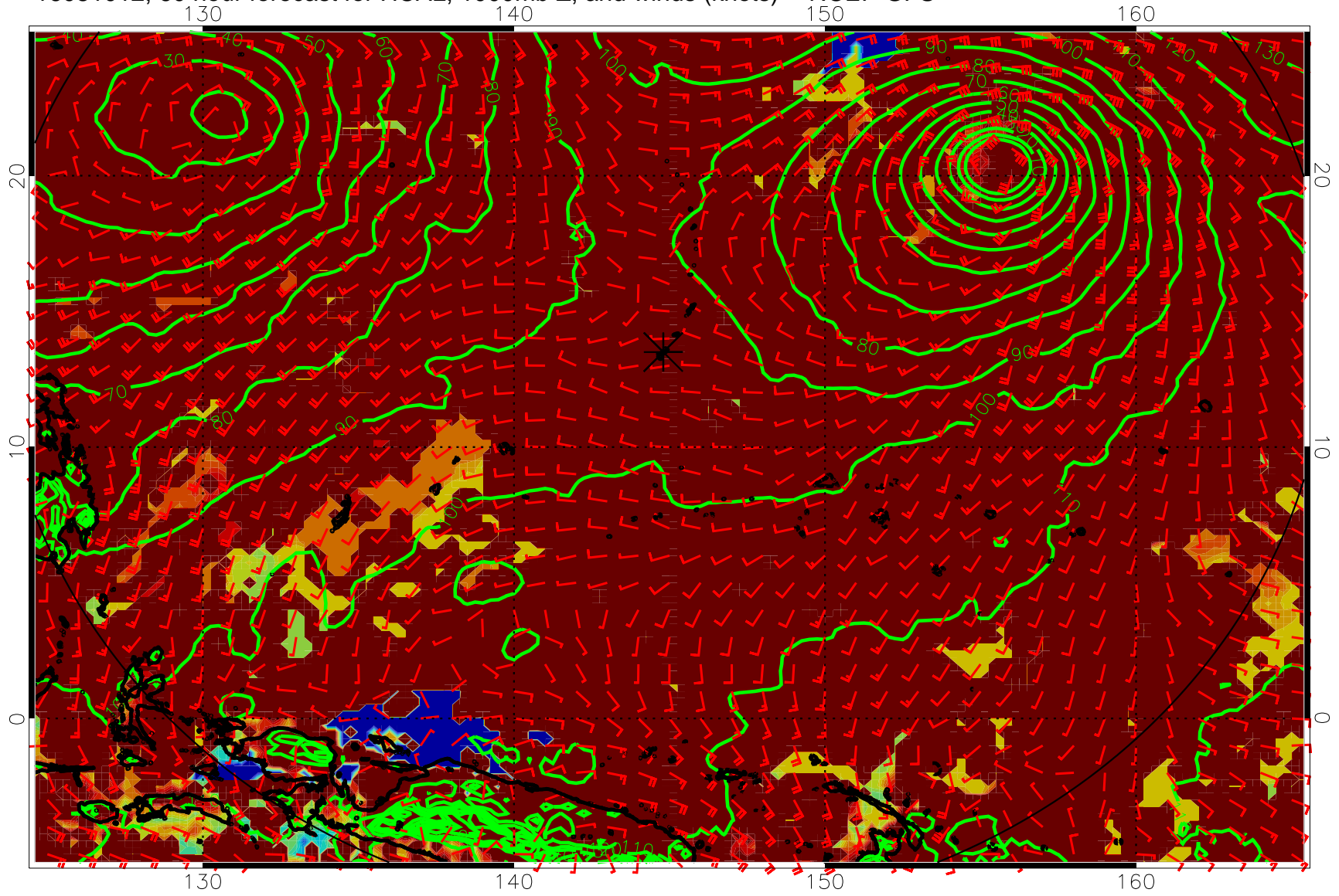
16081012, 60 hour forecast for HCAL, 1000mb Z, and winds (knots) -- NCEP GFS
