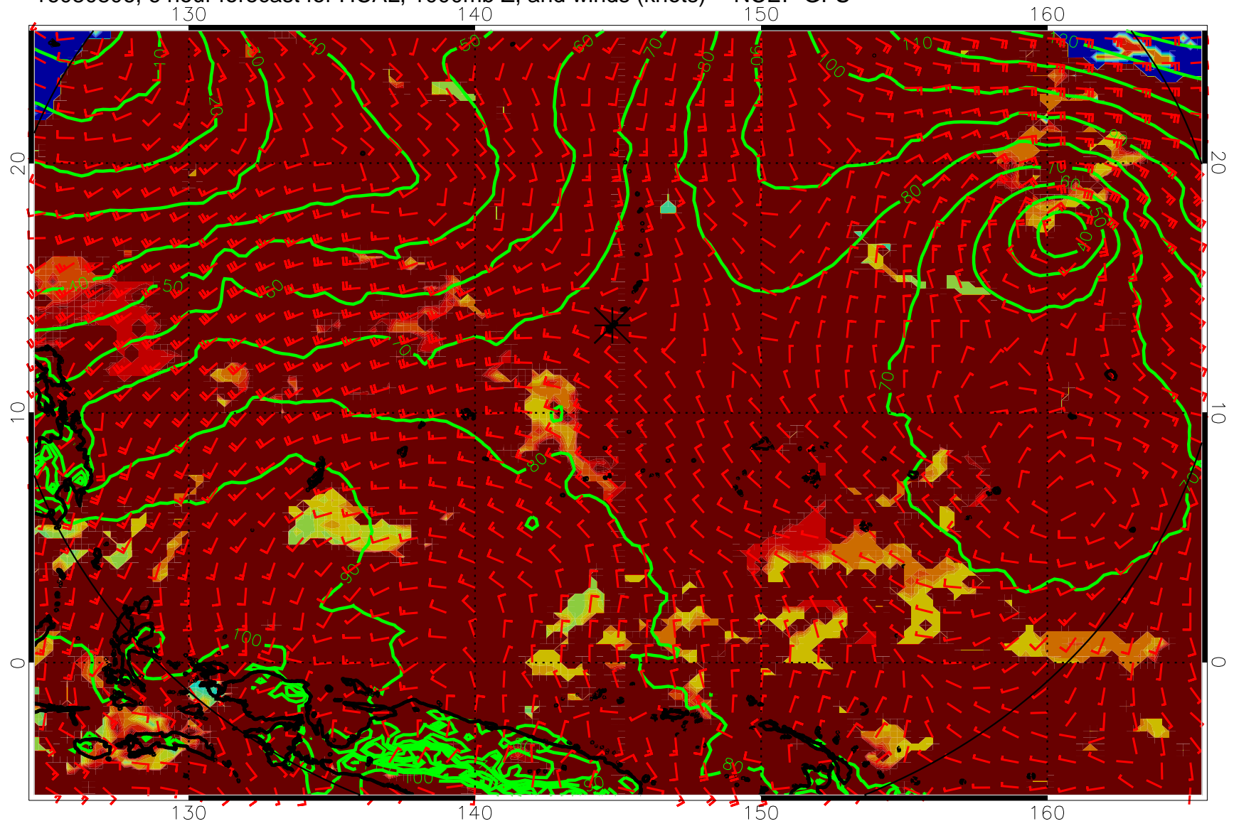
16080806, 6 hour forecast for HCAL, 1000mb Z, and winds (knots) -- NCEP GFS
