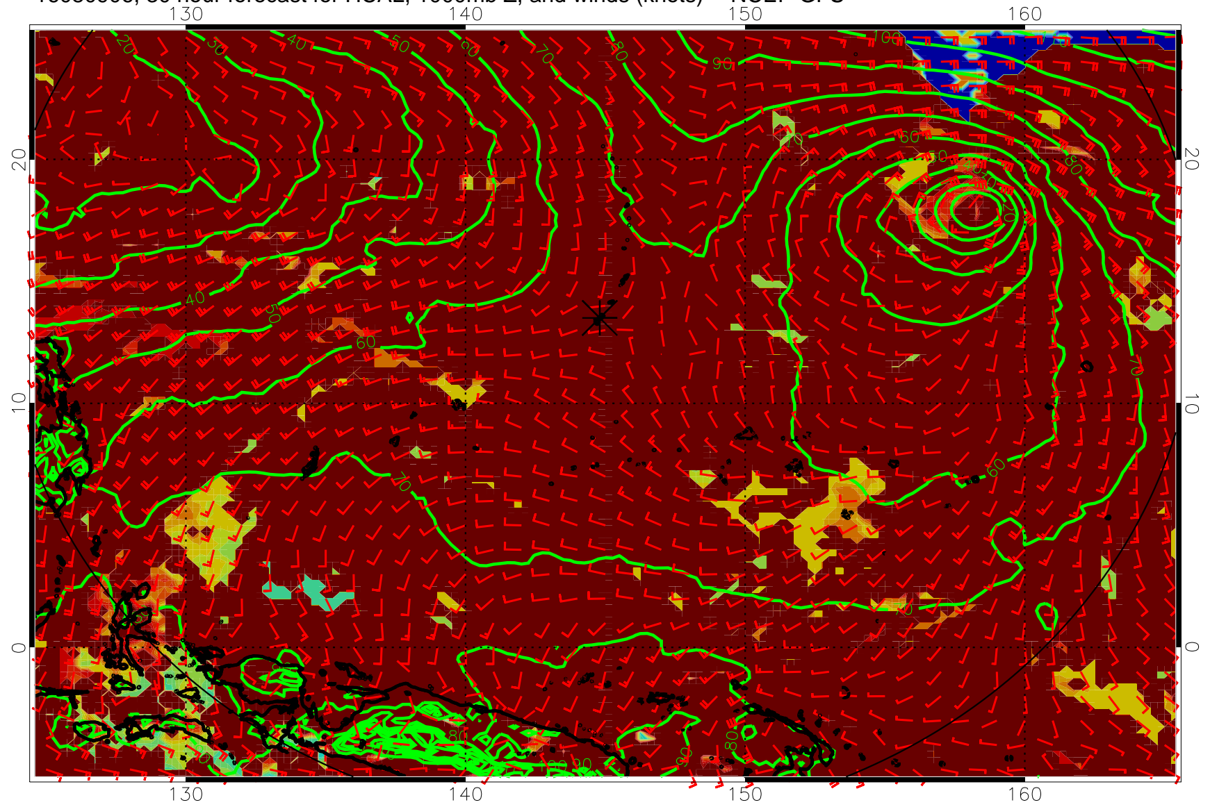
16080906, 30 hour forecast for HCAL, 1000mb Z, and winds (knots) -- NCEP GFS
