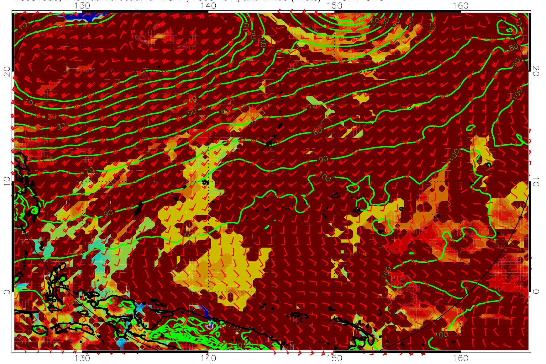
16081300, 120 hour forecast for HCAL, 1000mb Z, and winds (knots) -- NCEP GFS
