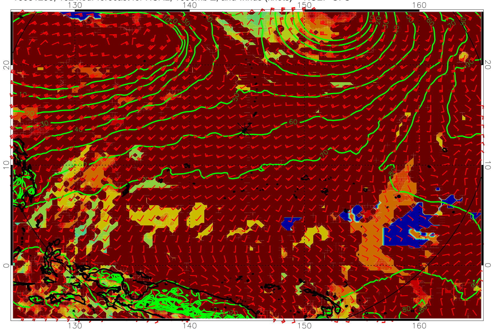
16081206, 102 hour forecast for HCAL, 1000mb Z, and winds (knots) -- NCEP GFS
