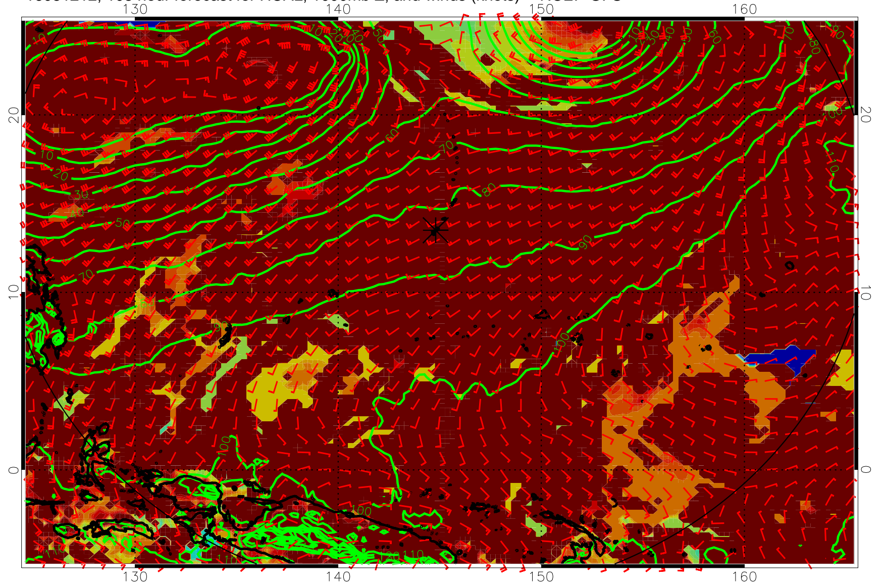
16081212, 108 hour forecast for HCAL, 1000mb Z, and winds (knots) -- NCEP GFS
