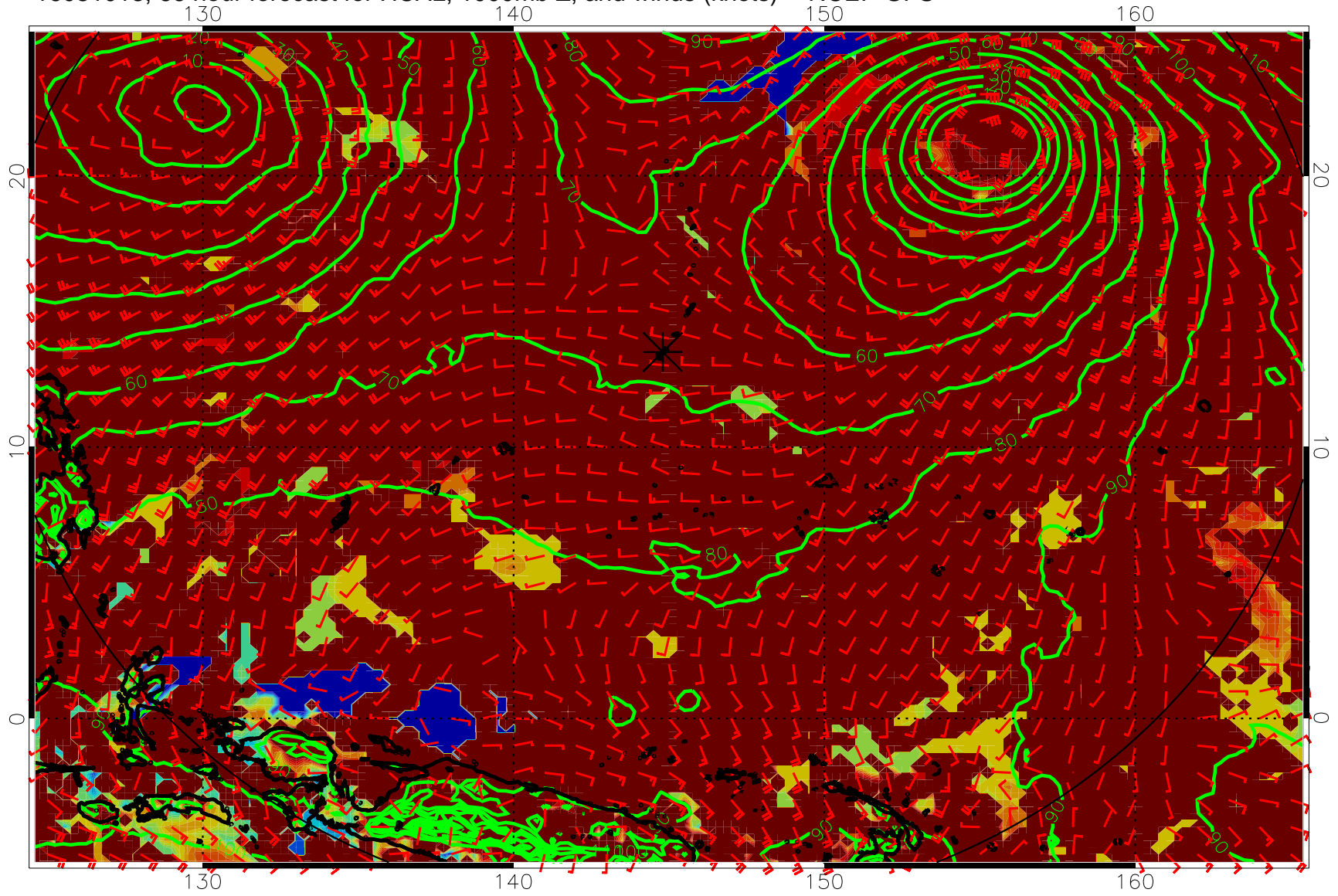
16081018, 66 hour forecast for HCAL, 1000mb Z, and winds (knots) -- NCEP GFS
