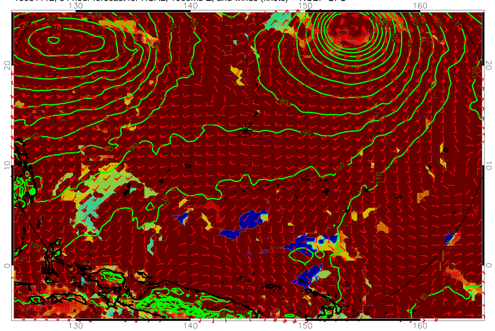
16081112, 84 hour forecast for HCAL, 1000mb Z, and winds (knots) -- NCEP GFS
