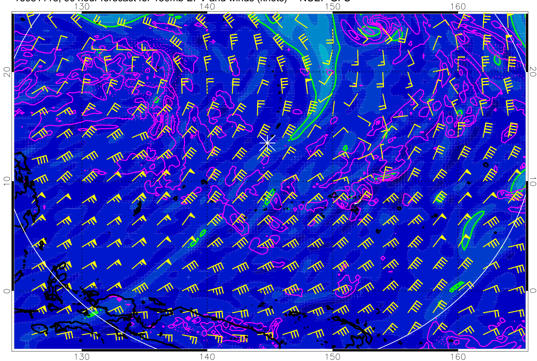
16081118, 90 hour forecast for 150mb EPV and winds (knots) -- NCEP GFS
