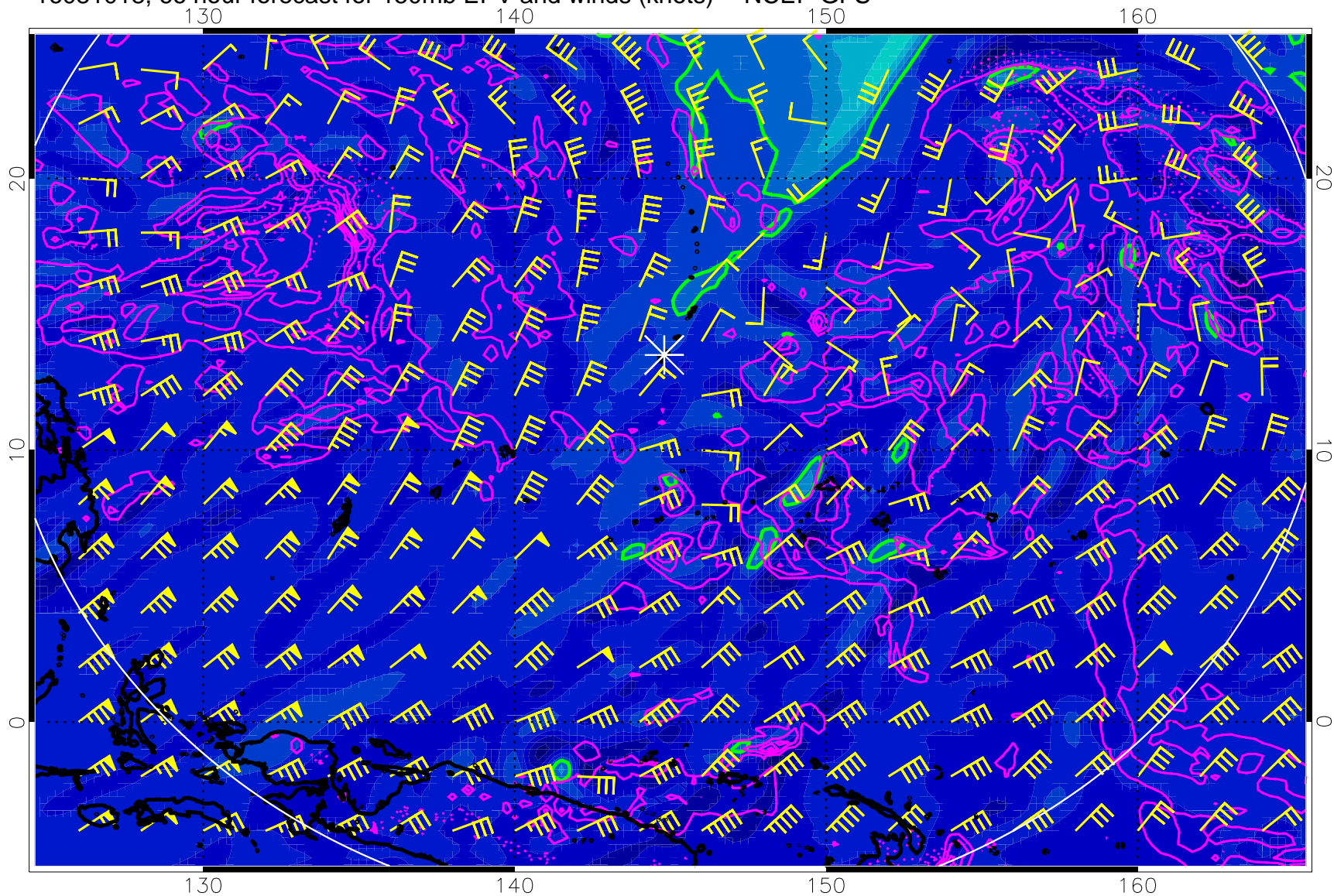
16081018, 66 hour forecast for 150mb EPV and winds (knots) -- NCEP GFS
