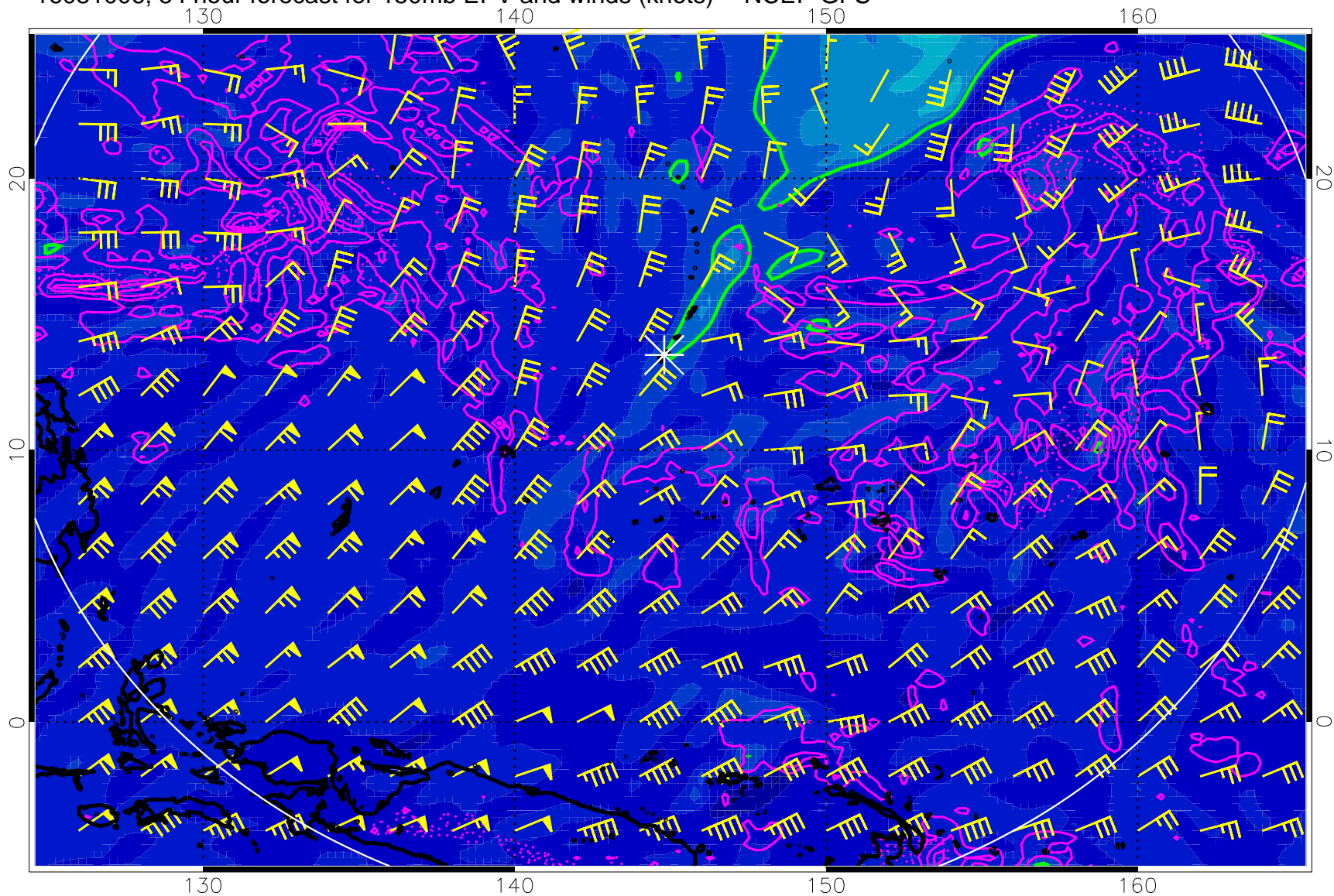
16081006, 54 hour forecast for 150mb EPV and winds (knots) -- NCEP GFS
