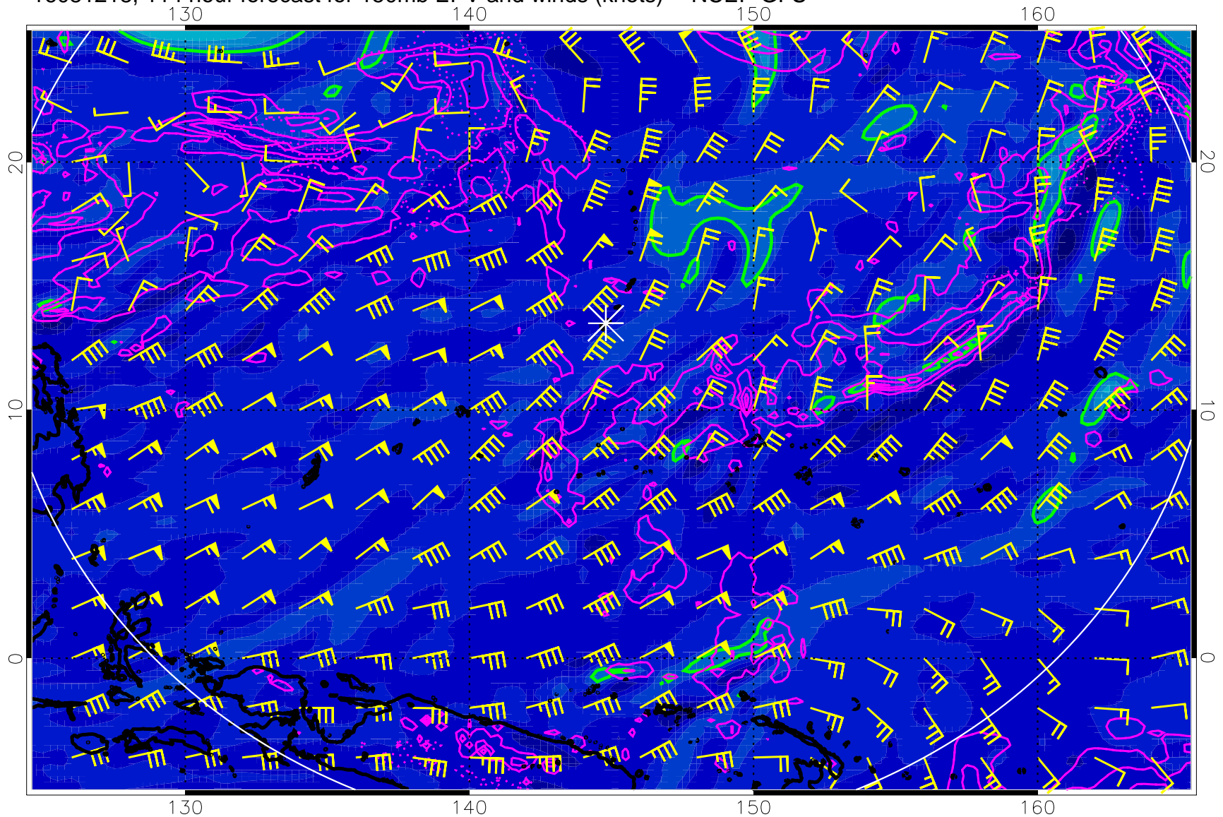
16081218, 114 hour forecast for 150mb EPV and winds (knots) -- NCEP GFS
