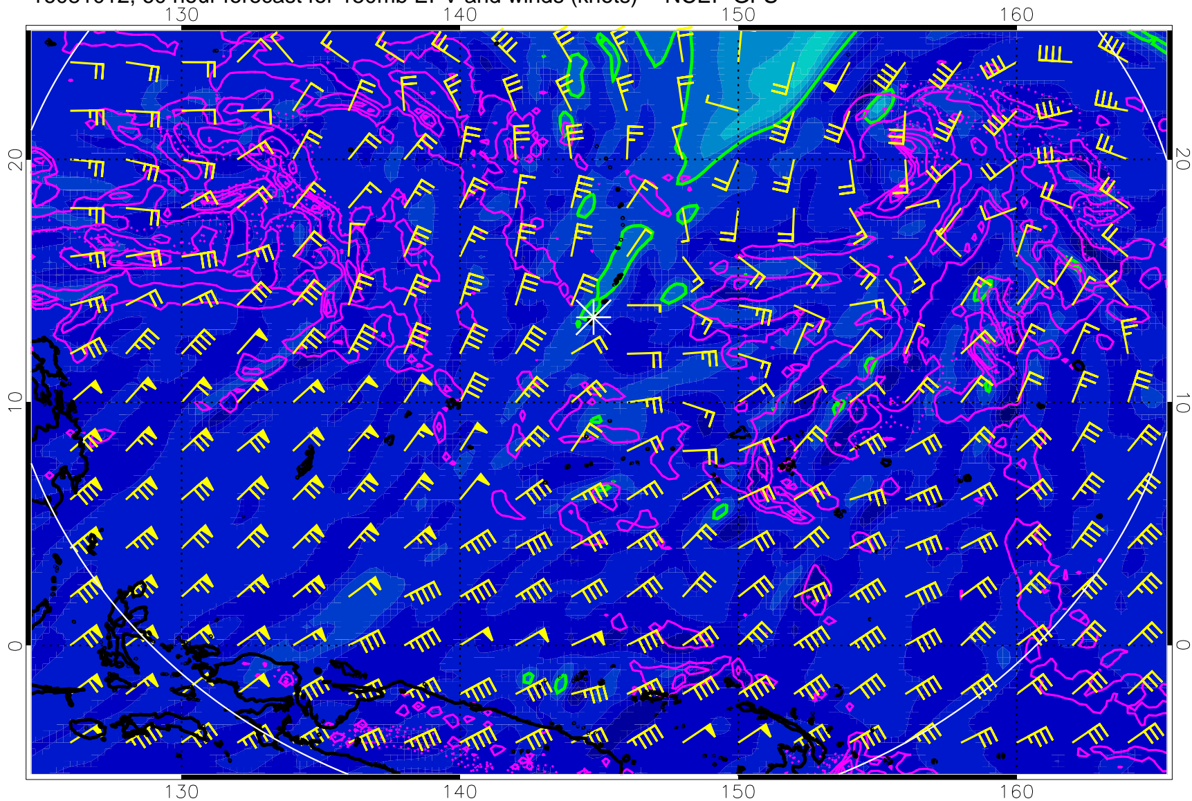
16081012, 60 hour forecast for 150mb EPV and winds (knots) -- NCEP GFS
