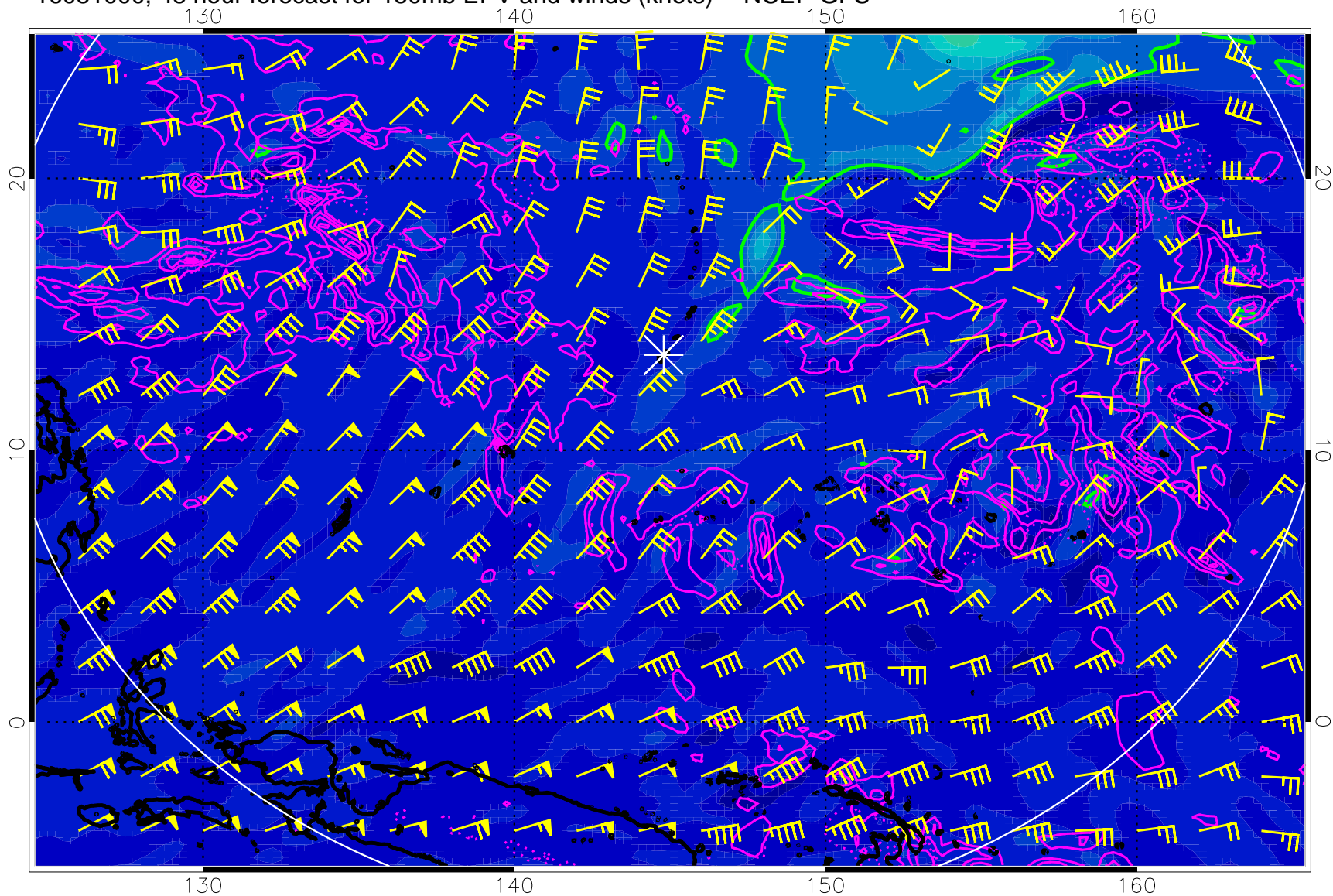
16081000, 48 hour forecast for 150mb EPV and winds (knots) -- NCEP GFS
