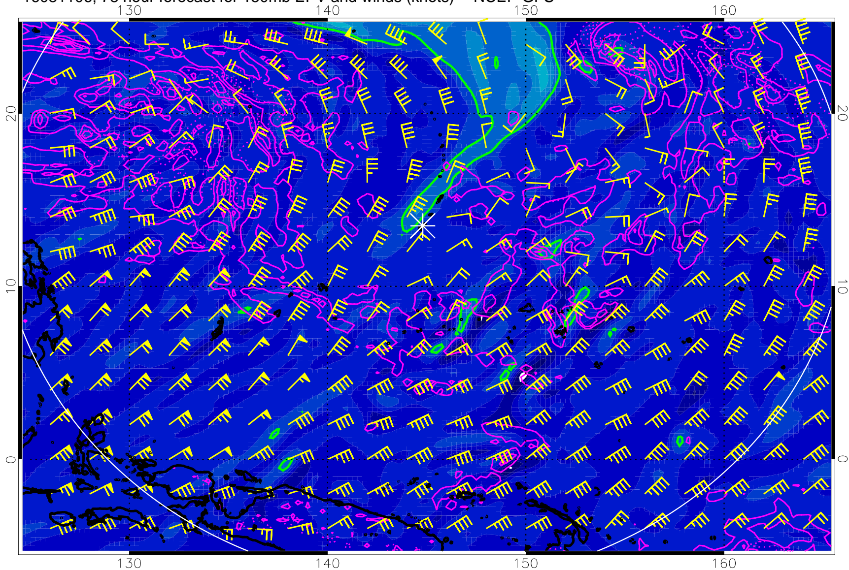
16081106, 78 hour forecast for 150mb EPV and winds (knots) -- NCEP GFS
