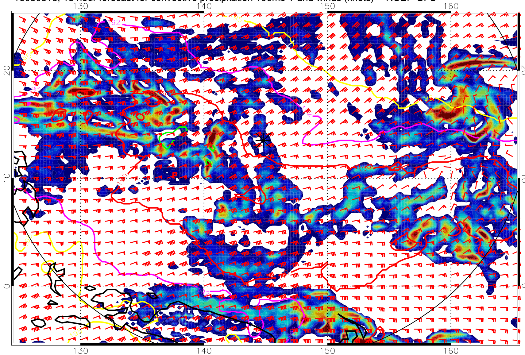
16080818, 18 hour forecast for convective precipitation 100mb T and winds (knots) -- NCEP GFS
