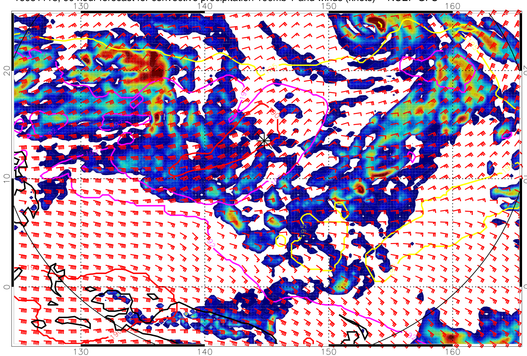
16081118, 90 hour forecast for convective precipitation 100mb T and winds (knots) -- NCEP GFS
