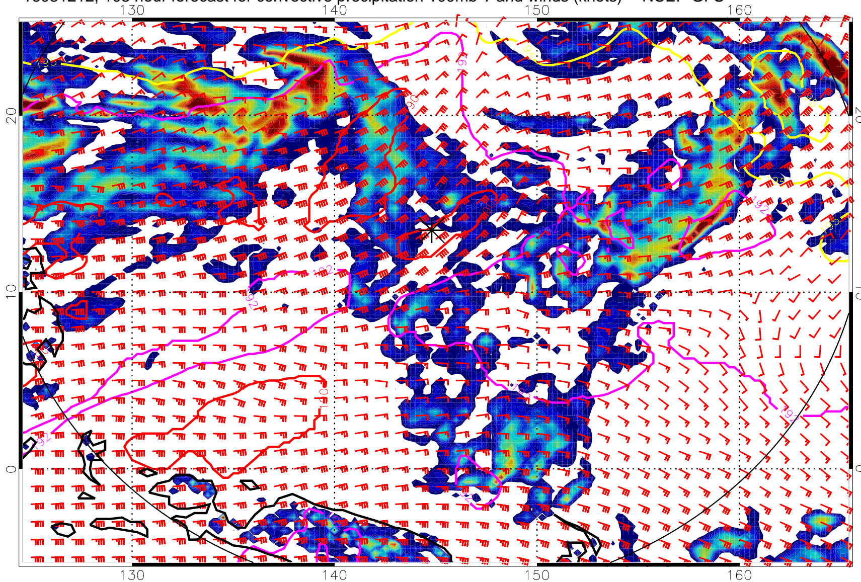
16081212, 108 hour forecast for convective precipitation 100mb T and winds (knots) -- NCEP GFS
