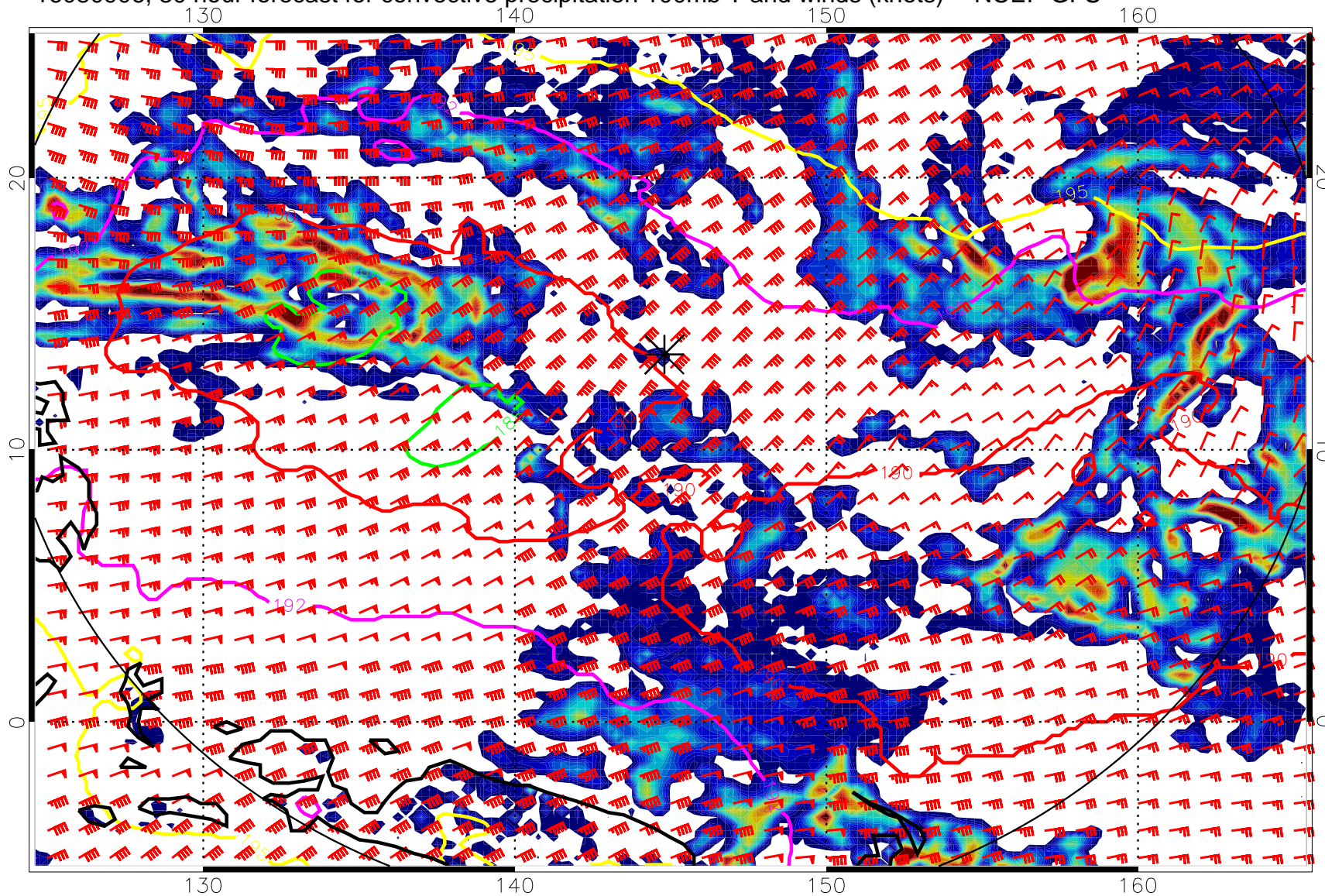
16080906, 30 hour forecast for convective precipitation 100mb T and winds (knots) -- NCEP GFS
