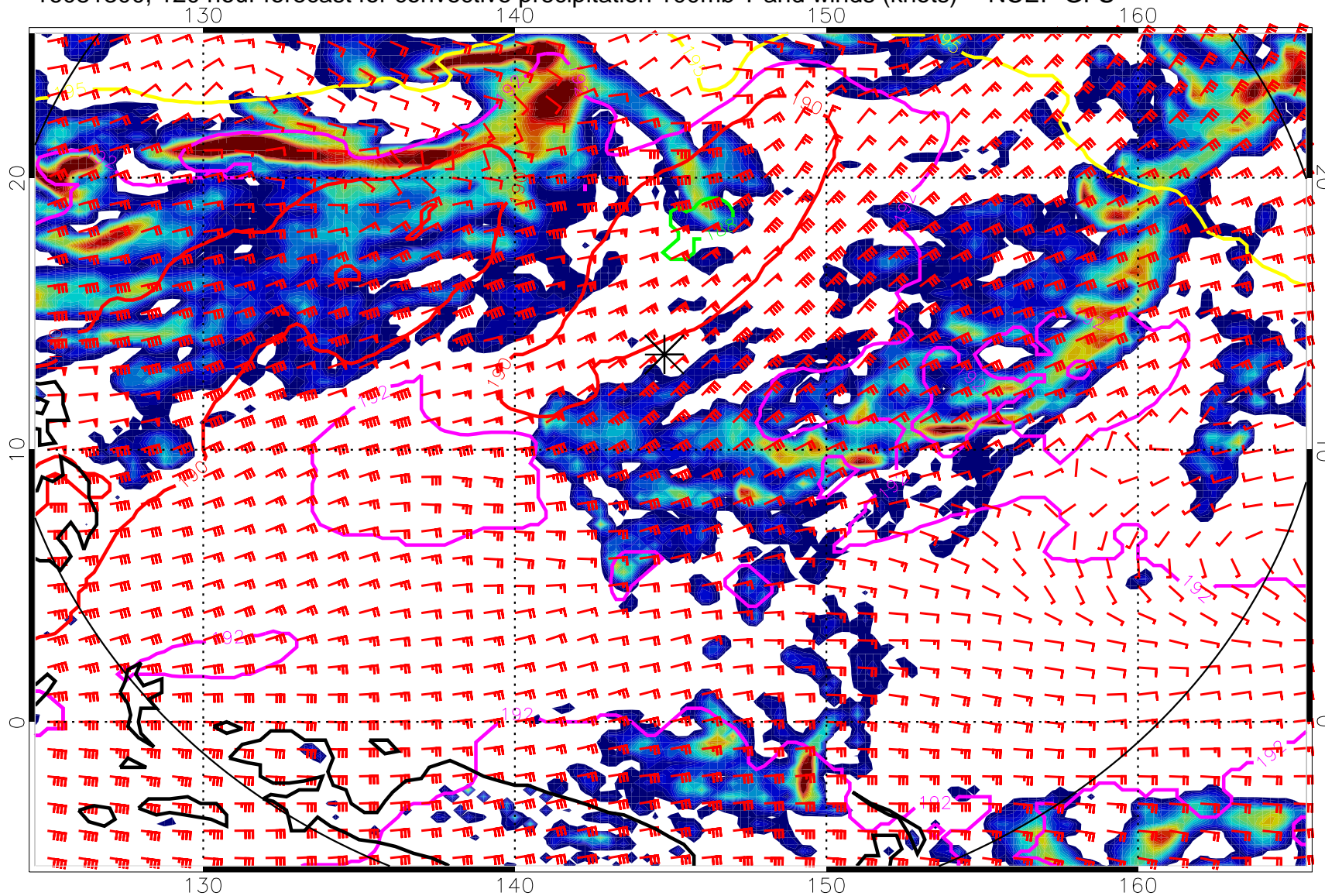
16081300, 120 hour forecast for convective precipitation 100mb T and winds (knots) -- NCEP GFS
