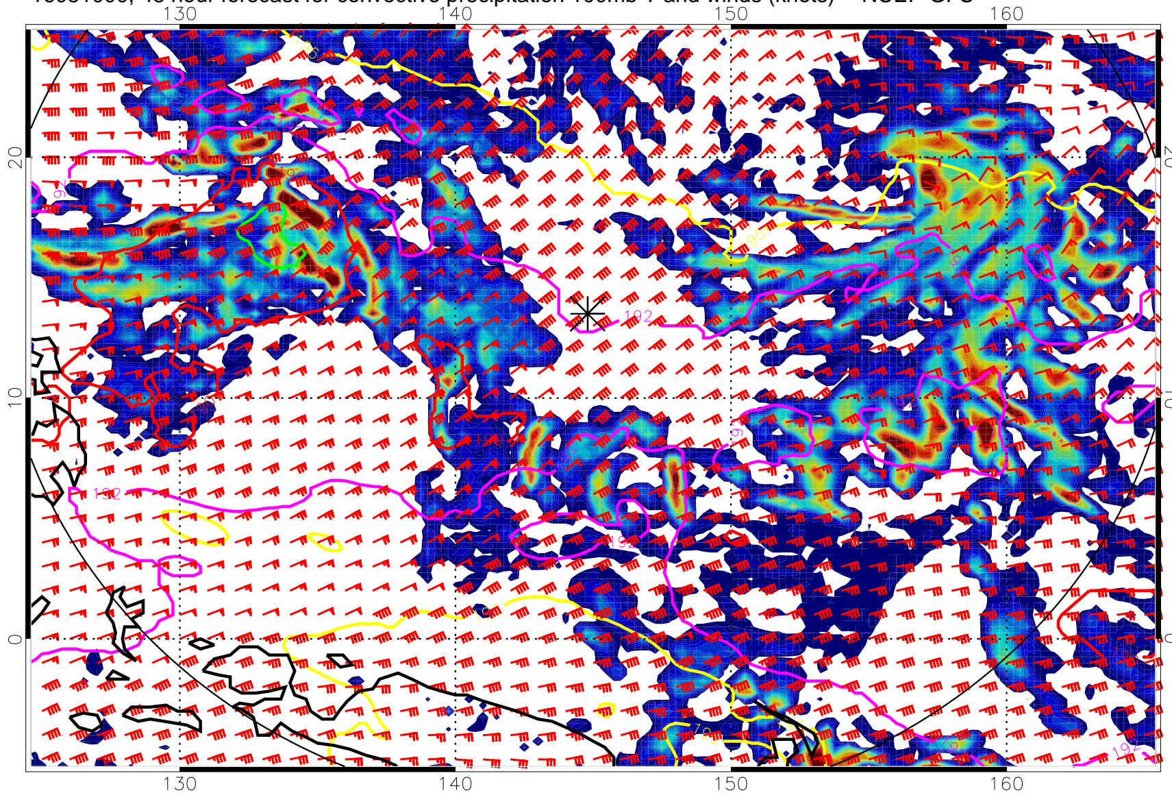
16081000, 48 hour forecast for convective precipitation 100mb T and winds (knots) -- NCEP GFS
