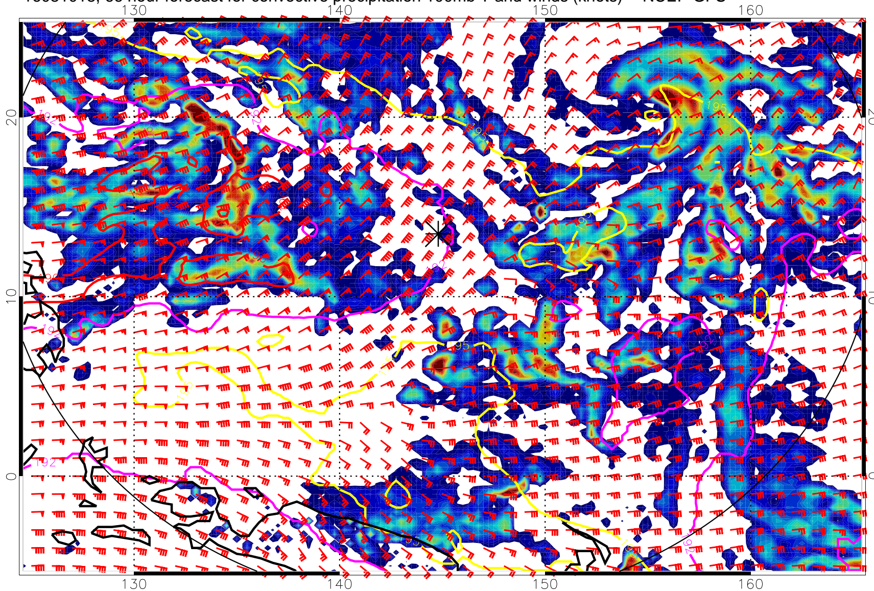
16081018, 66 hour forecast for convective precipitation 100mb T and winds (knots) -- NCEP GFS
