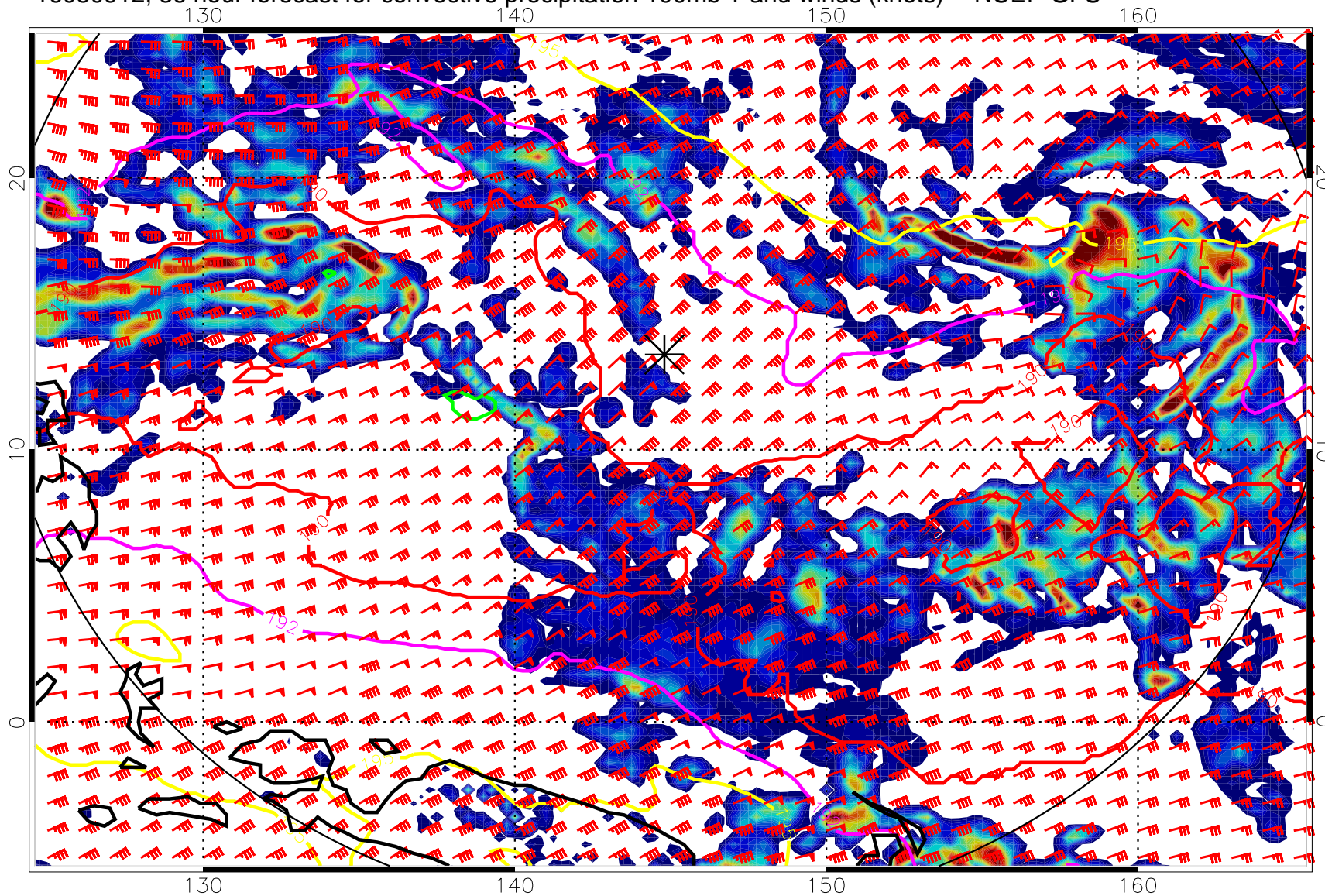
16080912, 36 hour forecast for convective precipitation 100mb T and winds (knots) -- NCEP GFS
