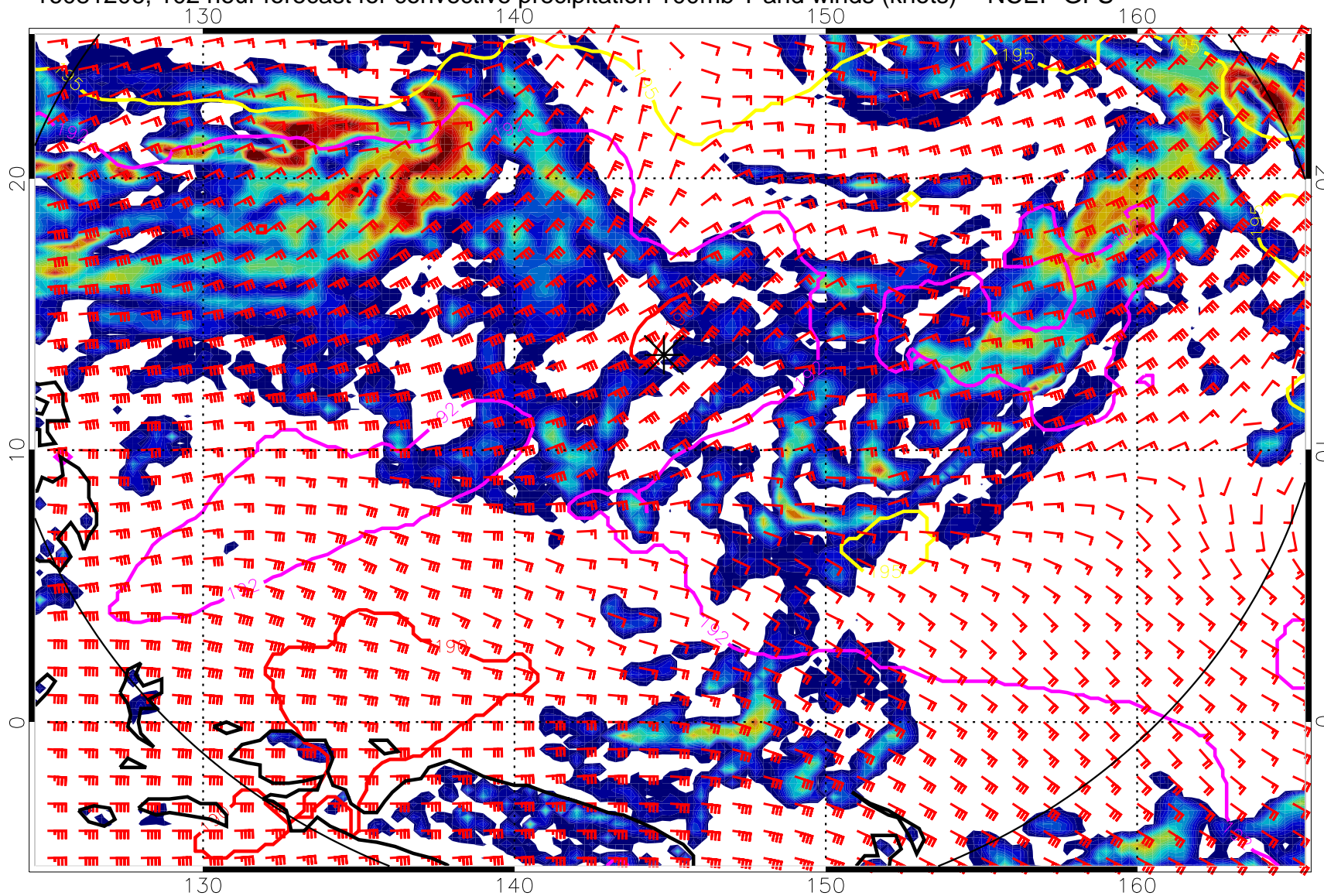
16081206, 102 hour forecast for convective precipitation 100mb T and winds (knots) -- NCEP GFS
