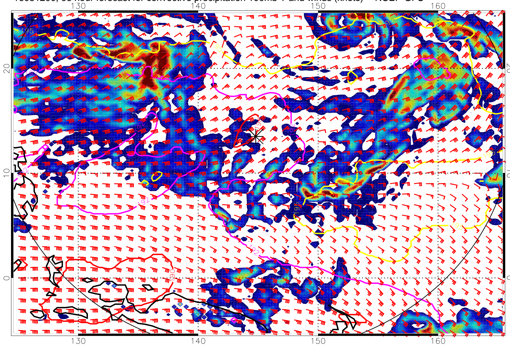
16081200, 96 hour forecast for convective precipitation 100mb T and winds (knots) -- NCEP GFS
