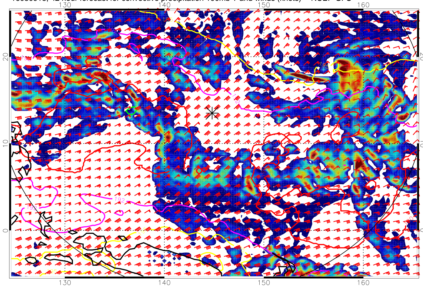
16080918, 42 hour forecast for convective precipitation 100mb T and winds (knots) -- NCEP GFS
