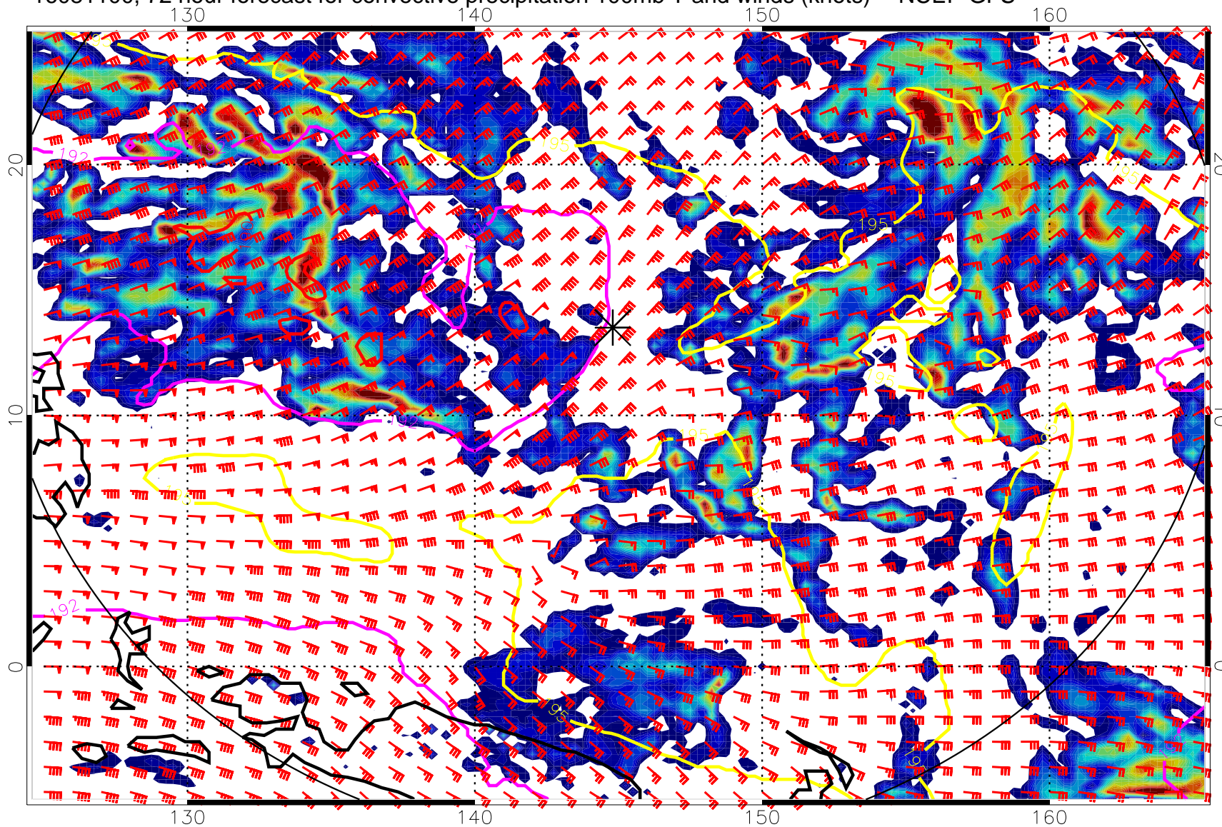
16081100, 72 hour forecast for convective precipitation 100mb T and winds (knots) -- NCEP GFS
