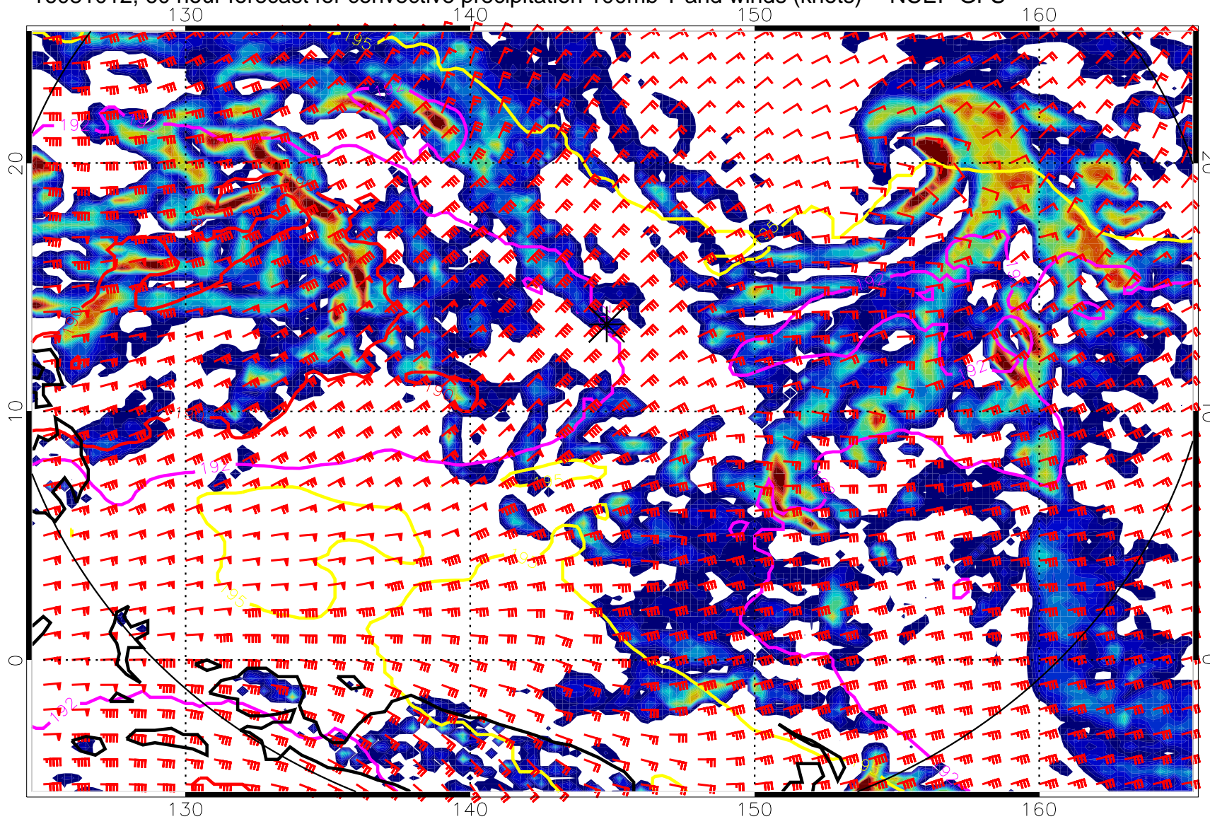
16081012, 60 hour forecast for convective precipitation 100mb T and winds (knots) -- NCEP GFS
