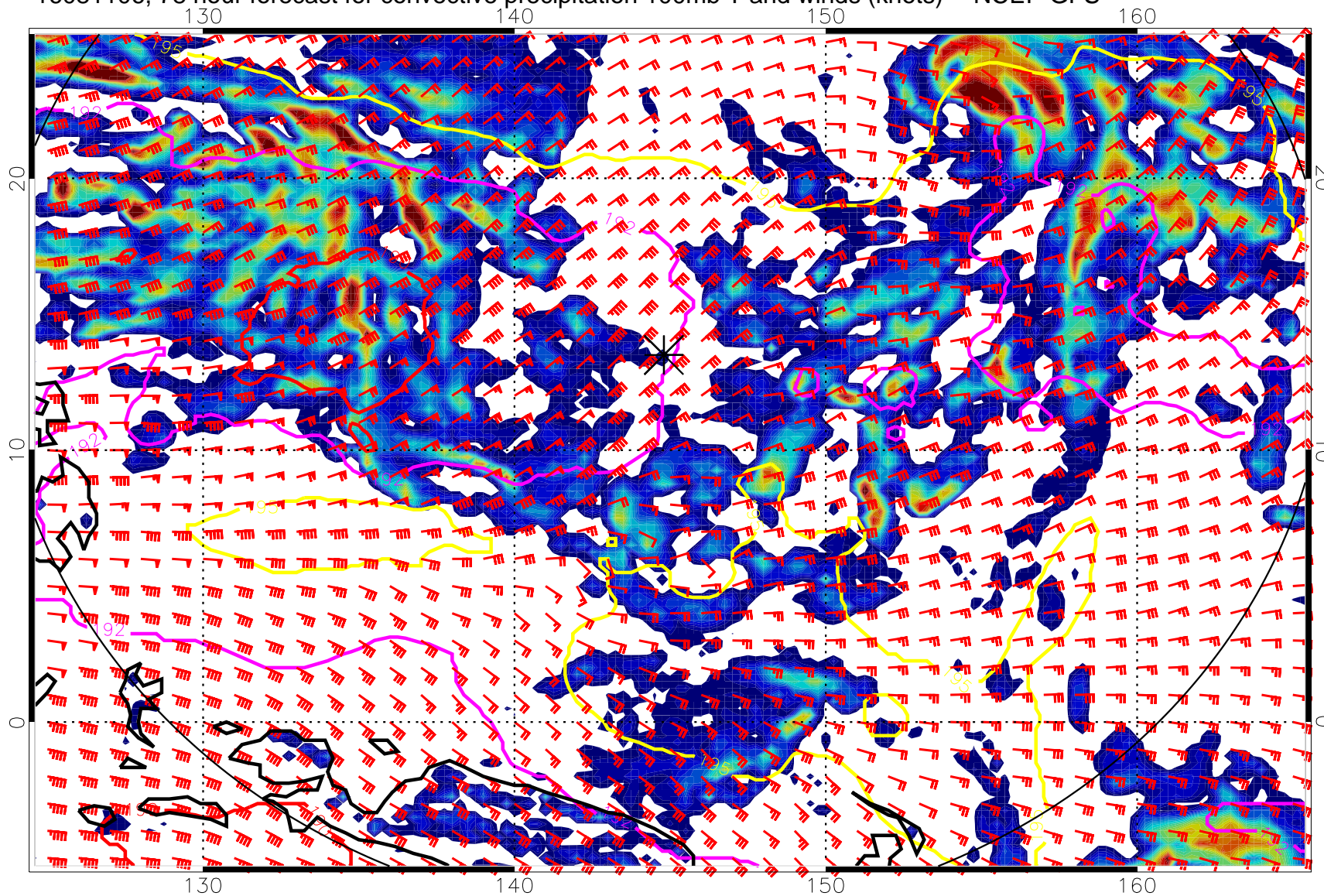
16081106, 78 hour forecast for convective precipitation 100mb T and winds (knots) -- NCEP GFS
