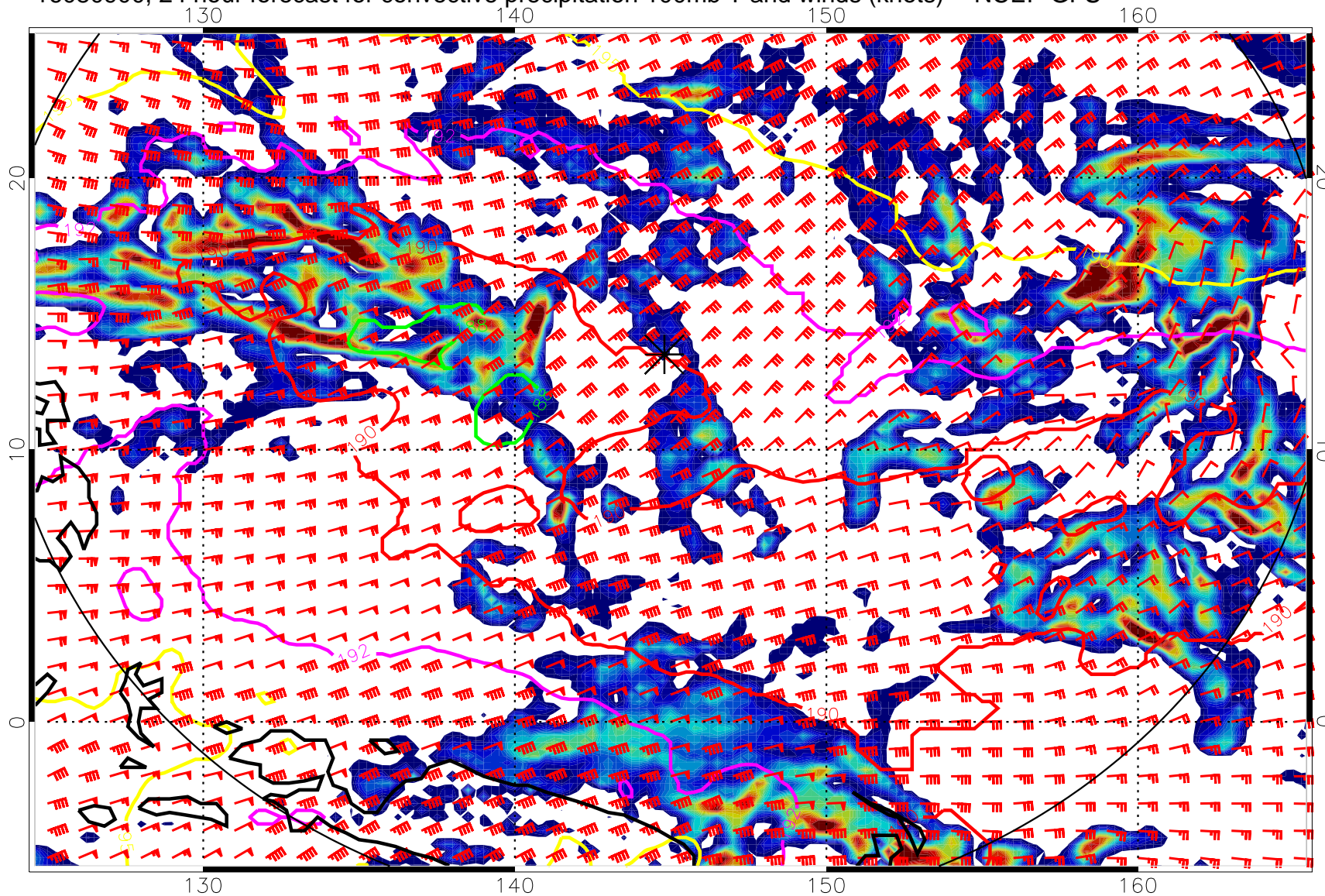
16080900, 24 hour forecast for convective precipitation 100mb T and winds (knots) -- NCEP GFS
