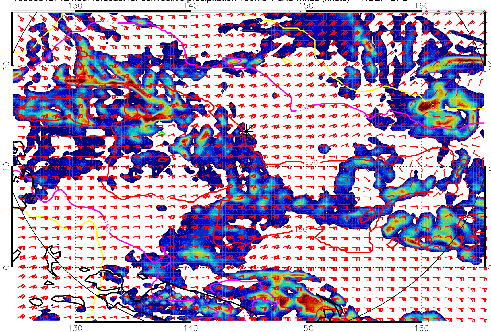
16080812, 12 hour forecast for convective precipitation 100mb T and winds (knots) -- NCEP GFS
