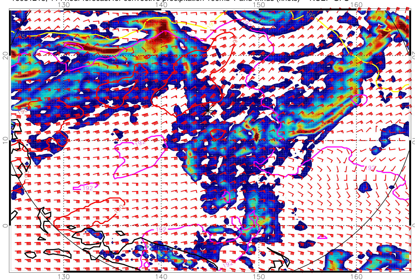
16081218, 114 hour forecast for convective precipitation 100mb T and winds (knots) -- NCEP GFS
