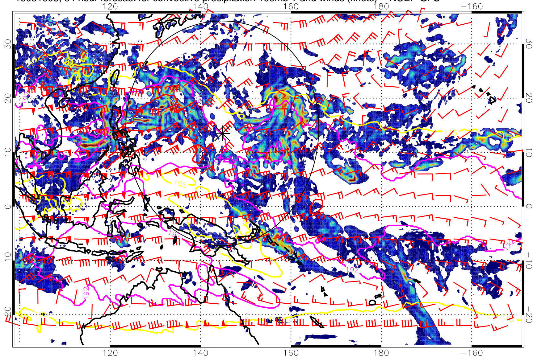
16081006, 54 hour forecast for convective precipitation 100mb T and winds (knots) -- NCEP GFS
