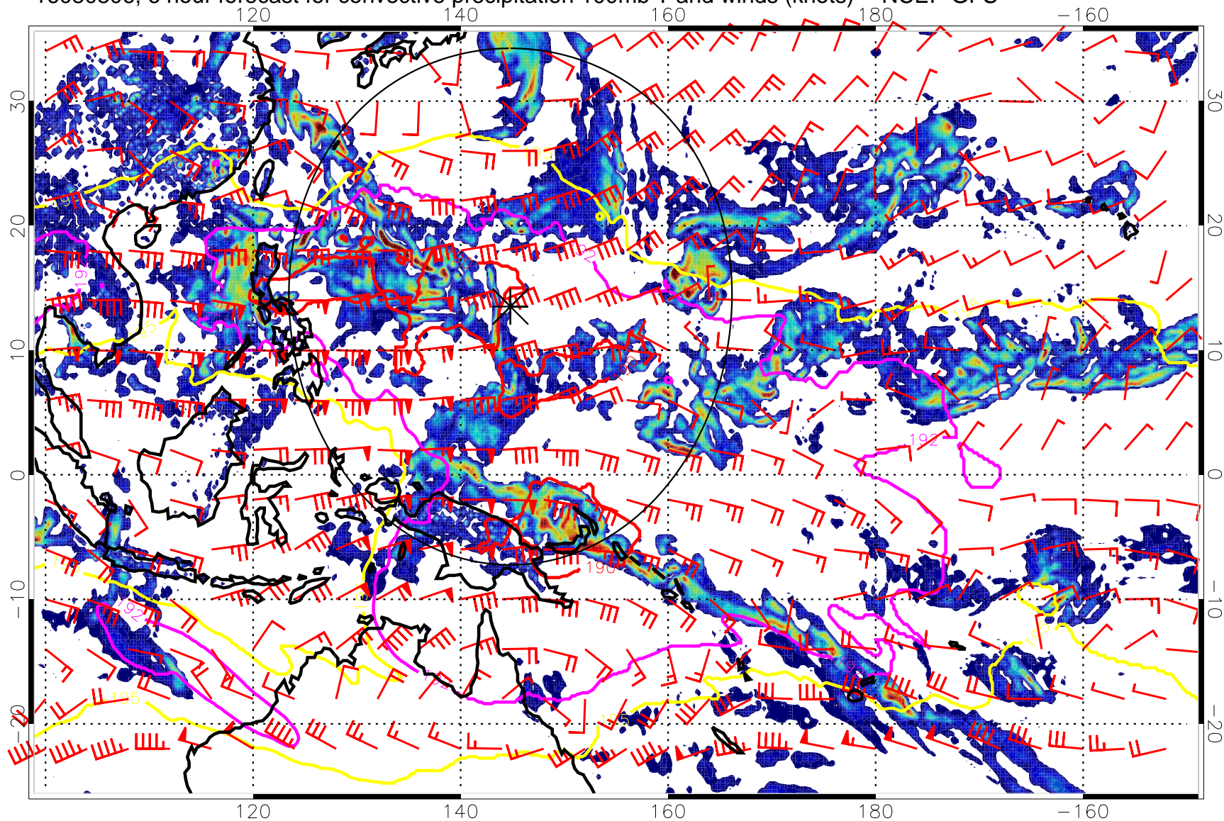
16080806, 6 hour forecast for convective precipitation 100mb T and winds (knots) -- NCEP GFS
