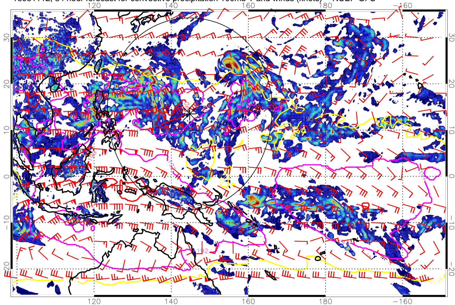
16081112, 84 hour forecast for convective precipitation 100mb T and winds (knots) -- NCEP GFS
