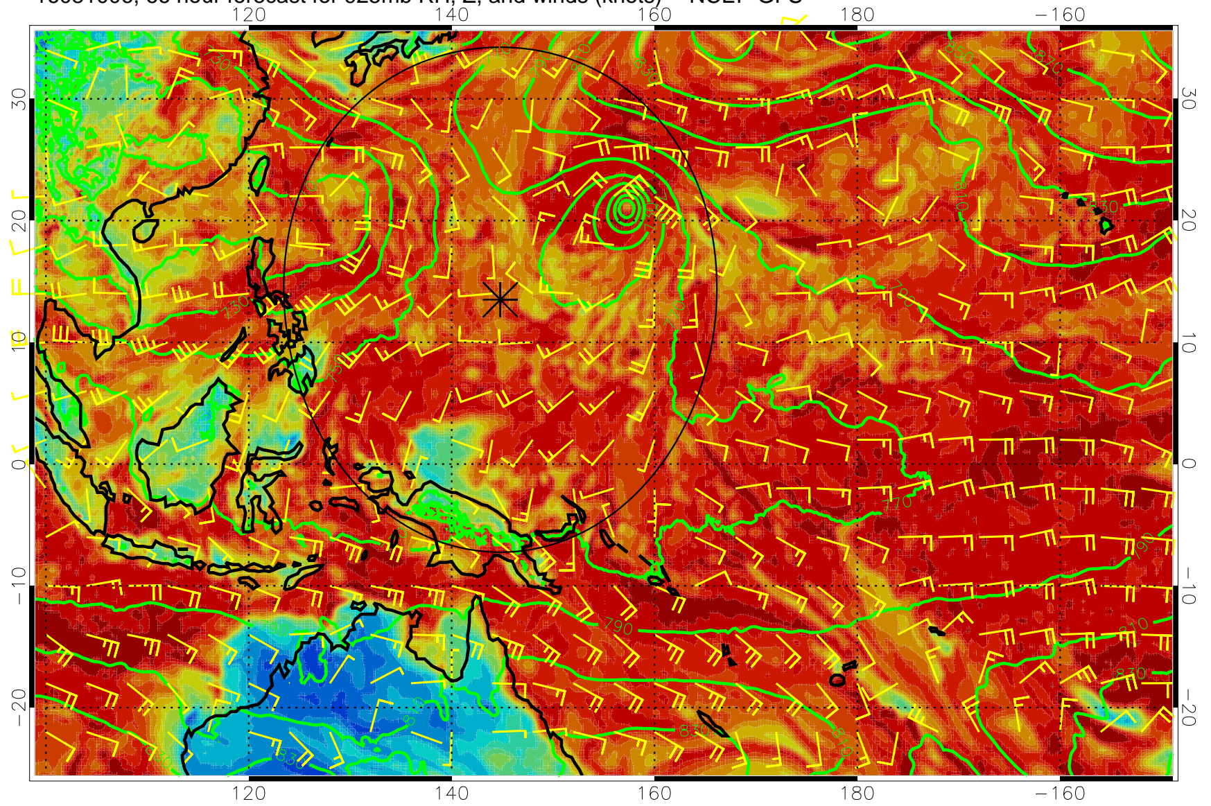
16081006, 66 hour forecast for 925mb RH, Z, and winds (knots) -- NCEP GFS
