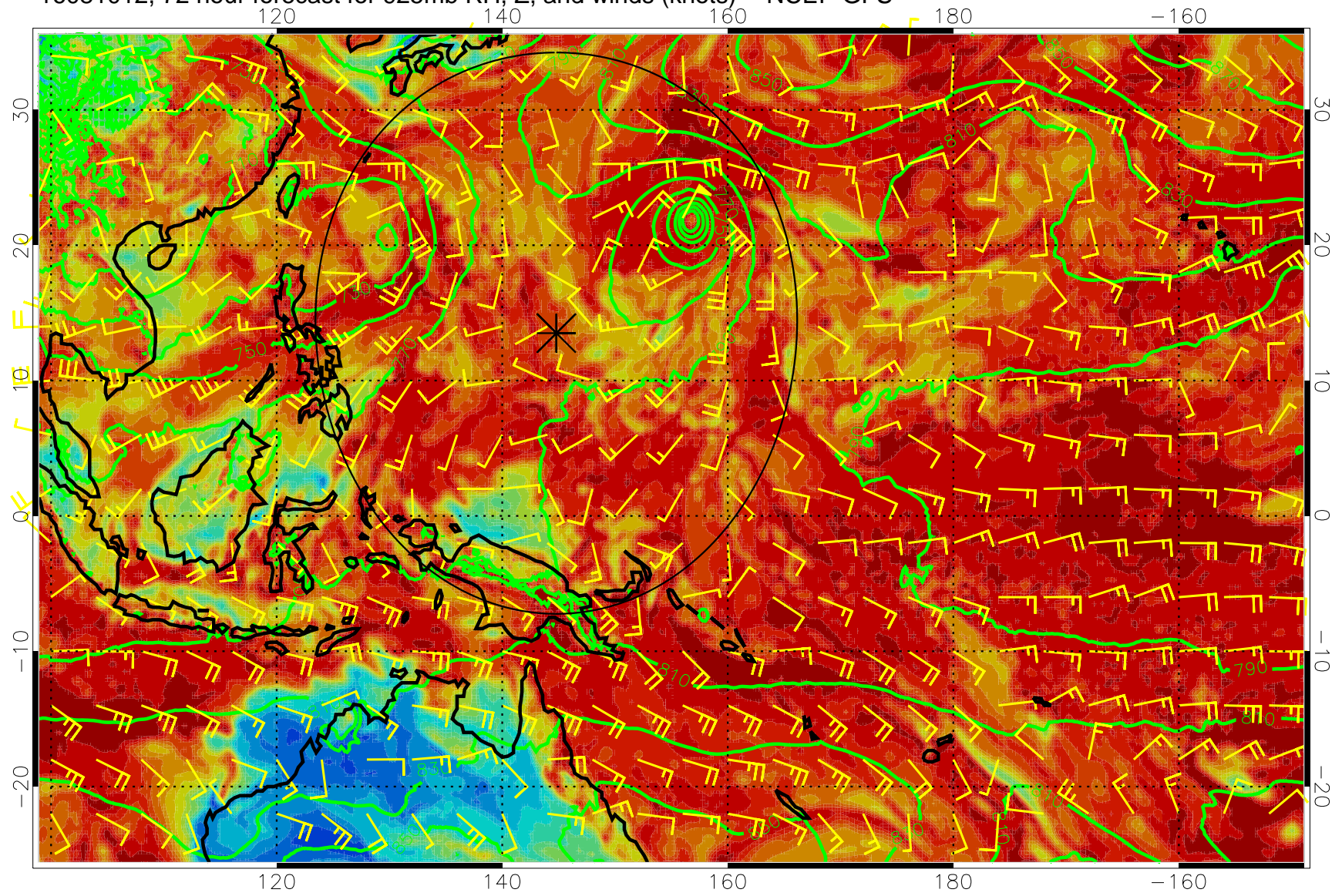
16081012, 72 hour forecast for 925mb RH, Z, and winds (knots) -- NCEP GFS
