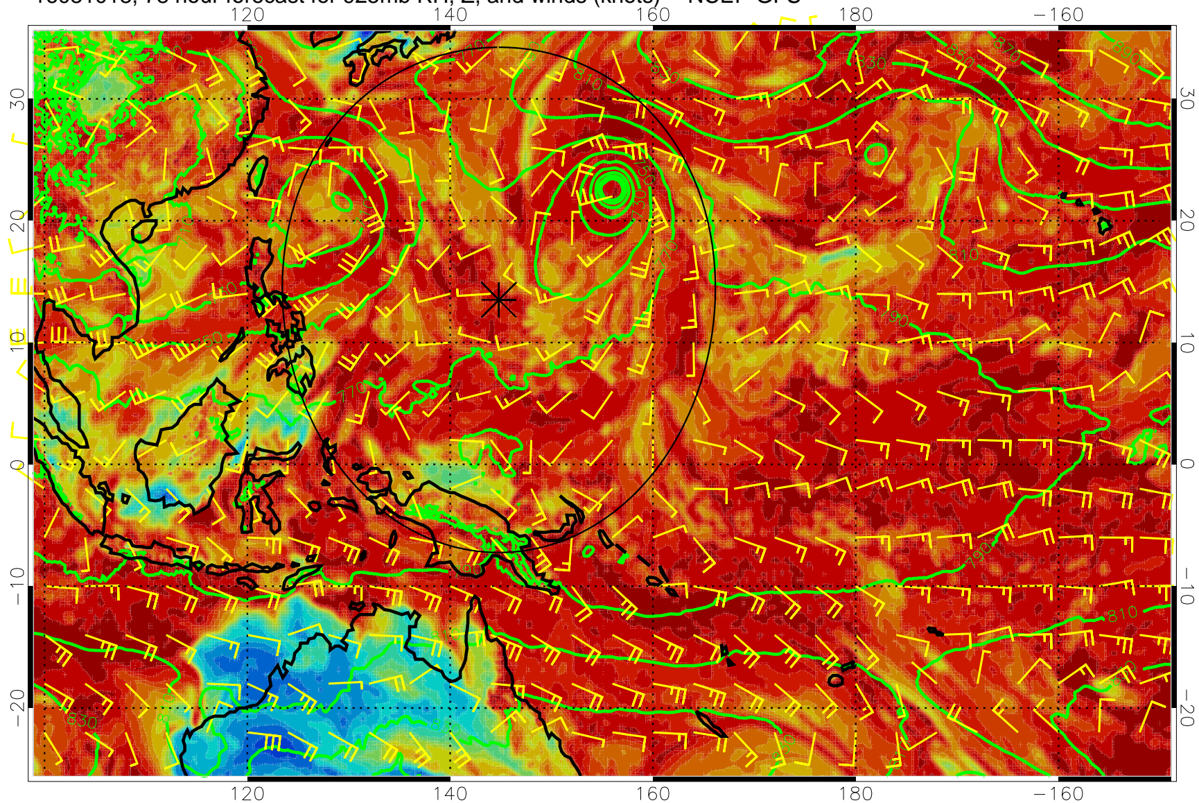
16081018, 78 hour forecast for 925mb RH, Z, and winds (knots) -- NCEP GFS
