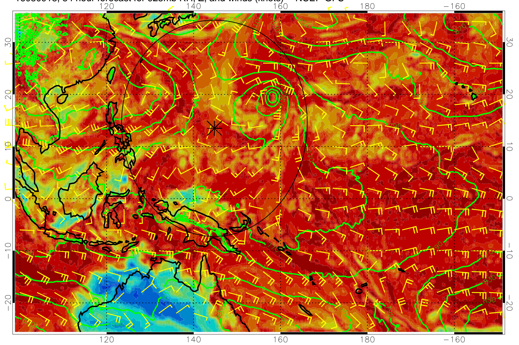
16080918, 54 hour forecast for 925mb RH, Z, and winds (knots) -- NCEP GFS
