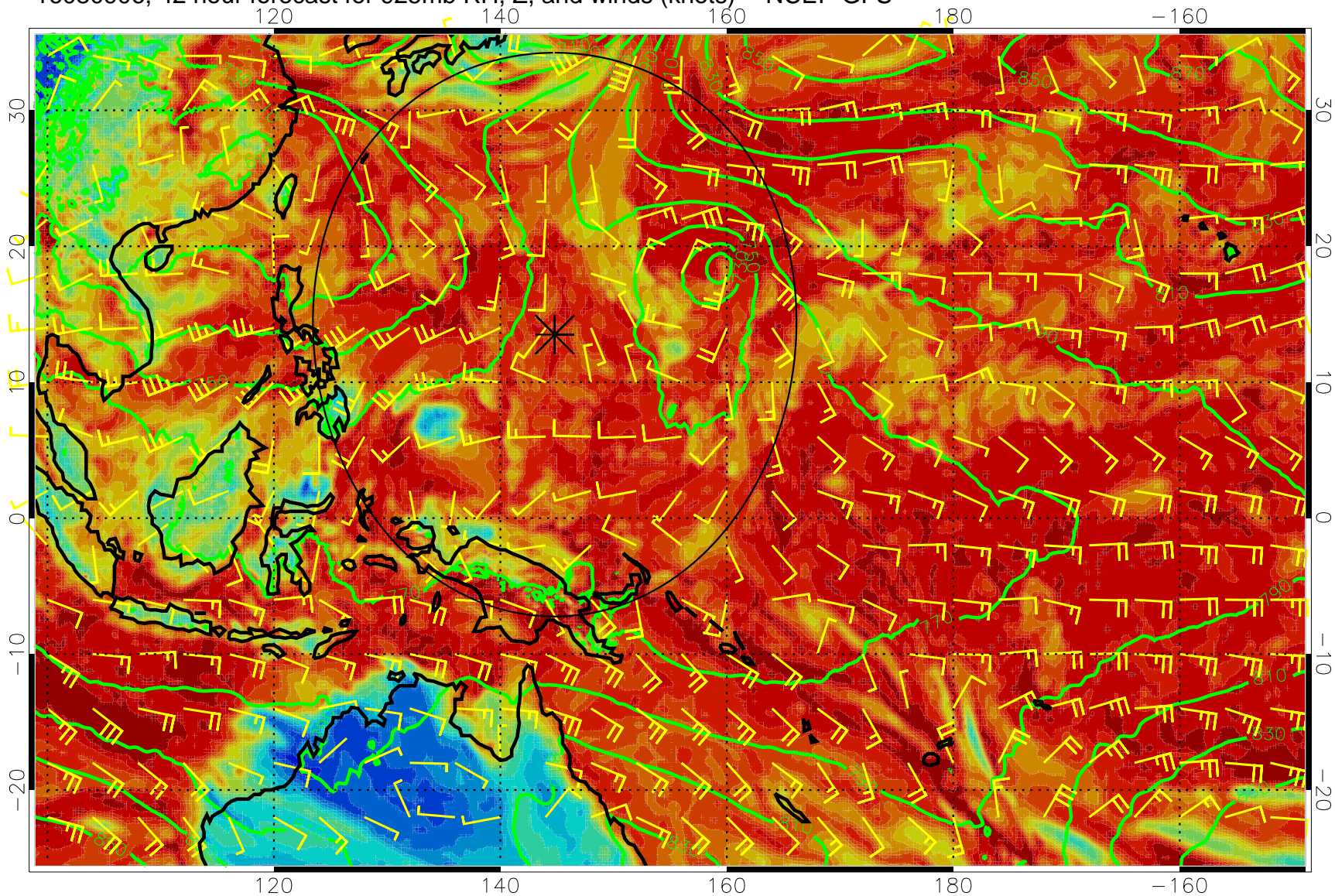
16080906, 42 hour forecast for 925mb RH, Z, and winds (knots) -- NCEP GFS
