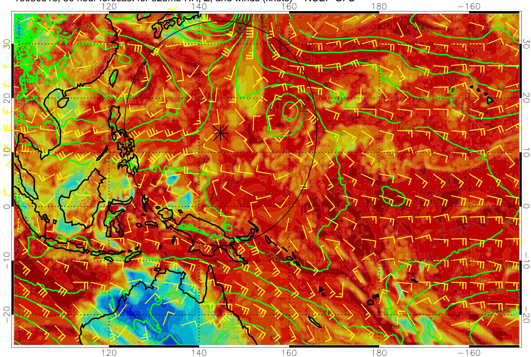
16080818, 30 hour forecast for 925mb RH, Z, and winds (knots) -- NCEP GFS
