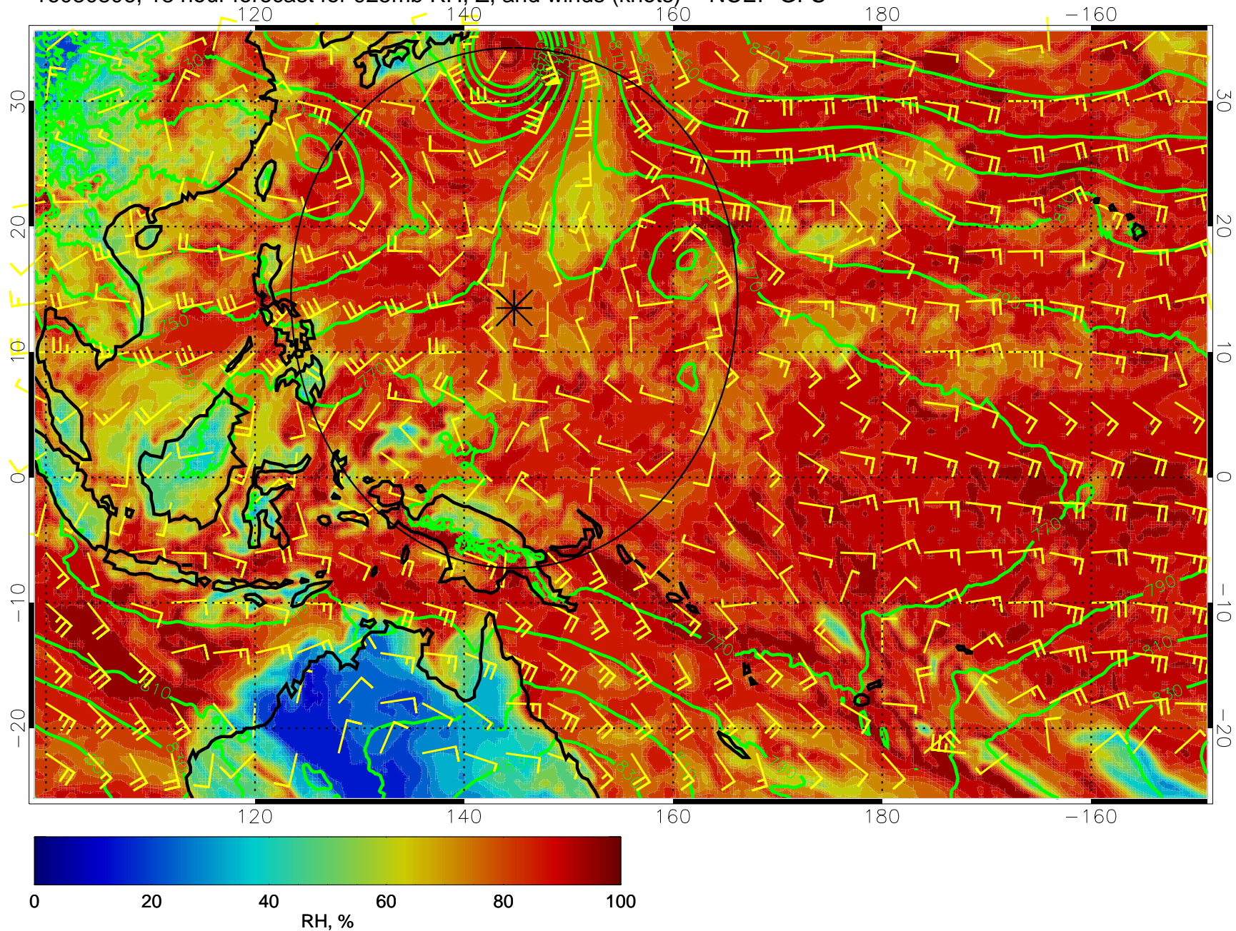
16080806, 18 hour forecast for 925mb RH, Z, and winds (knots) -- NCEP GFS
