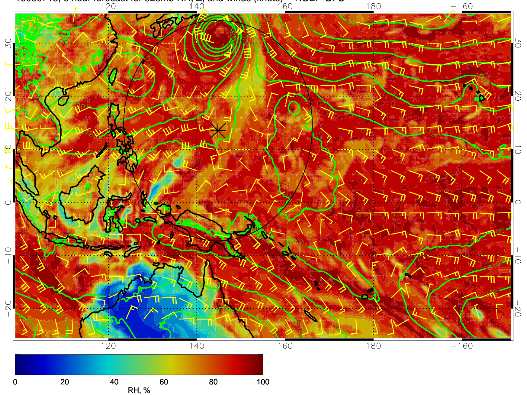
16080718, 6 hour forecast for 925mb RH, Z, and winds (knots) -- NCEP GFS
