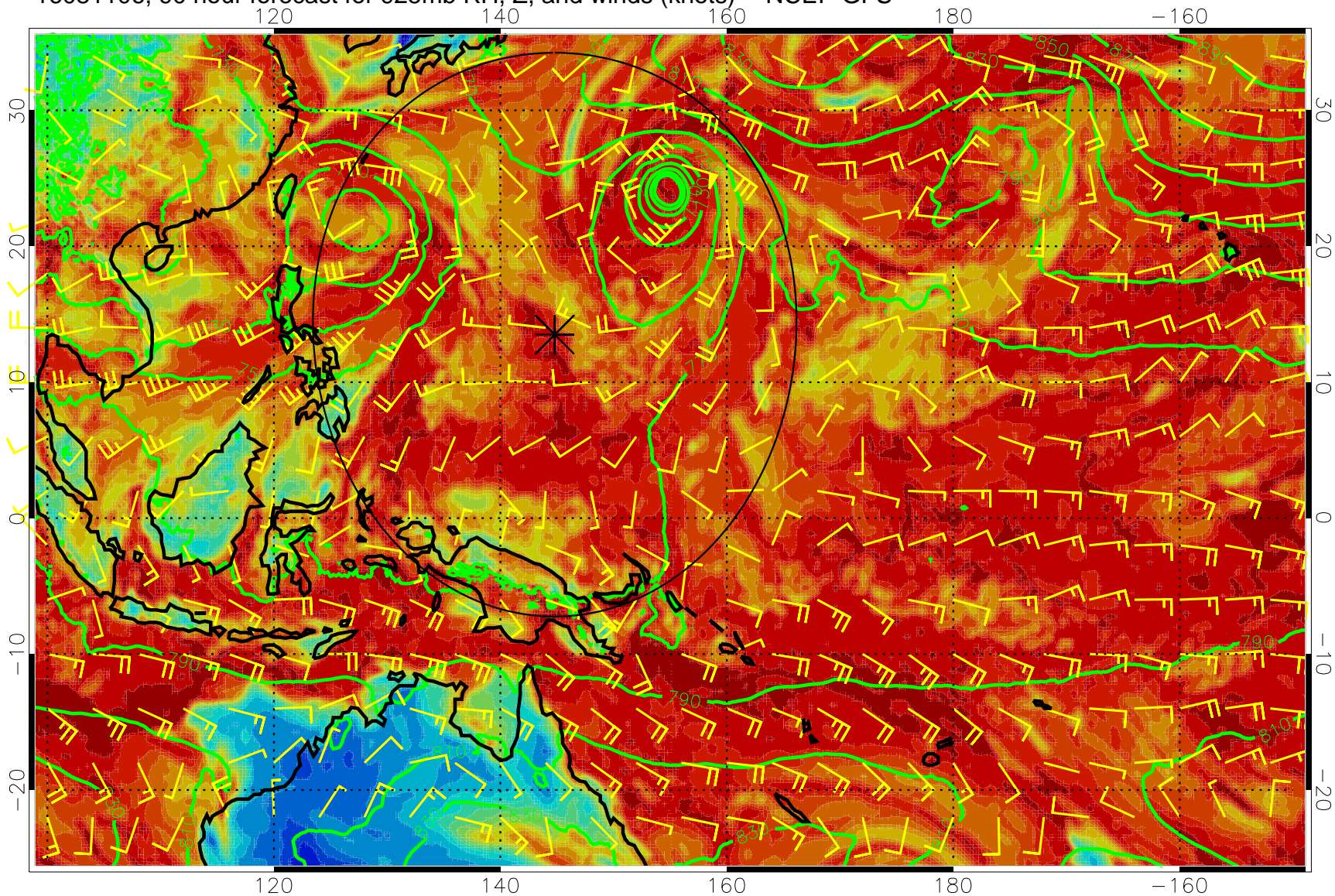
16081106, 90 hour forecast for 925mb RH, Z, and winds (knots) -- NCEP GFS
