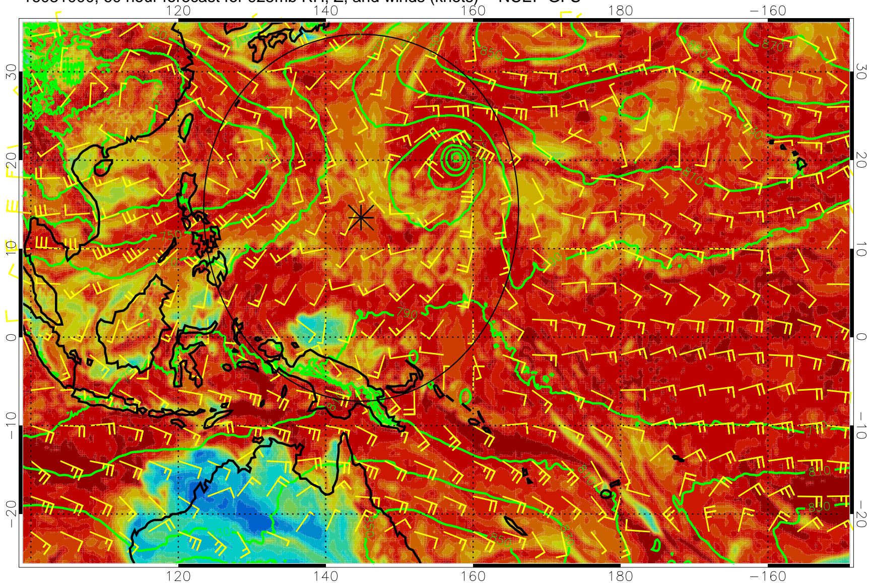
16081000, 60 hour forecast for 925mb RH, Z, and winds (knots) -- NCEP GFS
