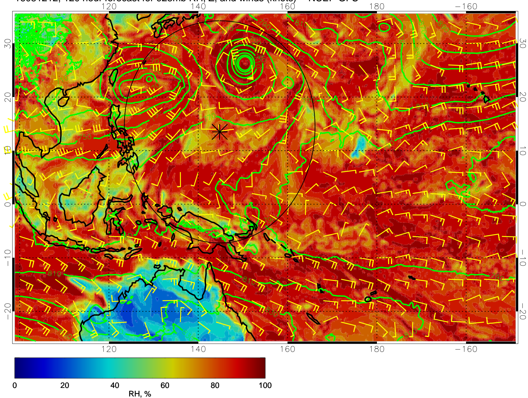
16081212, 120 hour forecast for 925mb RH, Z, and winds (knots) -- NCEP GFS
