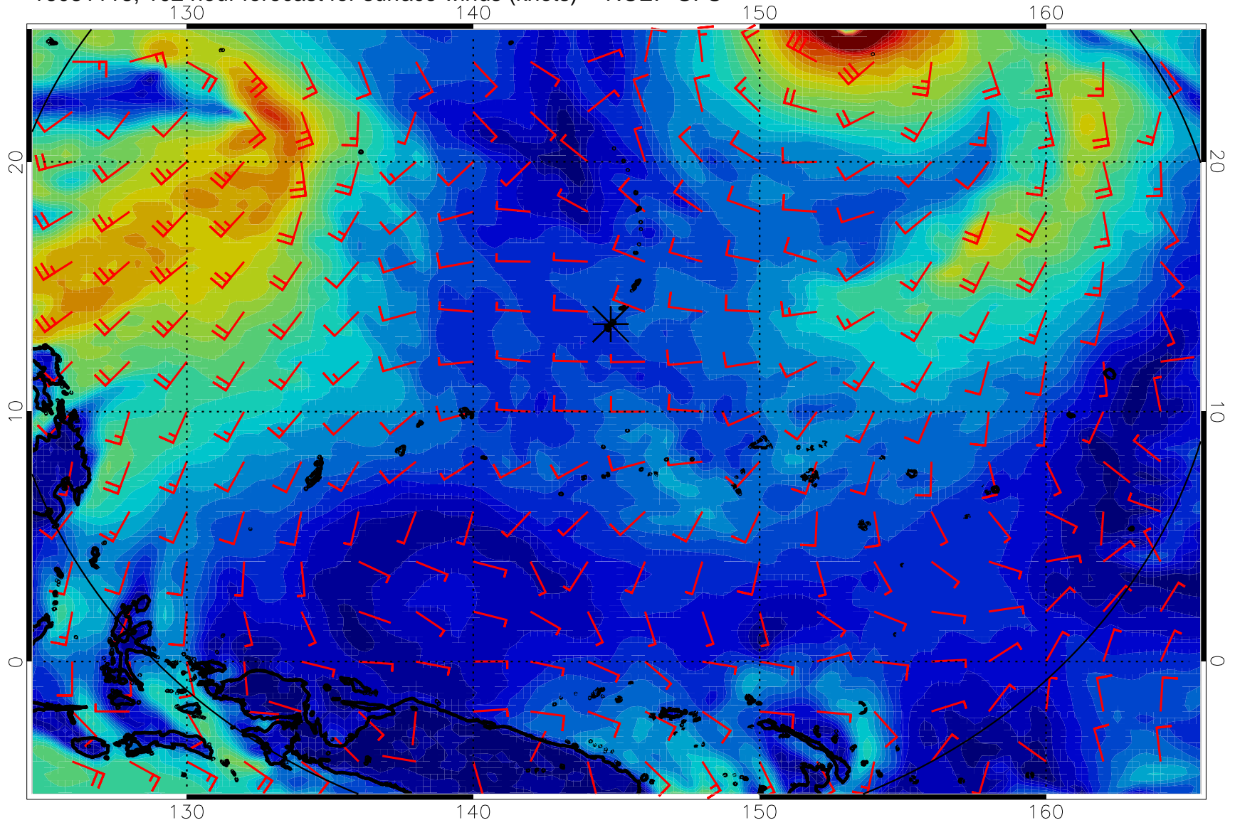
16081118, 102 hour forecast for surface winds (knots) -- NCEP GFS
