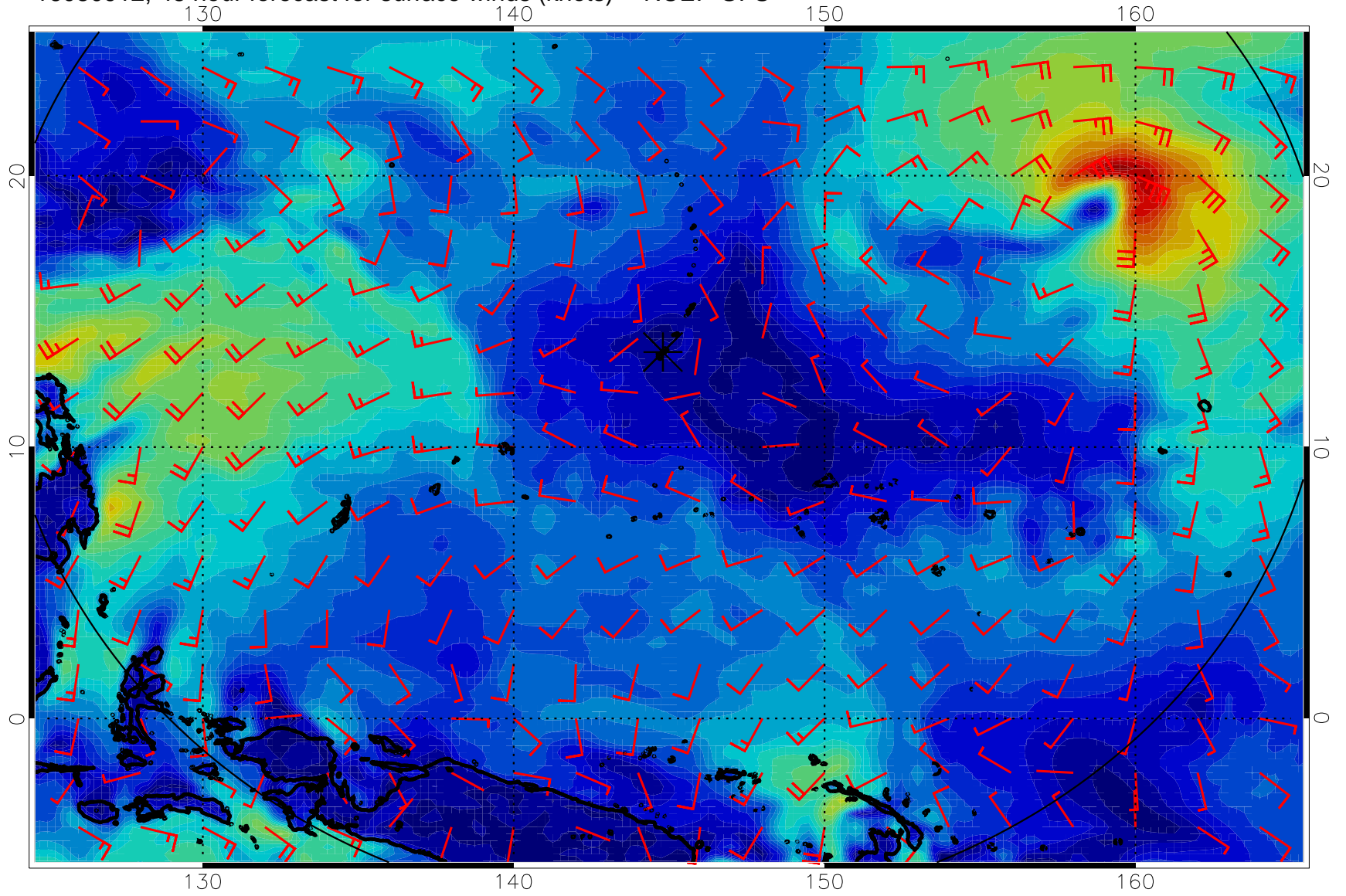
16080912, 48 hour forecast for surface winds (knots) -- NCEP GFS
