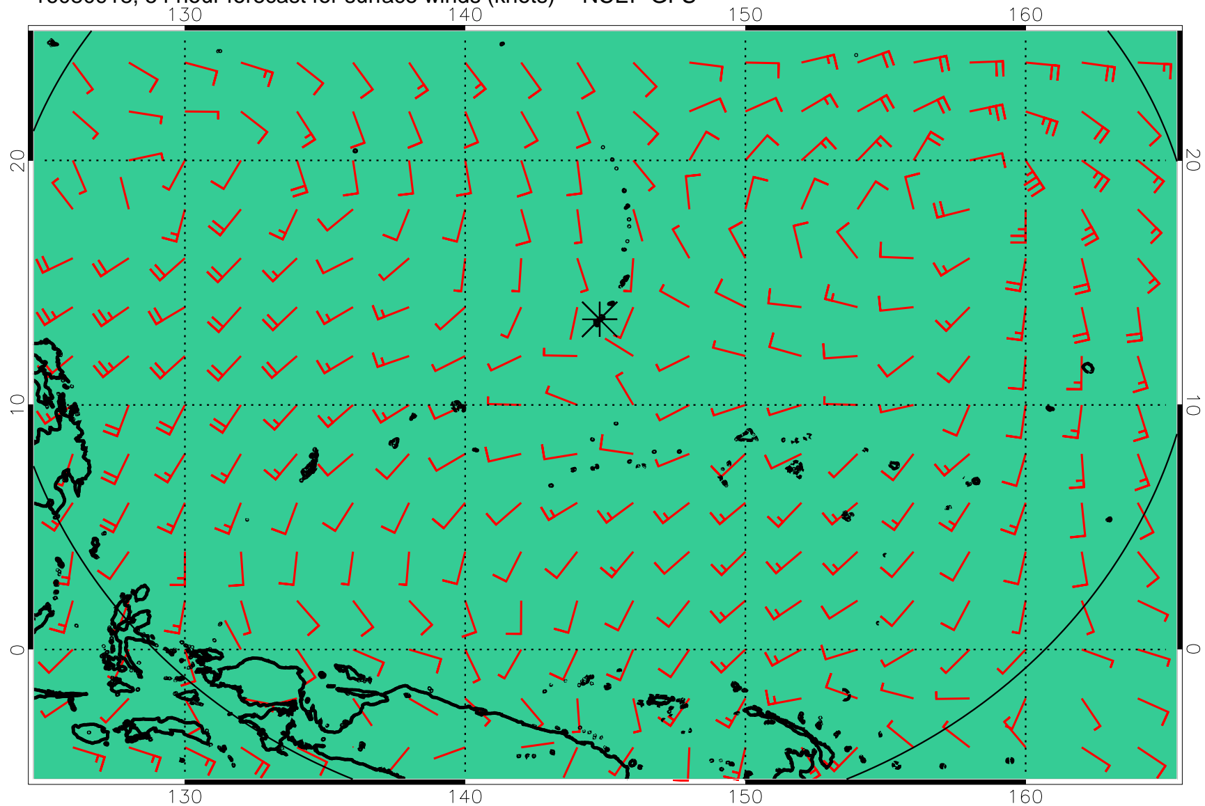
16080918, 54 hour forecast for surface winds (knots) -- NCEP GFS
