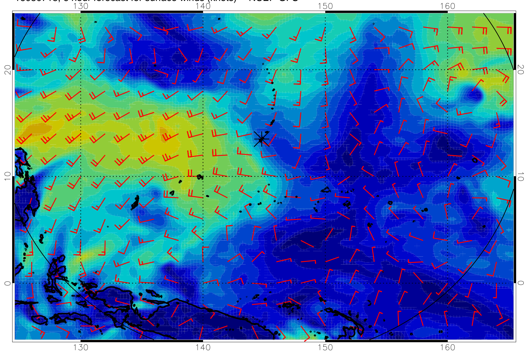
16080718, 6 hour forecast for surface winds (knots) -- NCEP GFS
