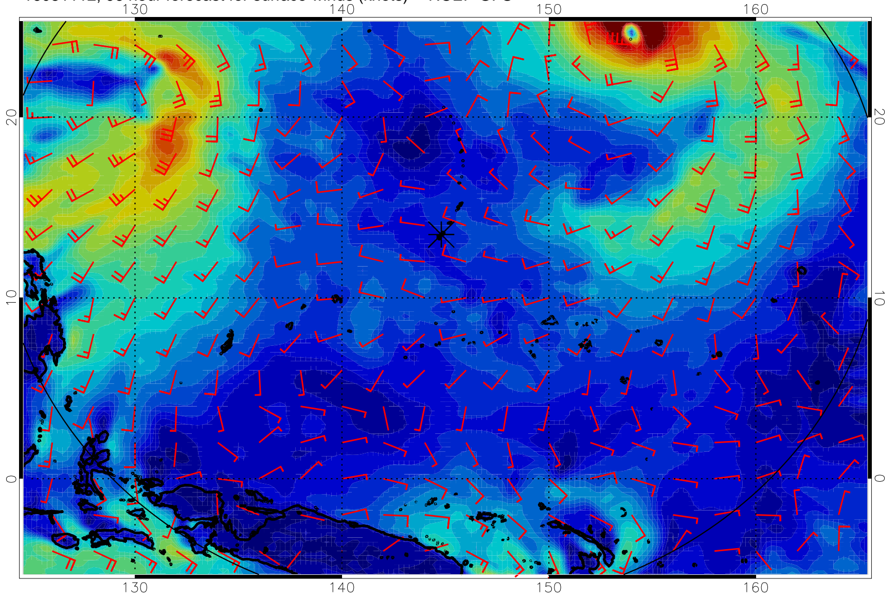
16081112, 96 hour forecast for surface winds (knots) -- NCEP GFS
