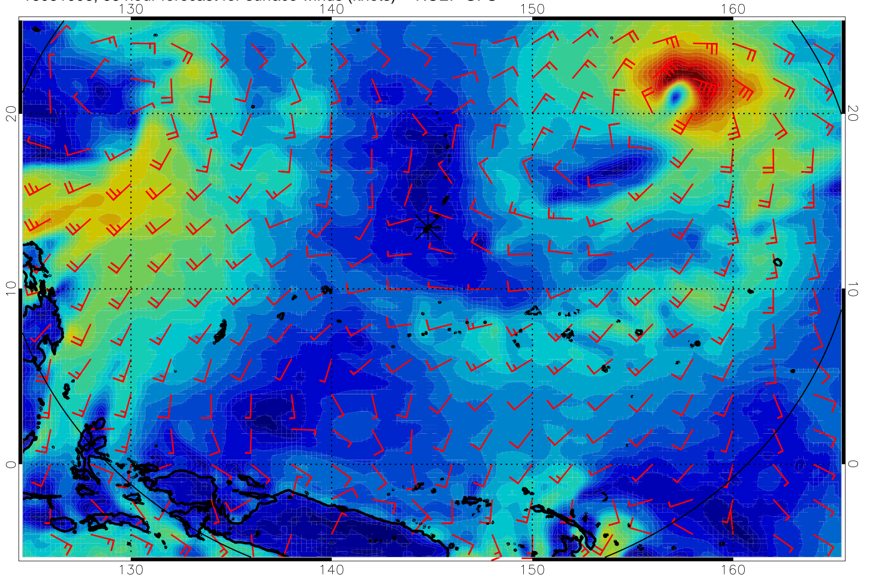
16081006, 66 hour forecast for surface winds (knots) -- NCEP GFS
