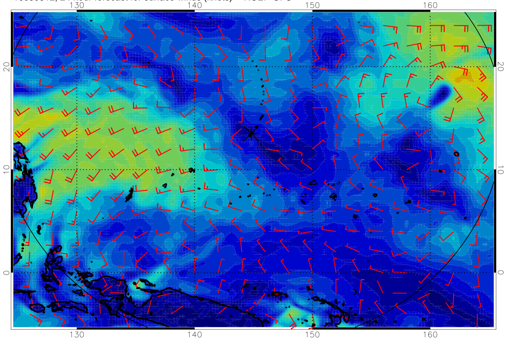
16080812, 24 hour forecast for surface winds (knots) -- NCEP GFS
