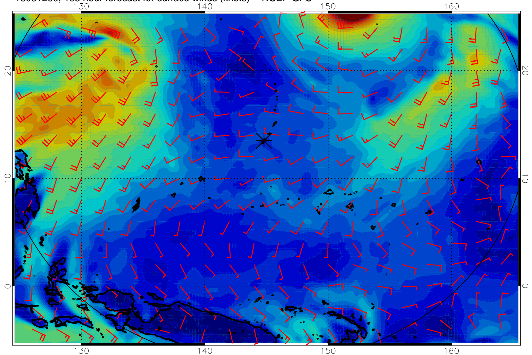
16081200, 108 hour forecast for surface winds (knots) -- NCEP GFS
