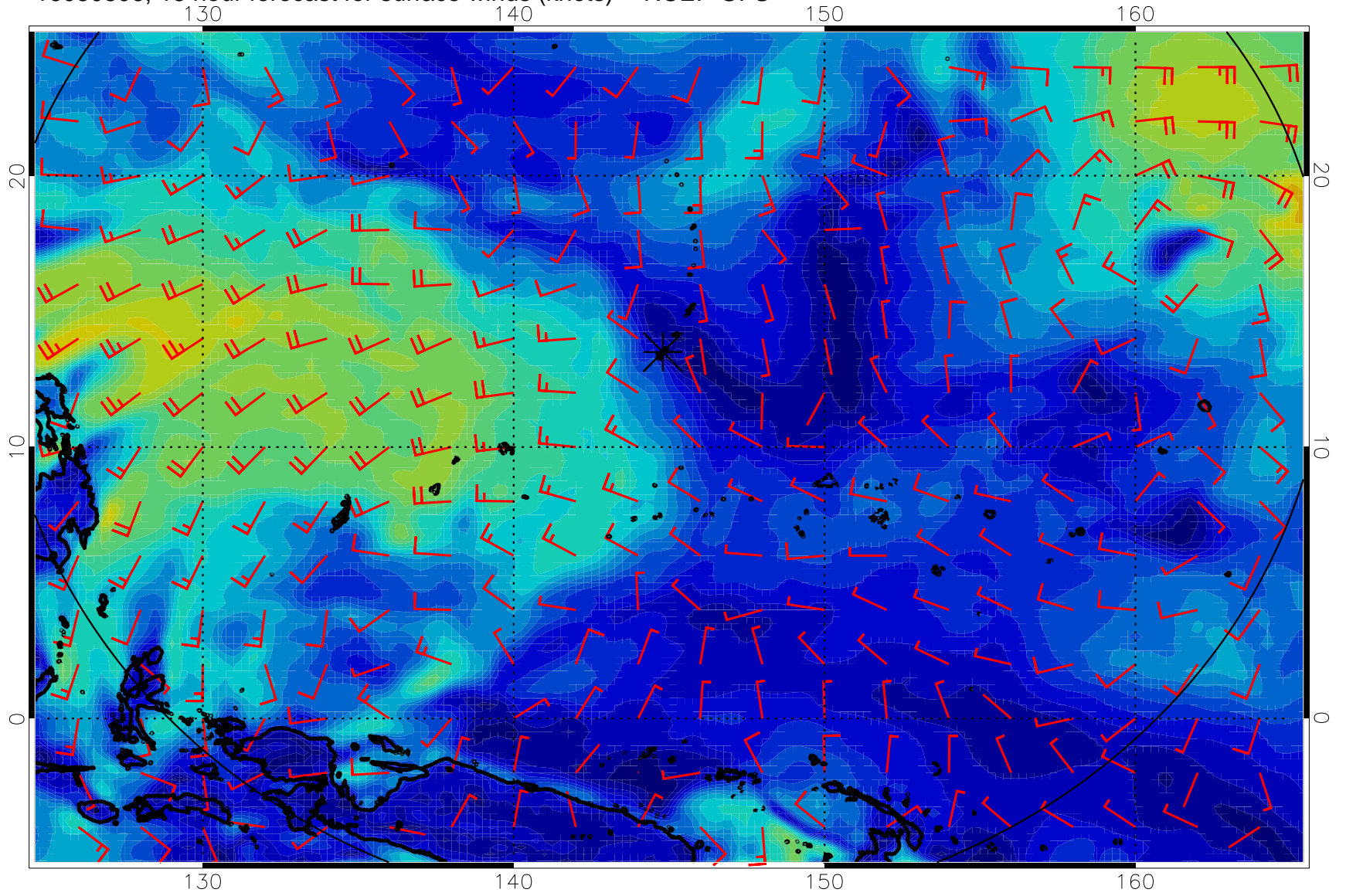
16080806, 18 hour forecast for surface winds (knots) -- NCEP GFS
