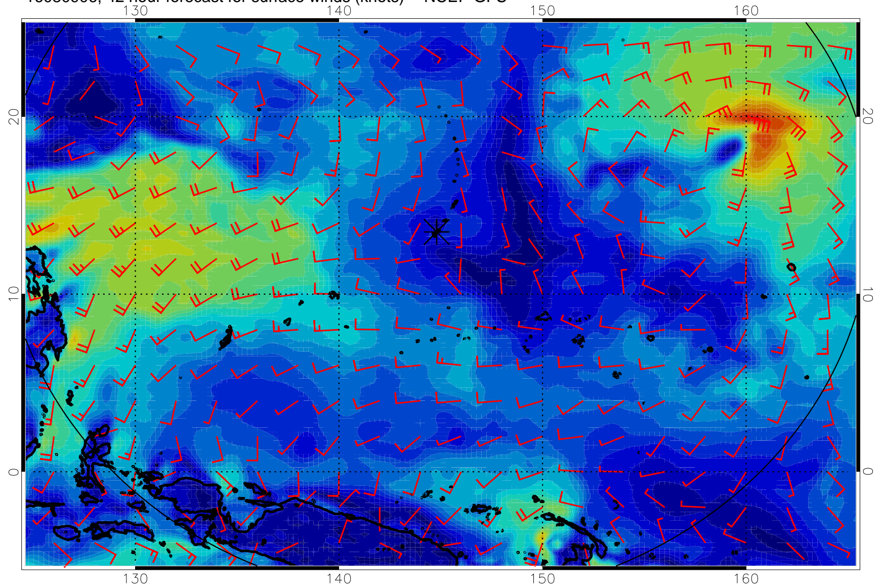
16080906, 42 hour forecast for surface winds (knots) -- NCEP GFS
