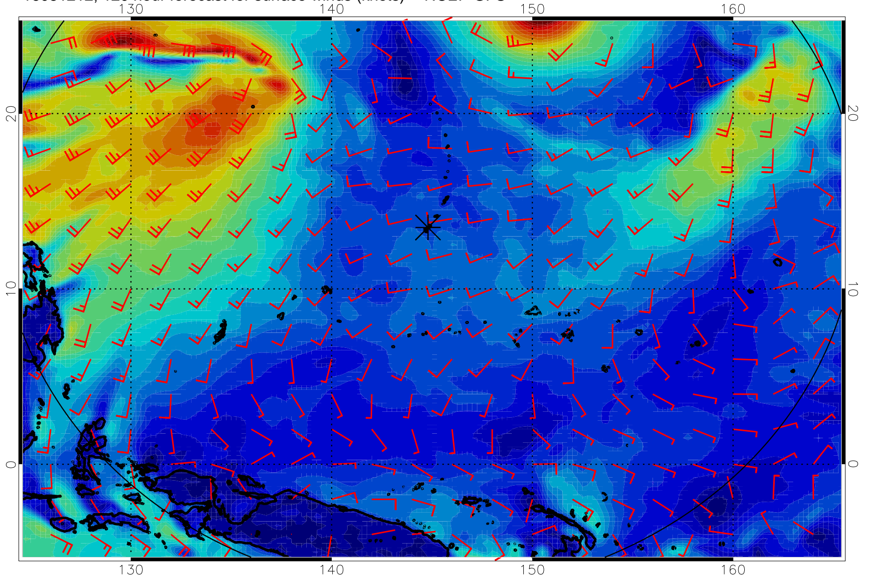
16081212, 120 hour forecast for surface winds (knots) -- NCEP GFS
