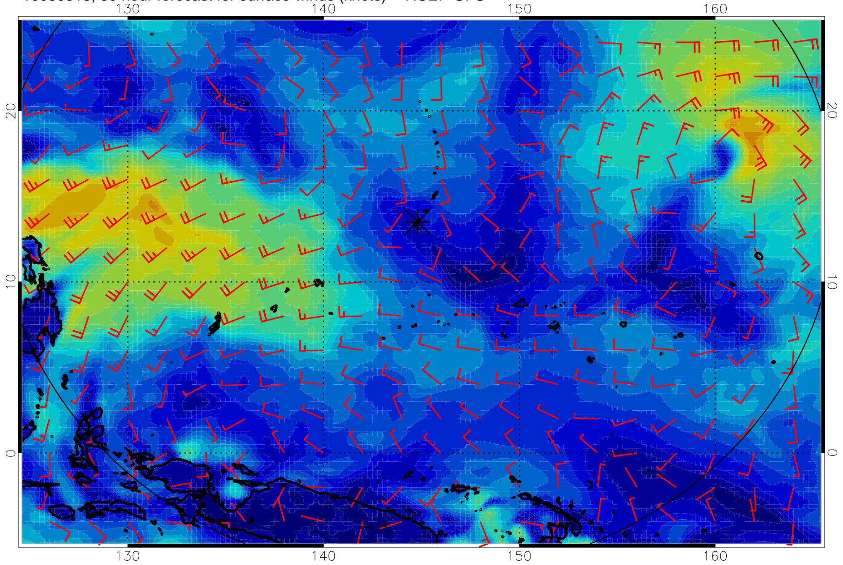
16080818, 30 hour forecast for surface winds (knots) -- NCEP GFS
