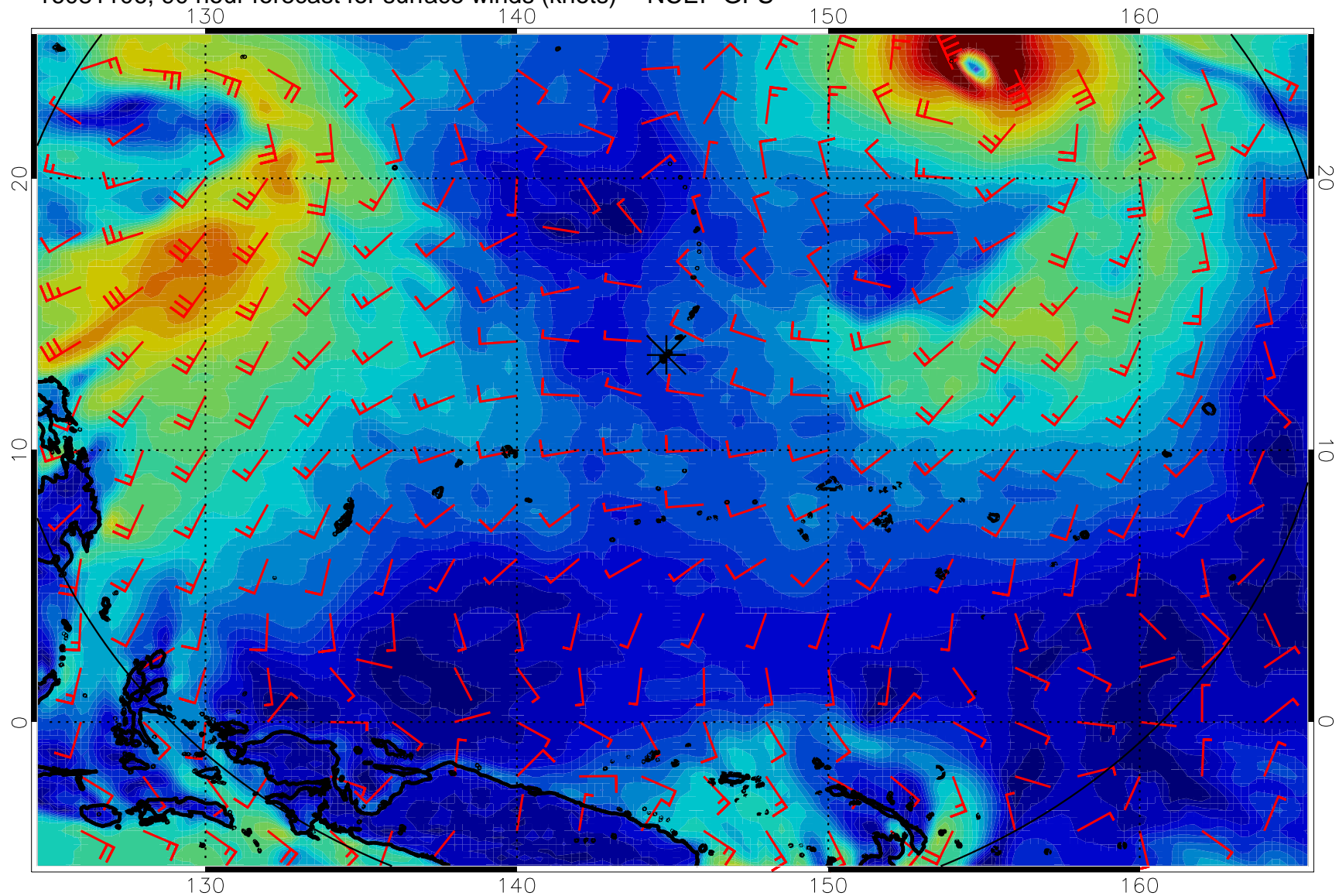
16081106, 90 hour forecast for surface winds (knots) -- NCEP GFS
