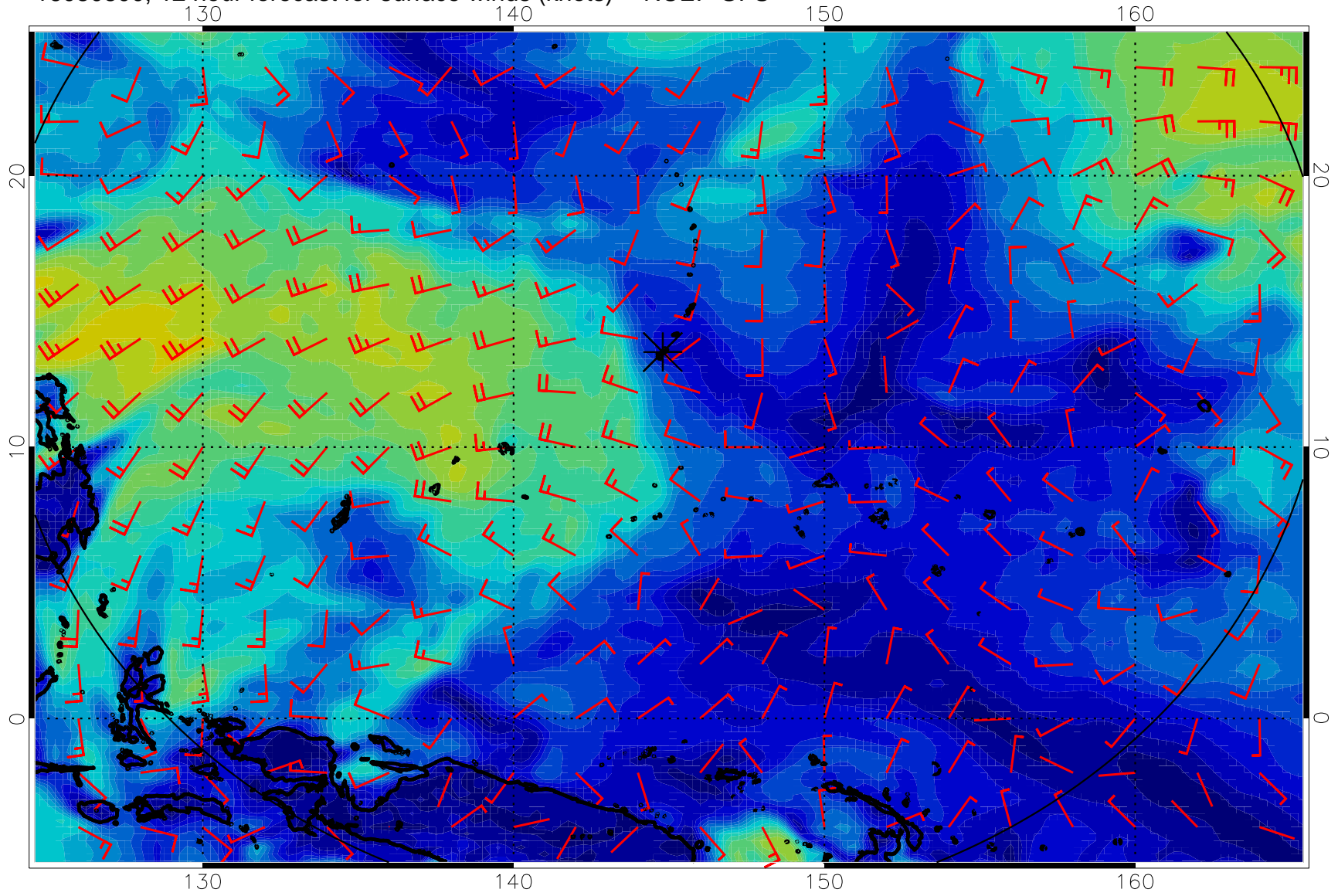
16080800, 12 hour forecast for surface winds (knots) -- NCEP GFS
