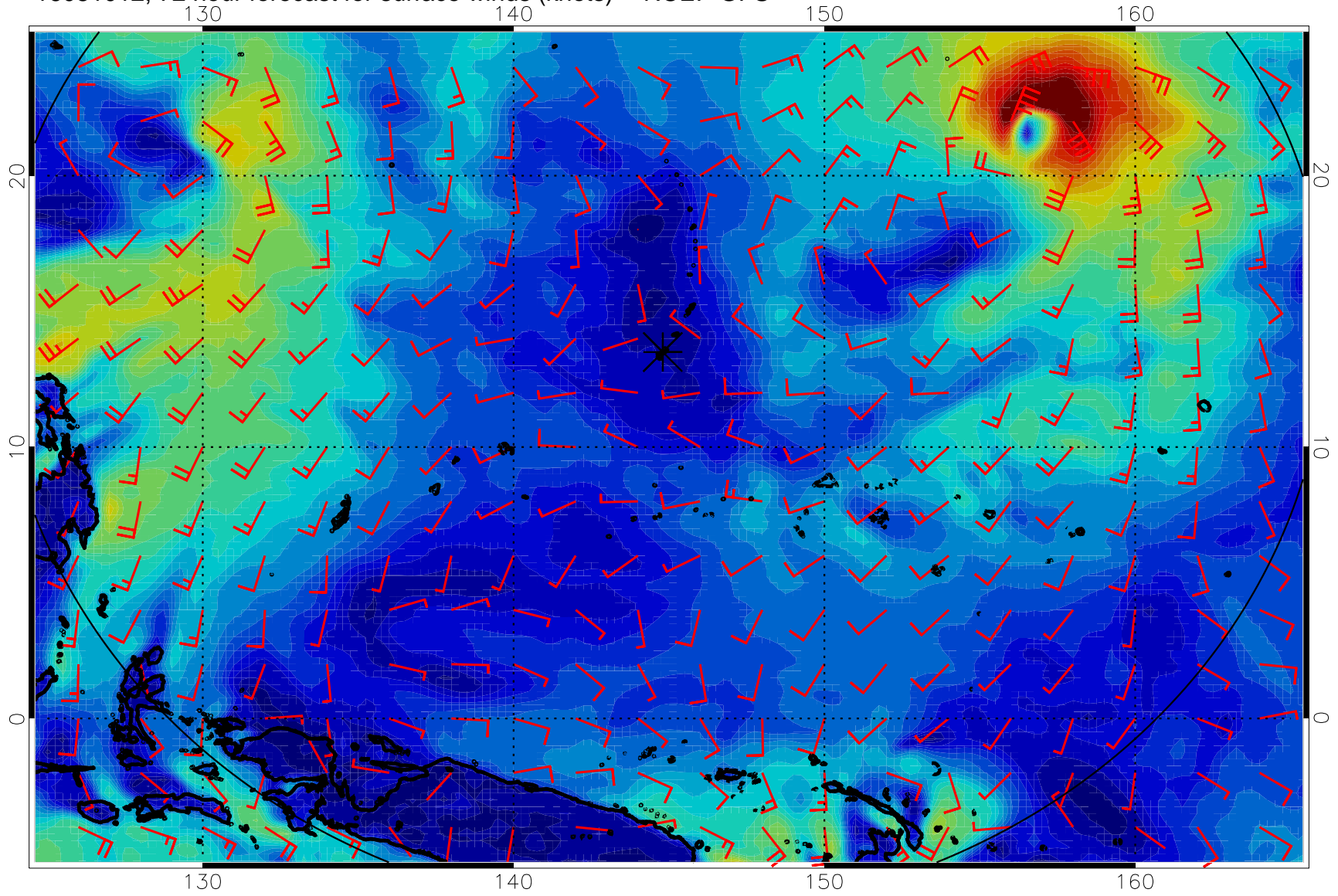
16081012, 72 hour forecast for surface winds (knots) -- NCEP GFS
