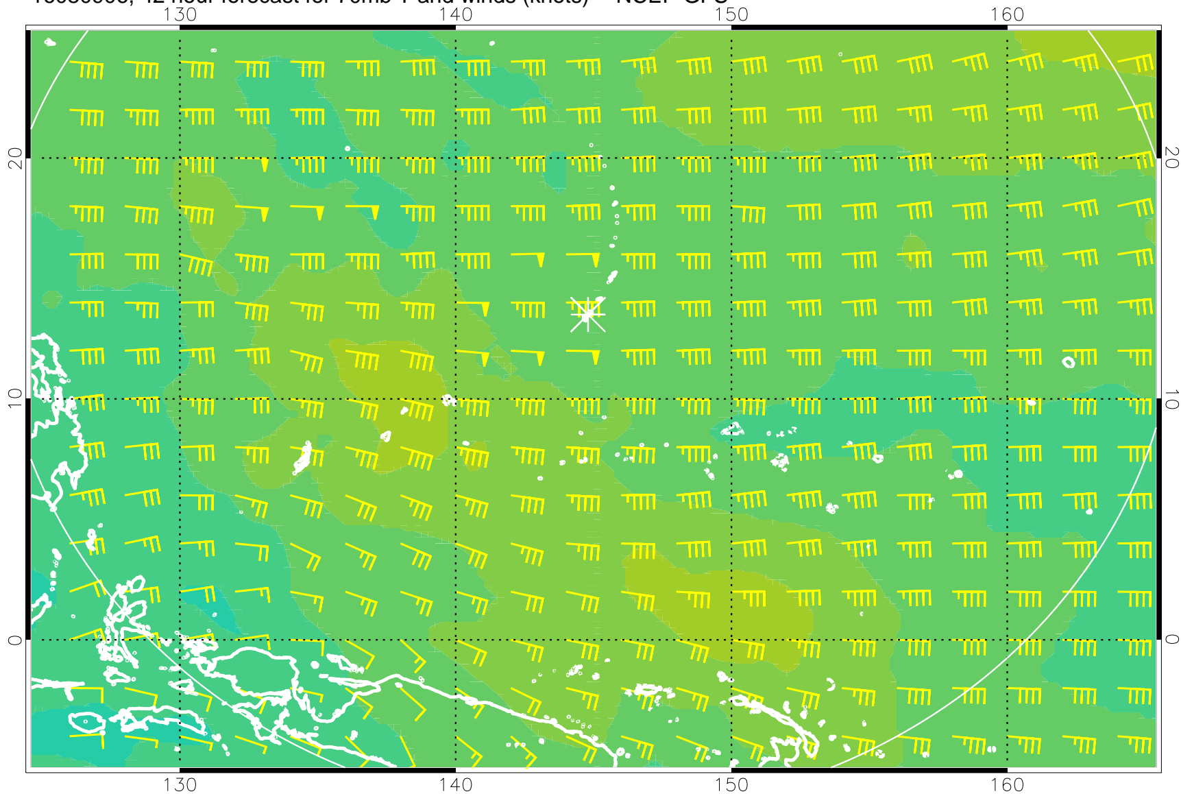
16080906, 42 hour forecast for 70mb T and winds (knots) -- NCEP GFS
