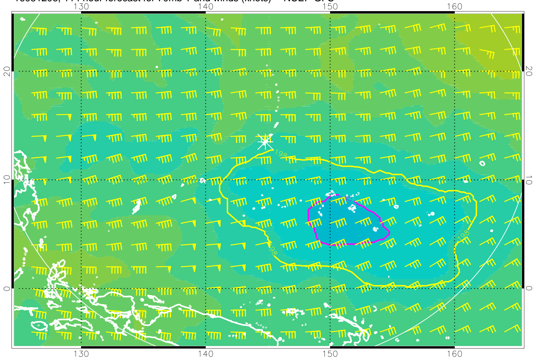
16081206, 114 hour forecast for 70mb T and winds (knots) -- NCEP GFS
