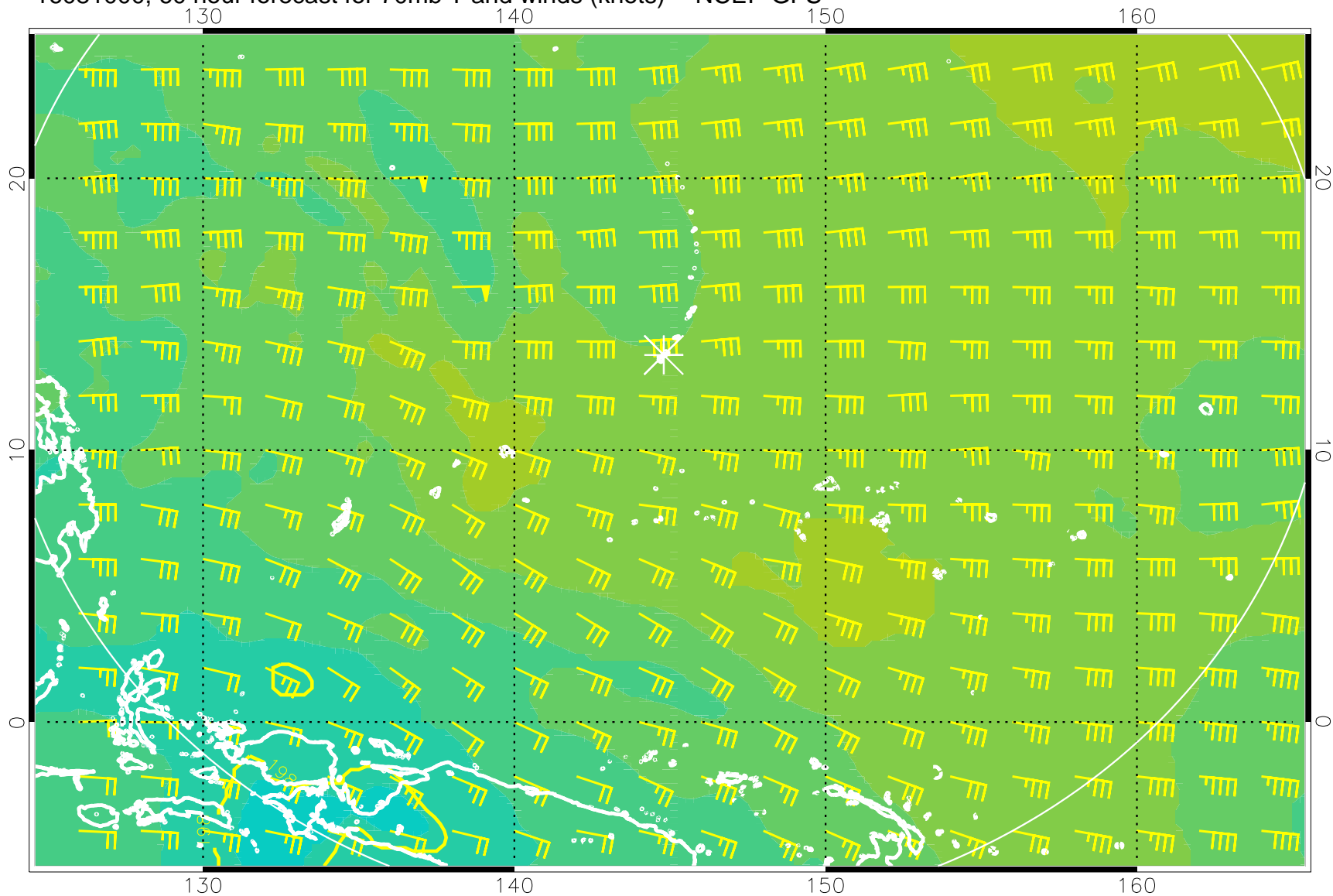
16081000, 60 hour forecast for 70mb T and winds (knots) -- NCEP GFS
