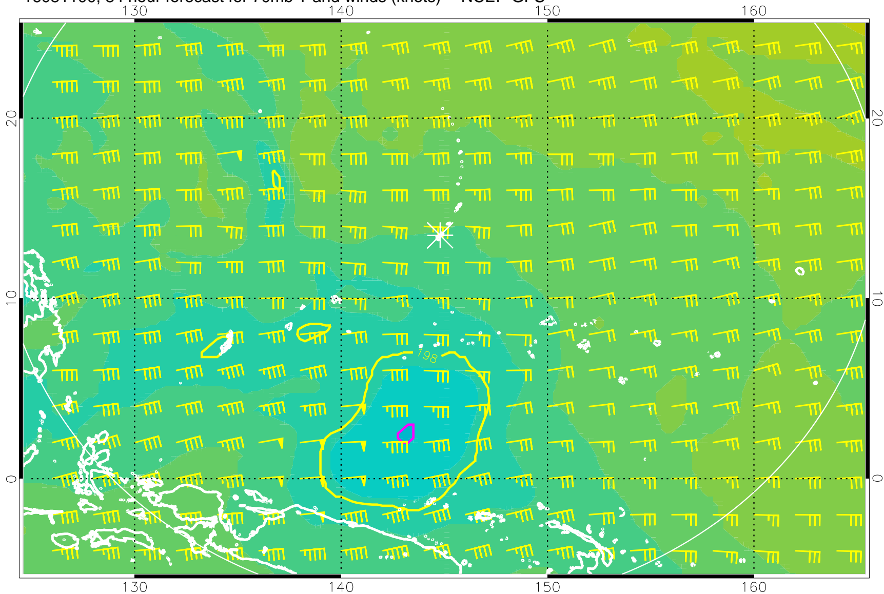
16081100, 84 hour forecast for 70mb T and winds (knots) -- NCEP GFS
