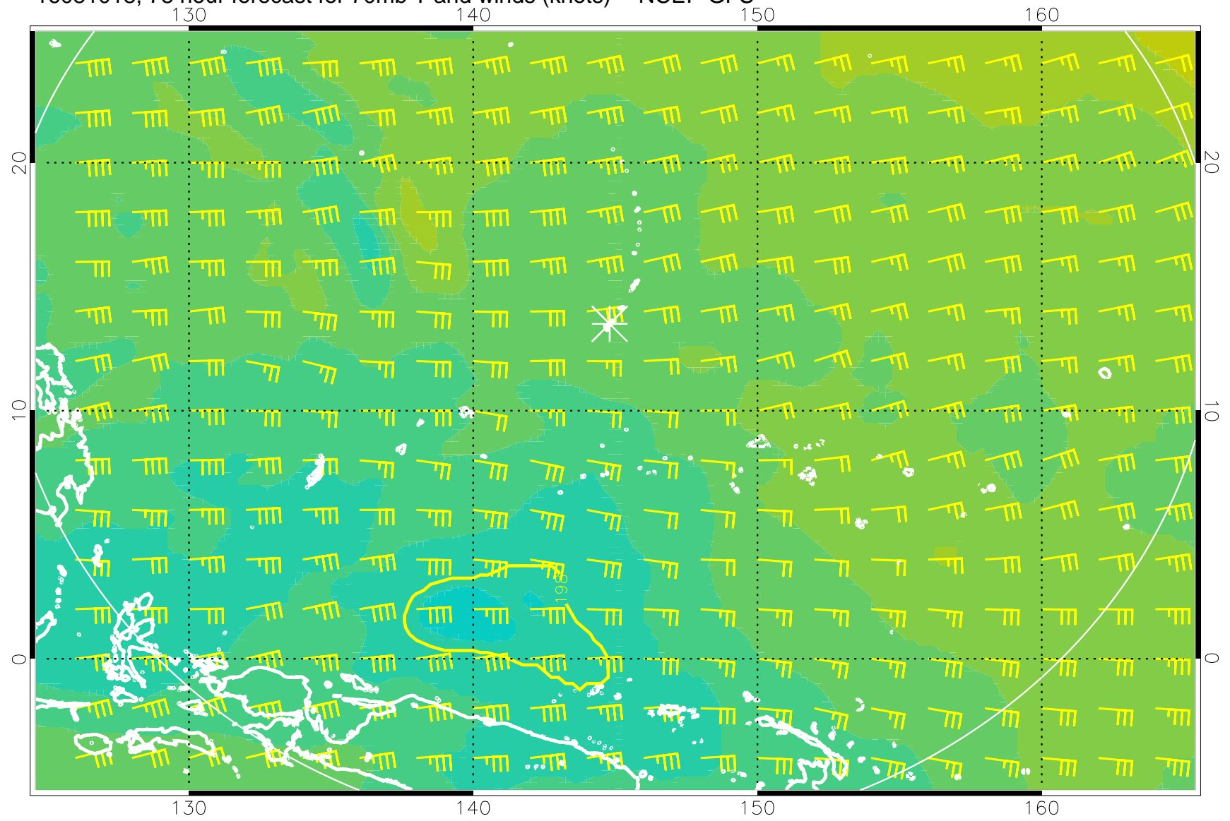
16081018, 78 hour forecast for 70mb T and winds (knots) -- NCEP GFS
