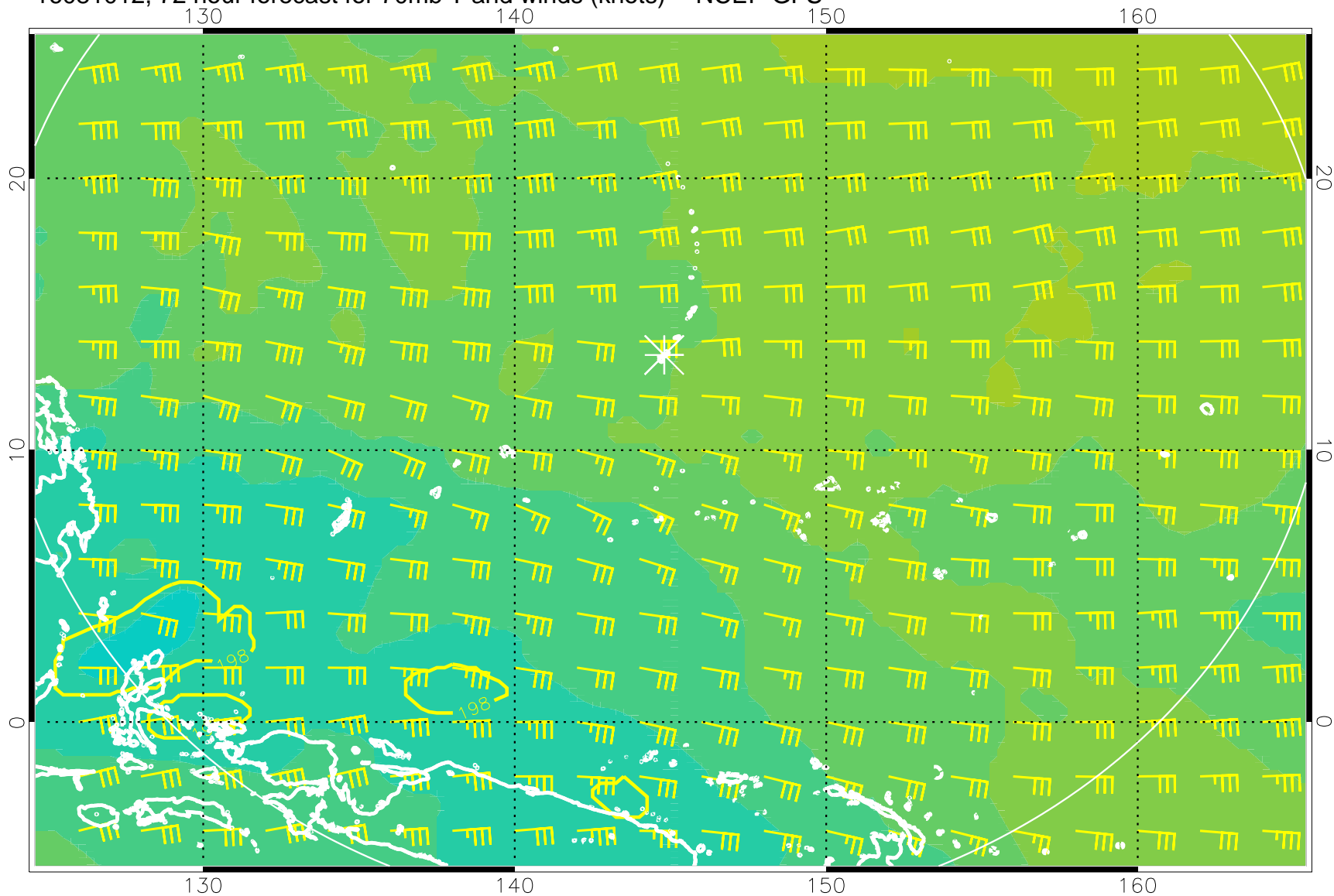
16081012, 72 hour forecast for 70mb T and winds (knots) -- NCEP GFS
