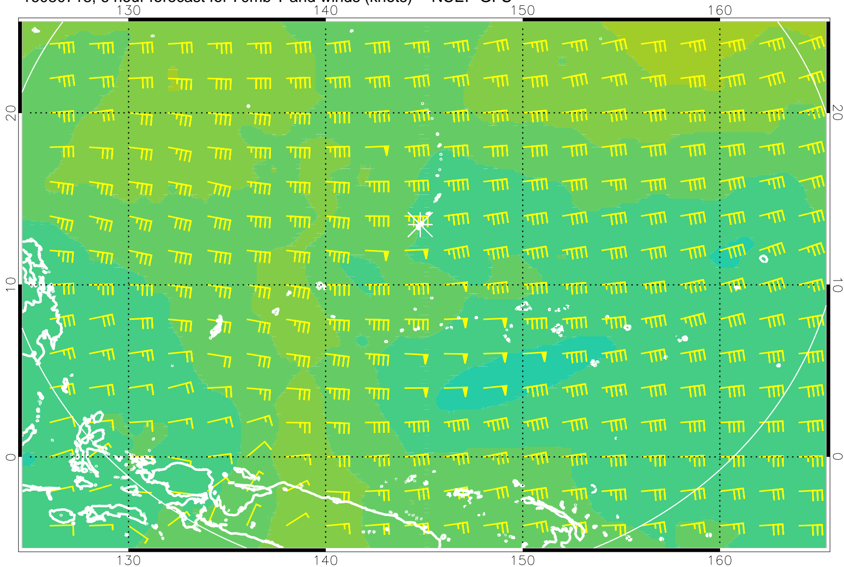
16080718, 6 hour forecast for 70mb T and winds (knots) -- NCEP GFS
