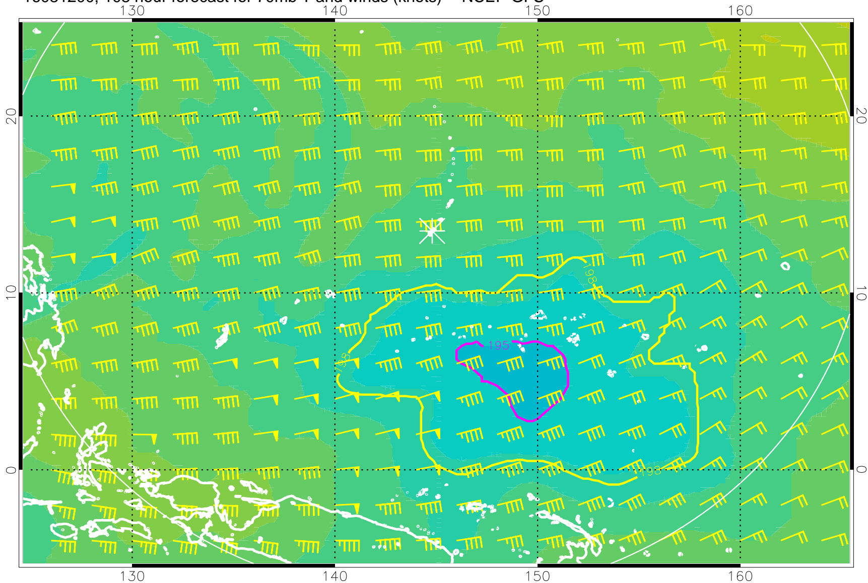
16081200, 108 hour forecast for 70mb T and winds (knots) -- NCEP GFS
