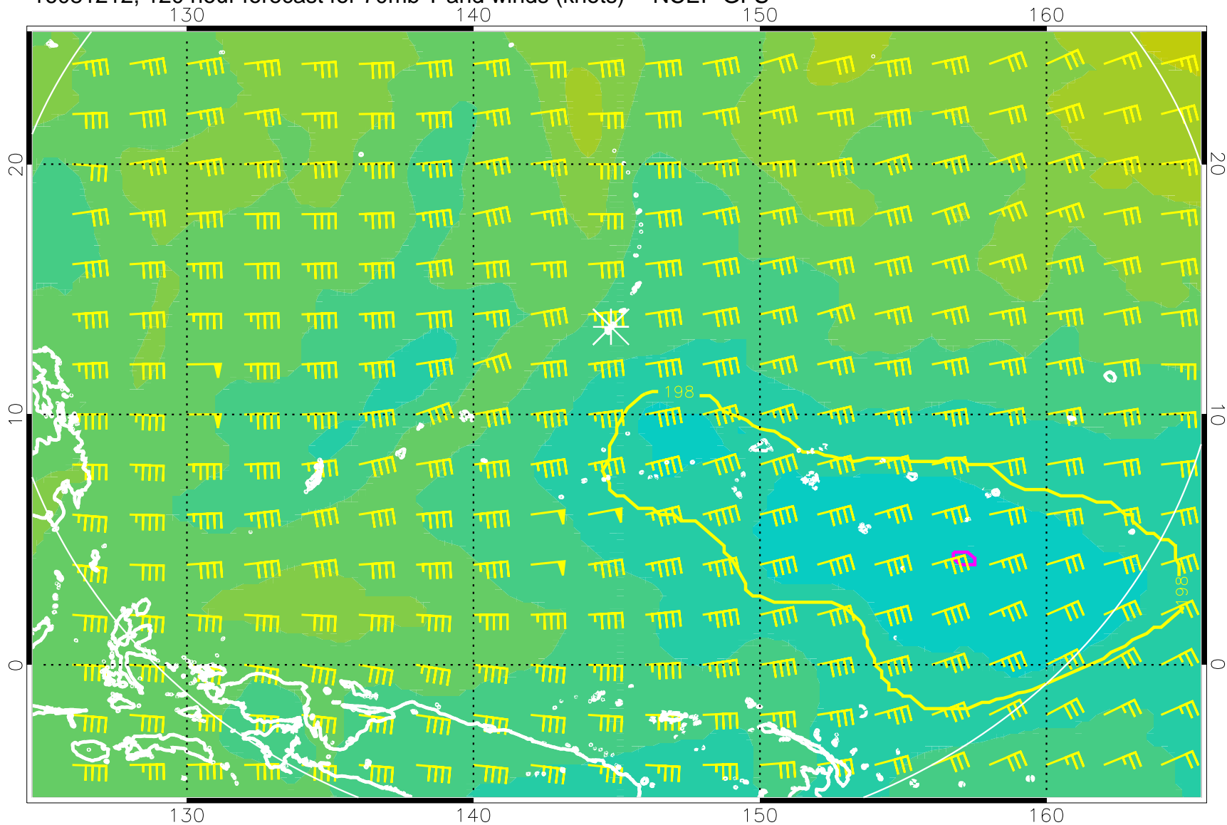
16081212, 120 hour forecast for 70mb T and winds (knots) -- NCEP GFS
