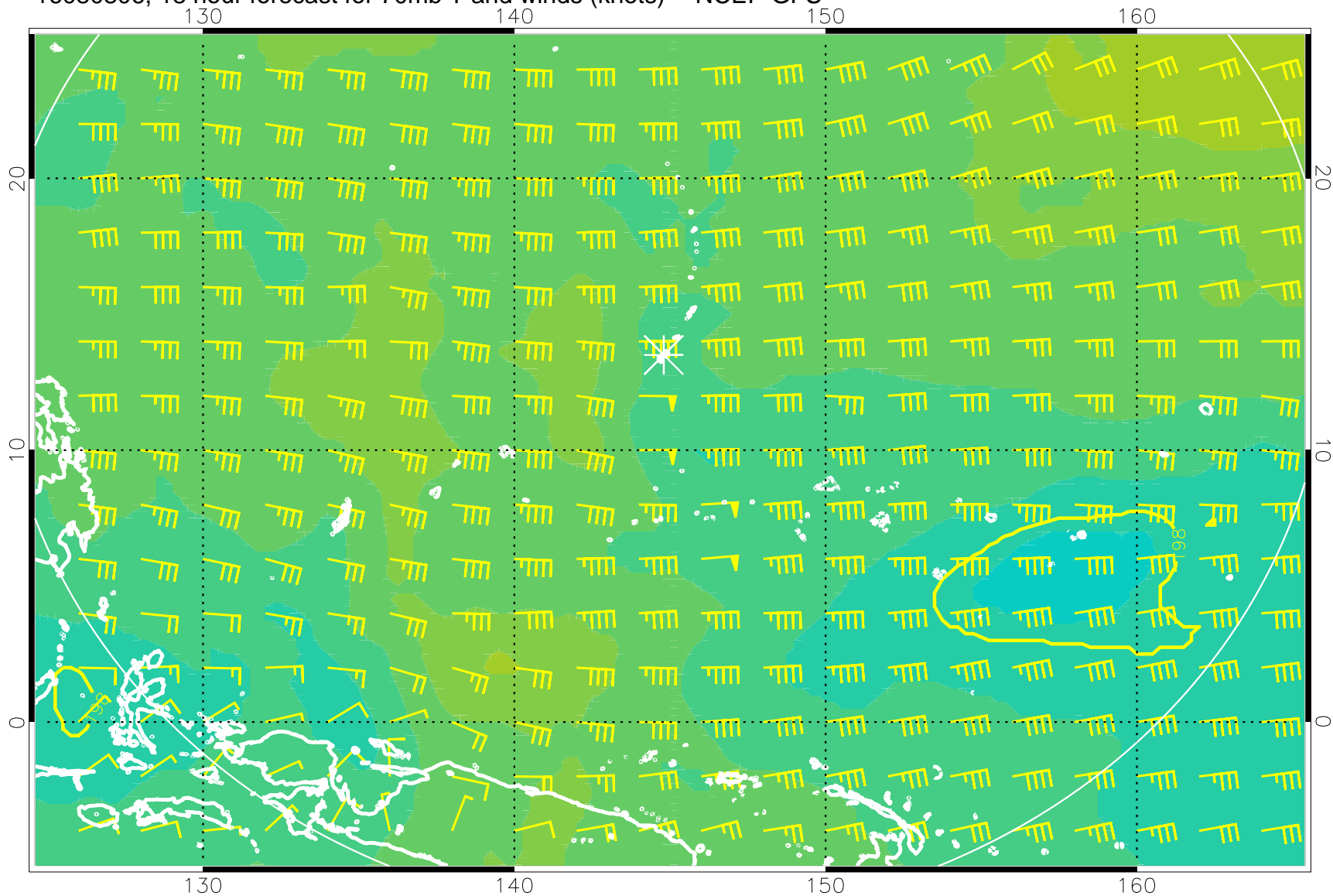
16080806, 18 hour forecast for 70mb T and winds (knots) -- NCEP GFS
