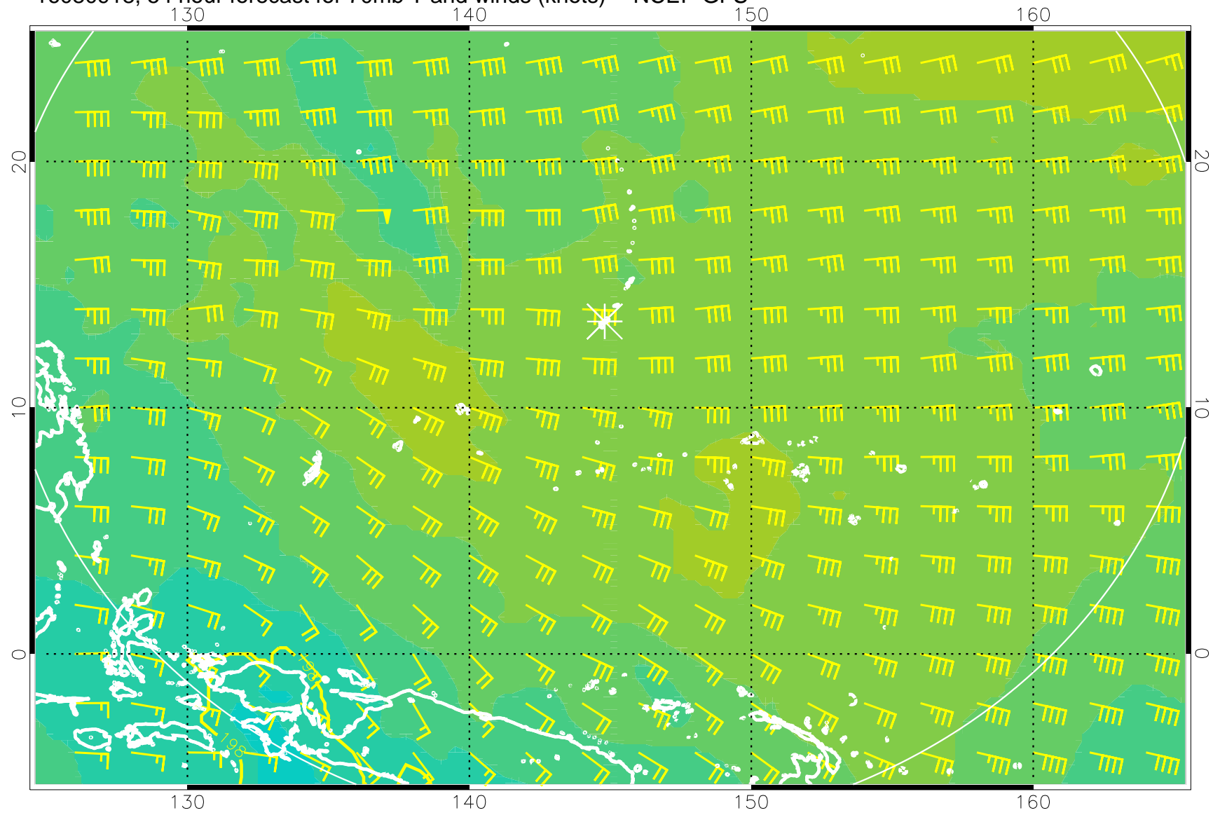
16080918, 54 hour forecast for 70mb T and winds (knots) -- NCEP GFS
