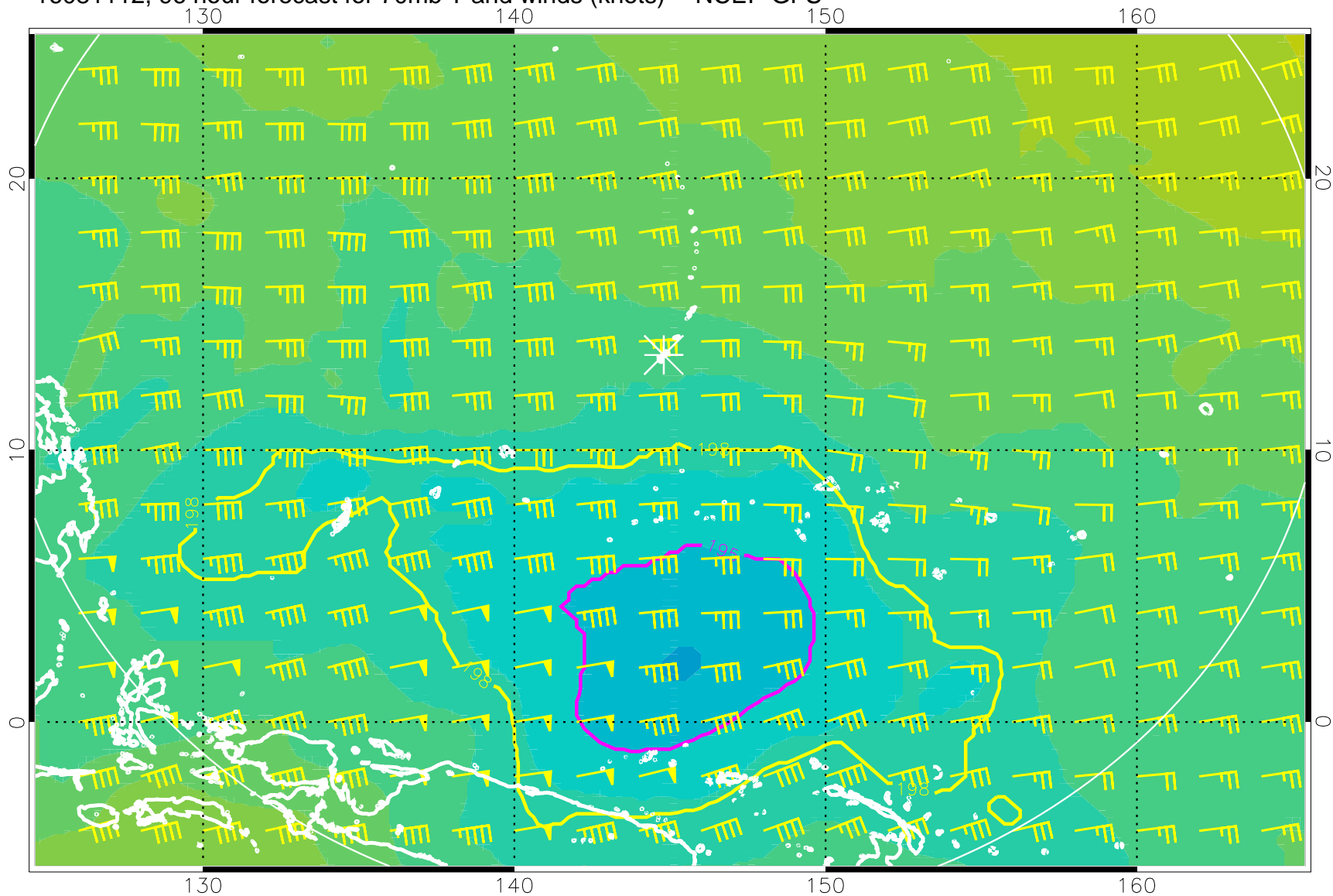
16081112, 96 hour forecast for 70mb T and winds (knots) -- NCEP GFS
