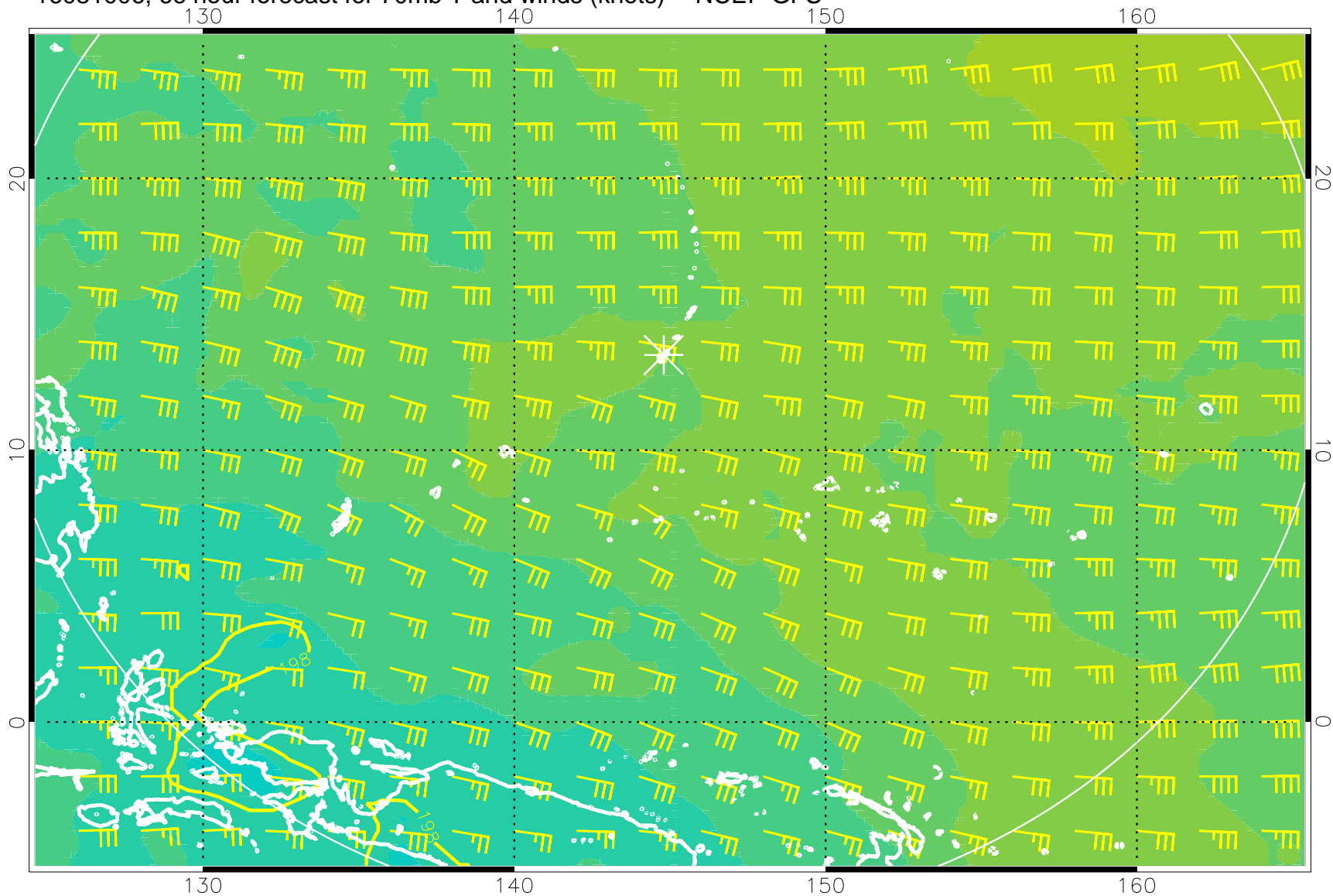
16081006, 66 hour forecast for 70mb T and winds (knots) -- NCEP GFS
