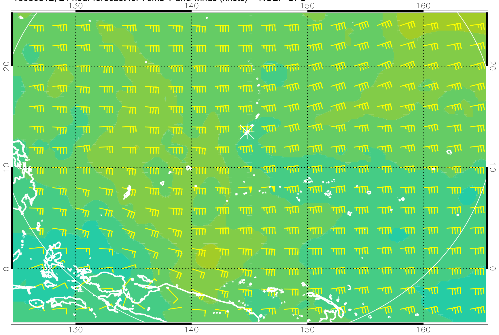
16080812, 24 hour forecast for 70mb T and winds (knots) -- NCEP GFS
