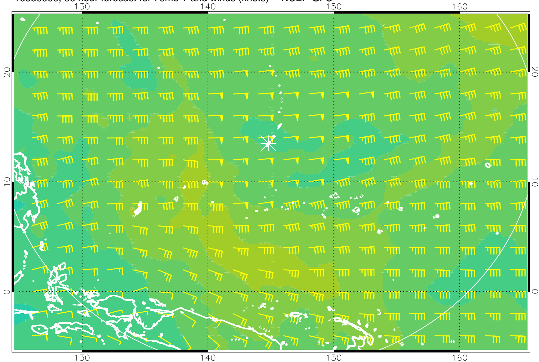
16080900, 36 hour forecast for 70mb T and winds (knots) -- NCEP GFS
