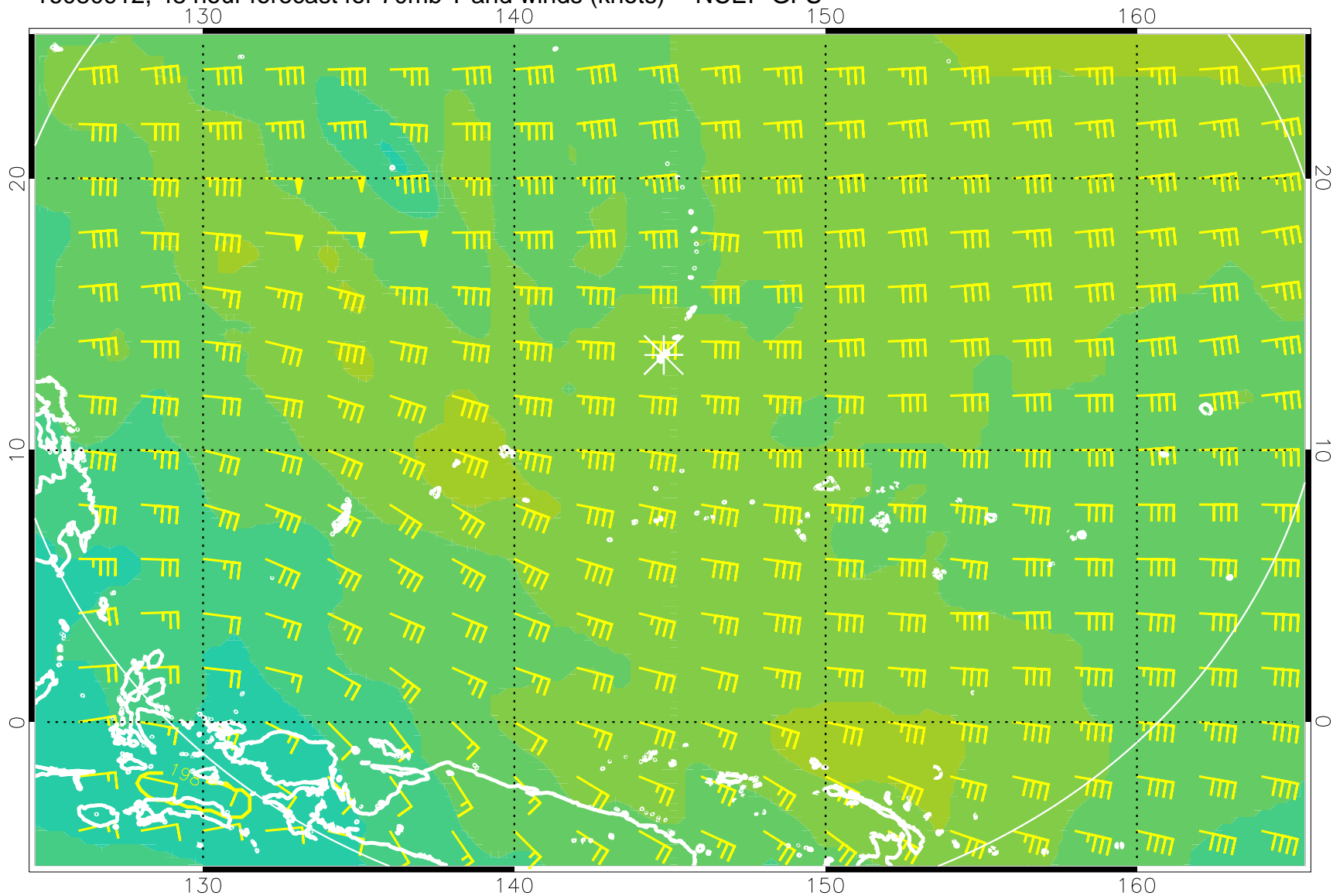
16080912, 48 hour forecast for 70mb T and winds (knots) -- NCEP GFS
