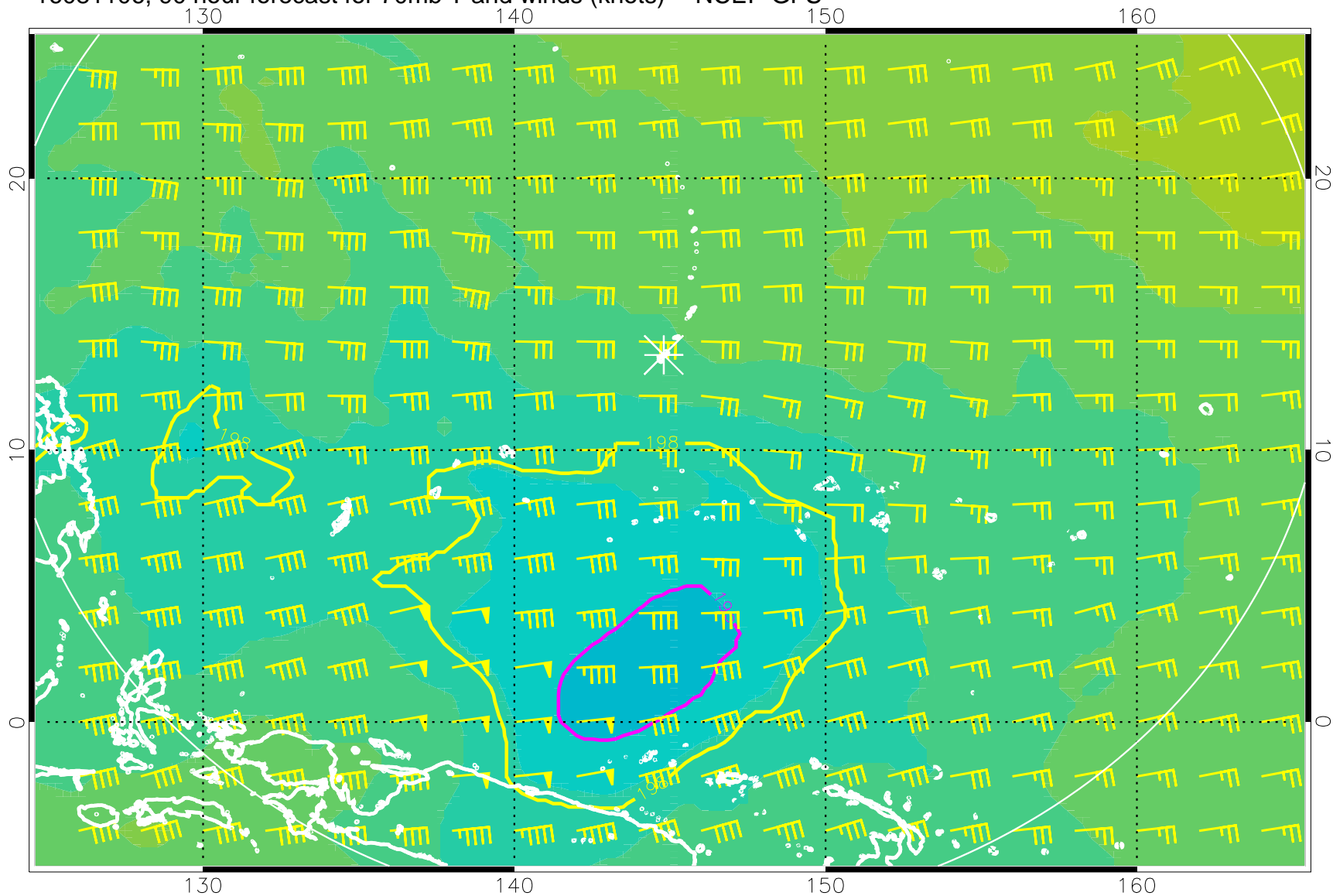
16081106, 90 hour forecast for 70mb T and winds (knots) -- NCEP GFS
