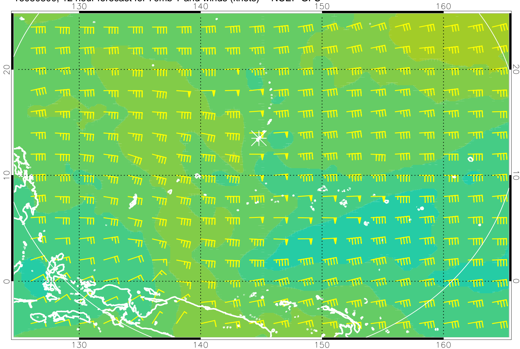
16080800, 12 hour forecast for 70mb T and winds (knots) -- NCEP GFS
