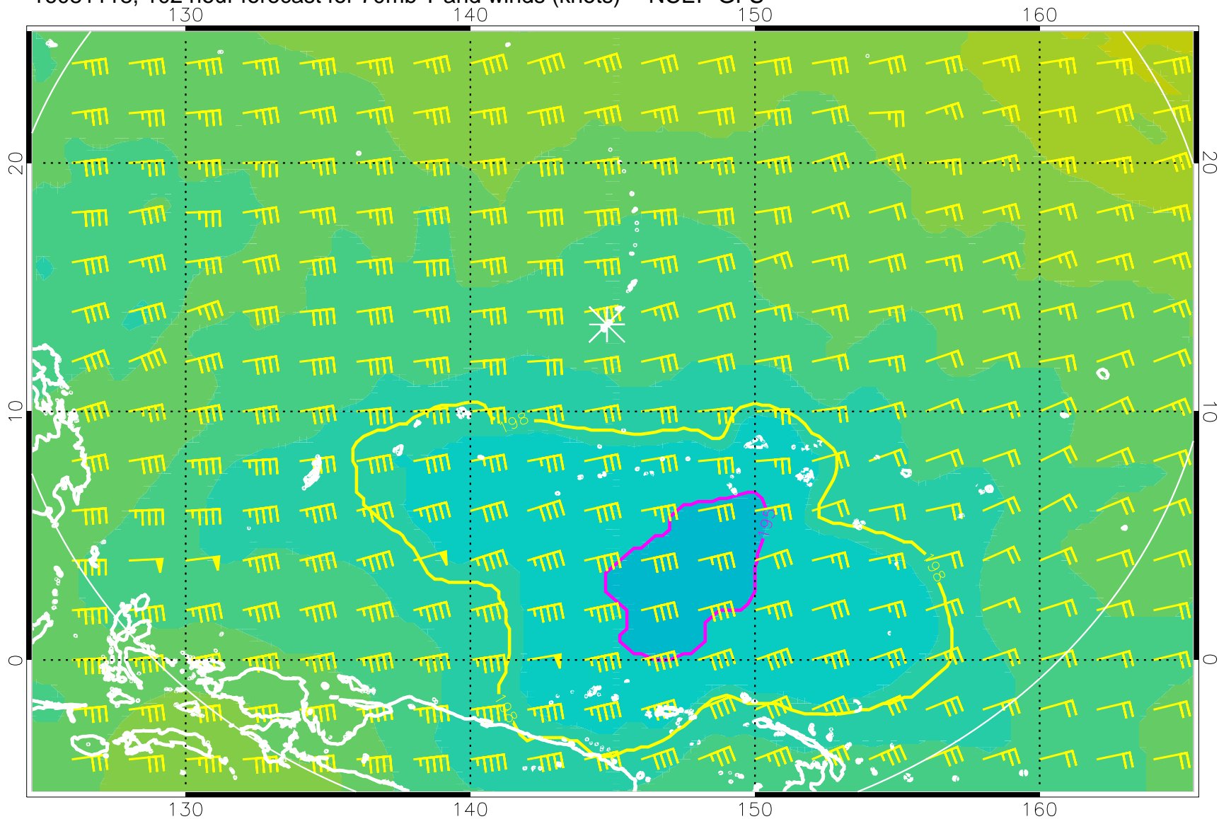
16081118, 102 hour forecast for 70mb T and winds (knots) -- NCEP GFS
