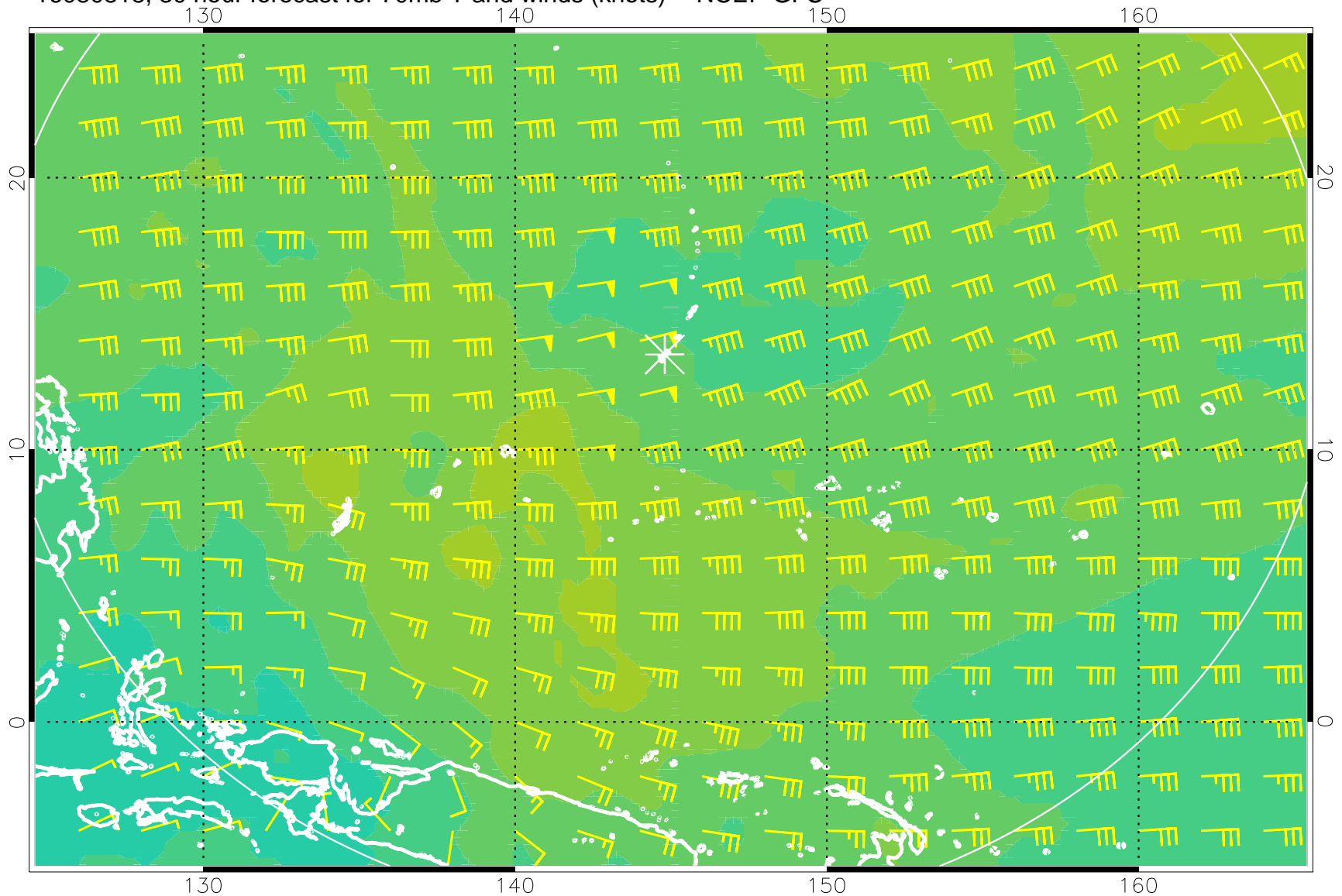
16080818, 30 hour forecast for 70mb T and winds (knots) -- NCEP GFS
