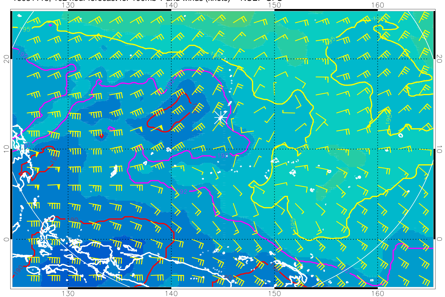
16081118, 102 hour forecast for 100mb T and winds (knots) -- NCEP GFS
