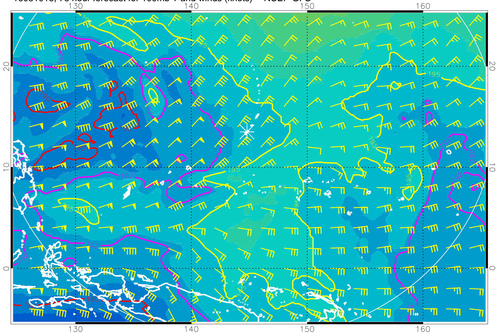
16081018, 78 hour forecast for 100mb T and winds (knots) -- NCEP GFS
