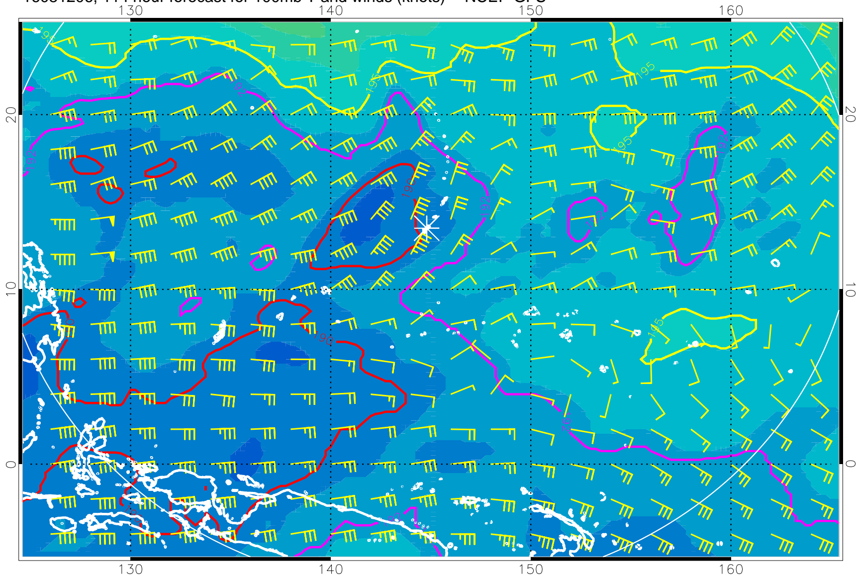
16081206, 114 hour forecast for 100mb T and winds (knots) -- NCEP GFS
