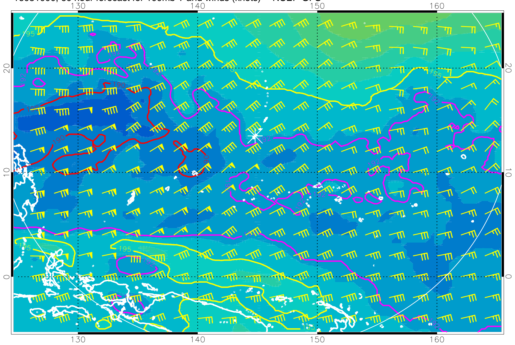
16081000, 60 hour forecast for 100mb T and winds (knots) -- NCEP GFS
