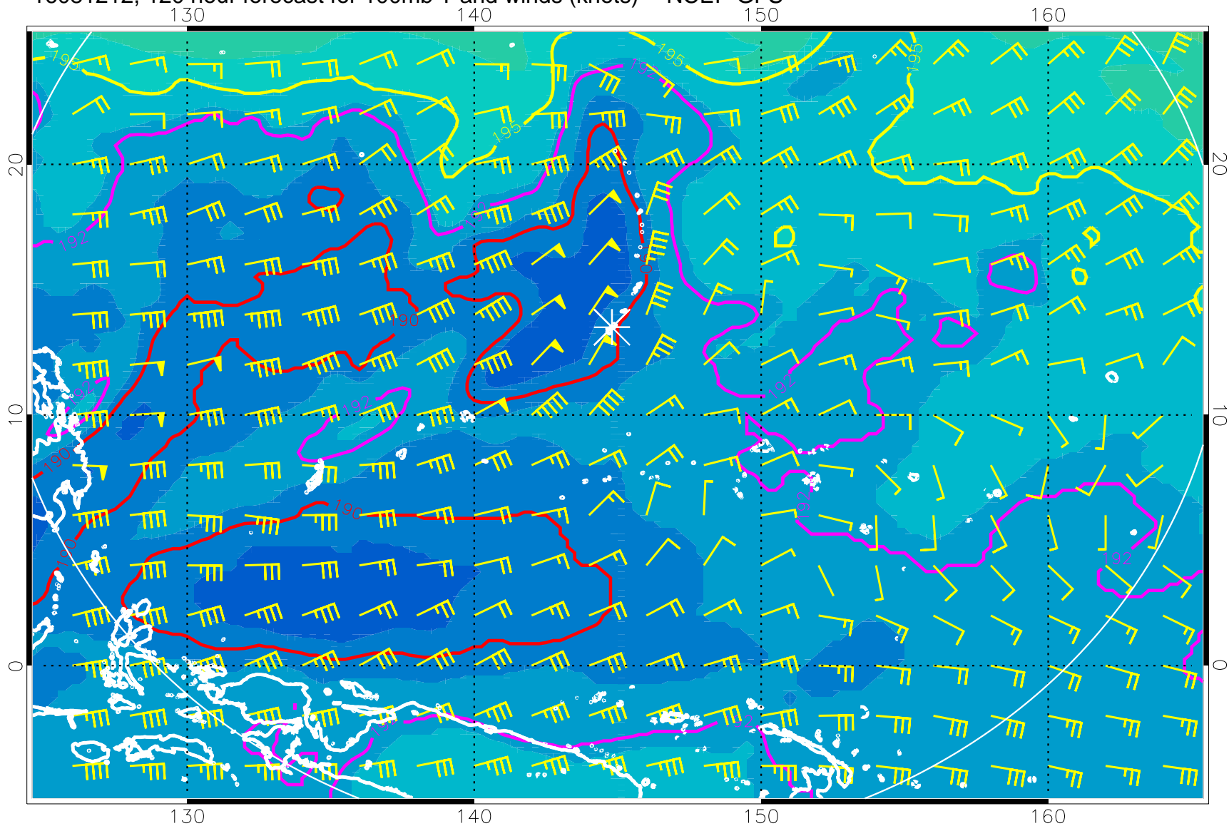
16081212, 120 hour forecast for 100mb T and winds (knots) -- NCEP GFS
