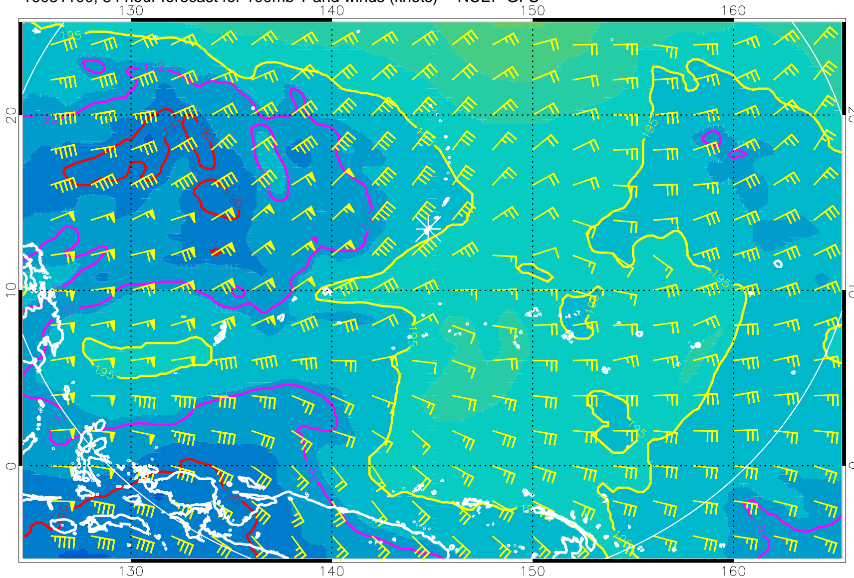
16081100, 84 hour forecast for 100mb T and winds (knots) -- NCEP GFS
