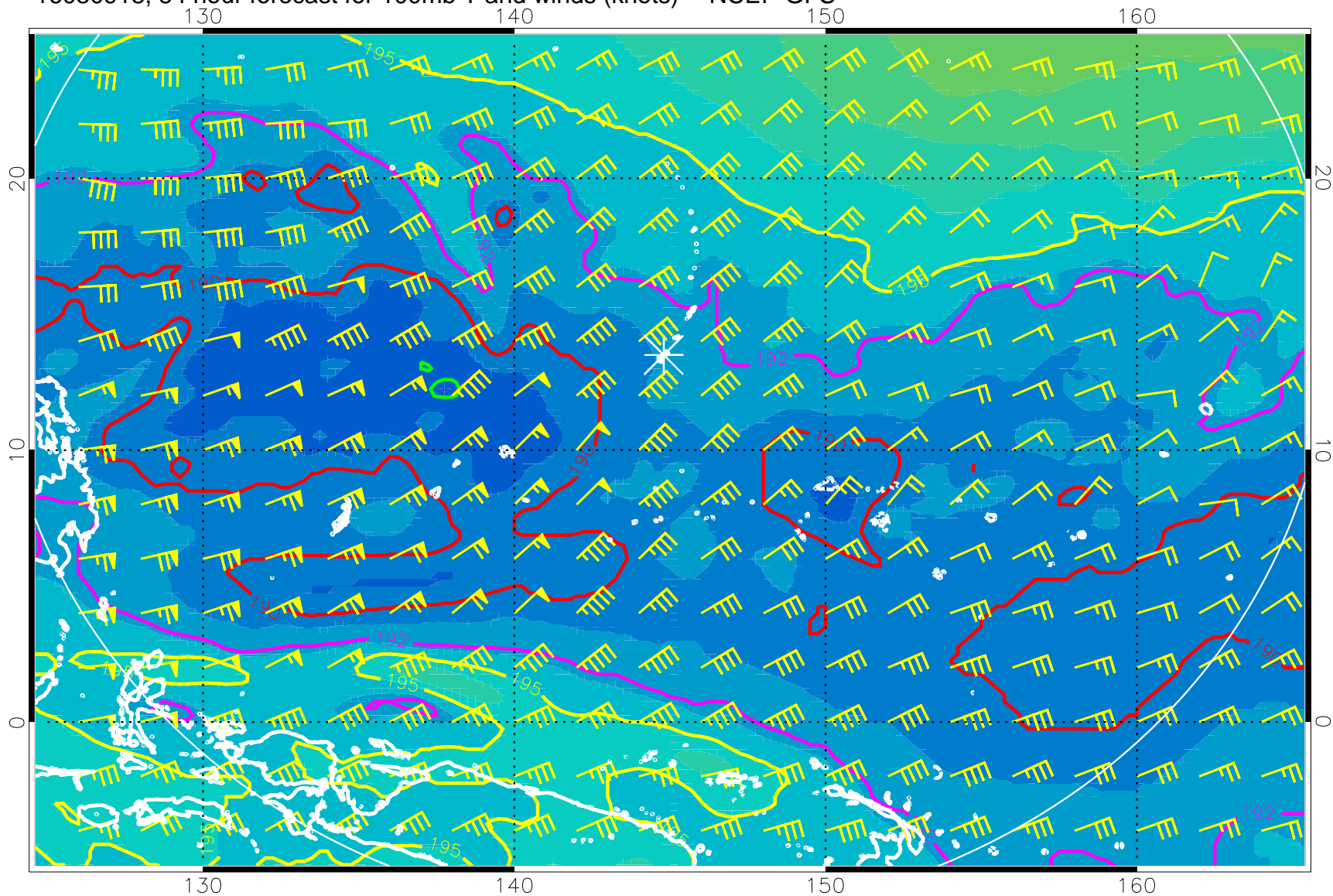
16080918, 54 hour forecast for 100mb T and winds (knots) -- NCEP GFS
