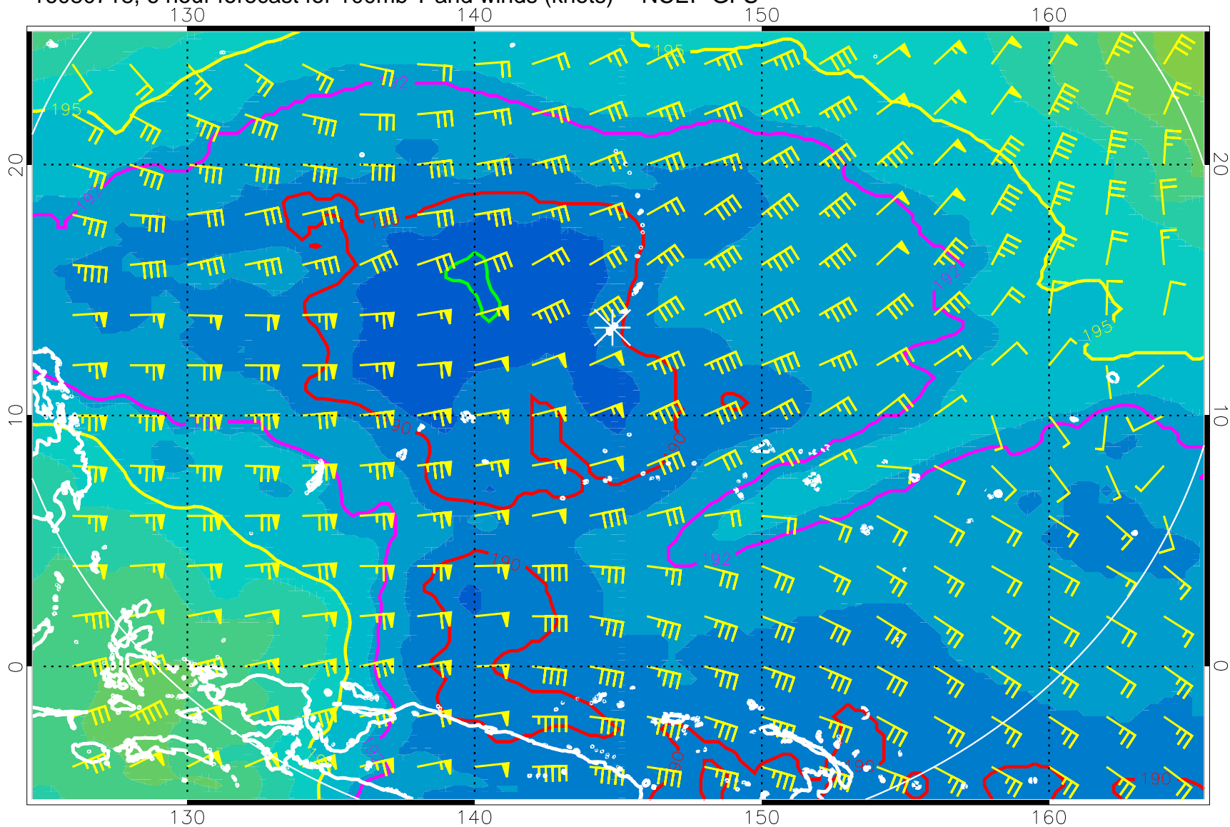
16080718, 6 hour forecast for 100mb T and winds (knots) -- NCEP GFS
