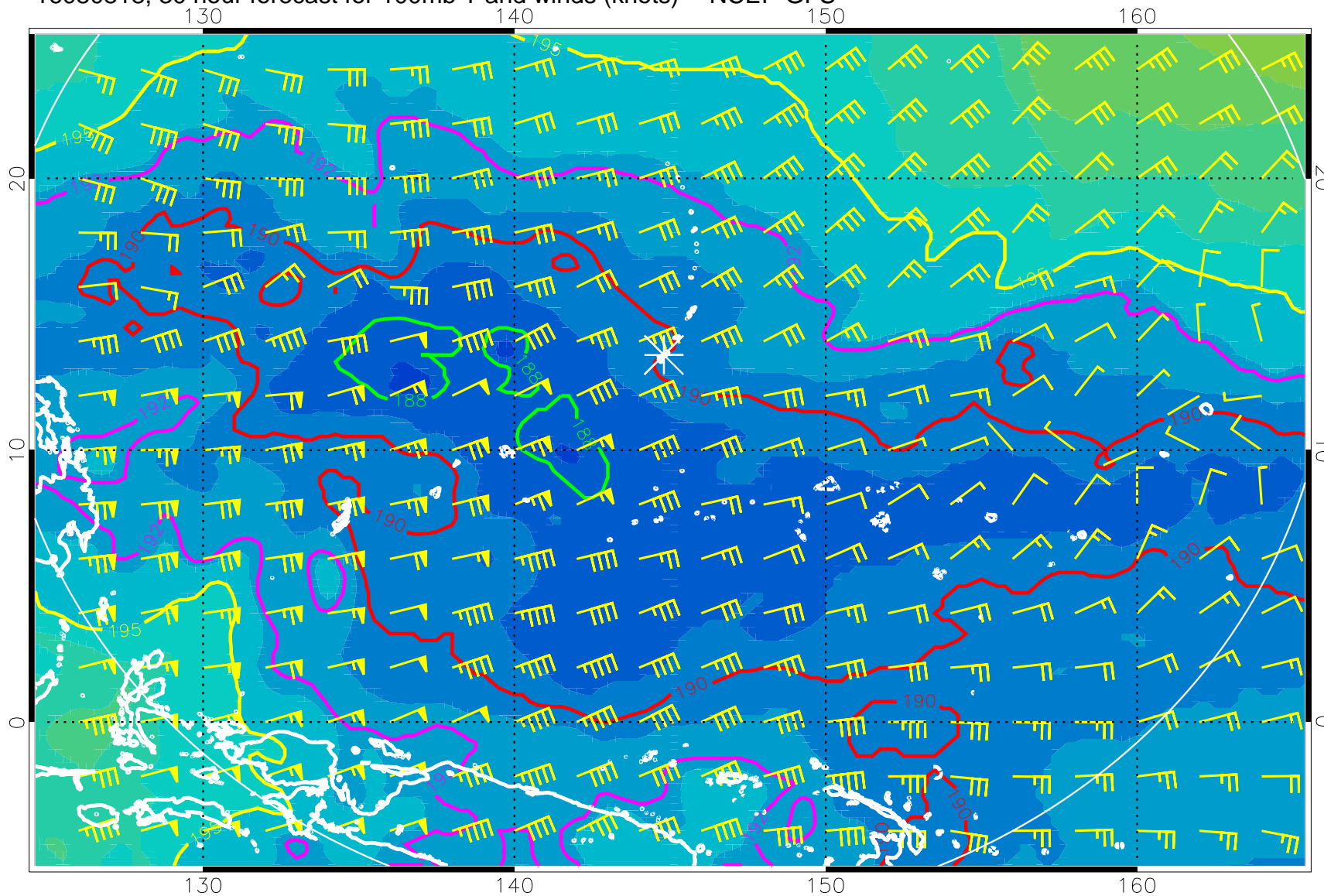
16080818, 30 hour forecast for 100mb T and winds (knots) -- NCEP GFS
