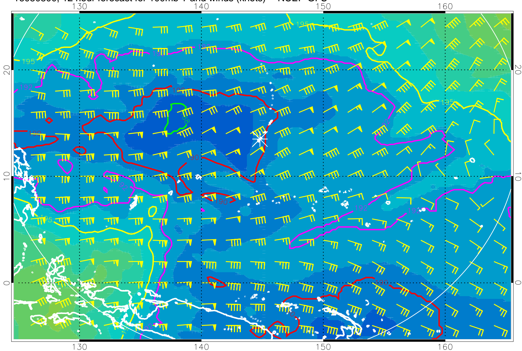
16080800, 12 hour forecast for 100mb T and winds (knots) -- NCEP GFS
