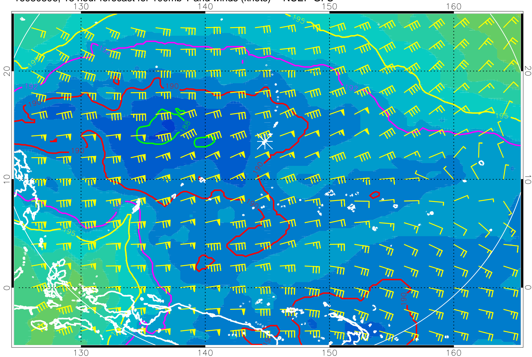
16080806, 18 hour forecast for 100mb T and winds (knots) -- NCEP GFS
