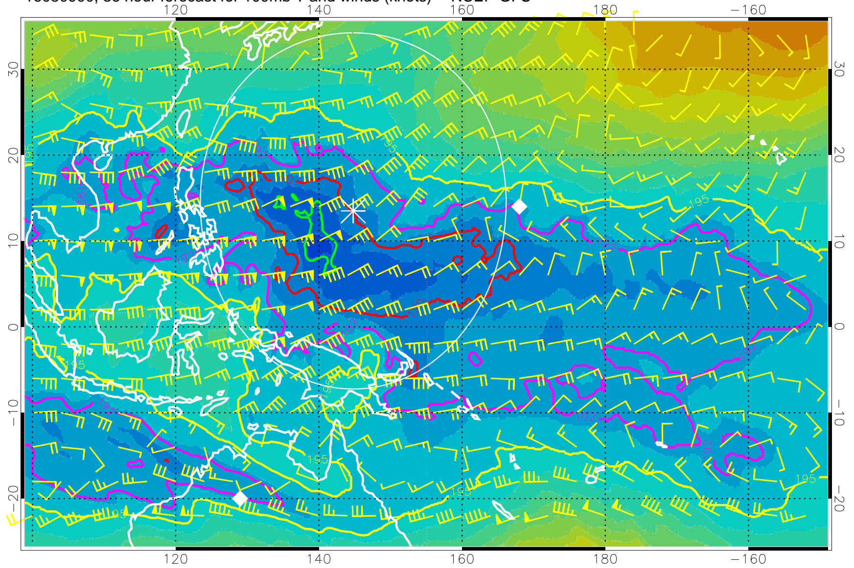
16080900, 36 hour forecast for 100mb T and winds (knots) -- NCEP GFS
