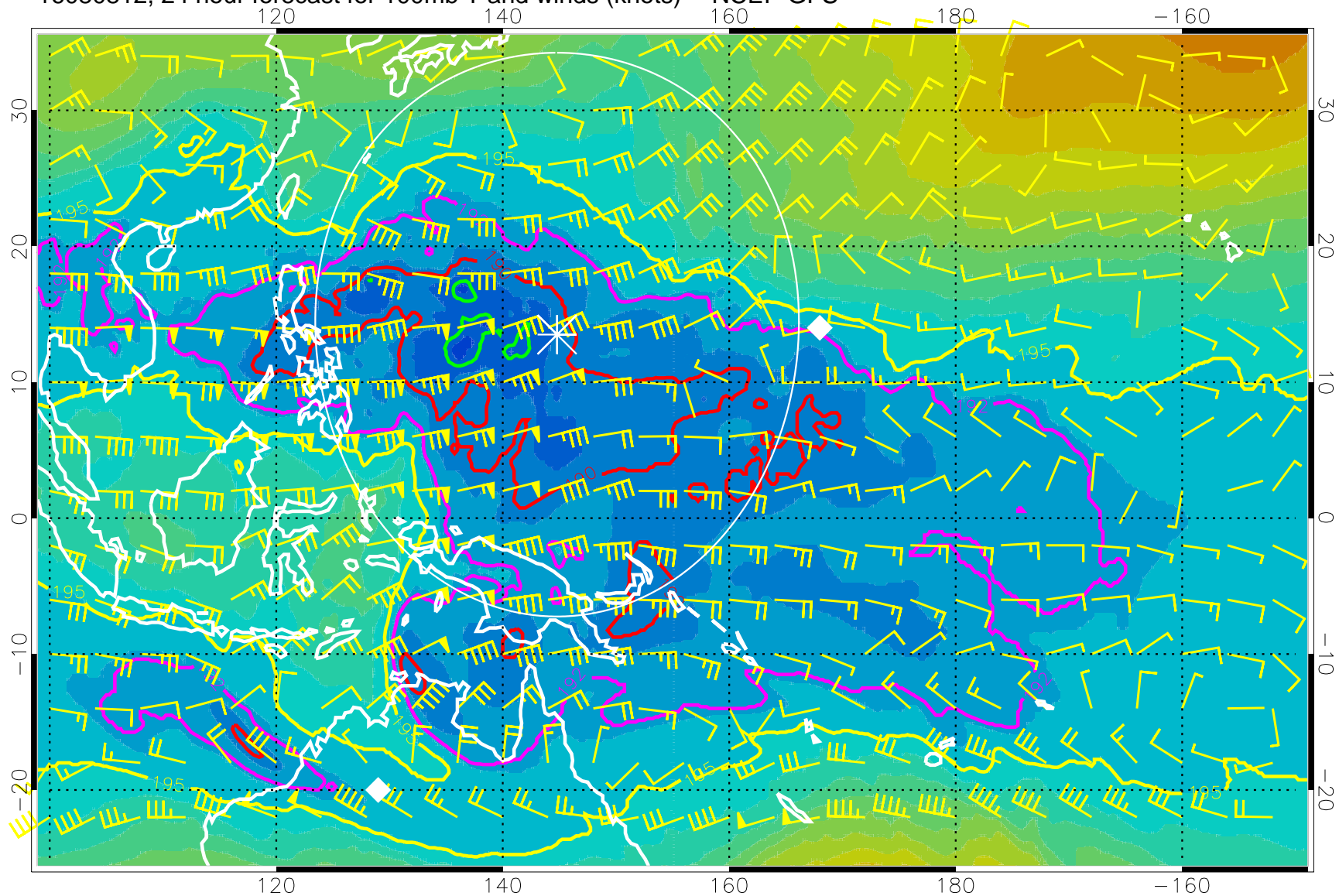
16080812, 24 hour forecast for 100mb T and winds (knots) -- NCEP GFS
