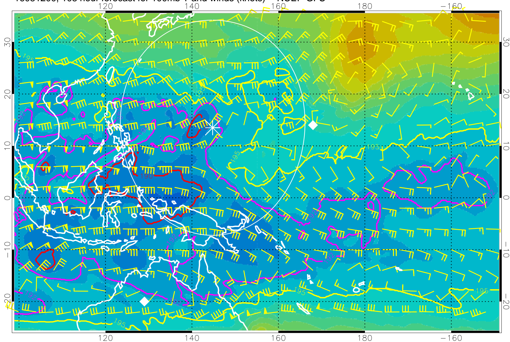
16081200, 108 hour forecast for 100mb T and winds (knots) -- NCEP GFS
