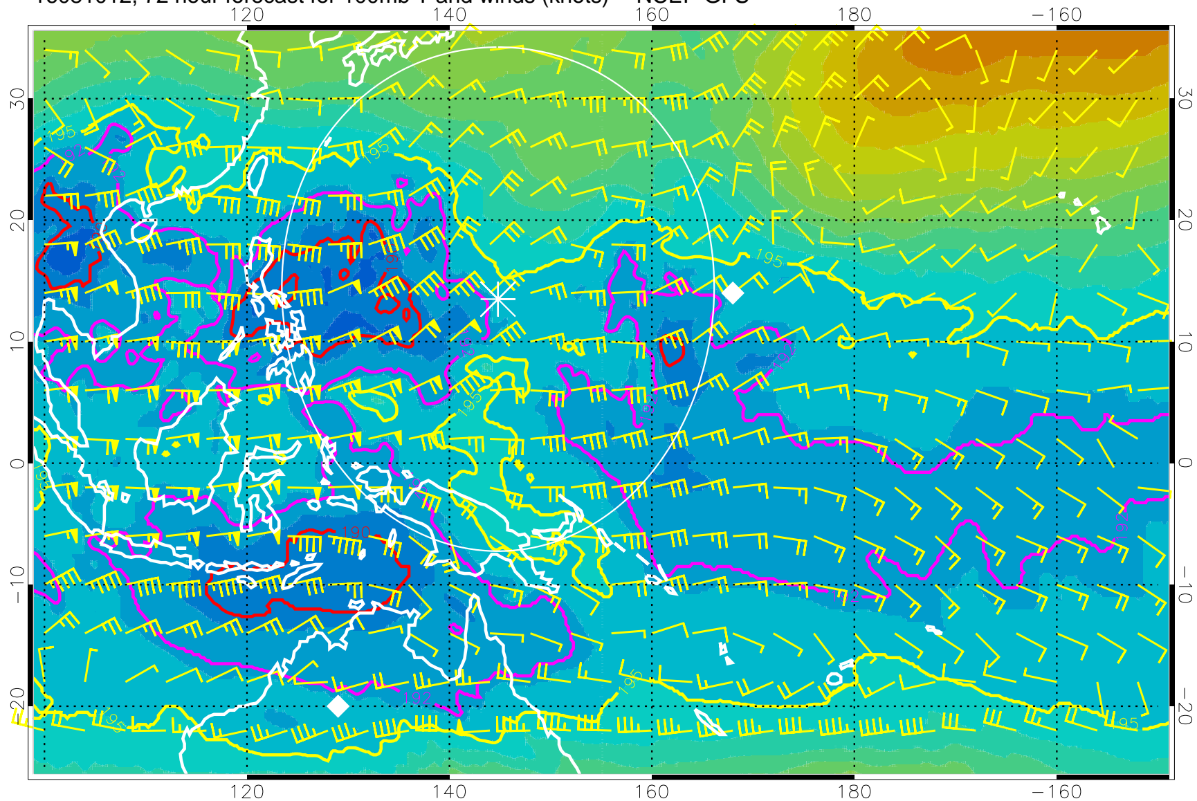
16081012, 72 hour forecast for 100mb T and winds (knots) -- NCEP GFS
