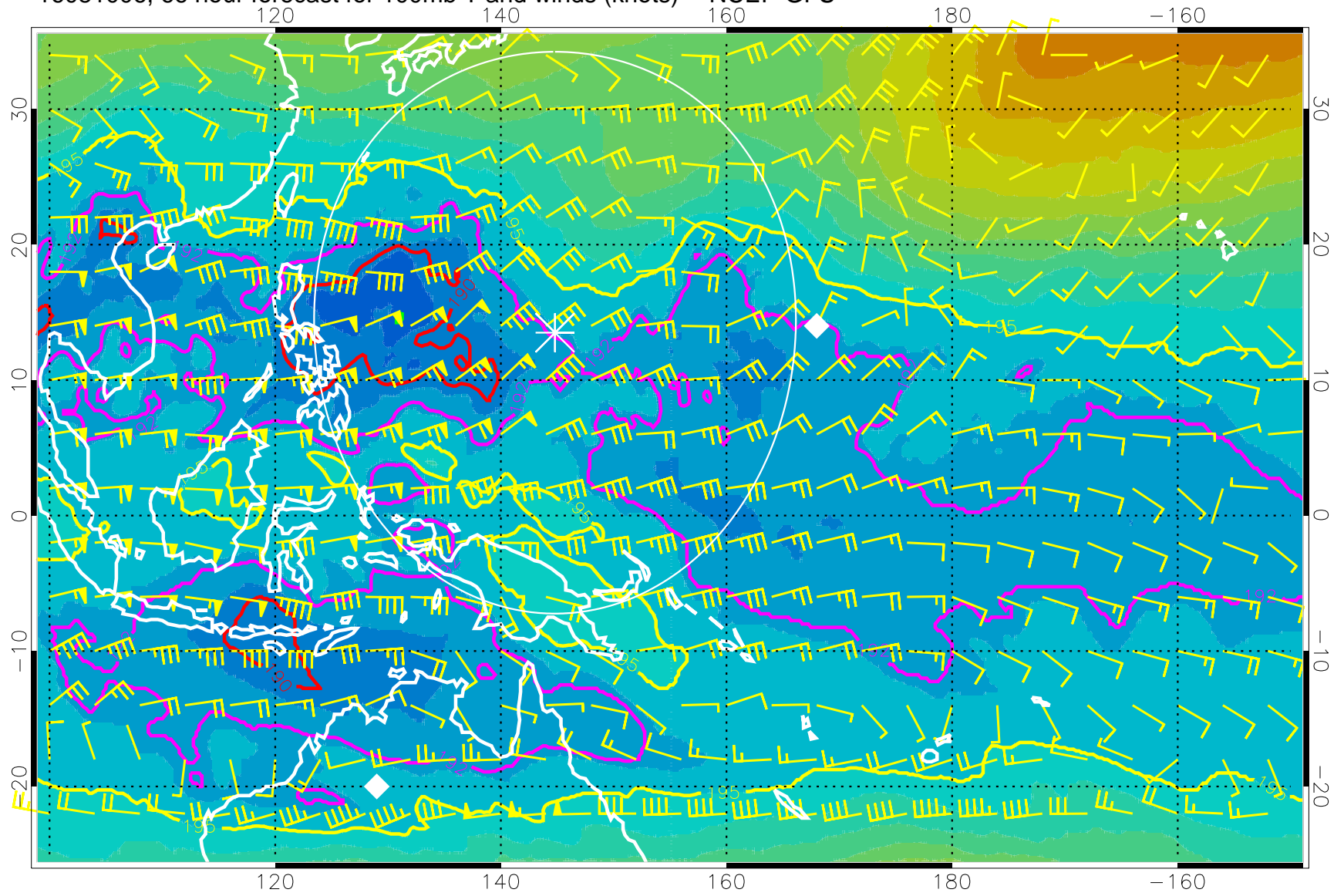
16081006, 66 hour forecast for 100mb T and winds (knots) -- NCEP GFS
