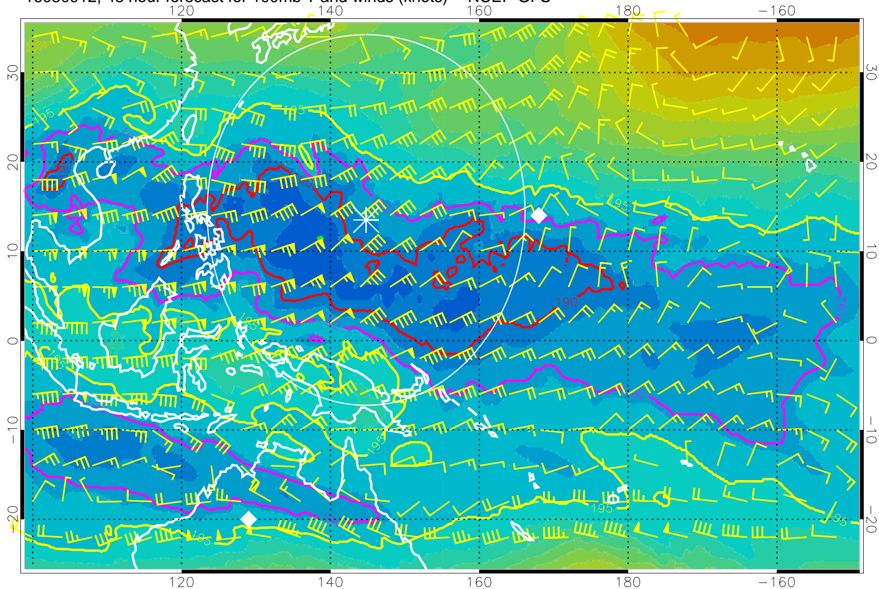
16080912, 48 hour forecast for 100mb T and winds (knots) -- NCEP GFS
