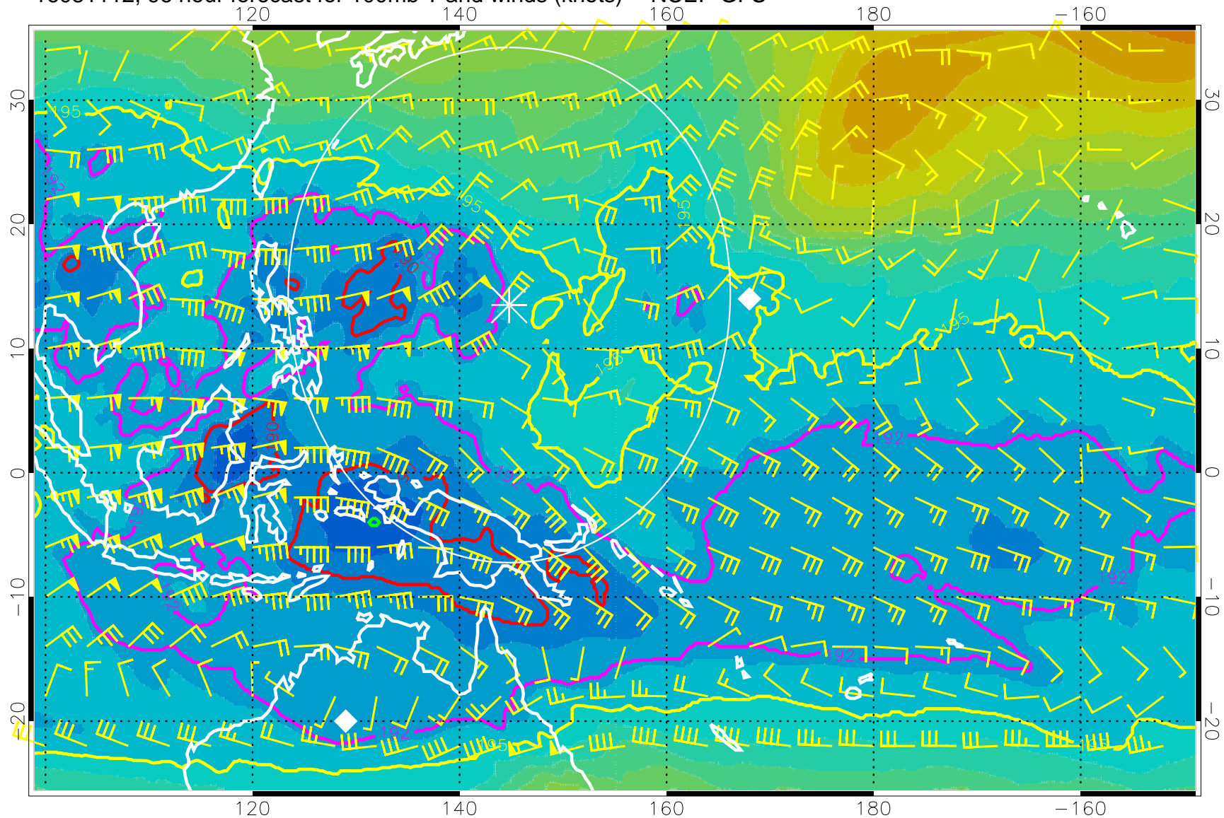
16081112, 96 hour forecast for 100mb T and winds (knots) -- NCEP GFS
