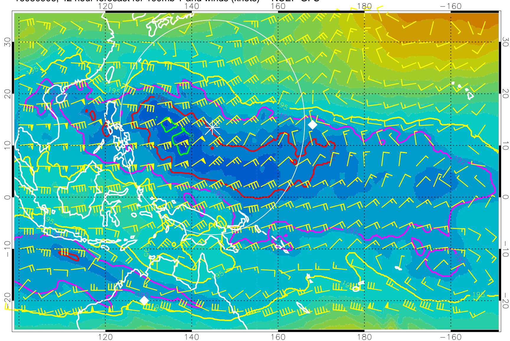
16080906, 42 hour forecast for 100mb T and winds (knots) -- NCEP GFS
