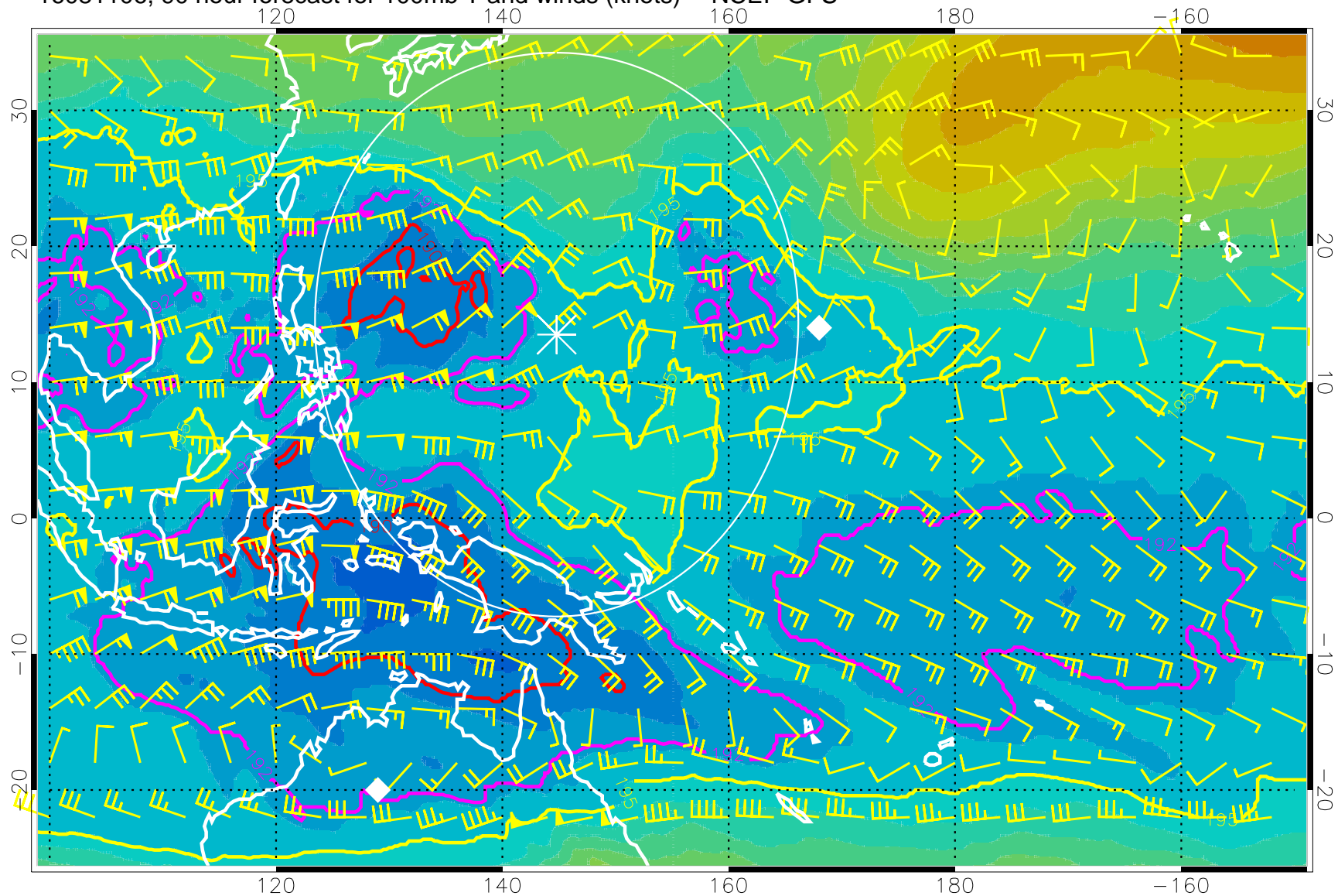
16081106, 90 hour forecast for 100mb T and winds (knots) -- NCEP GFS
