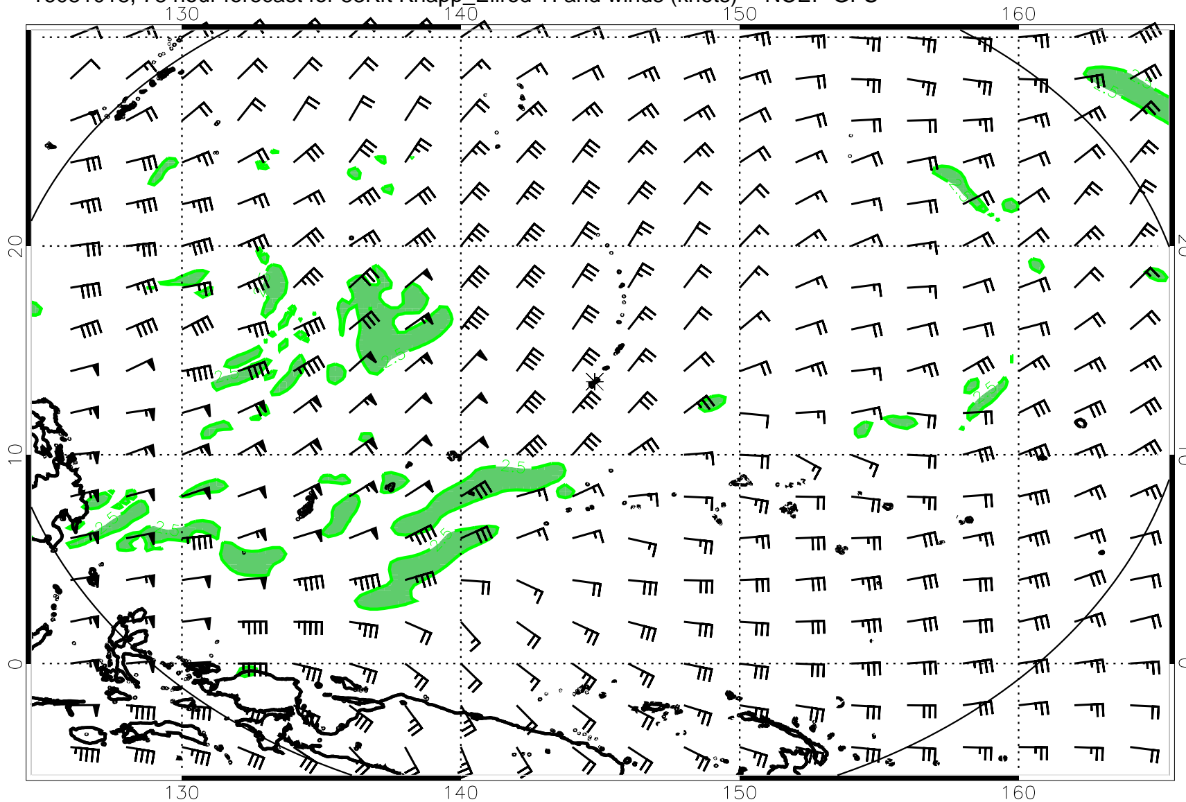
16081018, 78 hour forecast for 53Kft Knapp_Ellrod TI and winds (knots) -- NCEP GFS
