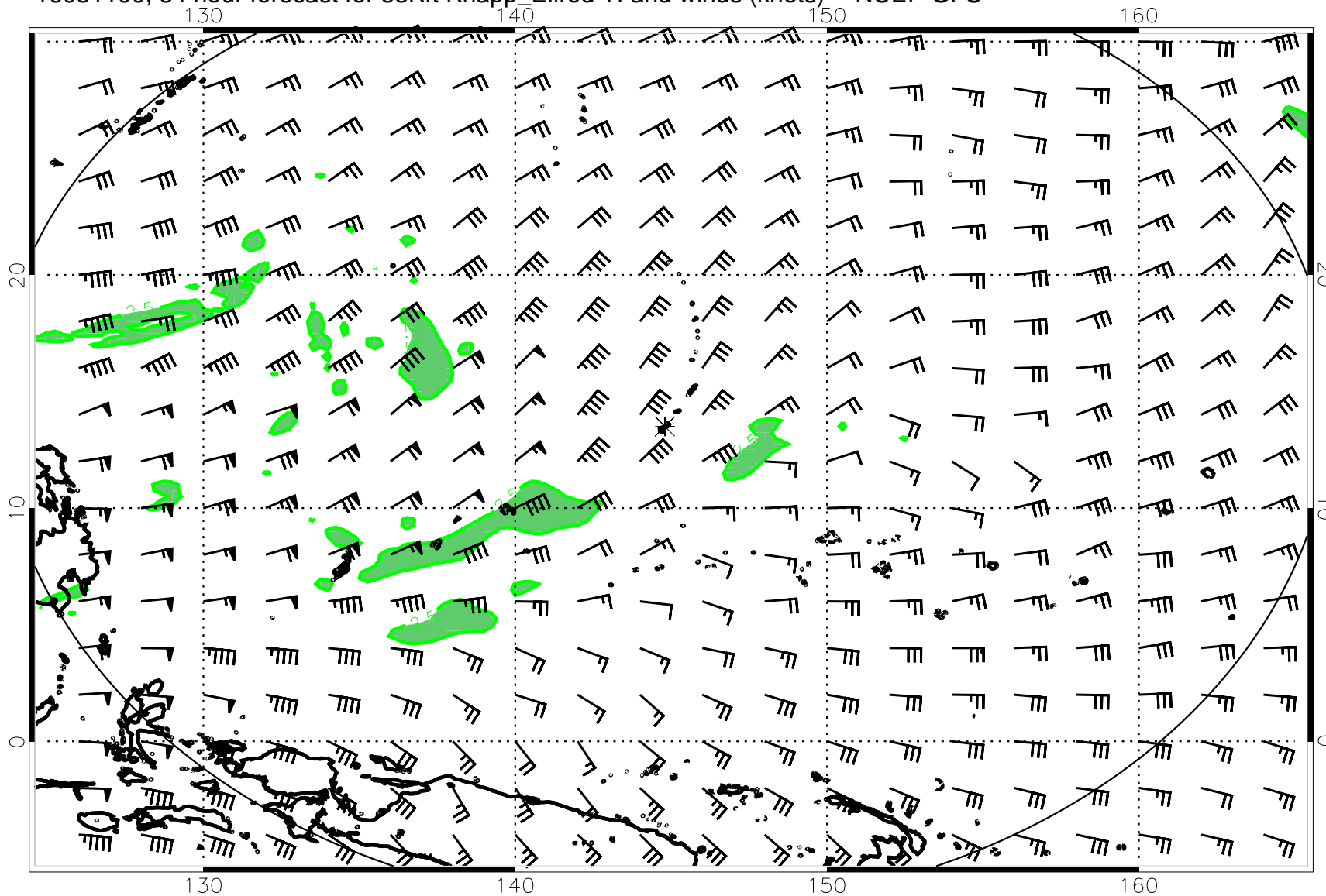
16081100, 84 hour forecast for 53Kft Knapp_Ellrod TI and winds (knots) -- NCEP GFS
