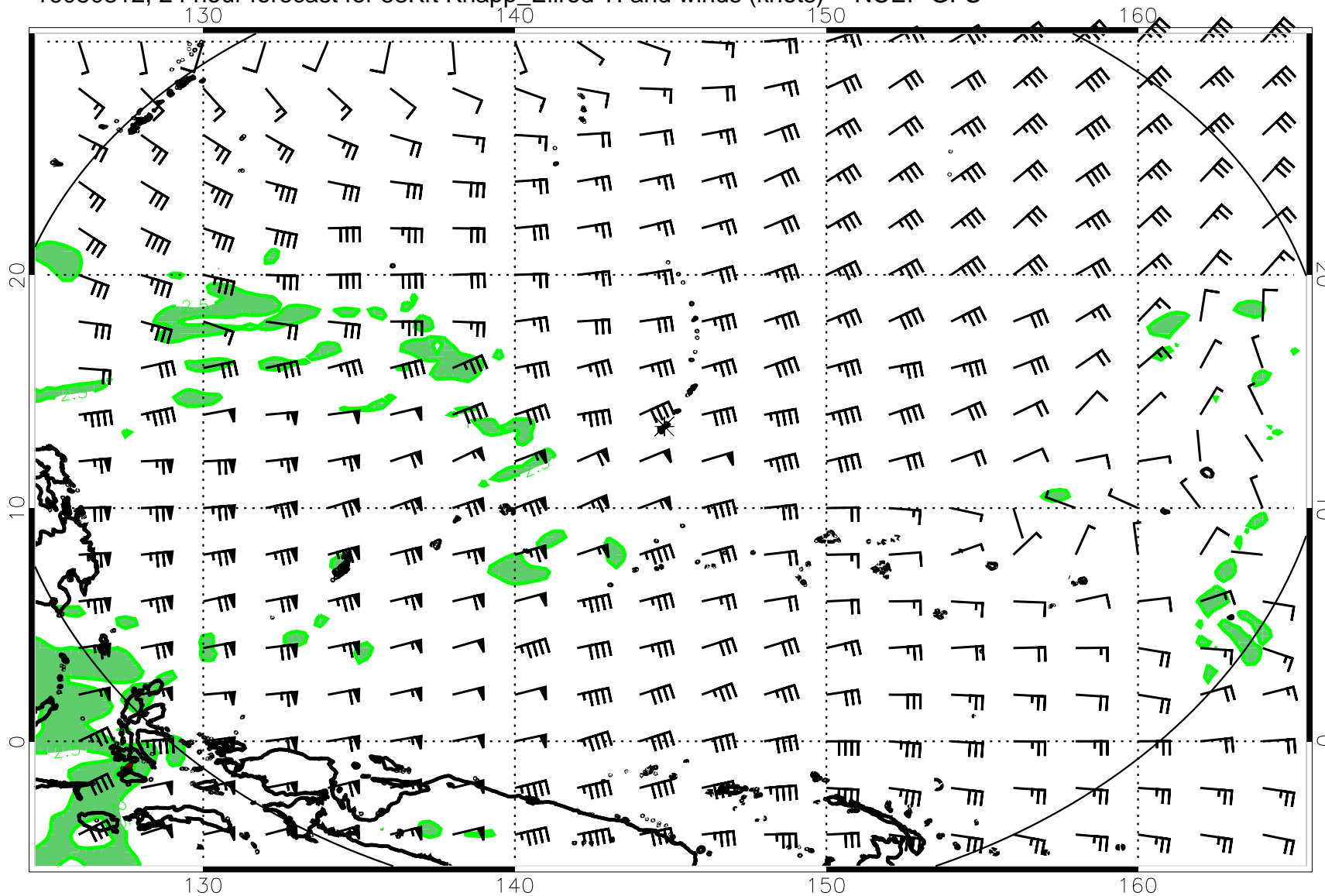
16080812, 24 hour forecast for 53Kft Knapp_Ellrod TI and winds (knots) -- NCEP GFS
