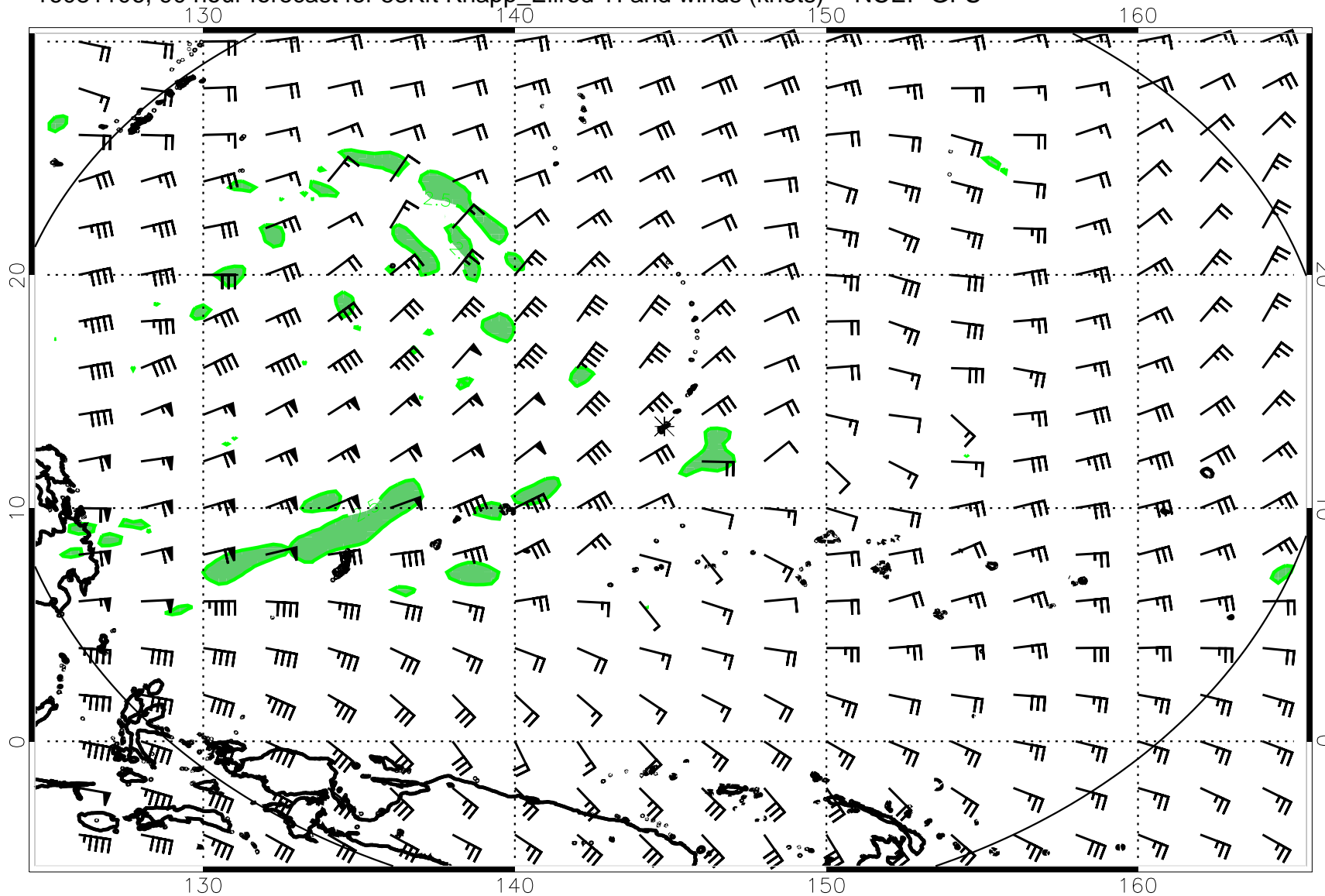
16081106, 90 hour forecast for 53Kft Knapp_Ellrod TI and winds (knots) -- NCEP GFS
