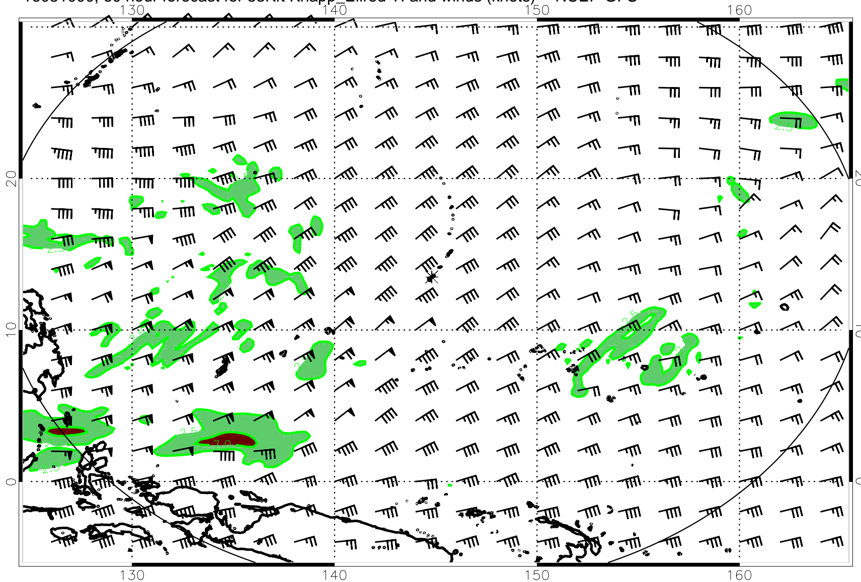
16081000, 60 hour forecast for 53Kft Knapp_Ellrod TI and winds (knots) -- NCEP GFS
