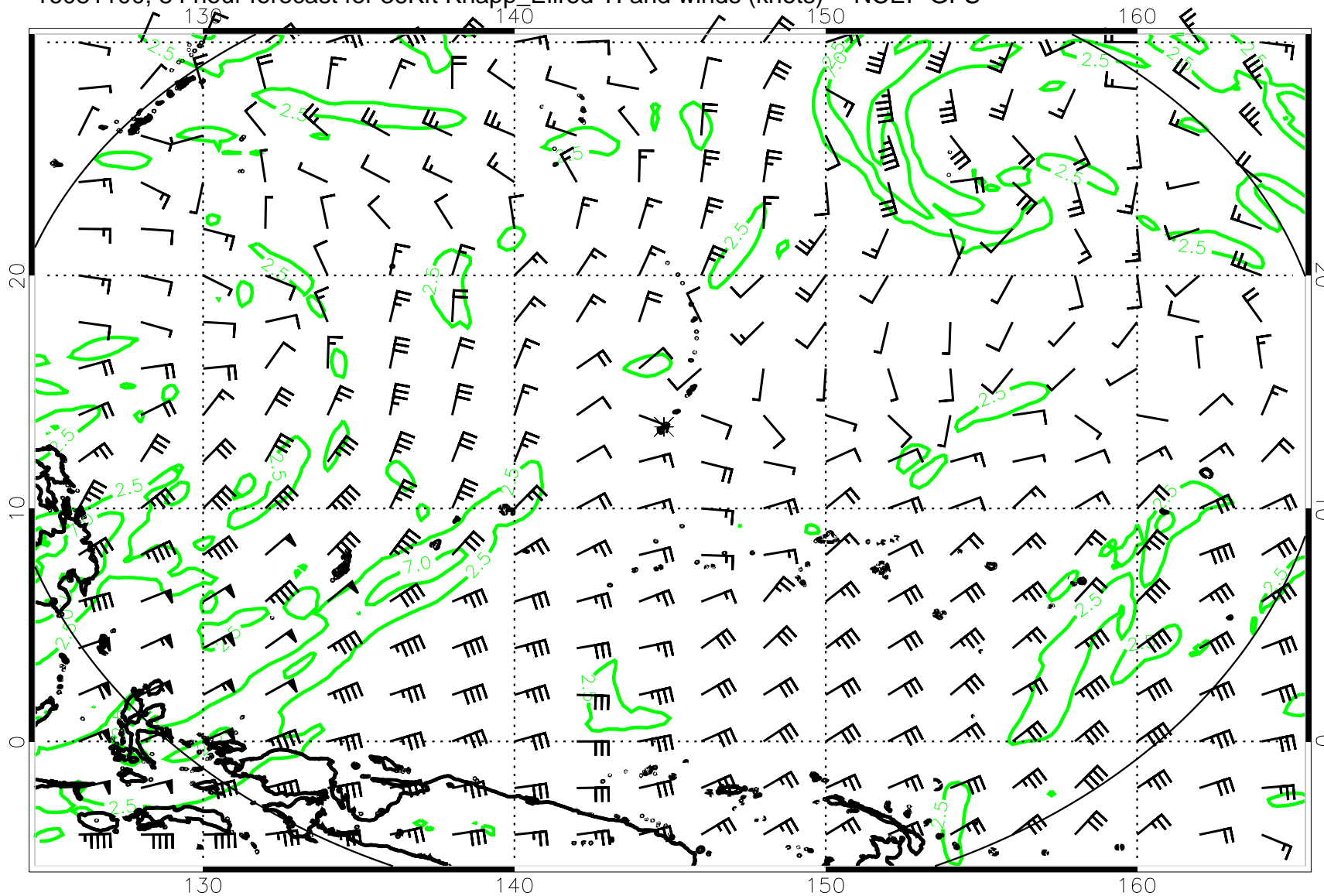
16081100, 84 hour forecast for 36Kft Knapp_Ellrod TI and winds (knots) -- NCEP GFS
