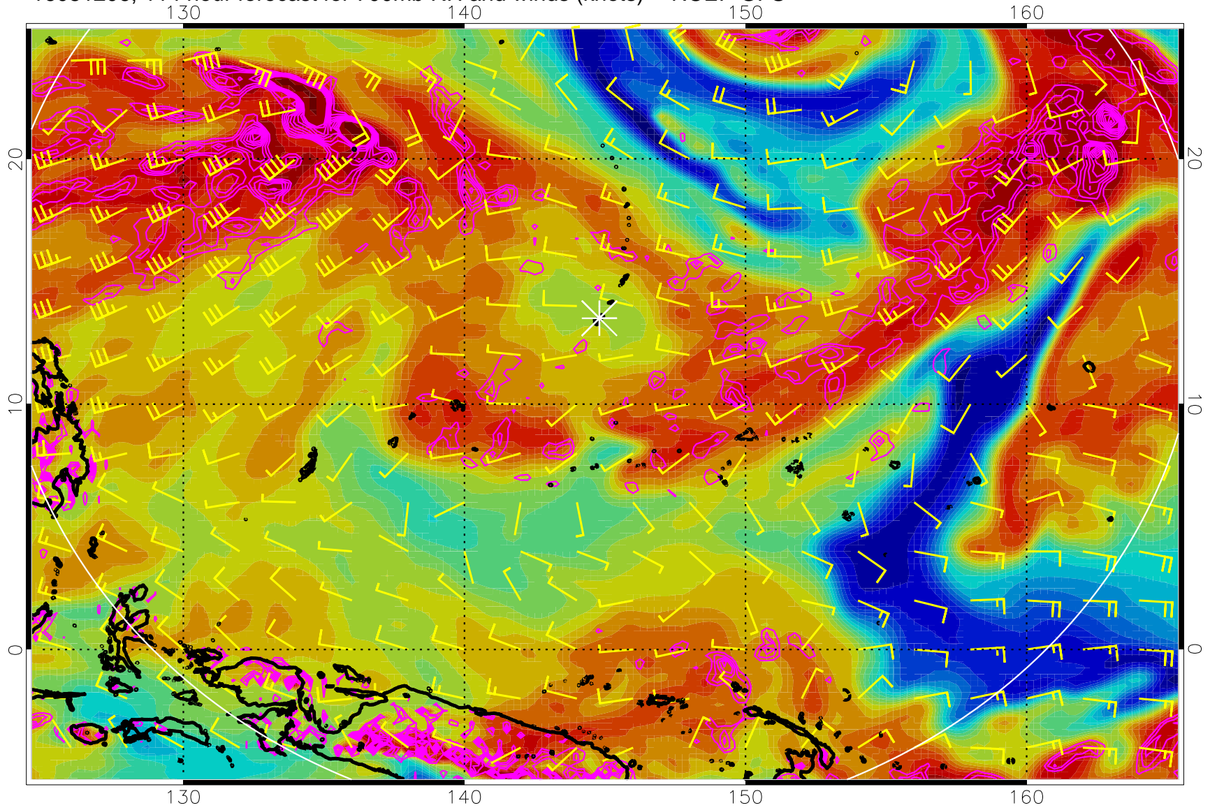
16081206, 114 hour forecast for 700mb RH and winds (knots) -- NCEP GFS
