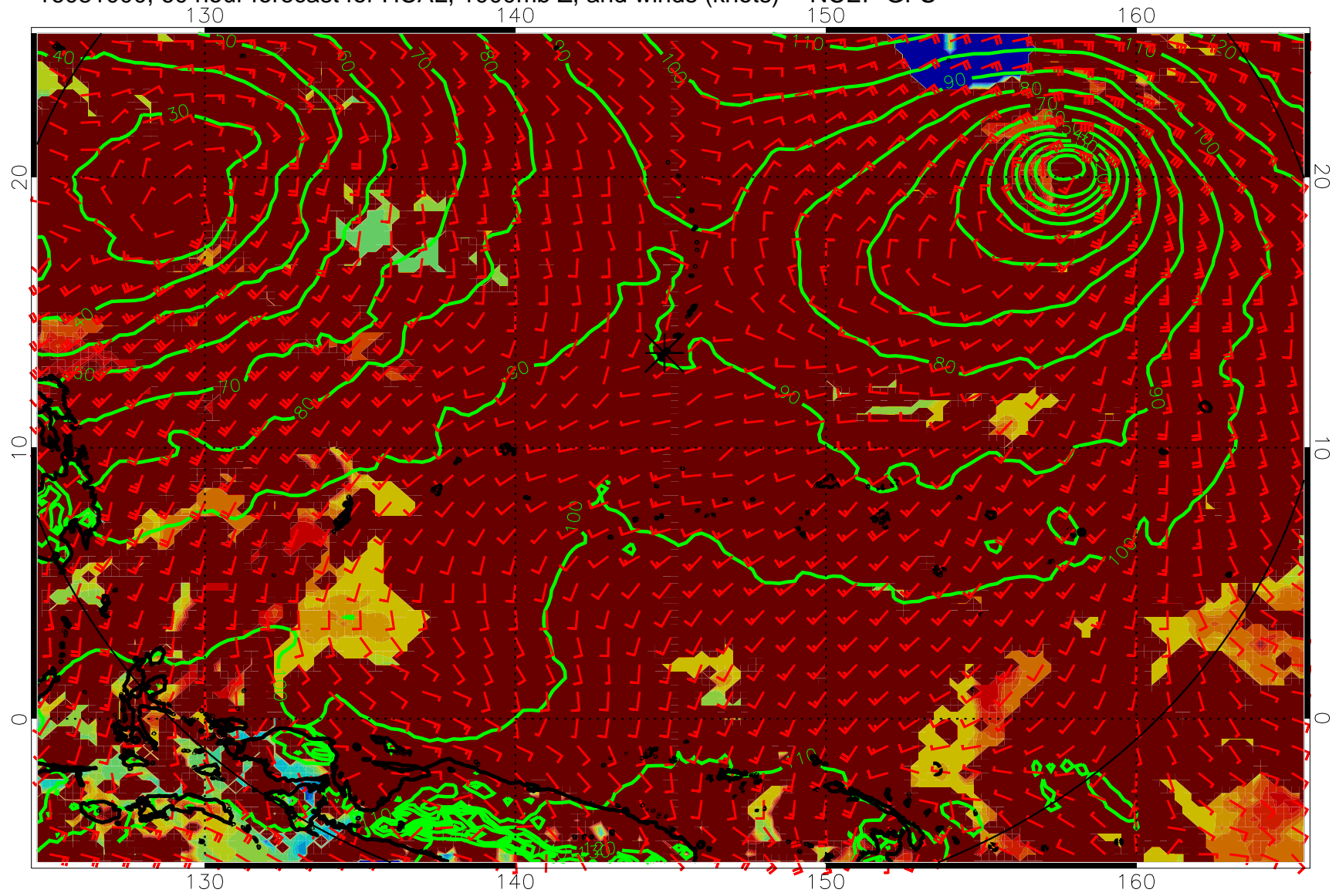
16081000, 60 hour forecast for HCAL, 1000mb Z, and winds (knots) -- NCEP GFS
