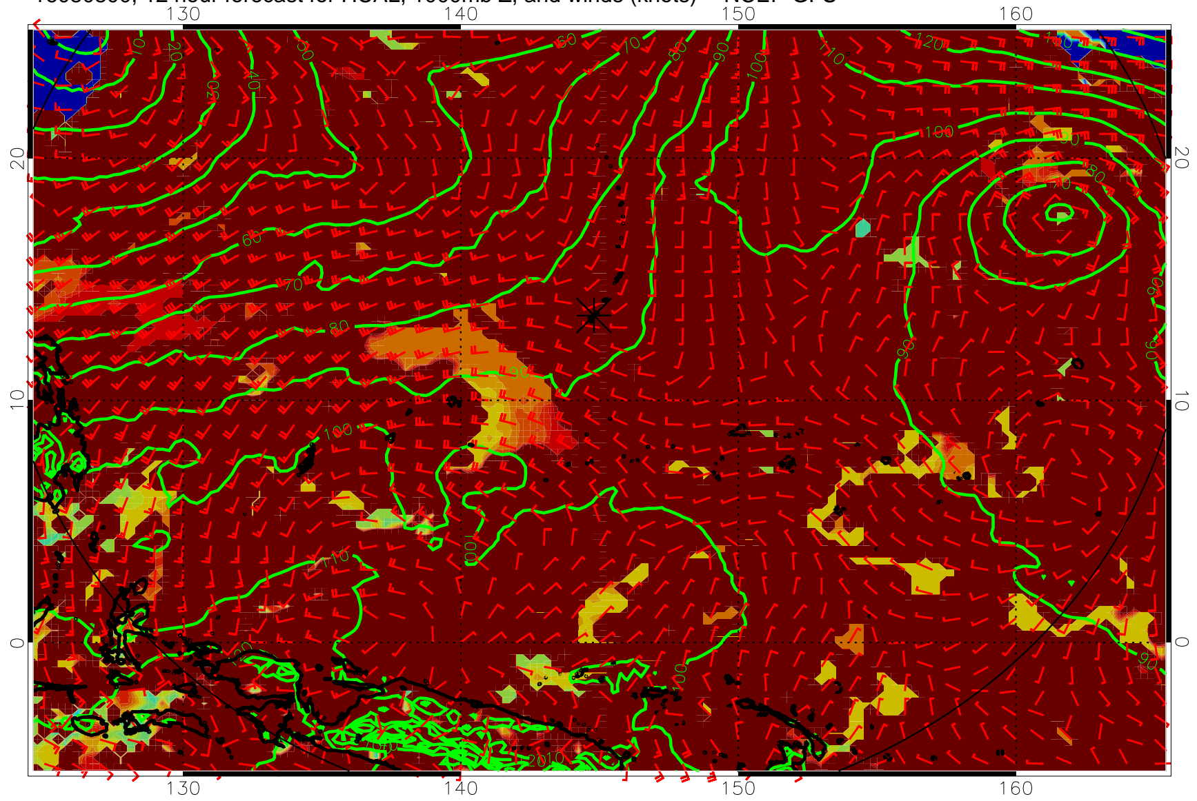
16080800, 12 hour forecast for HCAL, 1000mb Z, and winds (knots) -- NCEP GFS
