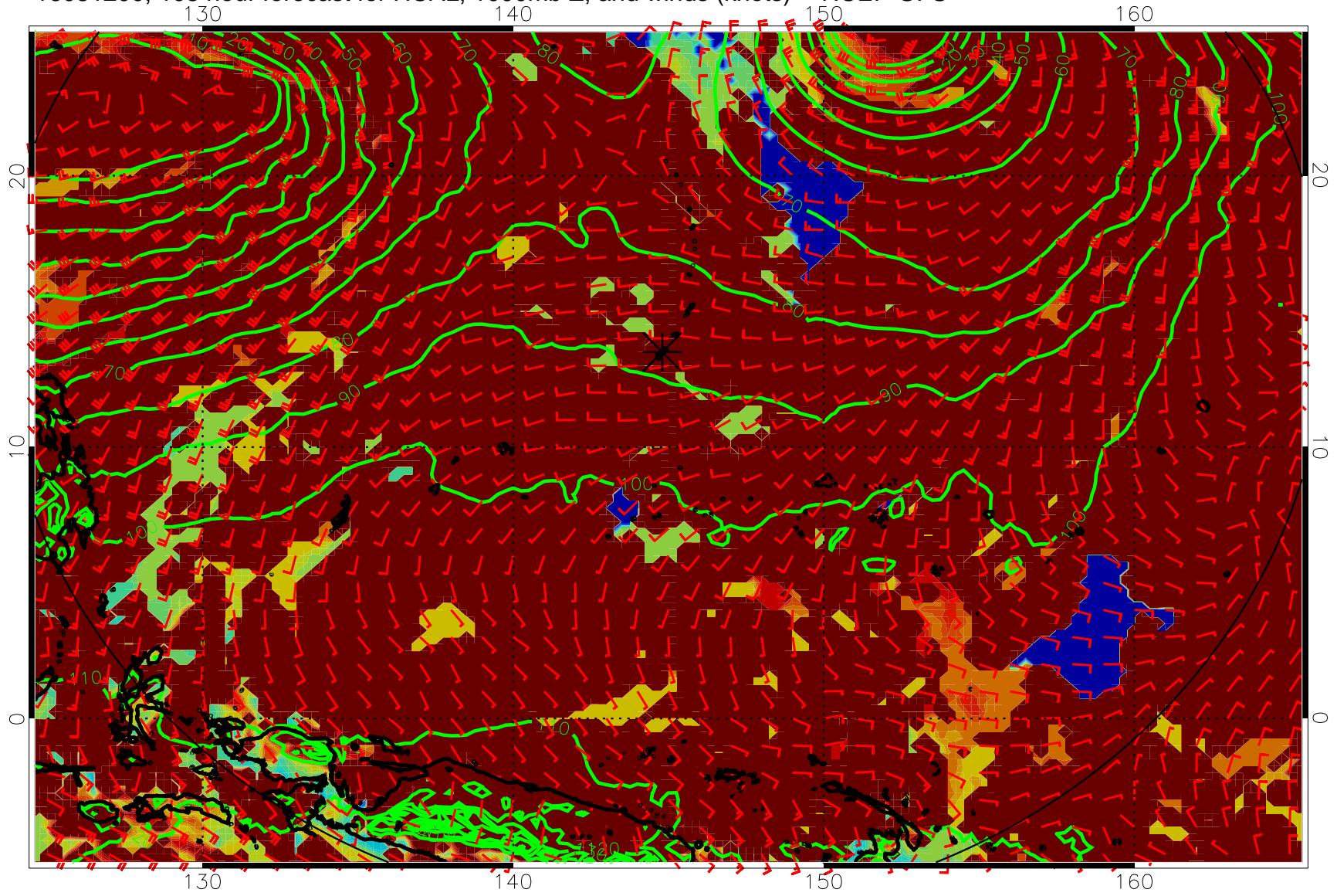
16081200, 108 hour forecast for HCAL, 1000mb Z, and winds (knots) -- NCEP GFS
