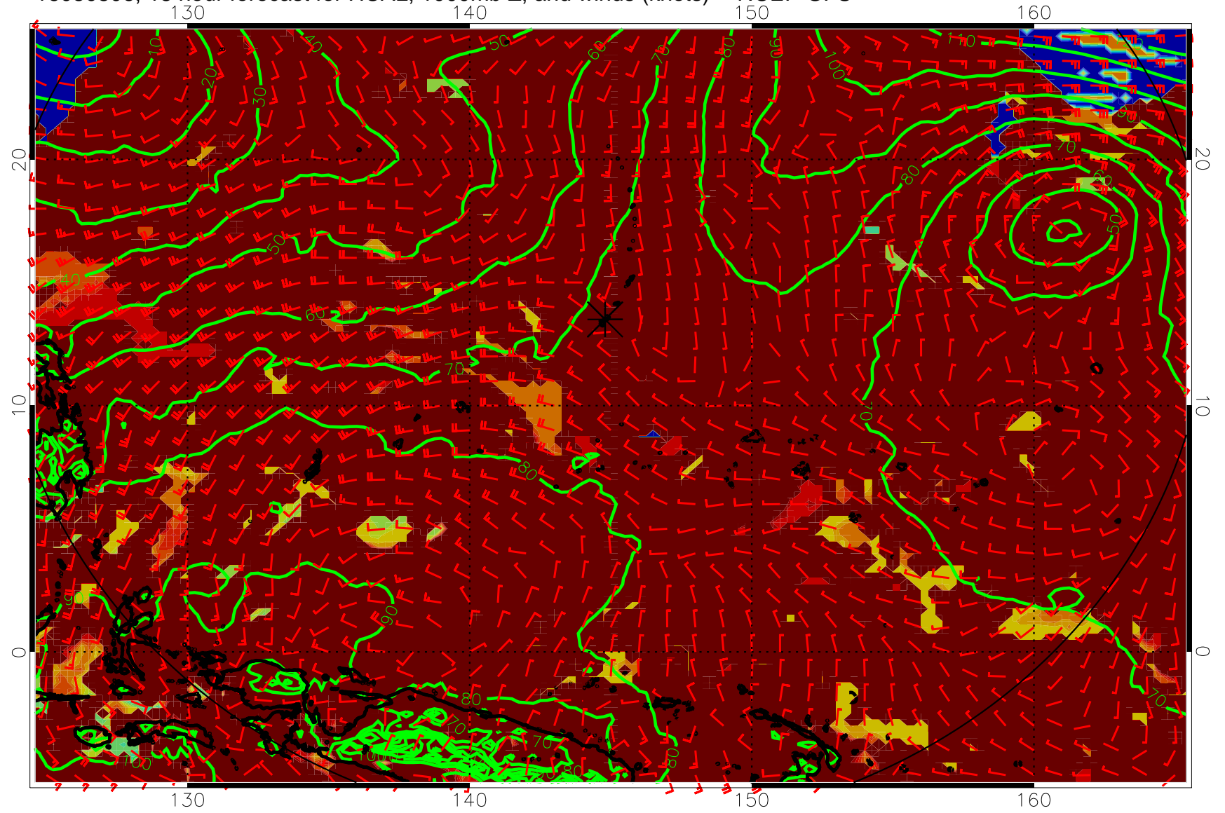
16080806, 18 hour forecast for HCAL, 1000mb Z, and winds (knots) -- NCEP GFS
