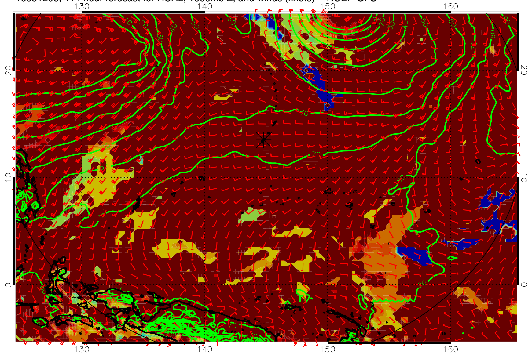
16081206, 114 hour forecast for HCAL, 1000mb Z, and winds (knots) -- NCEP GFS
