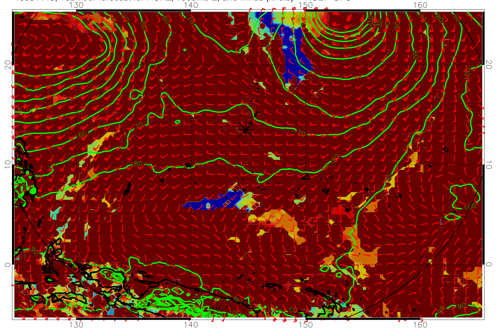
16081118, 102 hour forecast for HCAL, 1000mb Z, and winds (knots) -- NCEP GFS
