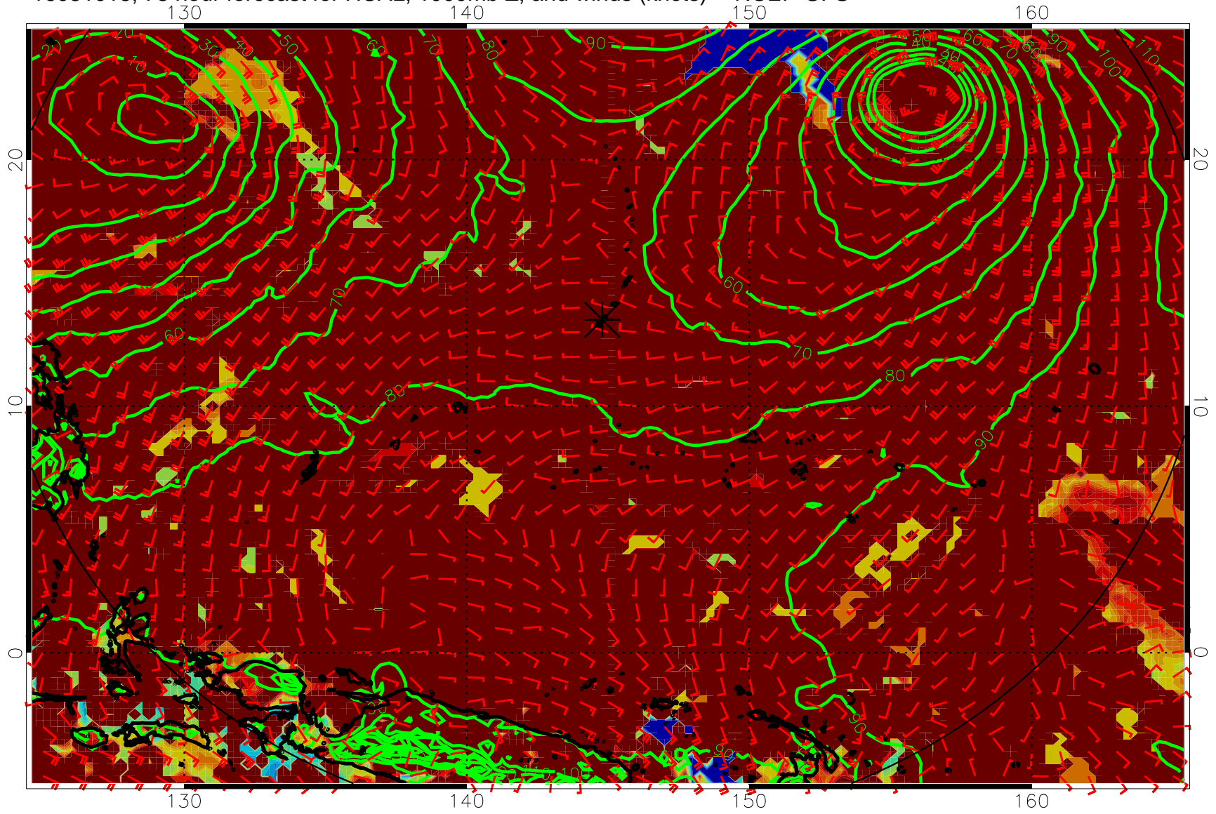
16081018, 78 hour forecast for HCAL, 1000mb Z, and winds (knots) -- NCEP GFS
