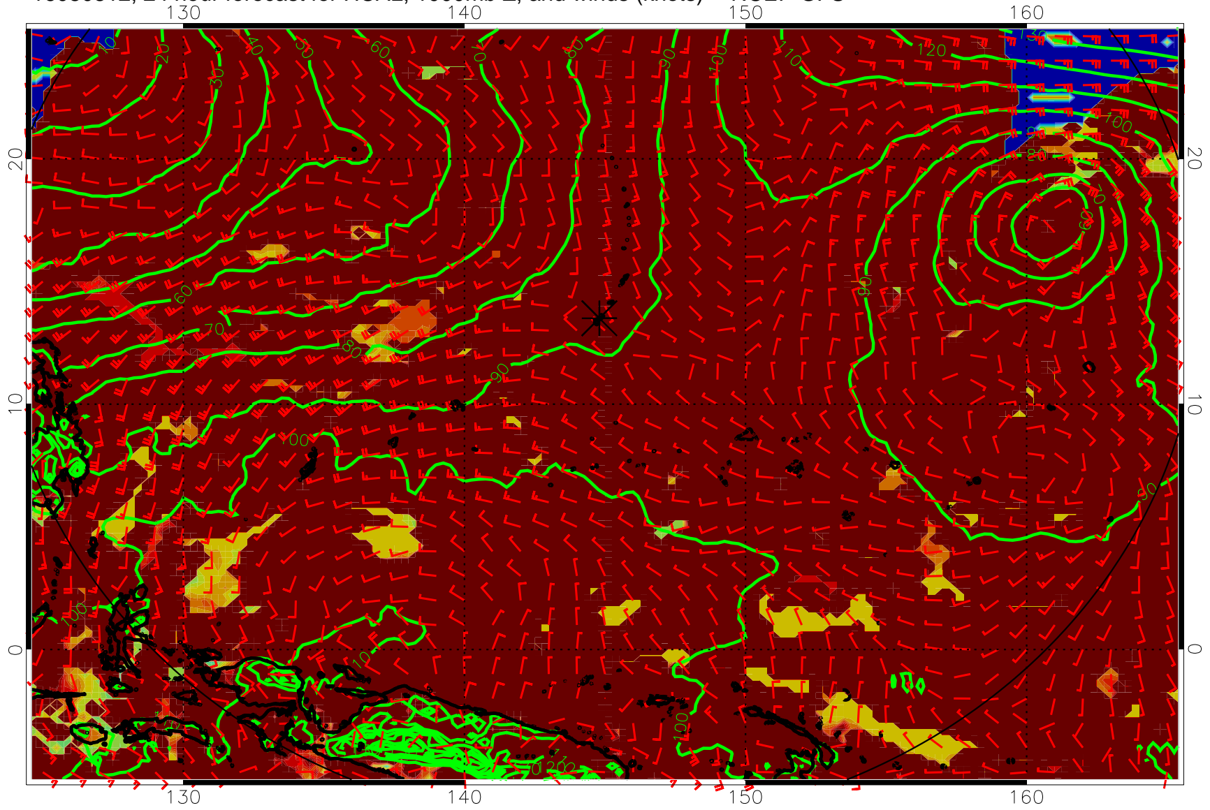
16080812, 24 hour forecast for HCAL, 1000mb Z, and winds (knots) -- NCEP GFS
