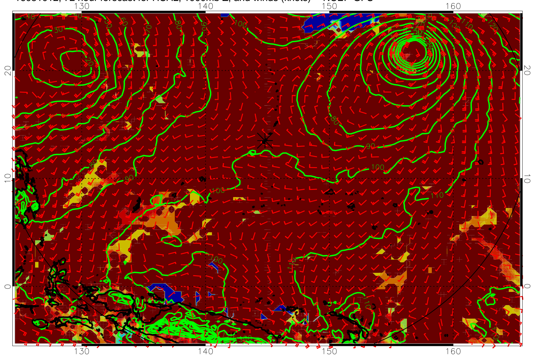
16081012, 72 hour forecast for HCAL, 1000mb Z, and winds (knots) -- NCEP GFS
