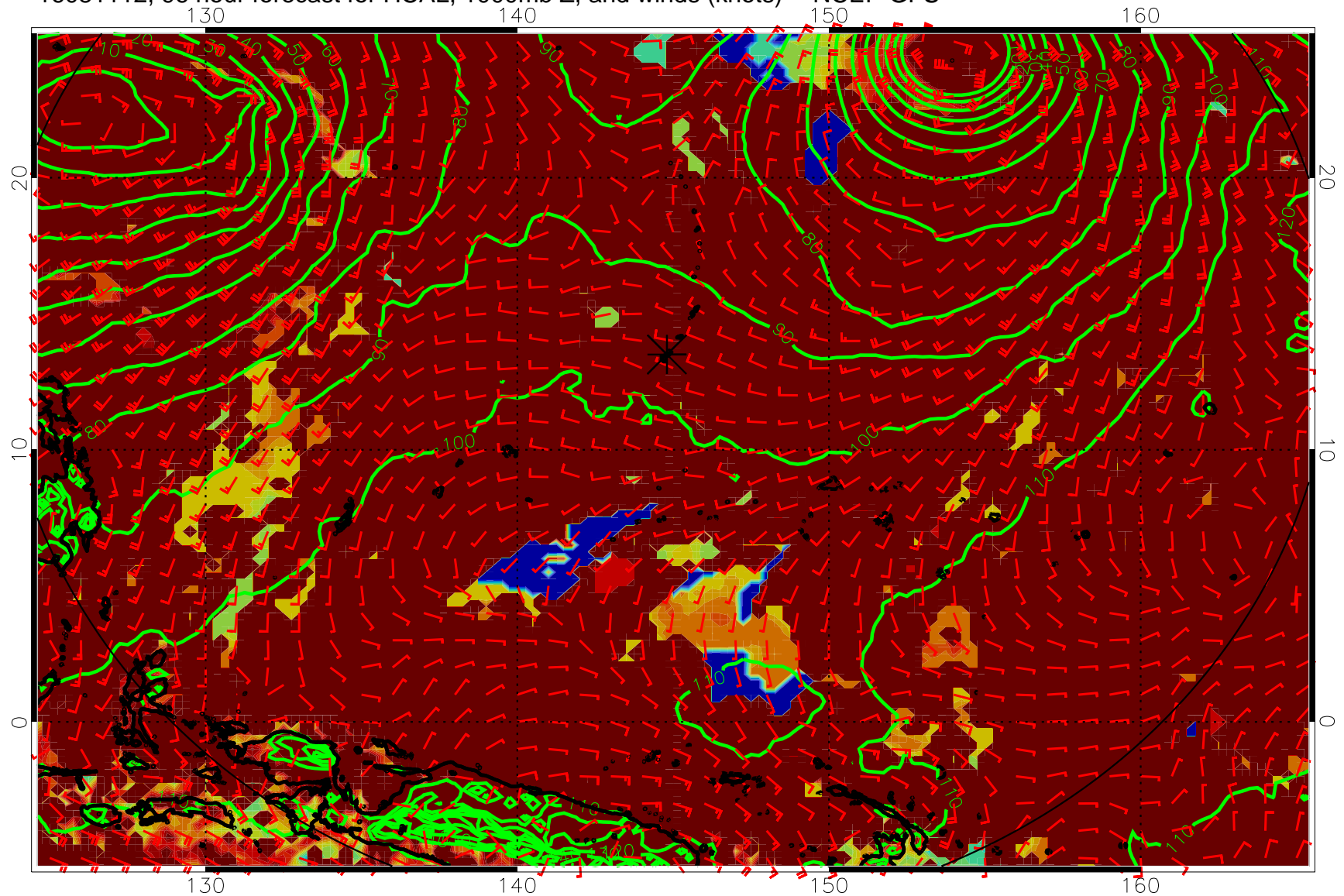
16081112, 96 hour forecast for HCAL, 1000mb Z, and winds (knots) -- NCEP GFS
