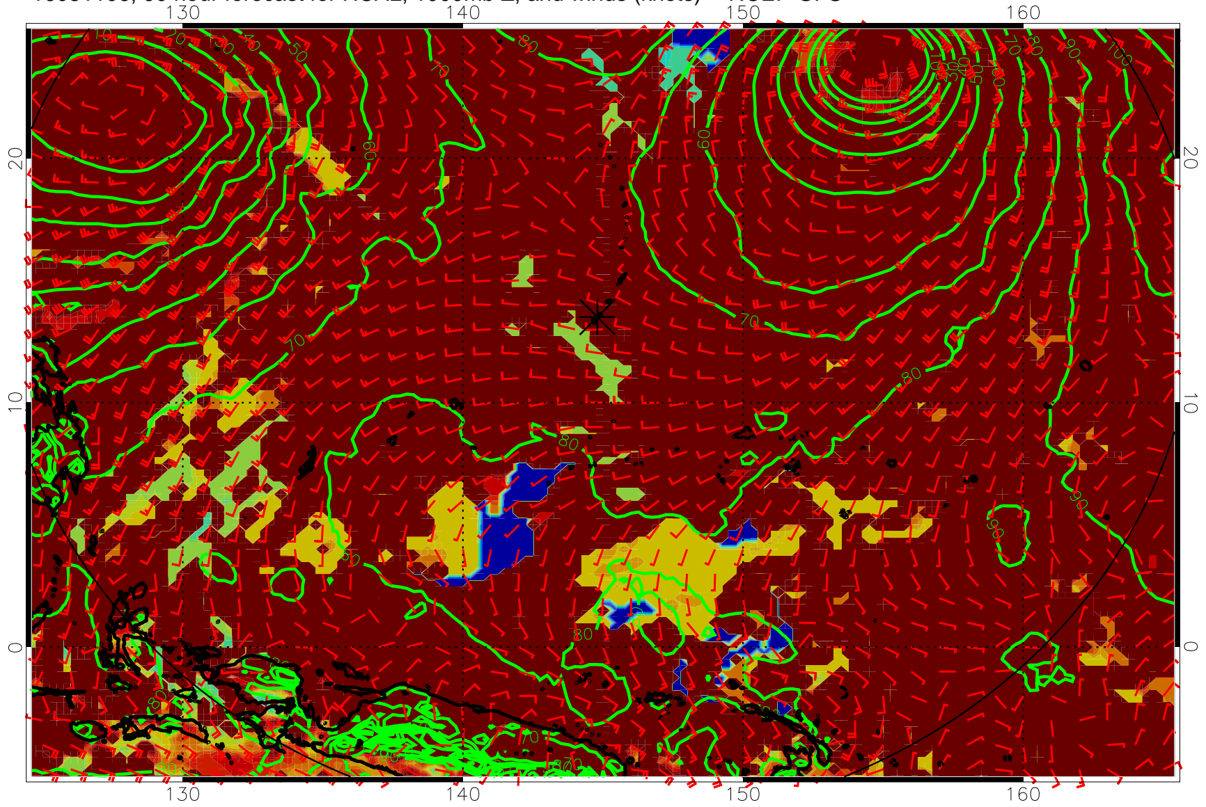
16081106, 90 hour forecast for HCAL, 1000mb Z, and winds (knots) -- NCEP GFS
