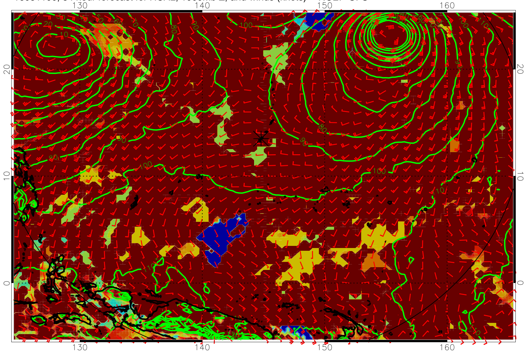
16081100, 84 hour forecast for HCAL, 1000mb Z, and winds (knots) -- NCEP GFS
