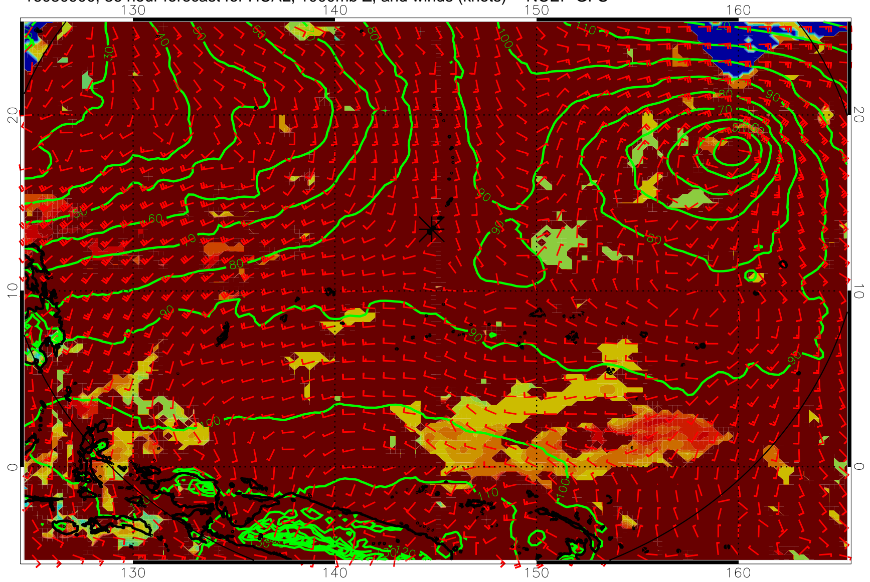
16080900, 36 hour forecast for HCAL, 1000mb Z, and winds (knots) -- NCEP GFS
