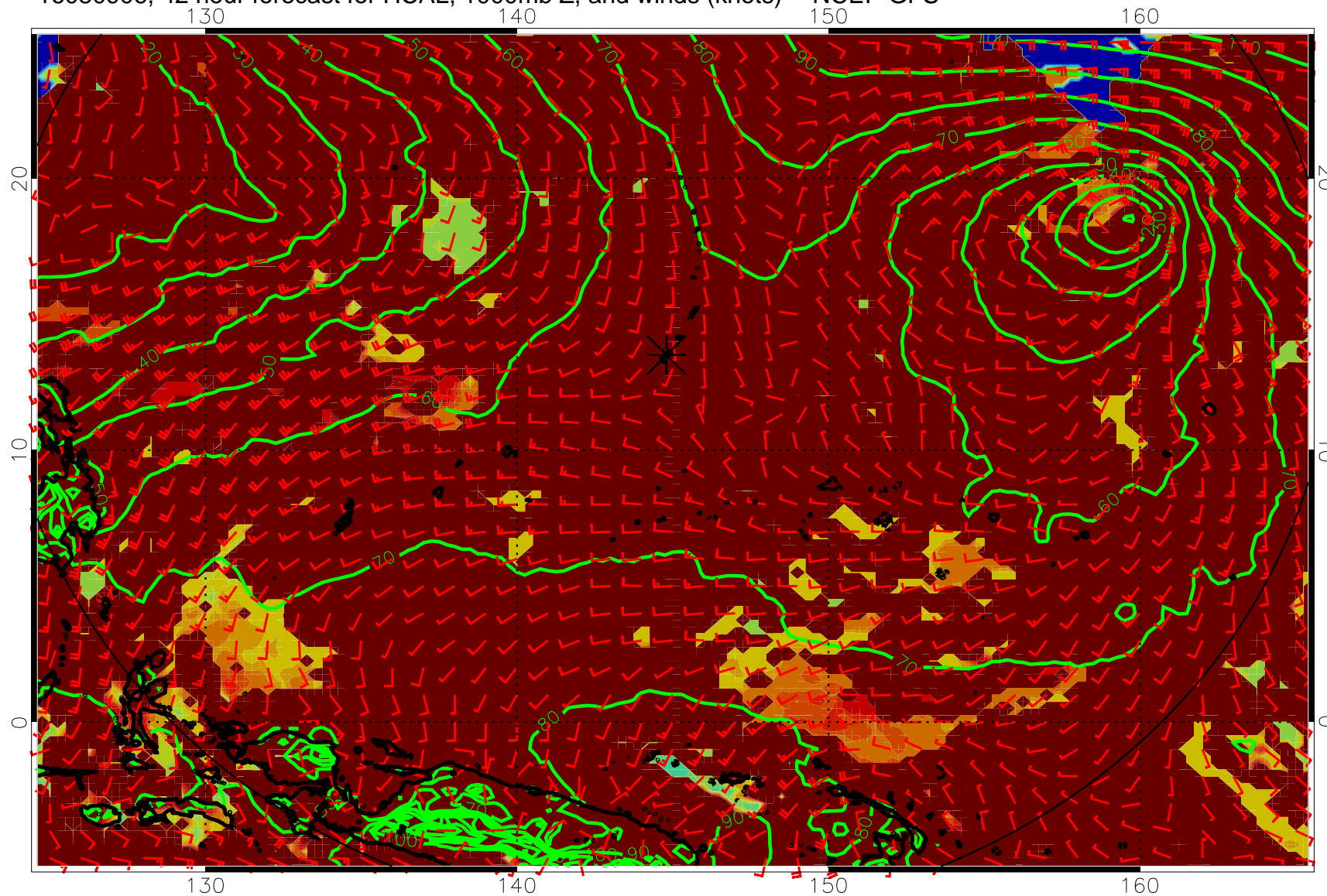
16080906, 42 hour forecast for HCAL, 1000mb Z, and winds (knots) -- NCEP GFS
