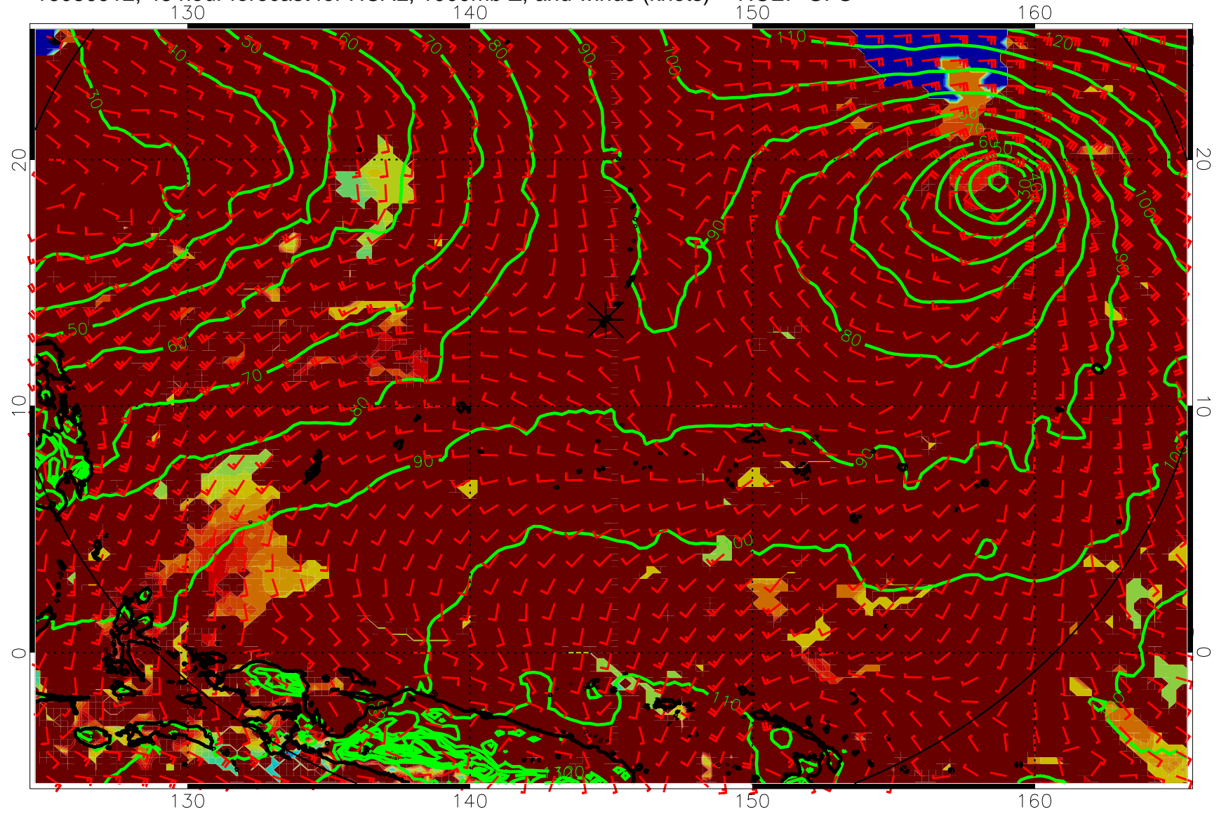
16080912, 48 hour forecast for HCAL, 1000mb Z, and winds (knots) -- NCEP GFS
