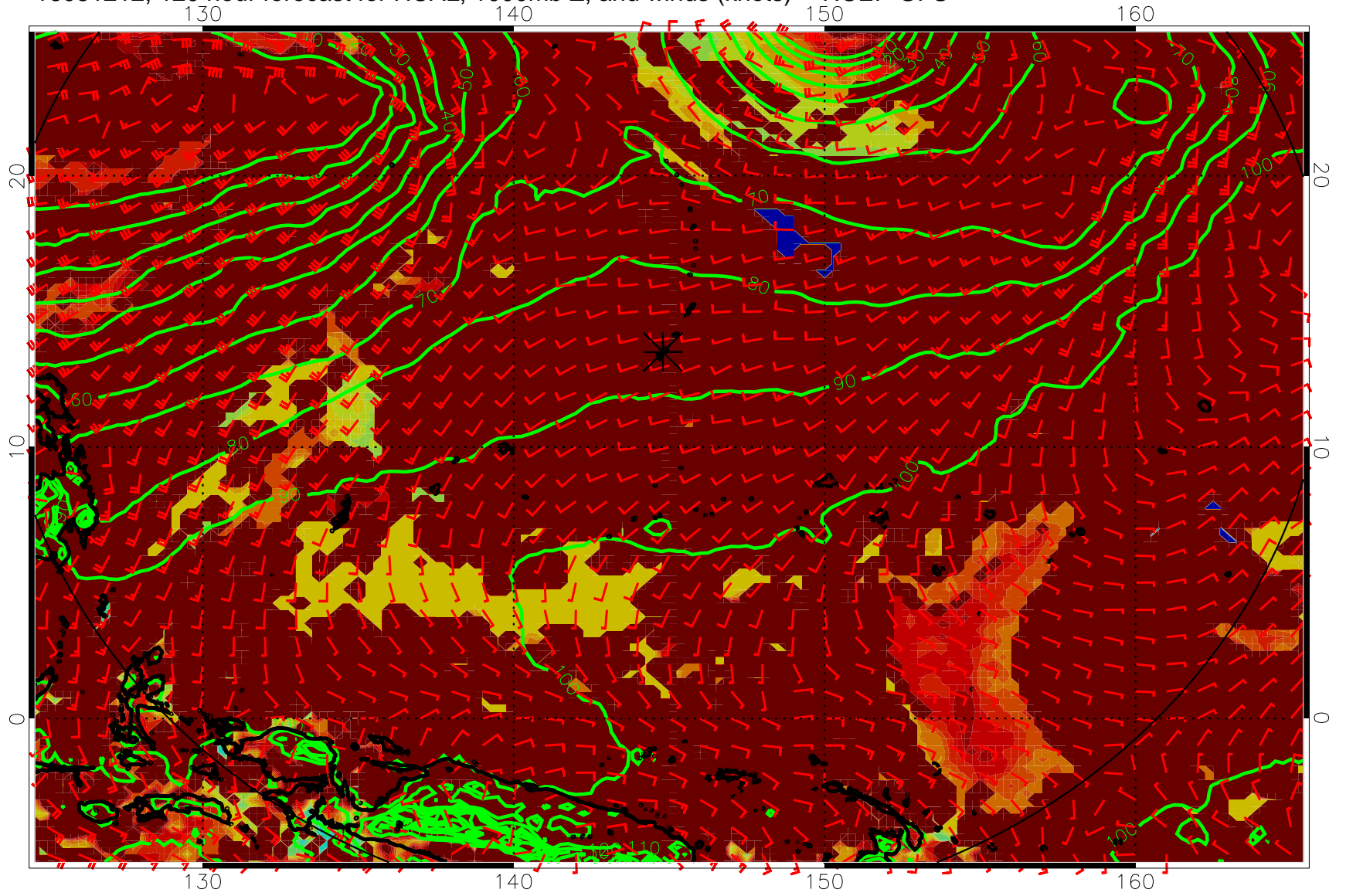
16081212, 120 hour forecast for HCAL, 1000mb Z, and winds (knots) -- NCEP GFS
