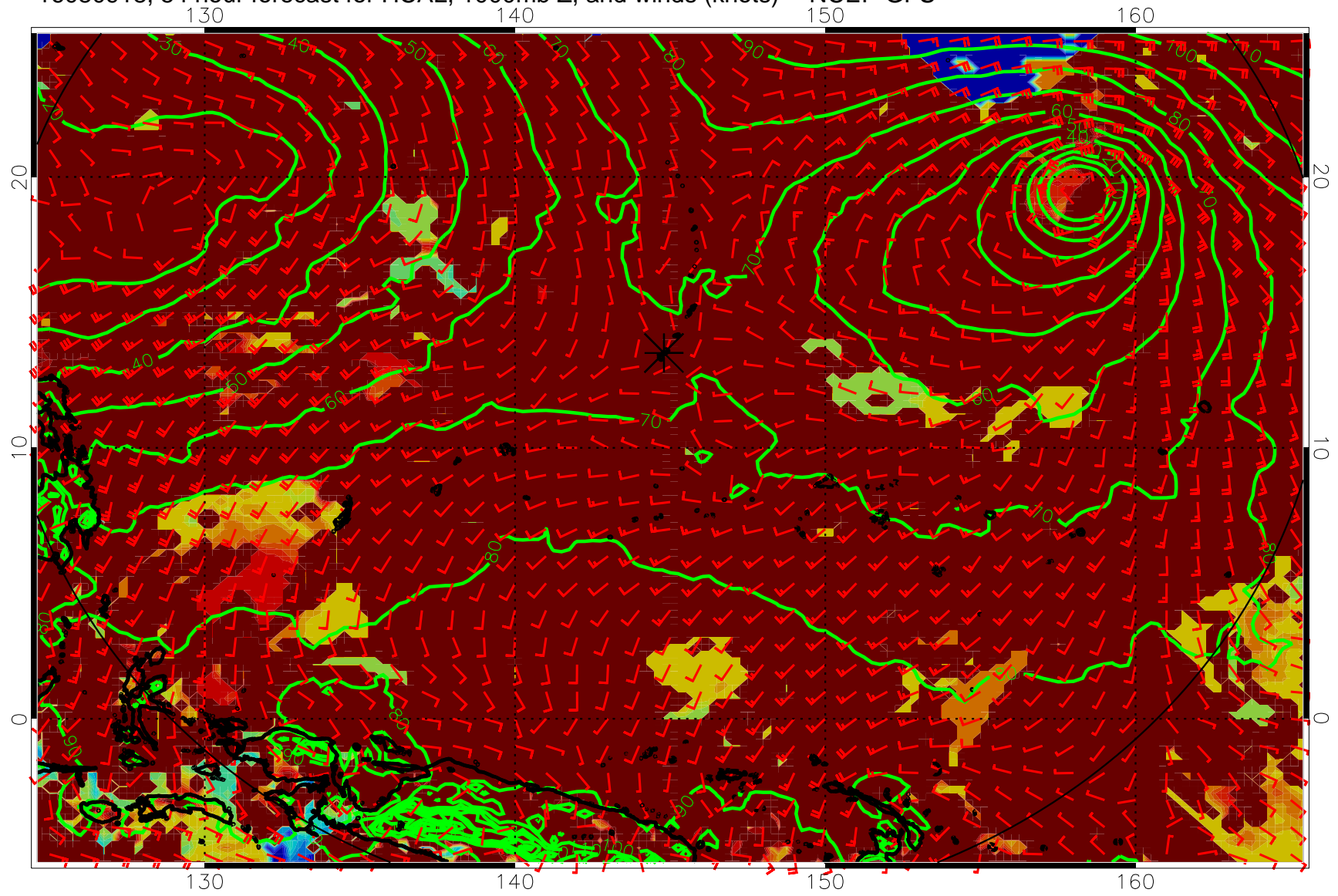
16080918, 54 hour forecast for HCAL, 1000mb Z, and winds (knots) -- NCEP GFS
