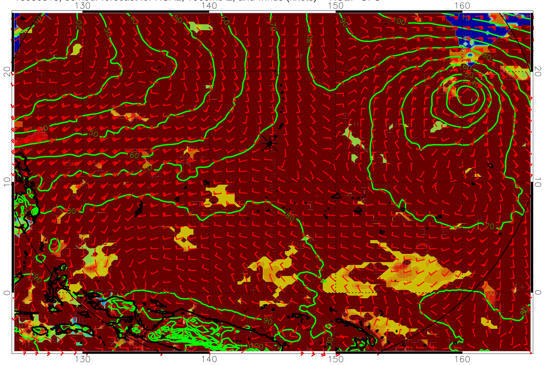
16080818, 30 hour forecast for HCAL, 1000mb Z, and winds (knots) -- NCEP GFS
