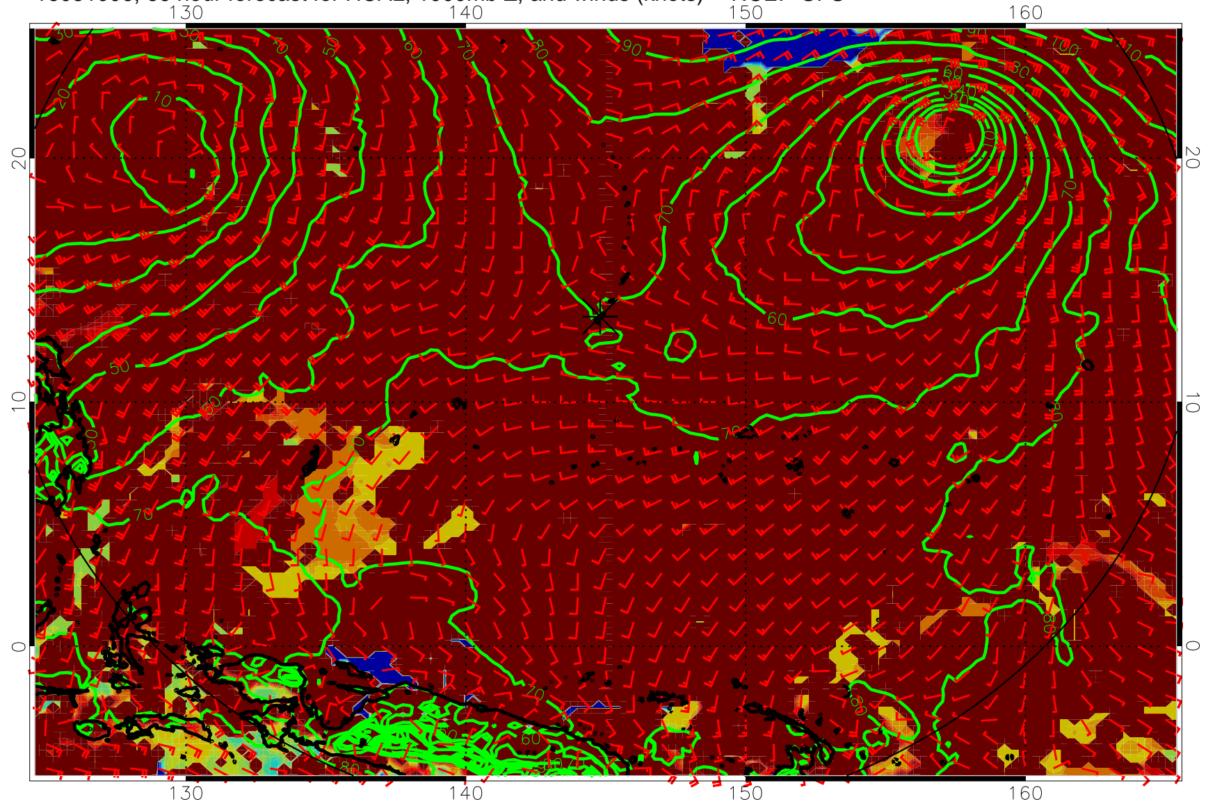
16081006, 66 hour forecast for HCAL, 1000mb Z, and winds (knots) -- NCEP GFS
