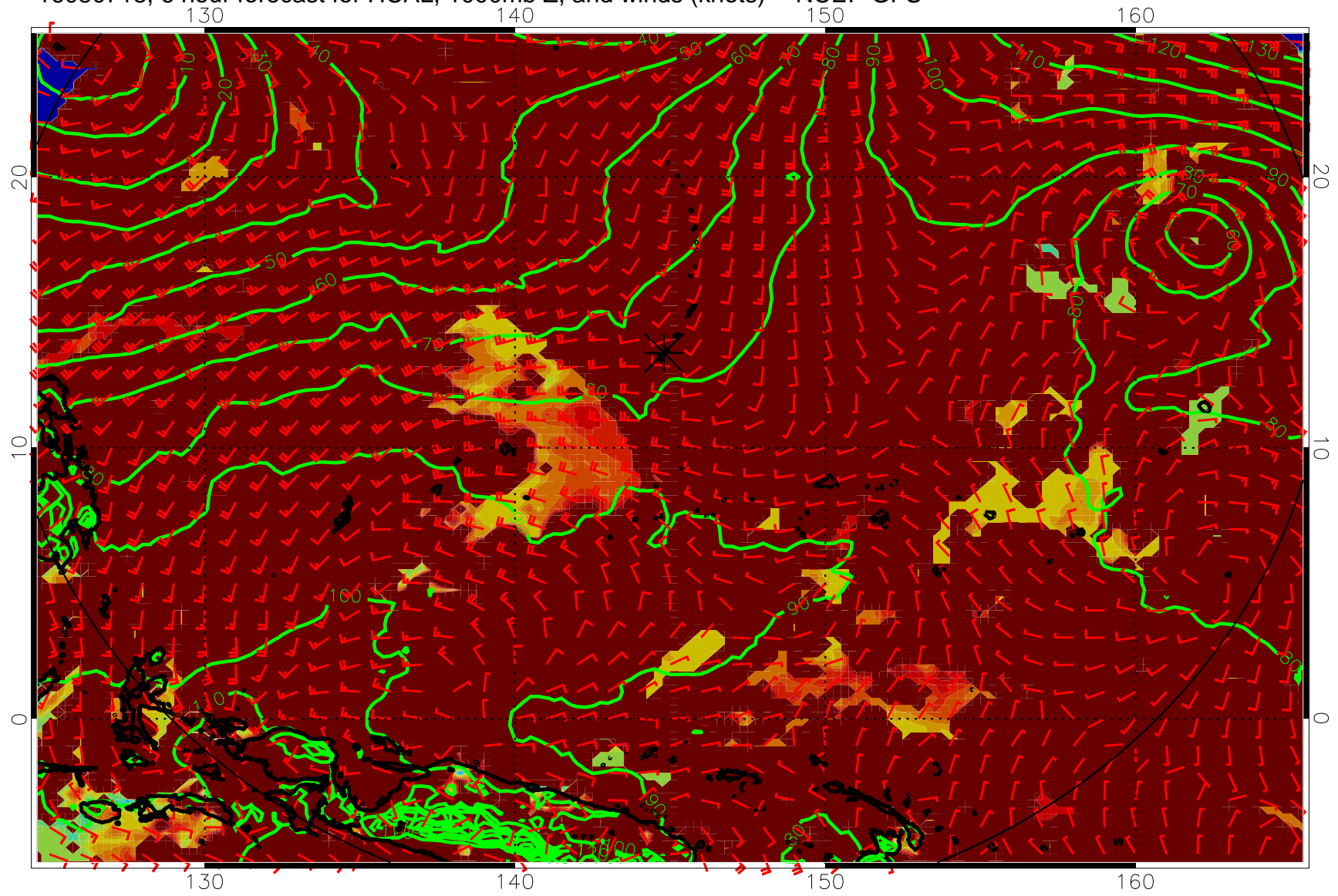
16080718, 6 hour forecast for HCAL, 1000mb Z, and winds (knots) -- NCEP GFS
