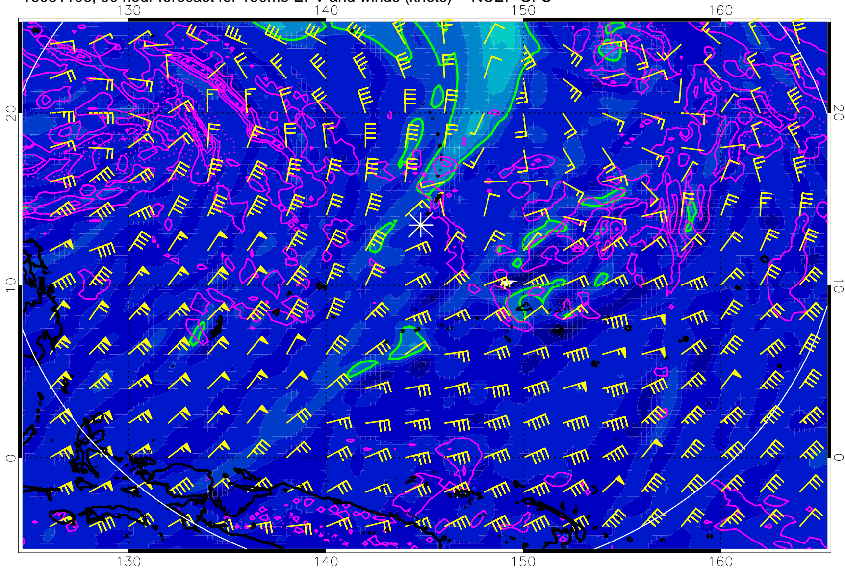
16081106, 90 hour forecast for 150mb EPV and winds (knots) -- NCEP GFS
