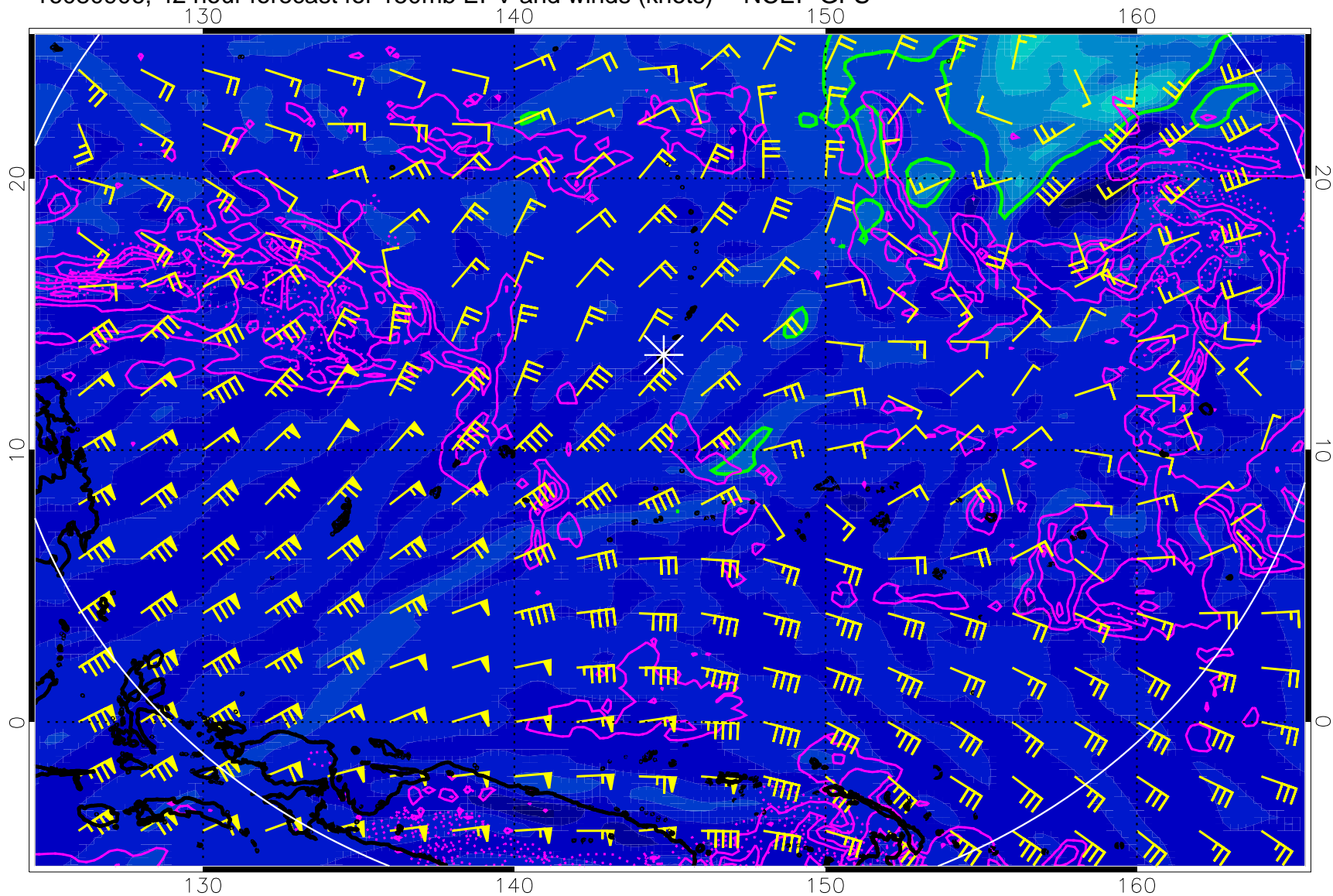
16080906, 42 hour forecast for 150mb EPV and winds (knots) -- NCEP GFS
