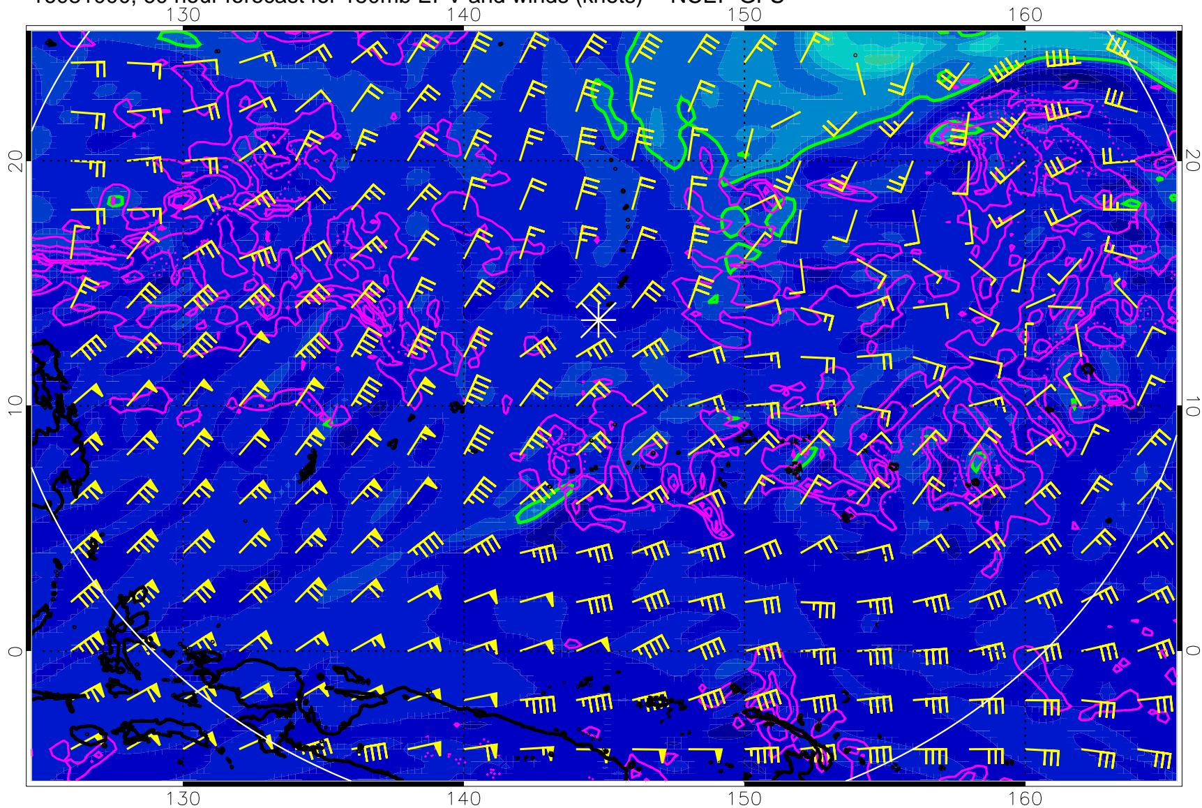
16081000, 60 hour forecast for 150mb EPV and winds (knots) -- NCEP GFS
