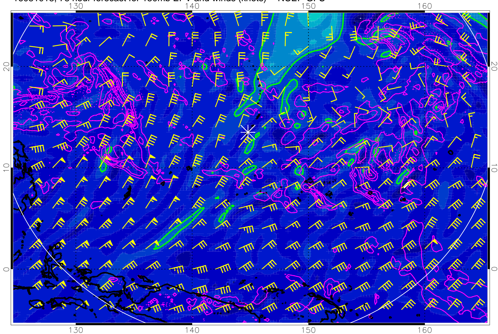
16081018, 78 hour forecast for 150mb EPV and winds (knots) -- NCEP GFS
