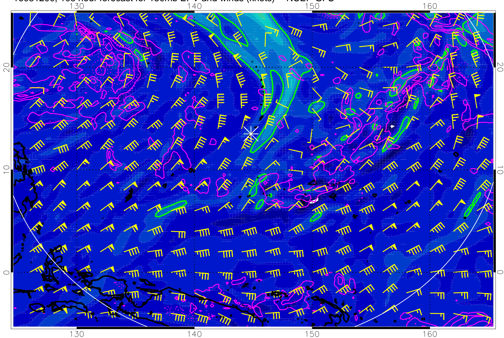
16081200, 108 hour forecast for 150mb EPV and winds (knots) -- NCEP GFS
