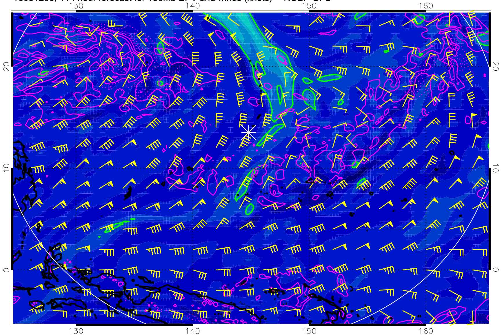
16081206, 114 hour forecast for 150mb EPV and winds (knots) -- NCEP GFS
