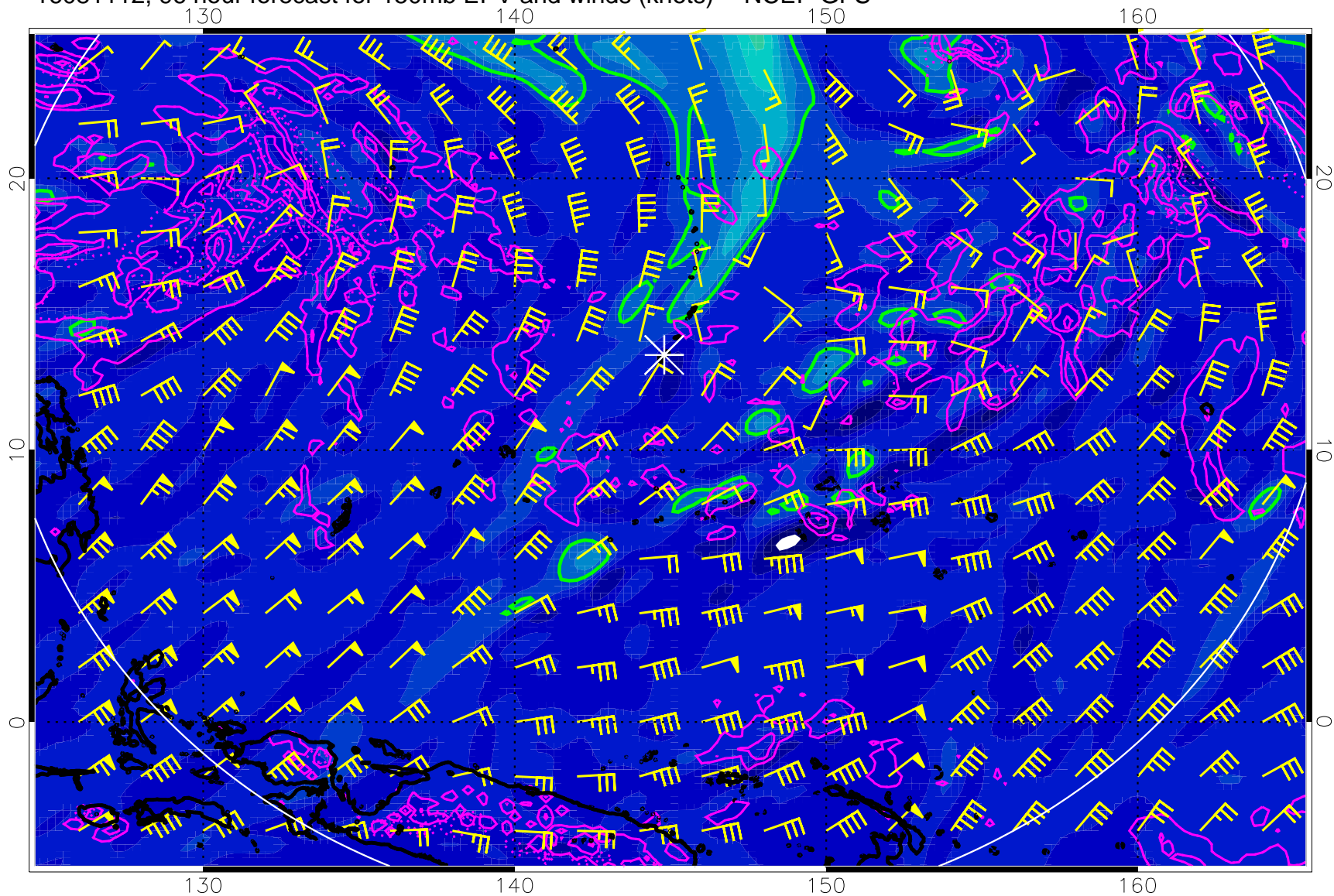
16081112, 96 hour forecast for 150mb EPV and winds (knots) -- NCEP GFS
