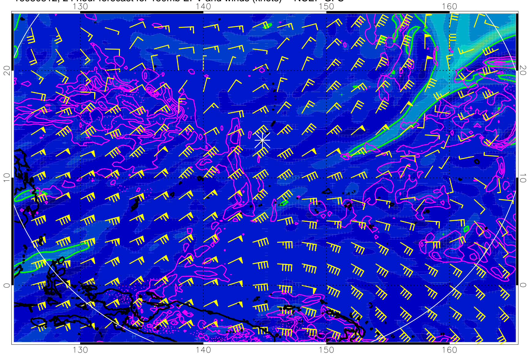
16080812, 24 hour forecast for 150mb EPV and winds (knots) -- NCEP GFS
