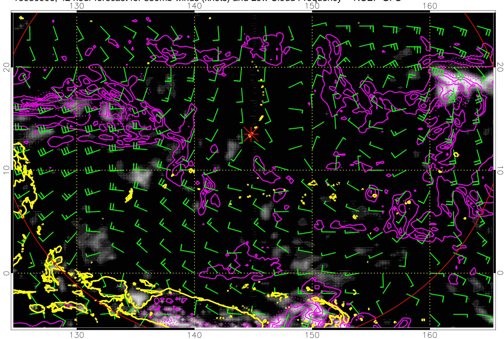
16080906, 42 hour forecast for 850mb winds (knots) and Low Cloud Frequency -- NCEP GFS
