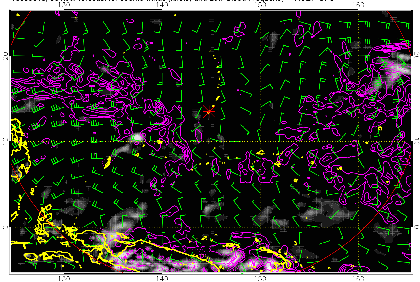
16080818, 30 hour forecast for 850mb winds (knots) and Low Cloud Frequency -- NCEP GFS
