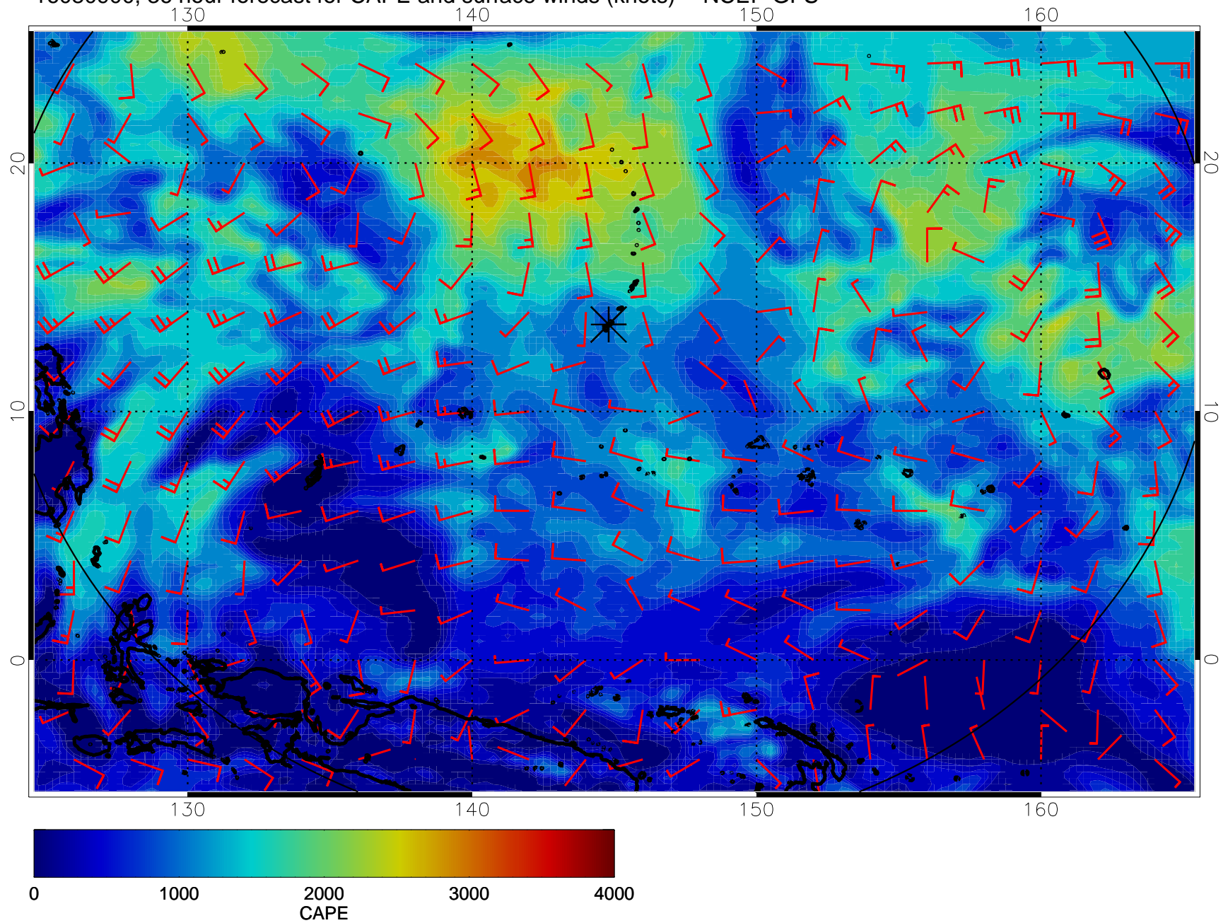
16080900, 36 hour forecast for CAPE and surface winds (knots) -- NCEP GFS
