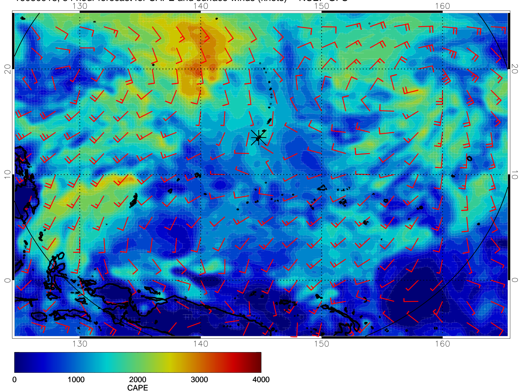
16080918, 54 hour forecast for CAPE and surface winds (knots) -- NCEP GFS
