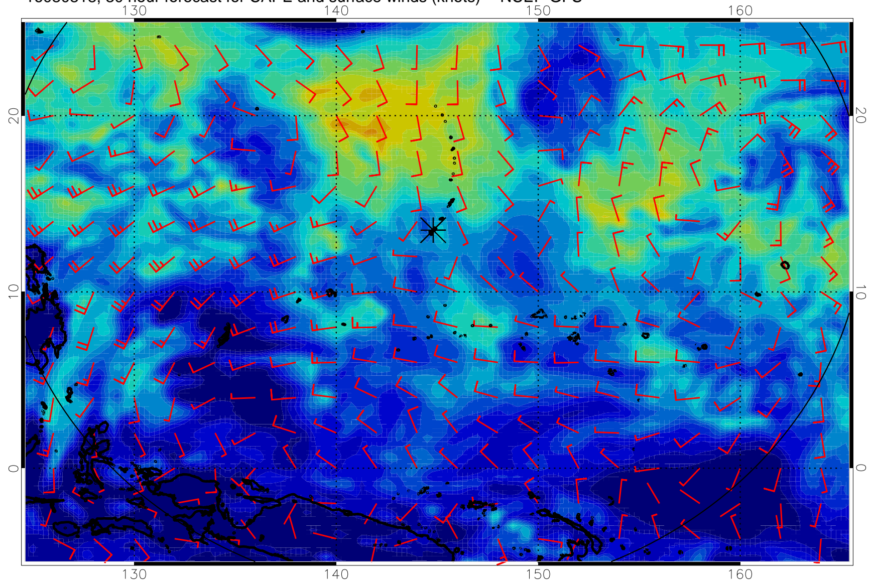
16080818, 30 hour forecast for CAPE and surface winds (knots) -- NCEP GFS
