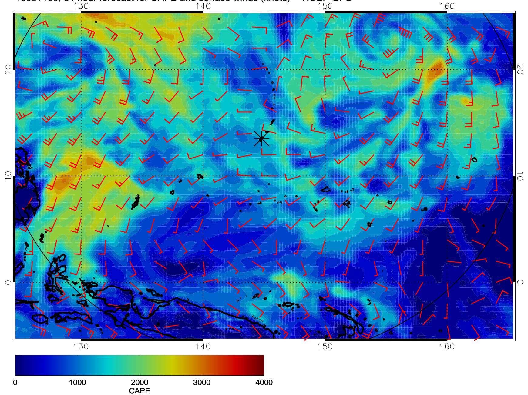
16081100, 84 hour forecast for CAPE and surface winds (knots) -- NCEP GFS
