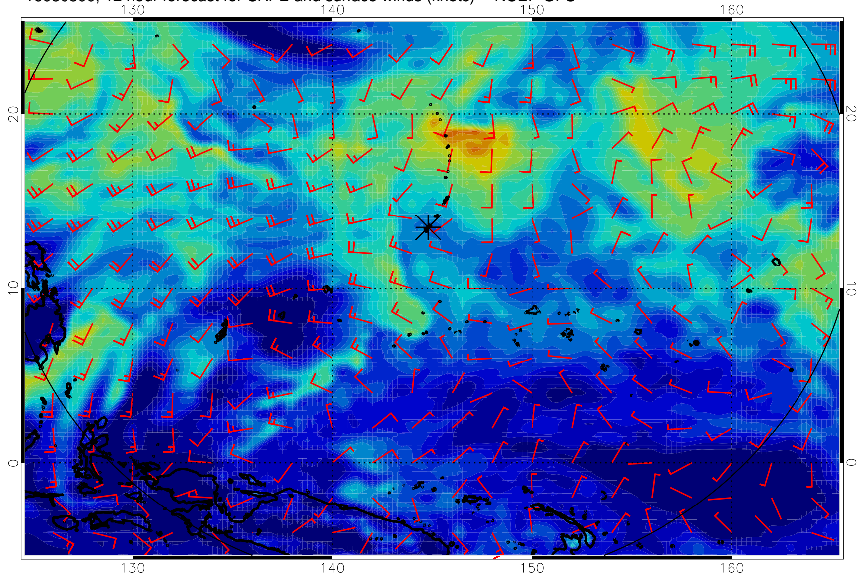
16080800, 12 hour forecast for CAPE and surface winds (knots) -- NCEP GFS
