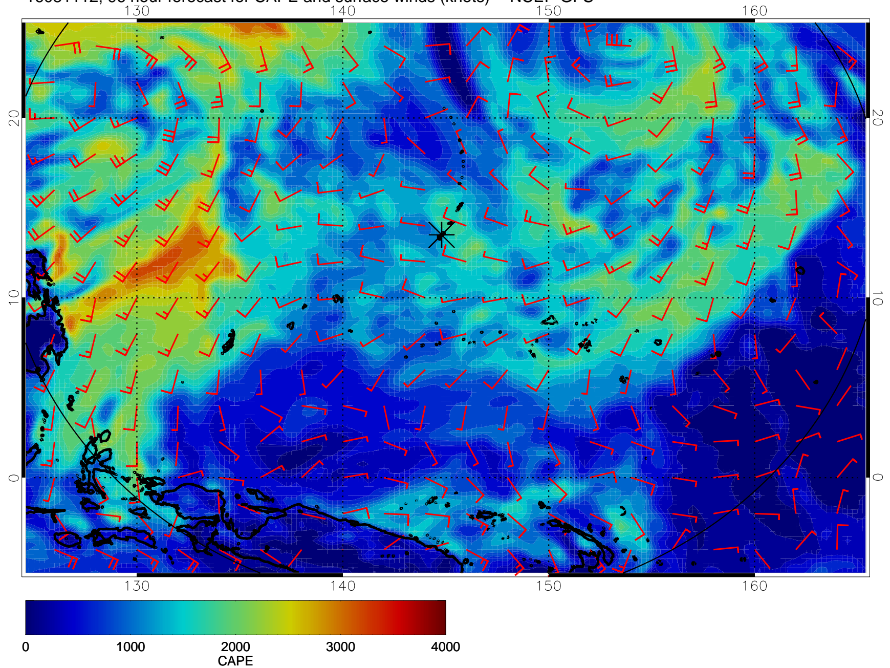
16081112, 96 hour forecast for CAPE and surface winds (knots) -- NCEP GFS
