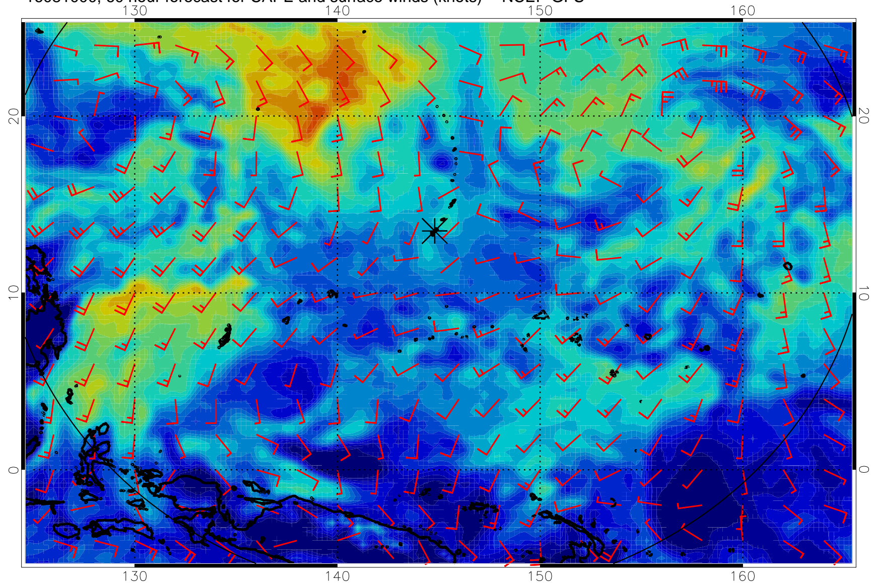
16081000, 60 hour forecast for CAPE and surface winds (knots) -- NCEP GFS
