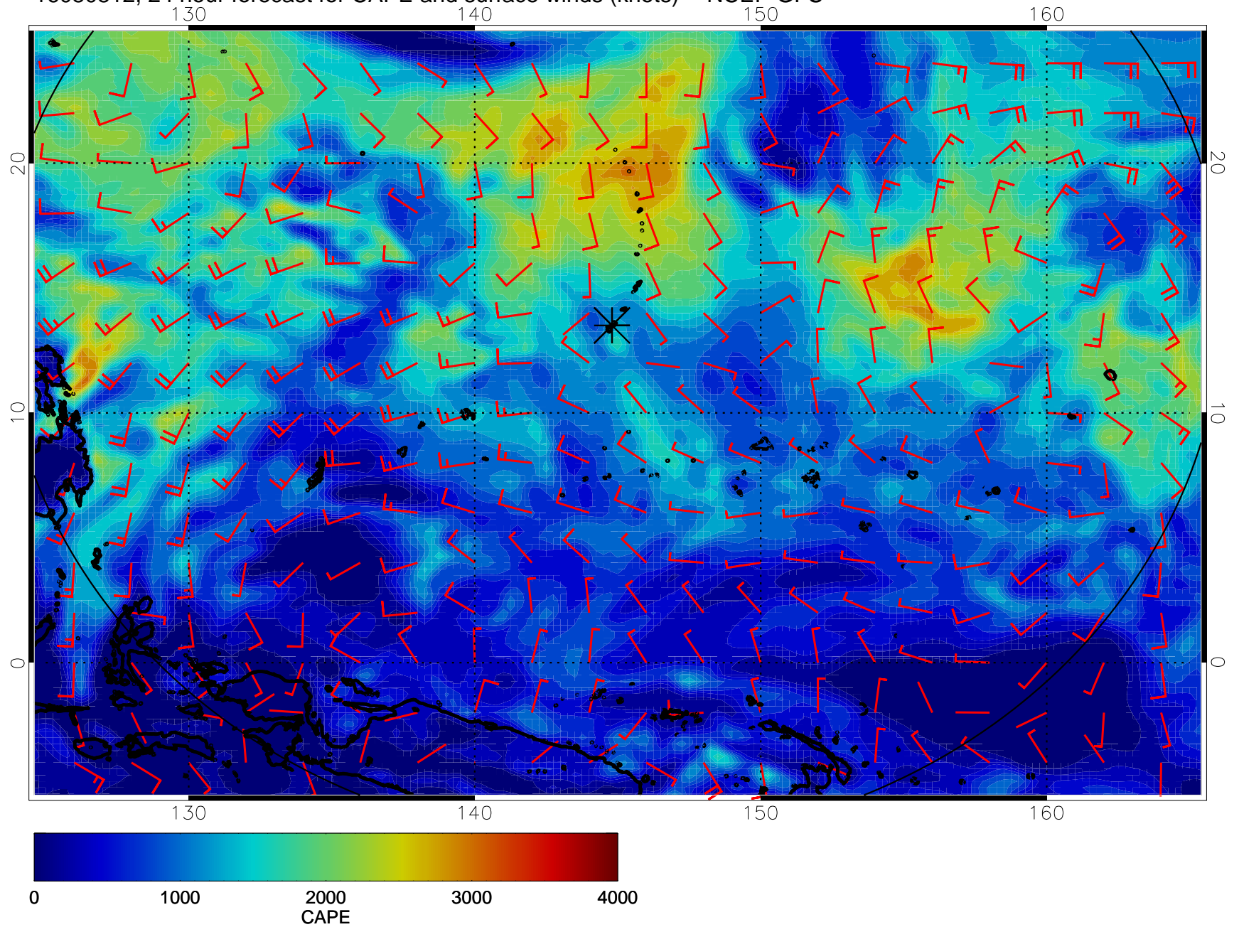
16080812, 24 hour forecast for CAPE and surface winds (knots) -- NCEP GFS
