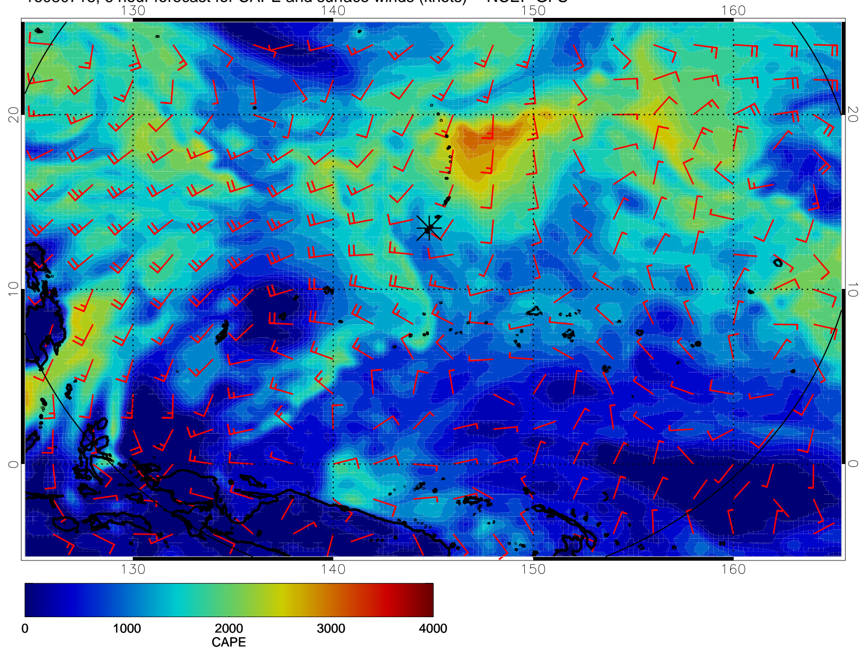
16080718, 6 hour forecast for CAPE and surface winds (knots) -- NCEP GFS
