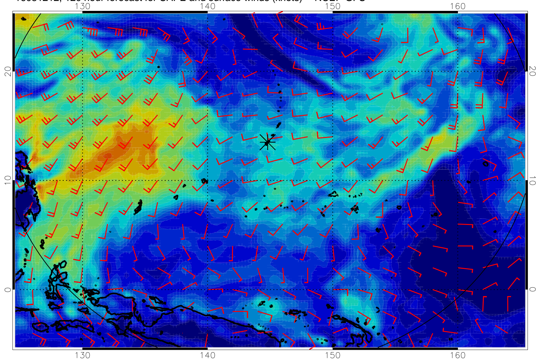
16081212, 120 hour forecast for CAPE and surface winds (knots) -- NCEP GFS
