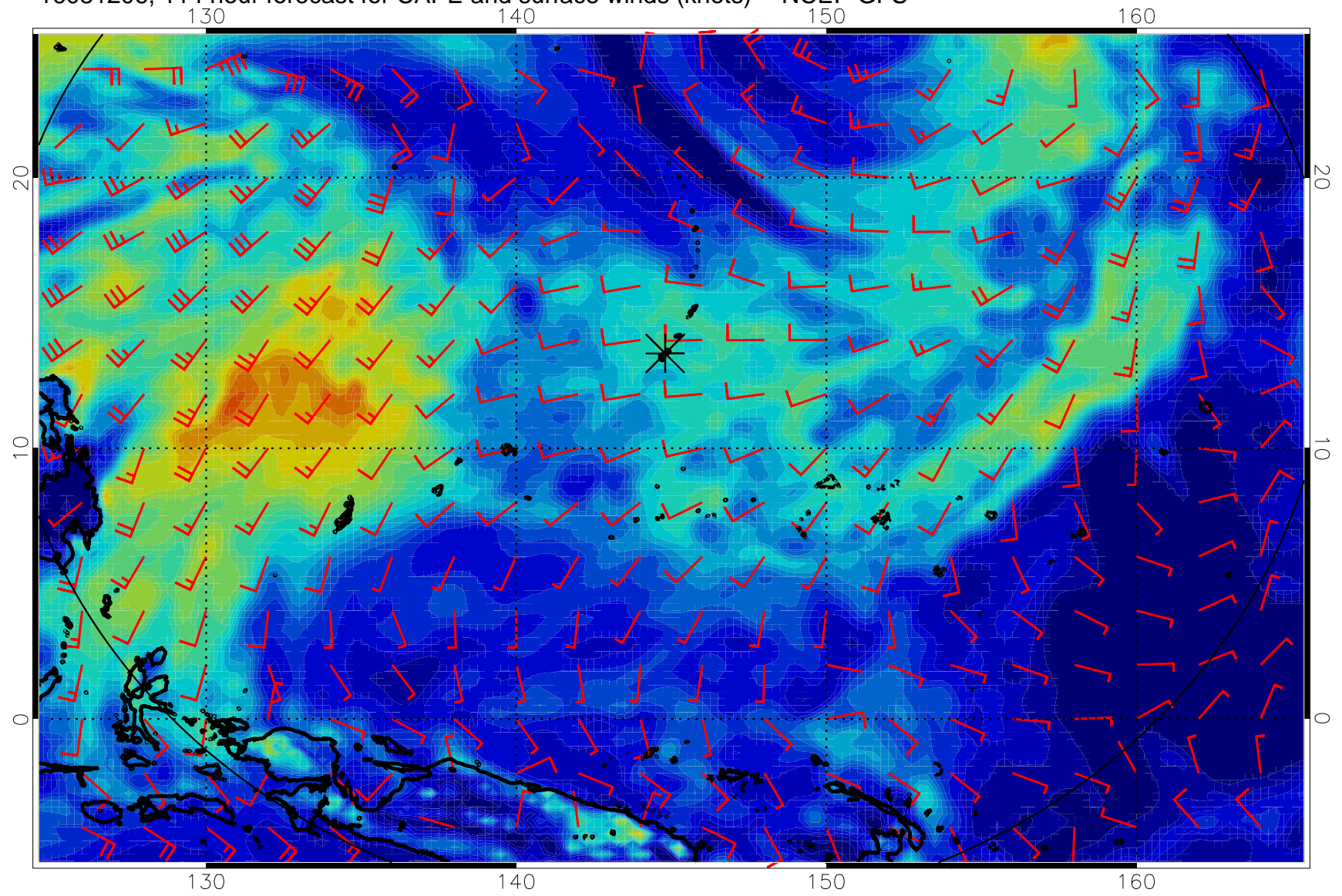
16081206, 114 hour forecast for CAPE and surface winds (knots) -- NCEP GFS
