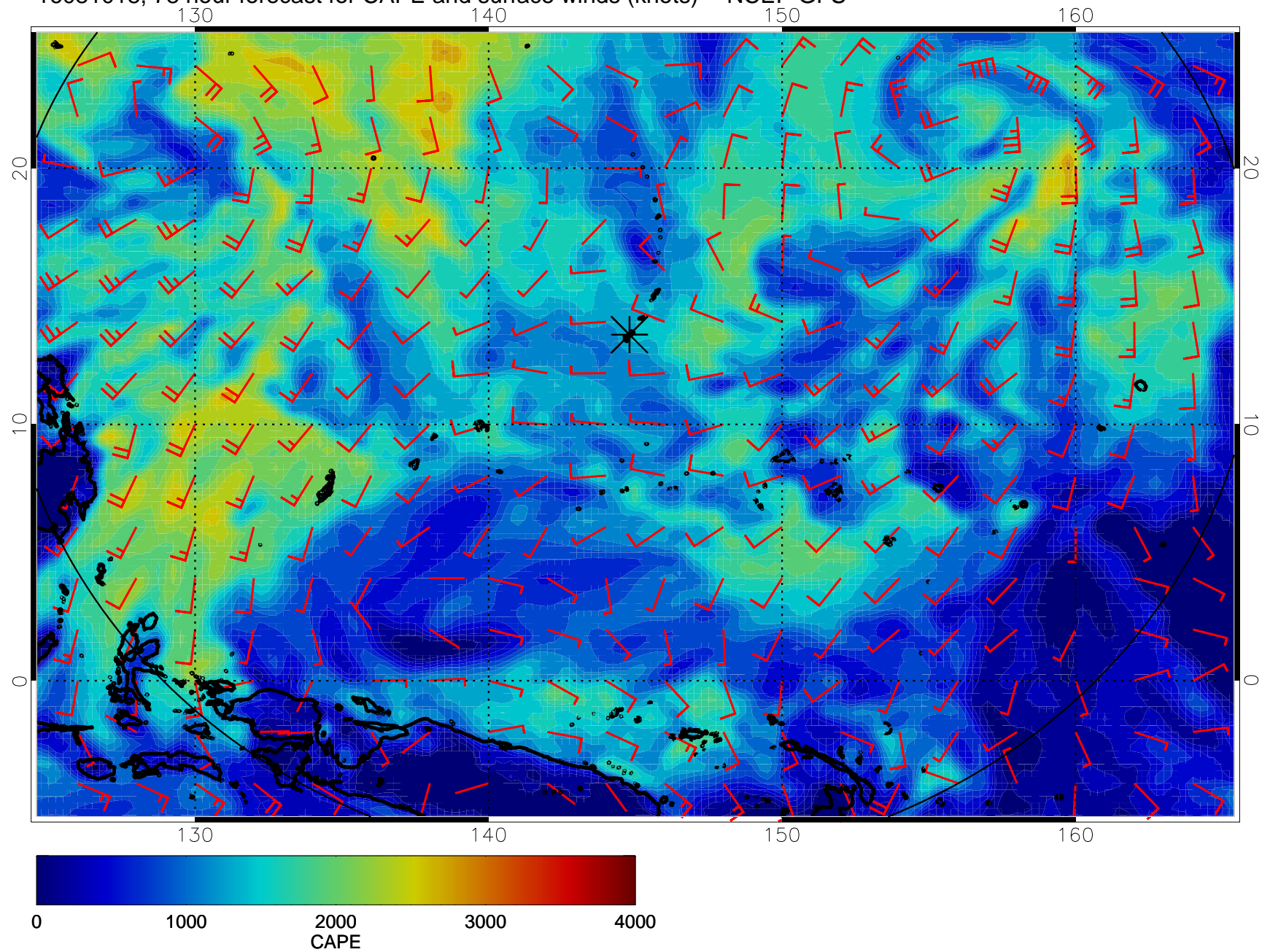
16081018, 78 hour forecast for CAPE and surface winds (knots) -- NCEP GFS
