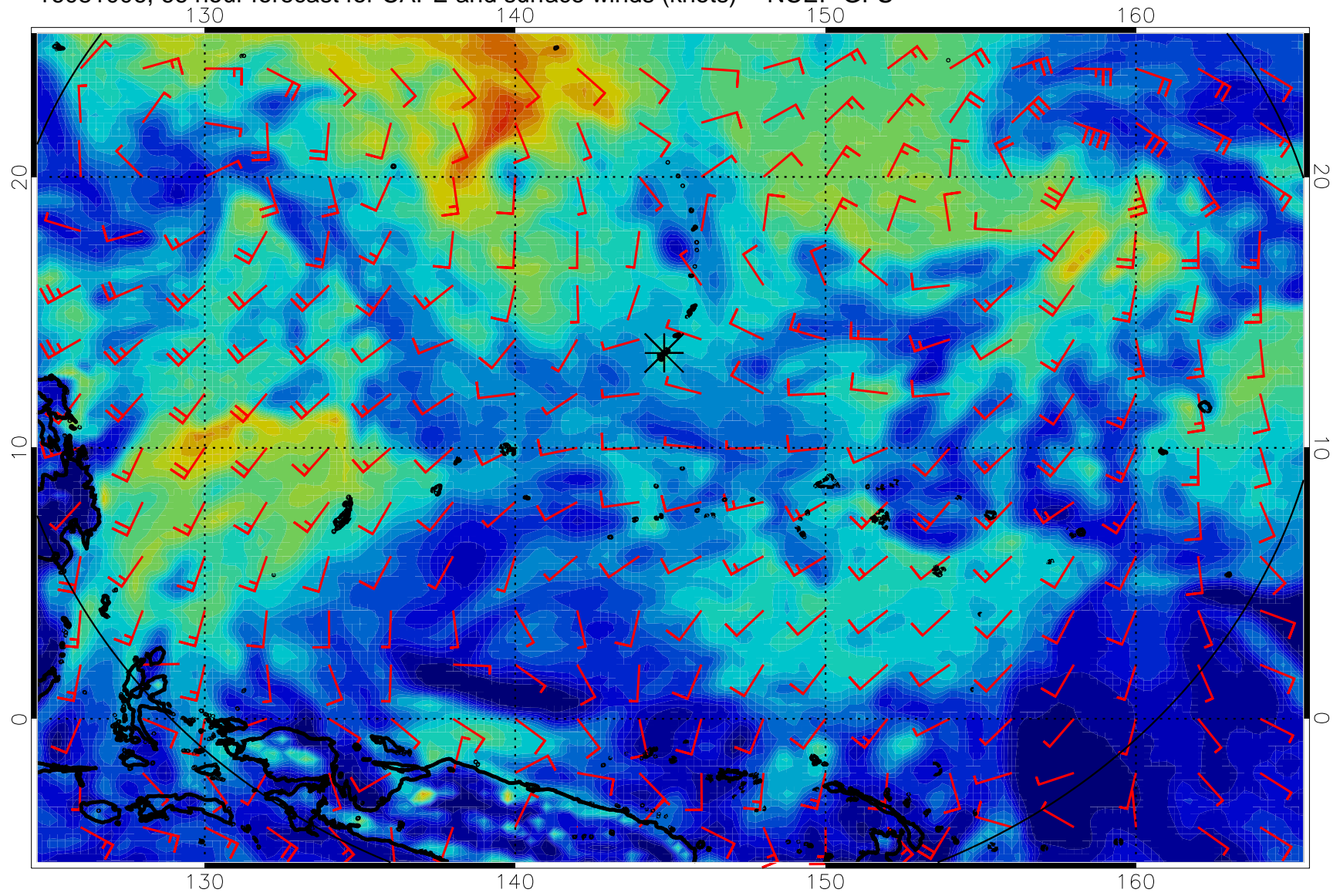
16081006, 66 hour forecast for CAPE and surface winds (knots) -- NCEP GFS
