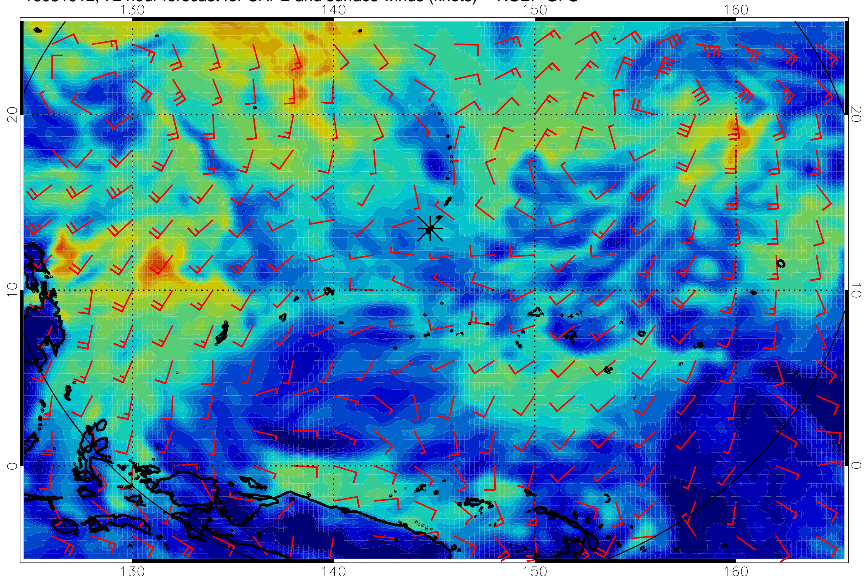
16081012, 72 hour forecast for CAPE and surface winds (knots) -- NCEP GFS
