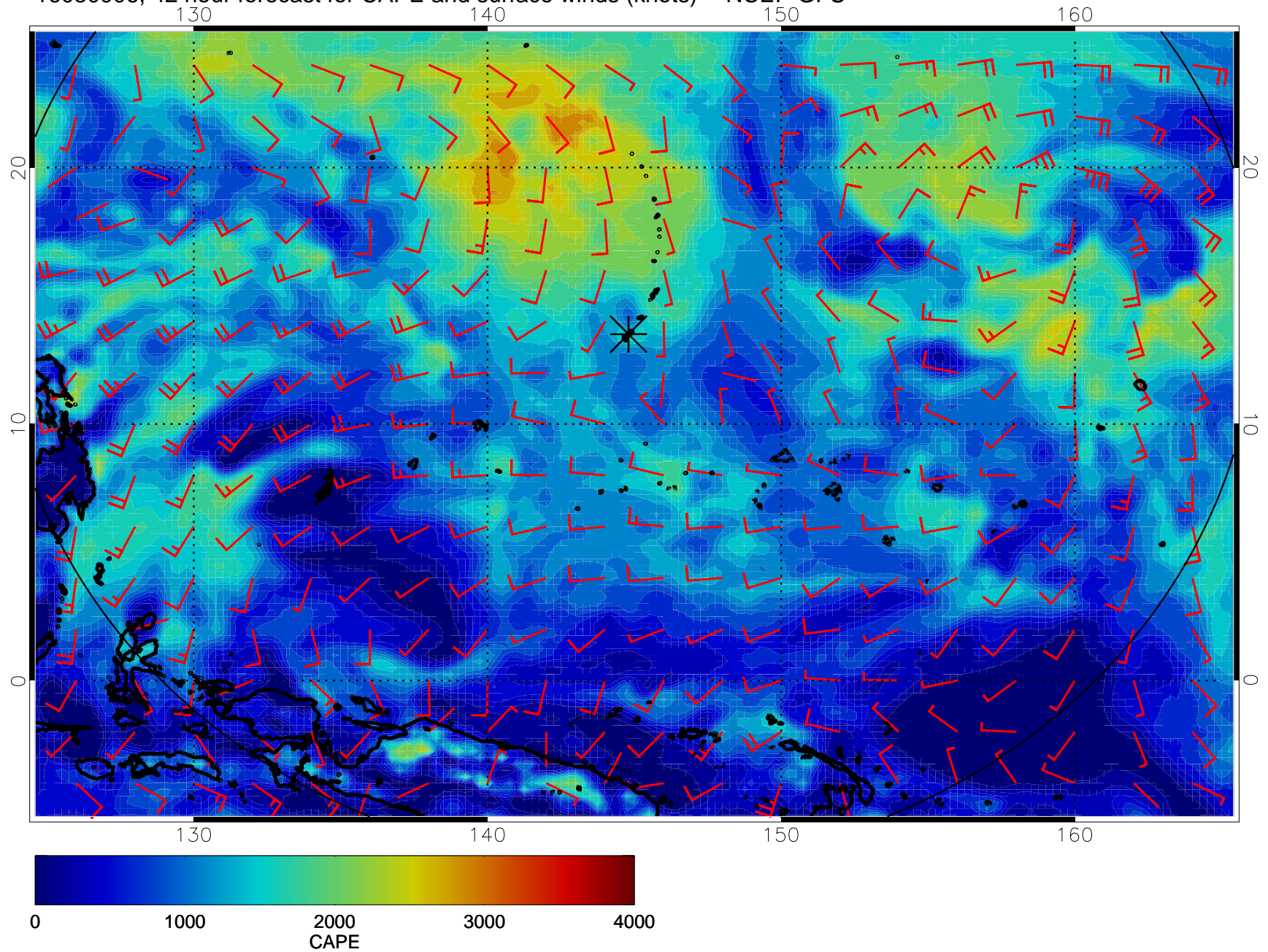
16080906, 42 hour forecast for CAPE and surface winds (knots) -- NCEP GFS
