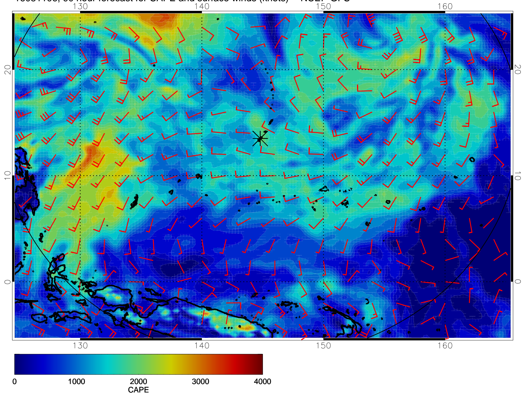
16081106, 90 hour forecast for CAPE and surface winds (knots) -- NCEP GFS
