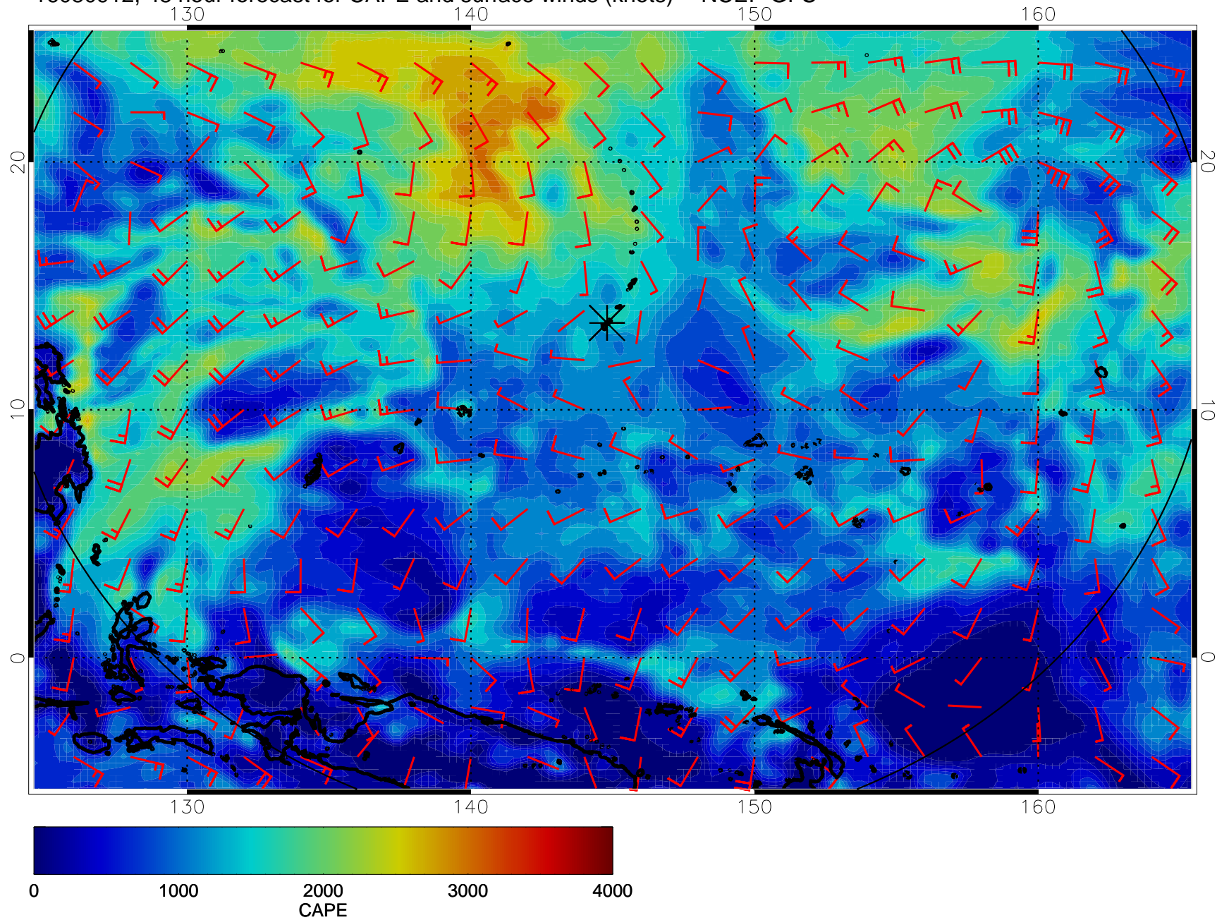
16080912, 48 hour forecast for CAPE and surface winds (knots) -- NCEP GFS
