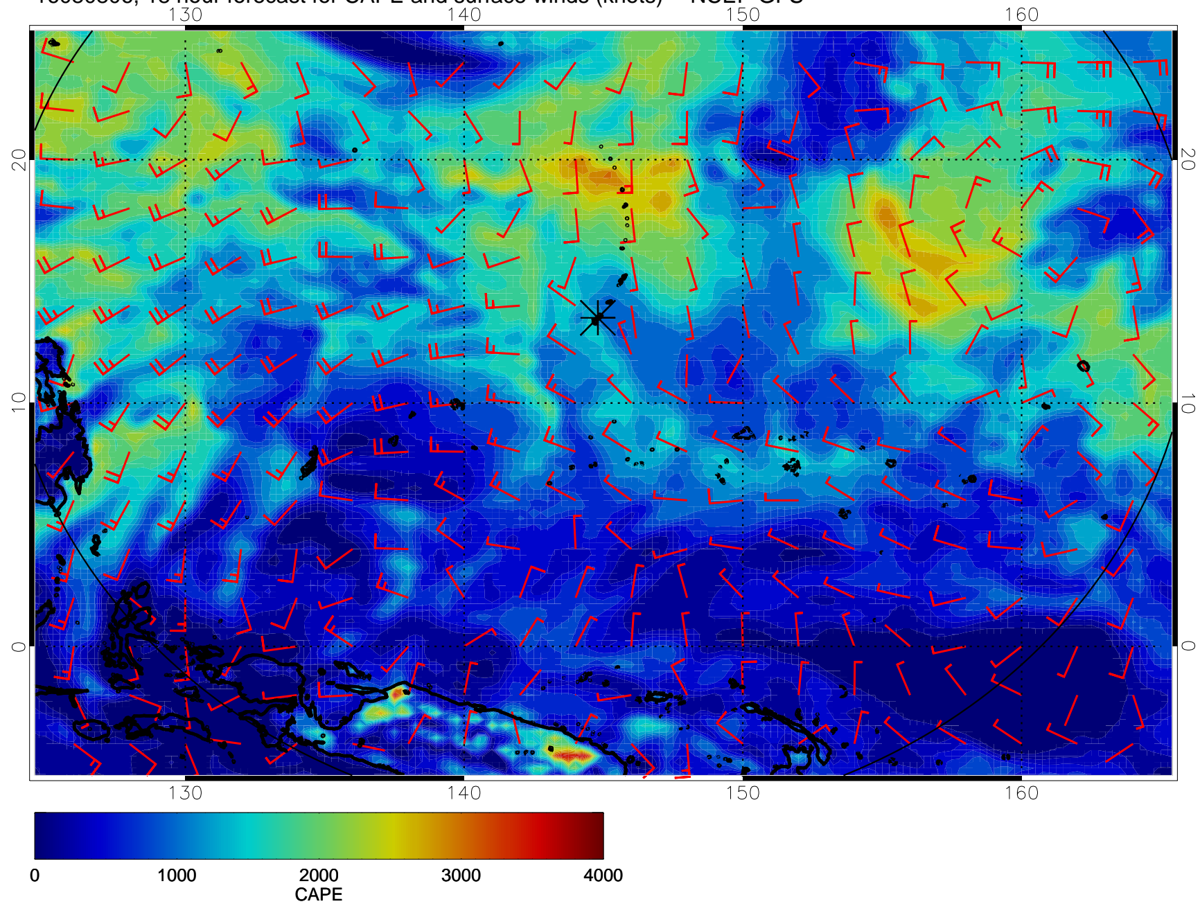
16080806, 18 hour forecast for CAPE and surface winds (knots) -- NCEP GFS
