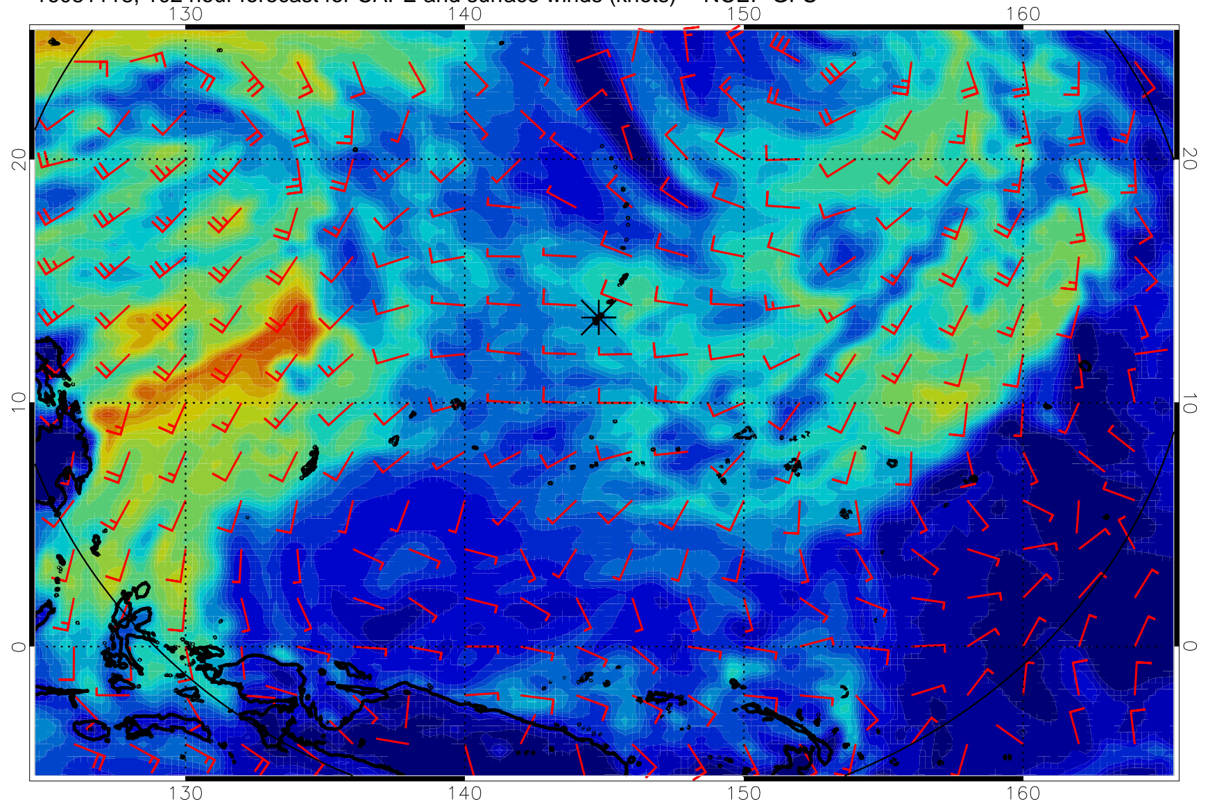
16081118, 102 hour forecast for CAPE and surface winds (knots) -- NCEP GFS
