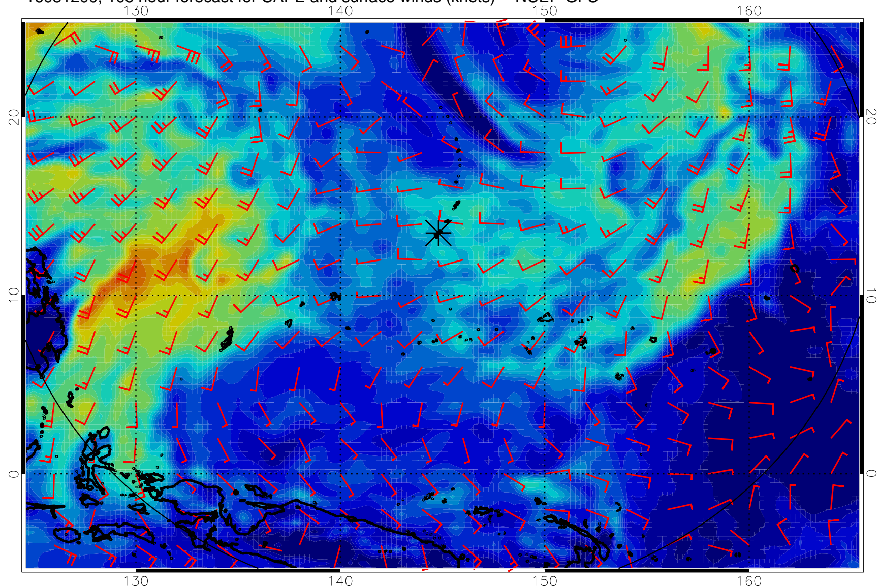
16081200, 108 hour forecast for CAPE and surface winds (knots) -- NCEP GFS
