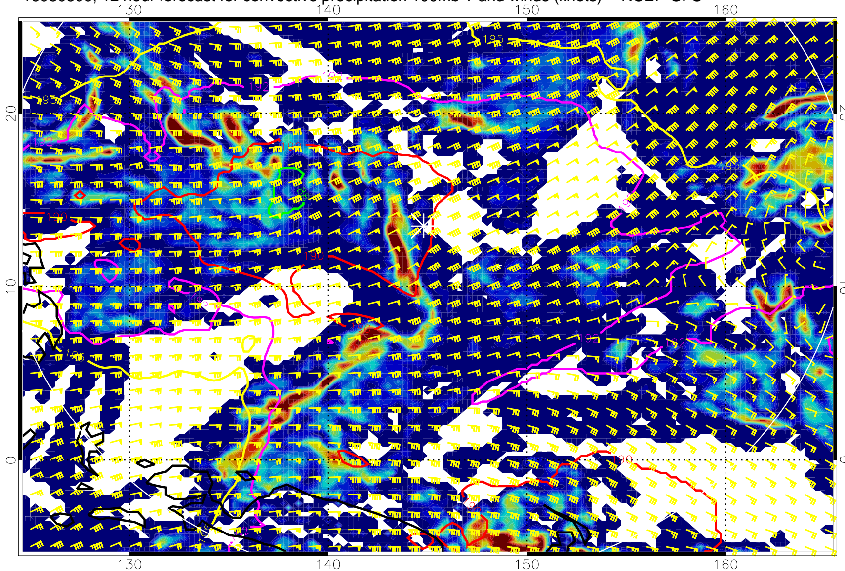
16080800, 12 hour forecast for convective precipitation 100mb T and winds (knots) -- NCEP GFS
