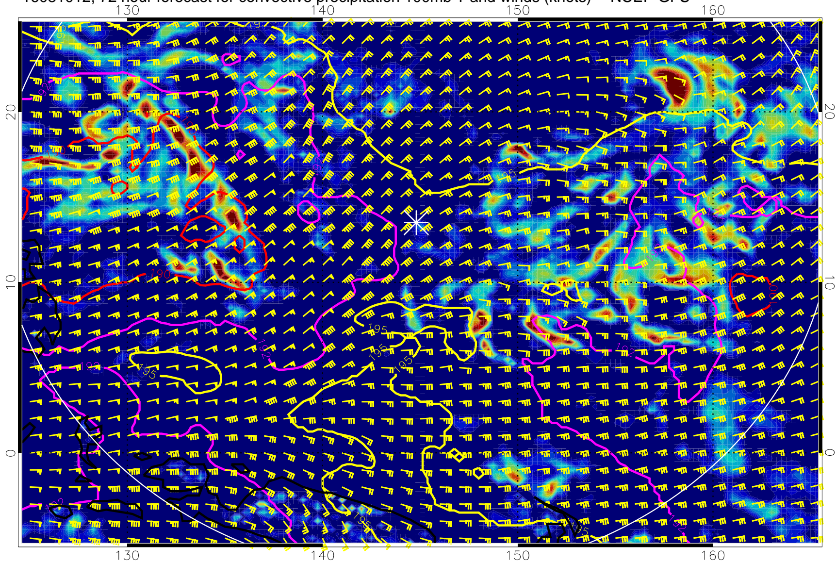
16081012, 72 hour forecast for convective precipitation 100mb T and winds (knots) -- NCEP GFS
