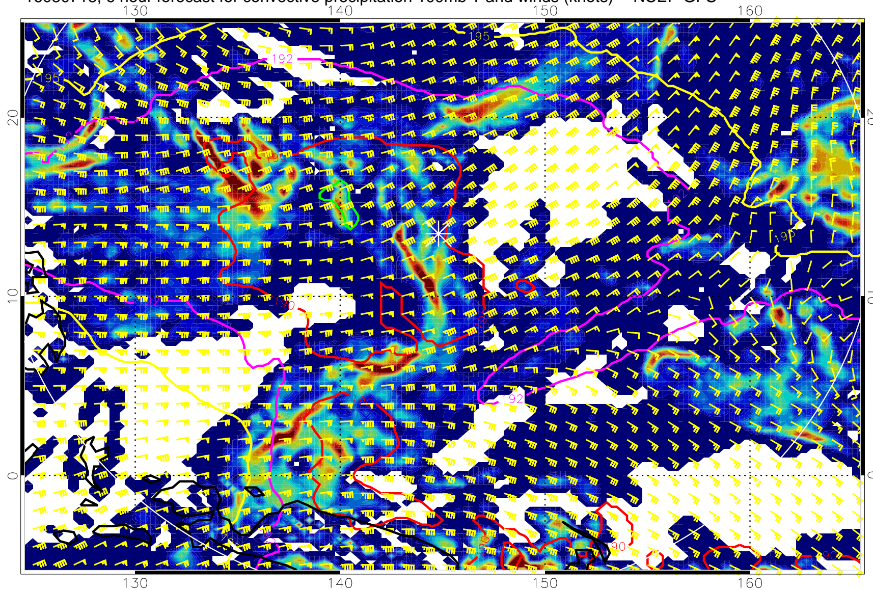
16080718, 6 hour forecast for convective precipitation 100mb T and winds (knots) -- NCEP GFS
