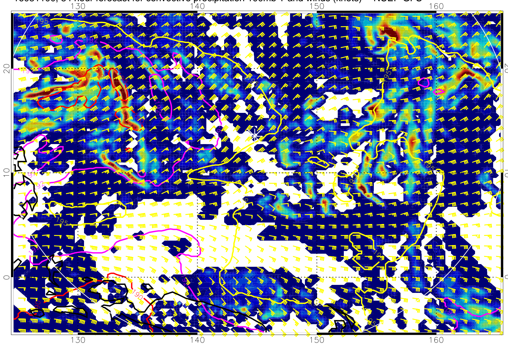
16081100, 84 hour forecast for convective precipitation 100mb T and winds (knots) -- NCEP GFS
