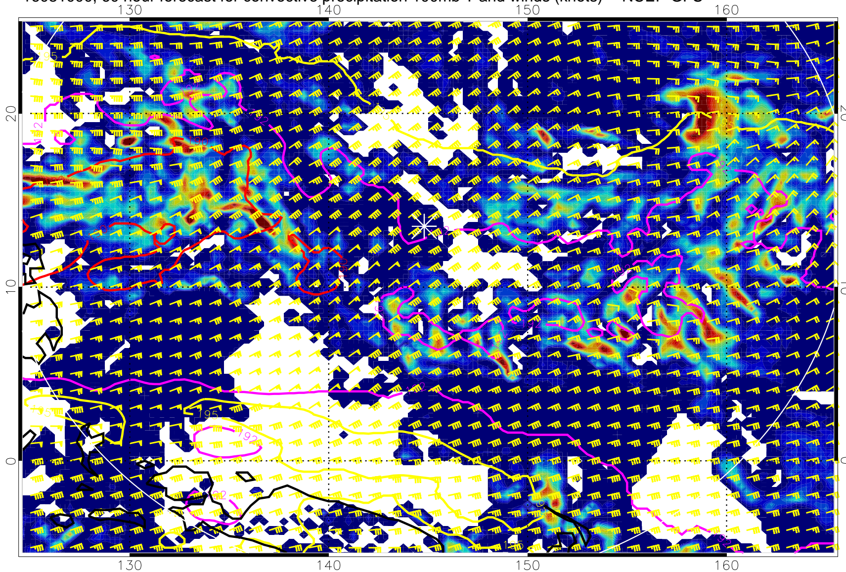
16081000, 60 hour forecast for convective precipitation 100mb T and winds (knots) -- NCEP GFS
