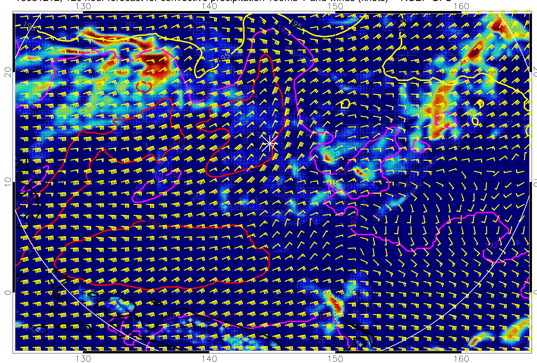
16081212, 120 hour forecast for convective precipitation 100mb T and winds (knots) -- NCEP GFS
