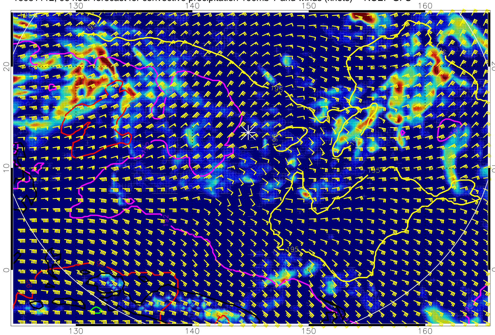
16081112, 96 hour forecast for convective precipitation 100mb T and winds (knots) -- NCEP GFS
