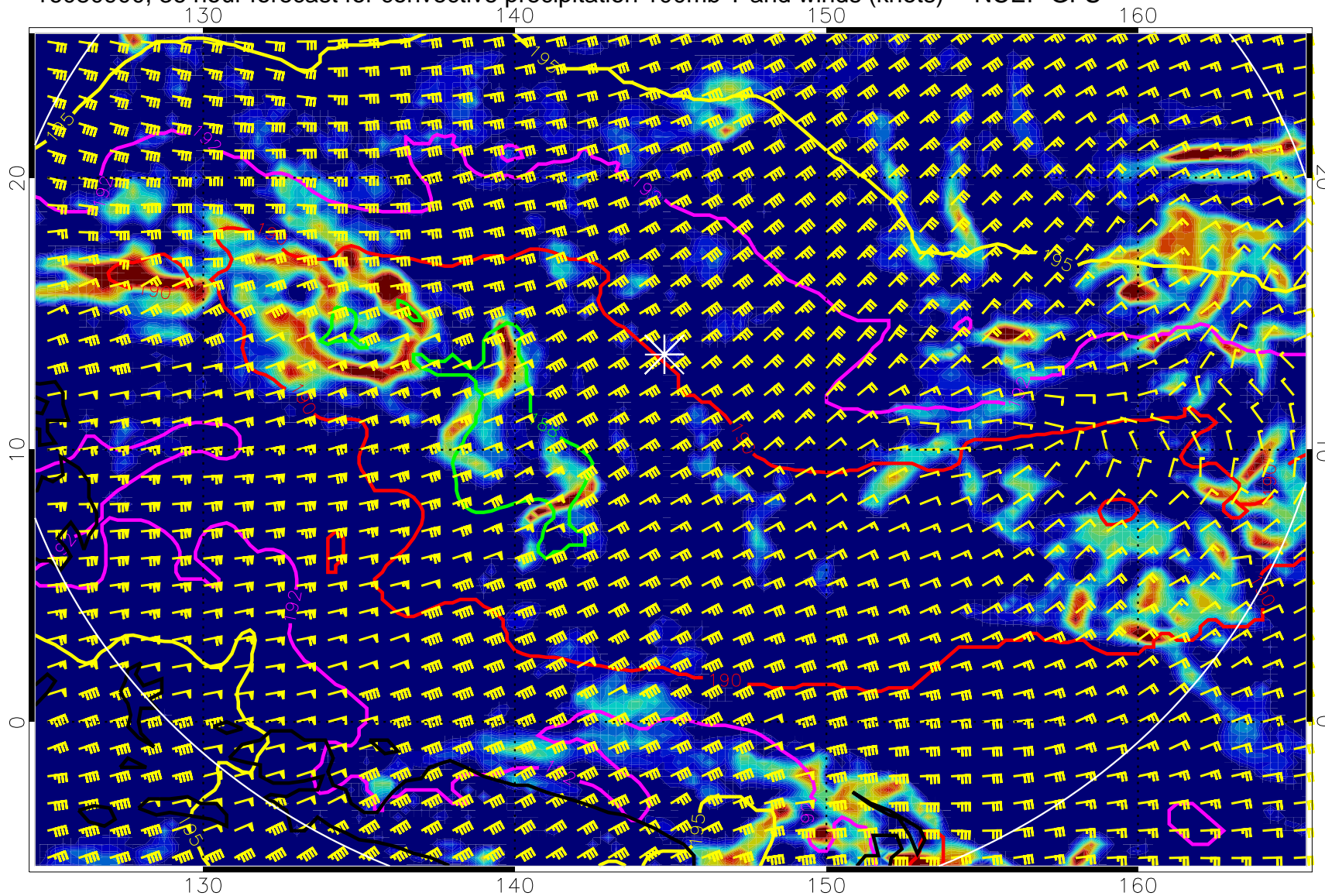
16080900, 36 hour forecast for convective precipitation 100mb T and winds (knots) -- NCEP GFS
