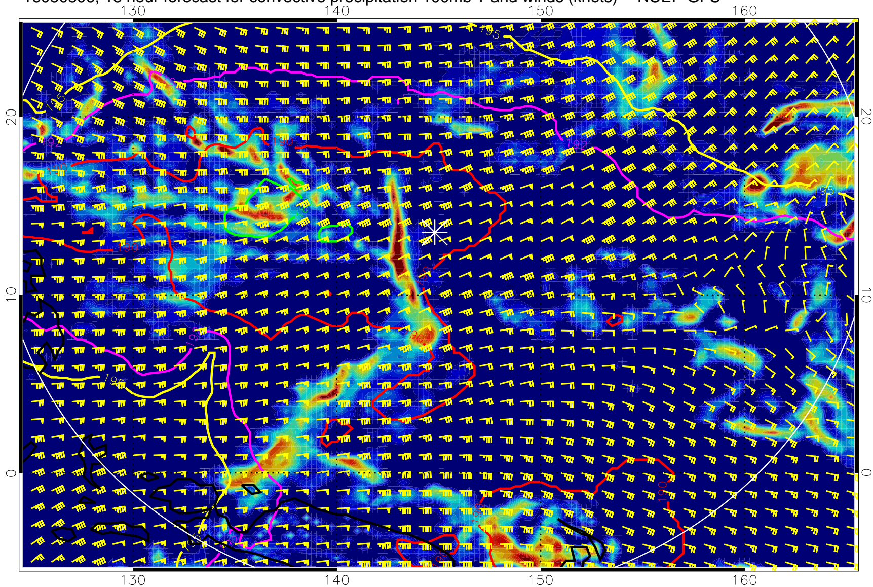
16080806, 18 hour forecast for convective precipitation 100mb T and winds (knots) -- NCEP GFS
