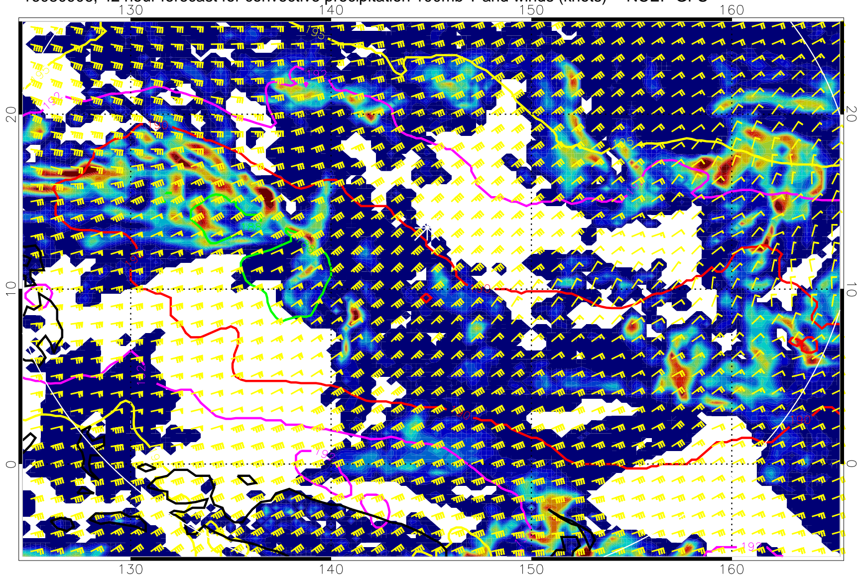
16080906, 42 hour forecast for convective precipitation 100mb T and winds (knots) -- NCEP GFS
