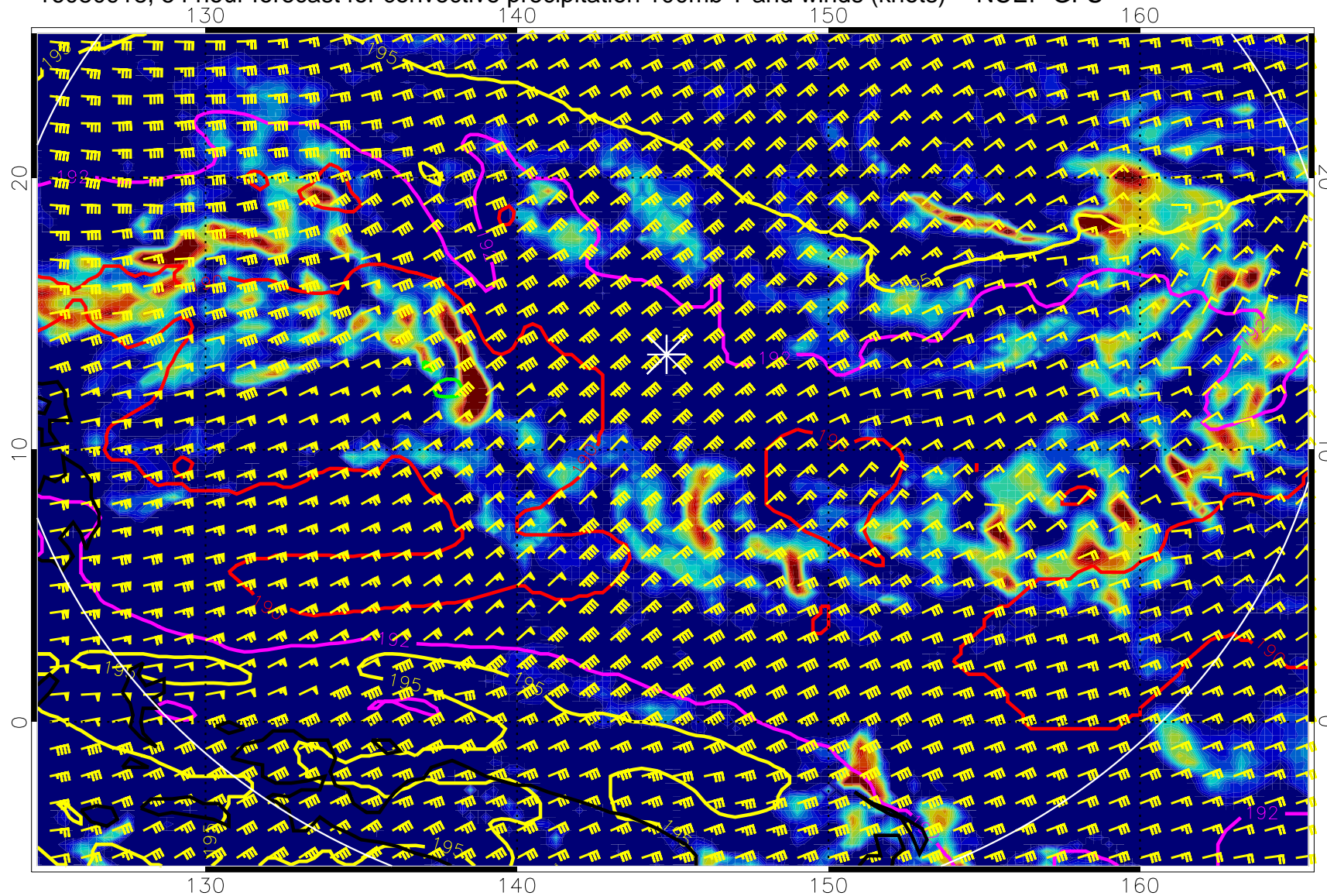
16080918, 54 hour forecast for convective precipitation 100mb T and winds (knots) -- NCEP GFS
