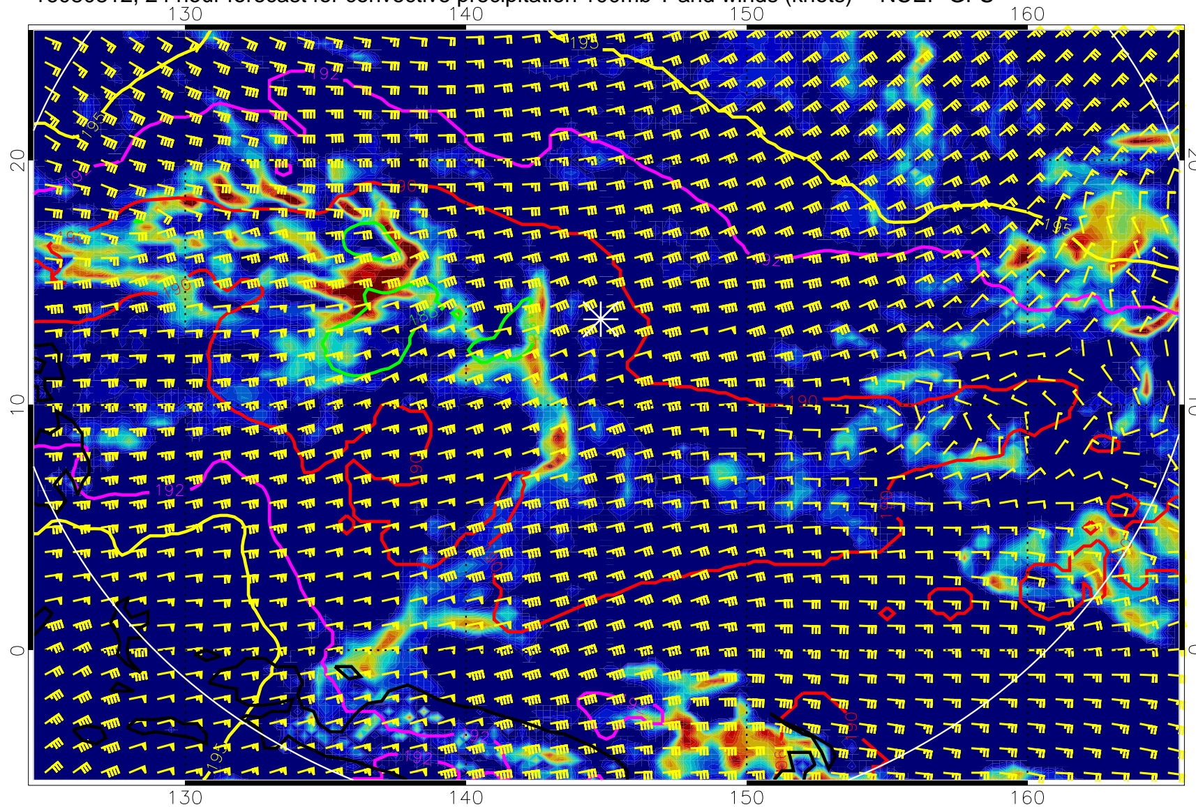
16080812, 24 hour forecast for convective precipitation 100mb T and winds (knots) -- NCEP GFS
