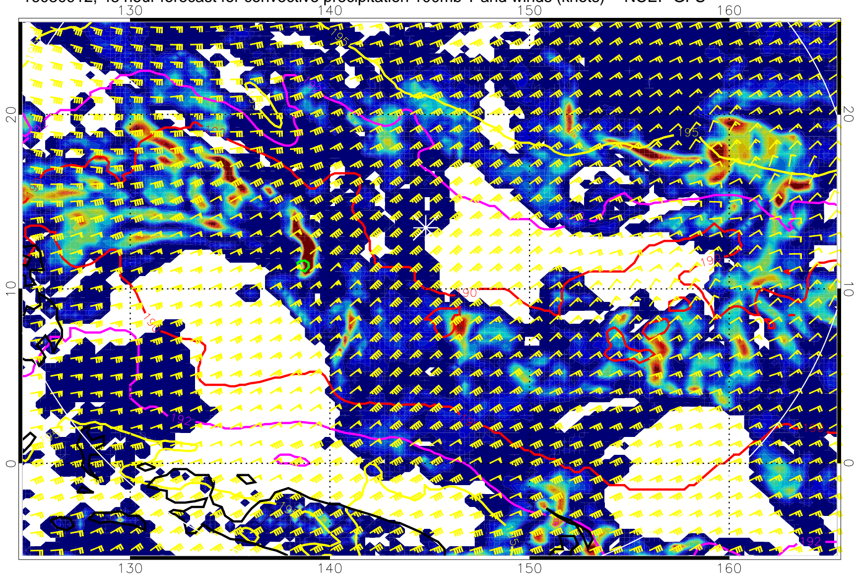
16080912, 48 hour forecast for convective precipitation 100mb T and winds (knots) -- NCEP GFS
