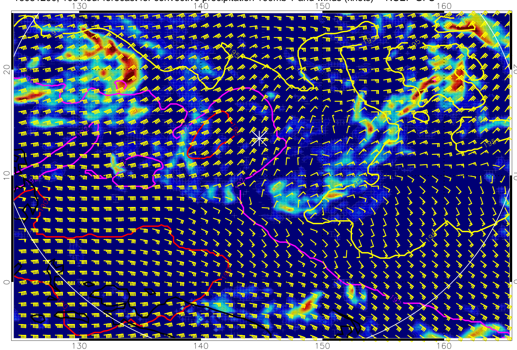
16081200, 108 hour forecast for convective precipitation 100mb T and winds (knots) -- NCEP GFS
