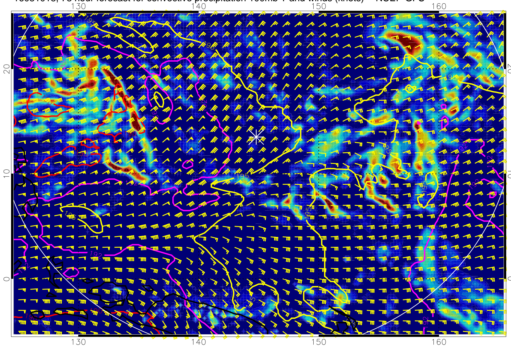
16081018, 78 hour forecast for convective precipitation 100mb T and winds (knots) -- NCEP GFS
