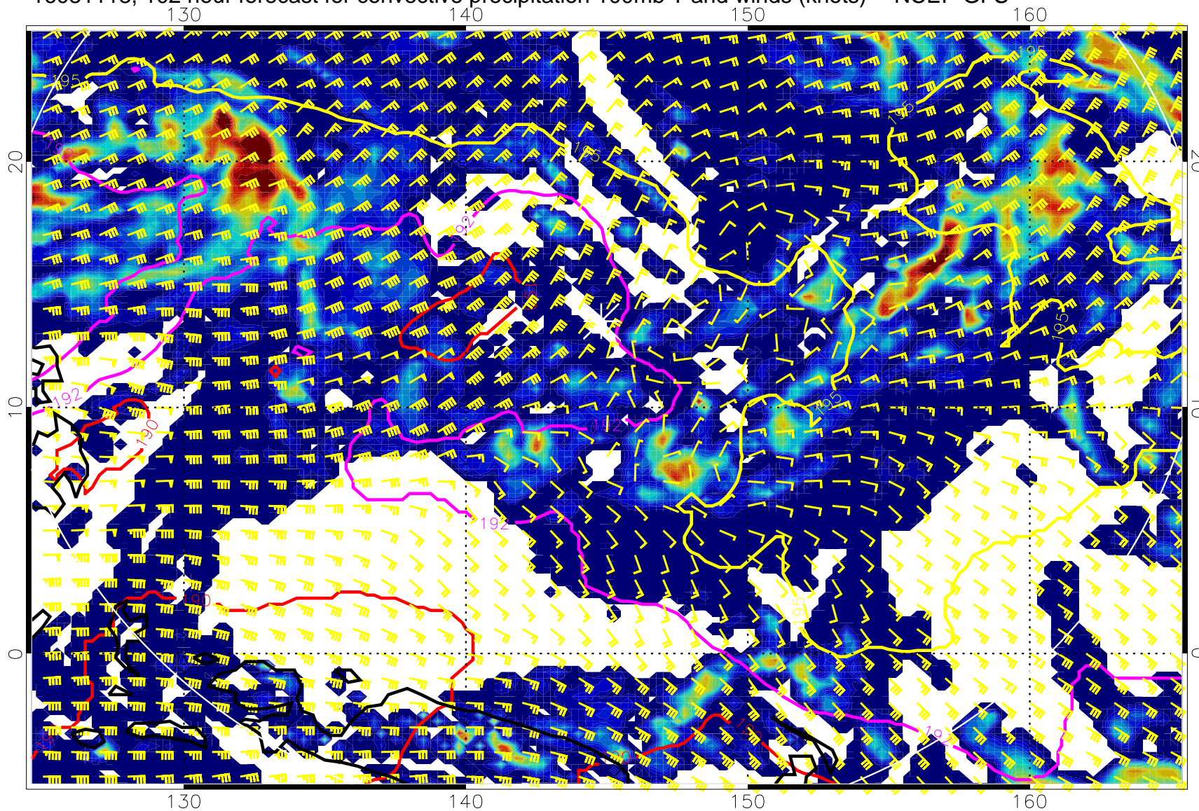
16081118, 102 hour forecast for convective precipitation 100mb T and winds (knots) -- NCEP GFS
