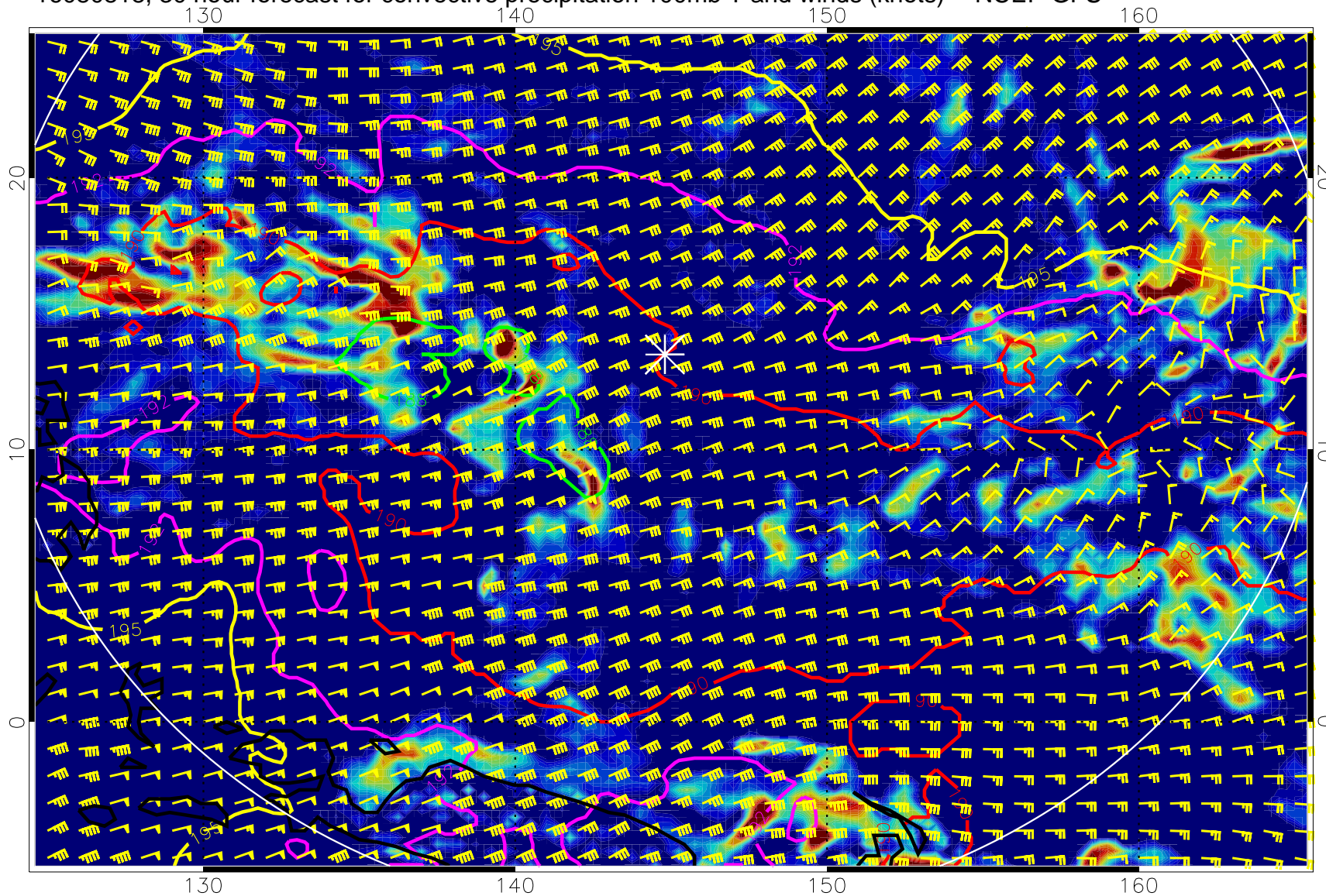
16080818, 30 hour forecast for convective precipitation 100mb T and winds (knots) -- NCEP GFS
