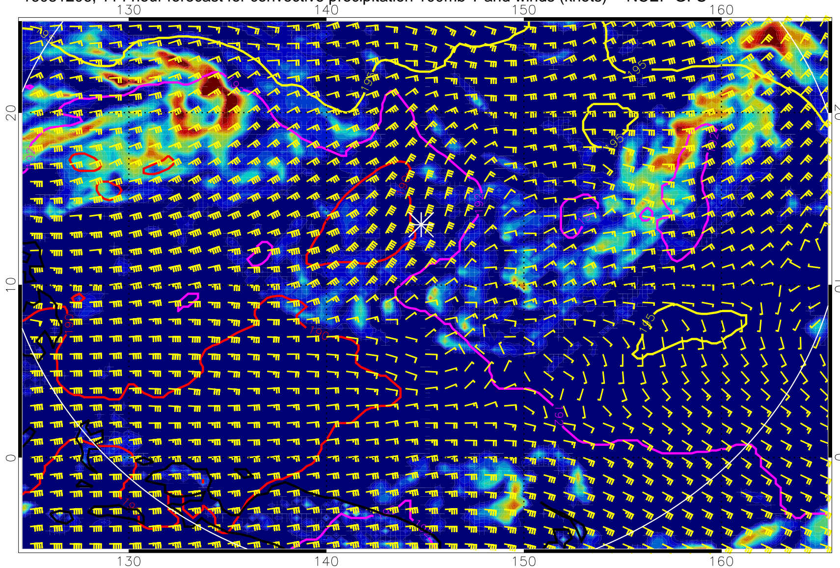
16081206, 114 hour forecast for convective precipitation 100mb T and winds (knots) -- NCEP GFS
