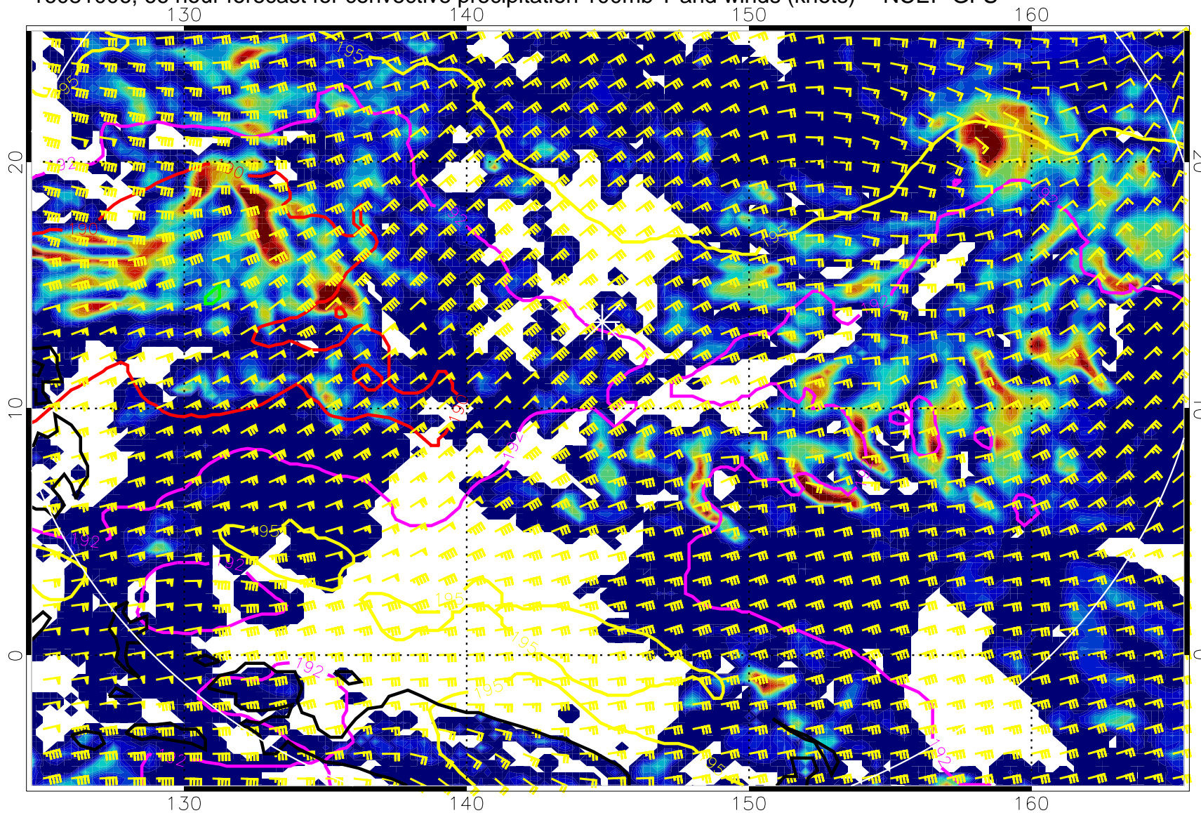
16081006, 66 hour forecast for convective precipitation 100mb T and winds (knots) -- NCEP GFS
