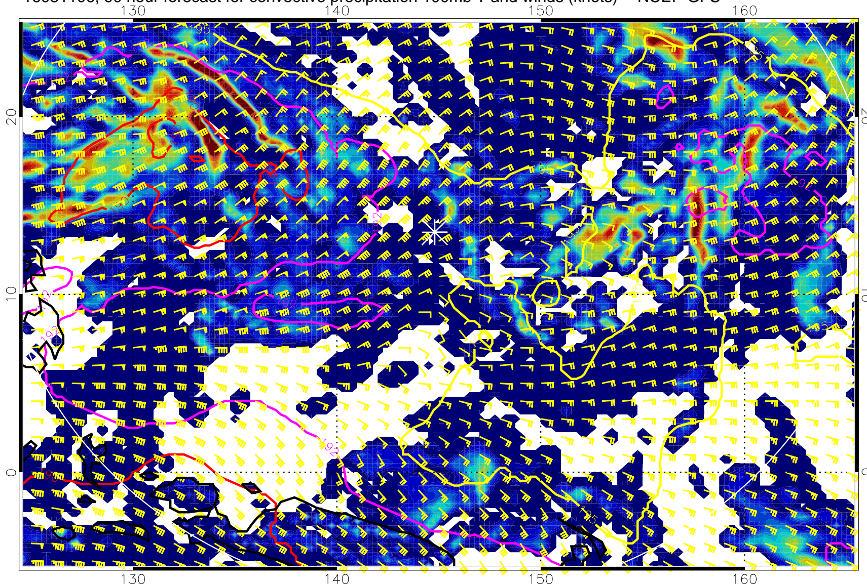
16081106, 90 hour forecast for convective precipitation 100mb T and winds (knots) -- NCEP GFS
