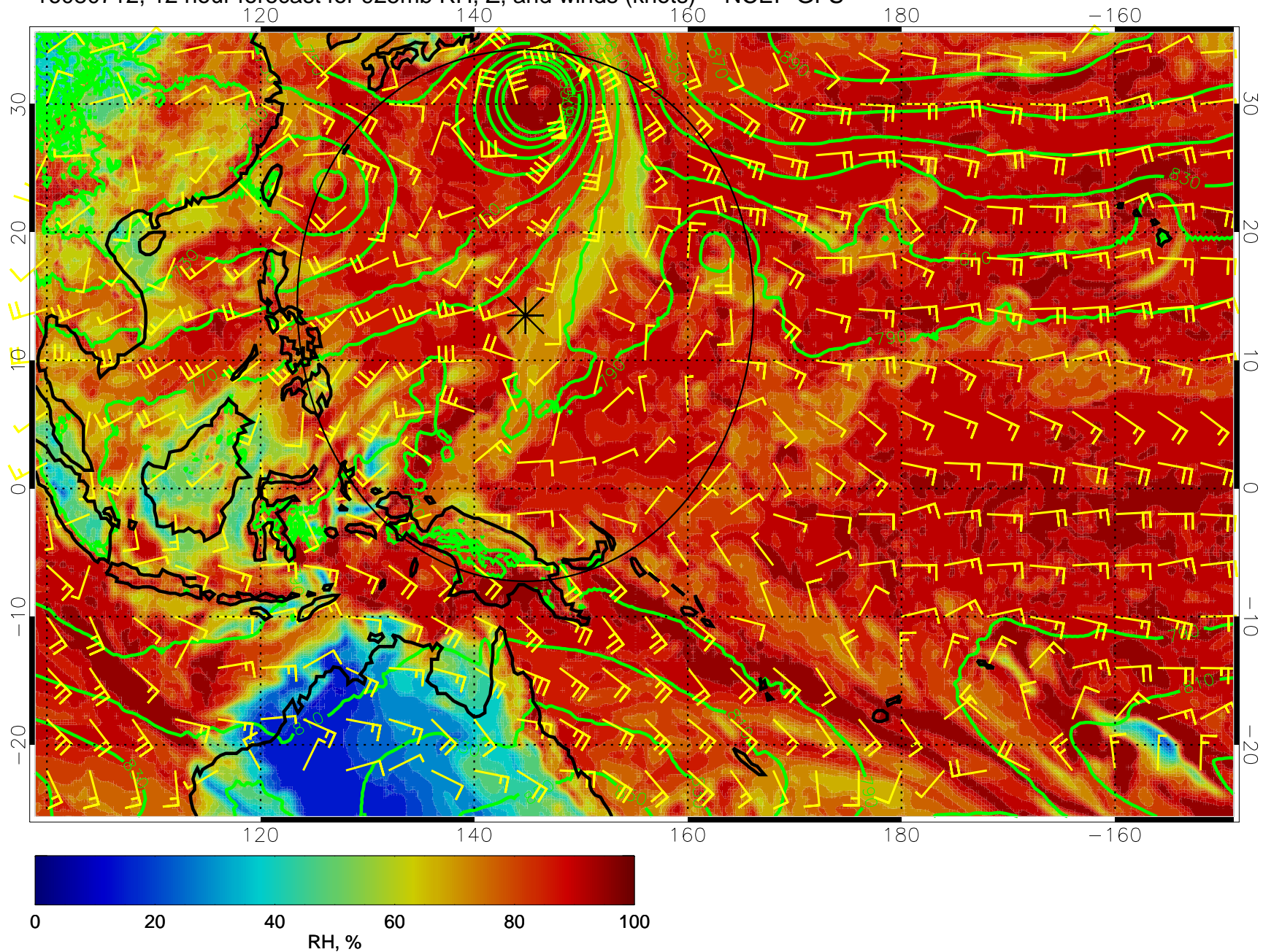
16080712, 12 hour forecast for 925mb RH, Z, and winds (knots) -- NCEP GFS
