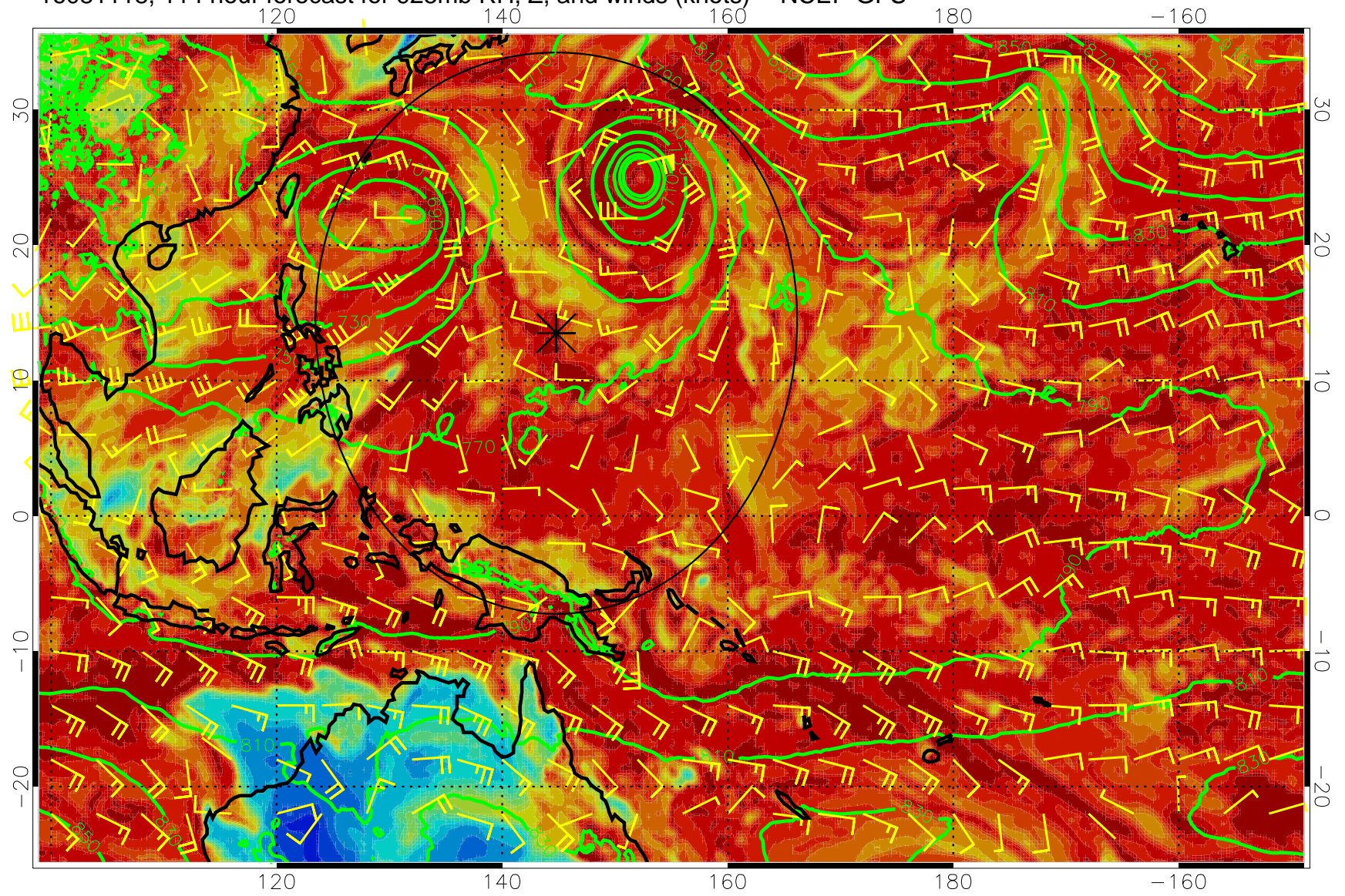
16081118, 114 hour forecast for 925mb RH, Z, and winds (knots) -- NCEP GFS
