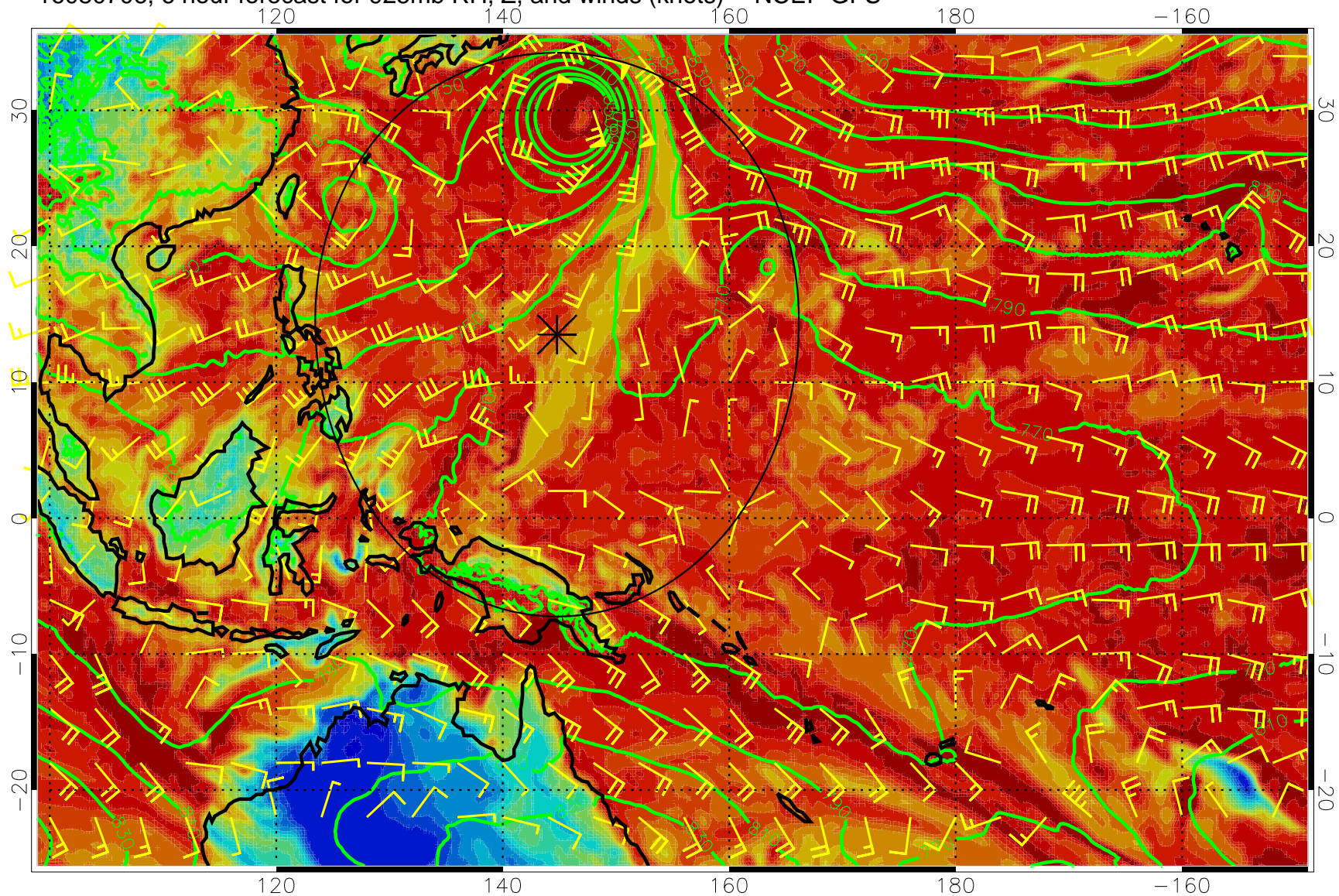
16080706, 6 hour forecast for 925mb RH, Z, and winds (knots) -- NCEP GFS
