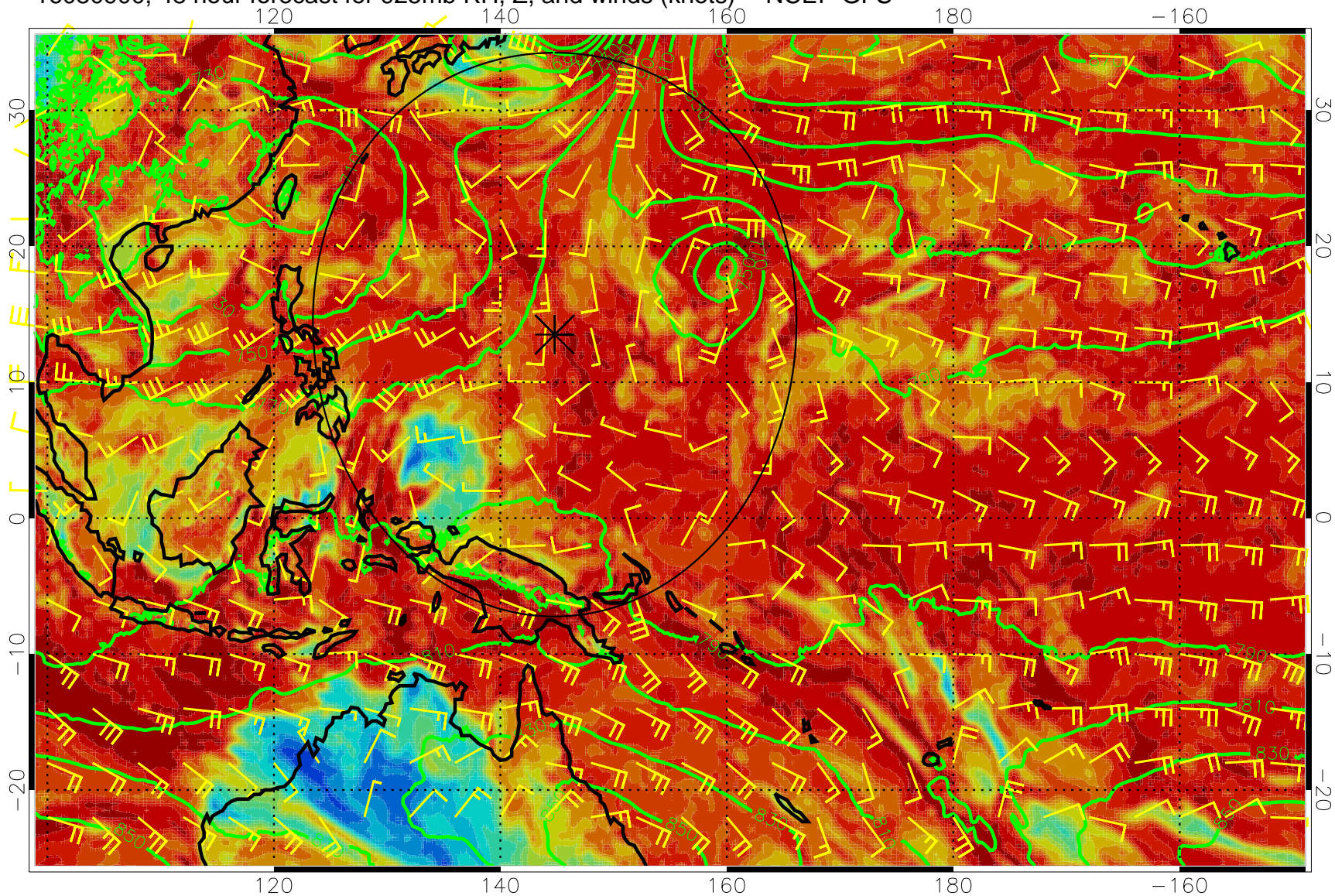
16080900, 48 hour forecast for 925mb RH, Z, and winds (knots) -- NCEP GFS
