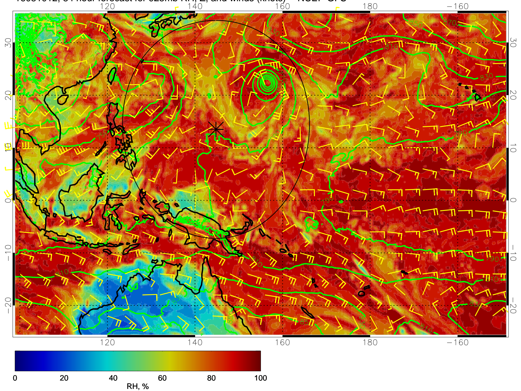
16081012, 84 hour forecast for 925mb RH, Z, and winds (knots) -- NCEP GFS
