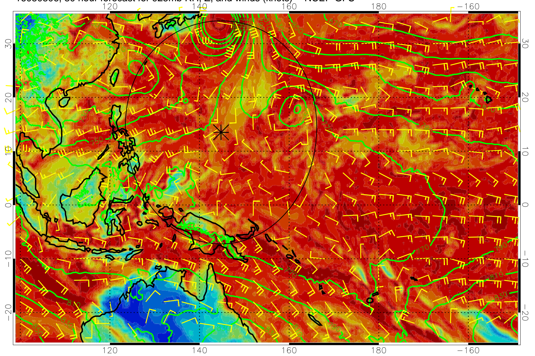
16080806, 30 hour forecast for 925mb RH, Z, and winds (knots) -- NCEP GFS
