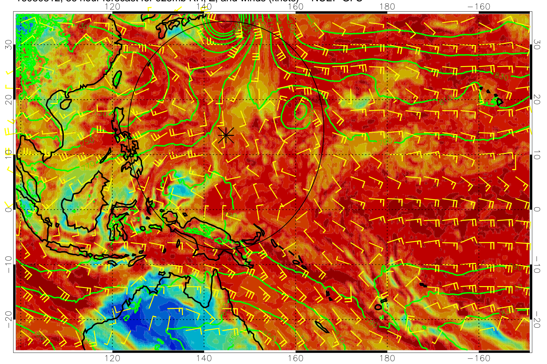
16080812, 36 hour forecast for 925mb RH, Z, and winds (knots) -- NCEP GFS
