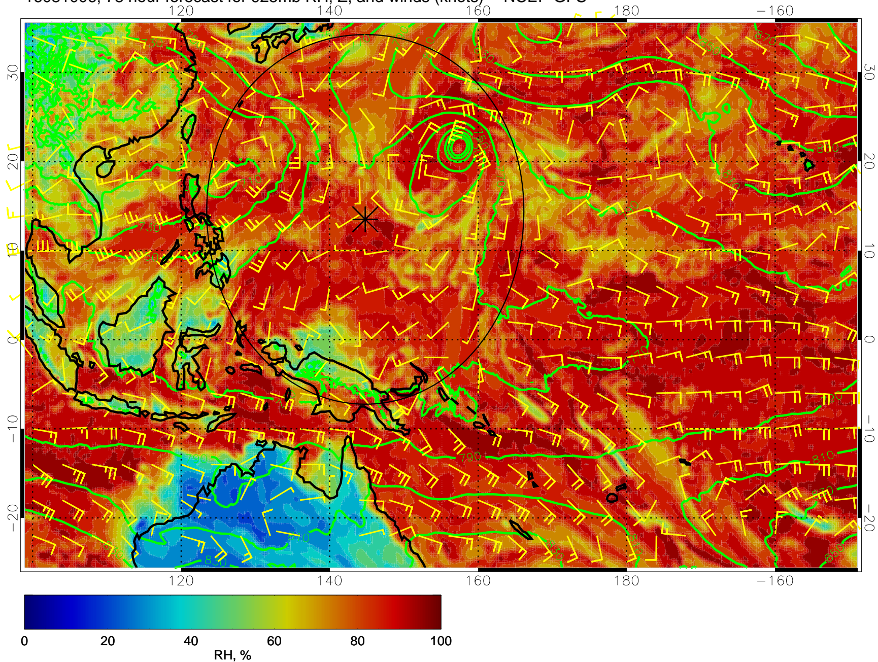
16081006, 78 hour forecast for 925mb RH, Z, and winds (knots) -- NCEP GFS
