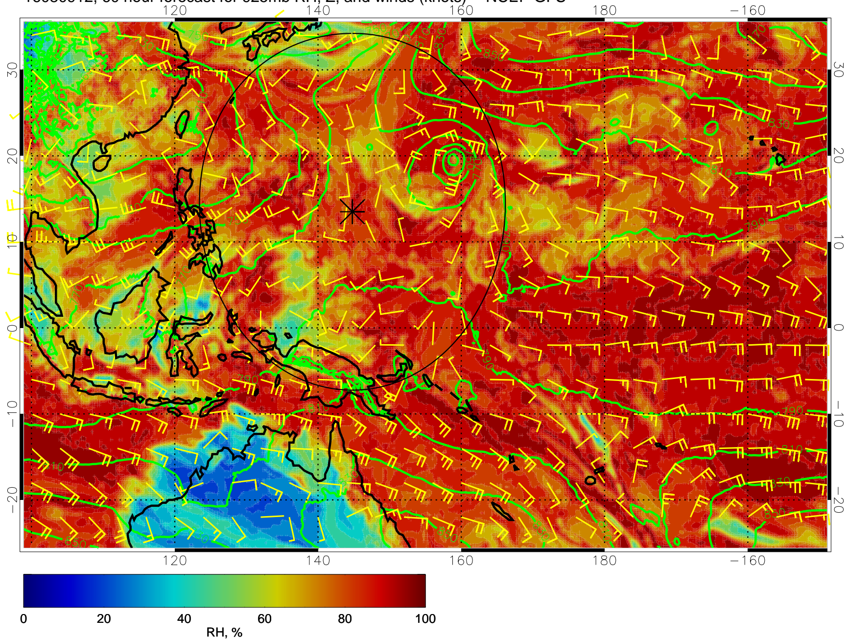
16080912, 60 hour forecast for 925mb RH, Z, and winds (knots) -- NCEP GFS
