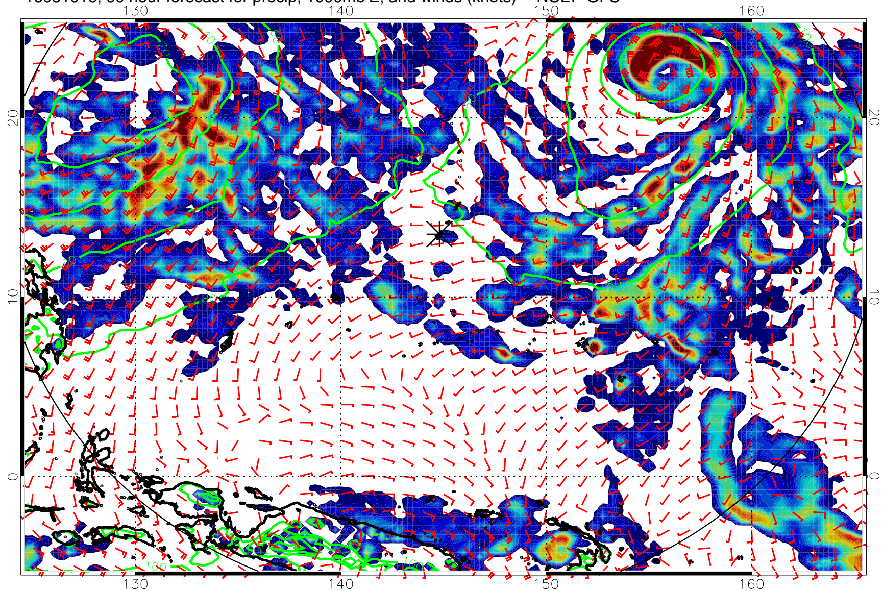
16081018, 90 hour forecast for precip, 1000mb Z, and winds (knots) -- NCEP GFS
