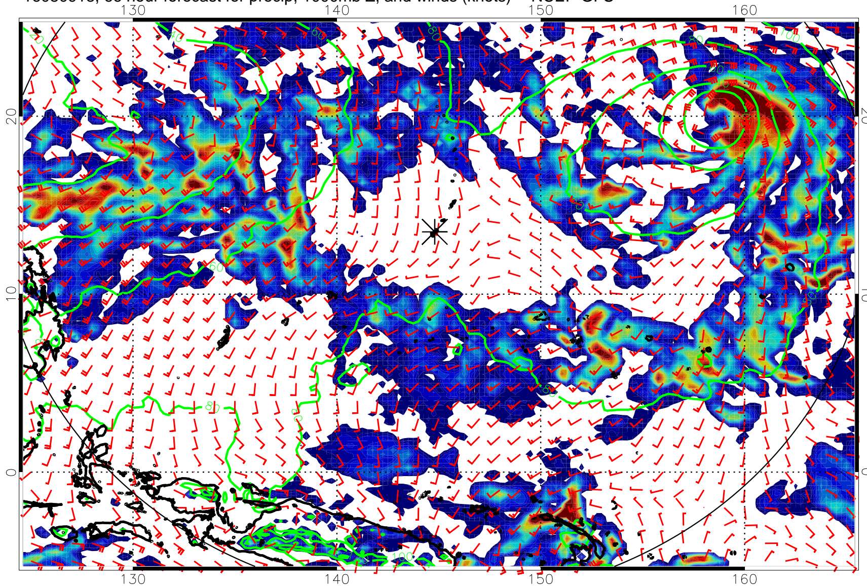
16080918, 66 hour forecast for precip, 1000mb Z, and winds (knots) -- NCEP GFS
