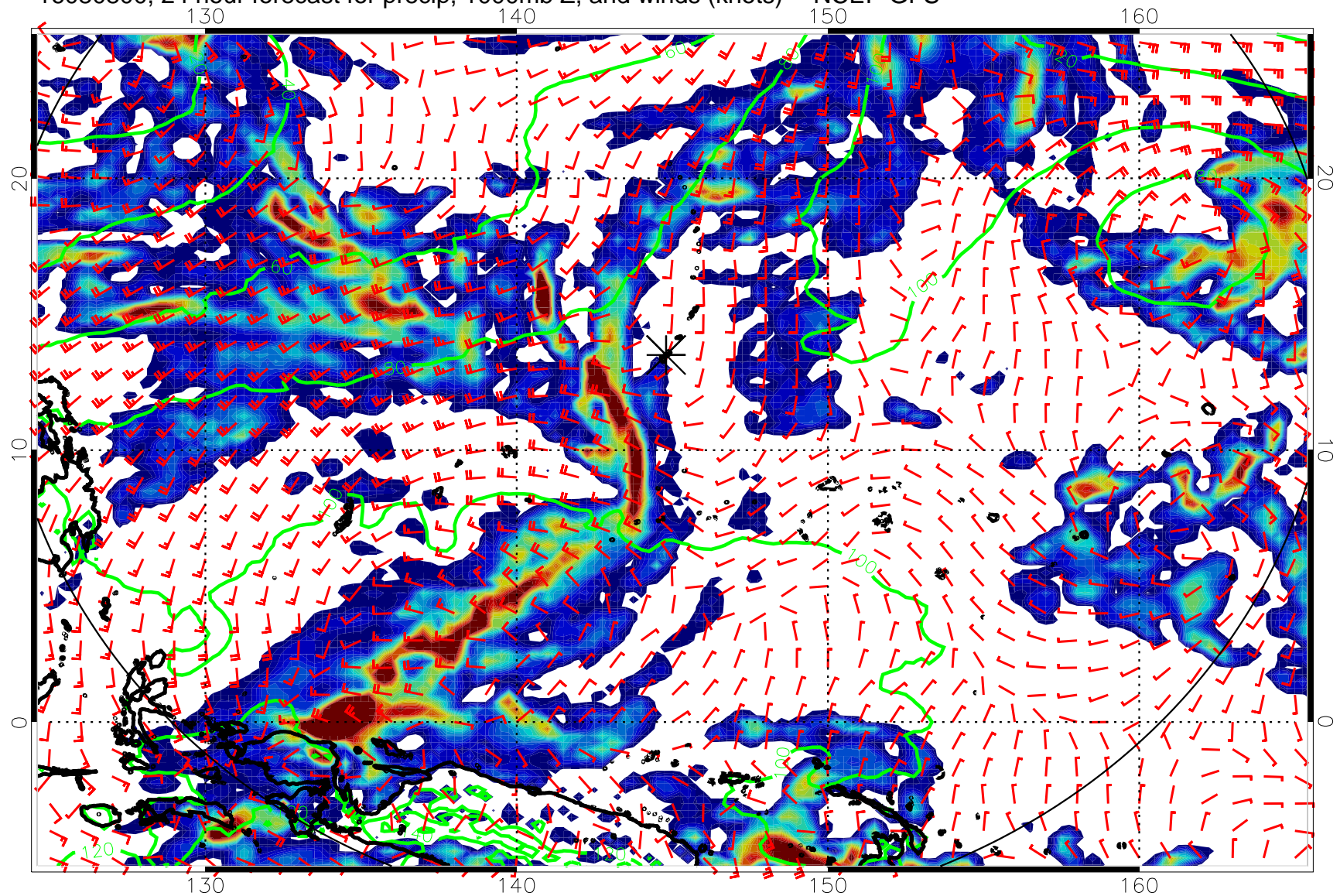
16080800, 24 hour forecast for precip, 1000mb Z, and winds (knots) -- NCEP GFS
