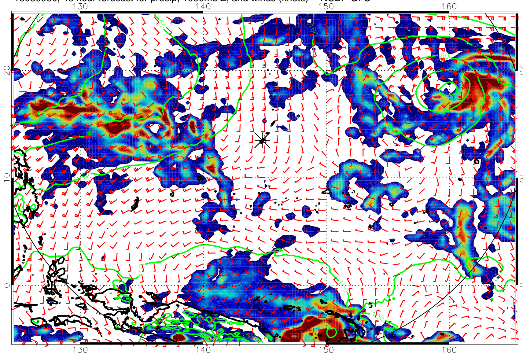
16080900, 48 hour forecast for precip, 1000mb Z, and winds (knots) -- NCEP GFS
