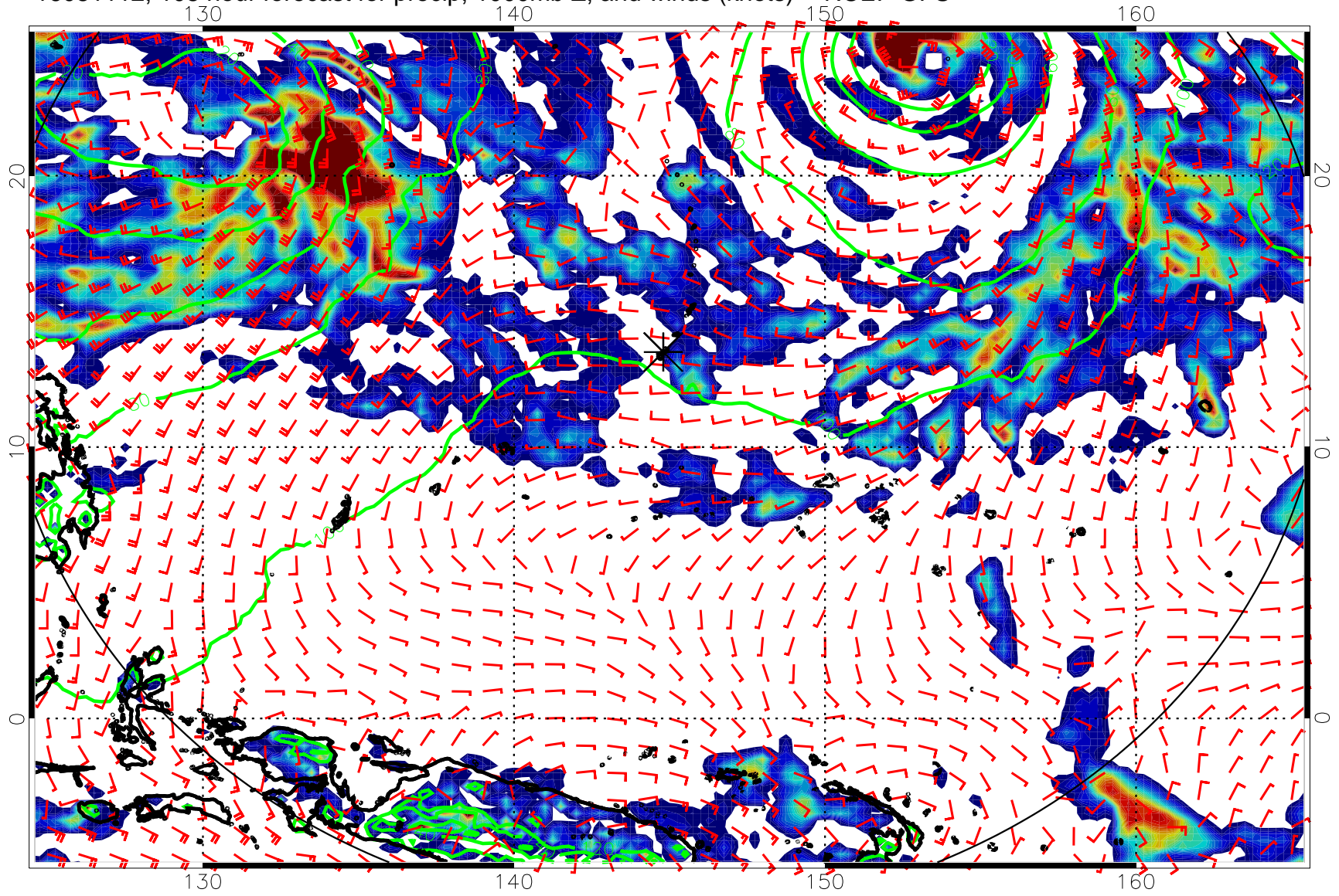
16081112, 108 hour forecast for precip, 1000mb Z, and winds (knots) -- NCEP GFS
