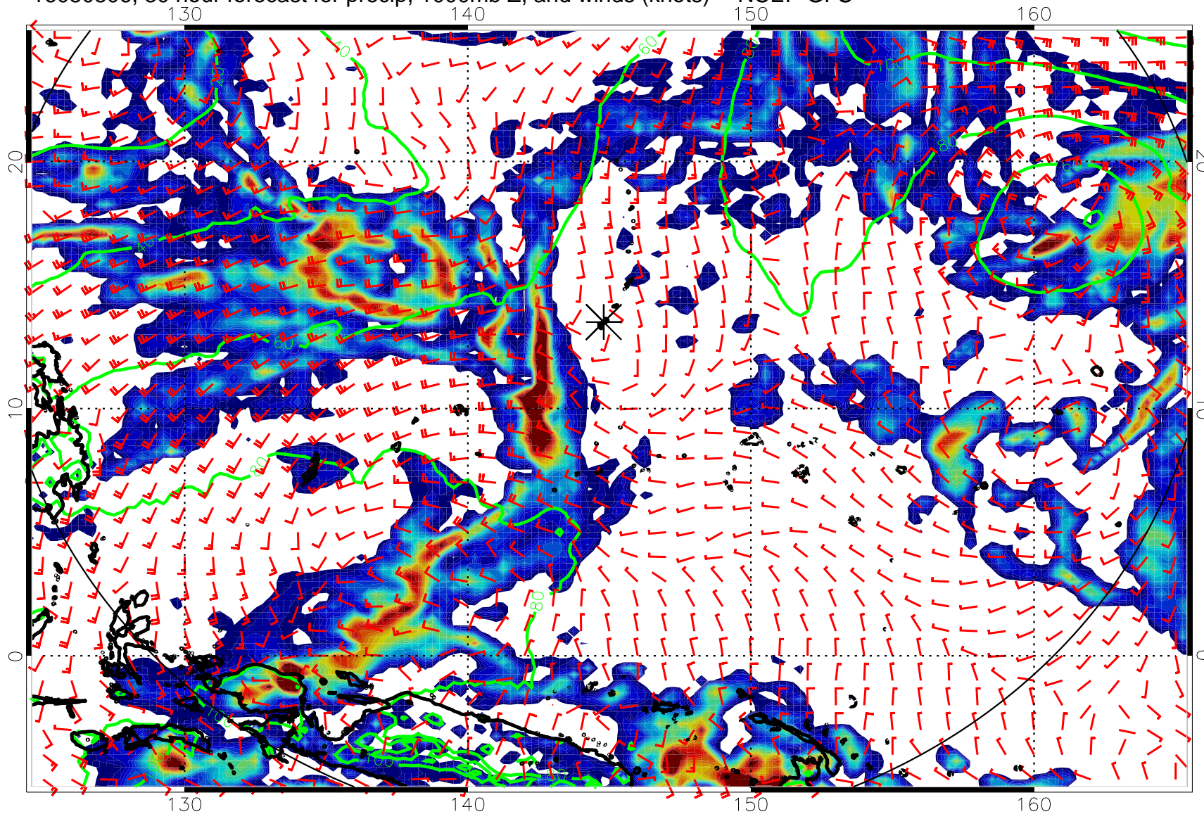
16080806, 30 hour forecast for precip, 1000mb Z, and winds (knots) -- NCEP GFS
