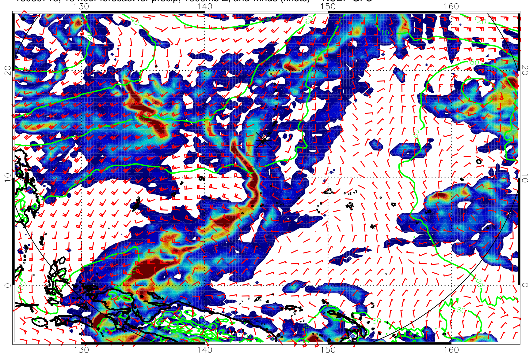
16080718, 18 hour forecast for precip, 1000mb Z, and winds (knots) -- NCEP GFS
