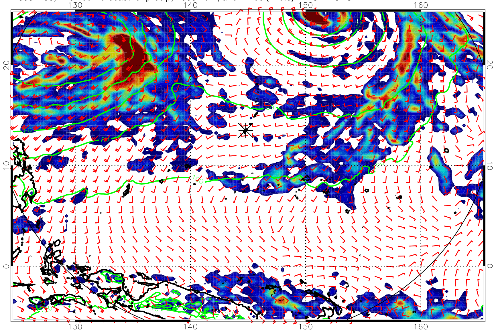
16081200, 120 hour forecast for precip, 1000mb Z, and winds (knots) -- NCEP GFS
