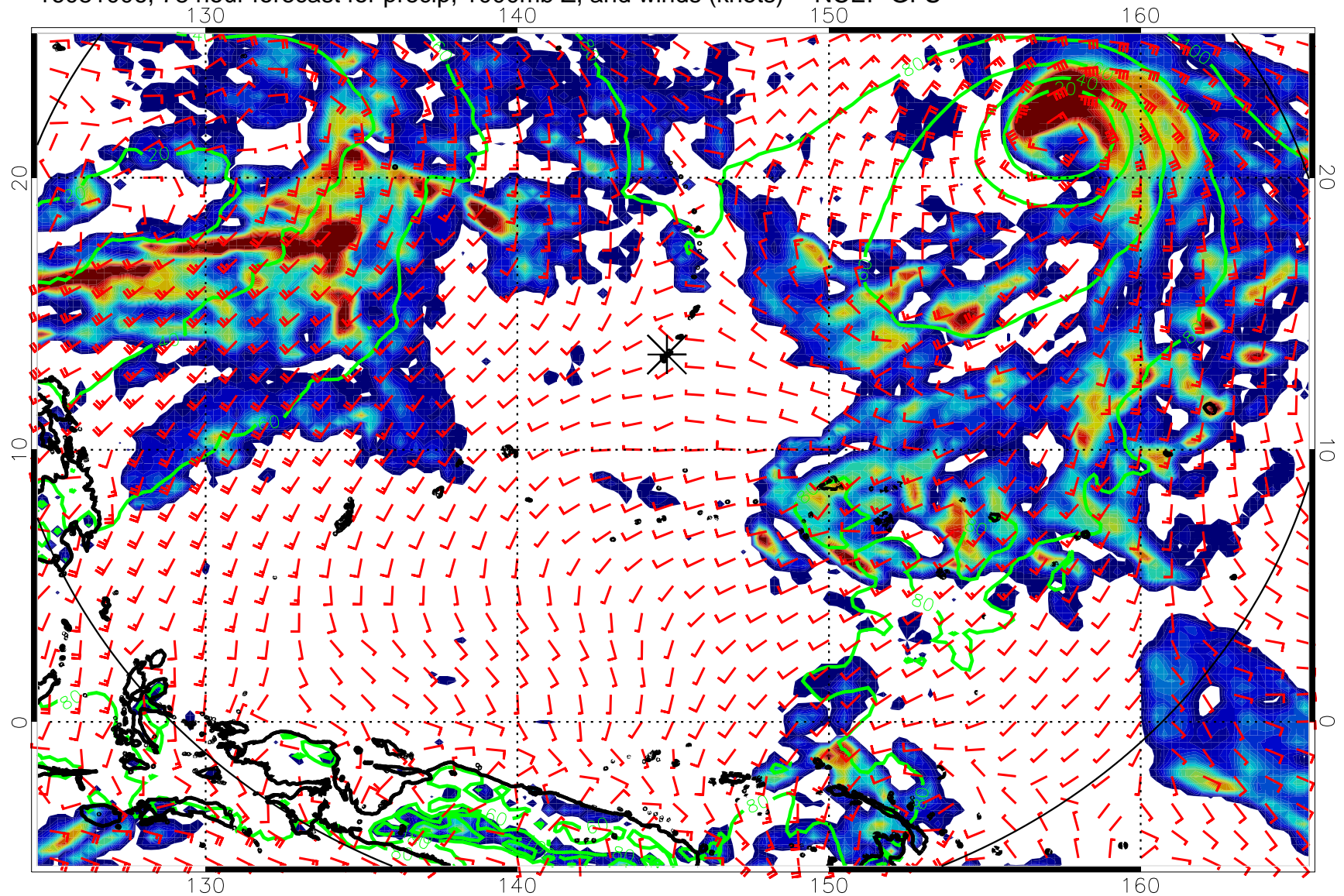
16081006, 78 hour forecast for precip, 1000mb Z, and winds (knots) -- NCEP GFS
