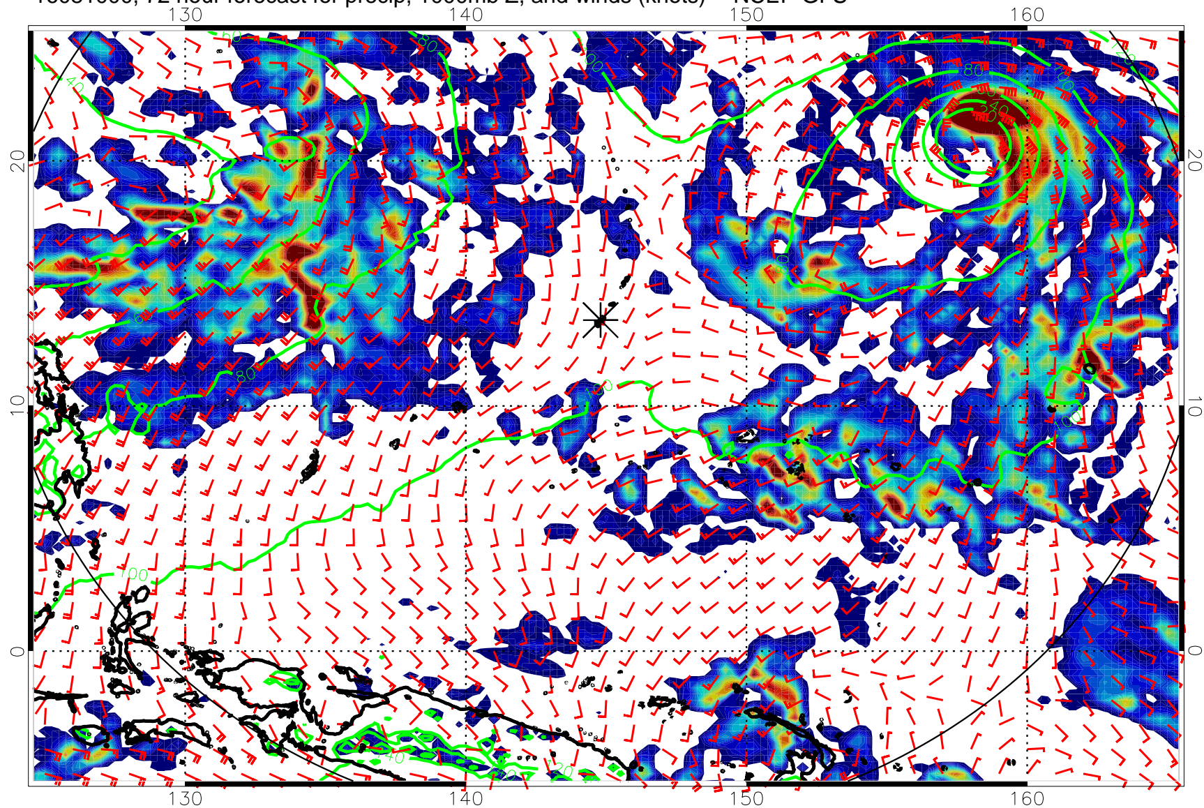
16081000, 72 hour forecast for precip, 1000mb Z, and winds (knots) -- NCEP GFS
