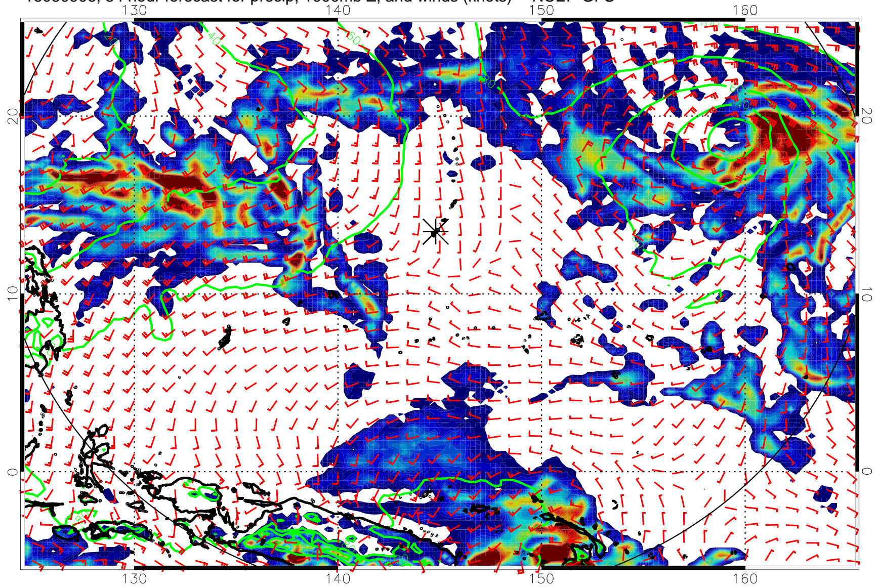
16080906, 54 hour forecast for precip, 1000mb Z, and winds (knots) -- NCEP GFS
