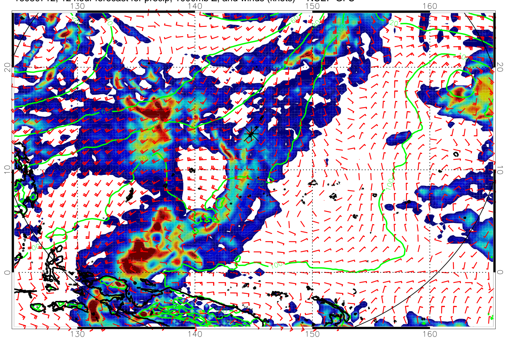
16080712, 12 hour forecast for precip, 1000mb Z, and winds (knots) -- NCEP GFS
