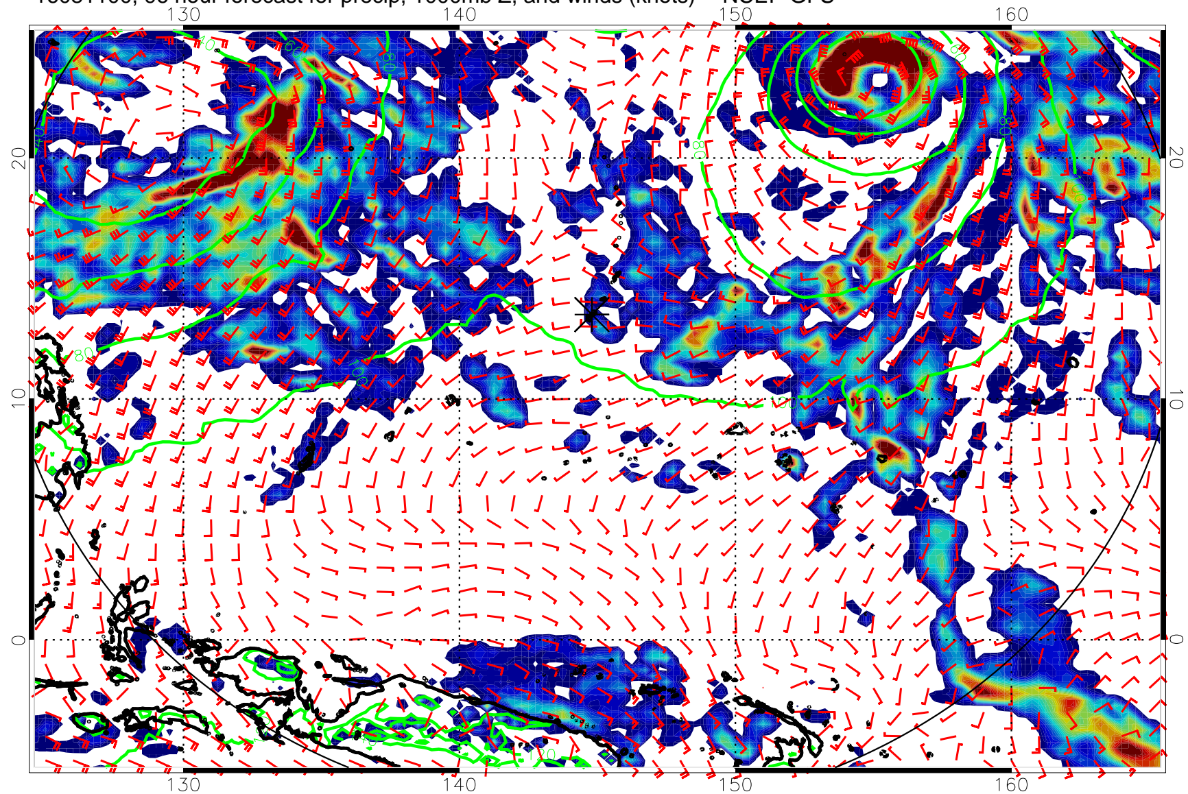
16081100, 96 hour forecast for precip, 1000mb Z, and winds (knots) -- NCEP GFS
