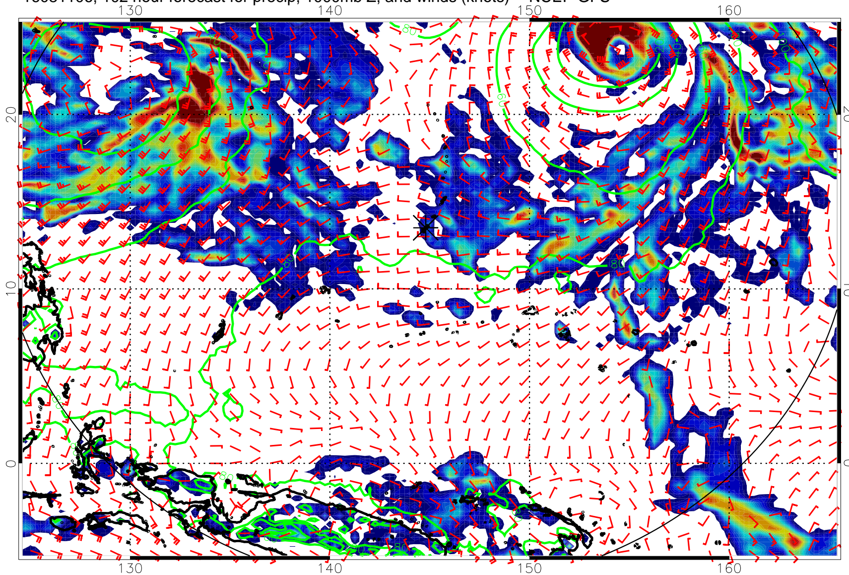
16081106, 102 hour forecast for precip, 1000mb Z, and winds (knots) -- NCEP GFS
