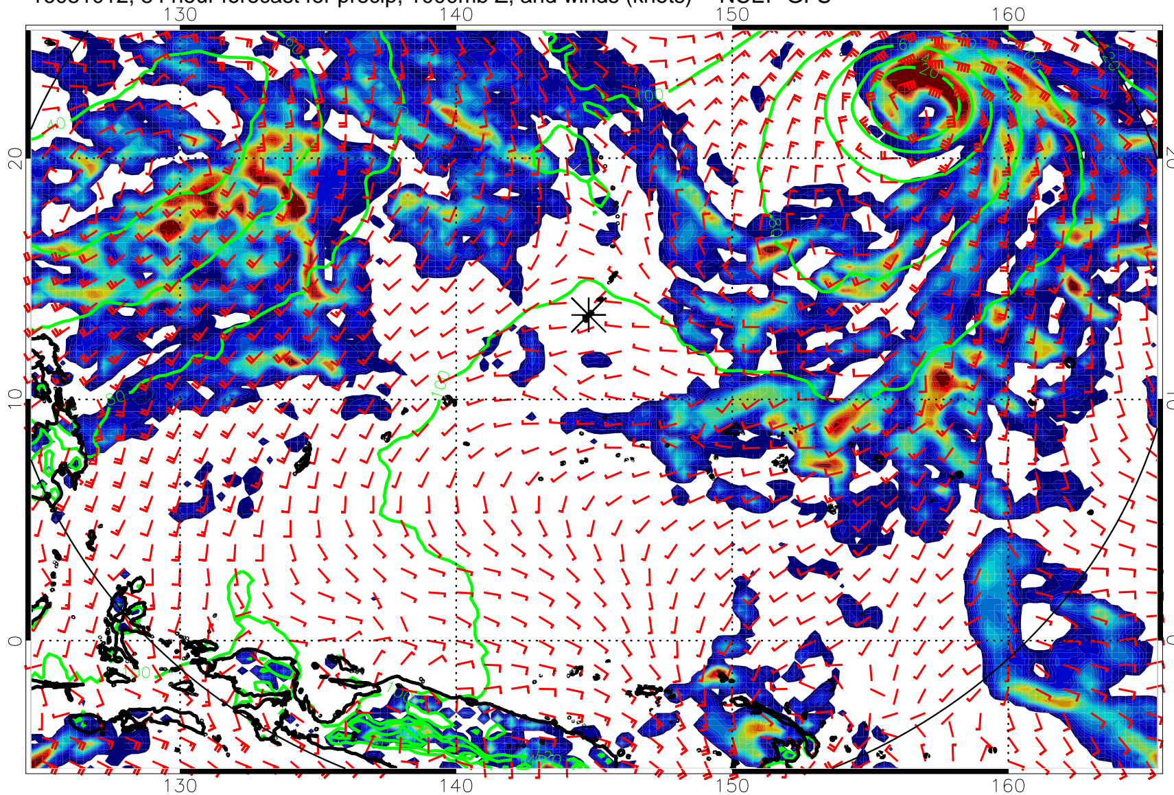
16081012, 84 hour forecast for precip, 1000mb Z, and winds (knots) -- NCEP GFS
