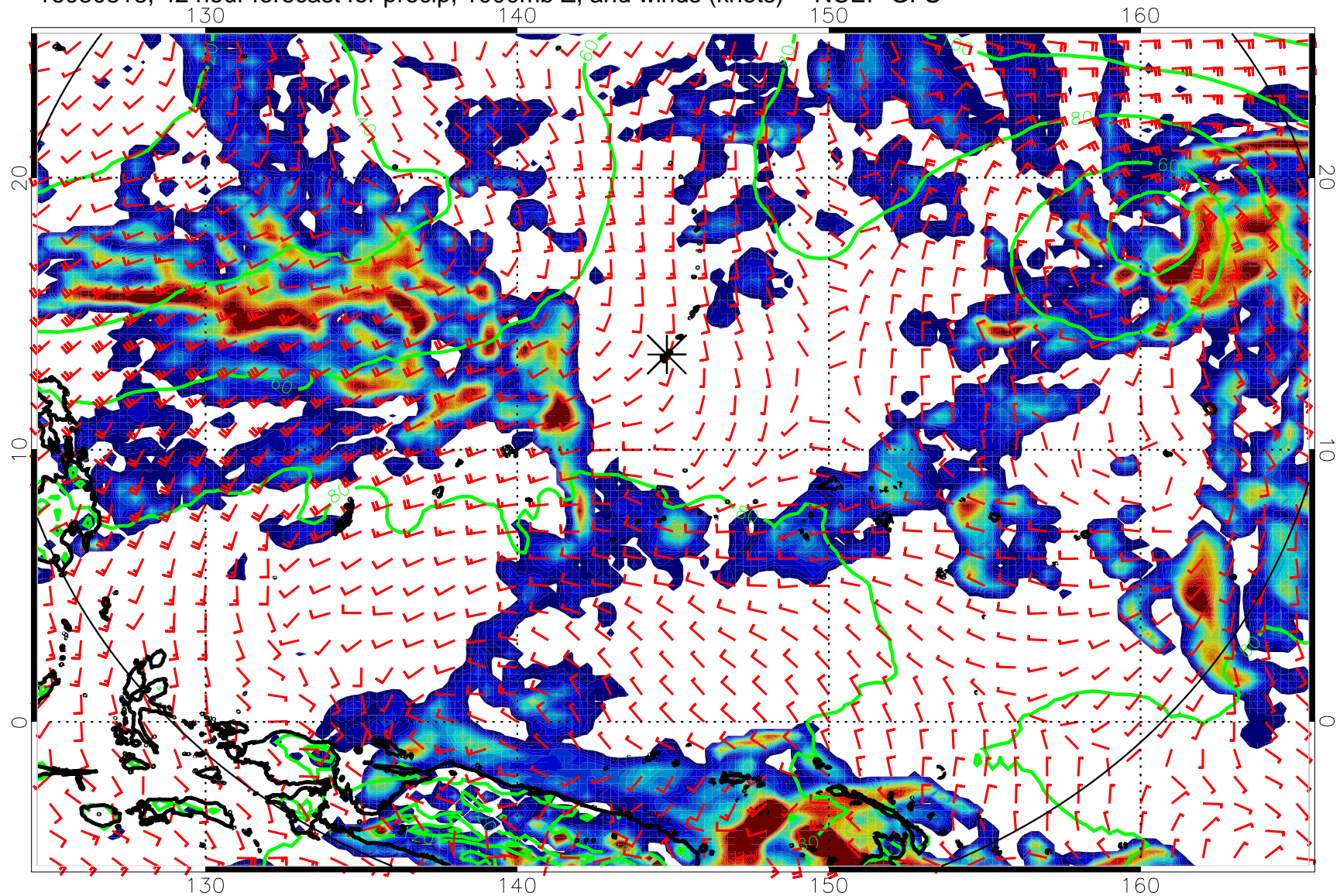
16080818, 42 hour forecast for precip, 1000mb Z, and winds (knots) -- NCEP GFS
