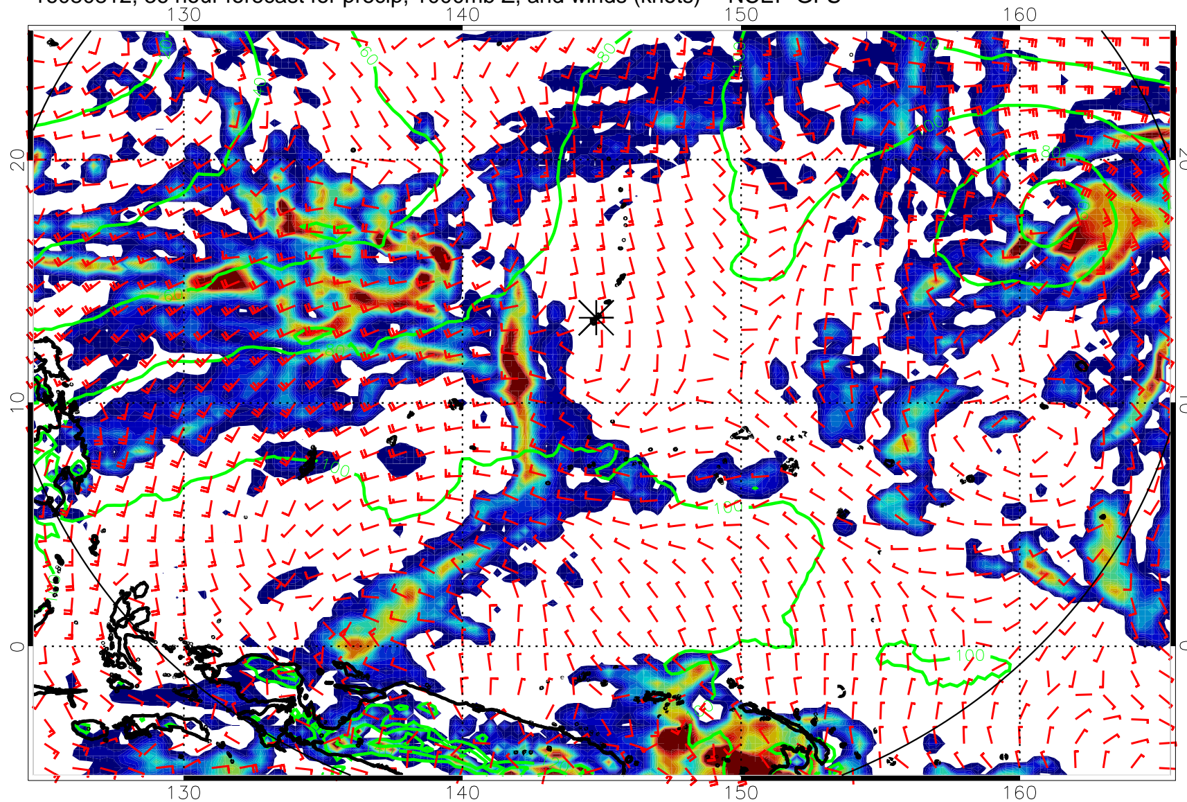
16080812, 36 hour forecast for precip, 1000mb Z, and winds (knots) -- NCEP GFS
