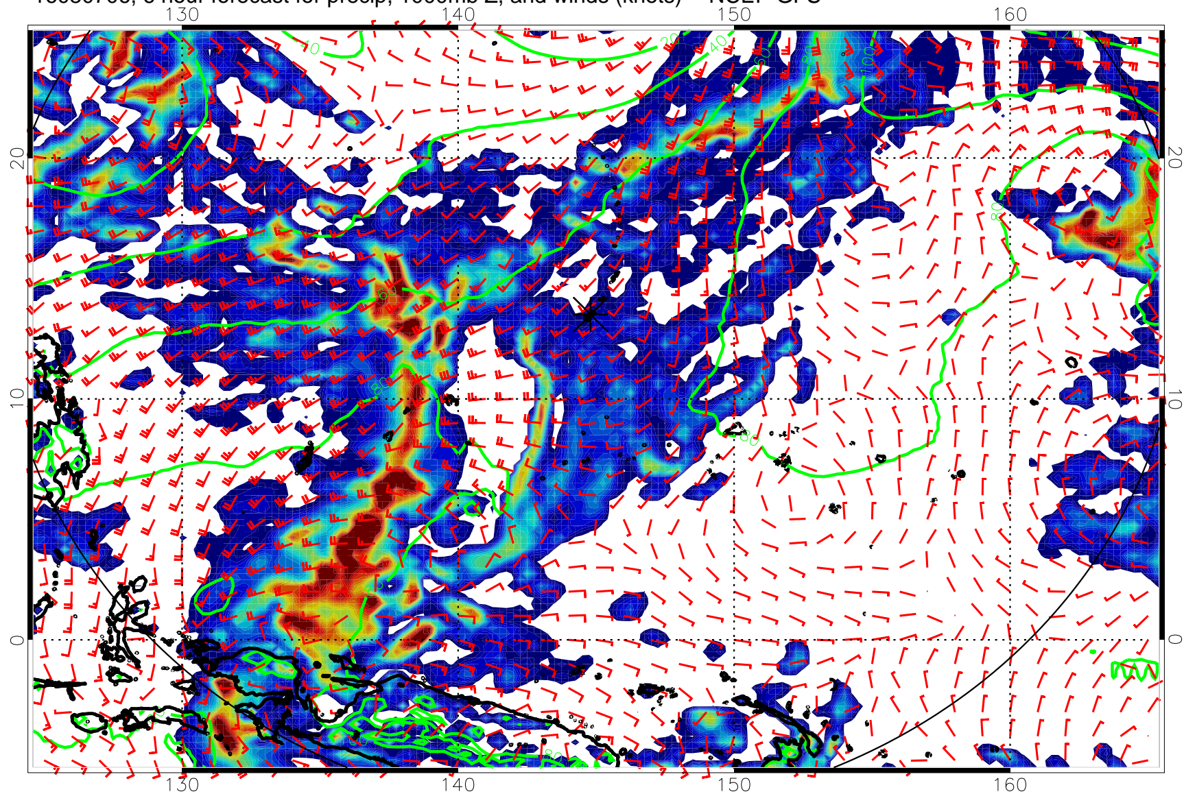
16080706, 6 hour forecast for precip, 1000mb Z, and winds (knots) -- NCEP GFS
