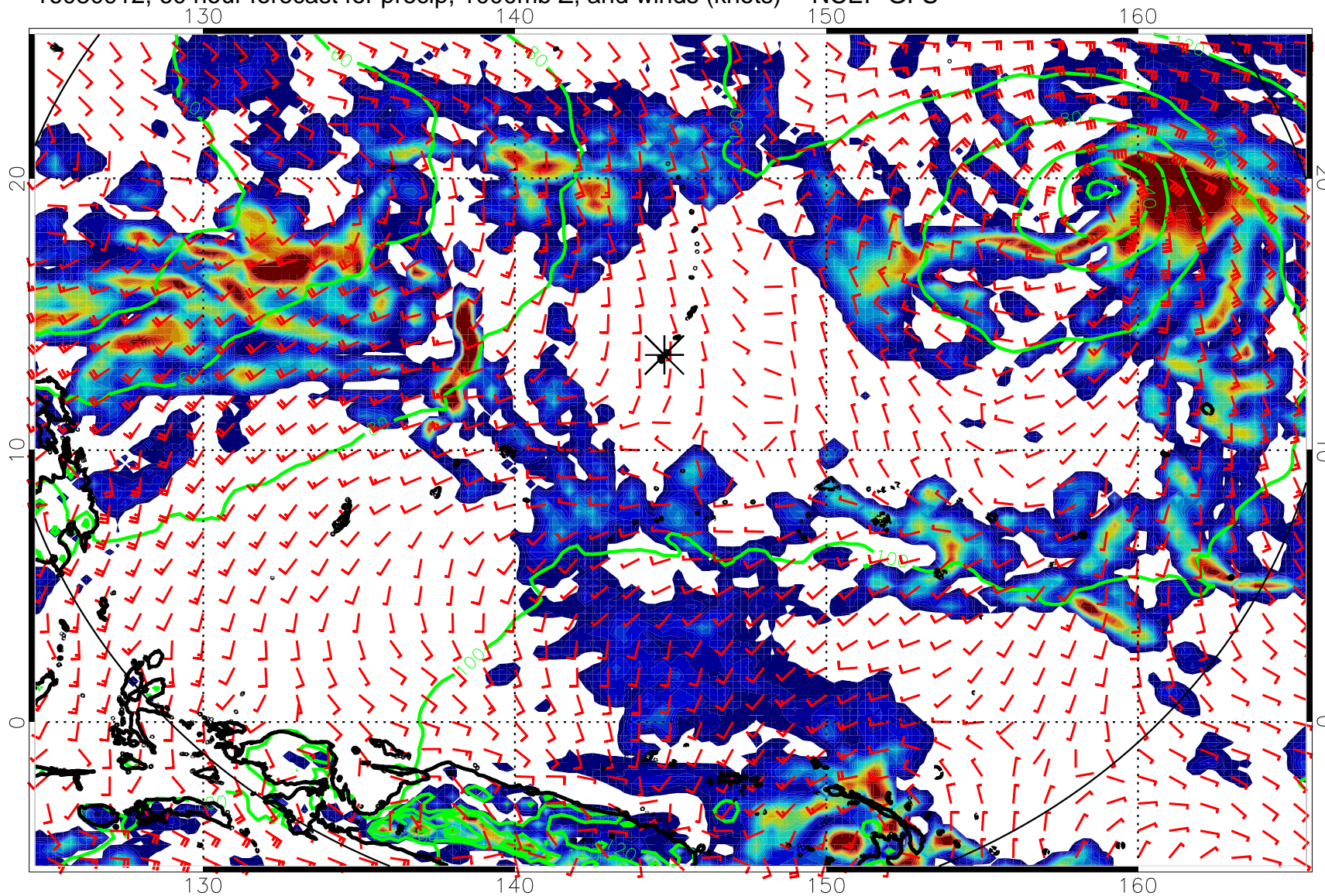
16080912, 60 hour forecast for precip, 1000mb Z, and winds (knots) -- NCEP GFS
