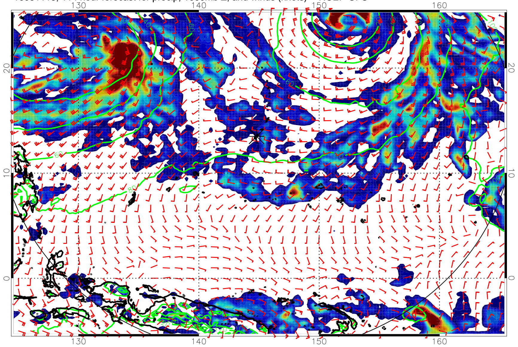
16081118, 114 hour forecast for precip, 1000mb Z, and winds (knots) -- NCEP GFS
