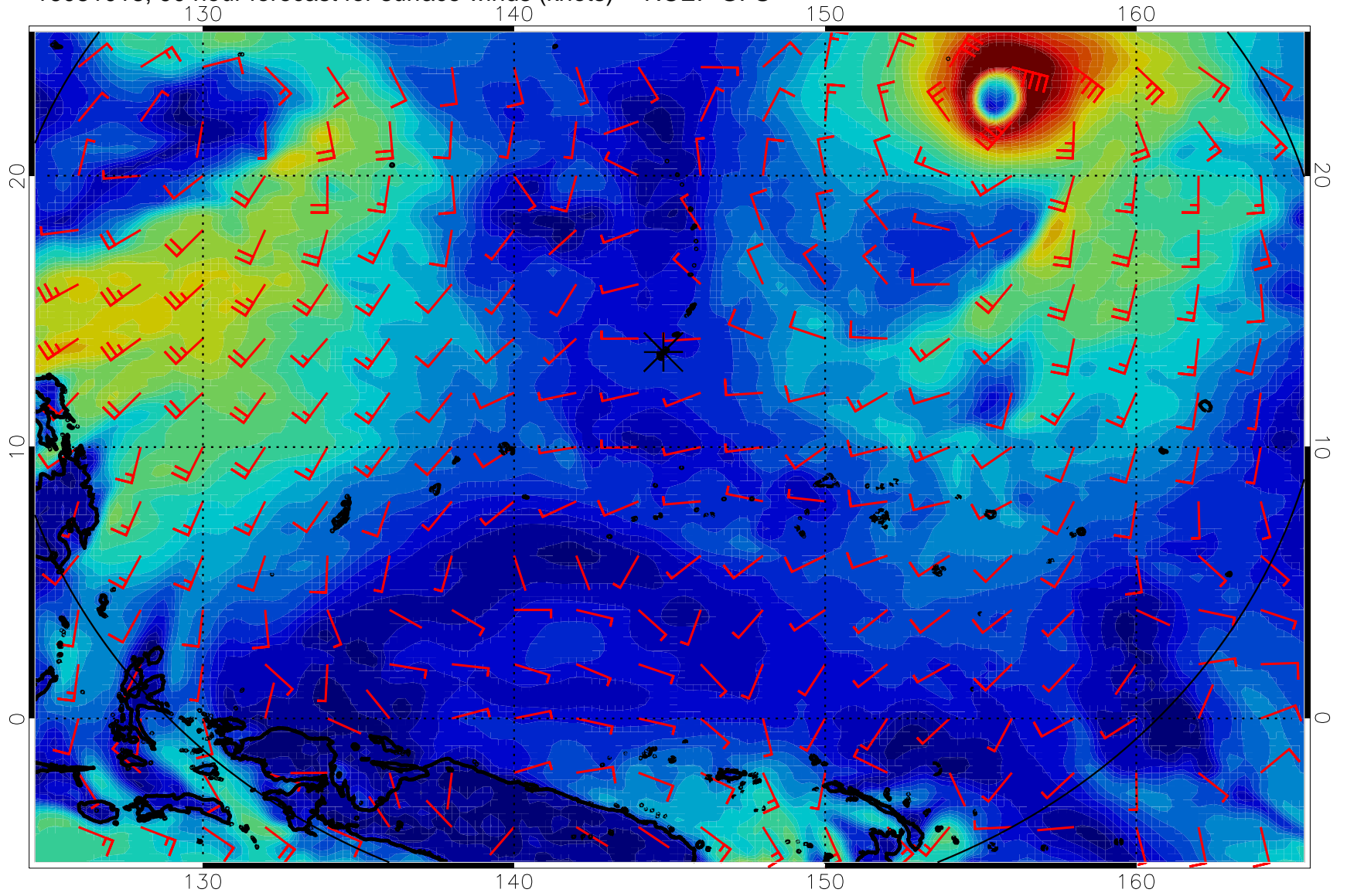
16081018, 90 hour forecast for surface winds (knots) -- NCEP GFS
