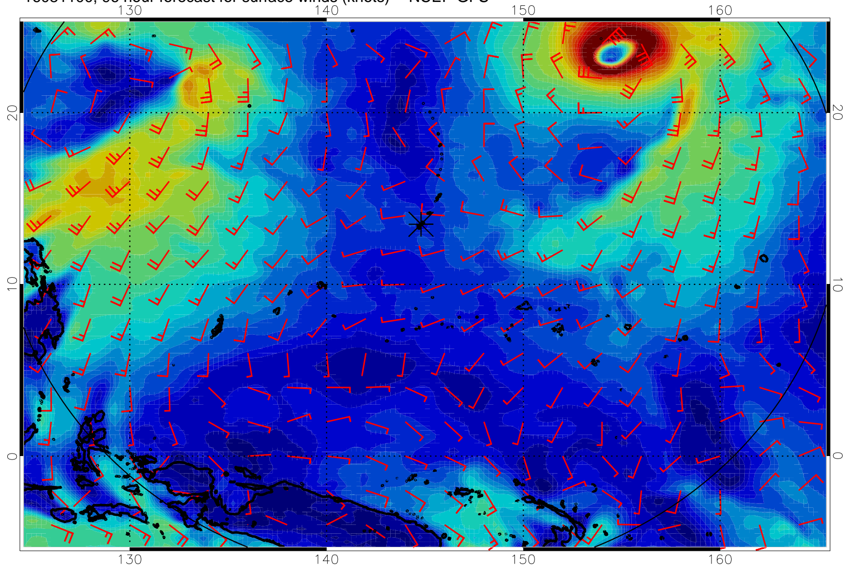
16081100, 96 hour forecast for surface winds (knots) -- NCEP GFS
