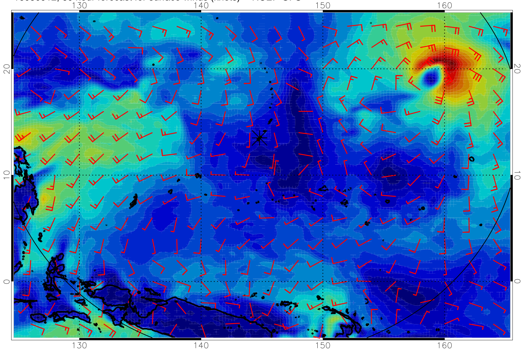
16080912, 60 hour forecast for surface winds (knots) -- NCEP GFS
