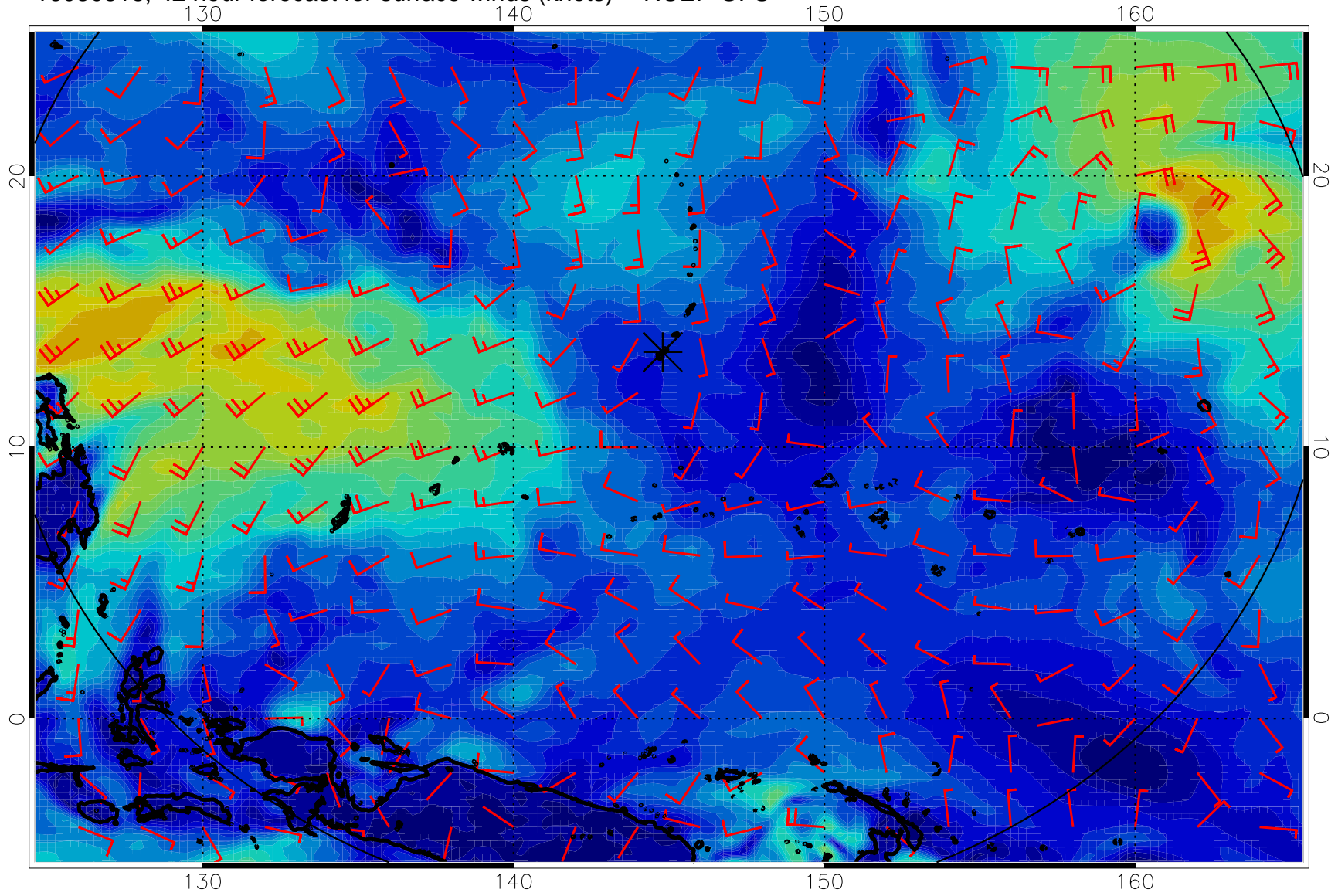
16080818, 42 hour forecast for surface winds (knots) -- NCEP GFS
