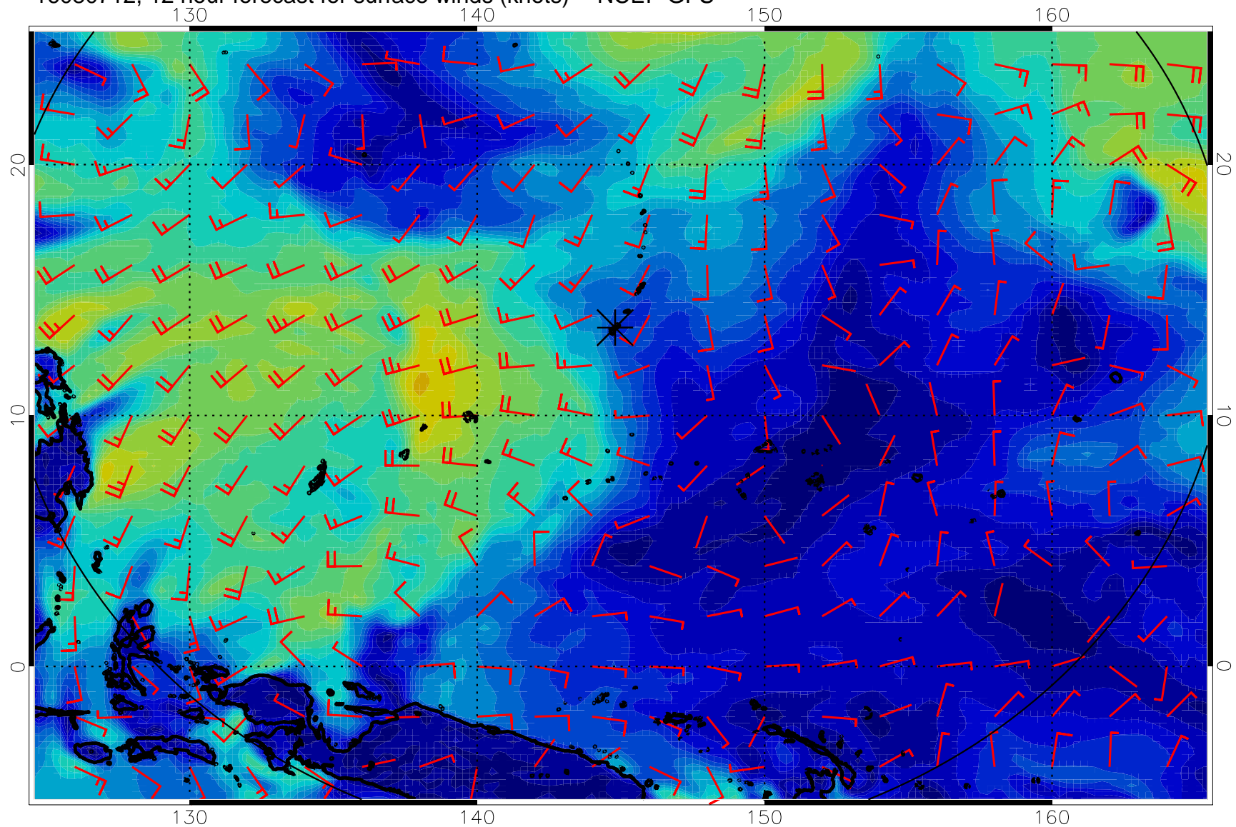
16080712, 12 hour forecast for surface winds (knots) -- NCEP GFS
