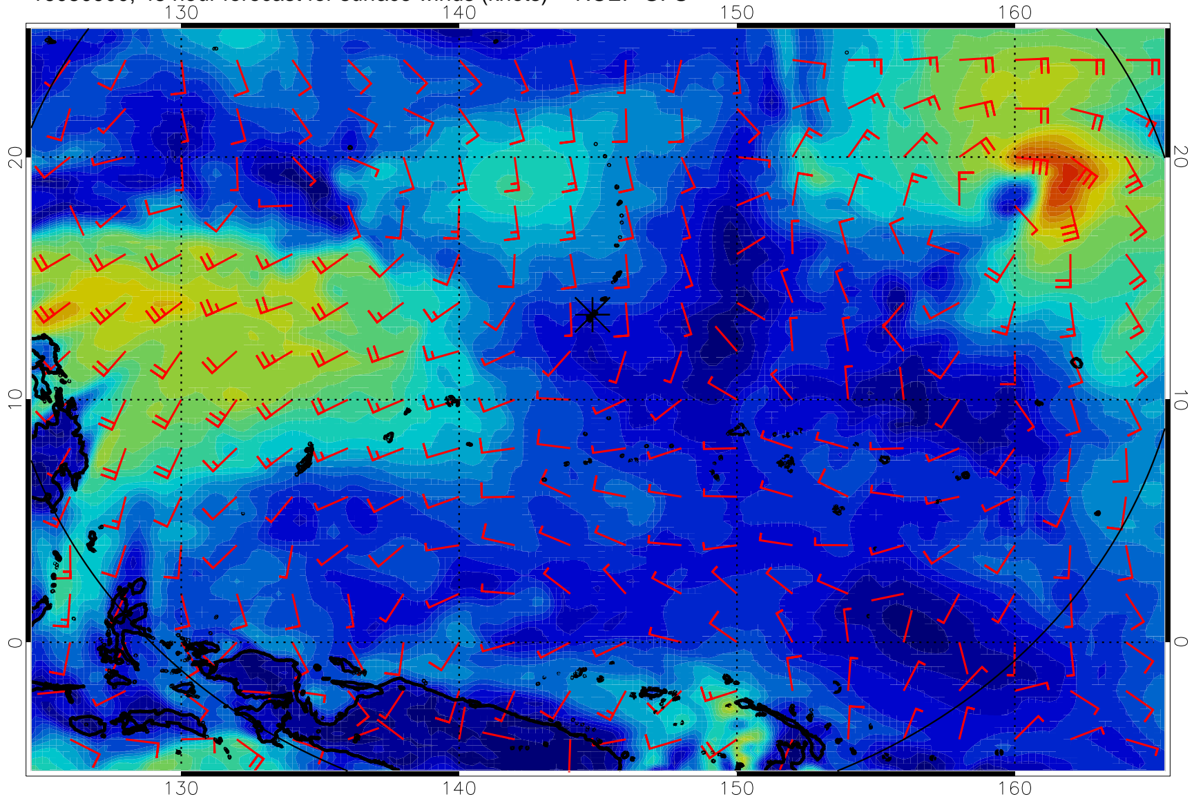
16080900, 48 hour forecast for surface winds (knots) -- NCEP GFS
