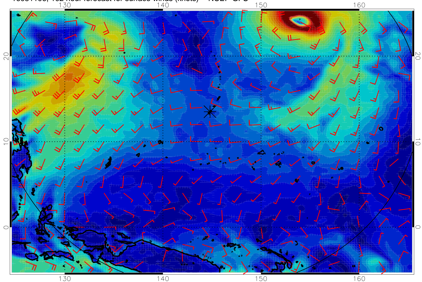
16081106, 102 hour forecast for surface winds (knots) -- NCEP GFS
