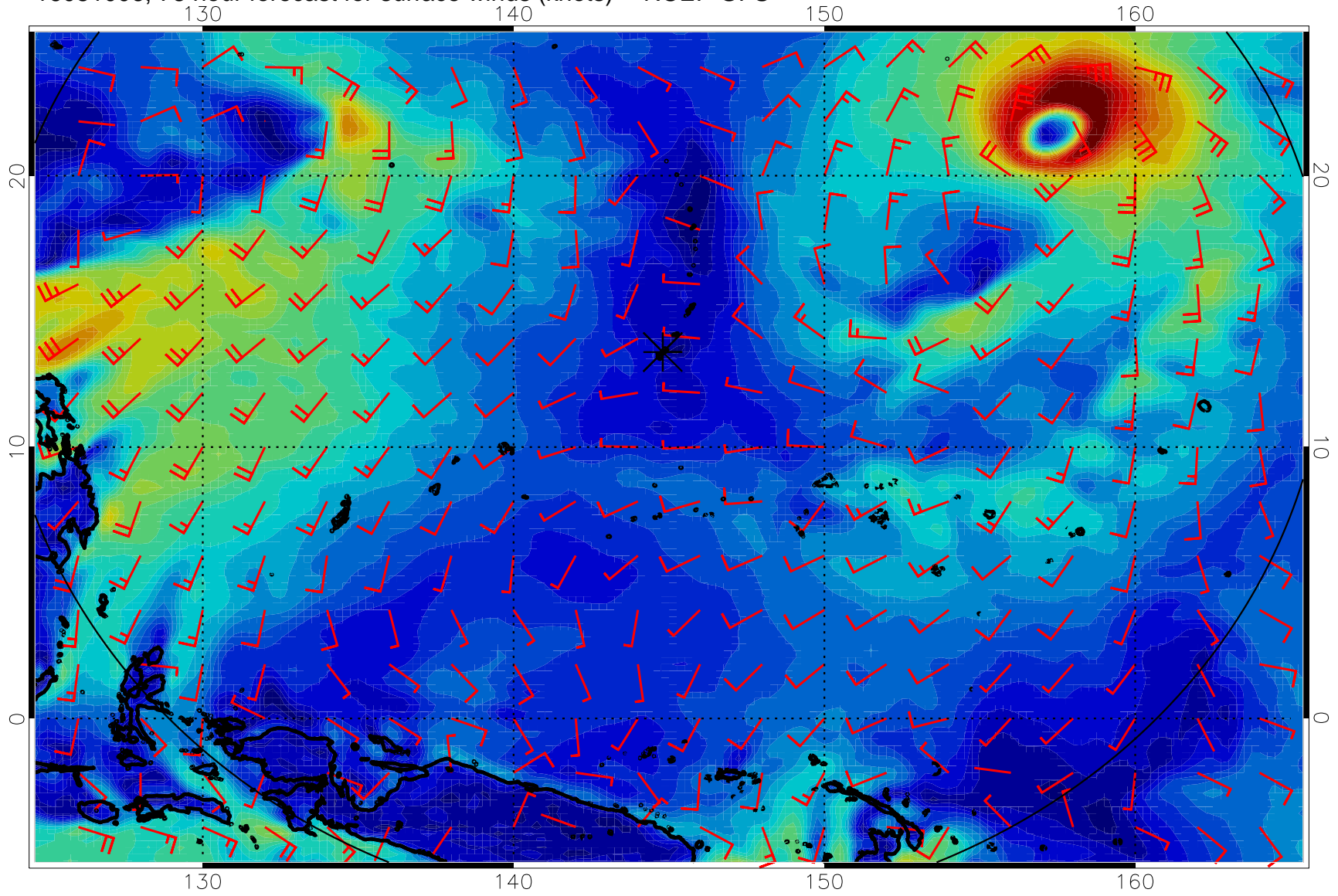
16081006, 78 hour forecast for surface winds (knots) -- NCEP GFS
