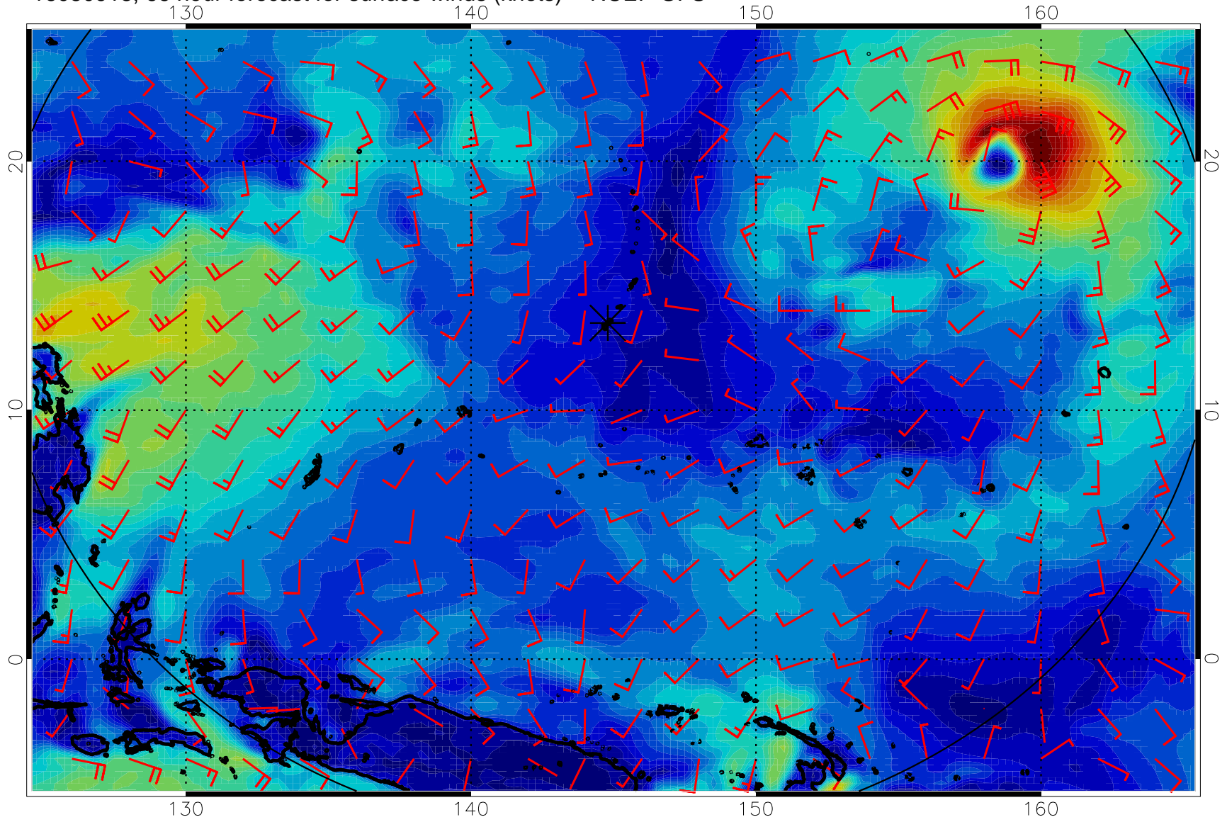
16080918, 66 hour forecast for surface winds (knots) -- NCEP GFS
