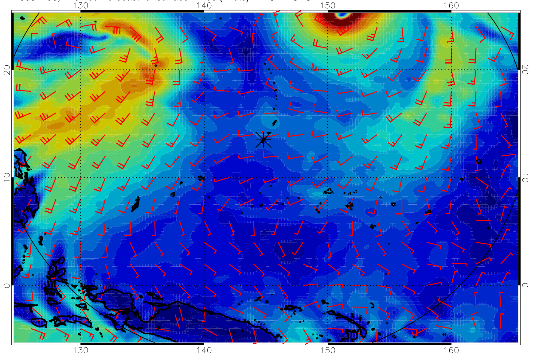
16081200, 120 hour forecast for surface winds (knots) -- NCEP GFS
