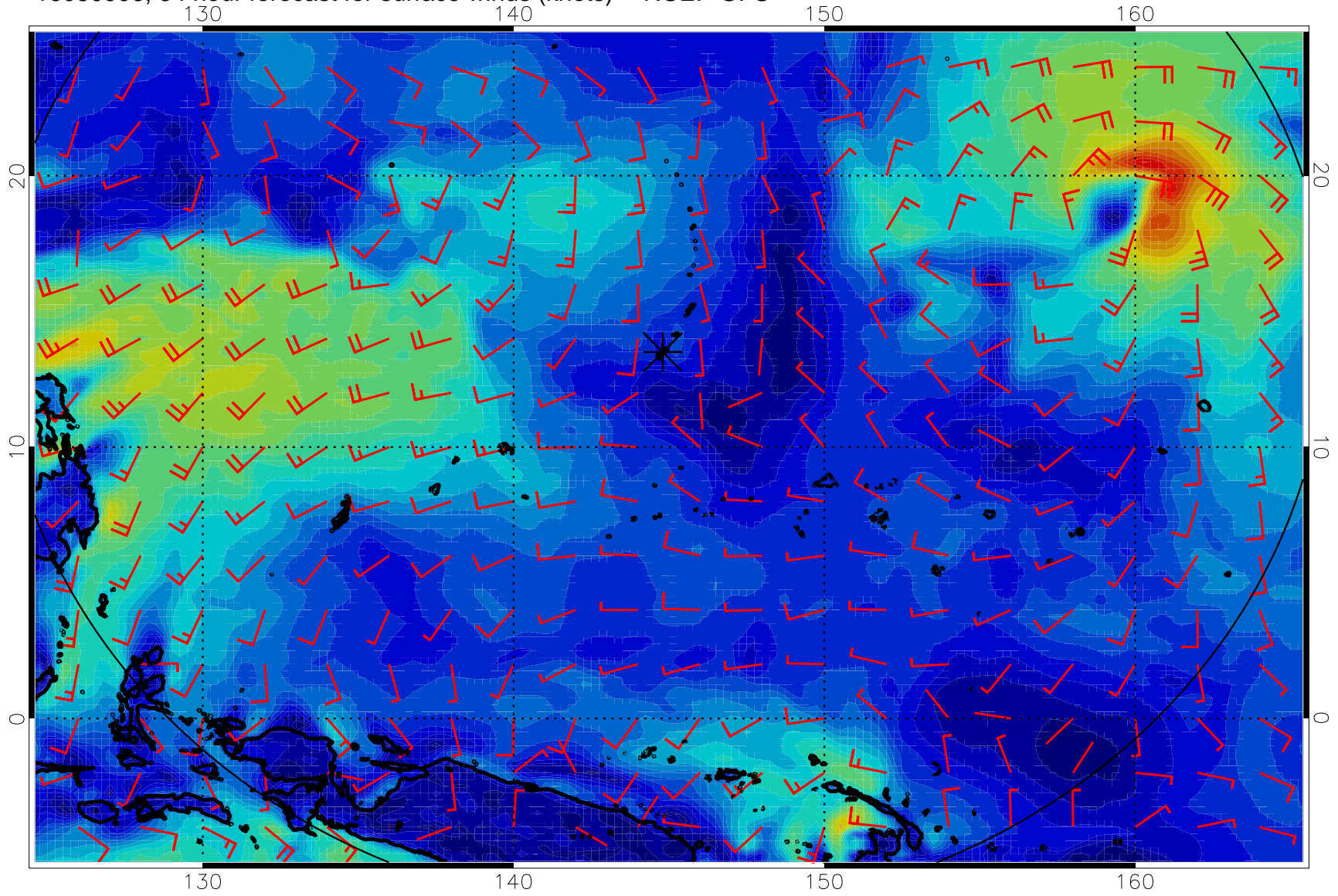
16080906, 54 hour forecast for surface winds (knots) -- NCEP GFS
