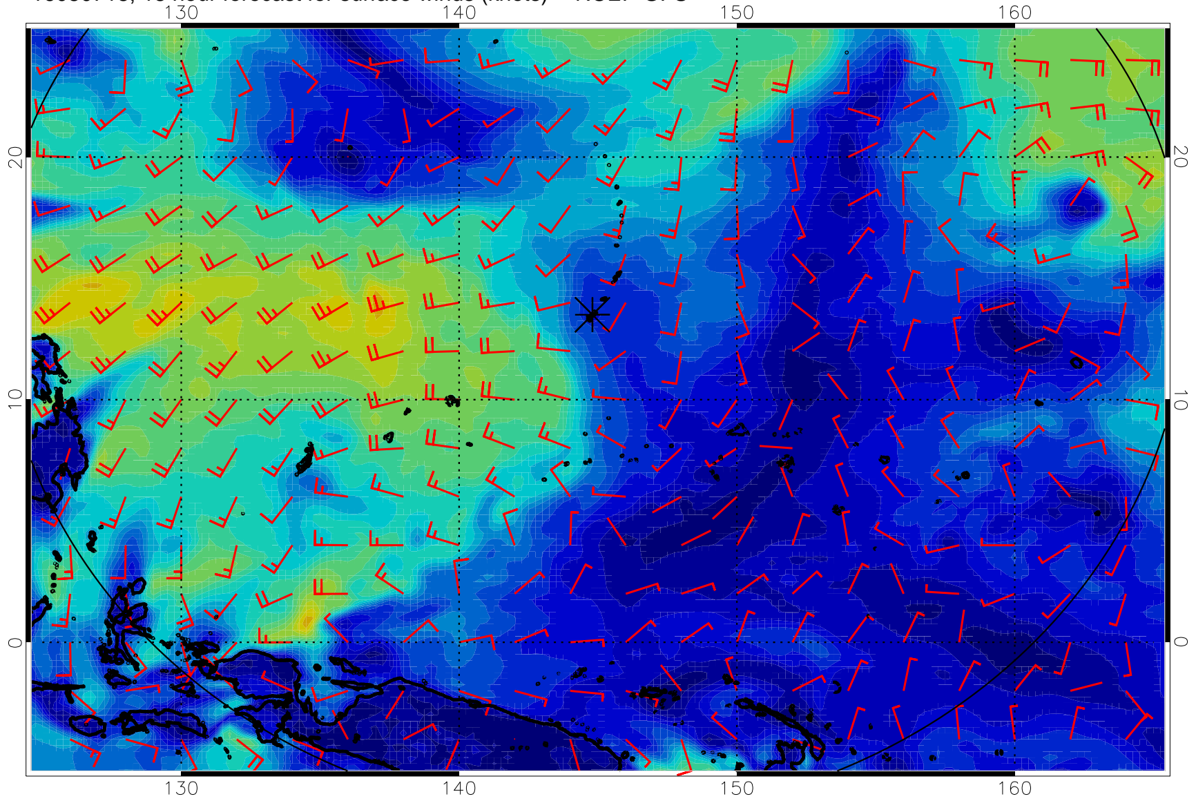
16080718, 18 hour forecast for surface winds (knots) -- NCEP GFS
