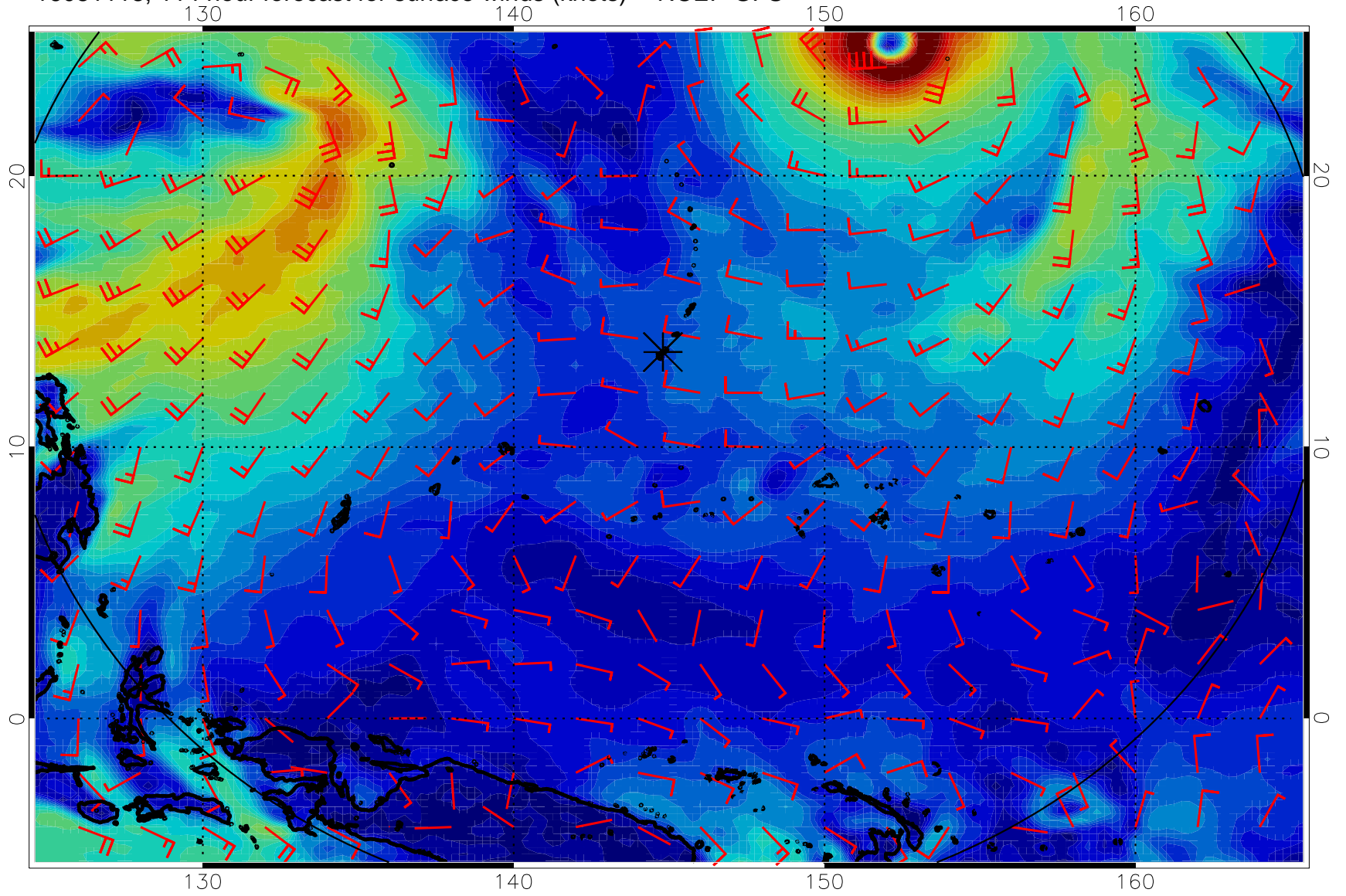
16081118, 114 hour forecast for surface winds (knots) -- NCEP GFS
