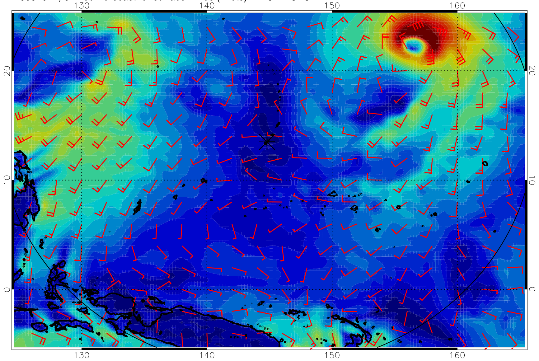
16081012, 84 hour forecast for surface winds (knots) -- NCEP GFS
