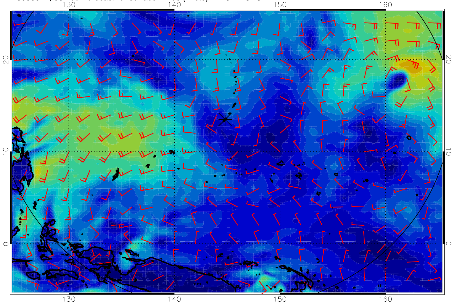
16080812, 36 hour forecast for surface winds (knots) -- NCEP GFS
