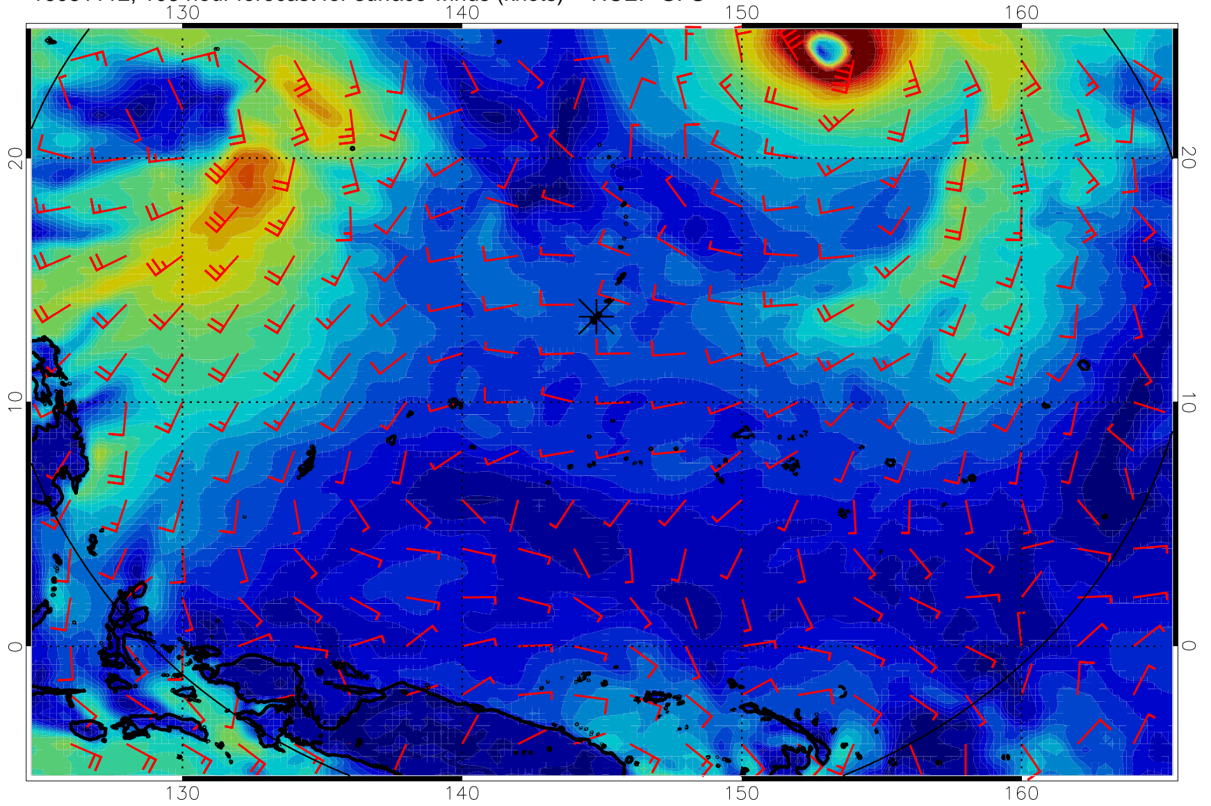
16081112, 108 hour forecast for surface winds (knots) -- NCEP GFS
