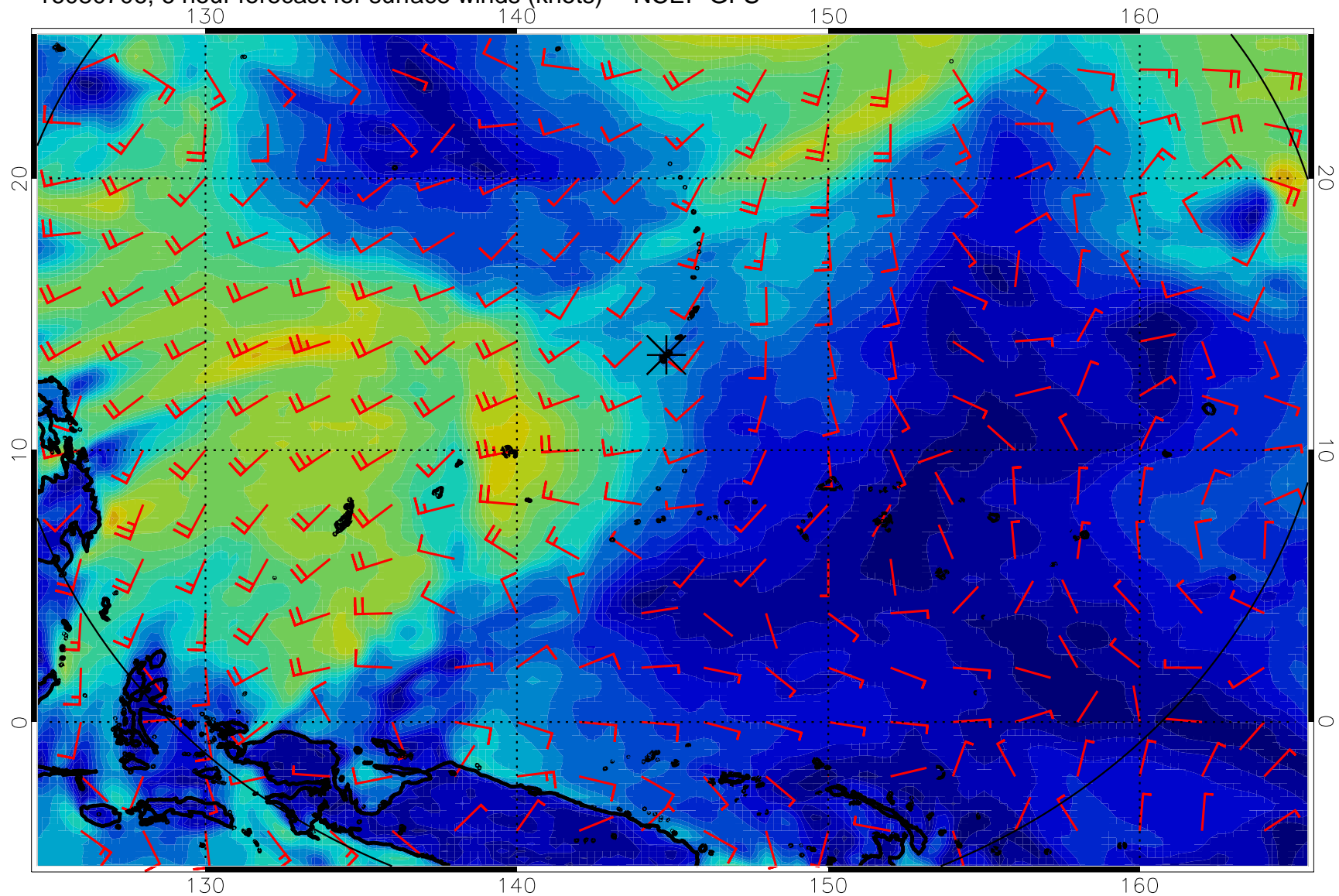
16080706, 6 hour forecast for surface winds (knots) -- NCEP GFS
