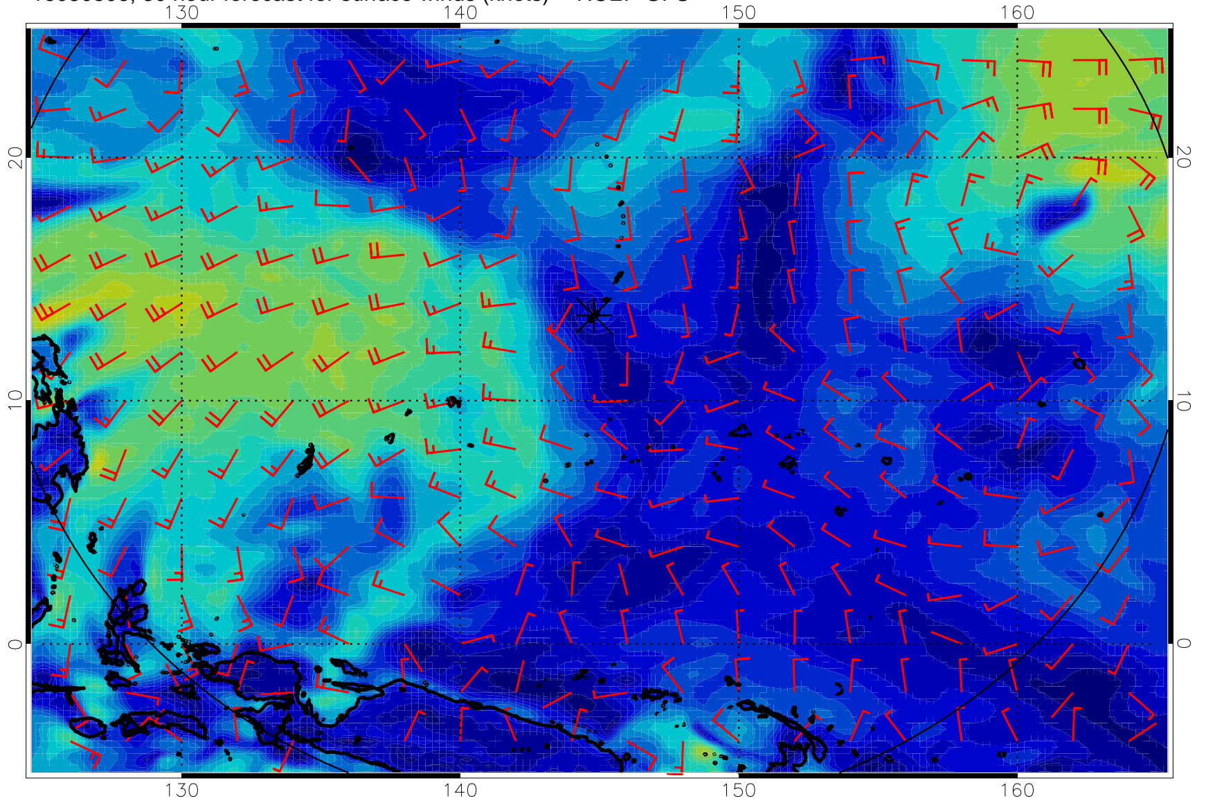
16080806, 30 hour forecast for surface winds (knots) -- NCEP GFS
