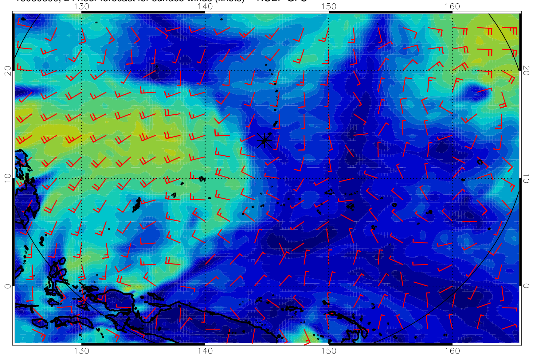
16080800, 24 hour forecast for surface winds (knots) -- NCEP GFS
