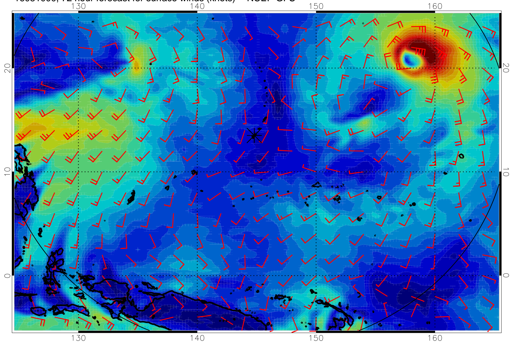
16081000, 72 hour forecast for surface winds (knots) -- NCEP GFS
