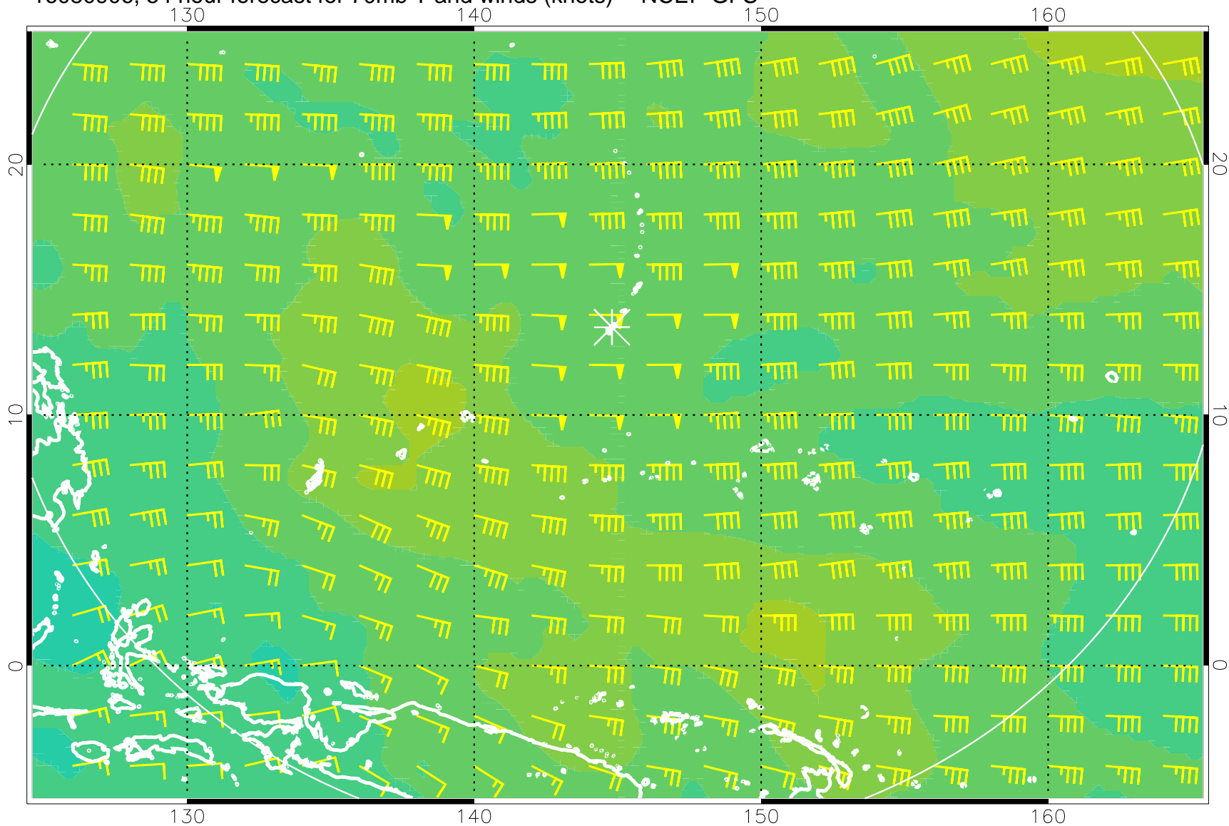
16080906, 54 hour forecast for 70mb T and winds (knots) -- NCEP GFS
