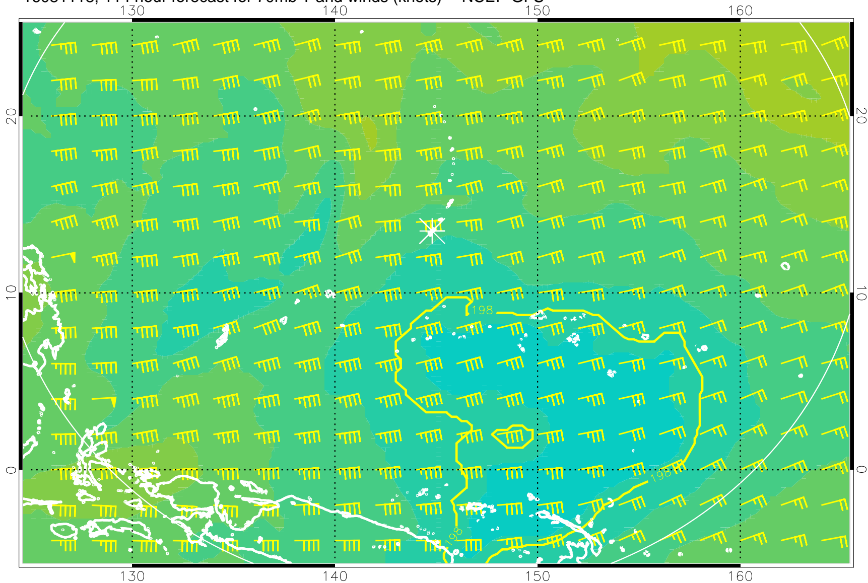
16081118, 114 hour forecast for 70mb T and winds (knots) -- NCEP GFS
