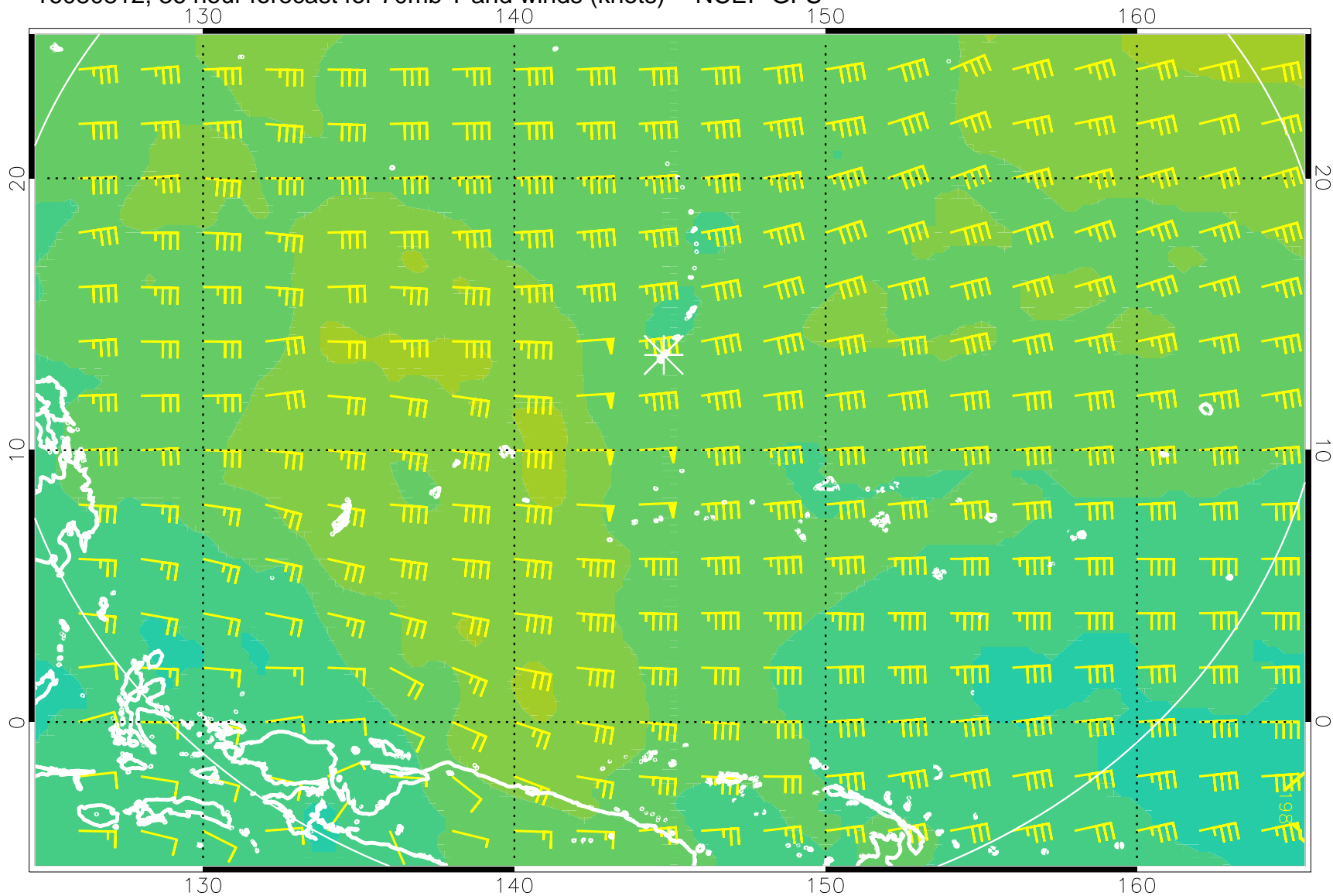
16080812, 36 hour forecast for 70mb T and winds (knots) -- NCEP GFS
