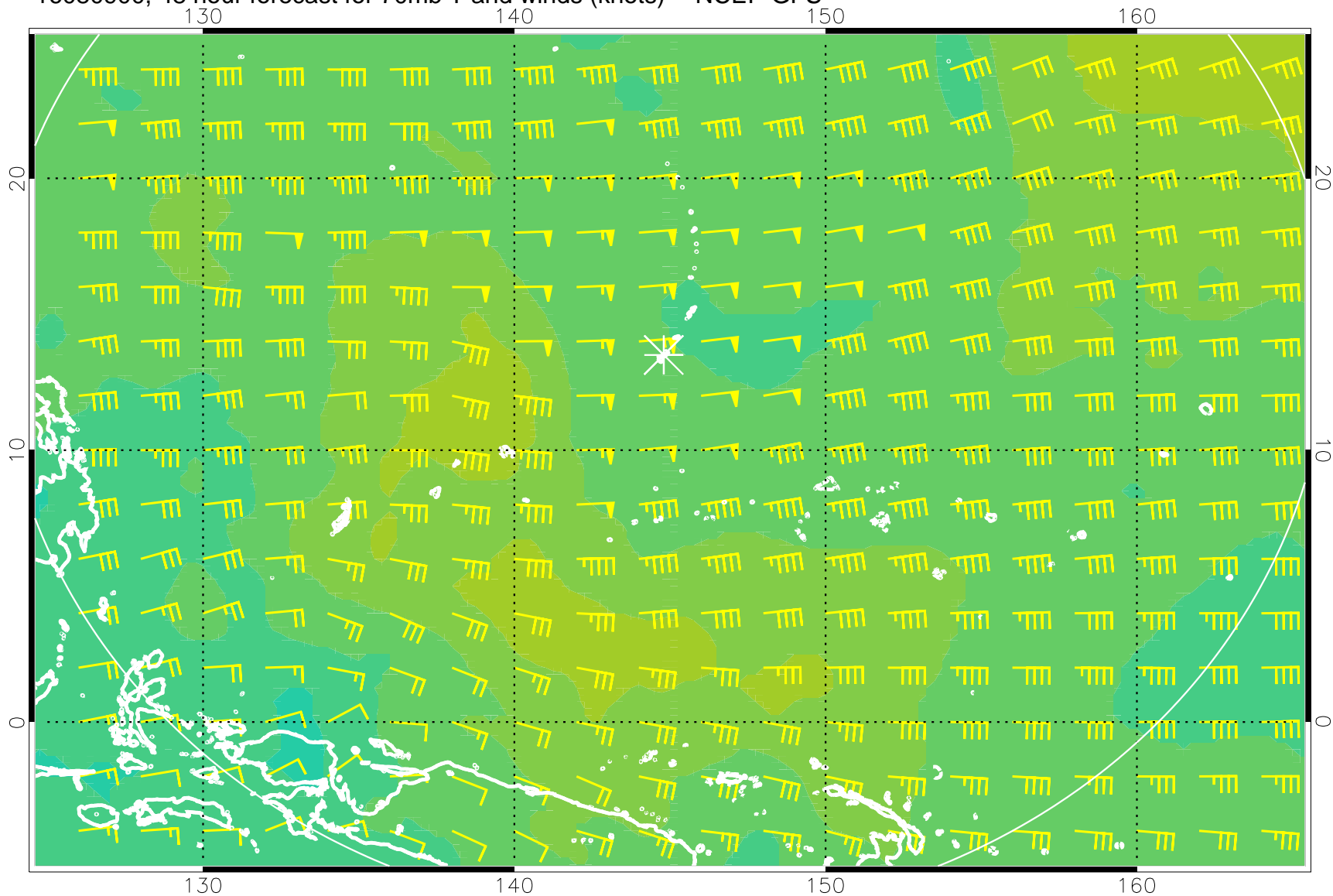
16080900, 48 hour forecast for 70mb T and winds (knots) -- NCEP GFS
