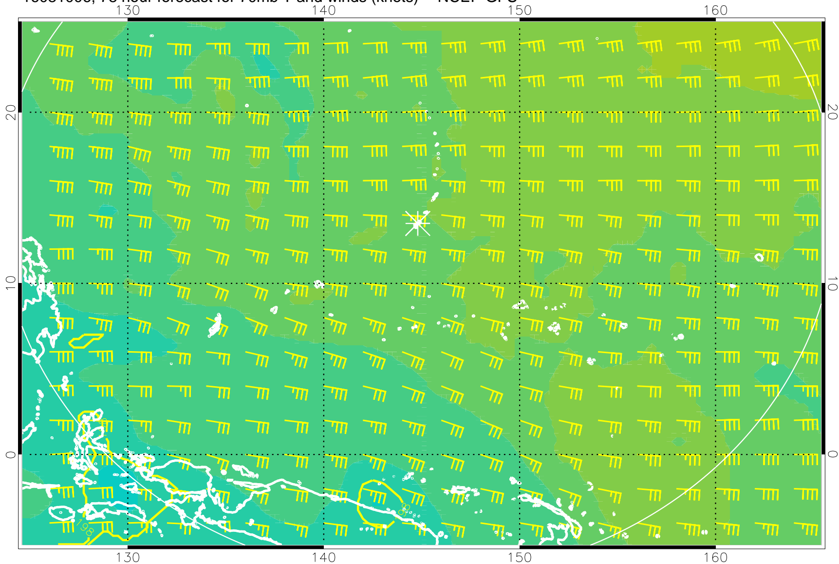
16081006, 78 hour forecast for 70mb T and winds (knots) -- NCEP GFS
