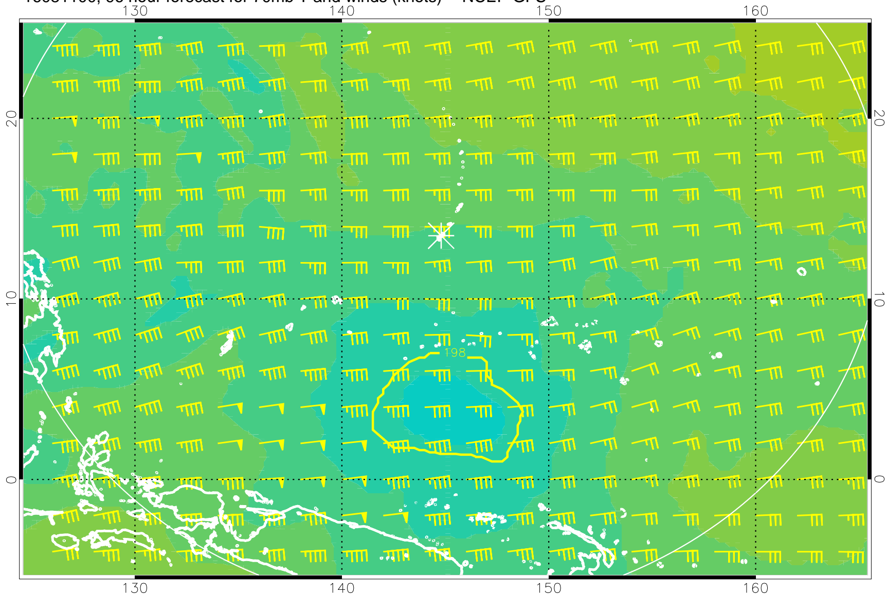
16081100, 96 hour forecast for 70mb T and winds (knots) -- NCEP GFS
