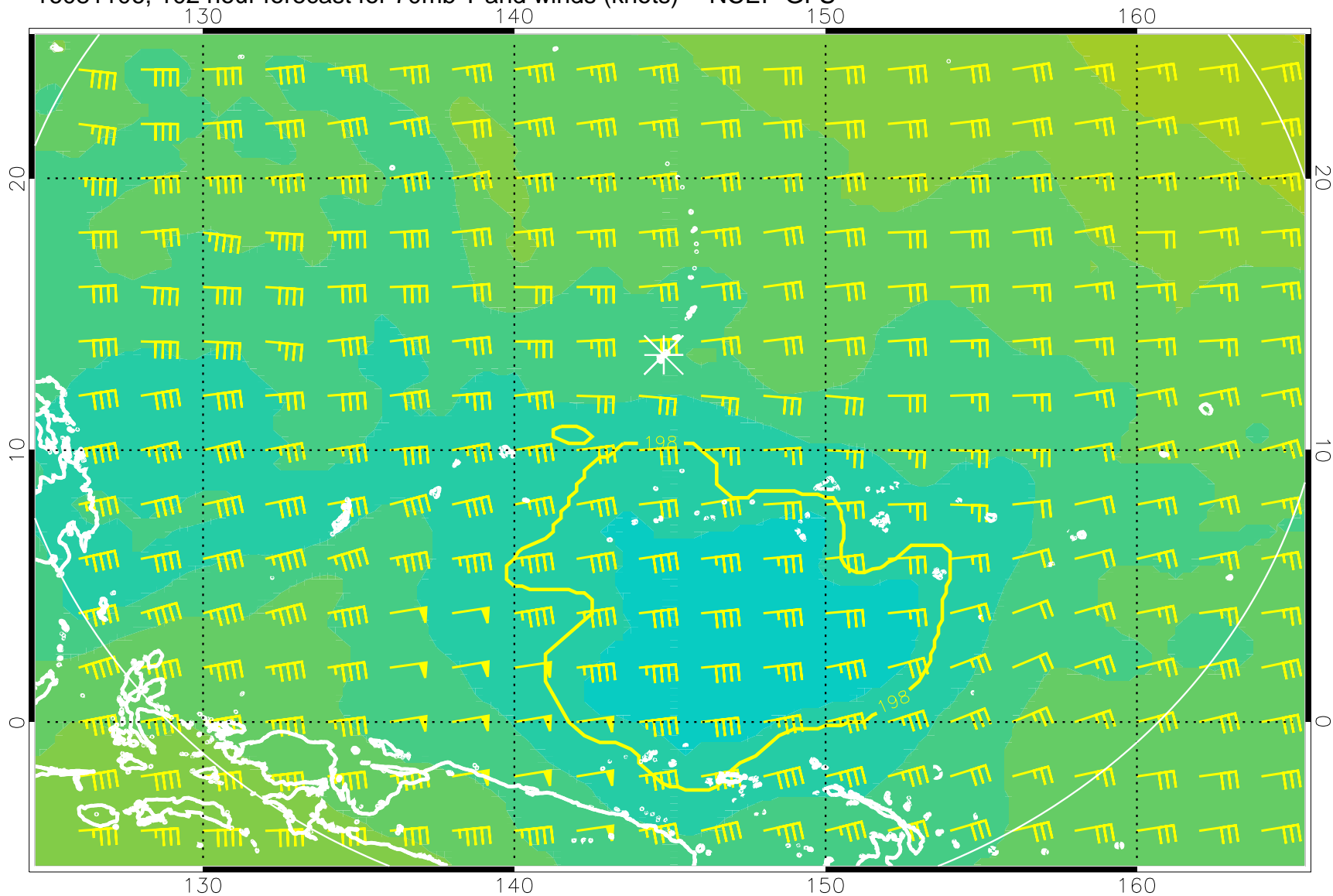
16081106, 102 hour forecast for 70mb T and winds (knots) -- NCEP GFS
