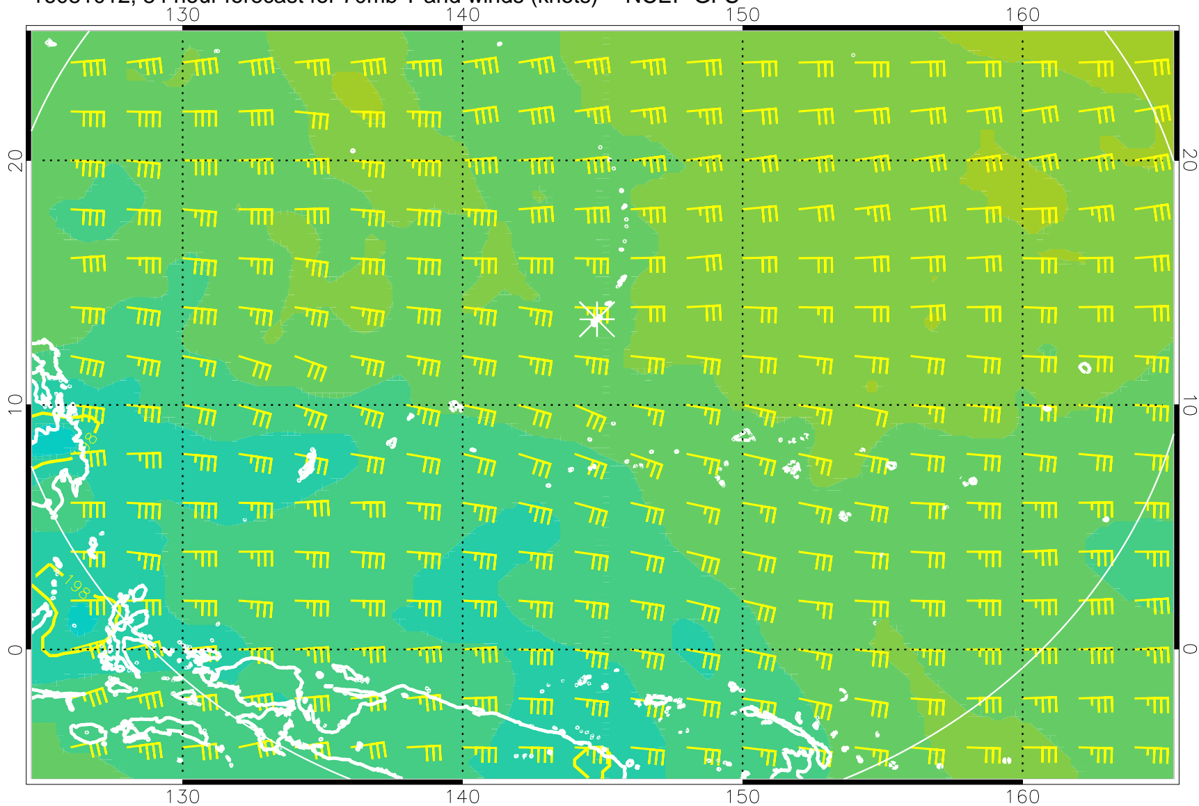
16081012, 84 hour forecast for 70mb T and winds (knots) -- NCEP GFS
