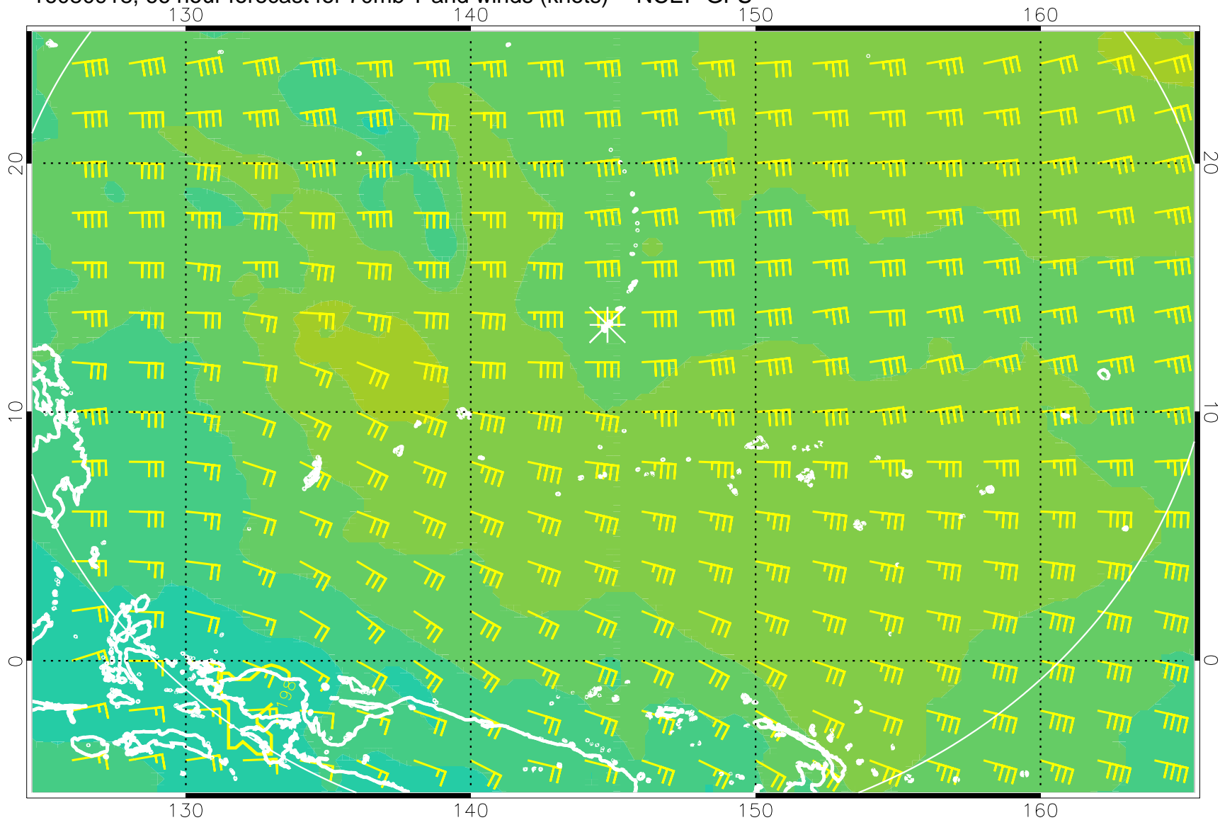
16080918, 66 hour forecast for 70mb T and winds (knots) -- NCEP GFS
