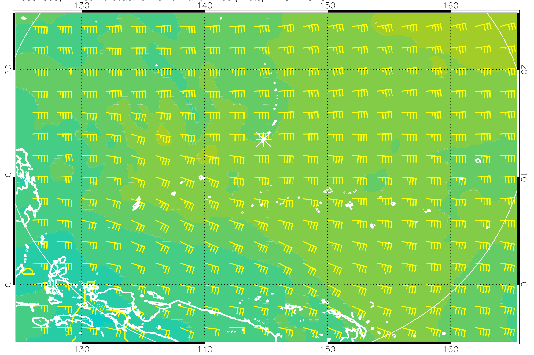
16081000, 72 hour forecast for 70mb T and winds (knots) -- NCEP GFS
