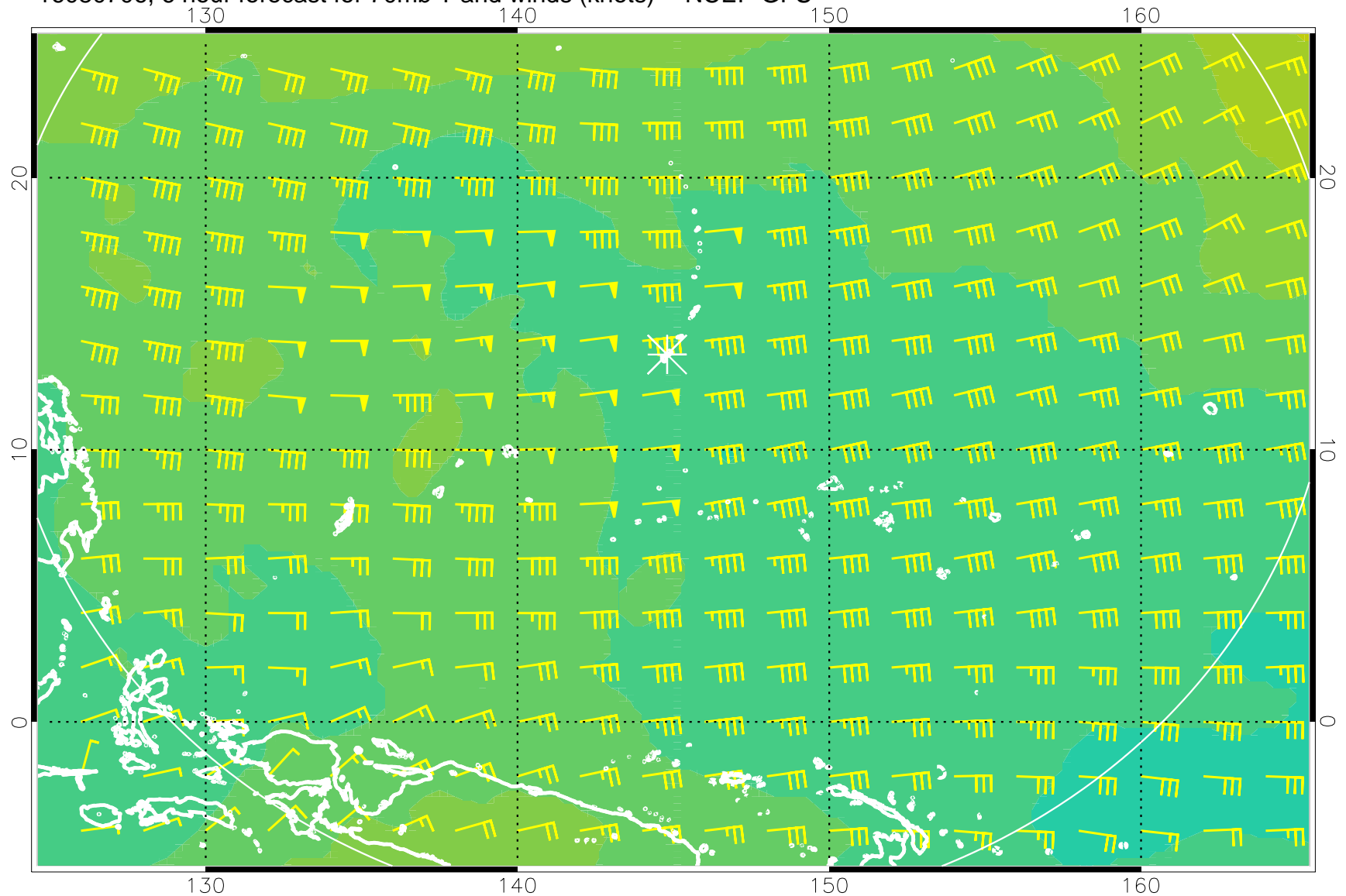
16080706, 6 hour forecast for 70mb T and winds (knots) -- NCEP GFS
