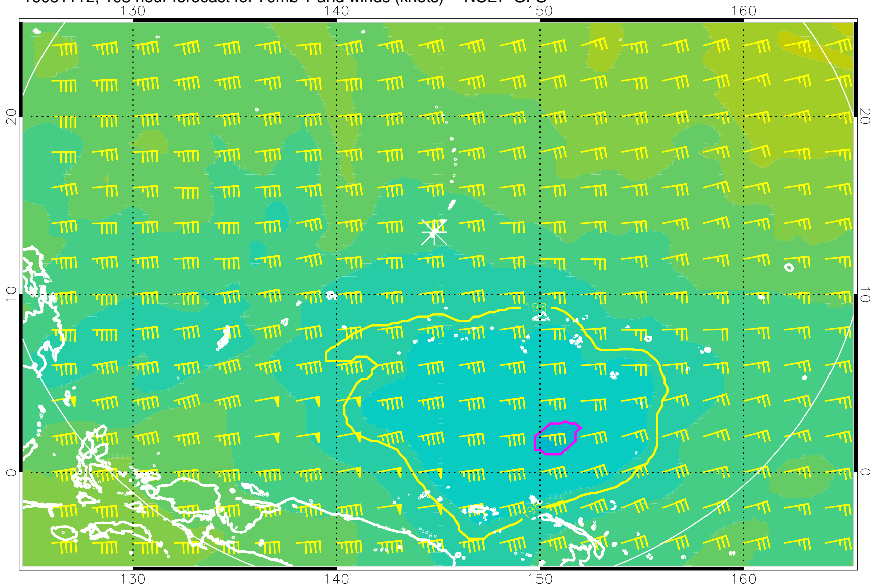
16081112, 108 hour forecast for 70mb T and winds (knots) -- NCEP GFS
