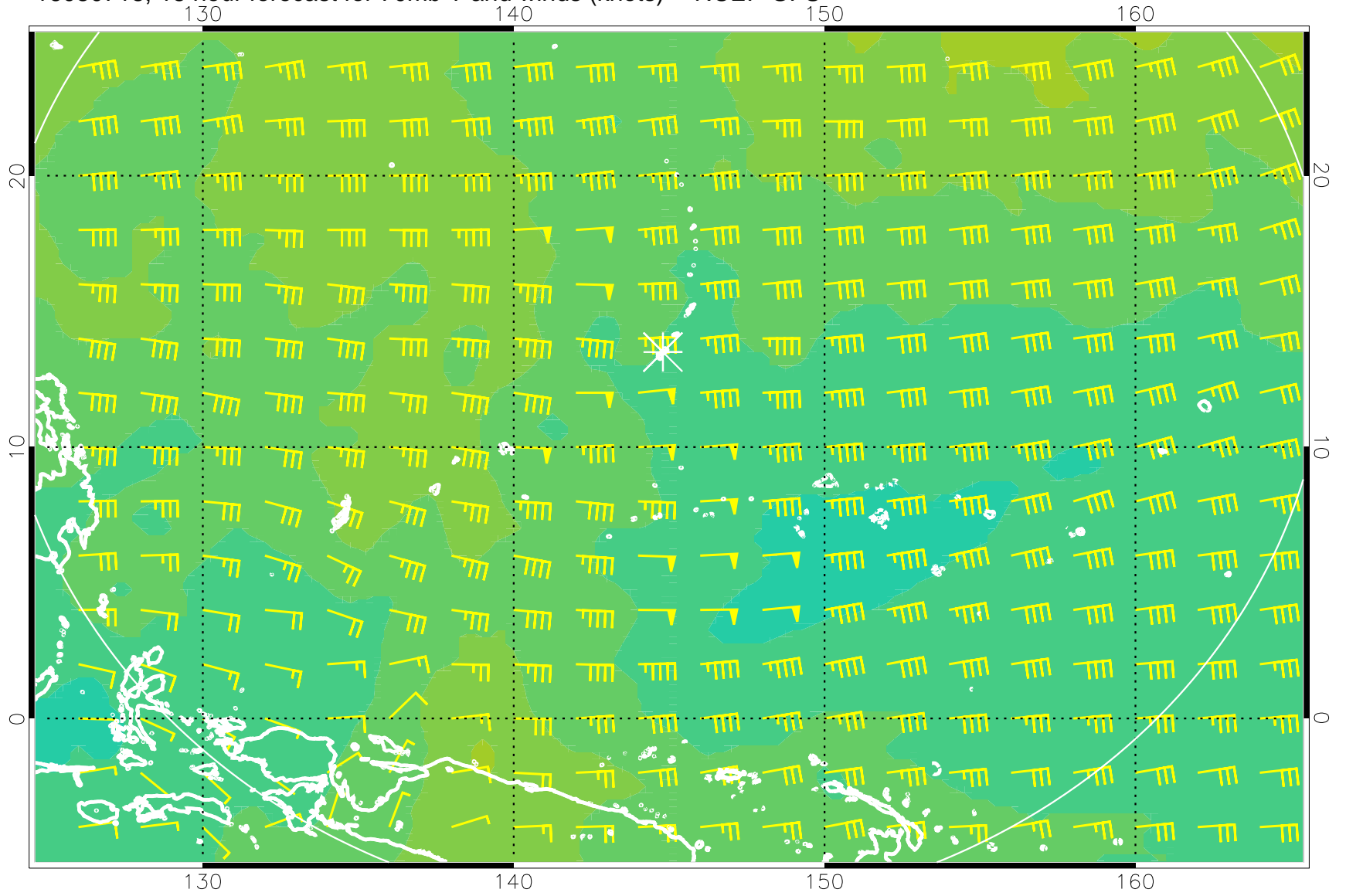
16080718, 18 hour forecast for 70mb T and winds (knots) -- NCEP GFS
