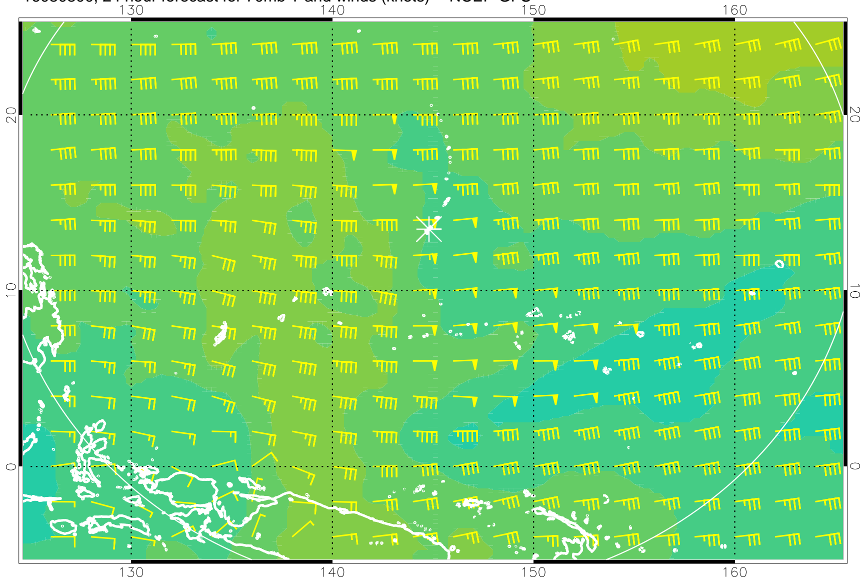
16080800, 24 hour forecast for 70mb T and winds (knots) -- NCEP GFS
