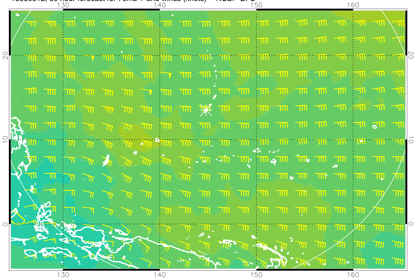
16080912, 60 hour forecast for 70mb T and winds (knots) -- NCEP GFS
