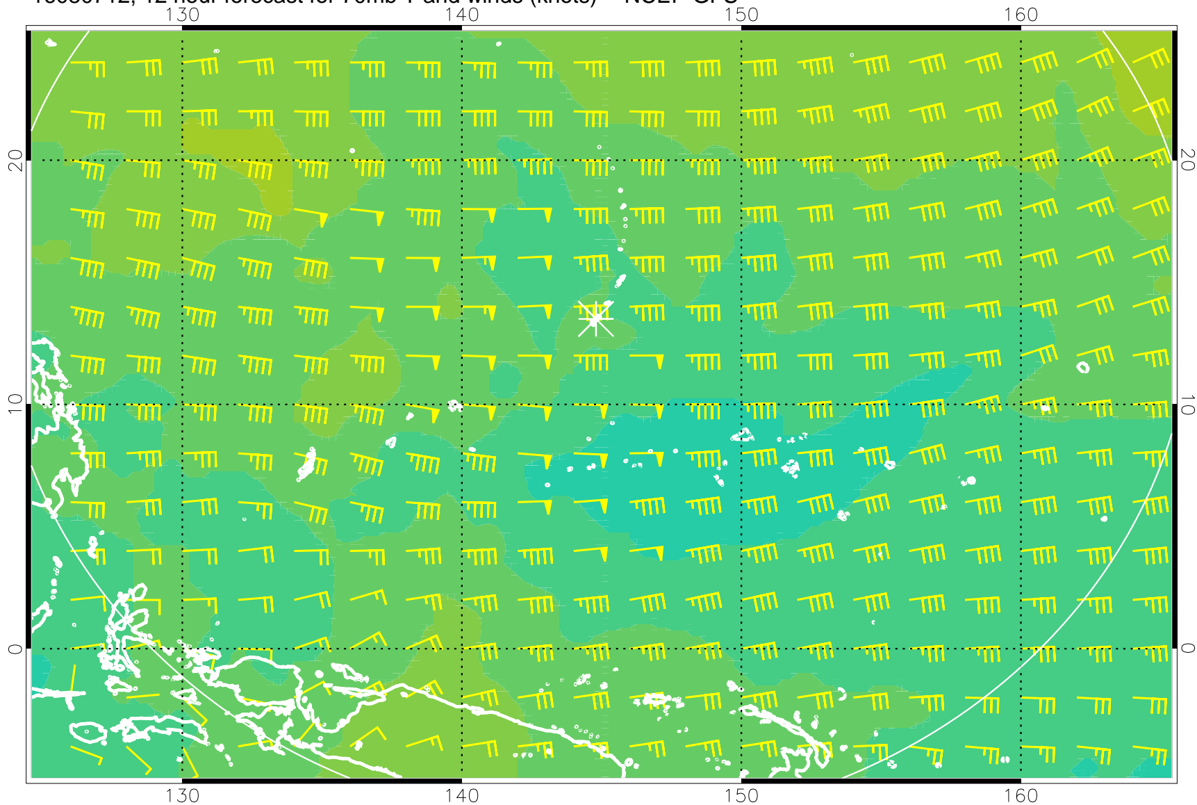
16080712, 12 hour forecast for 70mb T and winds (knots) -- NCEP GFS
