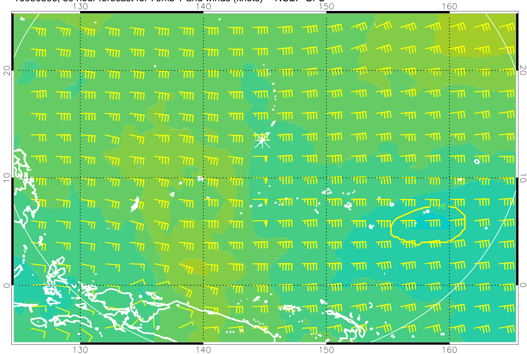
16080806, 30 hour forecast for 70mb T and winds (knots) -- NCEP GFS
