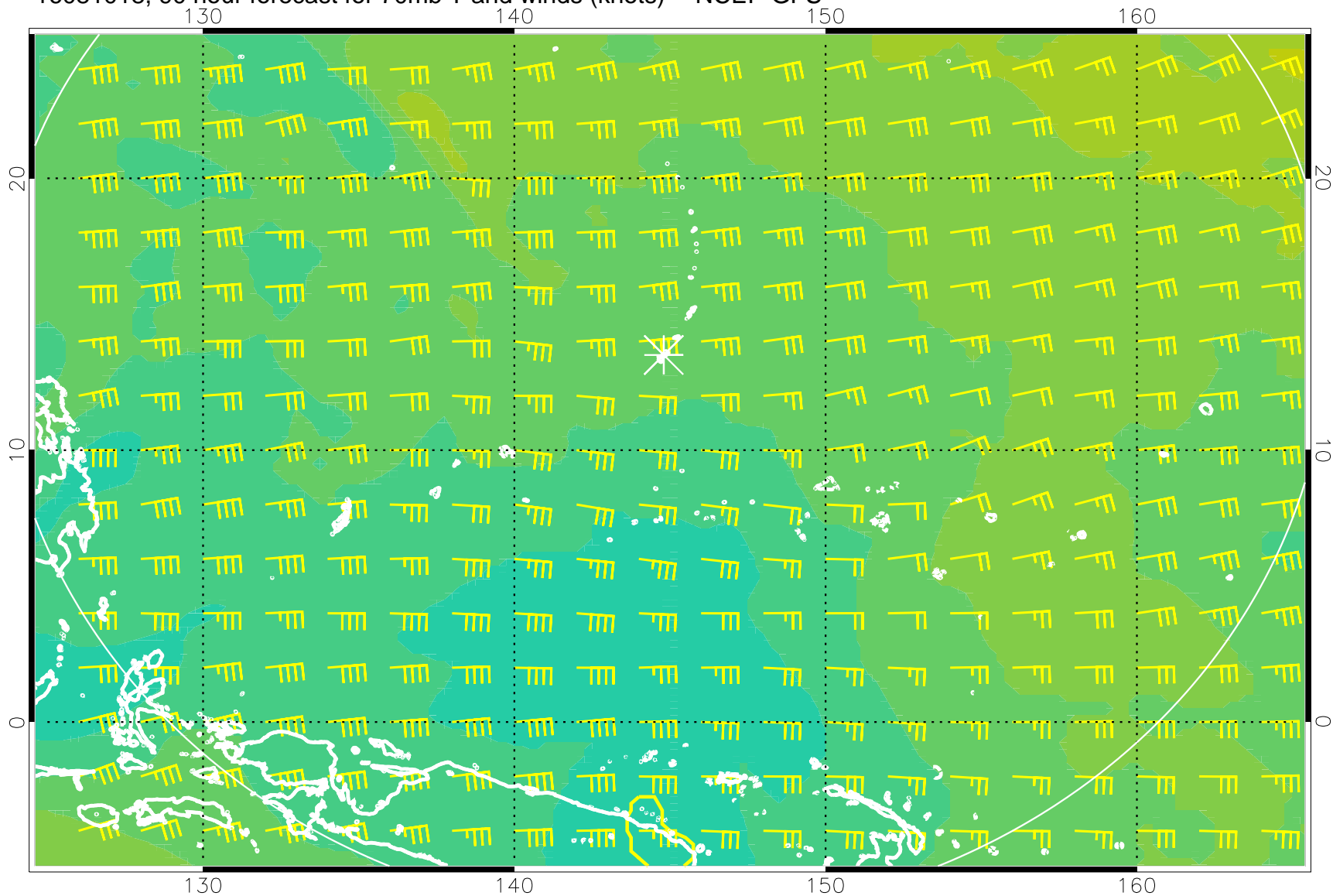
16081018, 90 hour forecast for 70mb T and winds (knots) -- NCEP GFS
