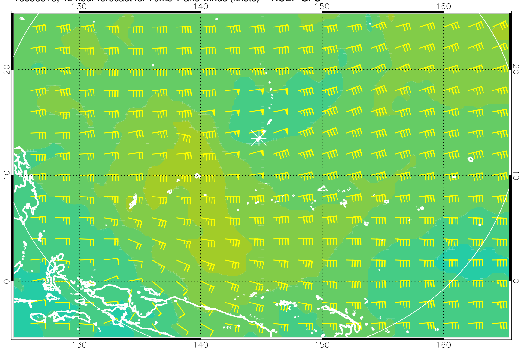
16080818, 42 hour forecast for 70mb T and winds (knots) -- NCEP GFS
