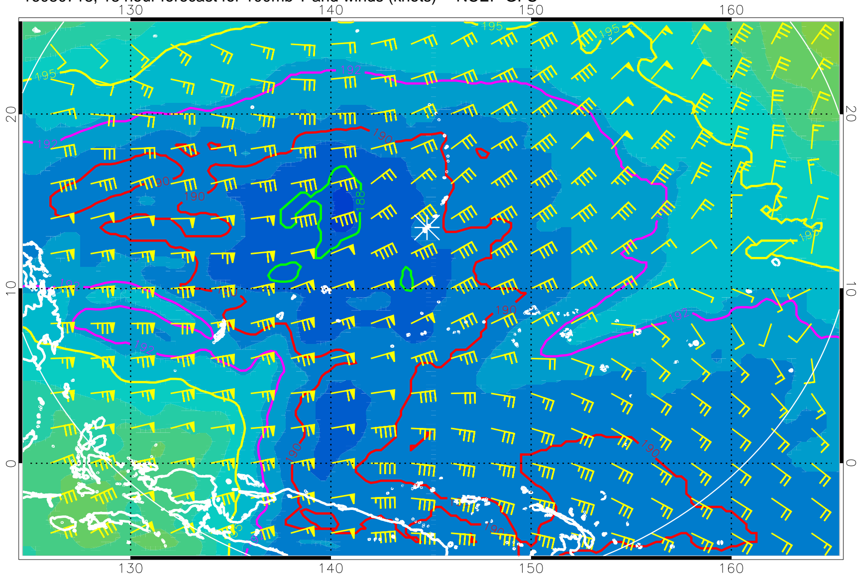
16080718, 18 hour forecast for 100mb T and winds (knots) -- NCEP GFS
