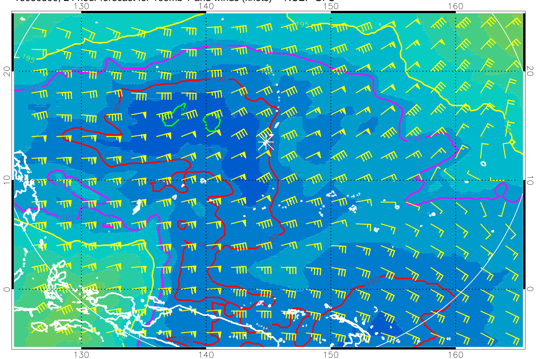
16080800, 24 hour forecast for 100mb T and winds (knots) -- NCEP GFS
