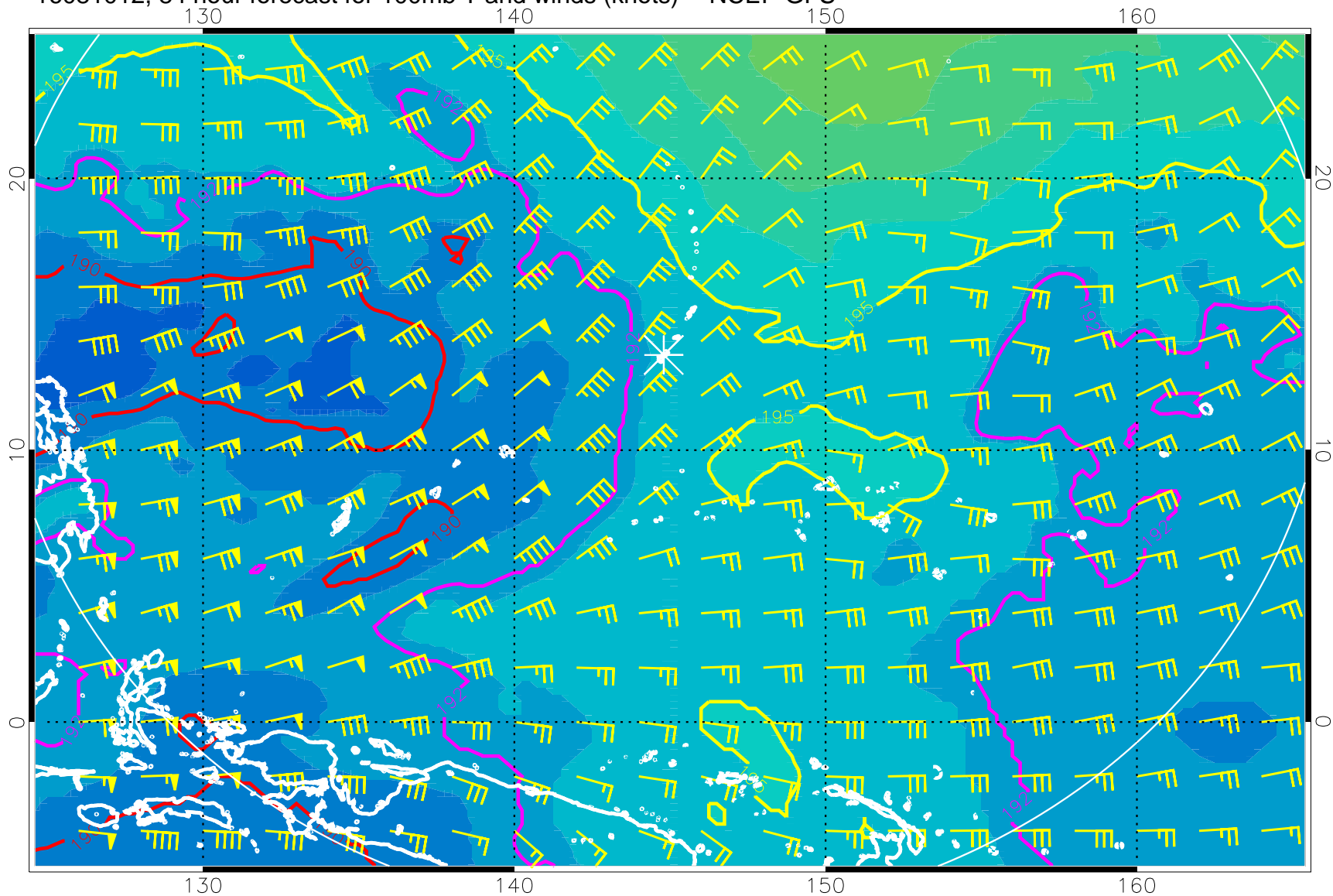
16081012, 84 hour forecast for 100mb T and winds (knots) -- NCEP GFS
