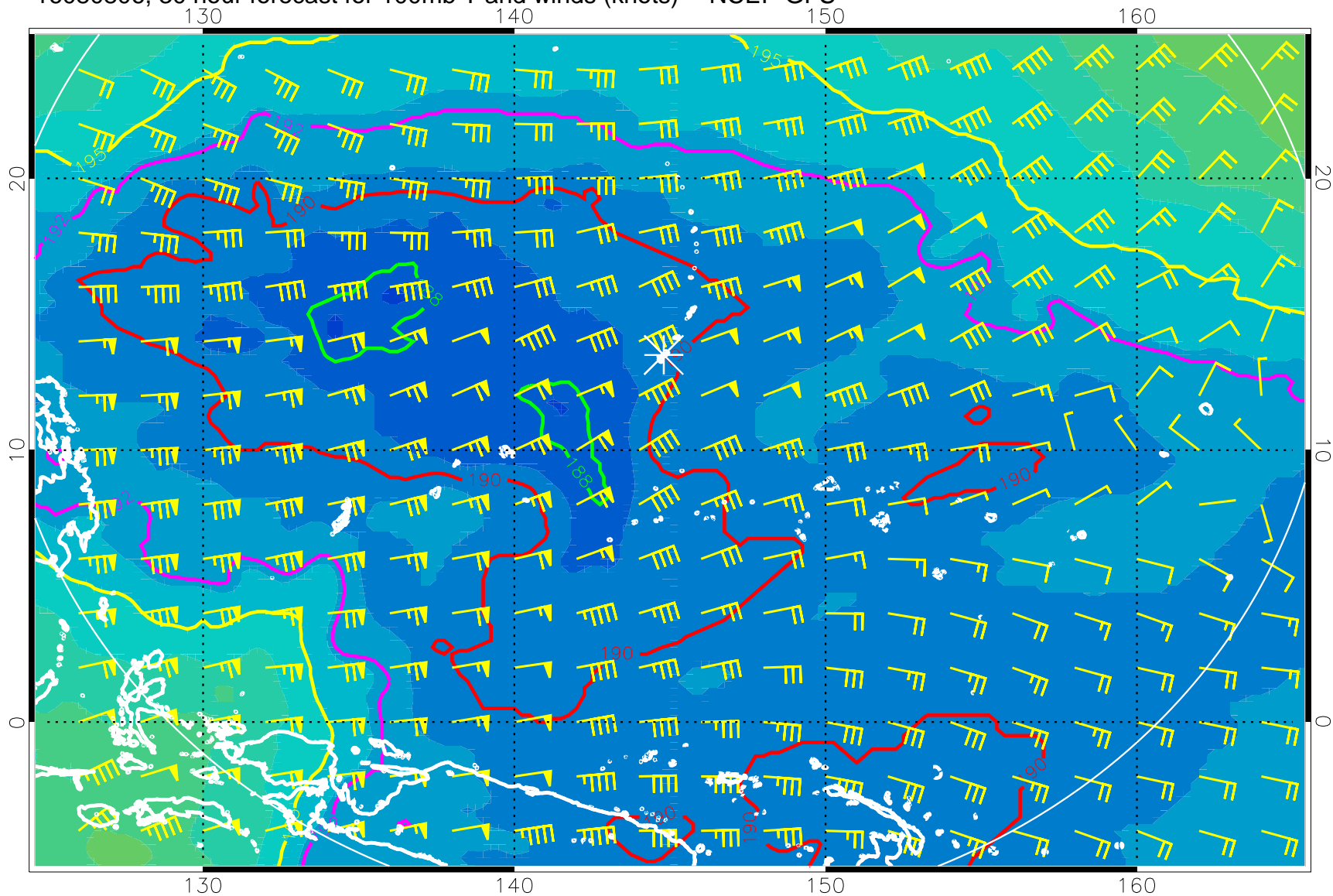
16080806, 30 hour forecast for 100mb T and winds (knots) -- NCEP GFS
