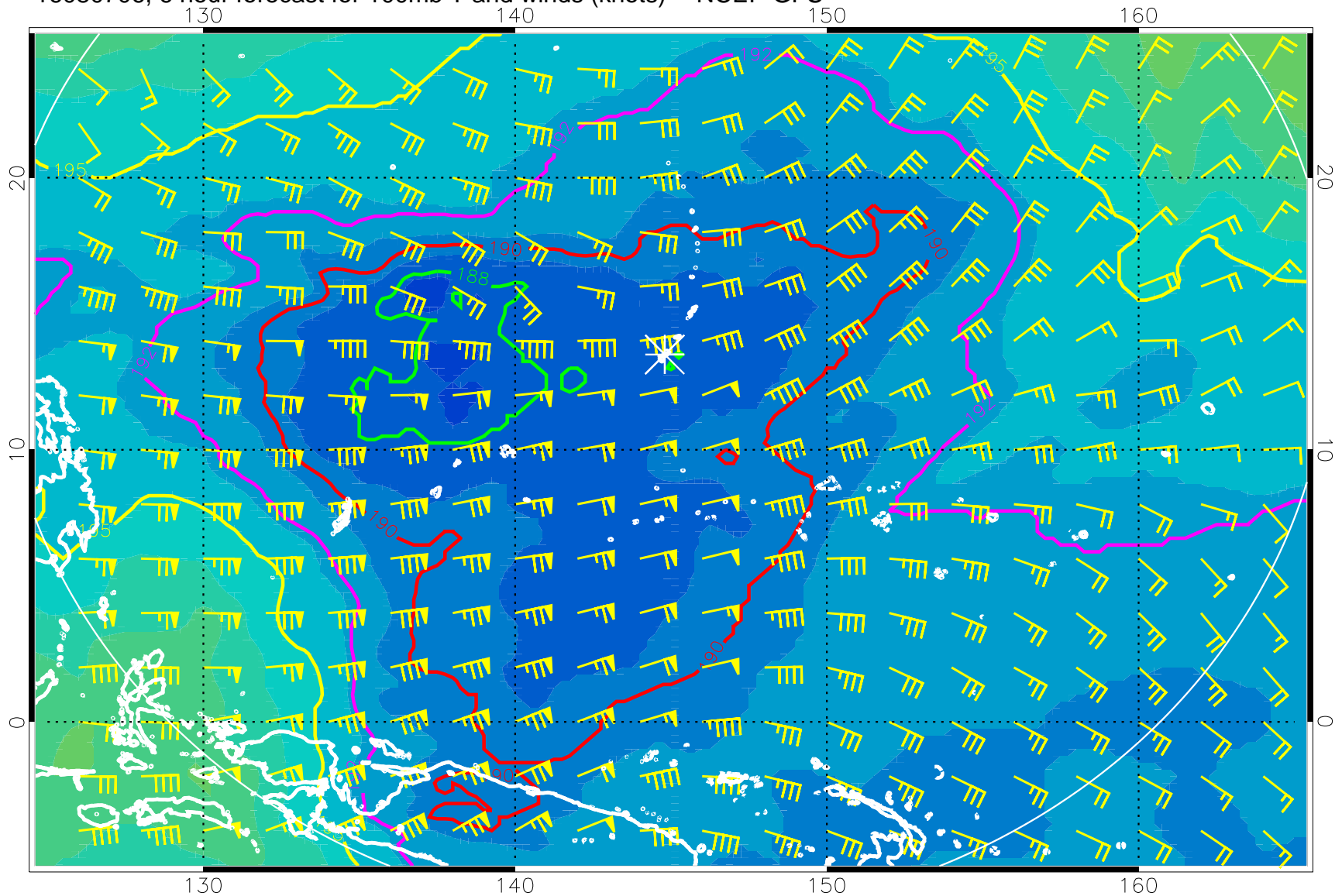
16080706, 6 hour forecast for 100mb T and winds (knots) -- NCEP GFS
