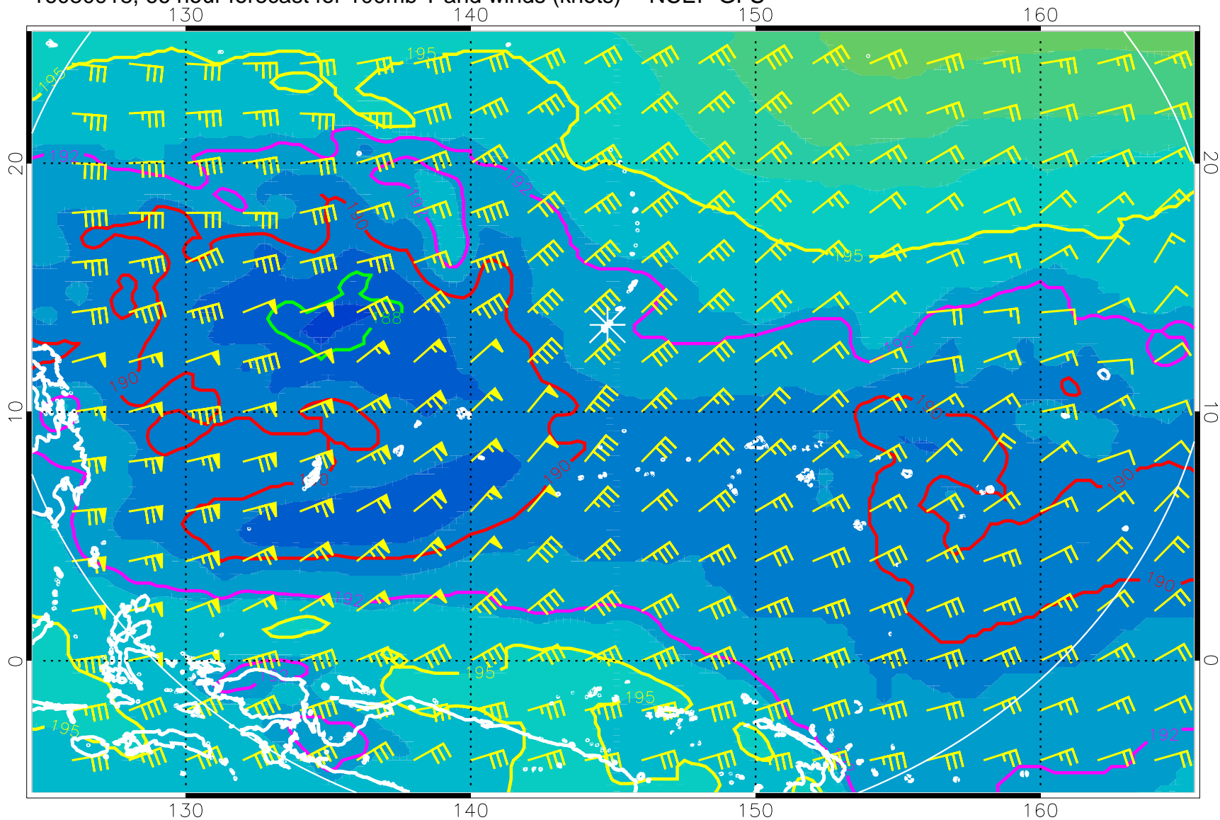
16080918, 66 hour forecast for 100mb T and winds (knots) -- NCEP GFS
