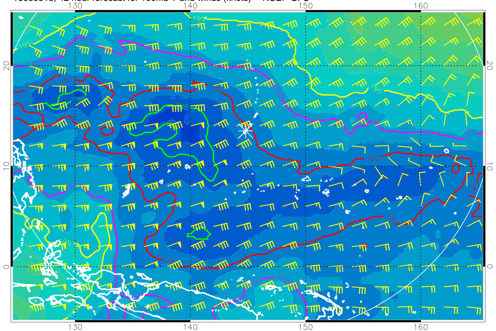
16080818, 42 hour forecast for 100mb T and winds (knots) -- NCEP GFS
