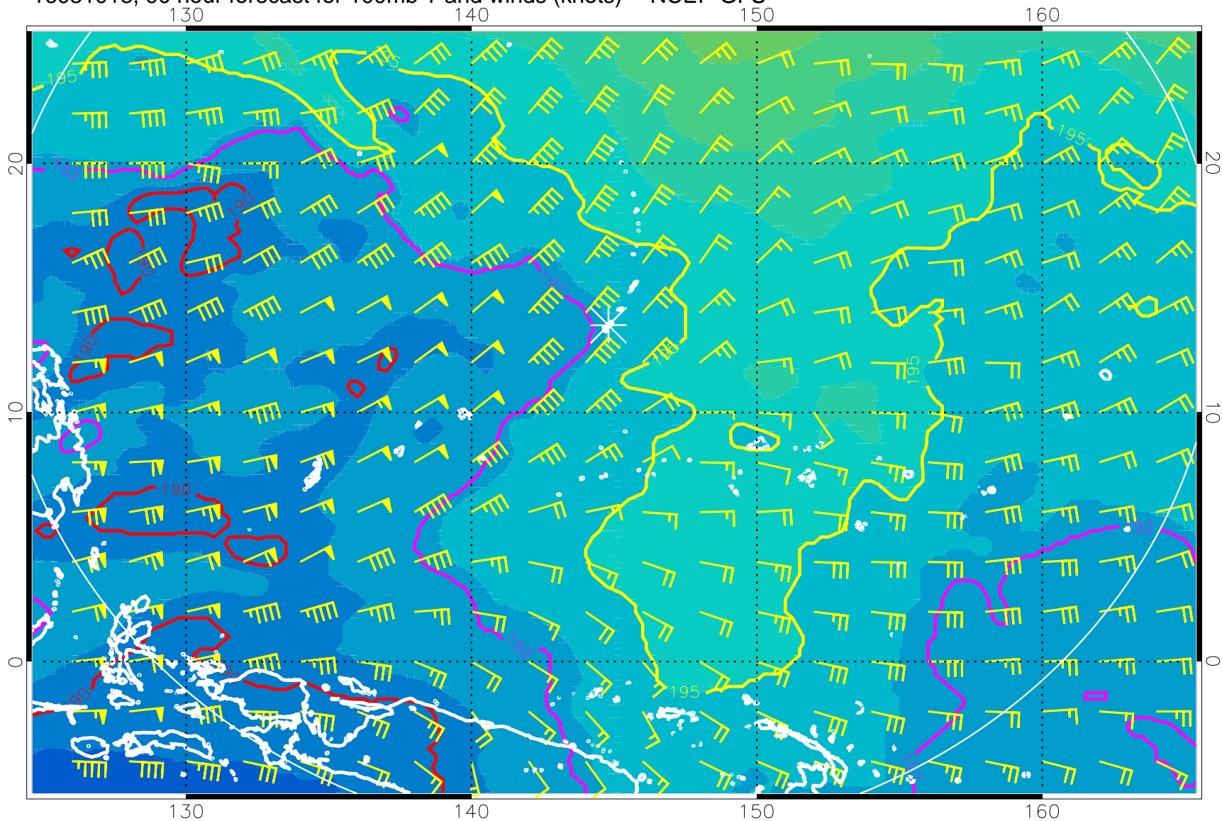
16081018, 90 hour forecast for 100mb T and winds (knots) -- NCEP GFS
