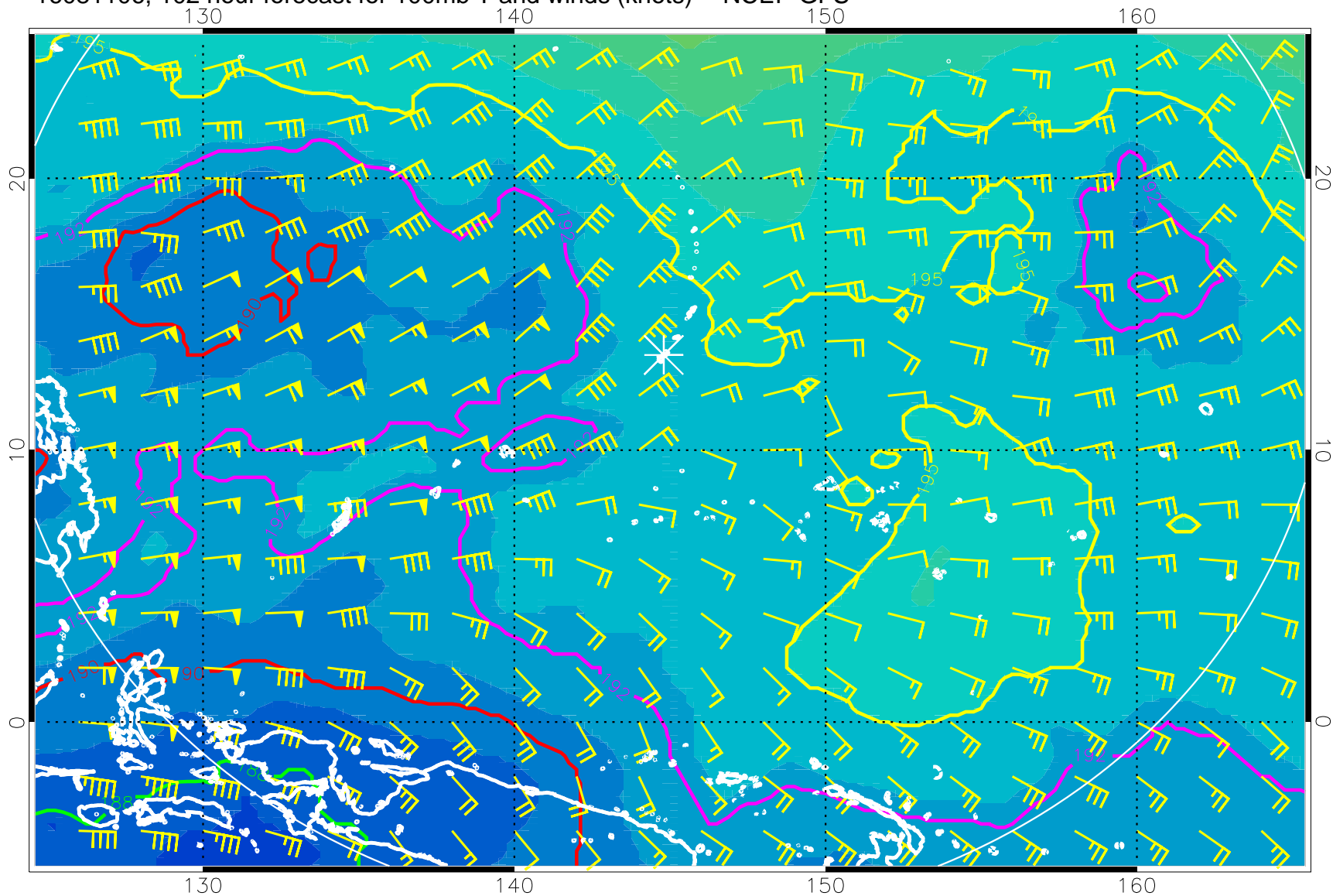
16081106, 102 hour forecast for 100mb T and winds (knots) -- NCEP GFS
