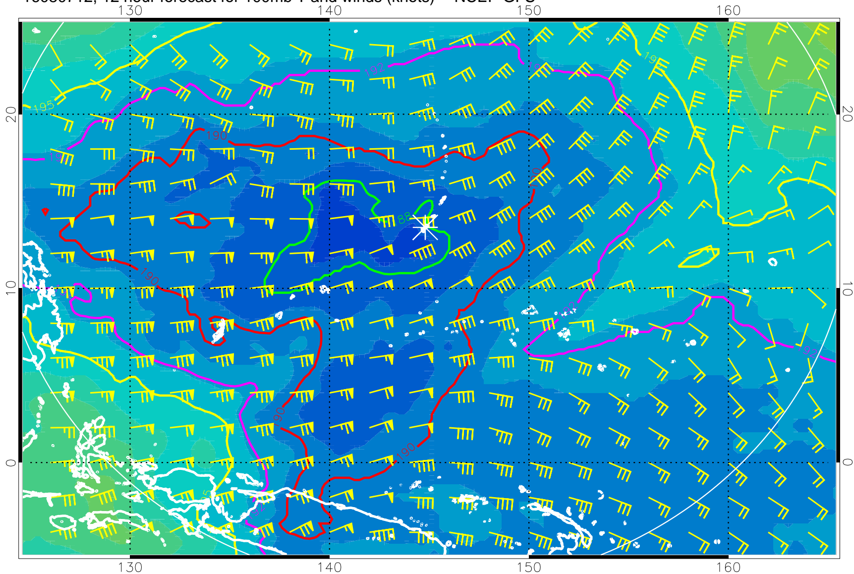
16080712, 12 hour forecast for 100mb T and winds (knots) -- NCEP GFS
