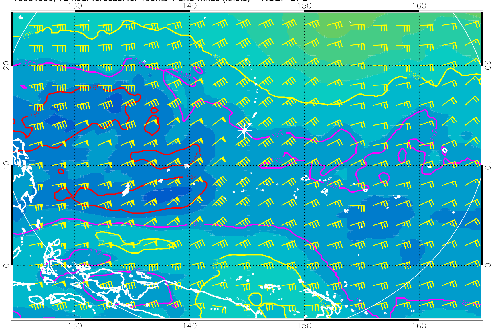
16081000, 72 hour forecast for 100mb T and winds (knots) -- NCEP GFS
