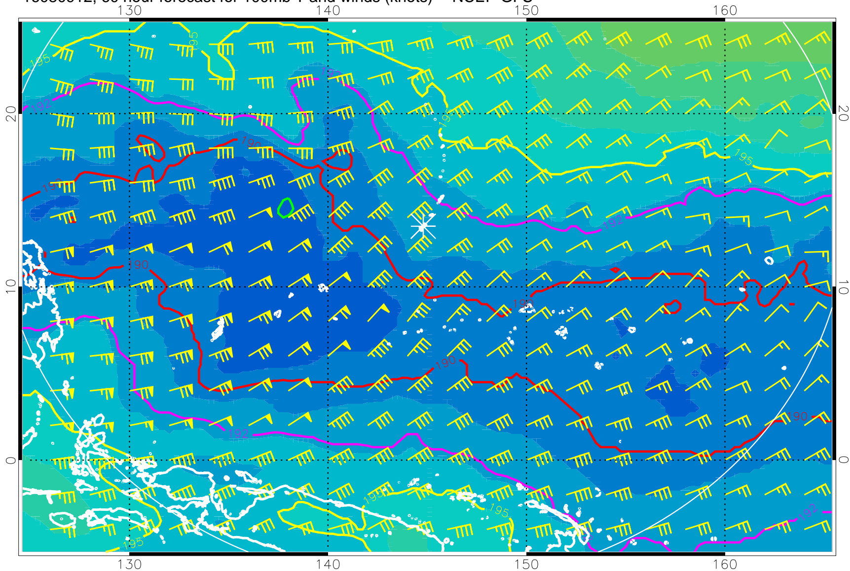
16080912, 60 hour forecast for 100mb T and winds (knots) -- NCEP GFS
