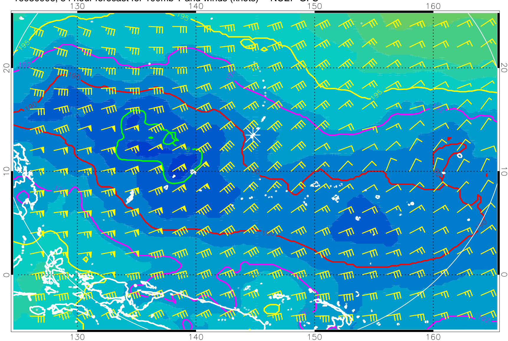
16080906, 54 hour forecast for 100mb T and winds (knots) -- NCEP GFS
