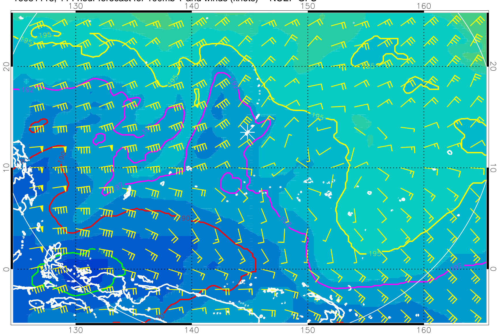
16081118, 114 hour forecast for 100mb T and winds (knots) -- NCEP GFS
