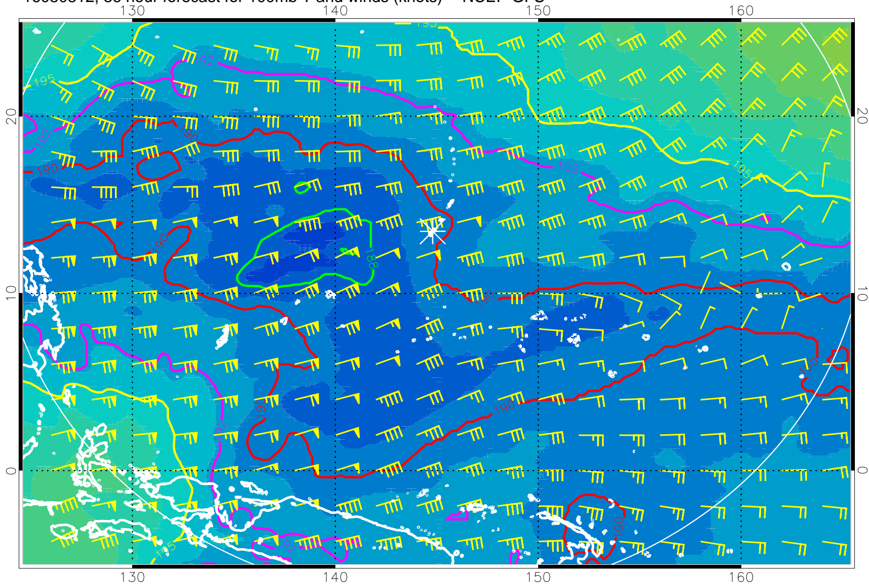
16080812, 36 hour forecast for 100mb T and winds (knots) -- NCEP GFS
