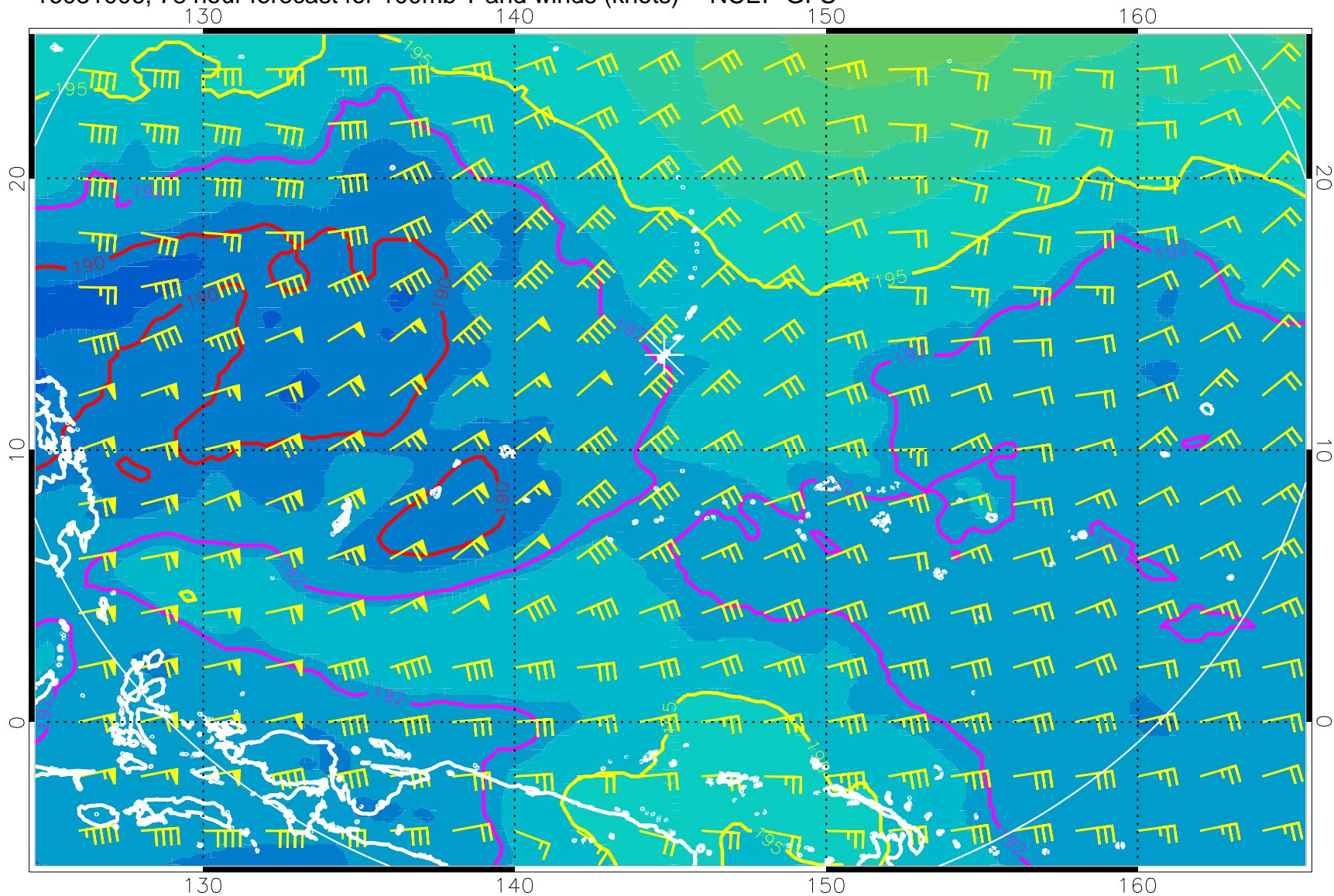
16081006, 78 hour forecast for 100mb T and winds (knots) -- NCEP GFS
