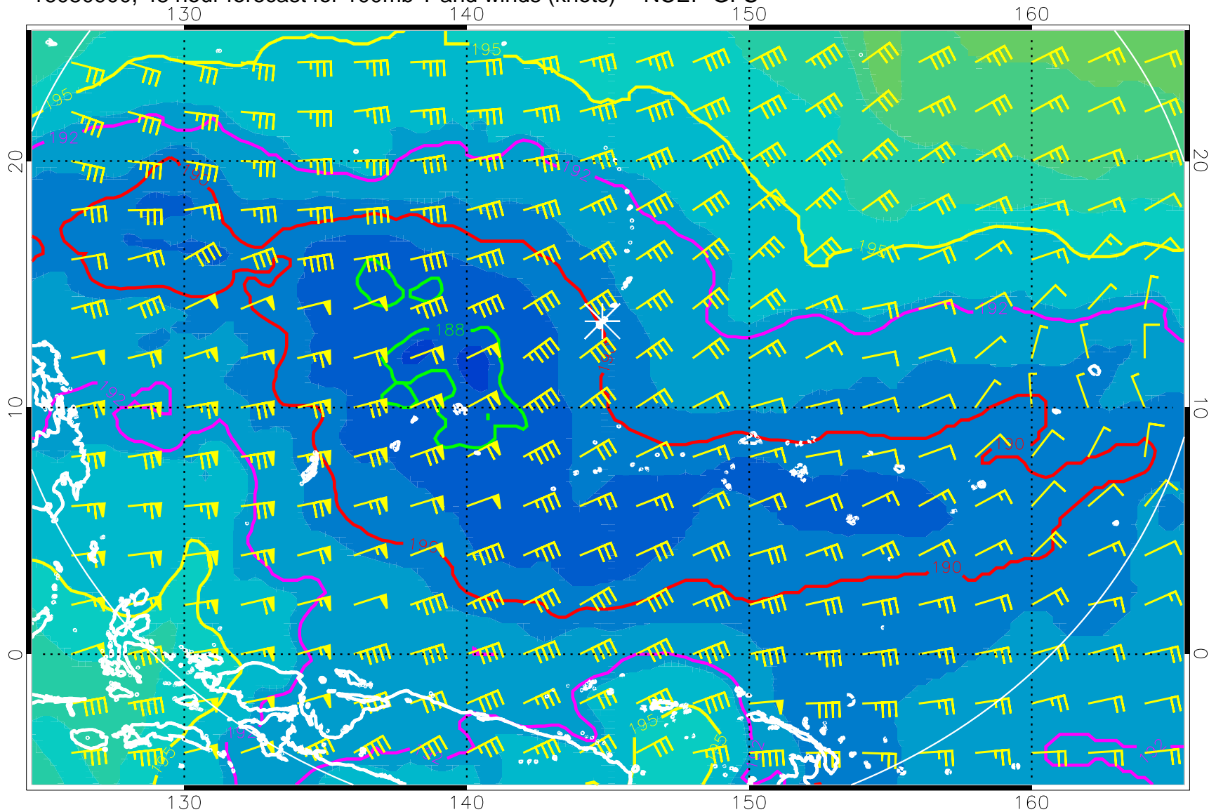
16080900, 48 hour forecast for 100mb T and winds (knots) -- NCEP GFS
