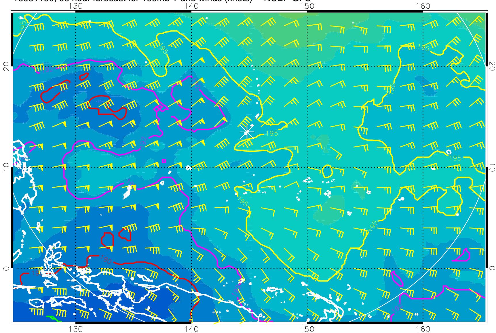
16081100, 96 hour forecast for 100mb T and winds (knots) -- NCEP GFS
