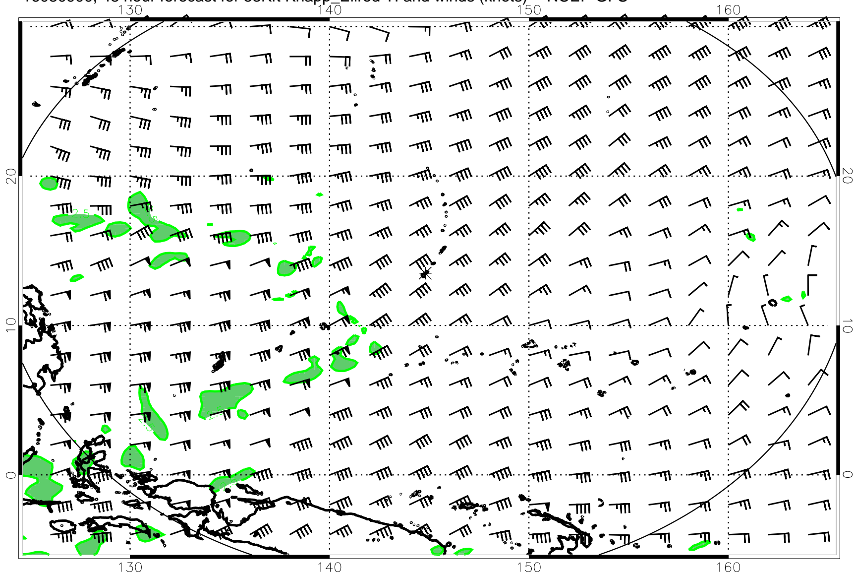
16080900, 48 hour forecast for 53Kft Knapp_Ellrod TI and winds (knots) -- NCEP GFS
