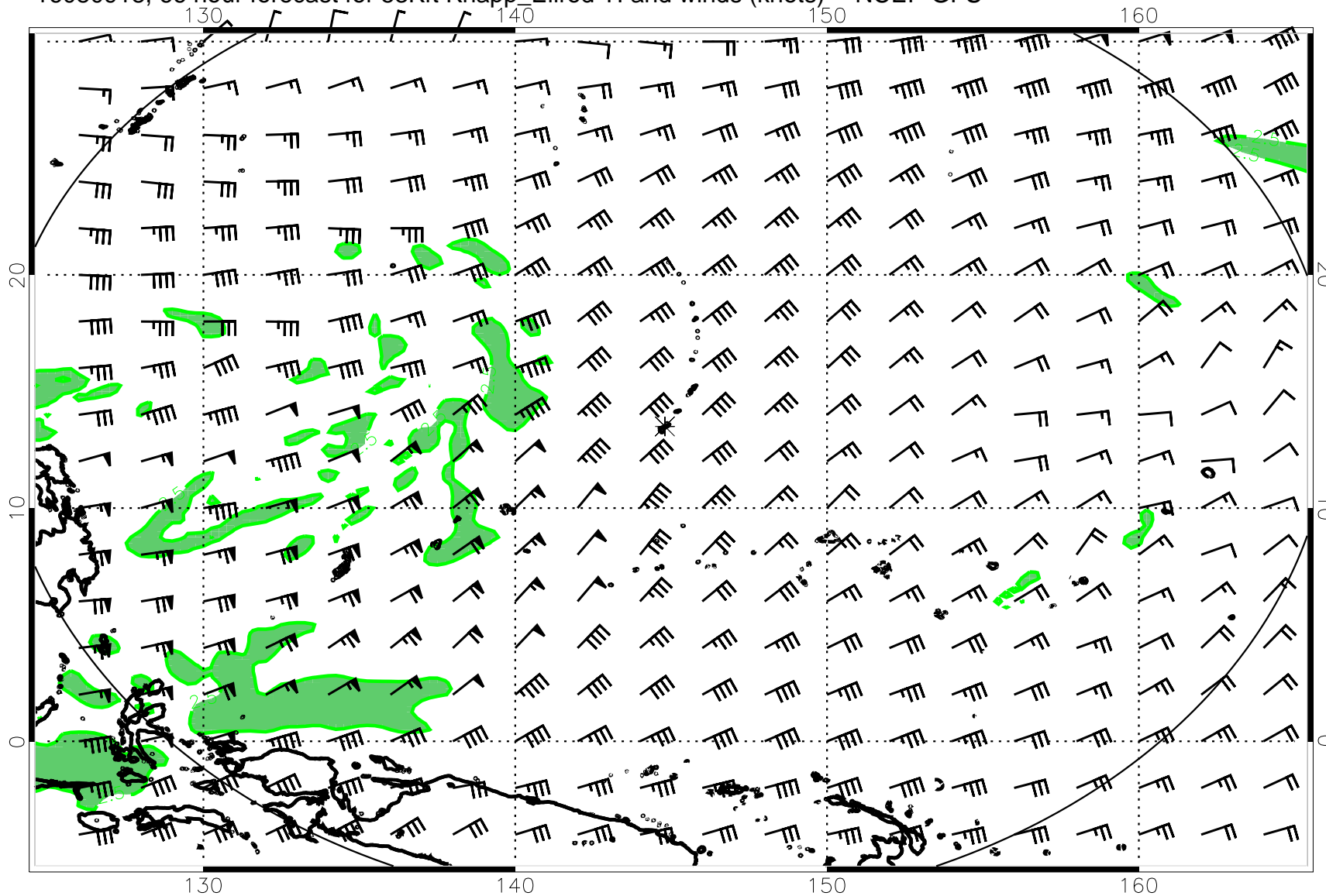
16080918, 66 hour forecast for 53Kft Knapp_Ellrod TI and winds (knots) -- NCEP GFS
