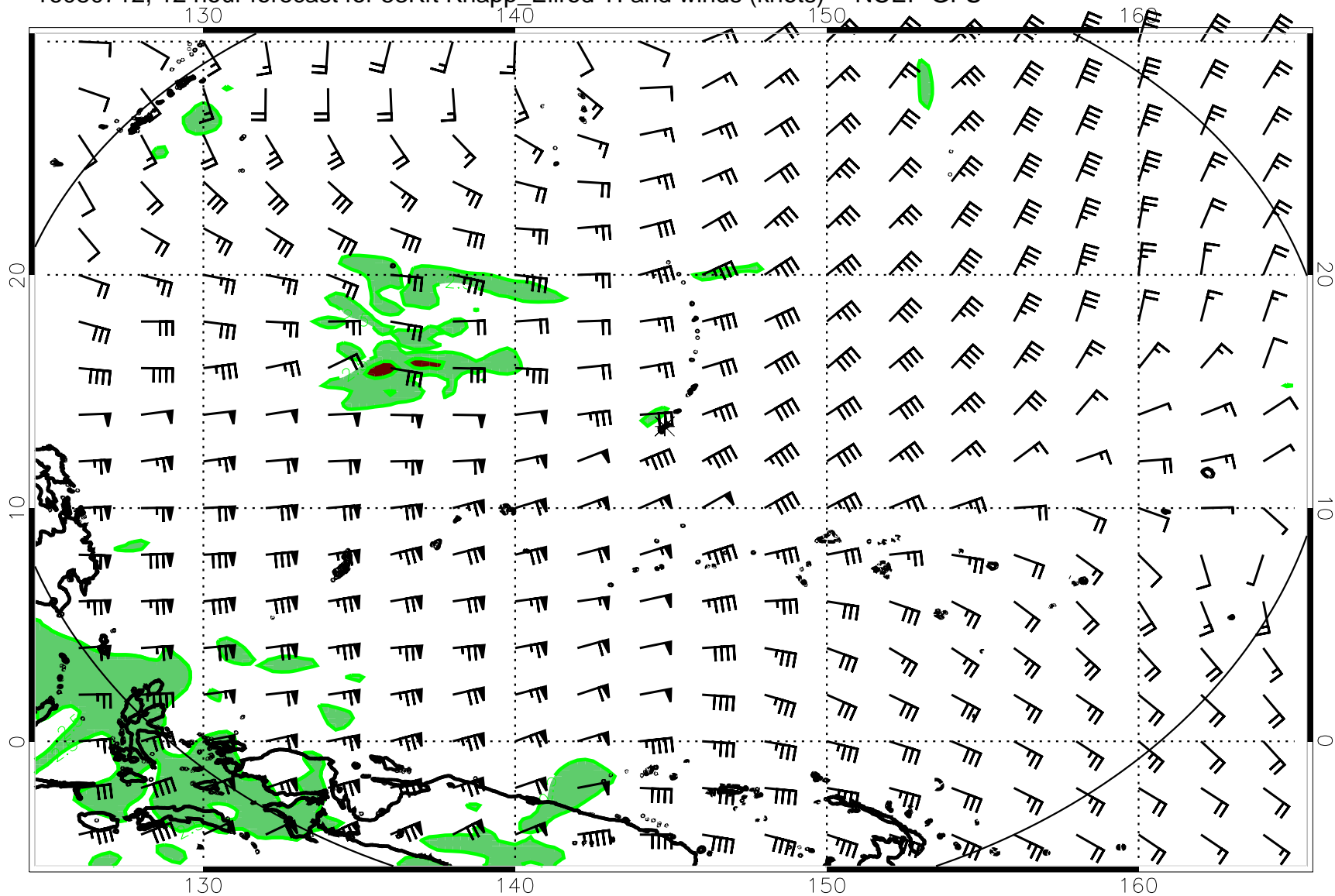
16080712, 12 hour forecast for 53Kft Knapp_Ellrod TI and winds (knots) -- NCEP GFS
