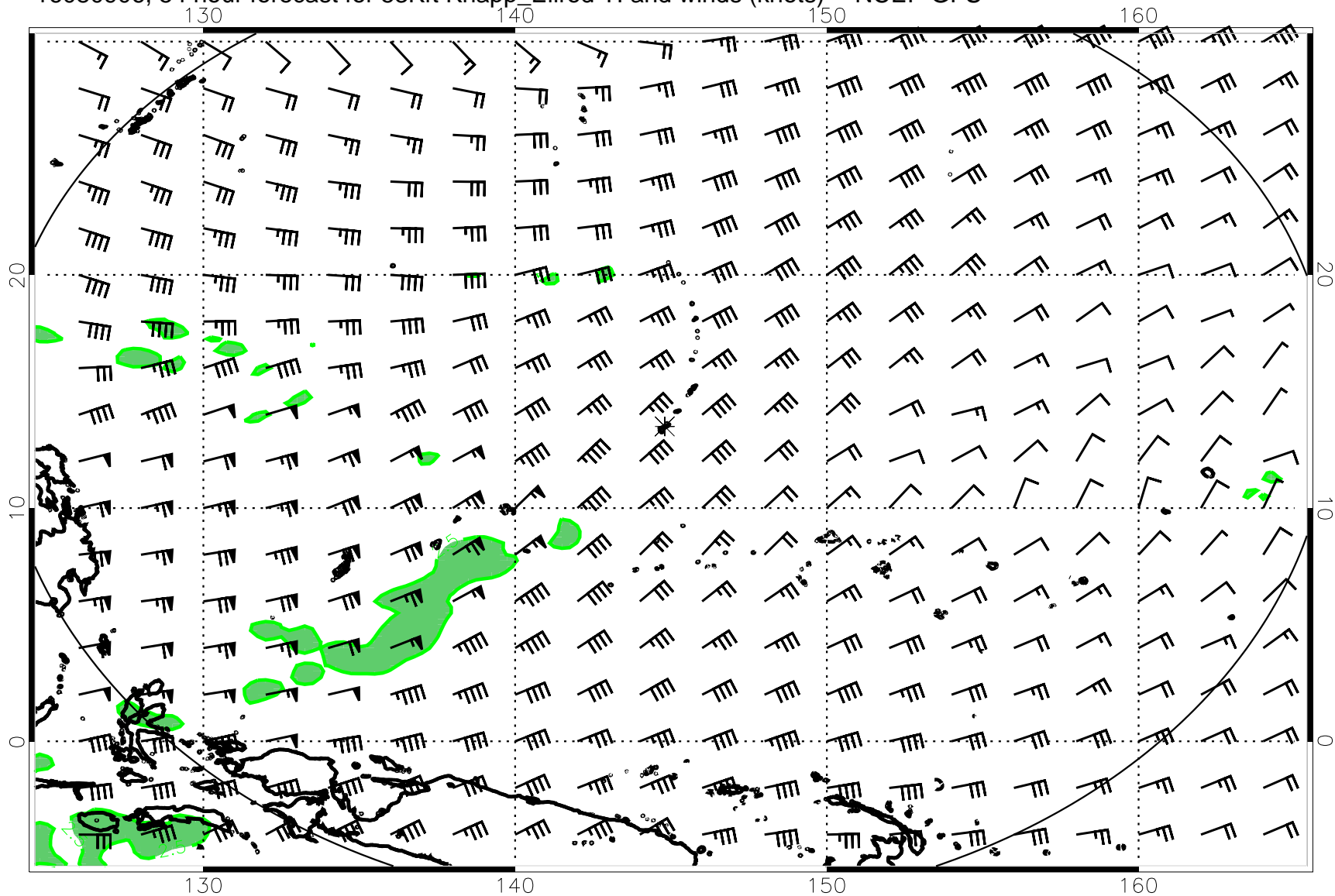
16080906, 54 hour forecast for 53Kft Knapp_Ellrod TI and winds (knots) -- NCEP GFS
