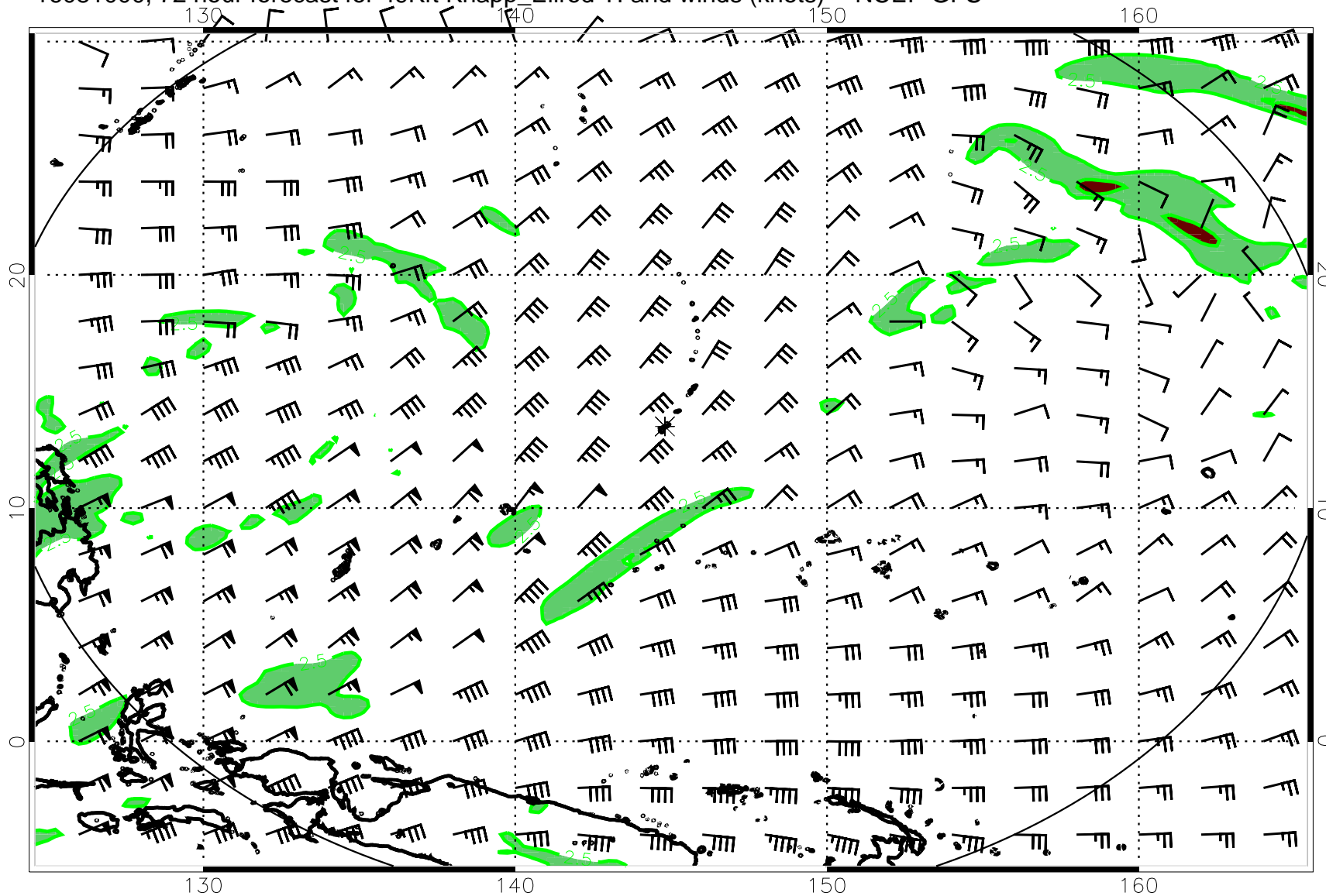
16081000, 72 hour forecast for 49Kft Knapp_Ellrod TI and winds (knots) -- NCEP GFS
