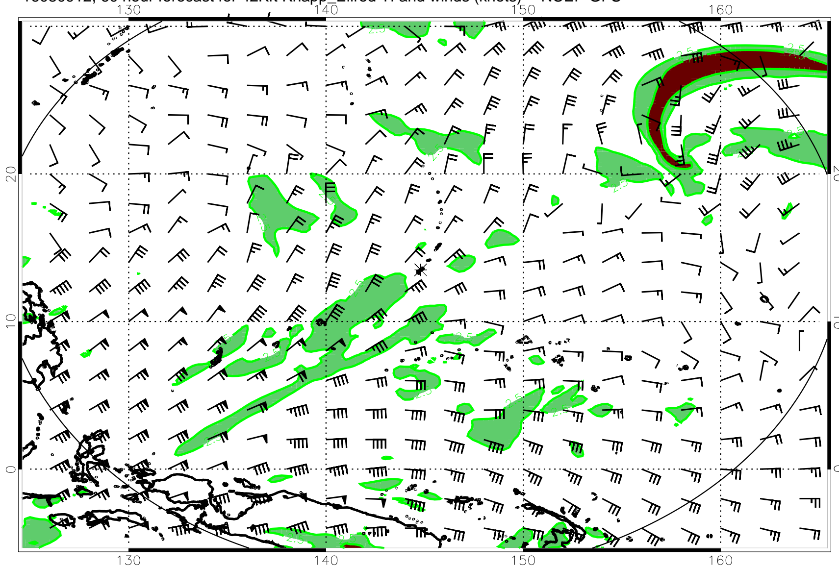
16080912, 60 hour forecast for 42Kft Knapp_Ellrod TI and winds (knots) -- NCEP GFS
