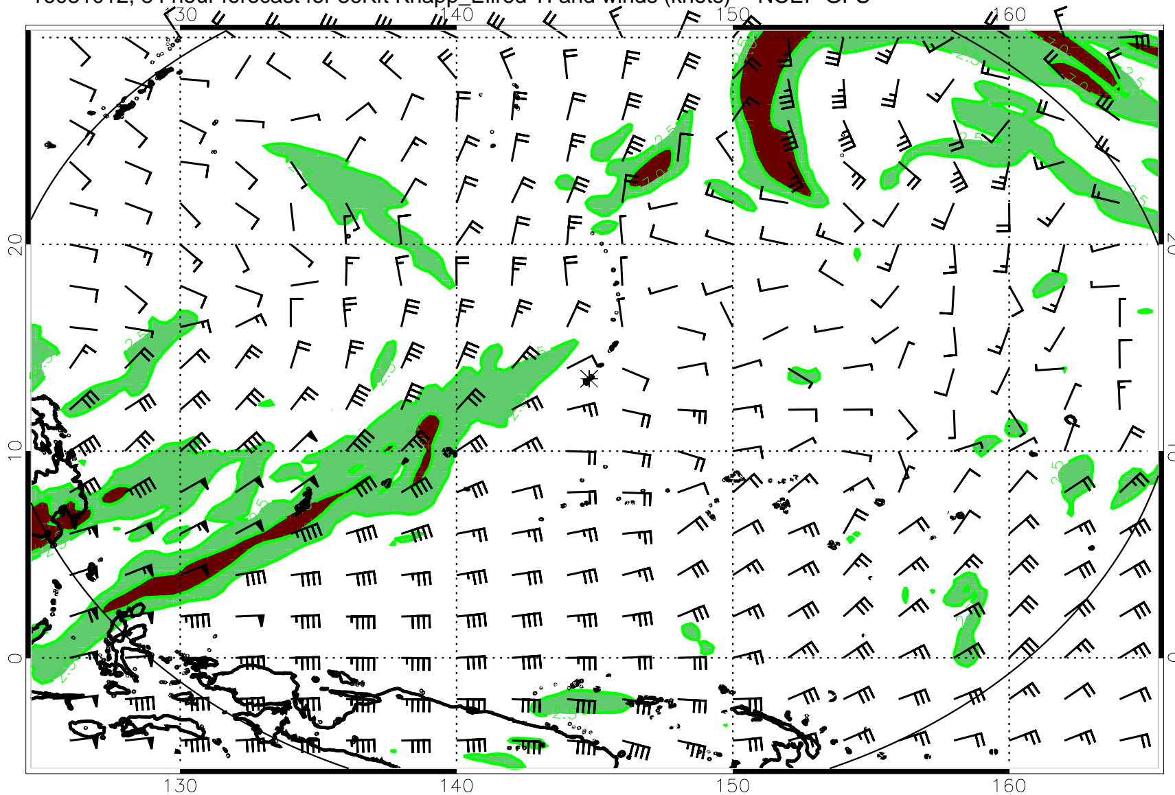
16081012, 84 hour forecast for 36Kft Knapp_Ellrod TI and winds (knots) -- NCEP GFS
