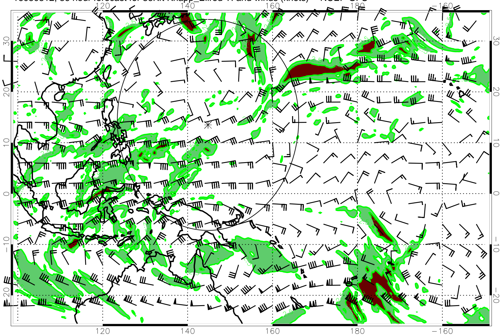
16080812, 36 hour forecast for 36Kft Knapp_Ellrod TI and winds (knots) -- NCEP GFS
