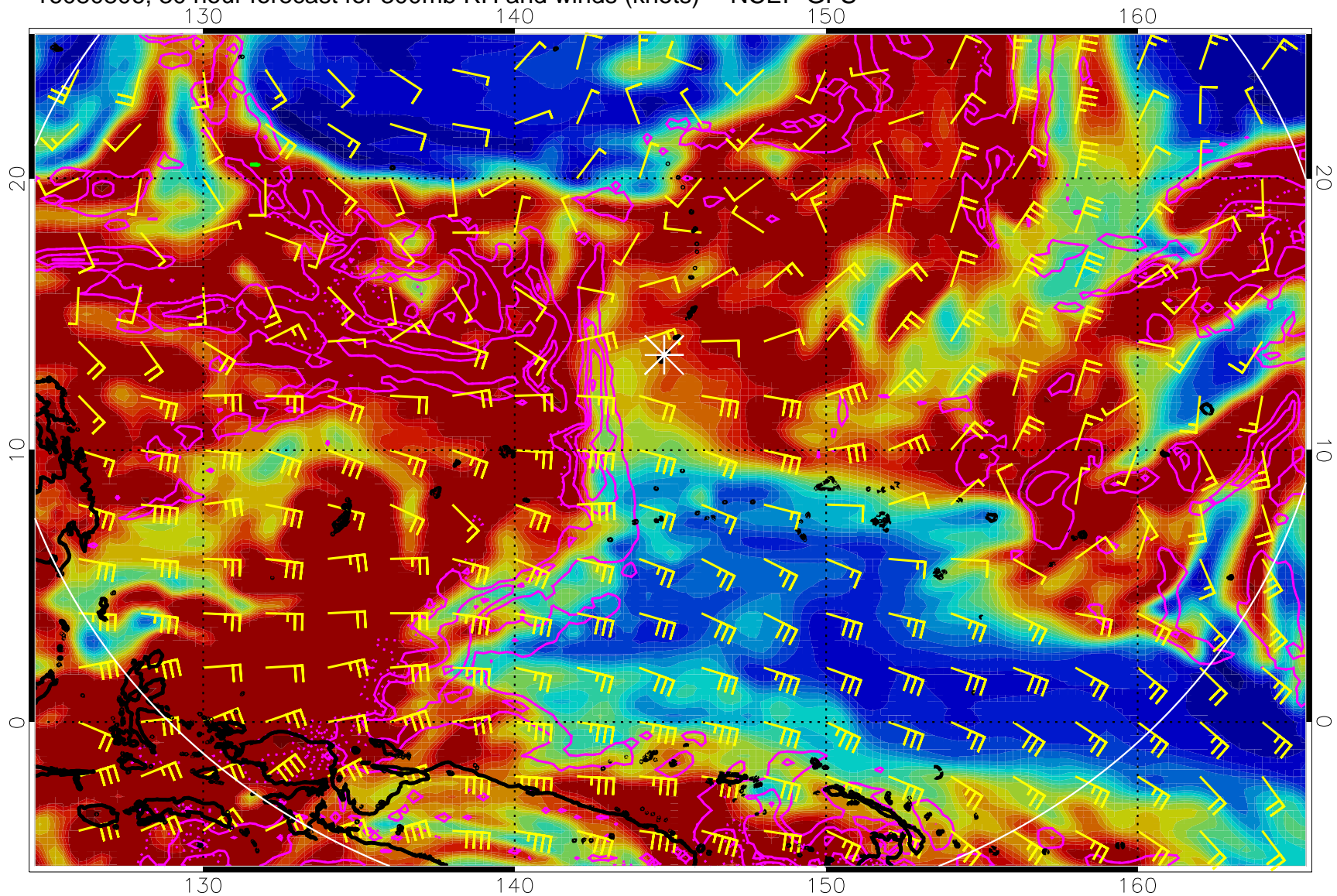
16080806, 30 hour forecast for 300mb RH and winds (knots) -- NCEP GFS
