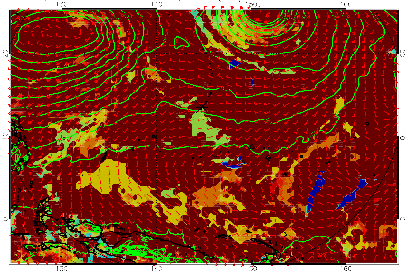
16081200, 120 hour forecast for HCAL, 1000mb Z, and winds (knots) -- NCEP GFS
