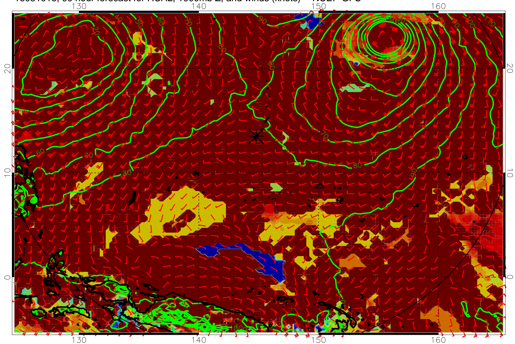
16081018, 90 hour forecast for HCAL, 1000mb Z, and winds (knots) -- NCEP GFS
