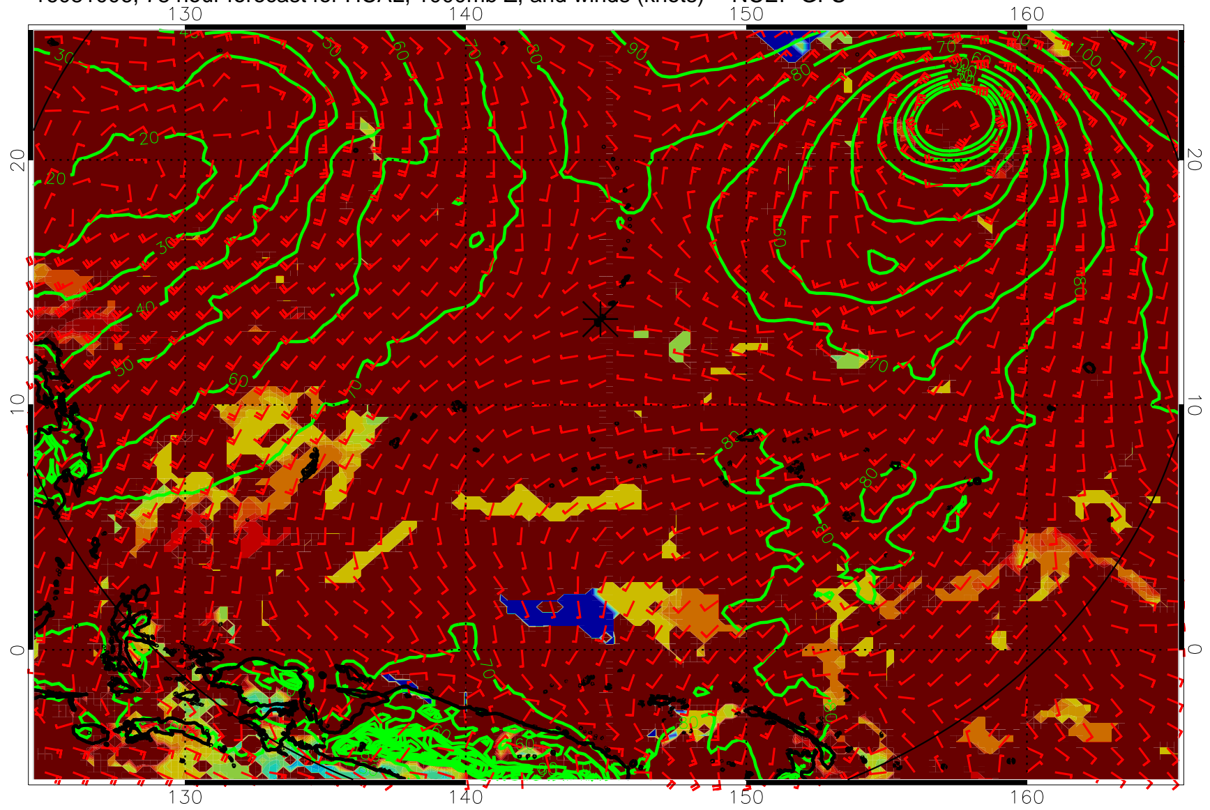
16081006, 78 hour forecast for HCAL, 1000mb Z, and winds (knots) -- NCEP GFS
