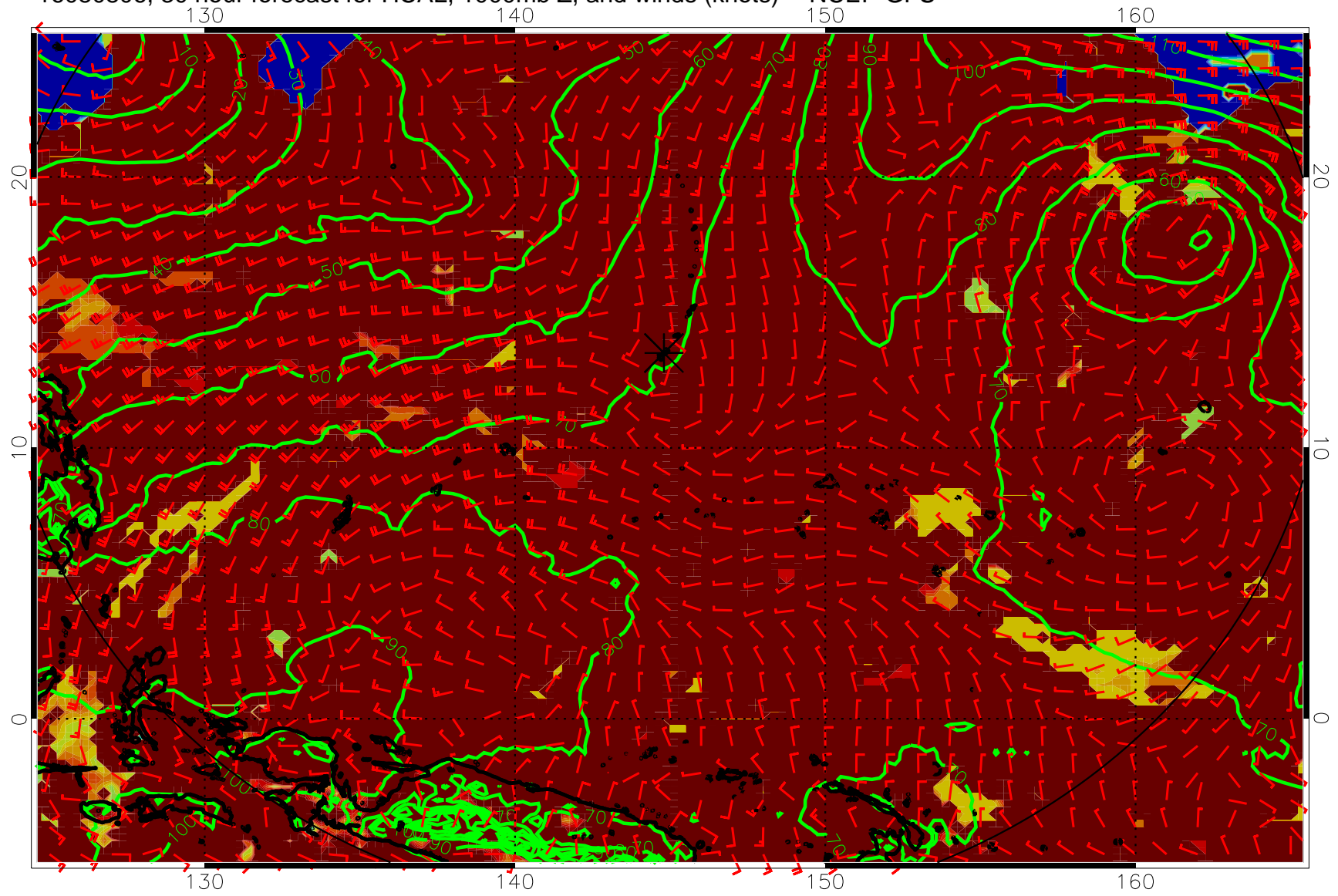
16080806, 30 hour forecast for HCAL, 1000mb Z, and winds (knots) -- NCEP GFS
