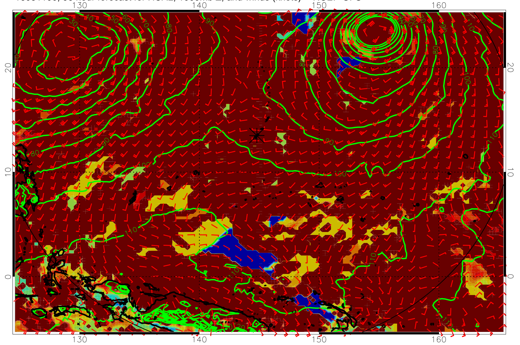
16081100, 96 hour forecast for HCAL, 1000mb Z, and winds (knots) -- NCEP GFS
