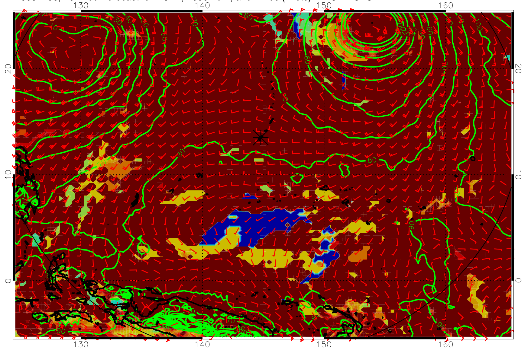
16081106, 102 hour forecast for HCAL, 1000mb Z, and winds (knots) -- NCEP GFS
