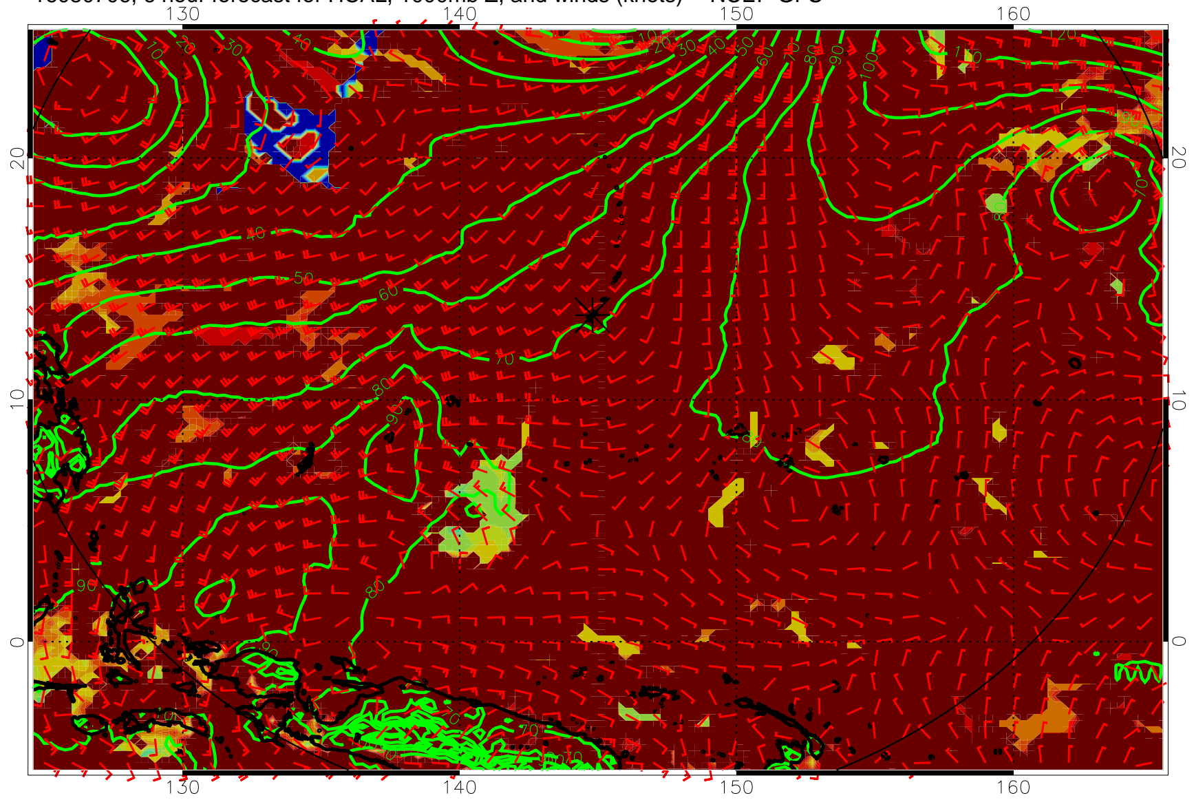
16080706, 6 hour forecast for HCAL, 1000mb Z, and winds (knots) -- NCEP GFS
