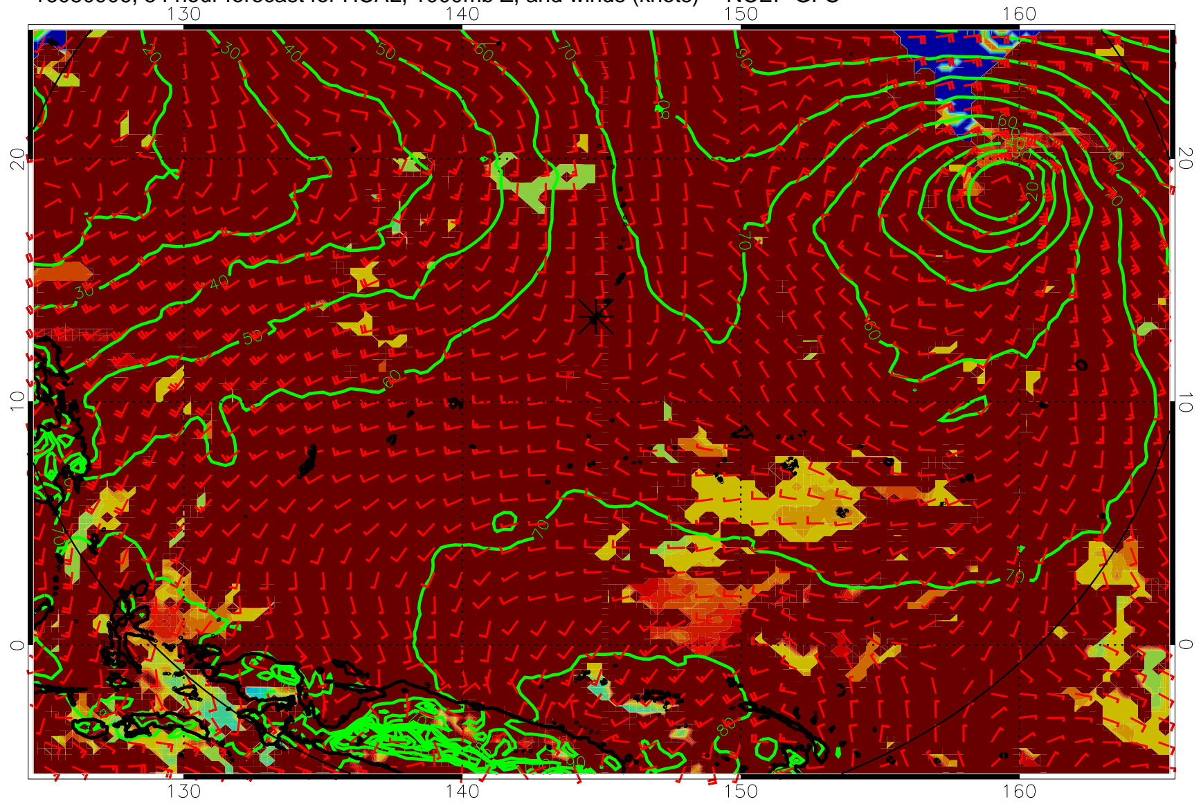
16080906, 54 hour forecast for HCAL, 1000mb Z, and winds (knots) -- NCEP GFS
