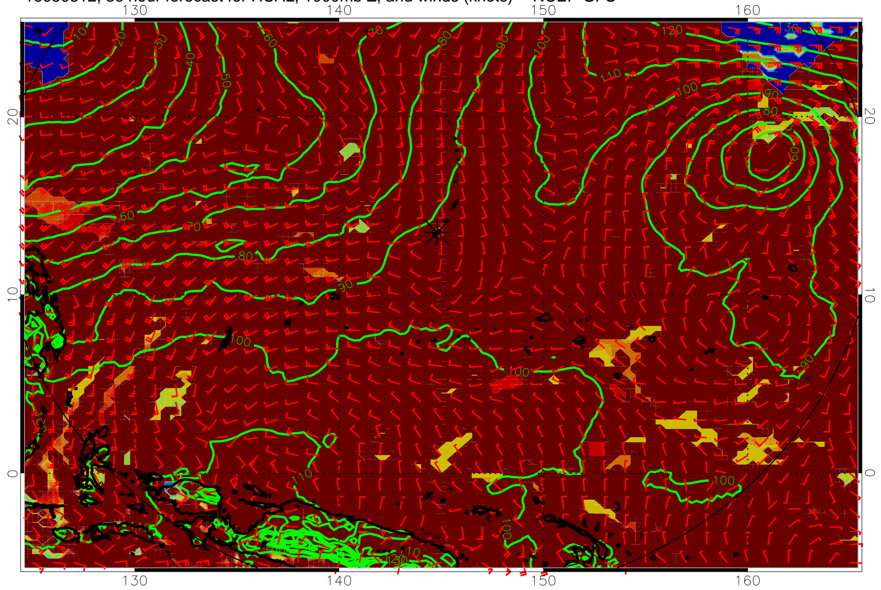
16080812, 36 hour forecast for HCAL, 1000mb Z, and winds (knots) -- NCEP GFS
