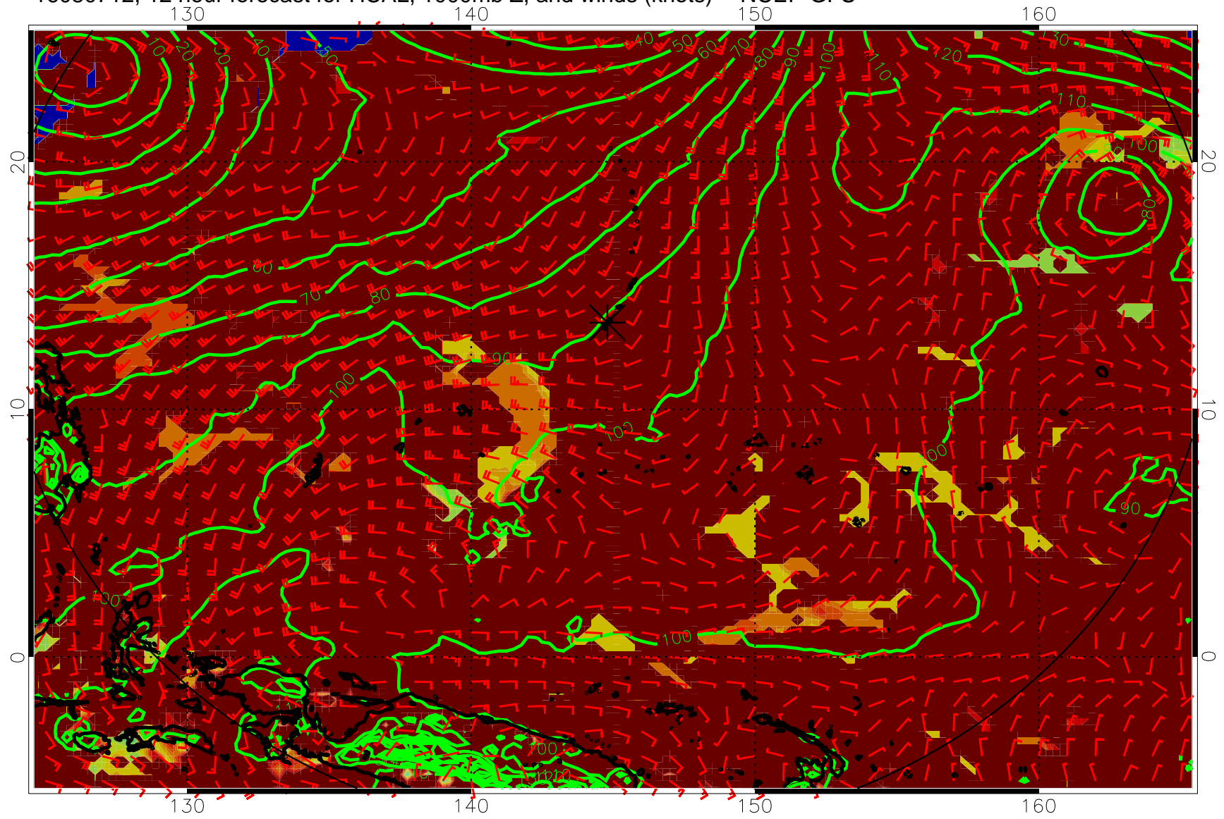
16080712, 12 hour forecast for HCAL, 1000mb Z, and winds (knots) -- NCEP GFS
