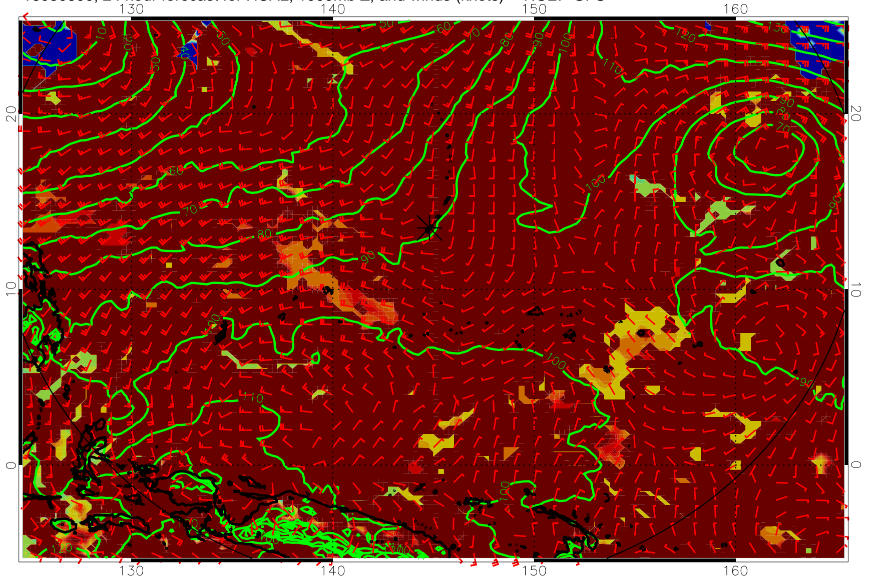
16080800, 24 hour forecast for HCAL, 1000mb Z, and winds (knots) -- NCEP GFS
