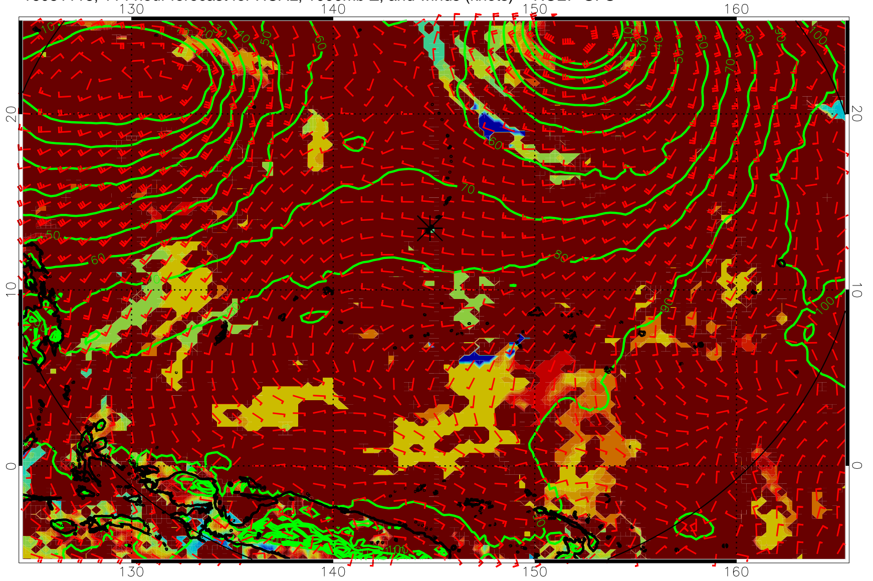
16081118, 114 hour forecast for HCAL, 1000mb Z, and winds (knots) -- NCEP GFS
