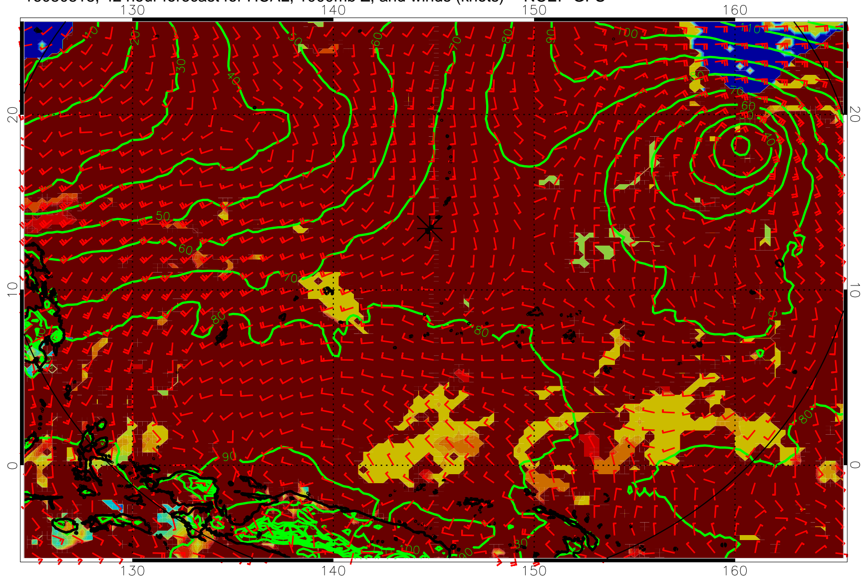
16080818, 42 hour forecast for HCAL, 1000mb Z, and winds (knots) -- NCEP GFS
