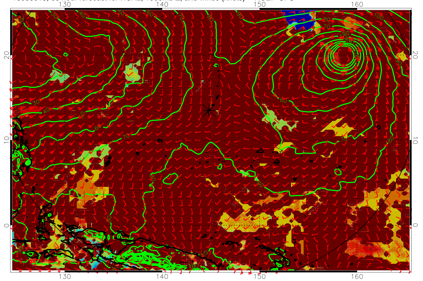
16080918, 66 hour forecast for HCAL, 1000mb Z, and winds (knots) -- NCEP GFS
