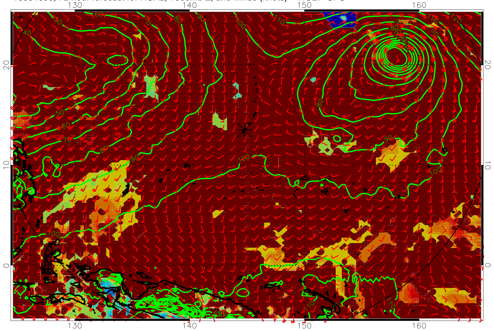
16081000, 72 hour forecast for HCAL, 1000mb Z, and winds (knots) -- NCEP GFS
