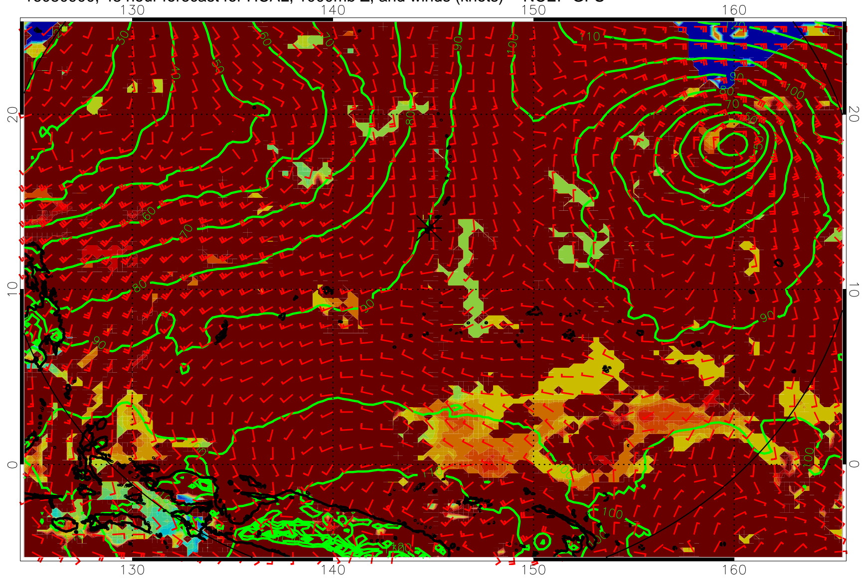
16080900, 48 hour forecast for HCAL, 1000mb Z, and winds (knots) -- NCEP GFS
