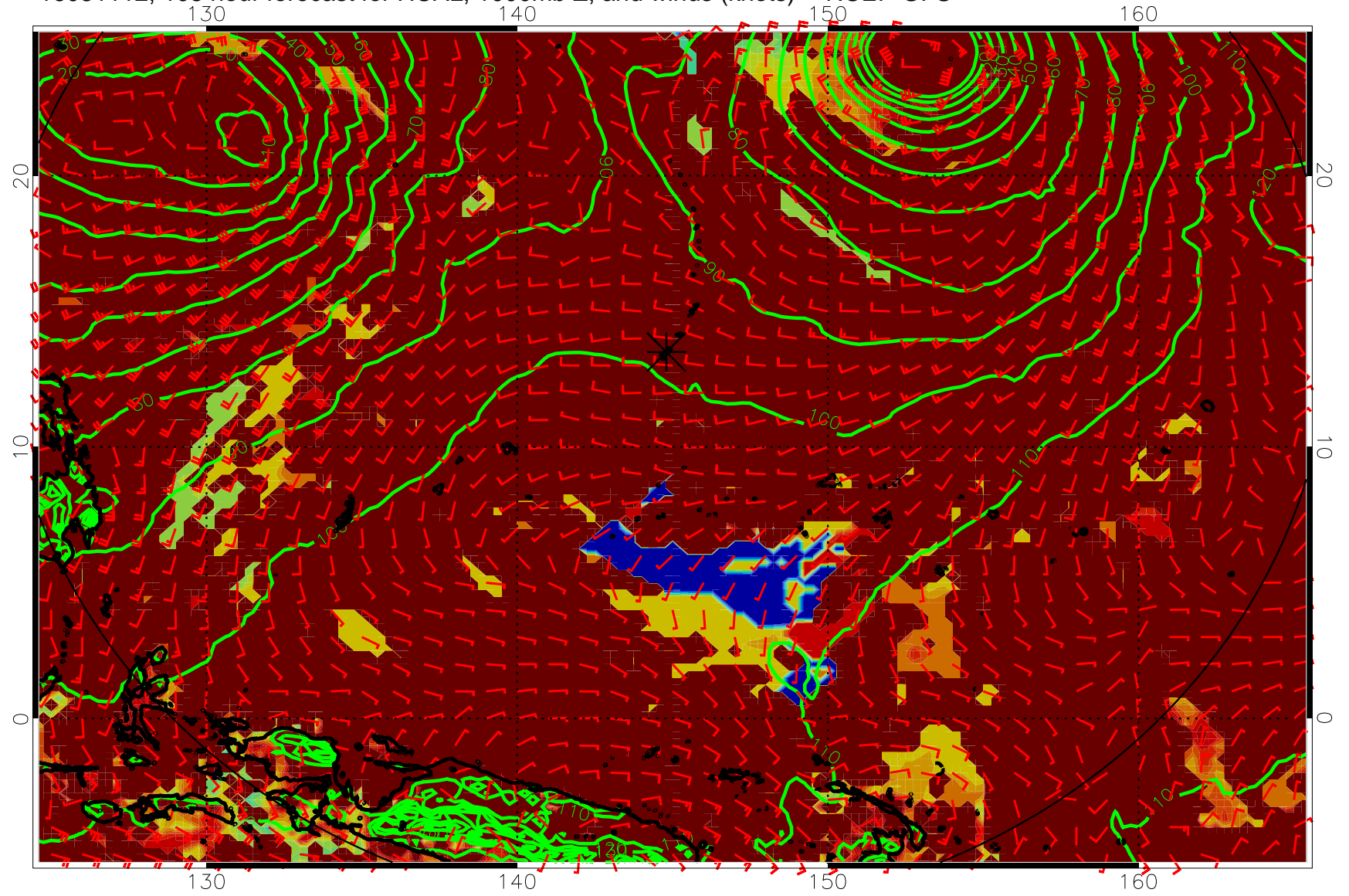
16081112, 108 hour forecast for HCAL, 1000mb Z, and winds (knots) -- NCEP GFS
