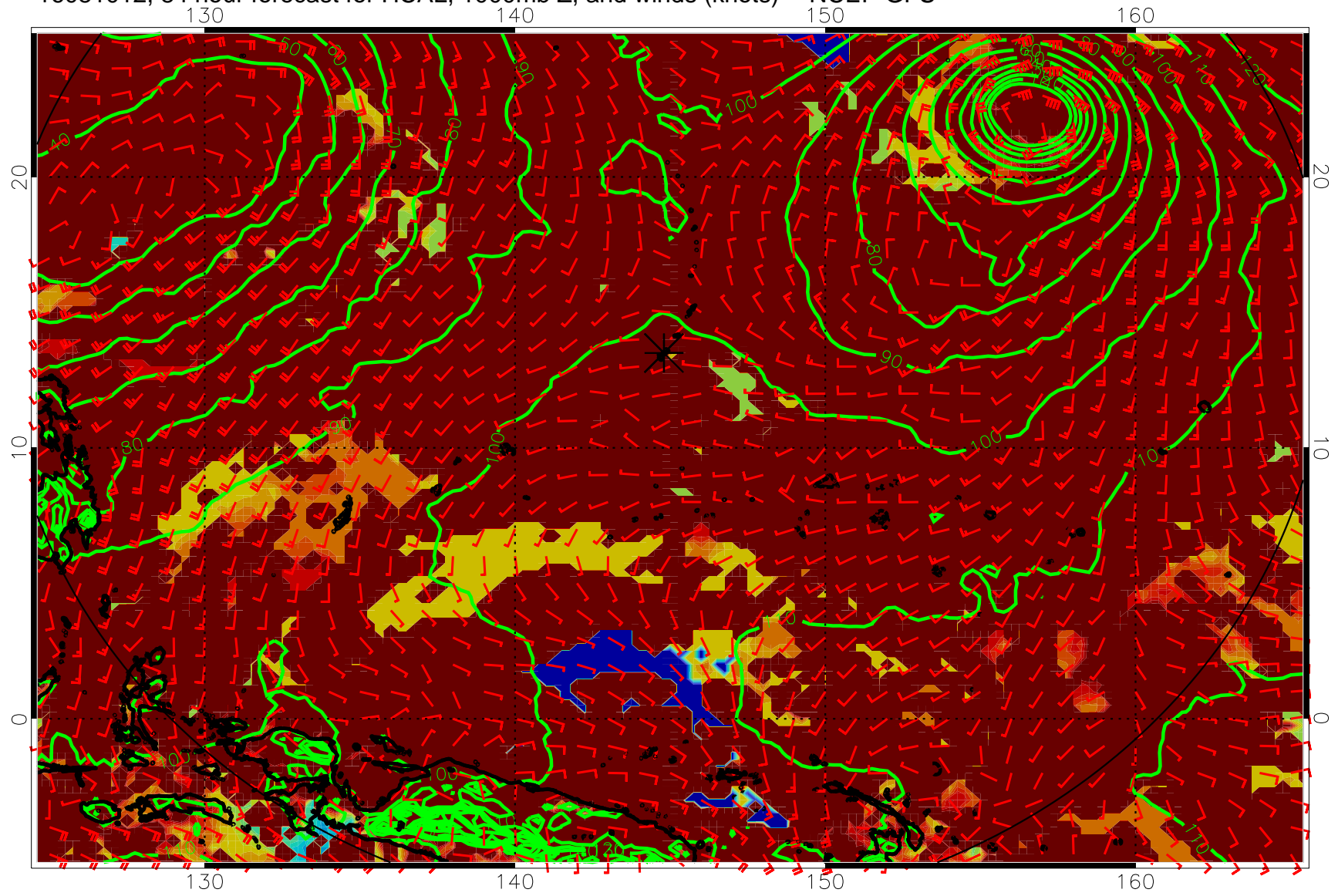
16081012, 84 hour forecast for HCAL, 1000mb Z, and winds (knots) -- NCEP GFS
