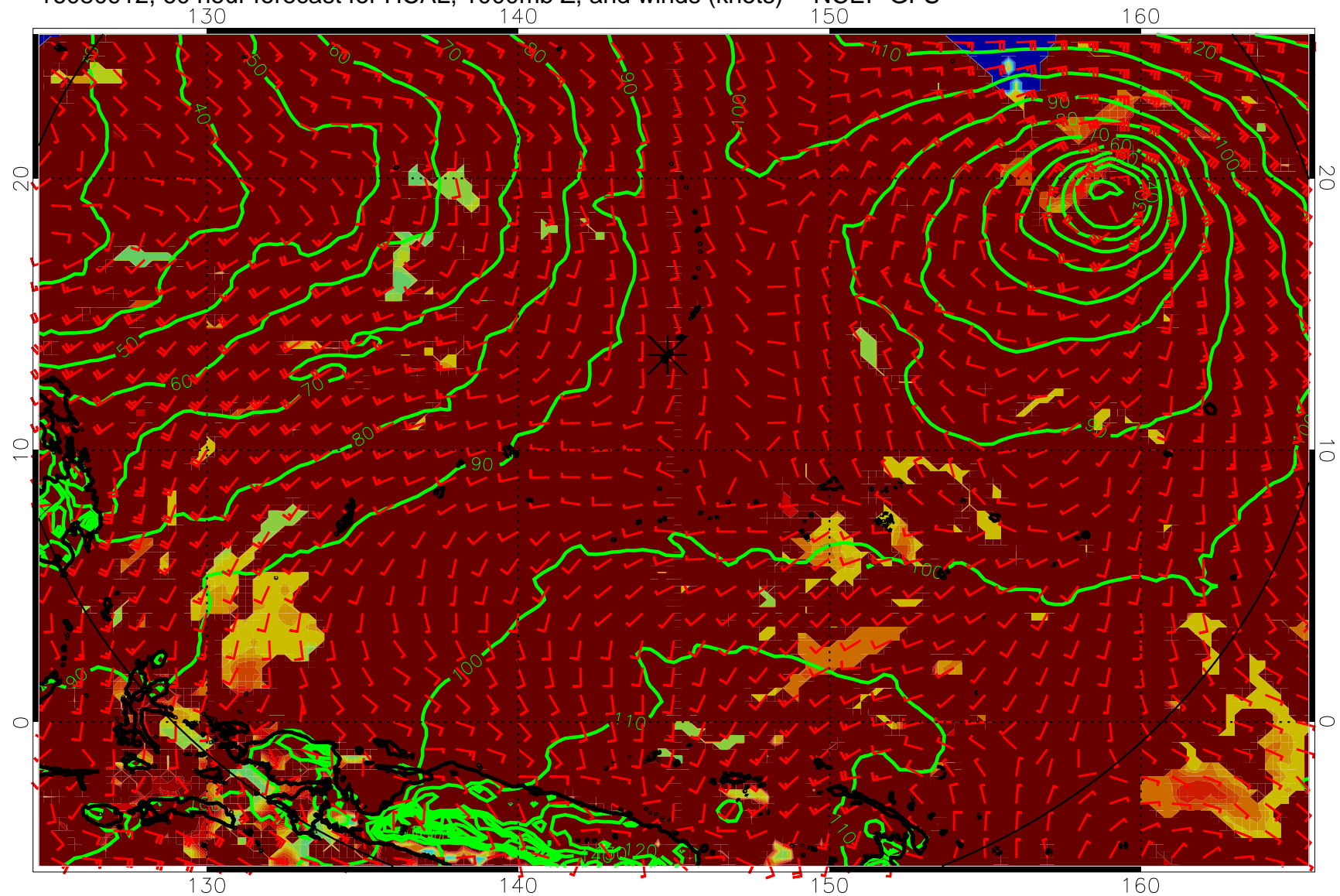
16080912, 60 hour forecast for HCAL, 1000mb Z, and winds (knots) -- NCEP GFS
