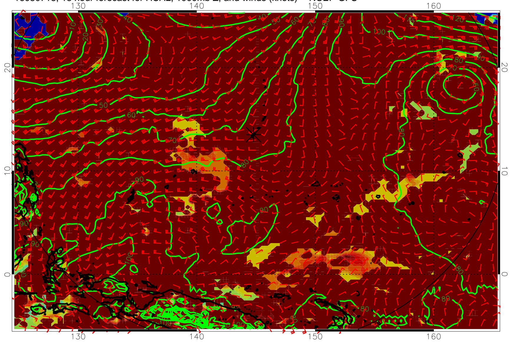
16080718, 18 hour forecast for HCAL, 1000mb Z, and winds (knots) -- NCEP GFS
