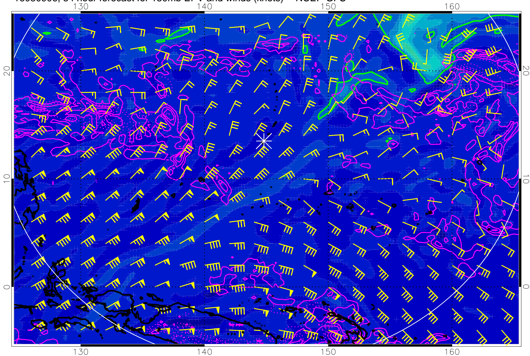
16080906, 54 hour forecast for 150mb EPV and winds (knots) -- NCEP GFS
