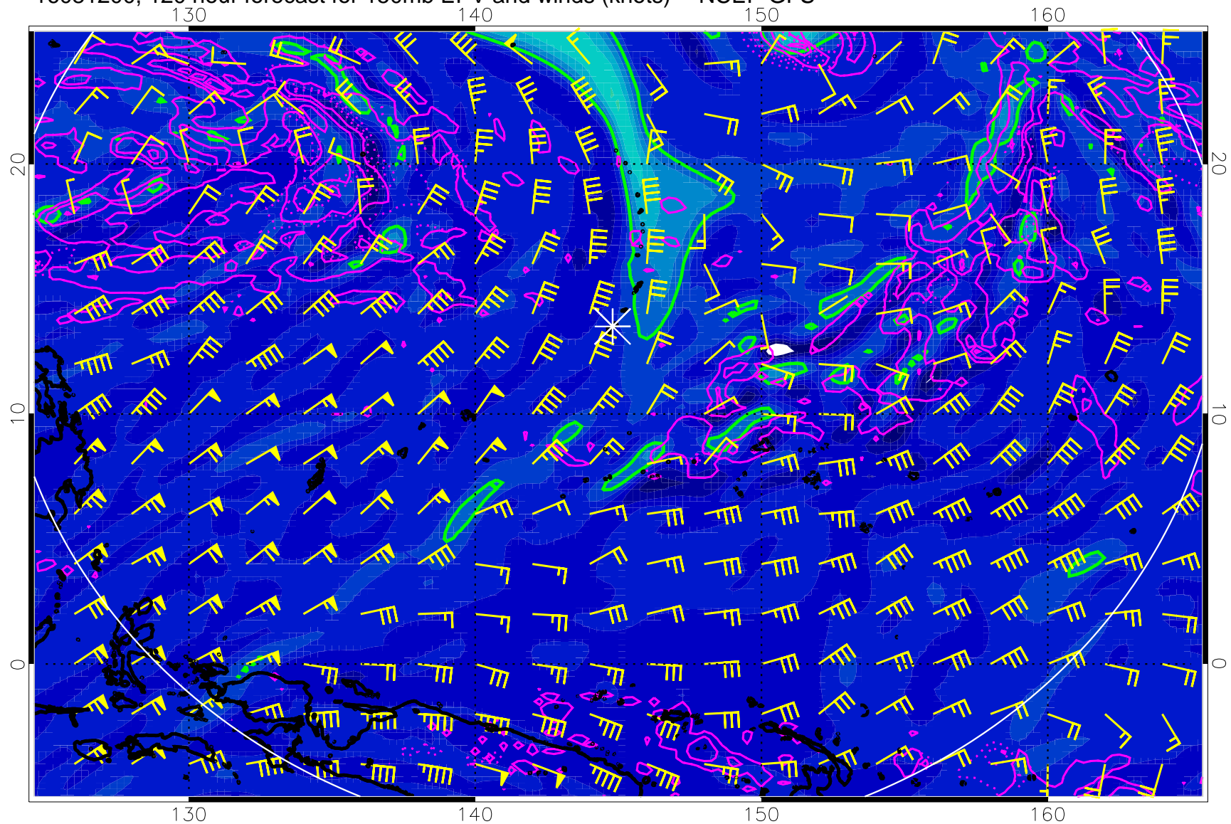
16081200, 120 hour forecast for 150mb EPV and winds (knots) -- NCEP GFS
