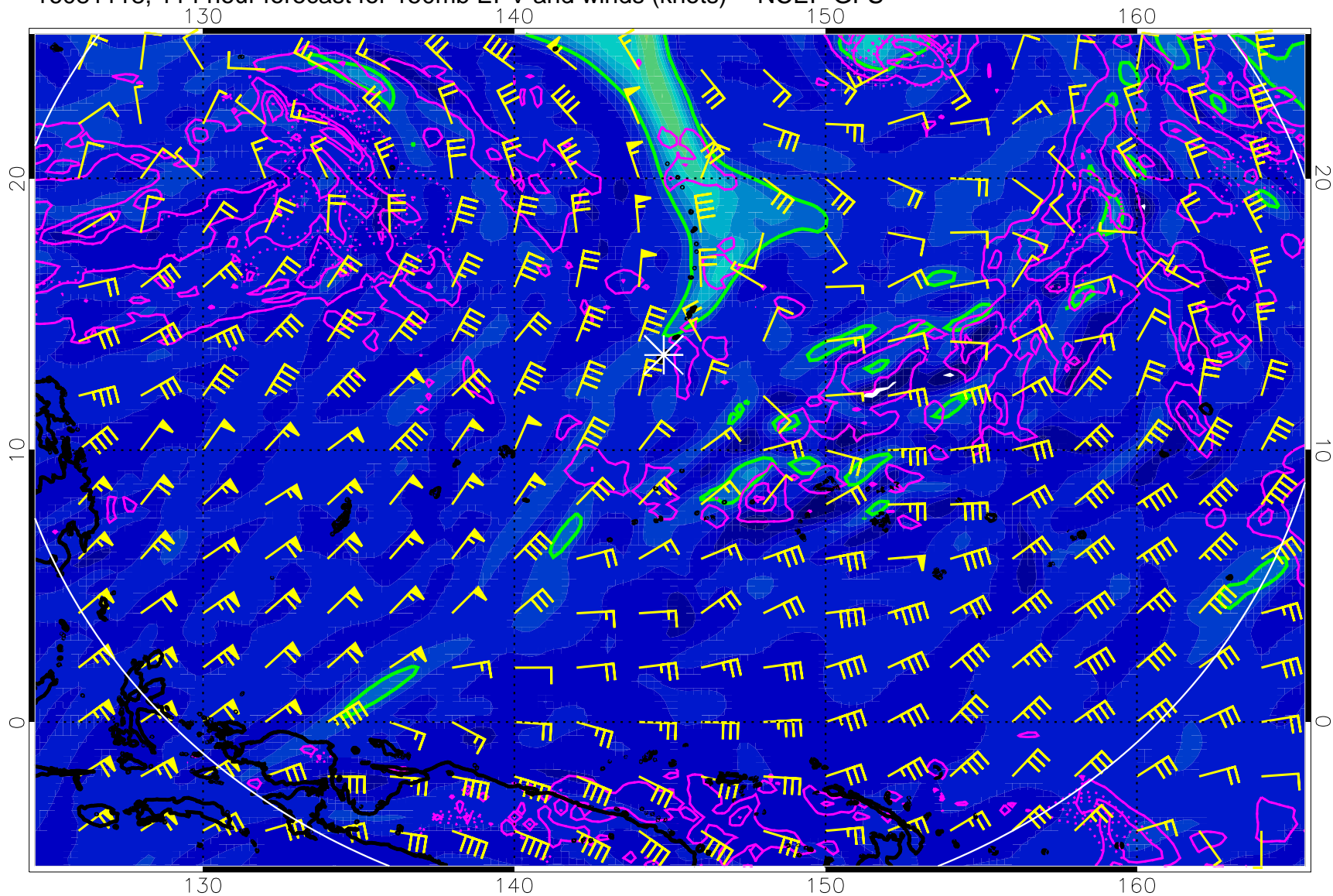
16081118, 114 hour forecast for 150mb EPV and winds (knots) -- NCEP GFS
