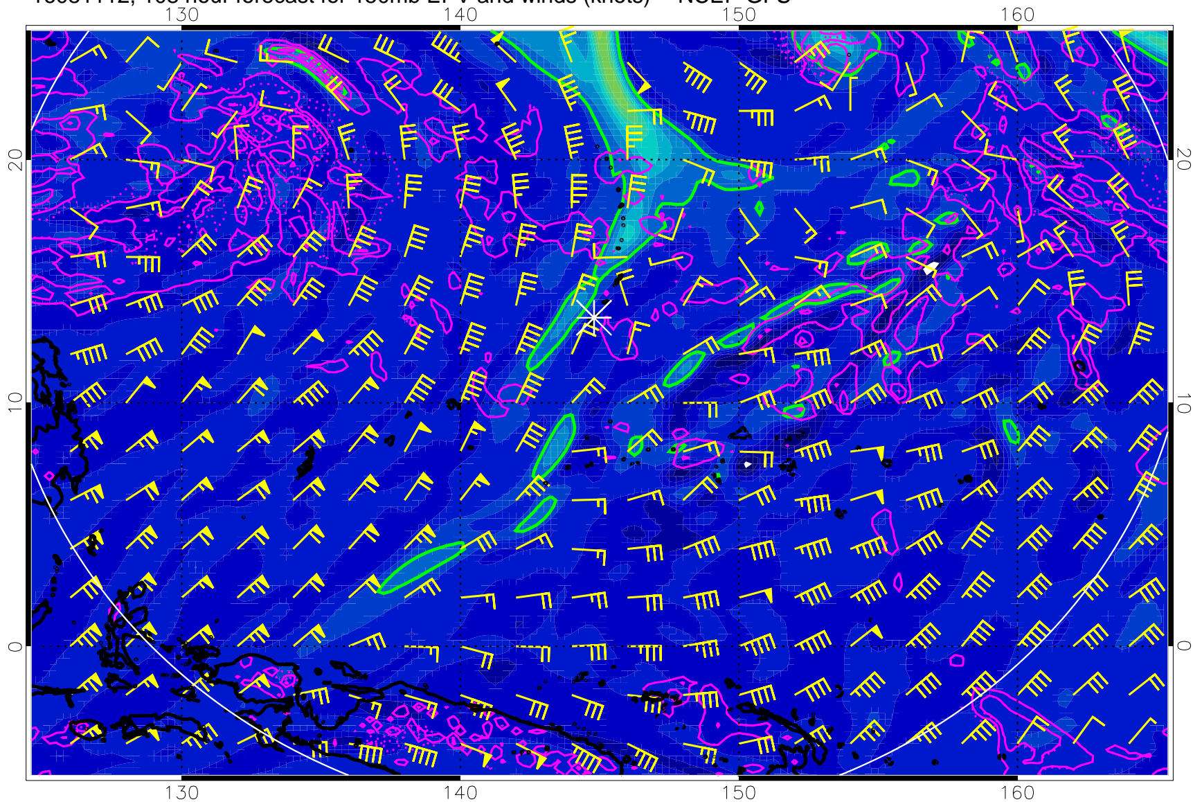
16081112, 108 hour forecast for 150mb EPV and winds (knots) -- NCEP GFS
