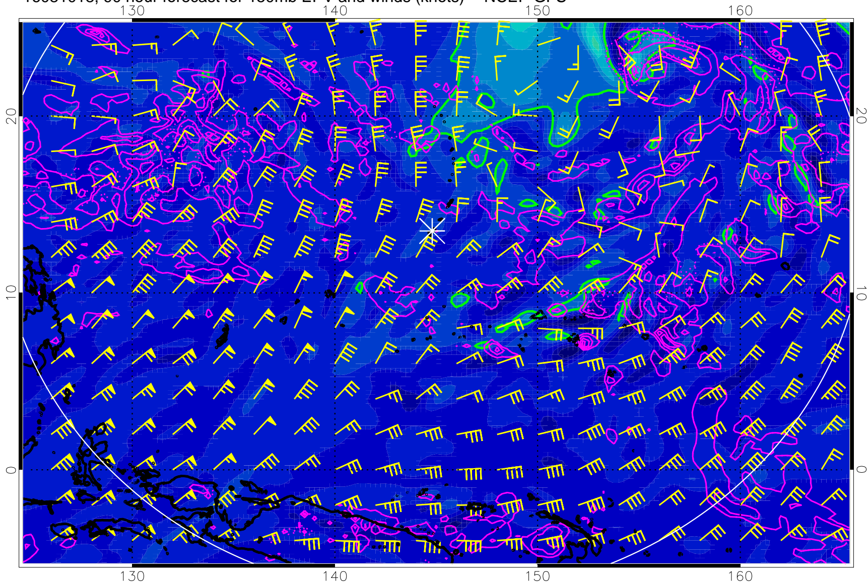
16081018, 90 hour forecast for 150mb EPV and winds (knots) -- NCEP GFS
