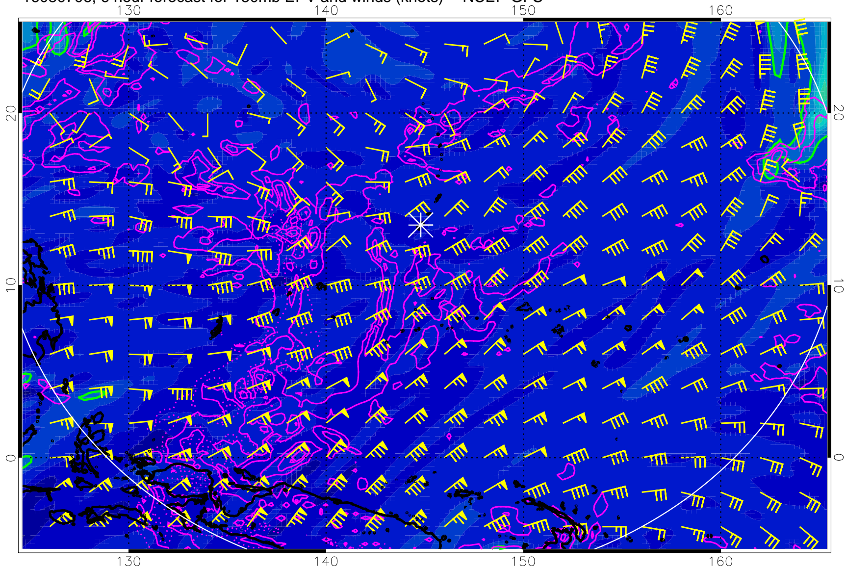
16080706, 6 hour forecast for 150mb EPV and winds (knots) -- NCEP GFS
