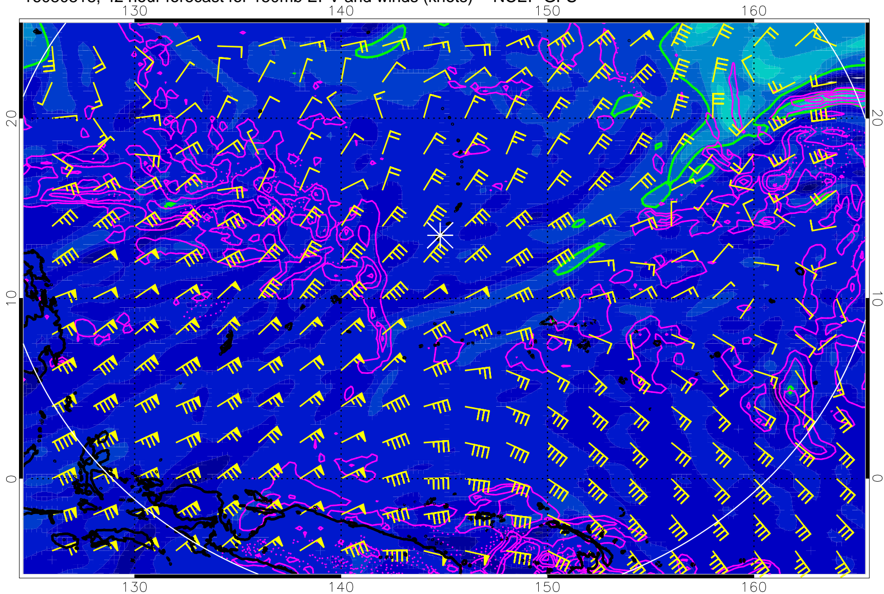
16080818, 42 hour forecast for 150mb EPV and winds (knots) -- NCEP GFS
