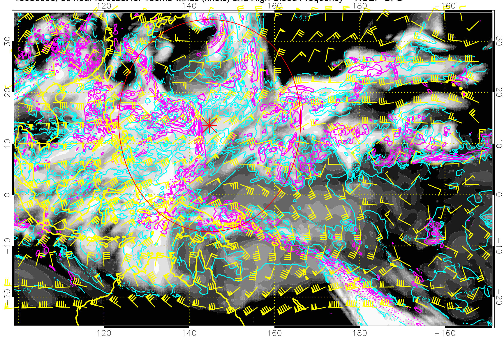
16080806, 30 hour forecast for 150mb winds (knots) and High Cloud Frequency -- NCEP GFS
