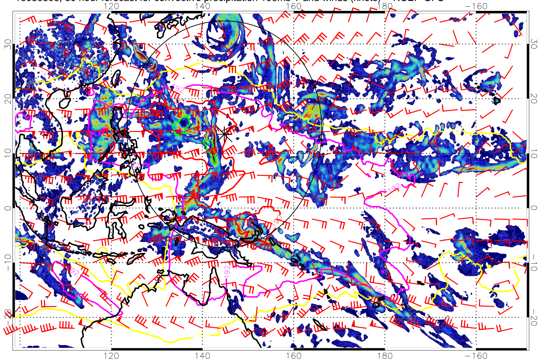
16080806, 30 hour forecast for convective precipitation 100mb T and winds (knots) -- NCEP GFS
