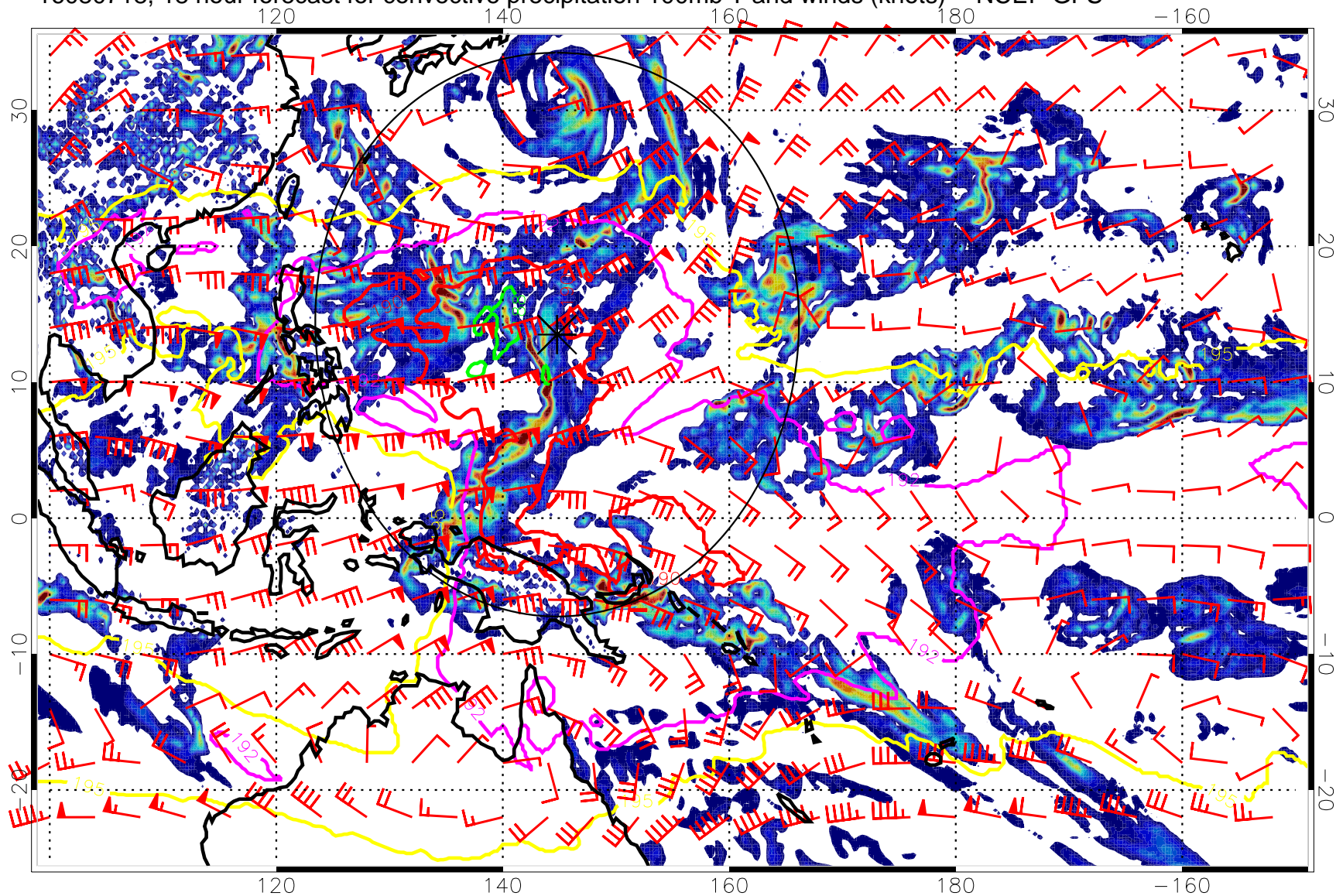
16080718, 18 hour forecast for convective precipitation 100mb T and winds (knots) -- NCEP GFS
