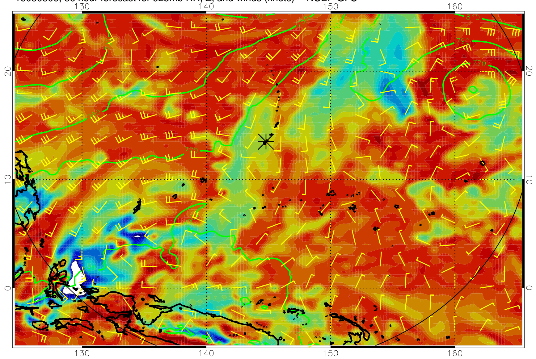
16080800, 36 hour forecast for 925mb RH, Z, and winds (knots) -- NCEP GFS
