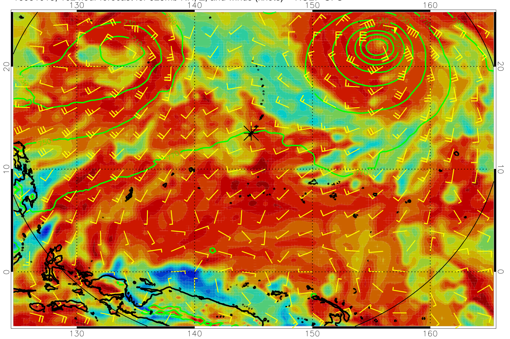
16081018, 102 hour forecast for 925mb RH, Z, and winds (knots) -- NCEP GFS
