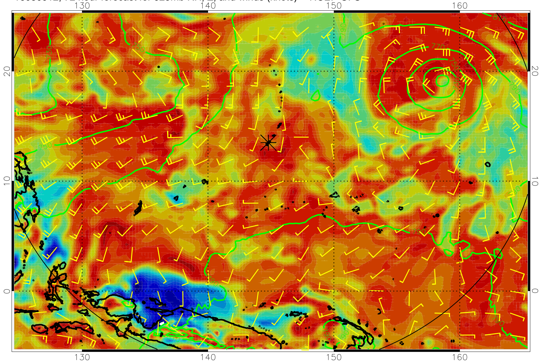
16080912, 72 hour forecast for 925mb RH, Z, and winds (knots) -- NCEP GFS
