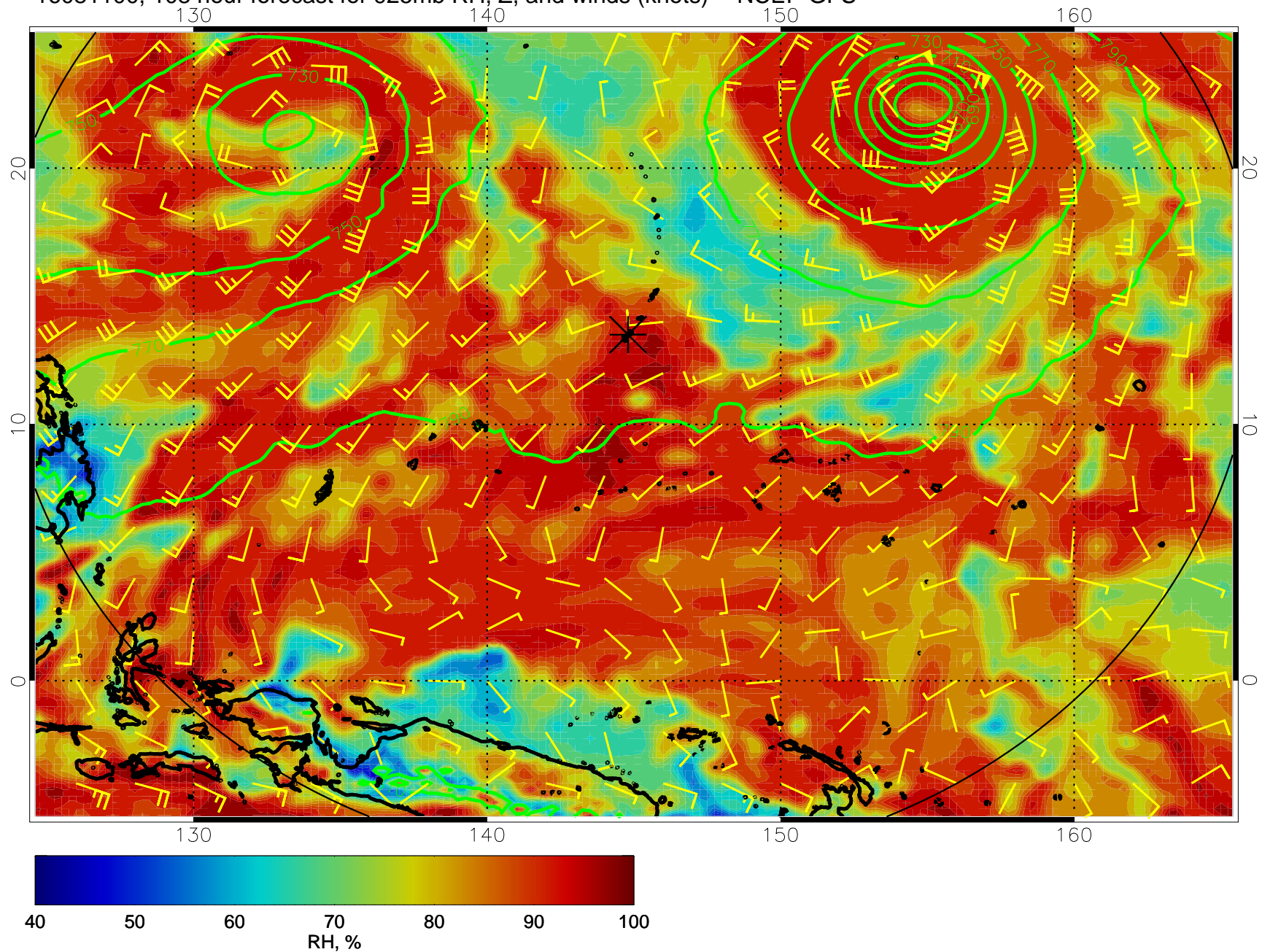
16081100, 108 hour forecast for 925mb RH, Z, and winds (knots) -- NCEP GFS
