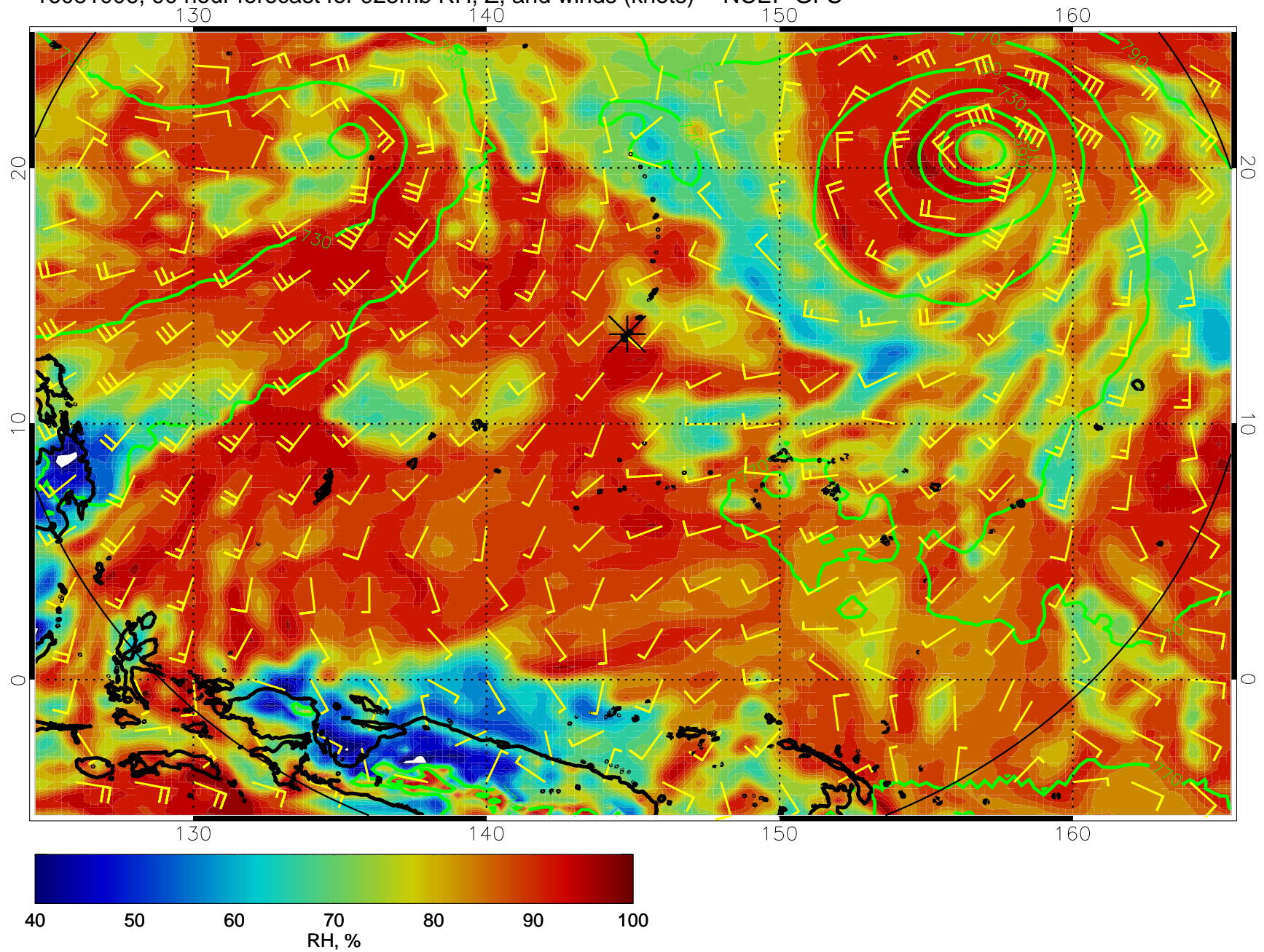
16081006, 90 hour forecast for 925mb RH, Z, and winds (knots) -- NCEP GFS
