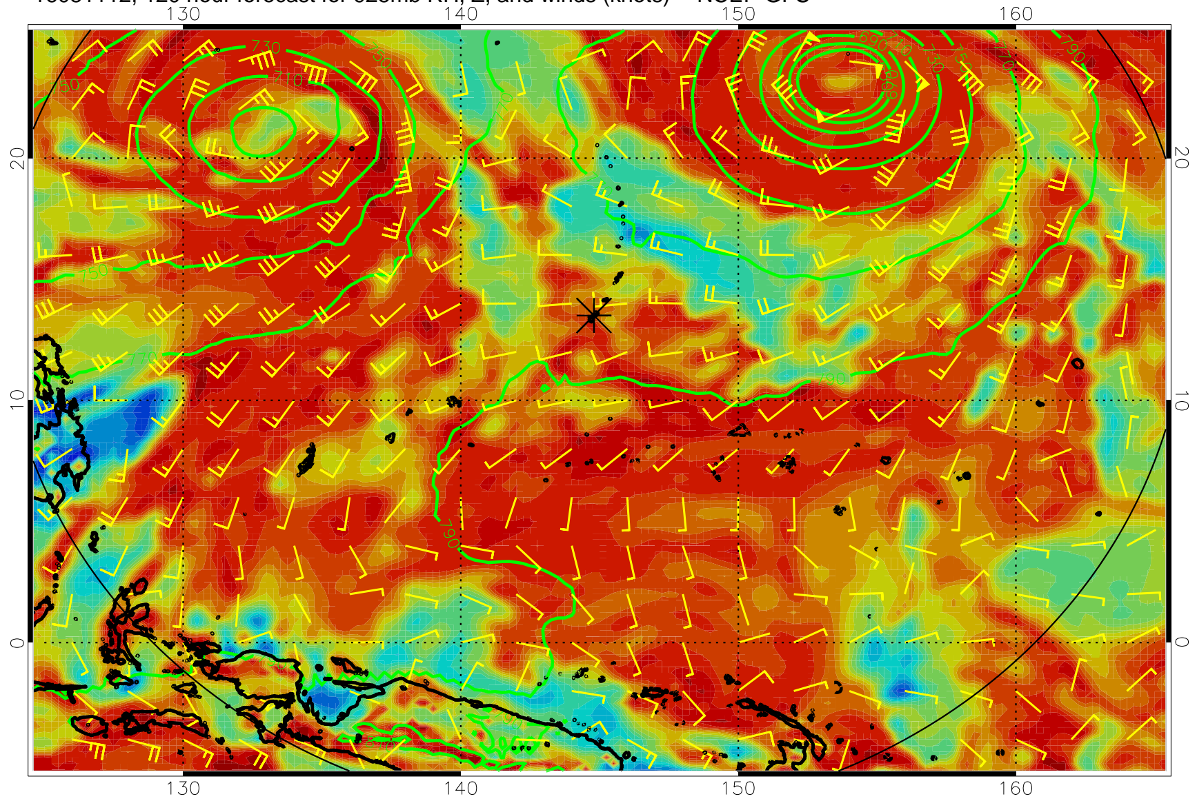
16081112, 120 hour forecast for 925mb RH, Z, and winds (knots) -- NCEP GFS
