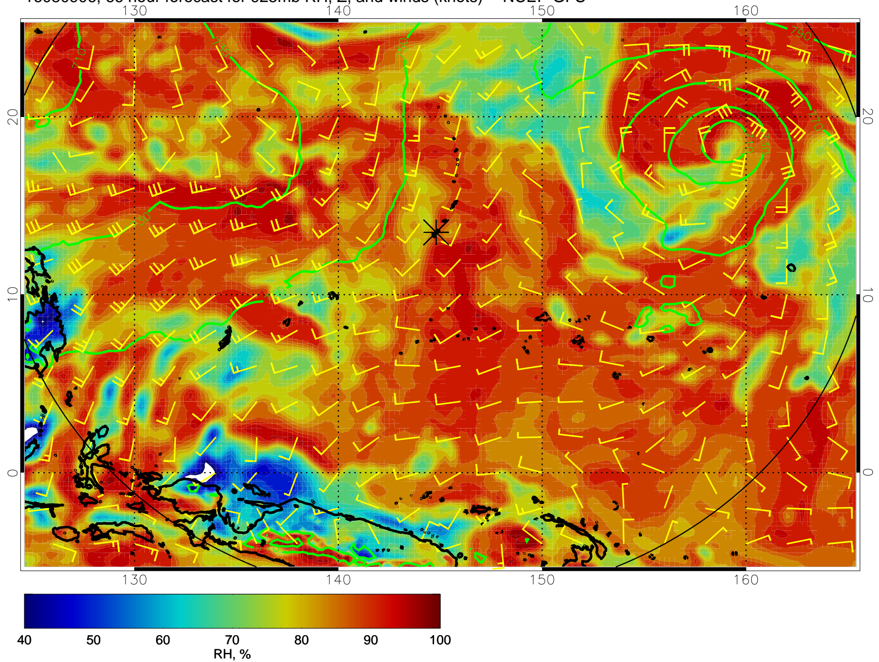
16080906, 66 hour forecast for 925mb RH, Z, and winds (knots) -- NCEP GFS
