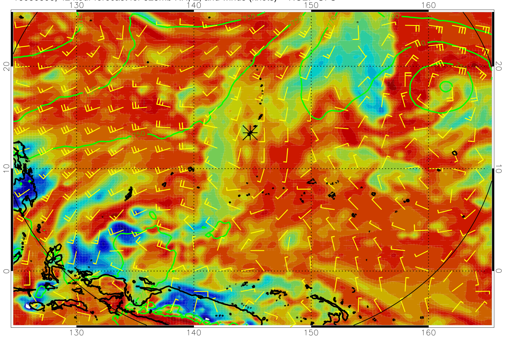
16080806, 42 hour forecast for 925mb RH, Z, and winds (knots) -- NCEP GFS
