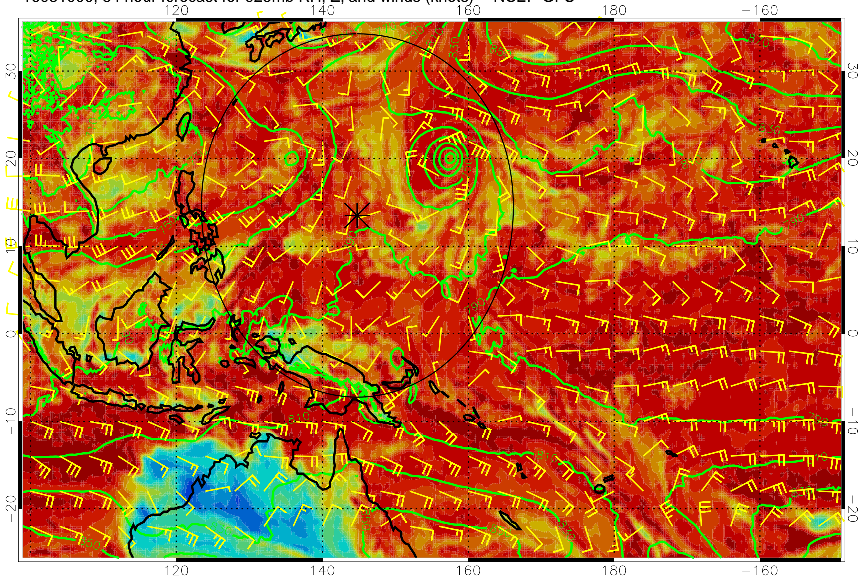
16081000, 84 hour forecast for 925mb RH, Z, and winds (knots) -- NCEP GFS
