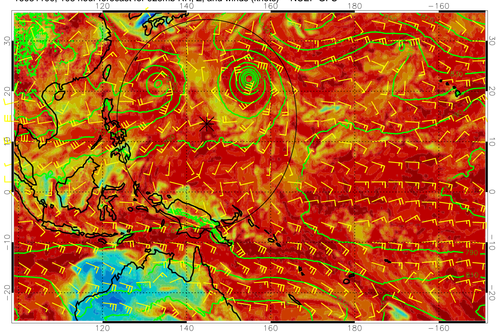
16081100, 108 hour forecast for 925mb RH, Z, and winds (knots) -- NCEP GFS
