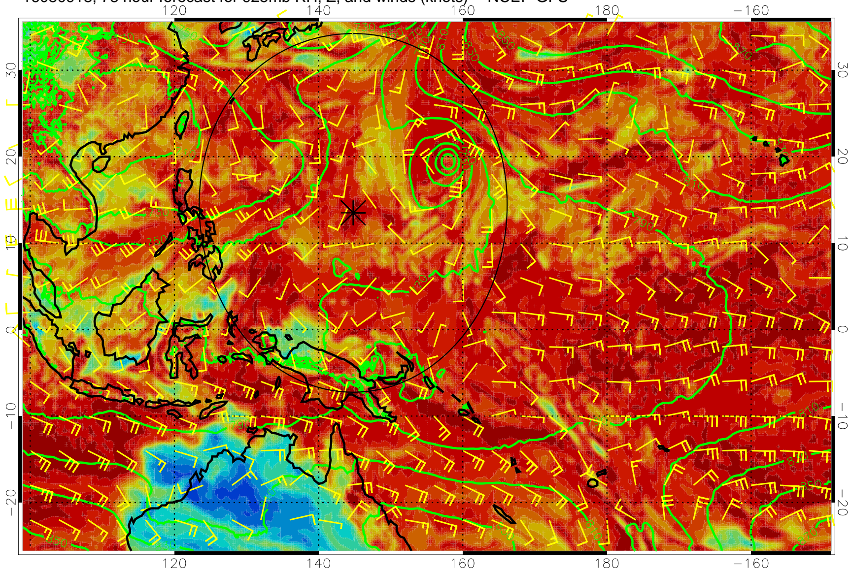
16080918, 78 hour forecast for 925mb RH, Z, and winds (knots) -- NCEP GFS
