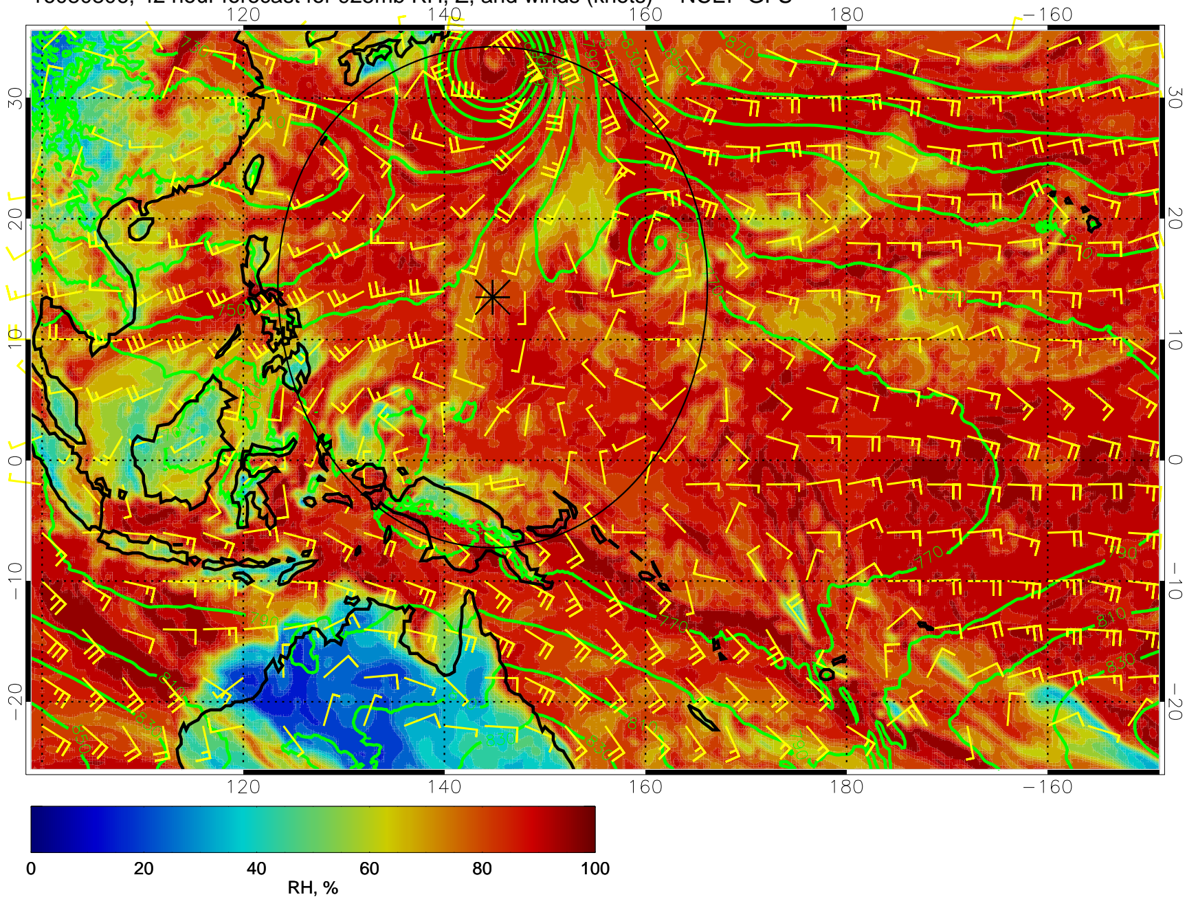
16080806, 42 hour forecast for 925mb RH, Z, and winds (knots) -- NCEP GFS
