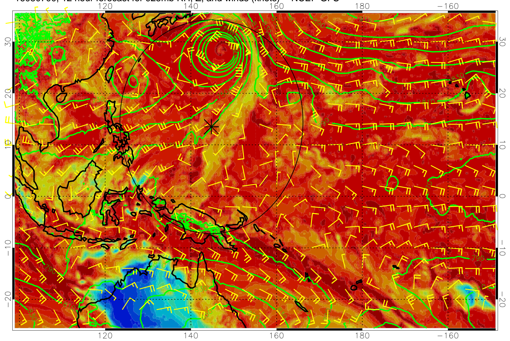
16080700, 12 hour forecast for 925mb RH, Z, and winds (knots) -- NCEP GFS
