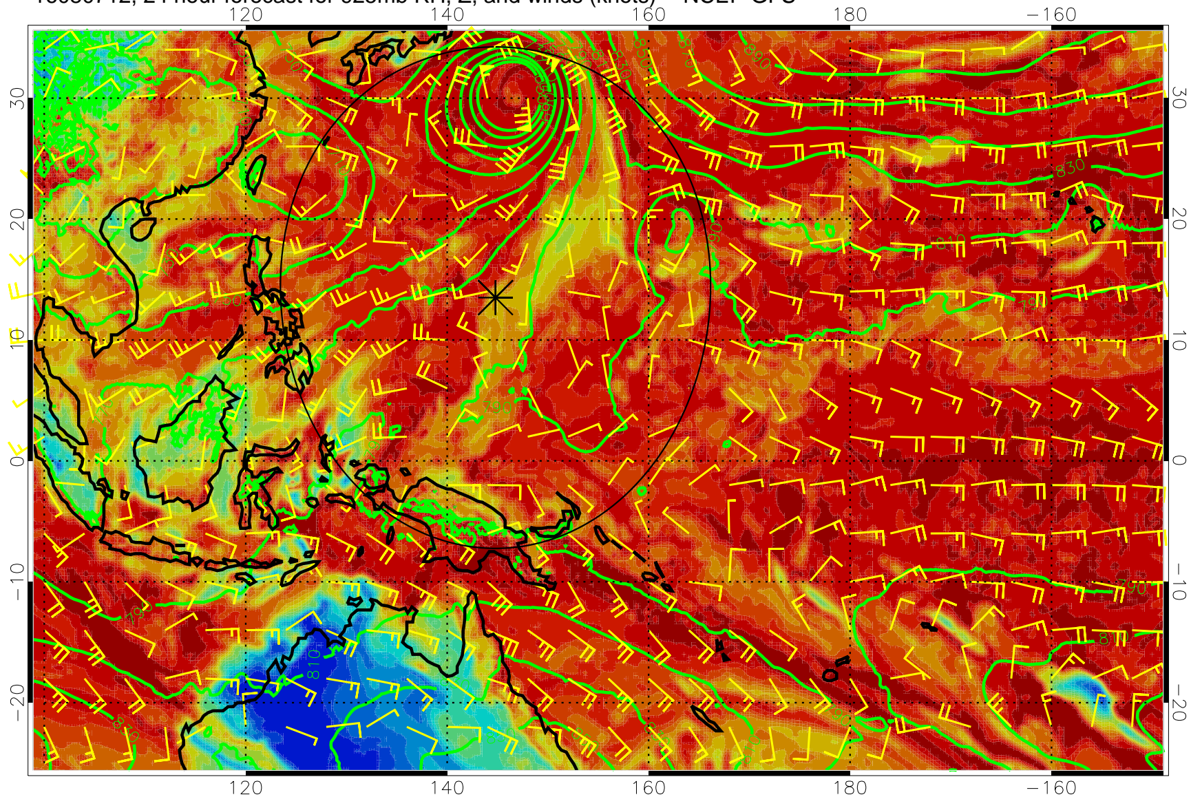
16080712, 24 hour forecast for 925mb RH, Z, and winds (knots) -- NCEP GFS
