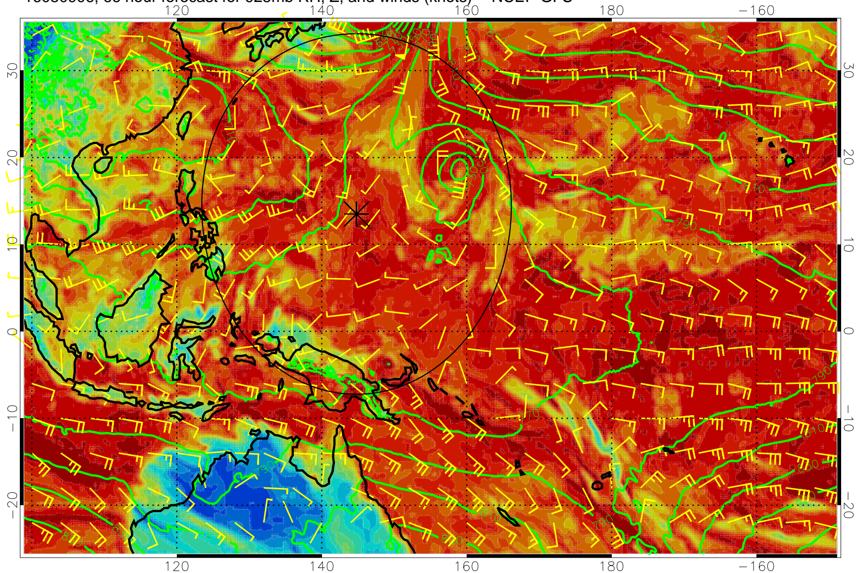
16080906, 66 hour forecast for 925mb RH, Z, and winds (knots) -- NCEP GFS
