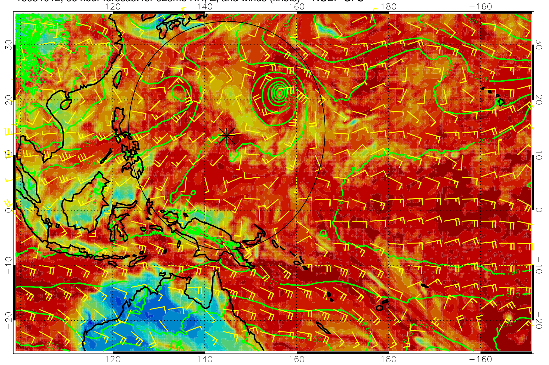
16081012, 96 hour forecast for 925mb RH, Z, and winds (knots) -- NCEP GFS
