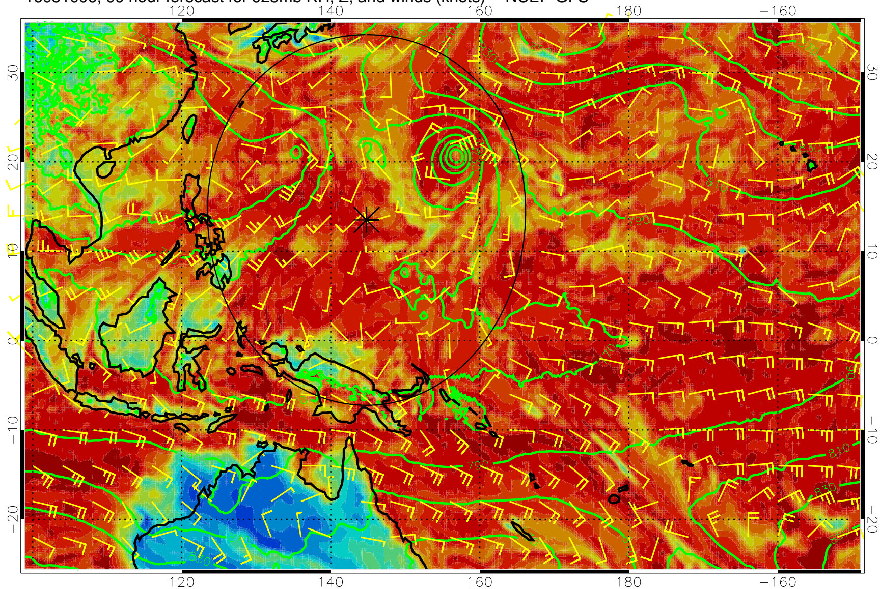
16081006, 90 hour forecast for 925mb RH, Z, and winds (knots) -- NCEP GFS
