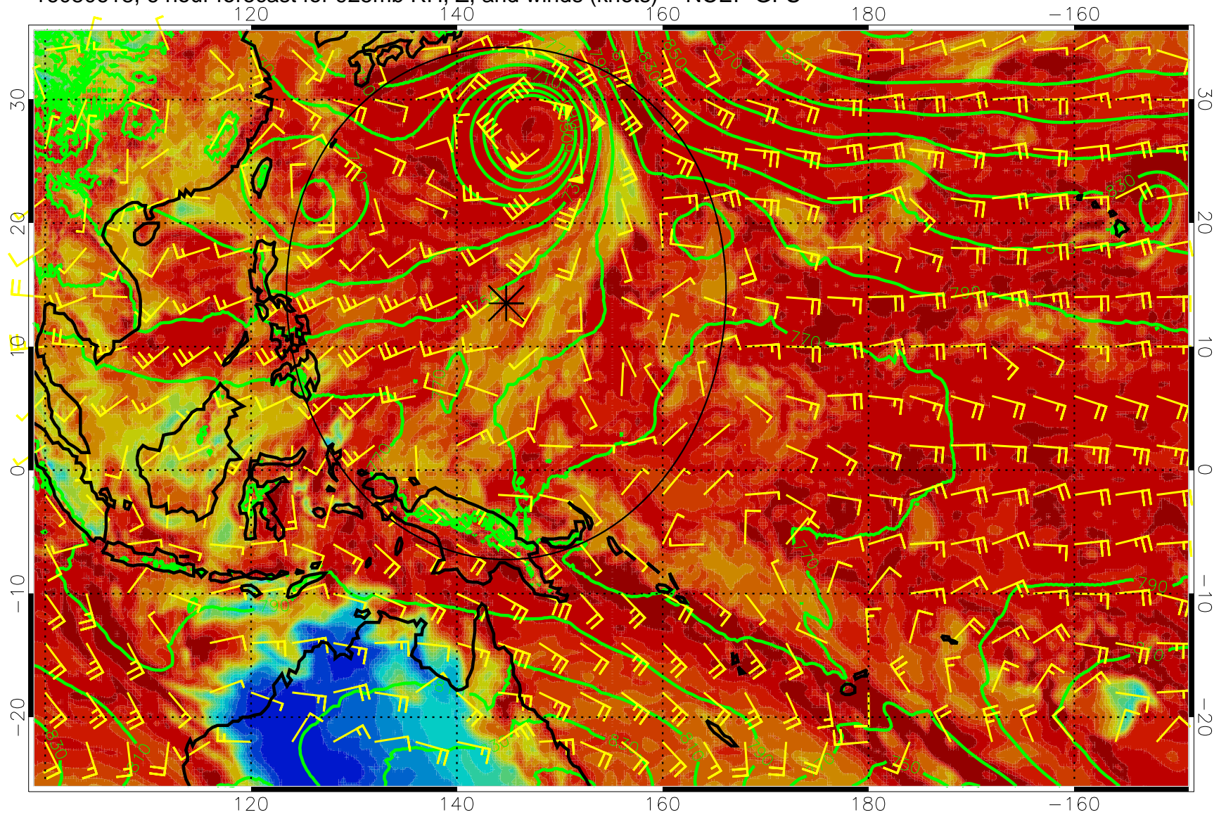
16080618, 6 hour forecast for 925mb RH, Z, and winds (knots) -- NCEP GFS
