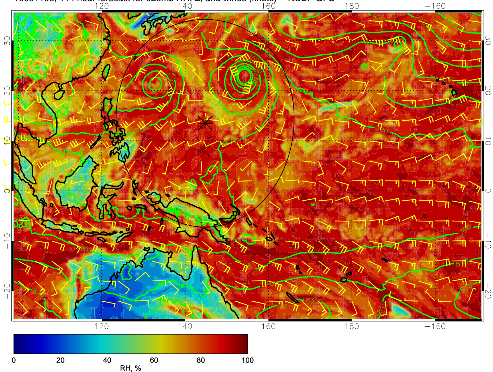
16081106, 114 hour forecast for 925mb RH, Z, and winds (knots) -- NCEP GFS
