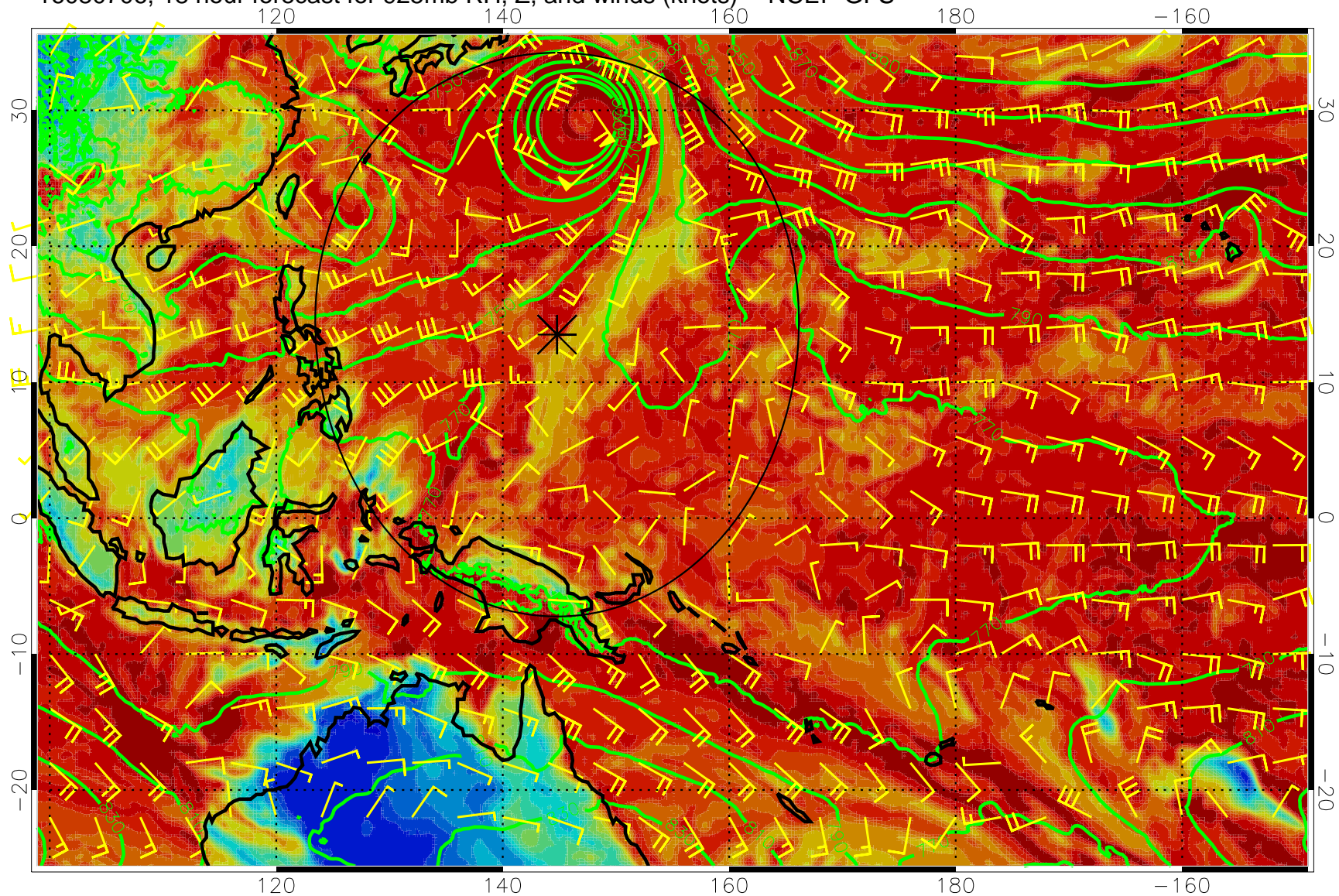
16080706, 18 hour forecast for 925mb RH, Z, and winds (knots) -- NCEP GFS
