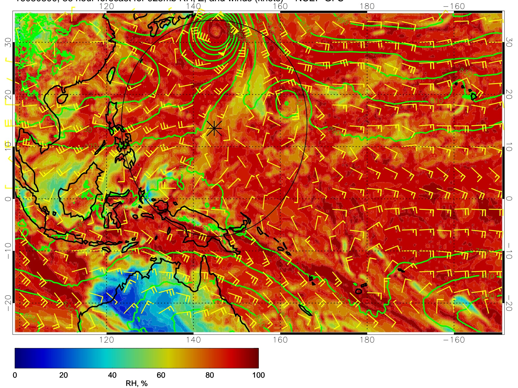
16080800, 36 hour forecast for 925mb RH, Z, and winds (knots) -- NCEP GFS
