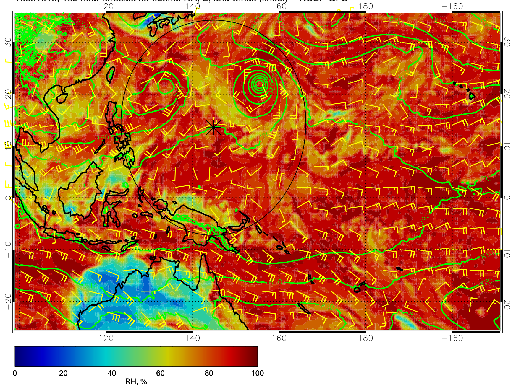
16081018, 102 hour forecast for 925mb RH, Z, and winds (knots) -- NCEP GFS
