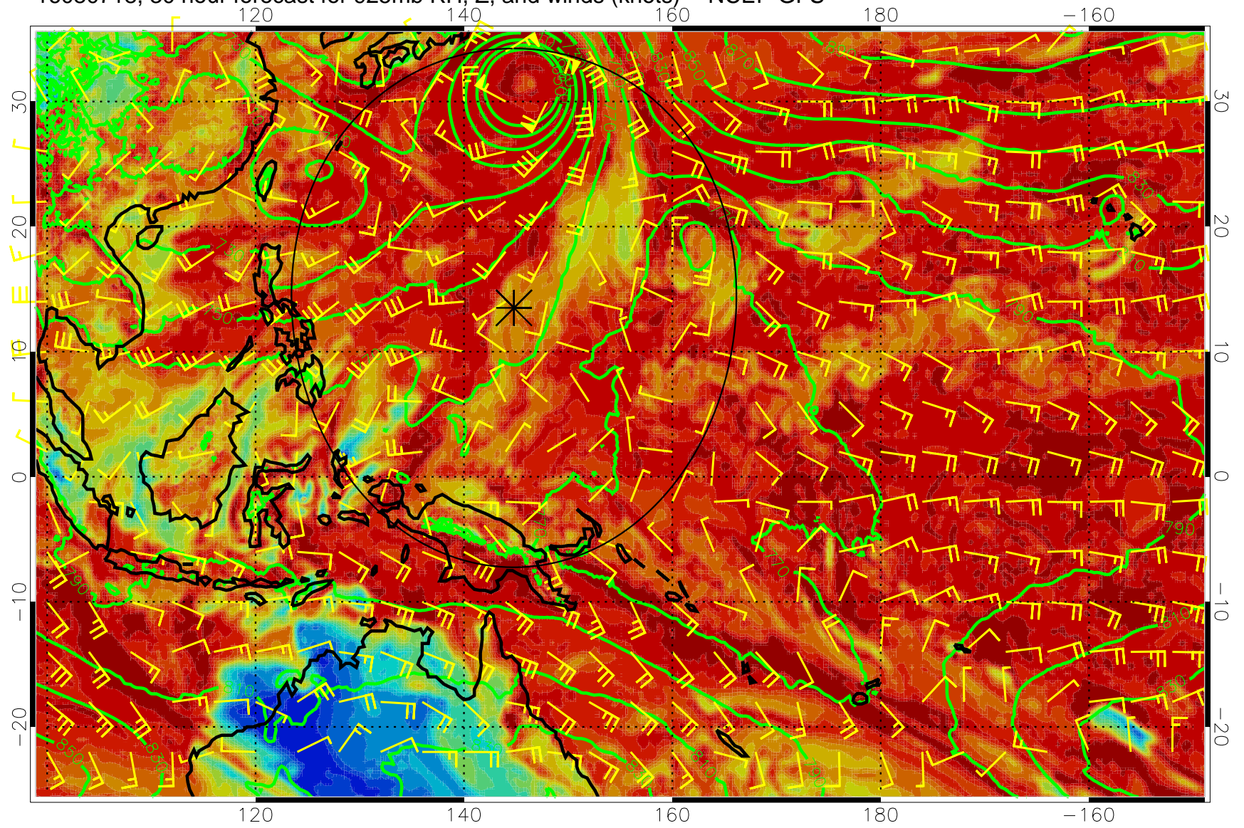
16080718, 30 hour forecast for 925mb RH, Z, and winds (knots) -- NCEP GFS
