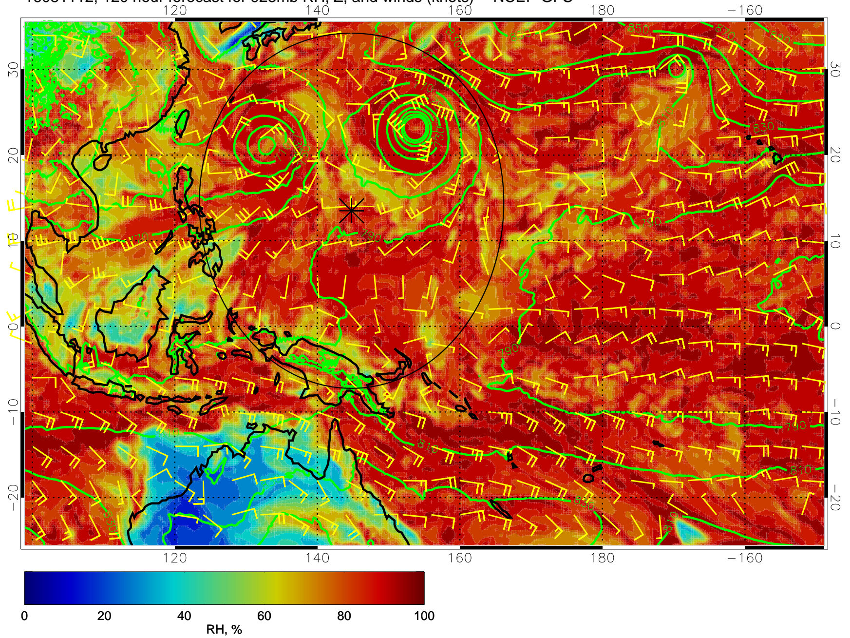
16081112, 120 hour forecast for 925mb RH, Z, and winds (knots) -- NCEP GFS
