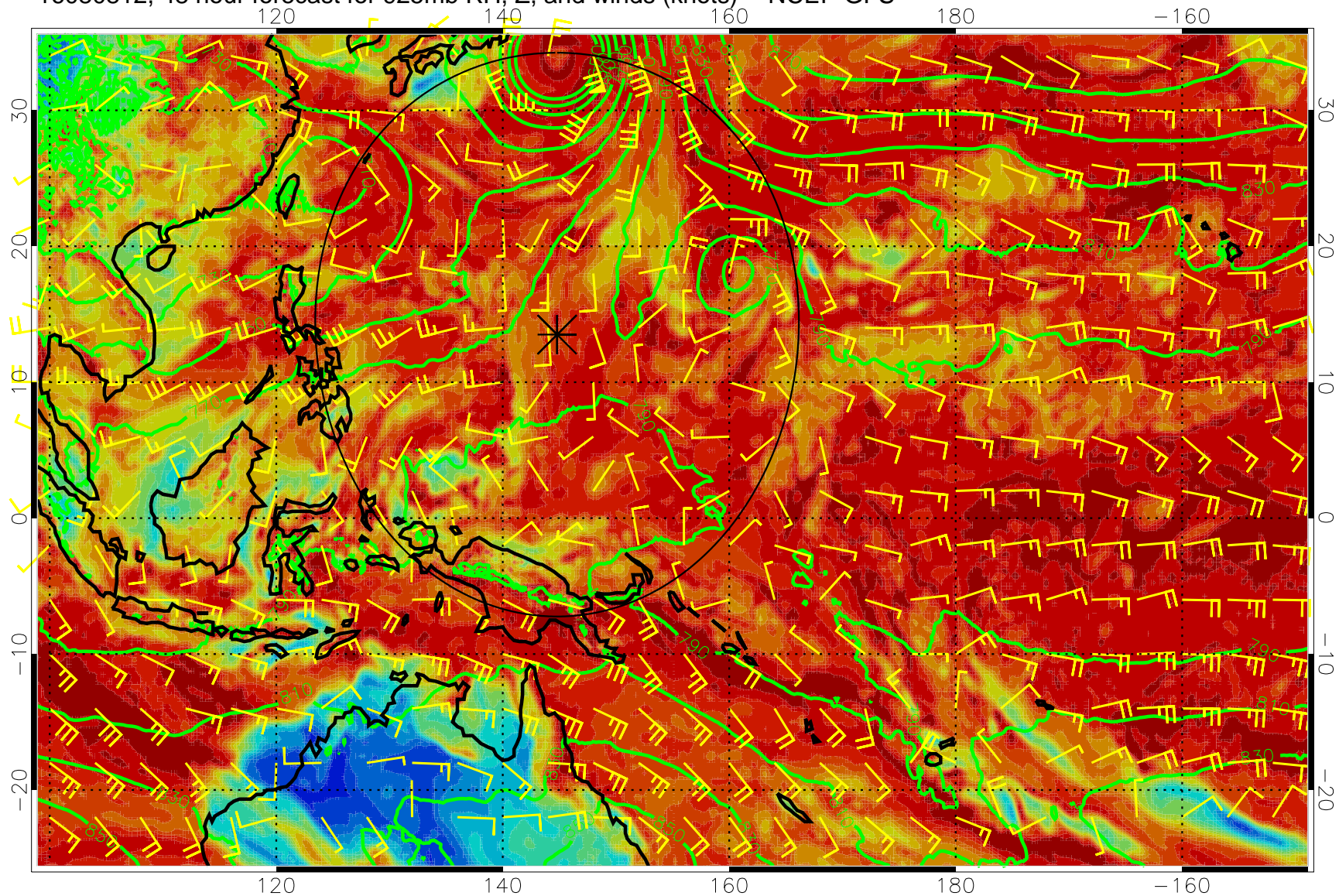
16080812, 48 hour forecast for 925mb RH, Z, and winds (knots) -- NCEP GFS
