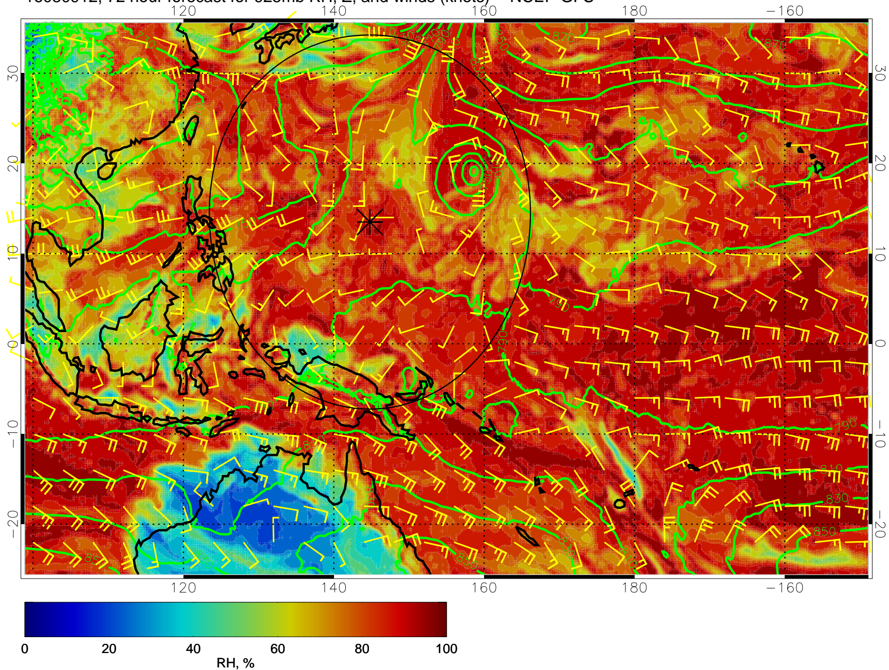
16080912, 72 hour forecast for 925mb RH, Z, and winds (knots) -- NCEP GFS
