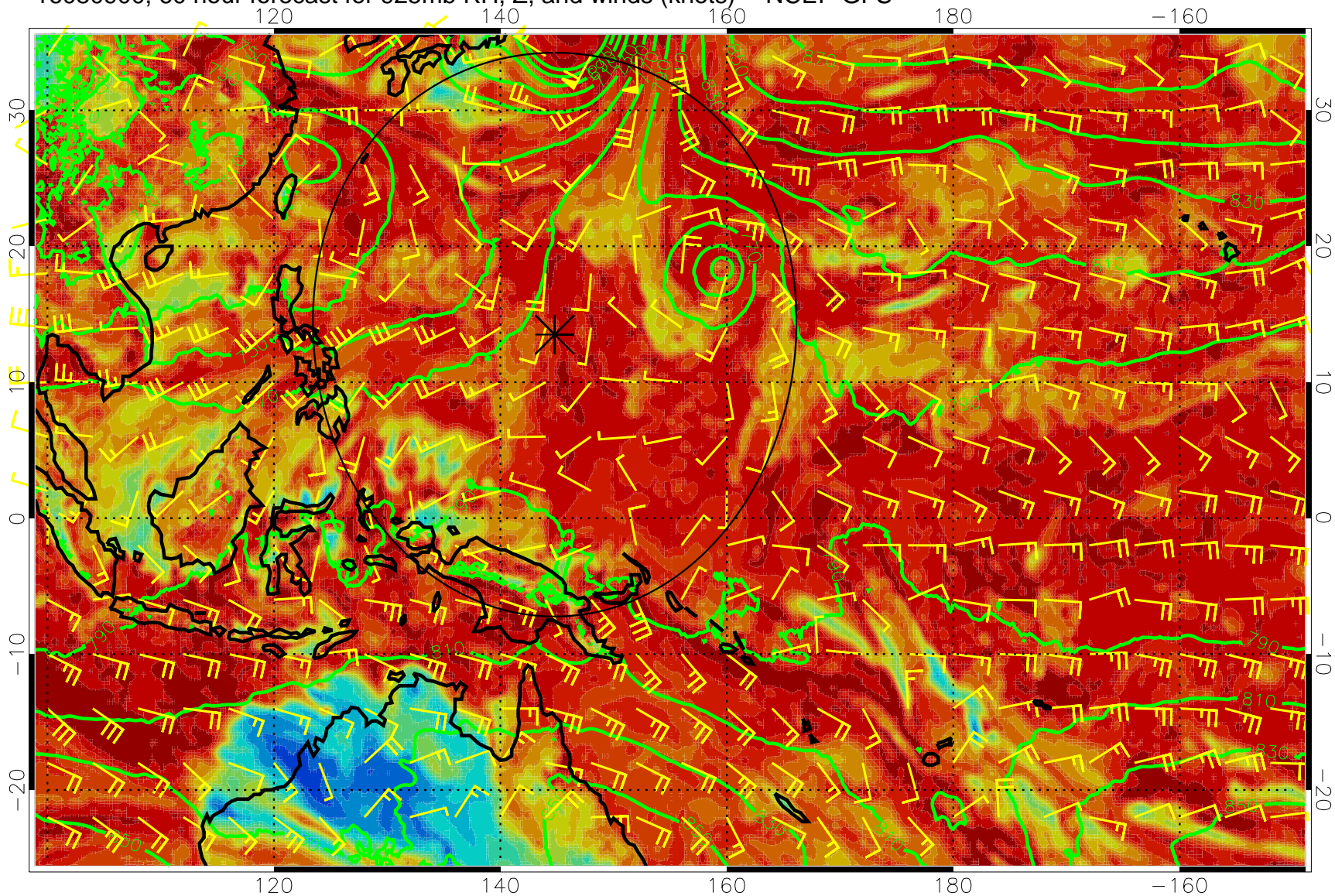
16080900, 60 hour forecast for 925mb RH, Z, and winds (knots) -- NCEP GFS
