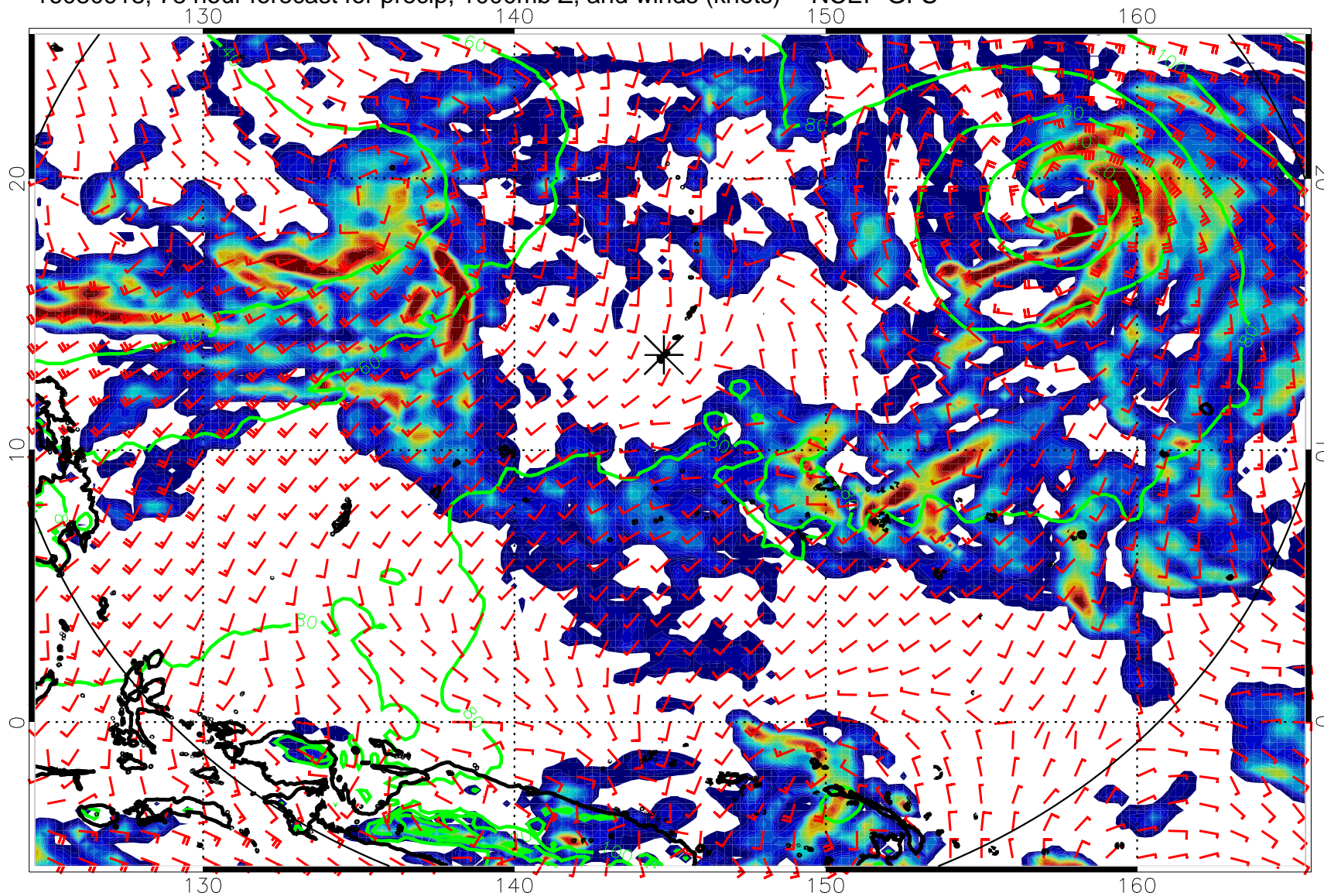
16080918, 78 hour forecast for precip, 1000mb Z, and winds (knots) -- NCEP GFS
