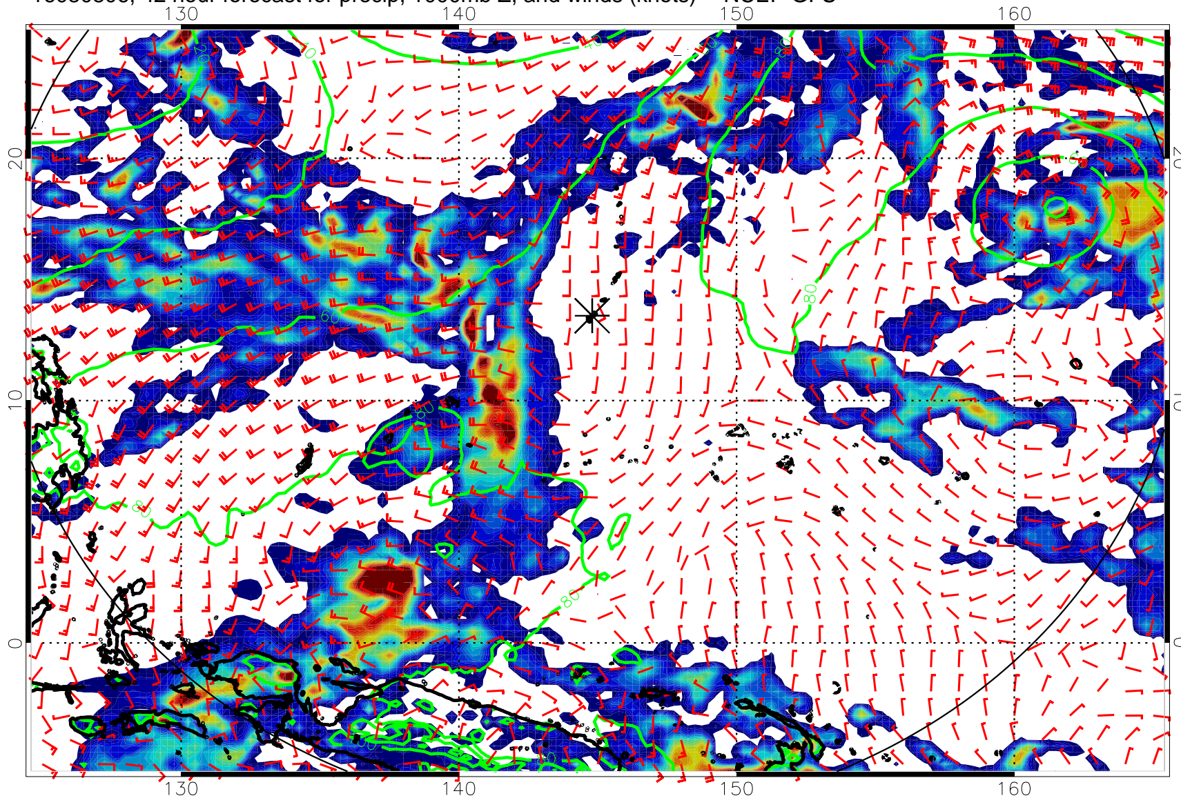
16080806, 42 hour forecast for precip, 1000mb Z, and winds (knots) -- NCEP GFS
