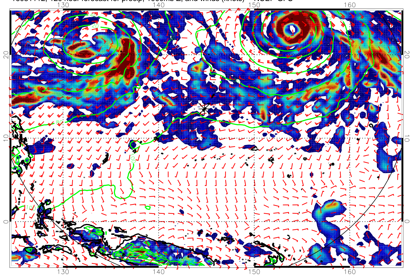
16081112, 120 hour forecast for precip, 1000mb Z, and winds (knots) -- NCEP GFS
