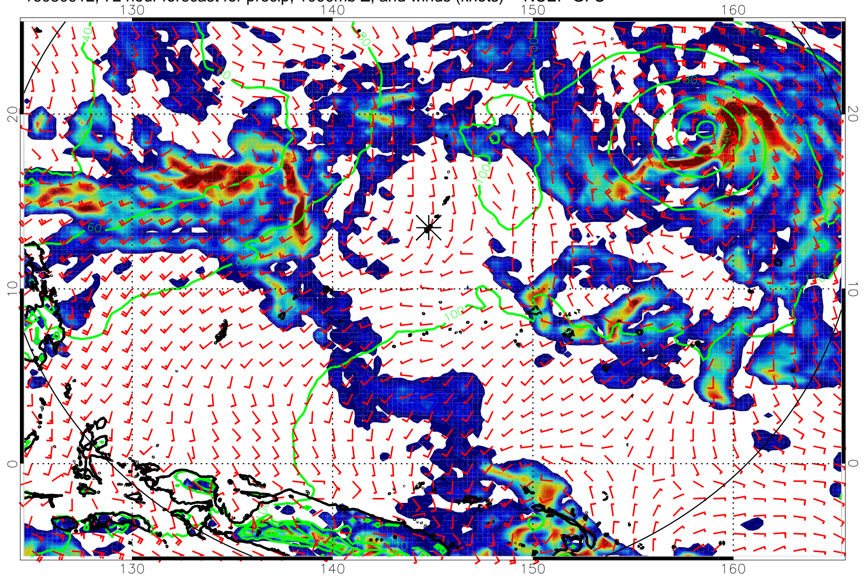
16080912, 72 hour forecast for precip, 1000mb Z, and winds (knots) -- NCEP GFS
