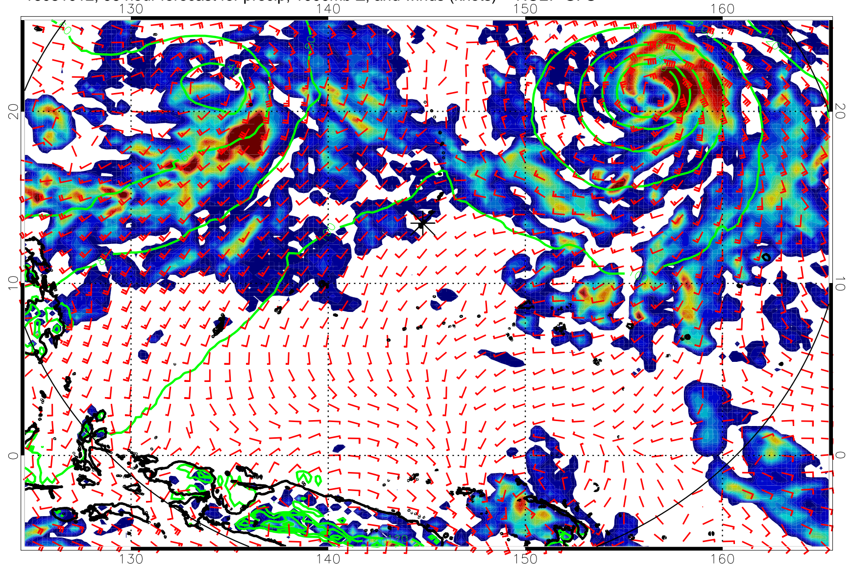
16081012, 96 hour forecast for precip, 1000mb Z, and winds (knots) -- NCEP GFS
