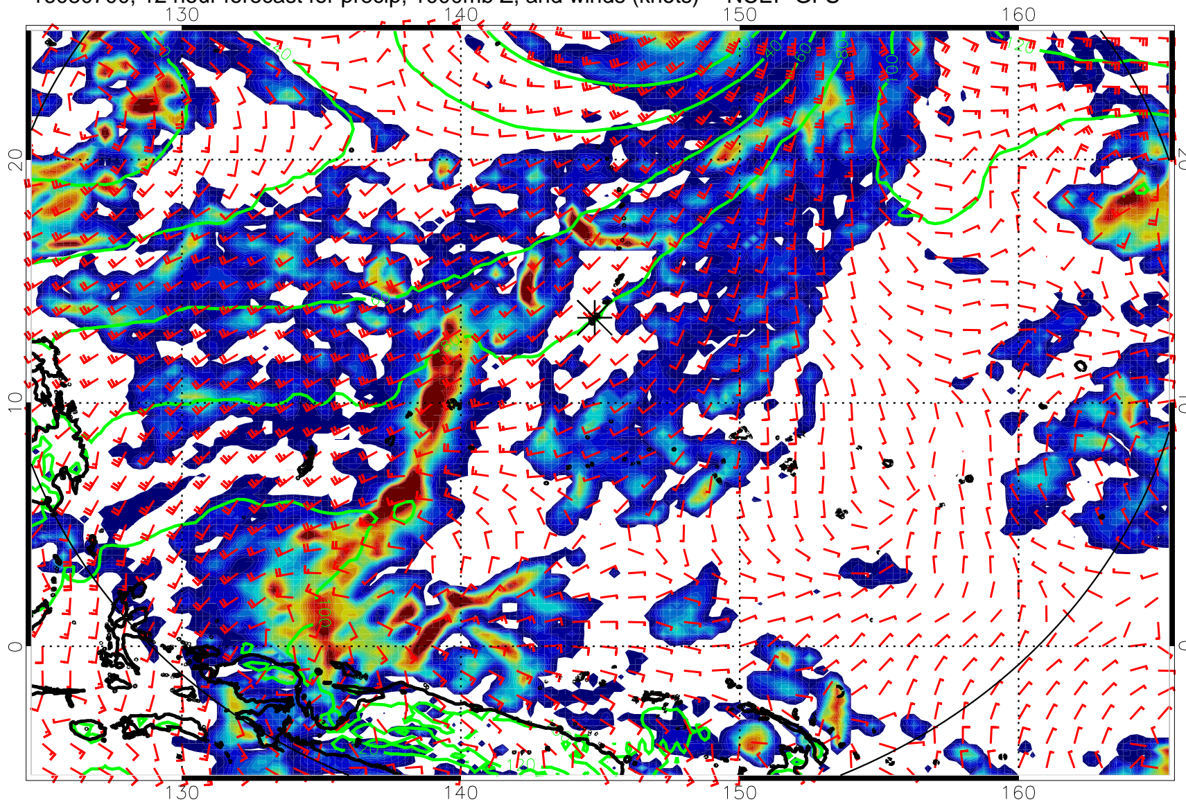
16080700, 12 hour forecast for precip, 1000mb Z, and winds (knots) -- NCEP GFS
