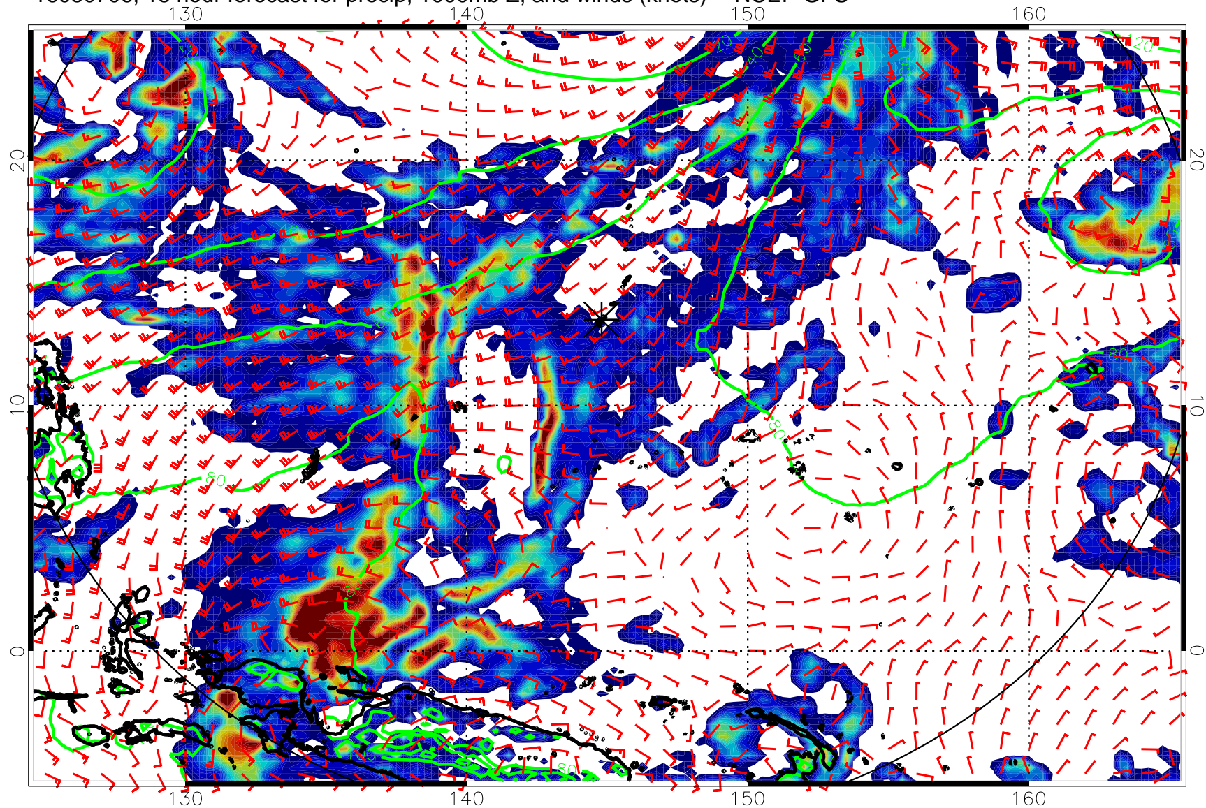
16080706, 18 hour forecast for precip, 1000mb Z, and winds (knots) -- NCEP GFS
