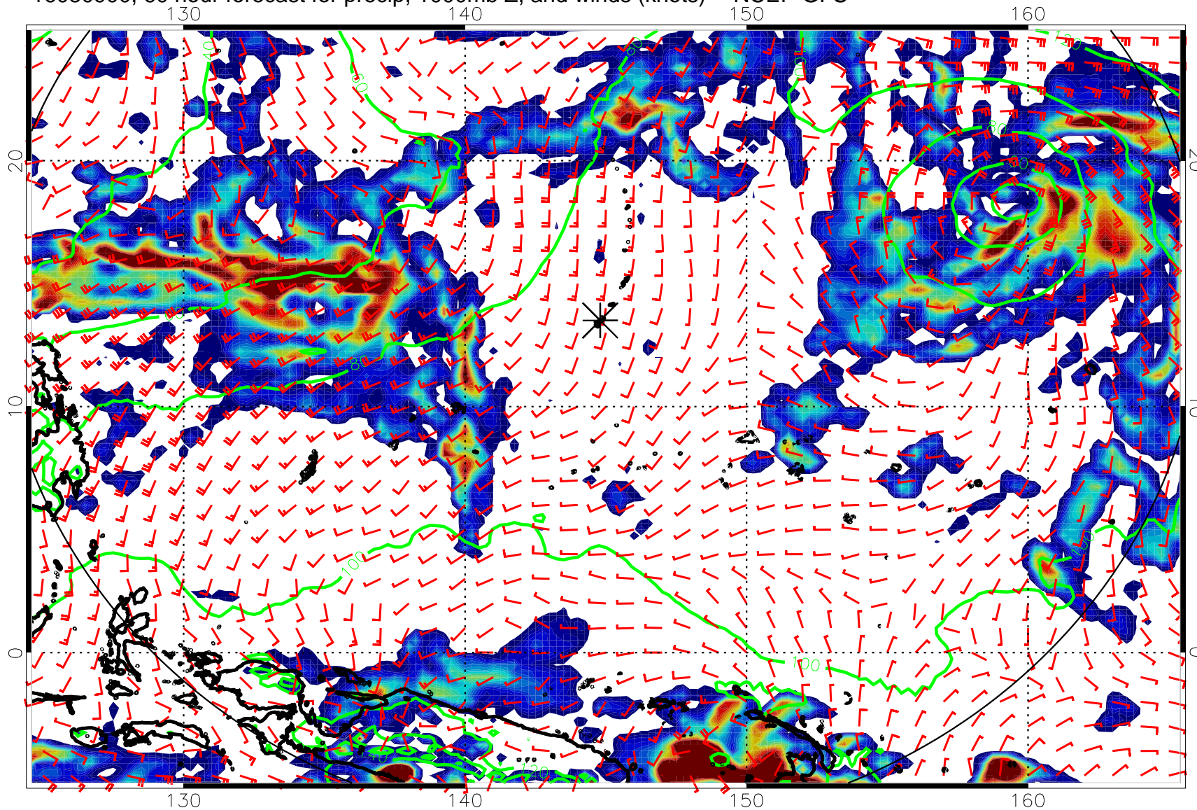
16080900, 60 hour forecast for precip, 1000mb Z, and winds (knots) -- NCEP GFS
