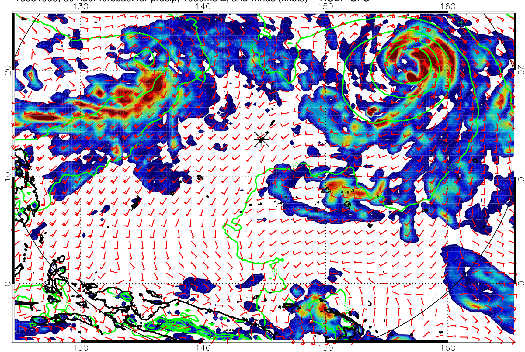
16081006, 90 hour forecast for precip, 1000mb Z, and winds (knots) -- NCEP GFS
