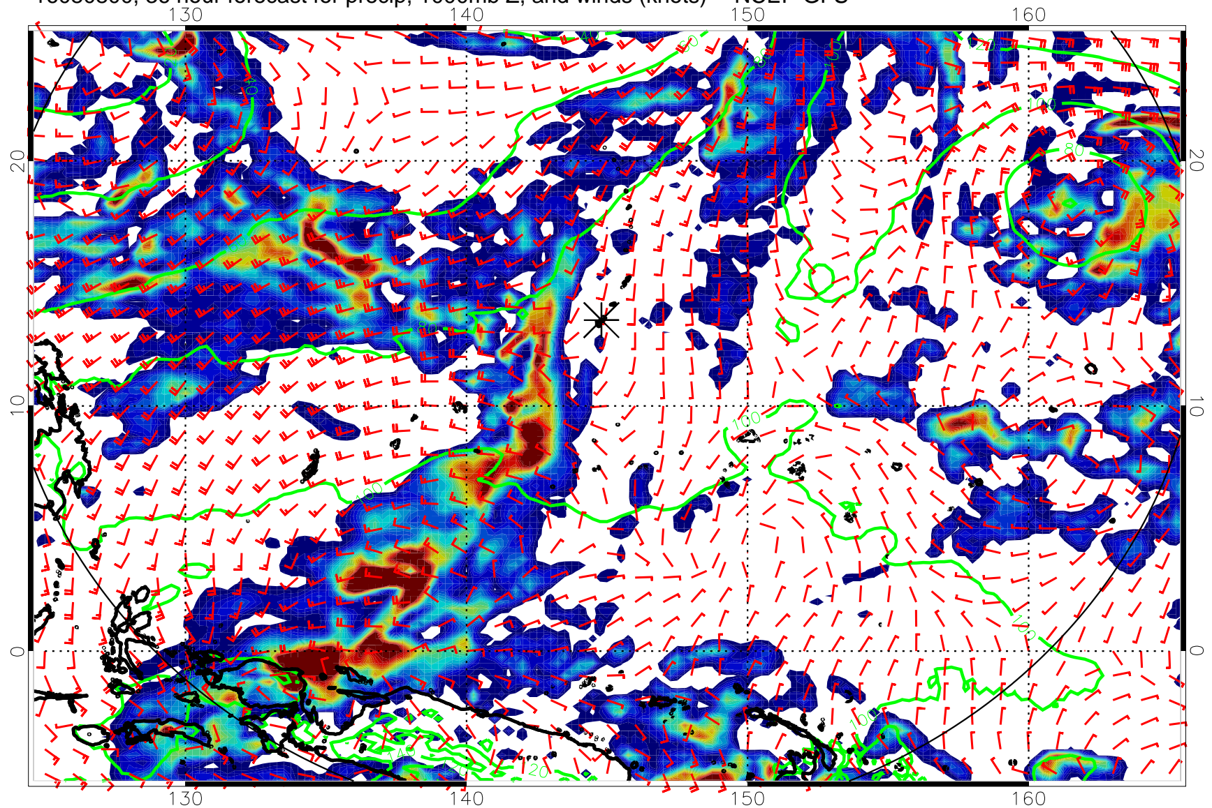
16080800, 36 hour forecast for precip, 1000mb Z, and winds (knots) -- NCEP GFS
