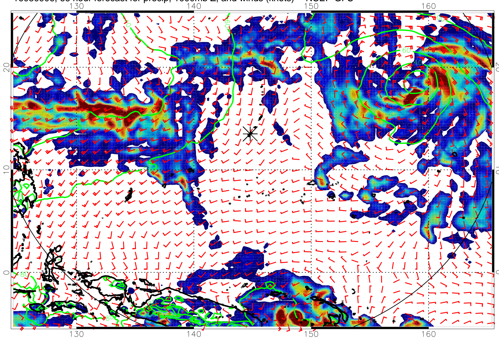
16080906, 66 hour forecast for precip, 1000mb Z, and winds (knots) -- NCEP GFS
