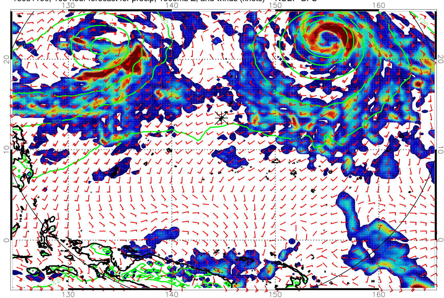
16081100, 108 hour forecast for precip, 1000mb Z, and winds (knots) -- NCEP GFS
