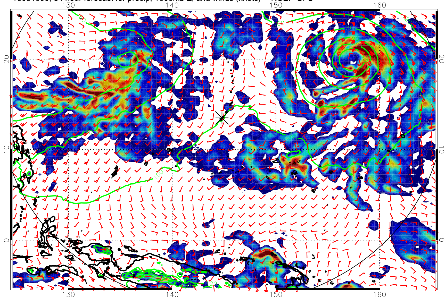
16081000, 84 hour forecast for precip, 1000mb Z, and winds (knots) -- NCEP GFS
