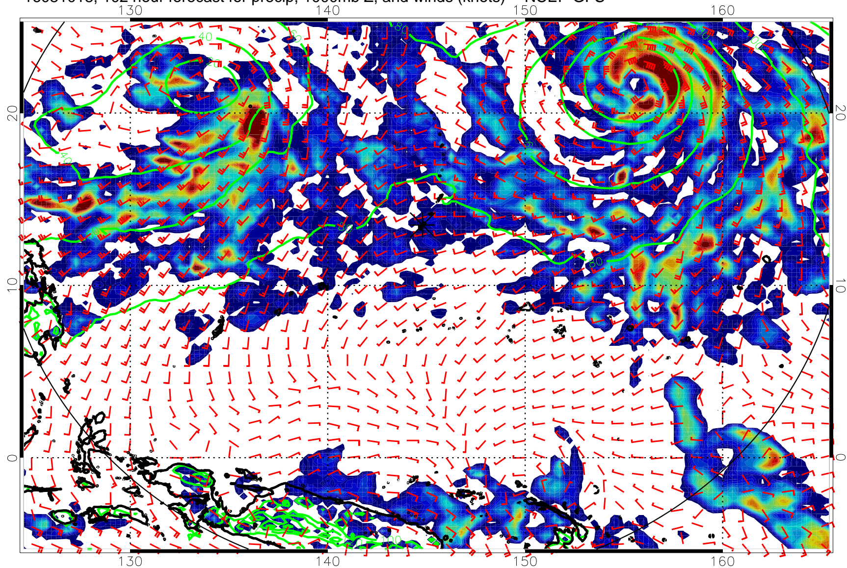
16081018, 102 hour forecast for precip, 1000mb Z, and winds (knots) -- NCEP GFS
