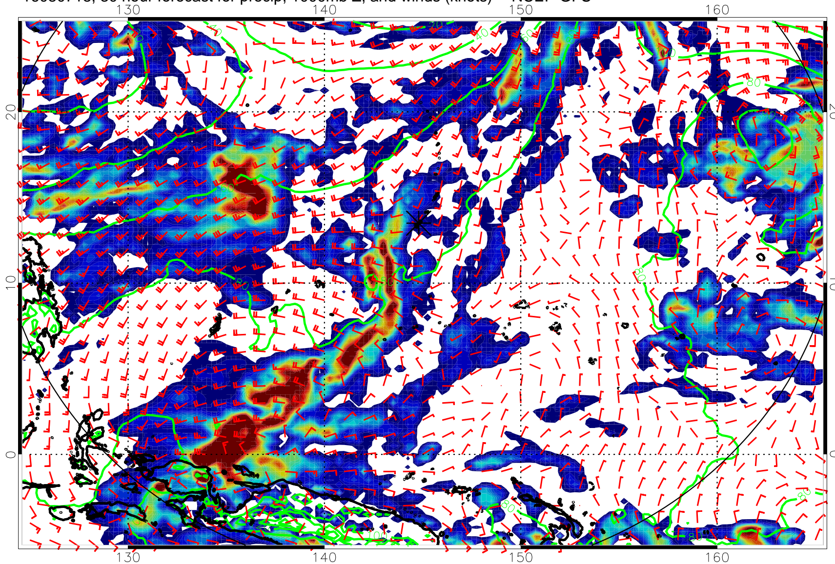
16080718, 30 hour forecast for precip, 1000mb Z, and winds (knots) -- NCEP GFS
