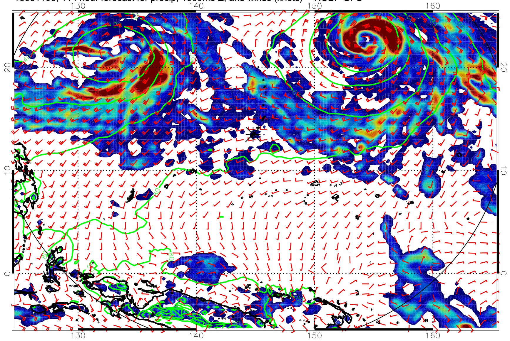
16081106, 114 hour forecast for precip, 1000mb Z, and winds (knots) -- NCEP GFS
