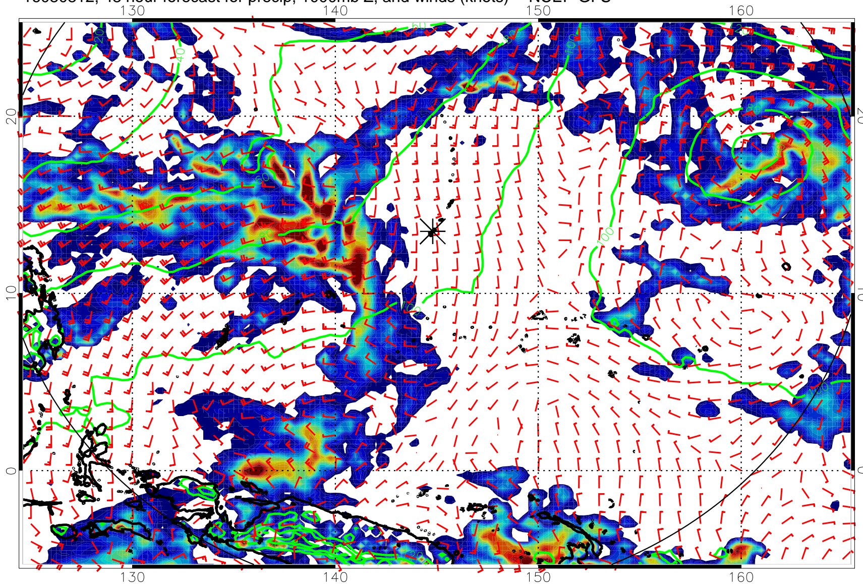
16080812, 48 hour forecast for precip, 1000mb Z, and winds (knots) -- NCEP GFS
