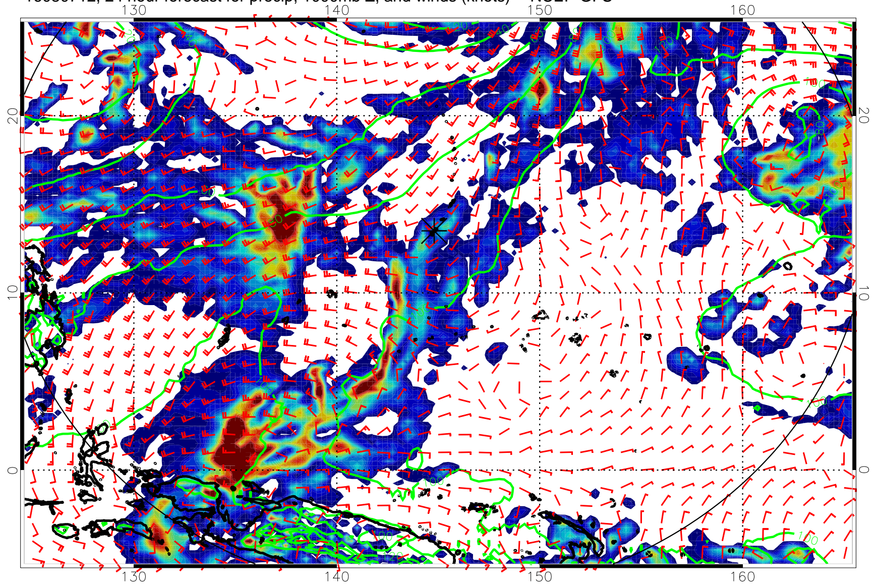
16080712, 24 hour forecast for precip, 1000mb Z, and winds (knots) -- NCEP GFS
