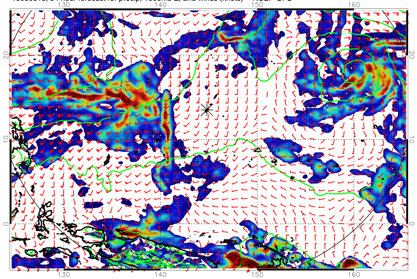
16080818, 54 hour forecast for precip, 1000mb Z, and winds (knots) -- NCEP GFS
