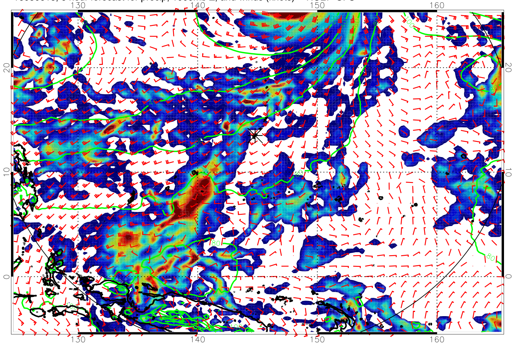
16080618, 6 hour forecast for precip, 1000mb Z, and winds (knots) -- NCEP GFS
