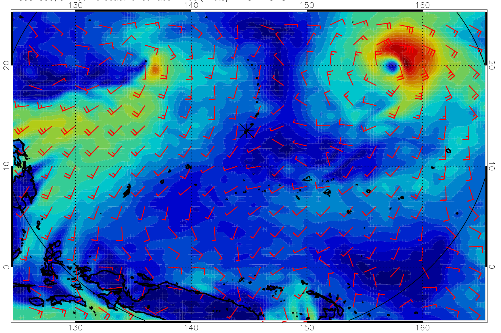
16081000, 84 hour forecast for surface winds (knots) -- NCEP GFS
