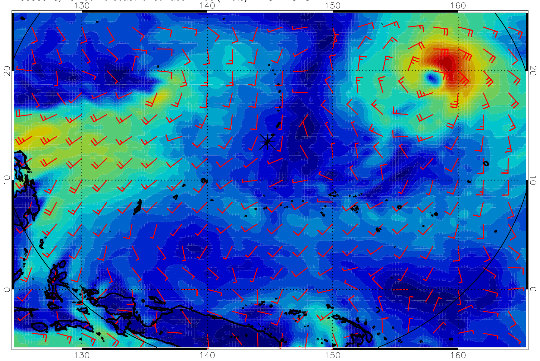
16080918, 78 hour forecast for surface winds (knots) -- NCEP GFS
