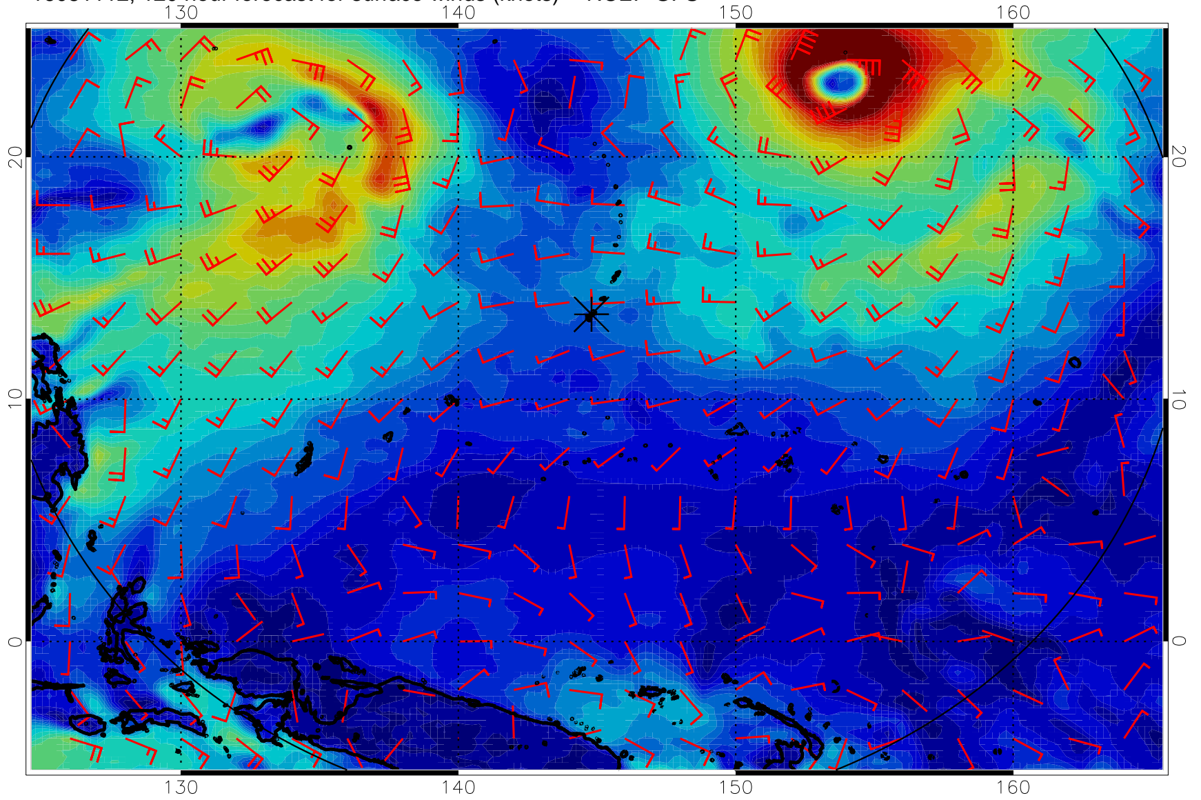
16081112, 120 hour forecast for surface winds (knots) -- NCEP GFS
