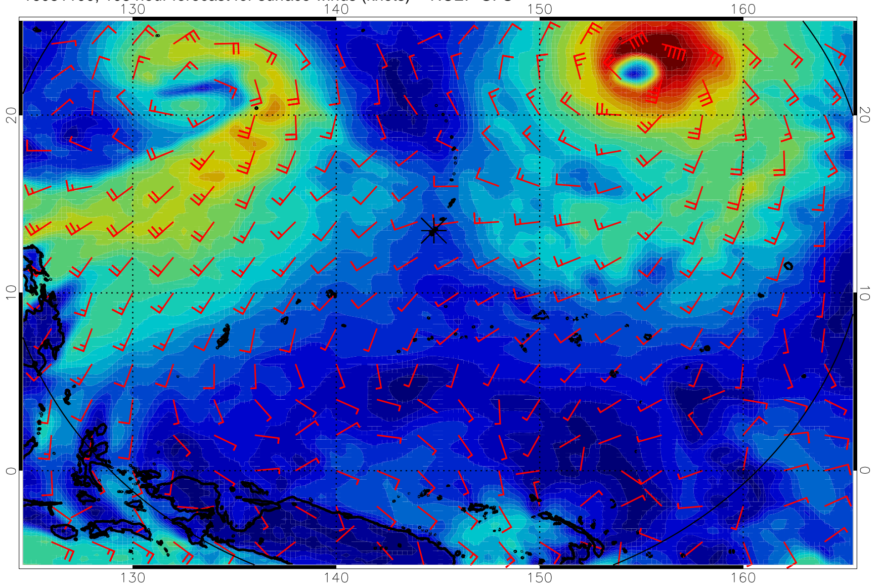
16081100, 108 hour forecast for surface winds (knots) -- NCEP GFS
