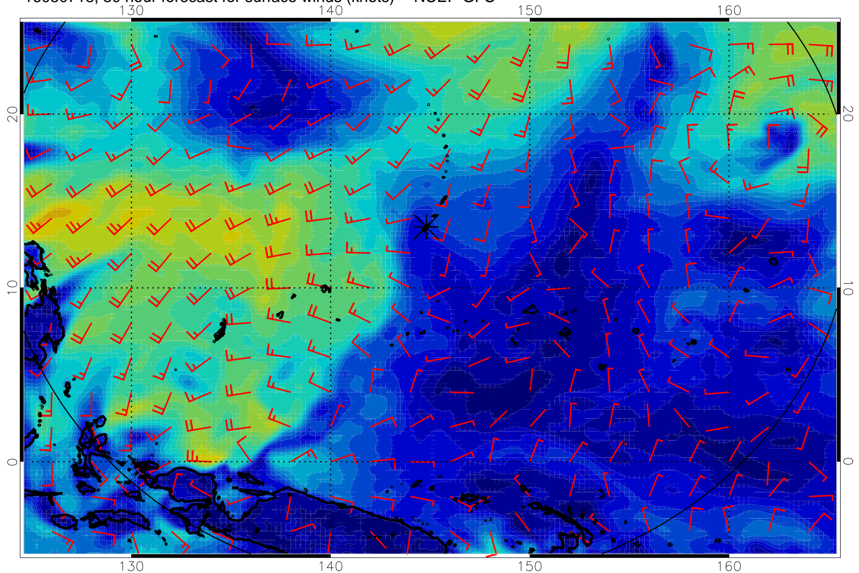
16080718, 30 hour forecast for surface winds (knots) -- NCEP GFS
