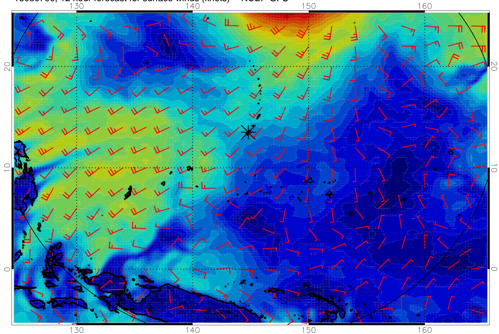
16080700, 12 hour forecast for surface winds (knots) -- NCEP GFS
