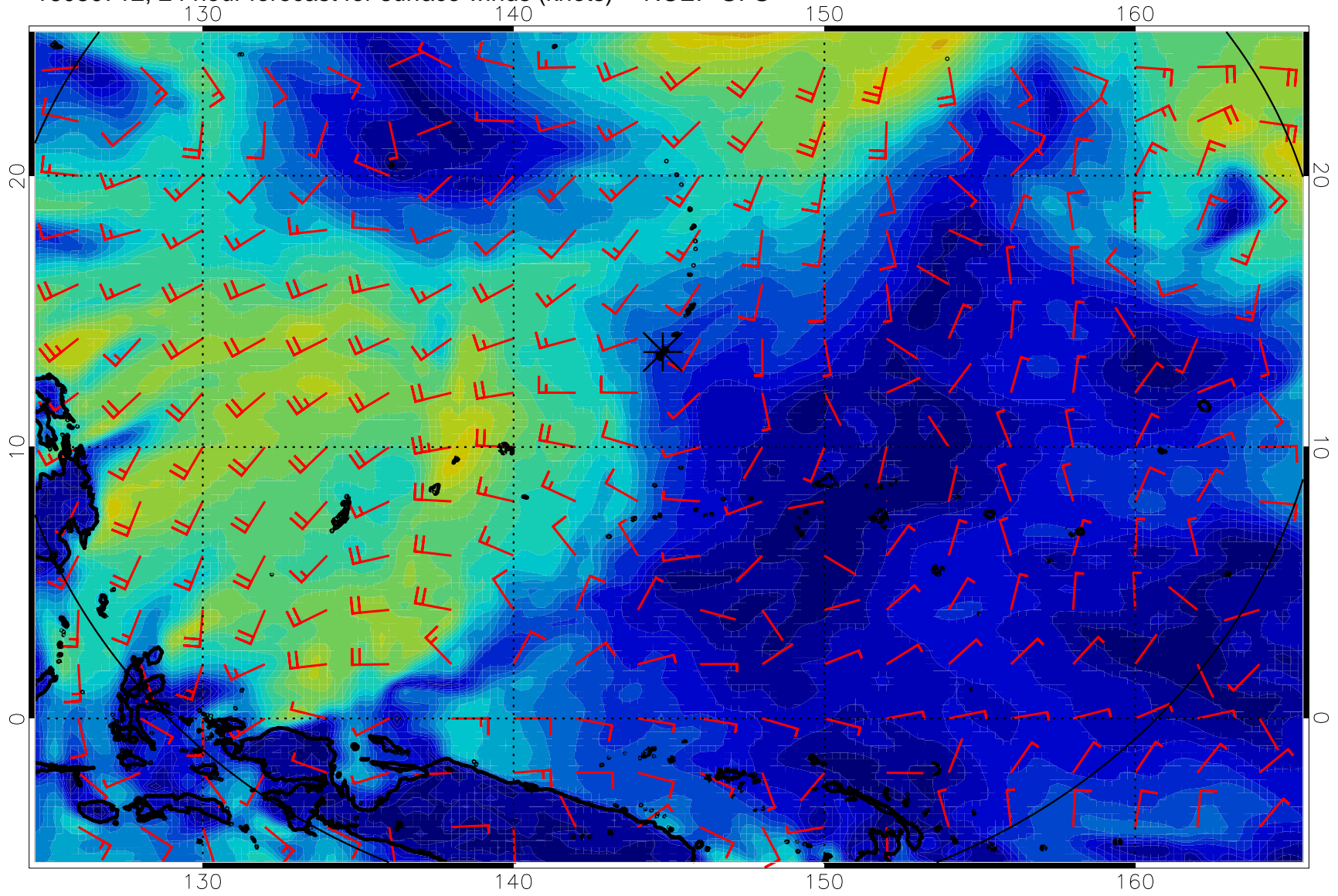
16080712, 24 hour forecast for surface winds (knots) -- NCEP GFS
