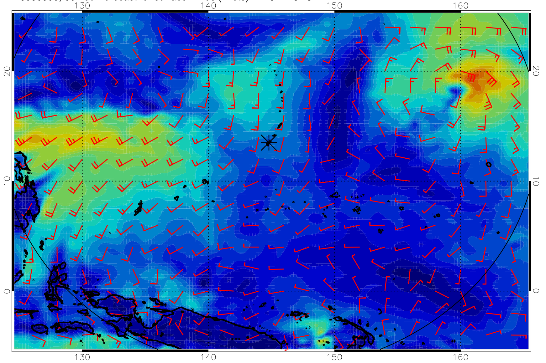
16080900, 60 hour forecast for surface winds (knots) -- NCEP GFS
