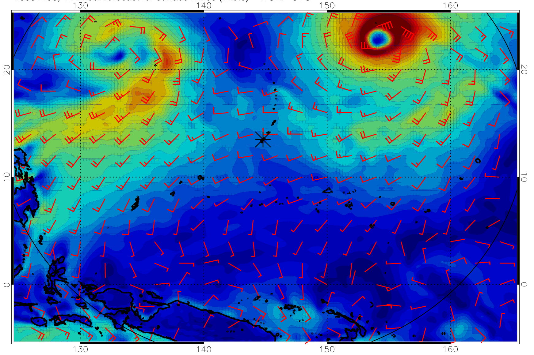
16081106, 114 hour forecast for surface winds (knots) -- NCEP GFS
