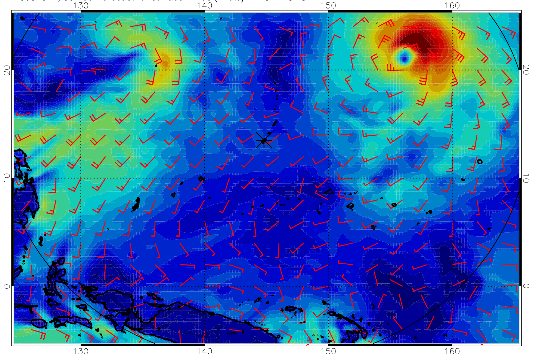
16081012, 96 hour forecast for surface winds (knots) -- NCEP GFS
