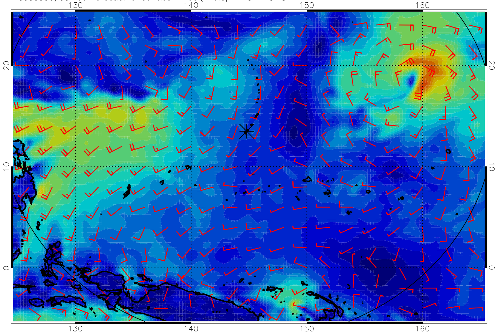
16080906, 66 hour forecast for surface winds (knots) -- NCEP GFS
