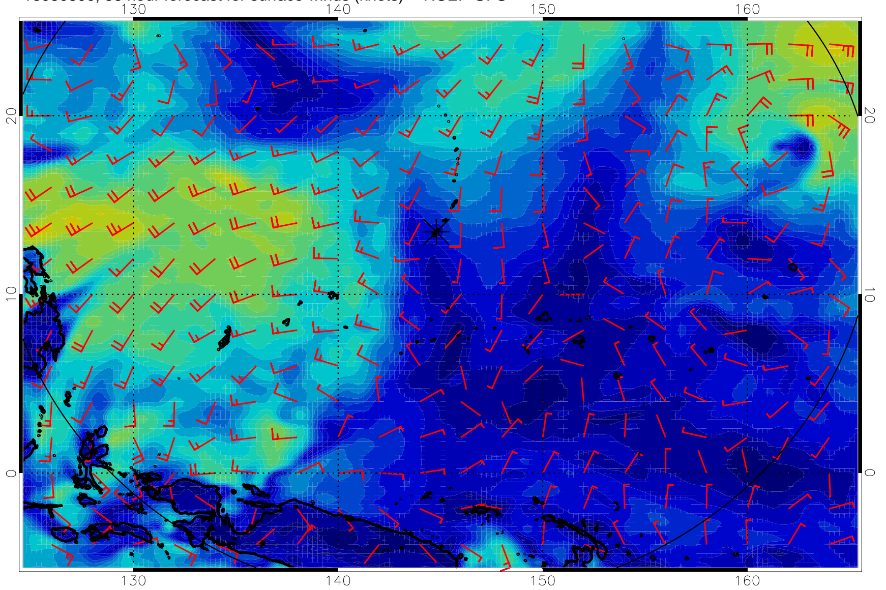
16080800, 36 hour forecast for surface winds (knots) -- NCEP GFS
