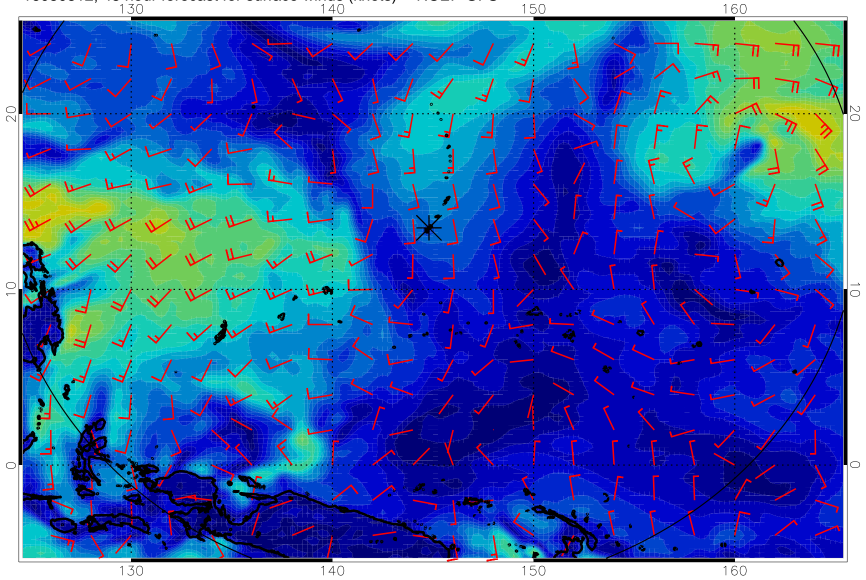
16080812, 48 hour forecast for surface winds (knots) -- NCEP GFS
