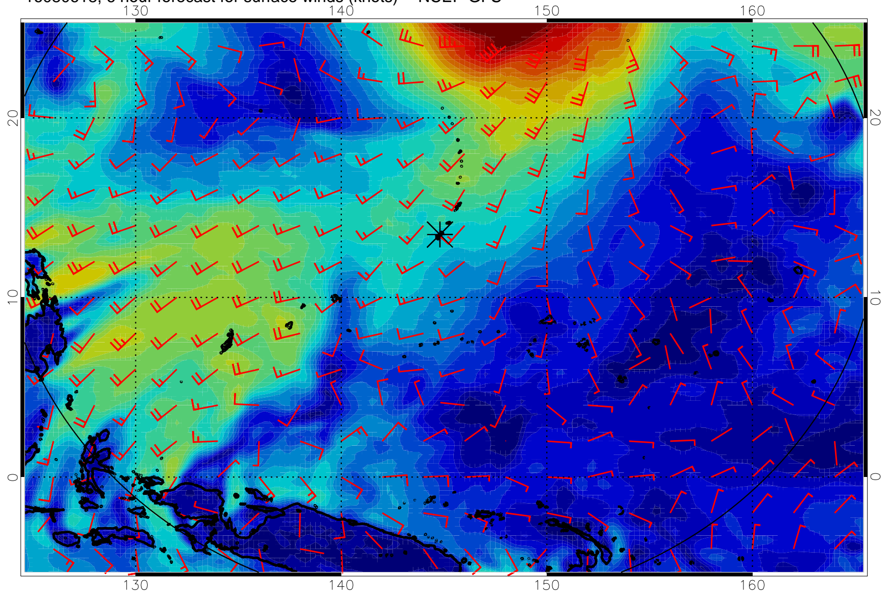
16080618, 6 hour forecast for surface winds (knots) -- NCEP GFS
