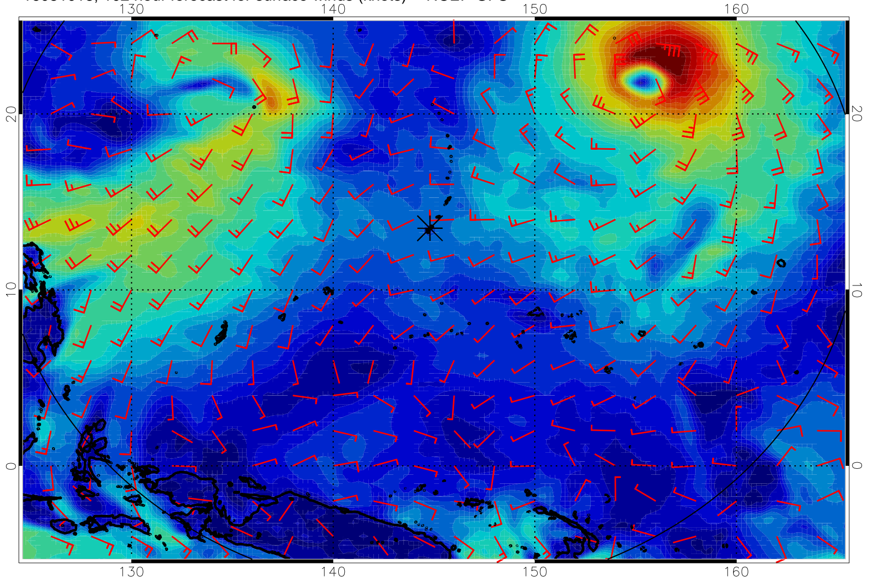
16081018, 102 hour forecast for surface winds (knots) -- NCEP GFS
