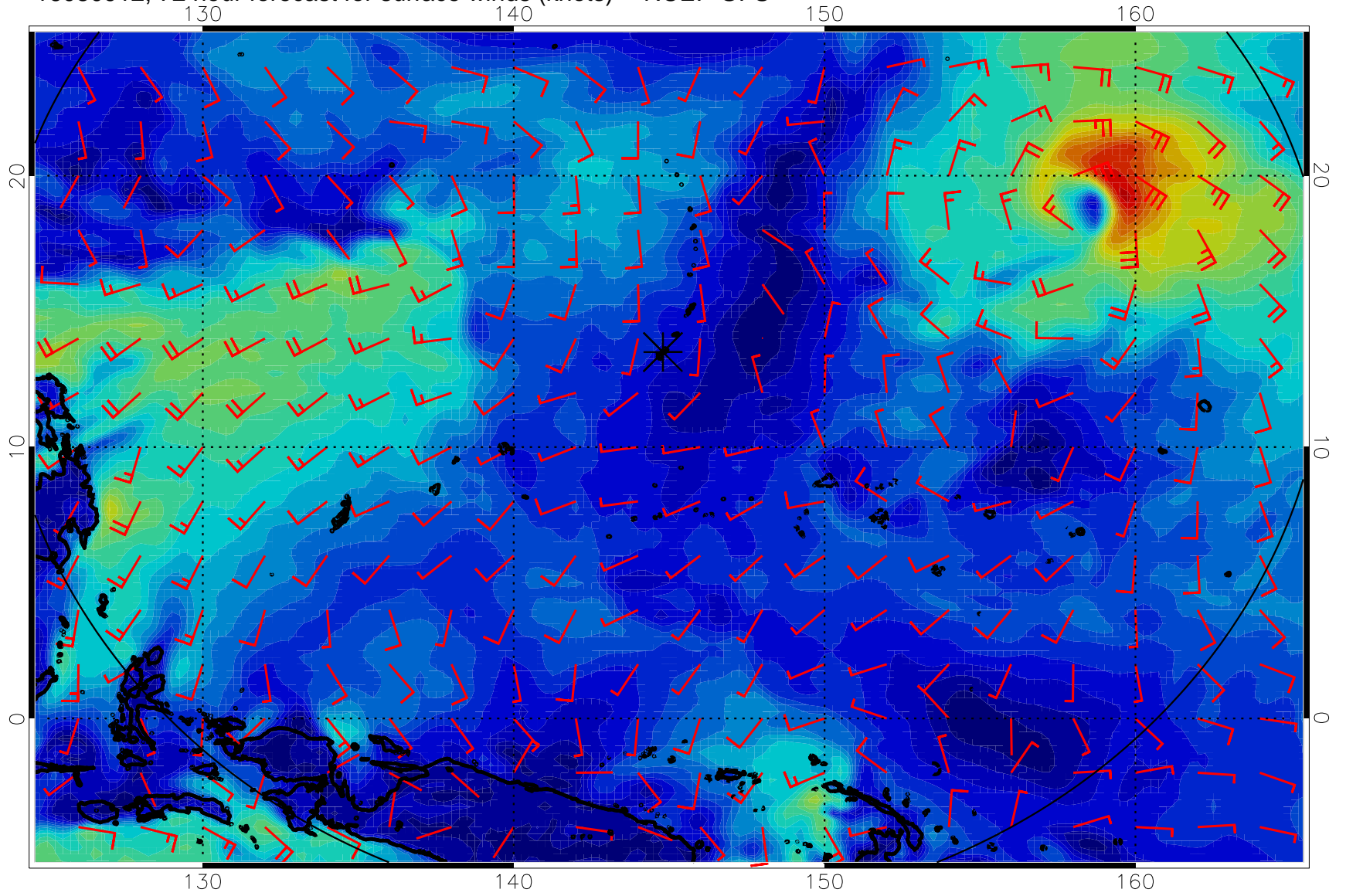
16080912, 72 hour forecast for surface winds (knots) -- NCEP GFS
