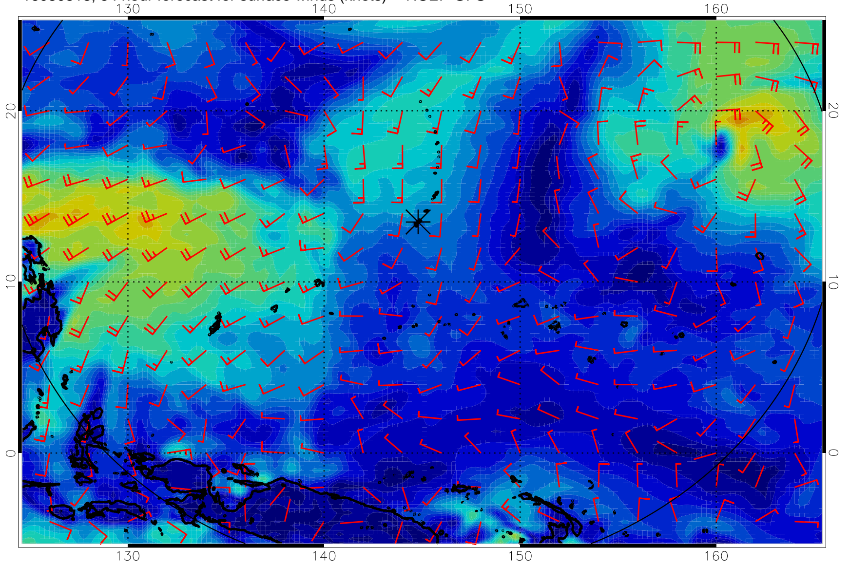
16080818, 54 hour forecast for surface winds (knots) -- NCEP GFS
