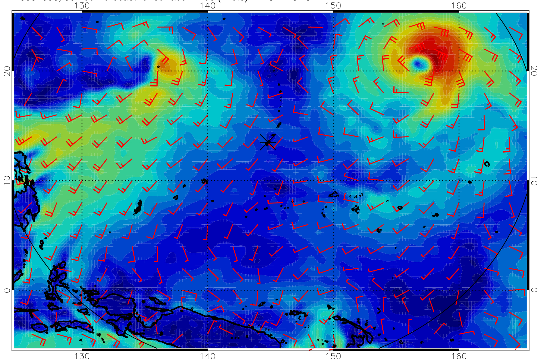
16081006, 90 hour forecast for surface winds (knots) -- NCEP GFS
