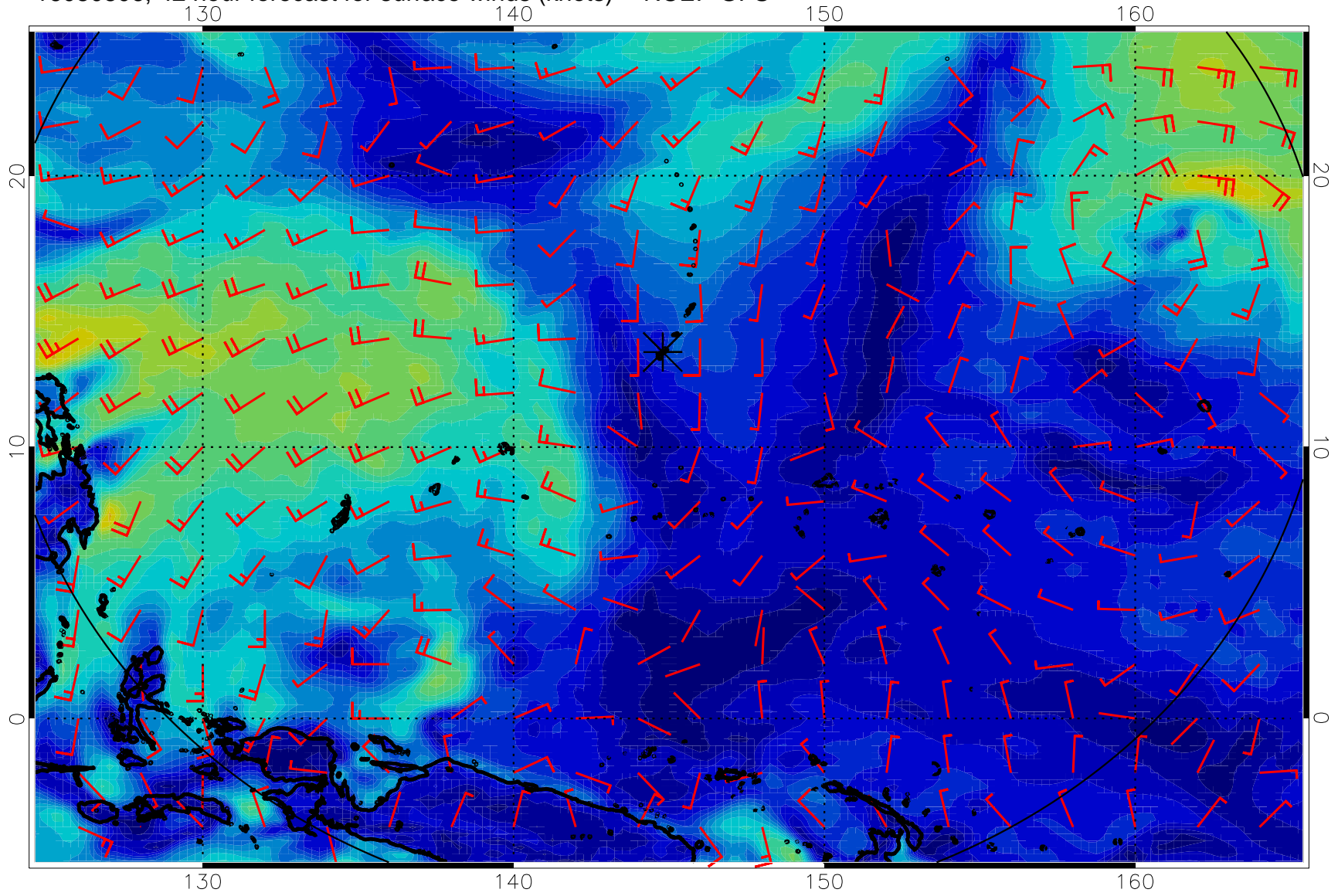
16080806, 42 hour forecast for surface winds (knots) -- NCEP GFS
