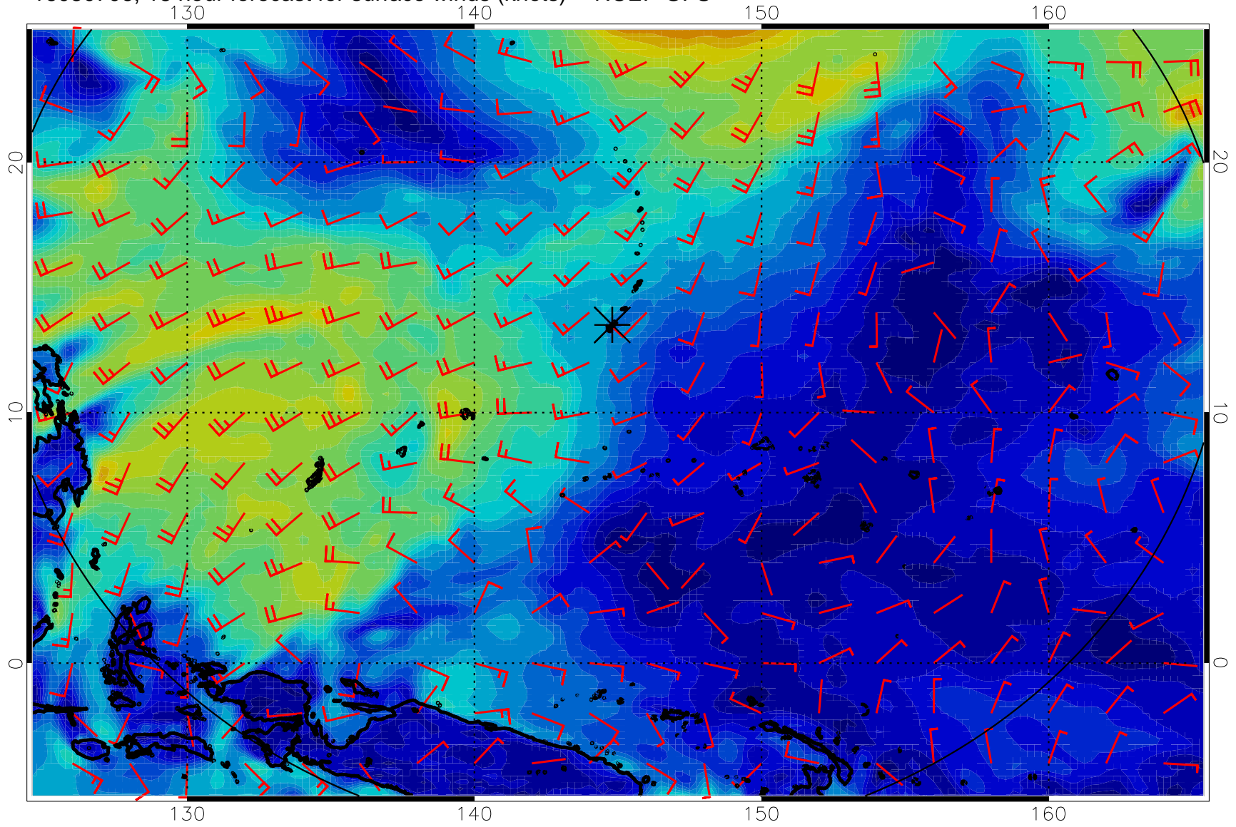
16080706, 18 hour forecast for surface winds (knots) -- NCEP GFS
