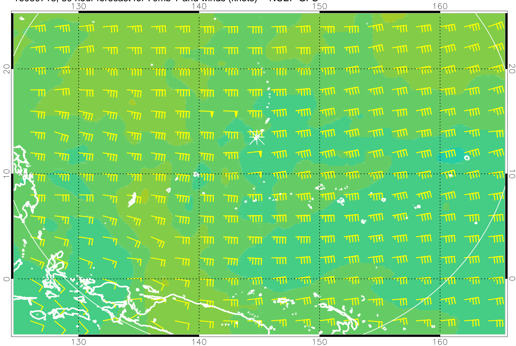
16080718, 30 hour forecast for 70mb T and winds (knots) -- NCEP GFS
