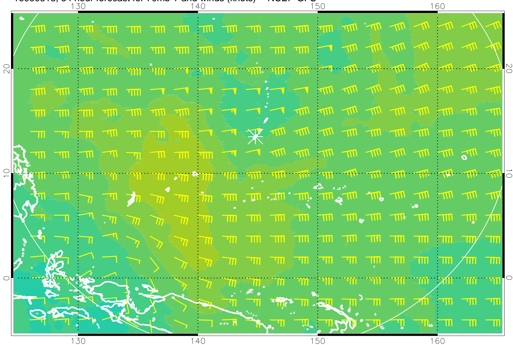
16080818, 54 hour forecast for 70mb T and winds (knots) -- NCEP GFS
