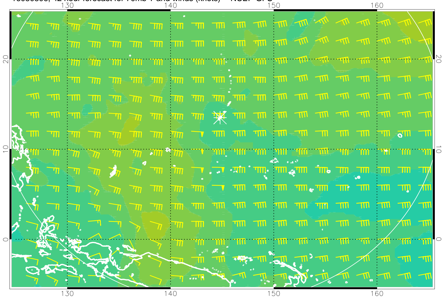
16080806, 42 hour forecast for 70mb T and winds (knots) -- NCEP GFS
