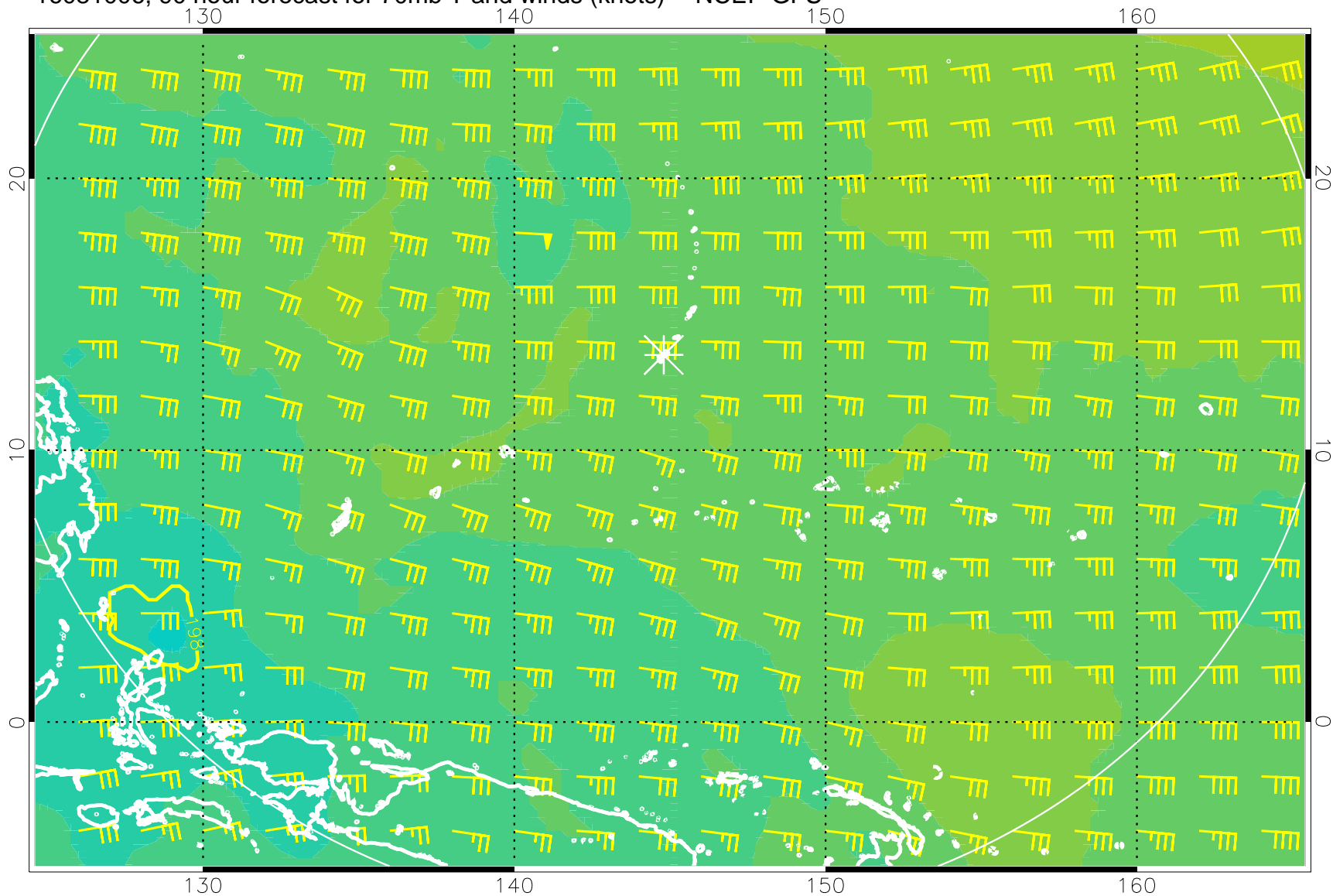
16081006, 90 hour forecast for 70mb T and winds (knots) -- NCEP GFS
