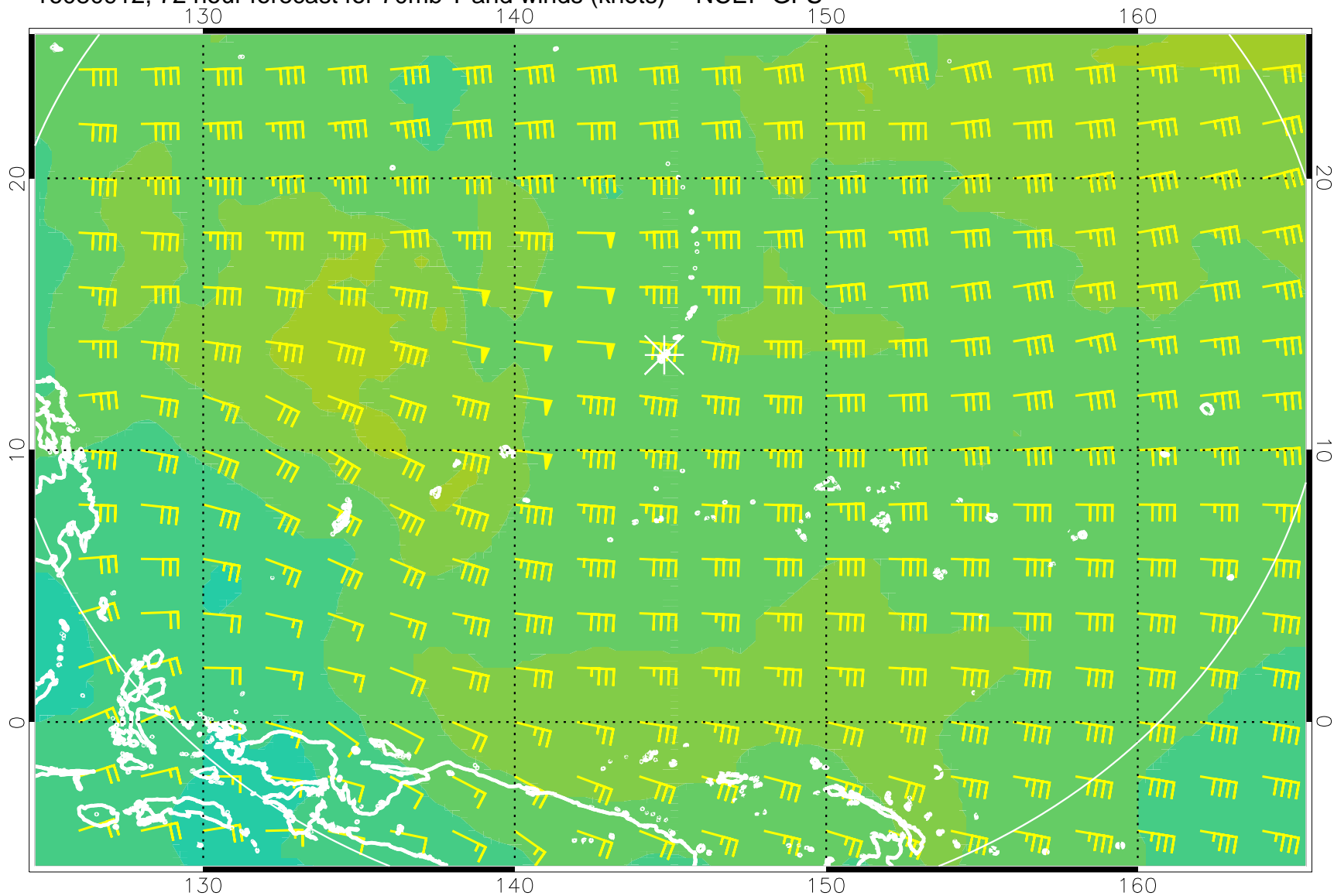
16080912, 72 hour forecast for 70mb T and winds (knots) -- NCEP GFS
