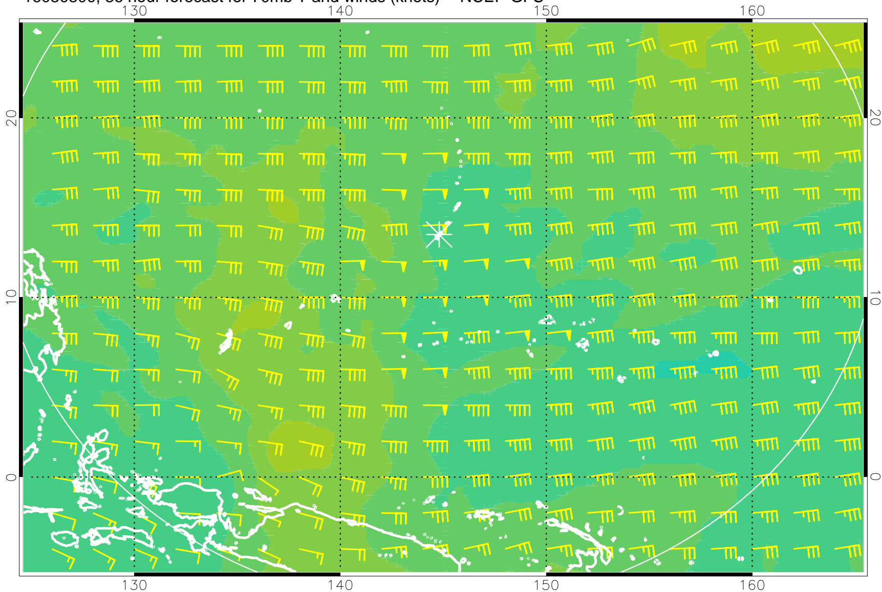
16080800, 36 hour forecast for 70mb T and winds (knots) -- NCEP GFS
