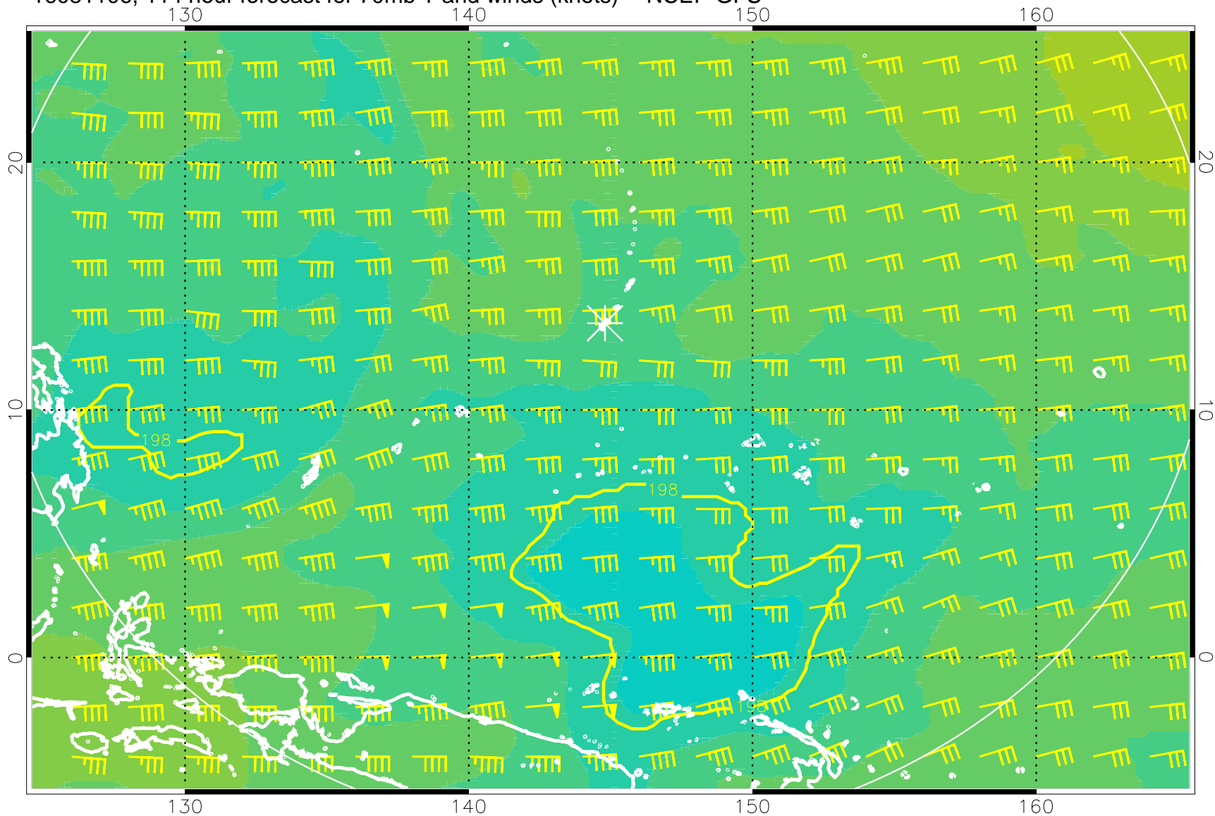
16081106, 114 hour forecast for 70mb T and winds (knots) -- NCEP GFS
