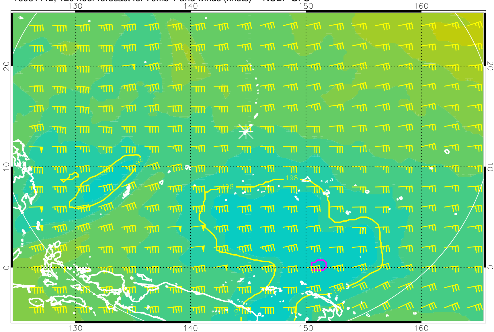
16081112, 120 hour forecast for 70mb T and winds (knots) -- NCEP GFS
