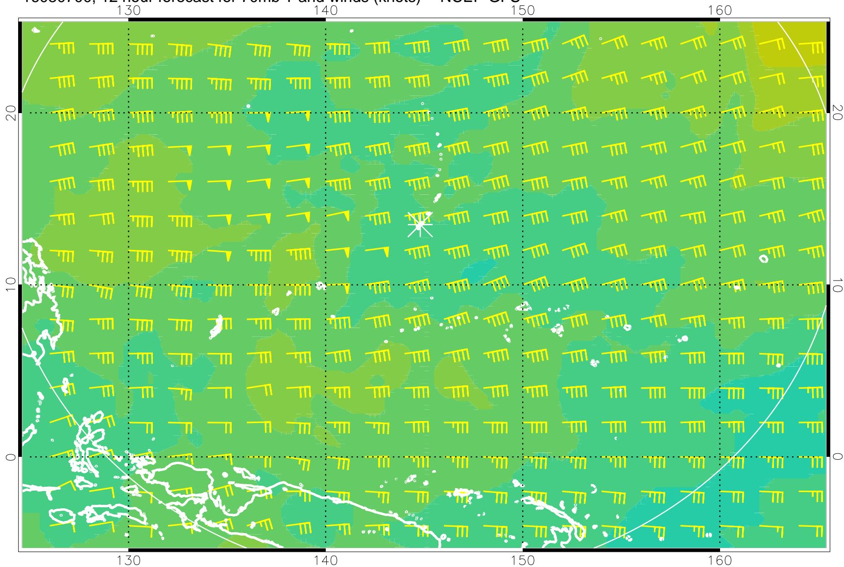
16080700, 12 hour forecast for 70mb T and winds (knots) -- NCEP GFS
