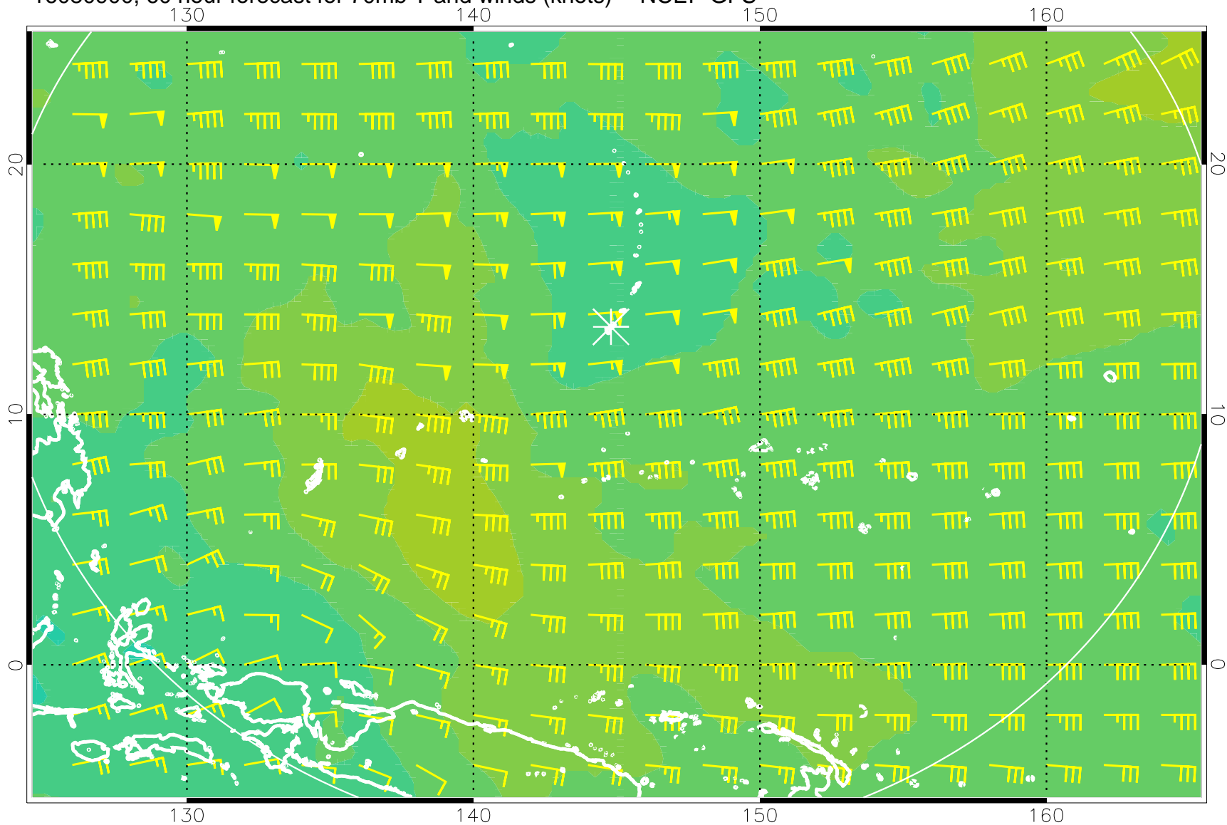
16080900, 60 hour forecast for 70mb T and winds (knots) -- NCEP GFS
