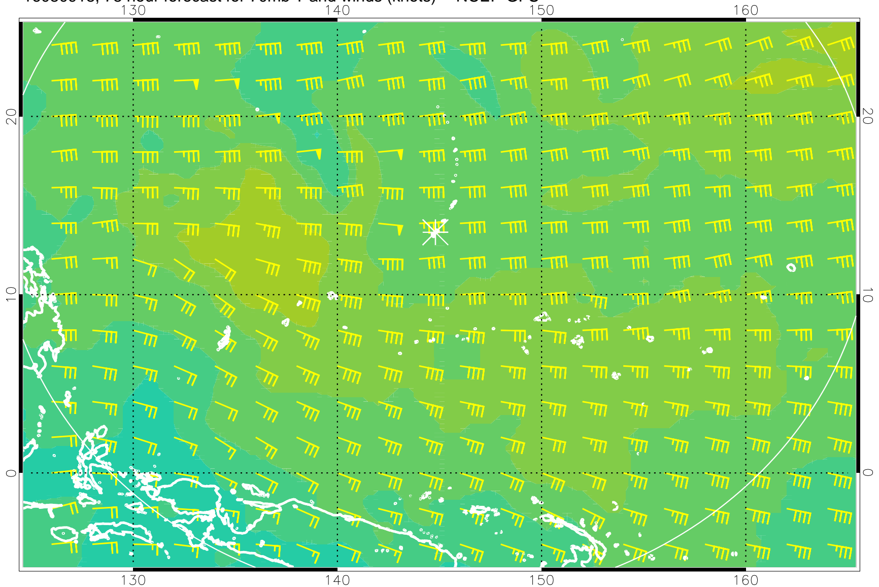
16080918, 78 hour forecast for 70mb T and winds (knots) -- NCEP GFS
