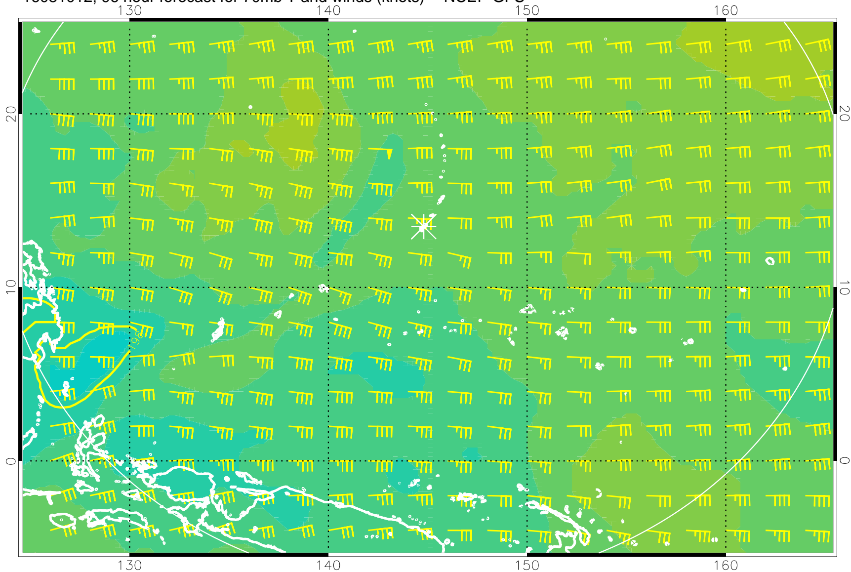
16081012, 96 hour forecast for 70mb T and winds (knots) -- NCEP GFS
