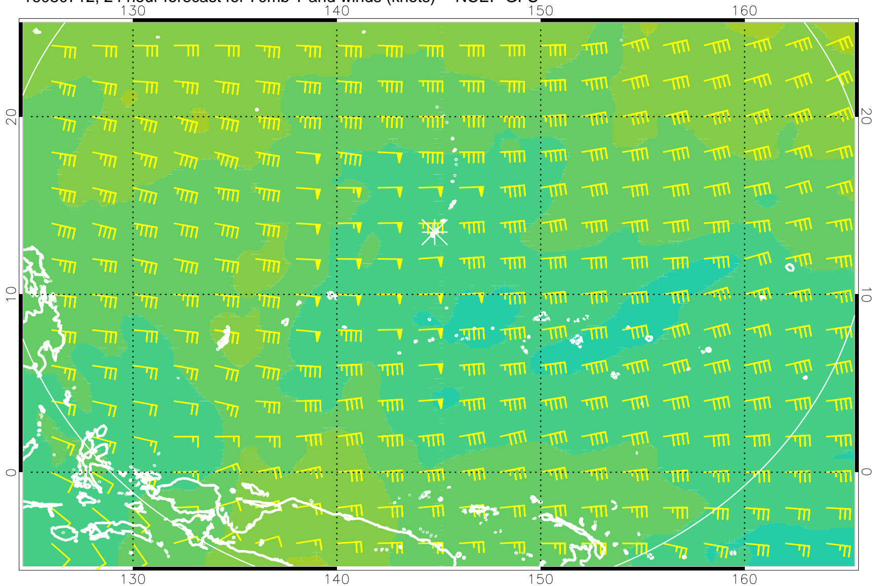
16080712, 24 hour forecast for 70mb T and winds (knots) -- NCEP GFS
