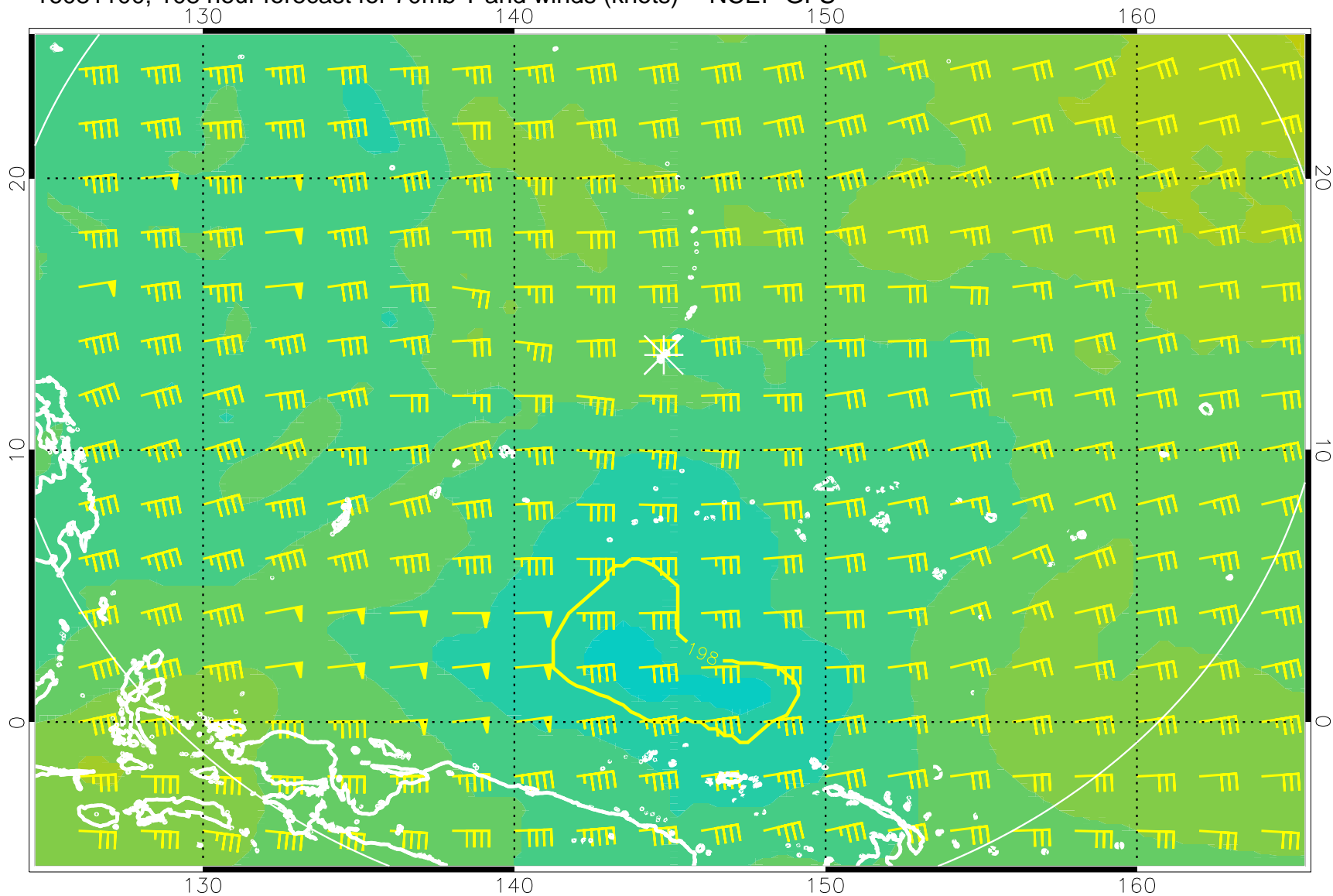
16081100, 108 hour forecast for 70mb T and winds (knots) -- NCEP GFS
