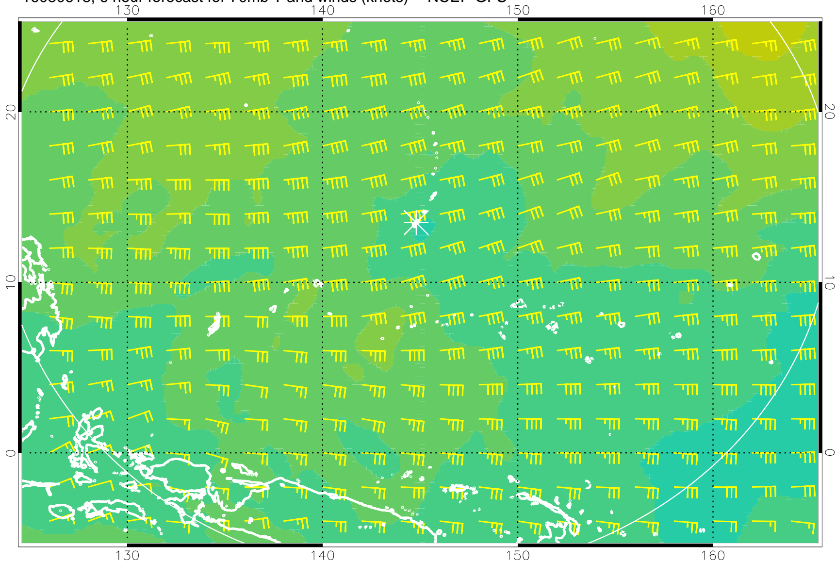
16080618, 6 hour forecast for 70mb T and winds (knots) -- NCEP GFS
