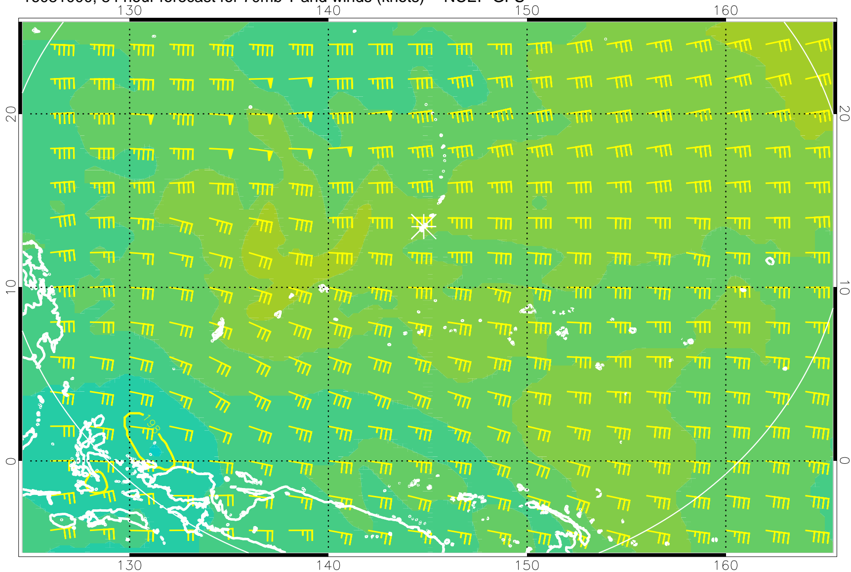
16081000, 84 hour forecast for 70mb T and winds (knots) -- NCEP GFS
