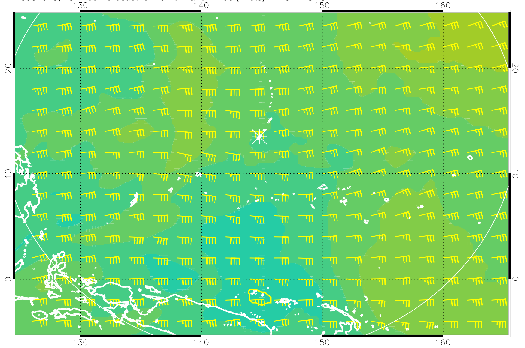
16081018, 102 hour forecast for 70mb T and winds (knots) -- NCEP GFS
