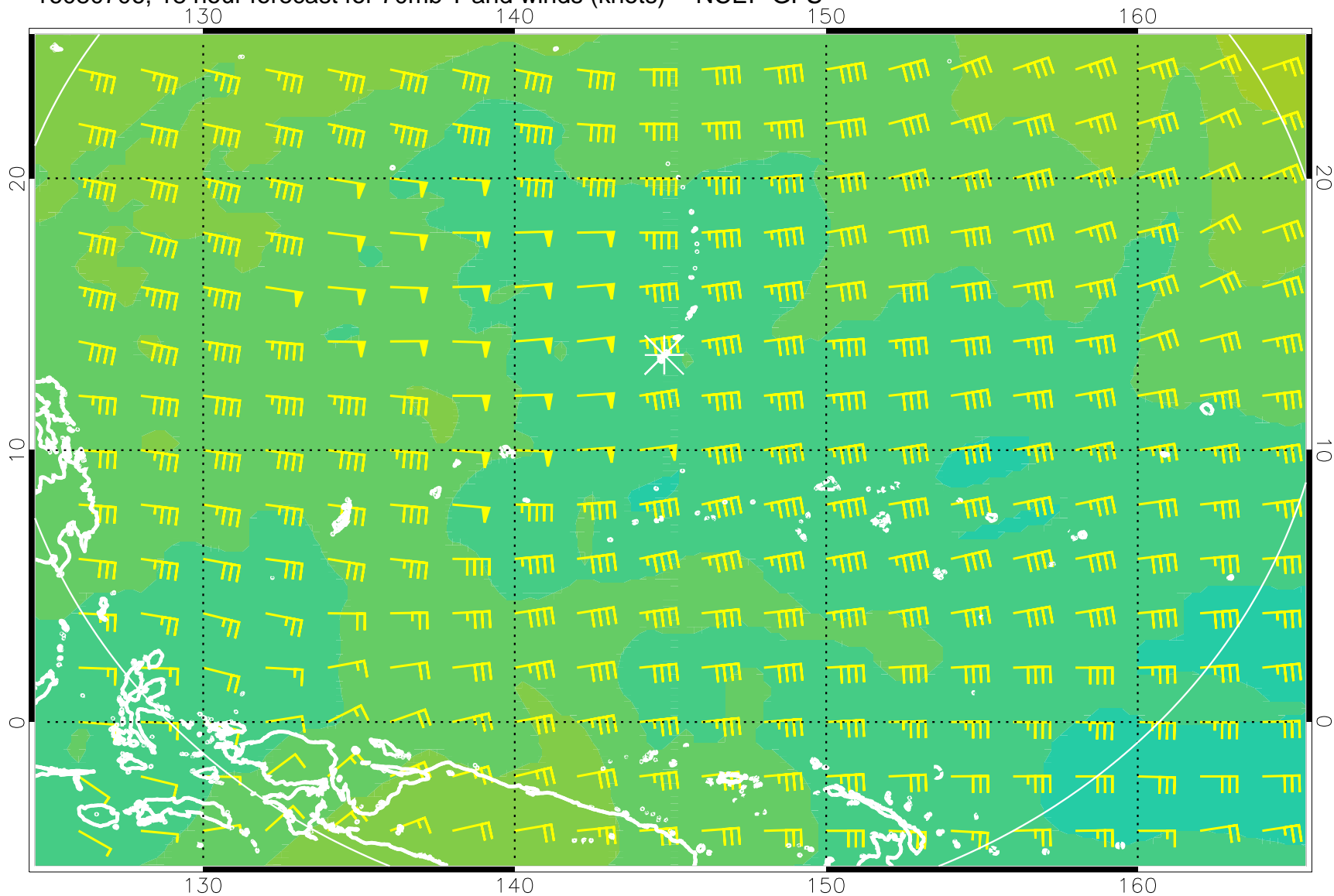
16080706, 18 hour forecast for 70mb T and winds (knots) -- NCEP GFS
