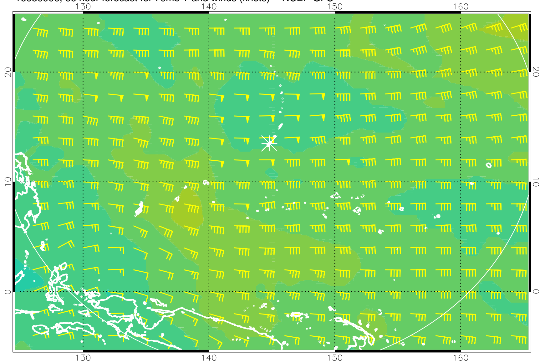
16080906, 66 hour forecast for 70mb T and winds (knots) -- NCEP GFS
