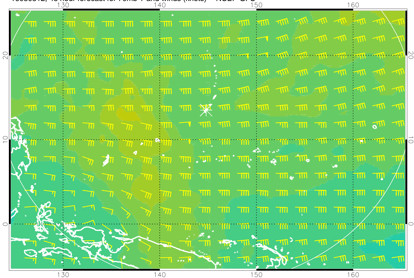
16080812, 48 hour forecast for 70mb T and winds (knots) -- NCEP GFS
