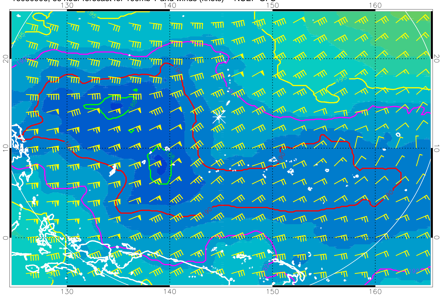
16080906, 66 hour forecast for 100mb T and winds (knots) -- NCEP GFS
