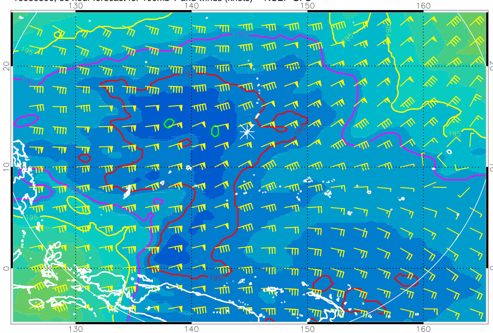
16080800, 36 hour forecast for 100mb T and winds (knots) -- NCEP GFS
