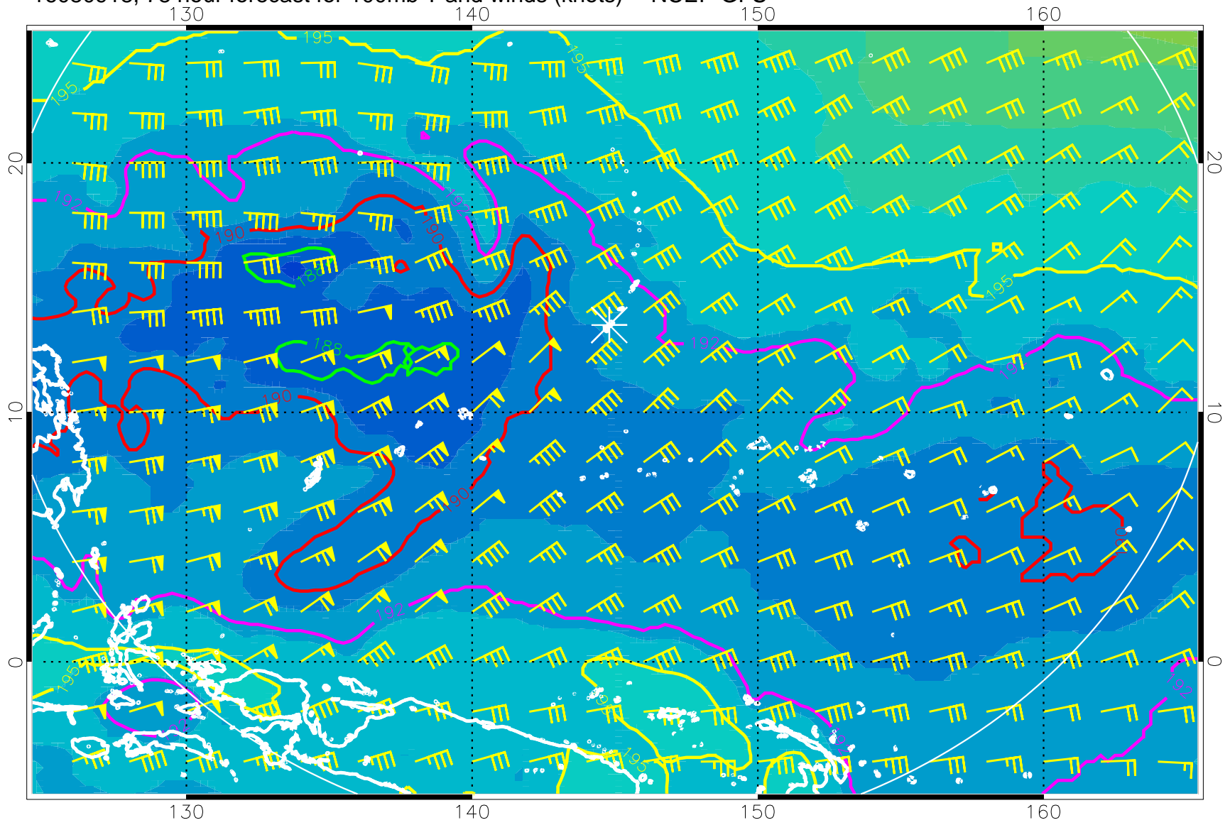
16080918, 78 hour forecast for 100mb T and winds (knots) -- NCEP GFS
