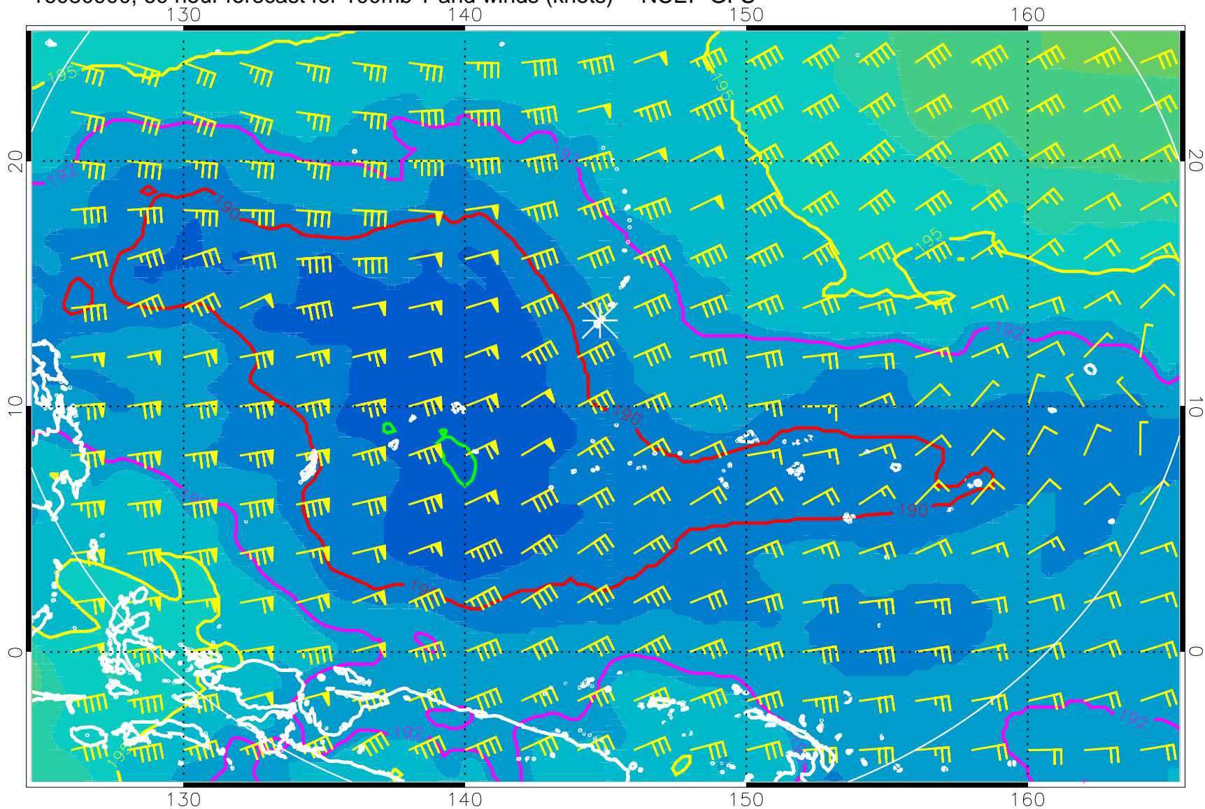
16080900, 60 hour forecast for 100mb T and winds (knots) -- NCEP GFS
