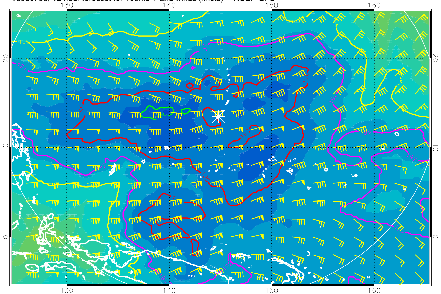
16080700, 12 hour forecast for 100mb T and winds (knots) -- NCEP GFS
