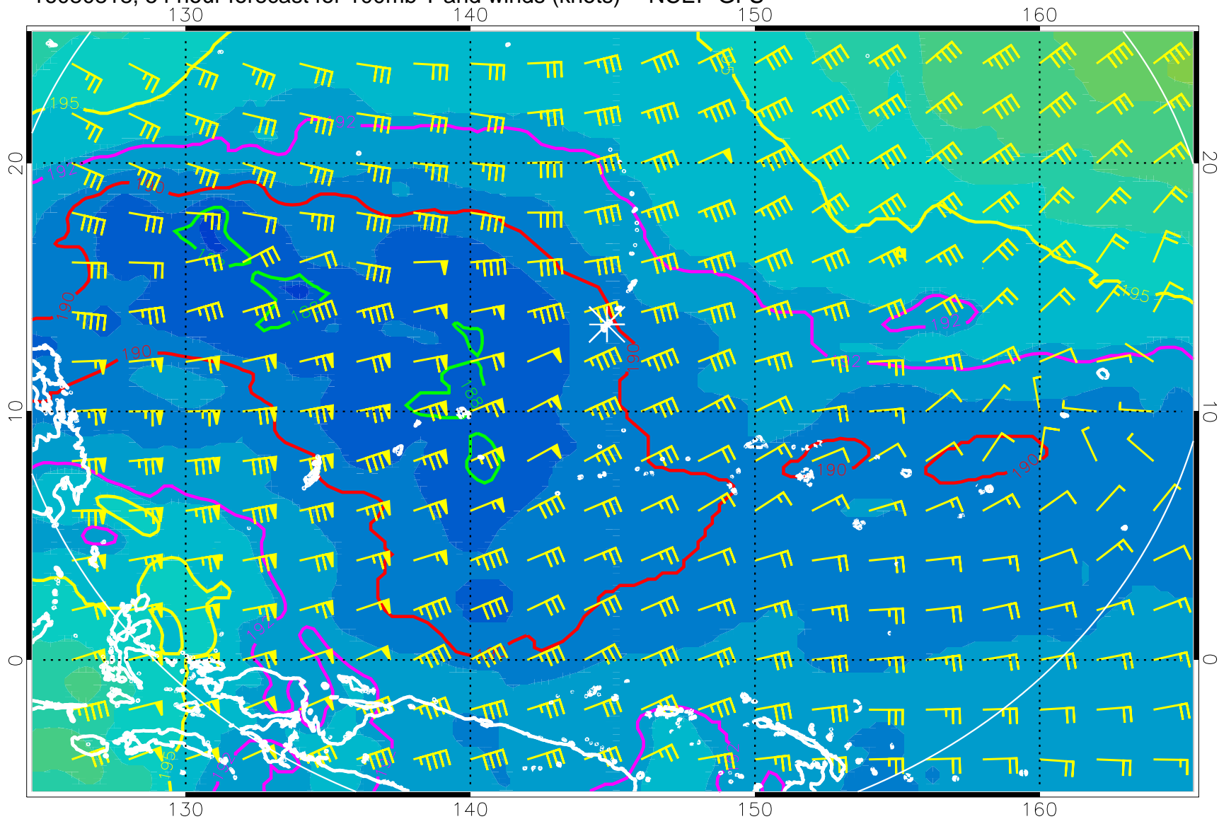
16080818, 54 hour forecast for 100mb T and winds (knots) -- NCEP GFS
