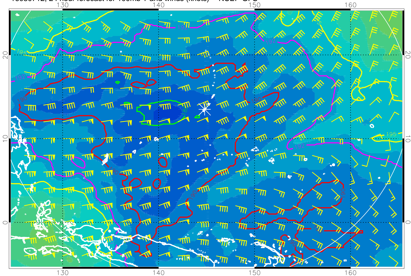
16080712, 24 hour forecast for 100mb T and winds (knots) -- NCEP GFS
