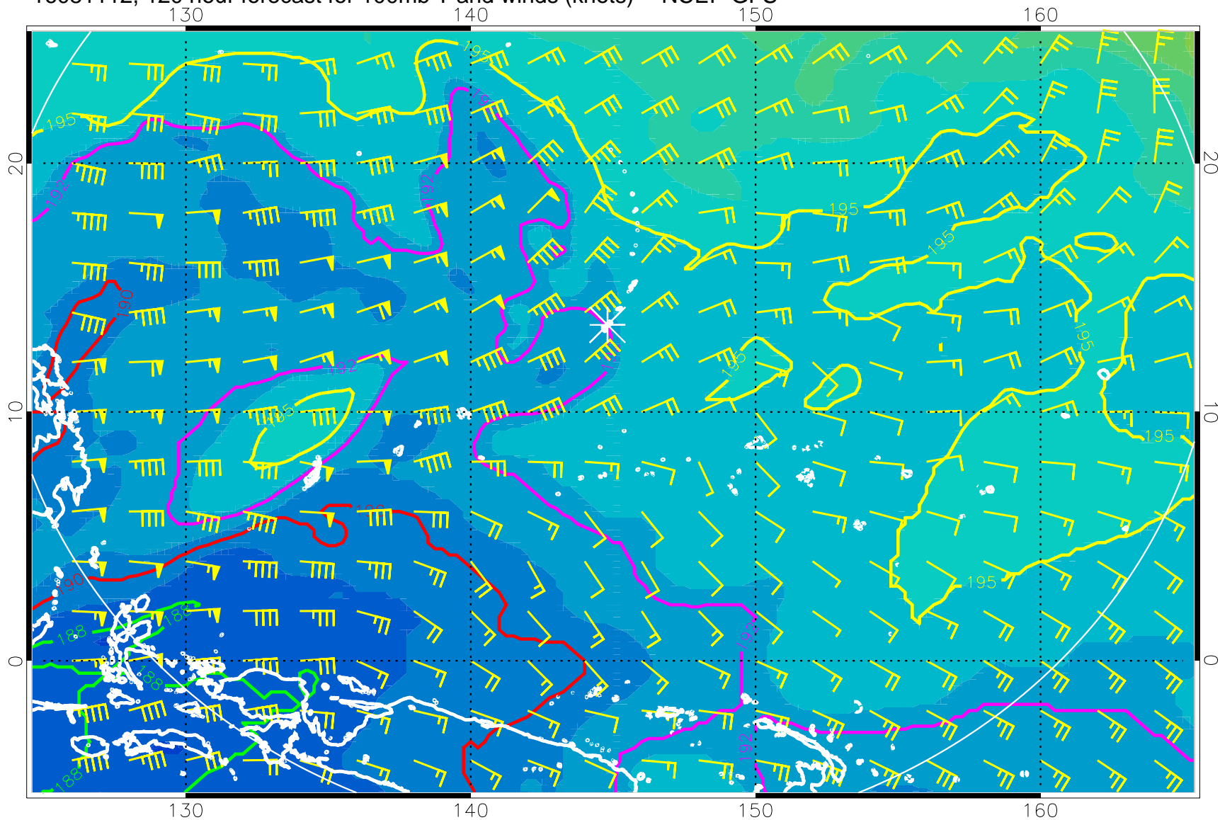
16081112, 120 hour forecast for 100mb T and winds (knots) -- NCEP GFS
