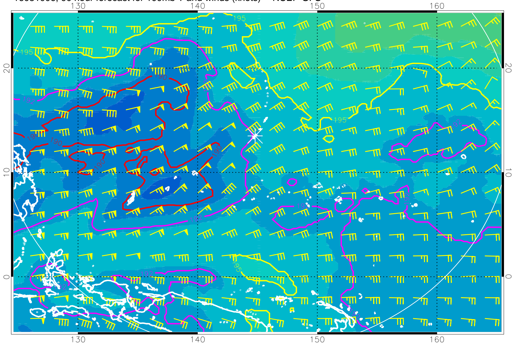
16081006, 90 hour forecast for 100mb T and winds (knots) -- NCEP GFS
