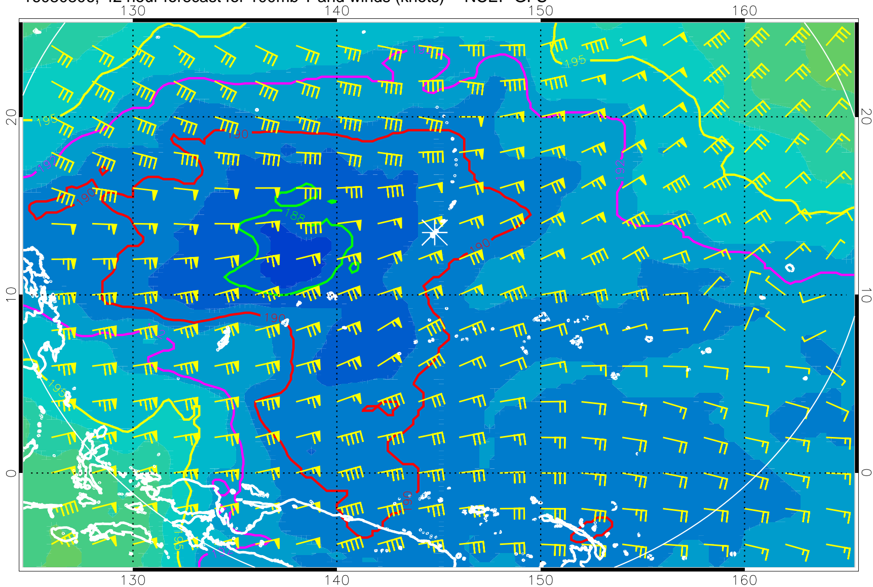
16080806, 42 hour forecast for 100mb T and winds (knots) -- NCEP GFS
