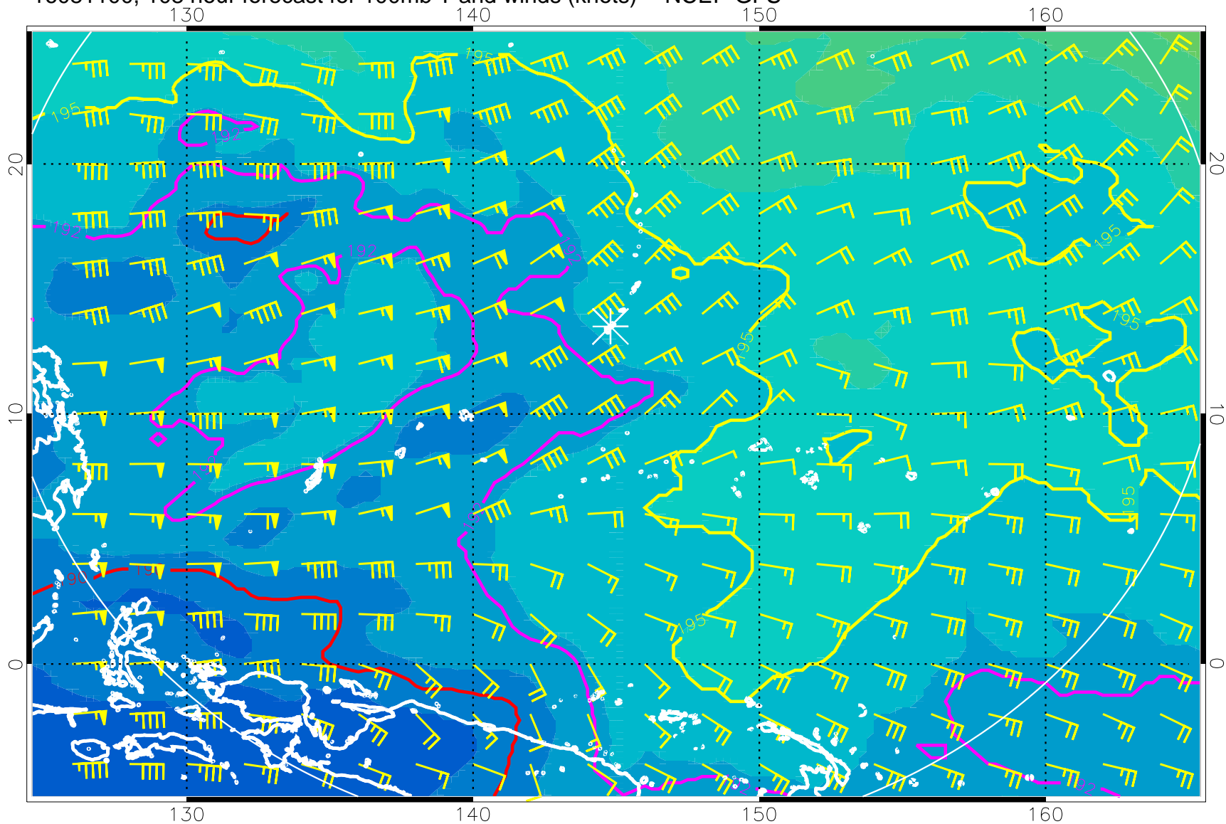
16081100, 108 hour forecast for 100mb T and winds (knots) -- NCEP GFS
