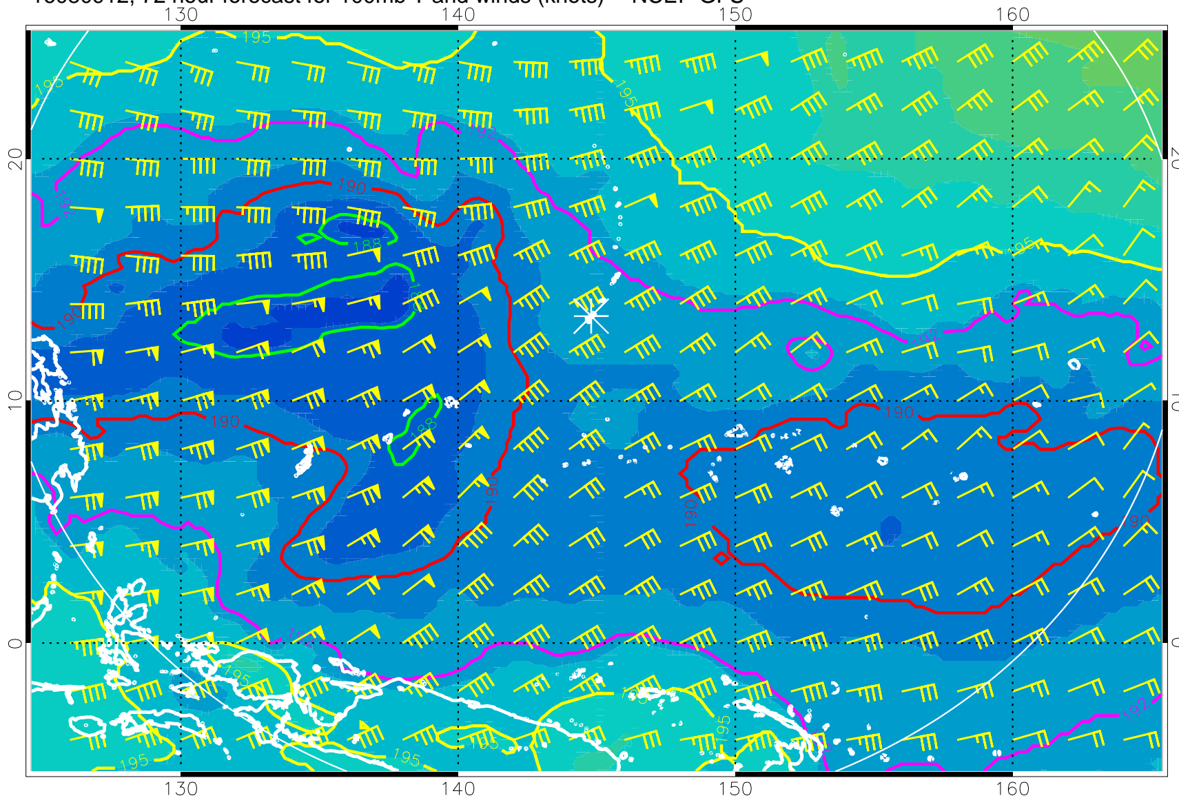
16080912, 72 hour forecast for 100mb T and winds (knots) -- NCEP GFS
