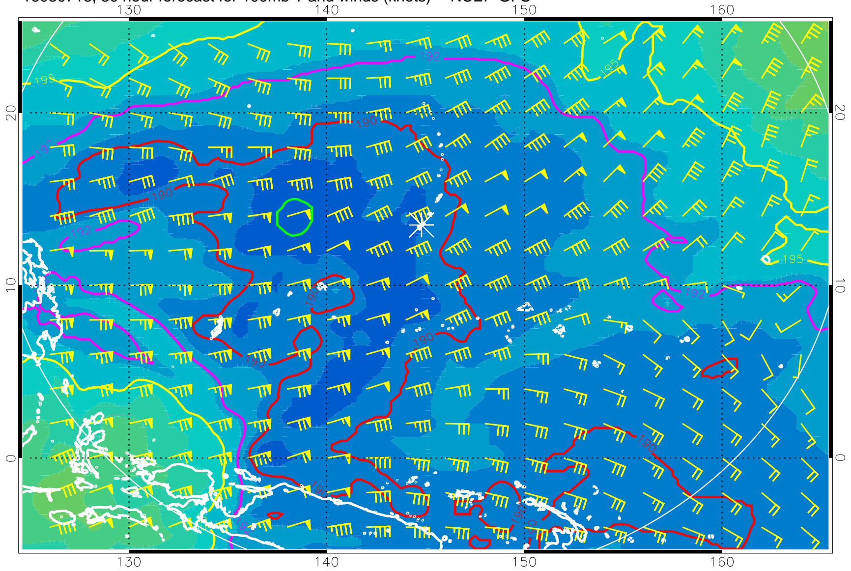
16080718, 30 hour forecast for 100mb T and winds (knots) -- NCEP GFS
