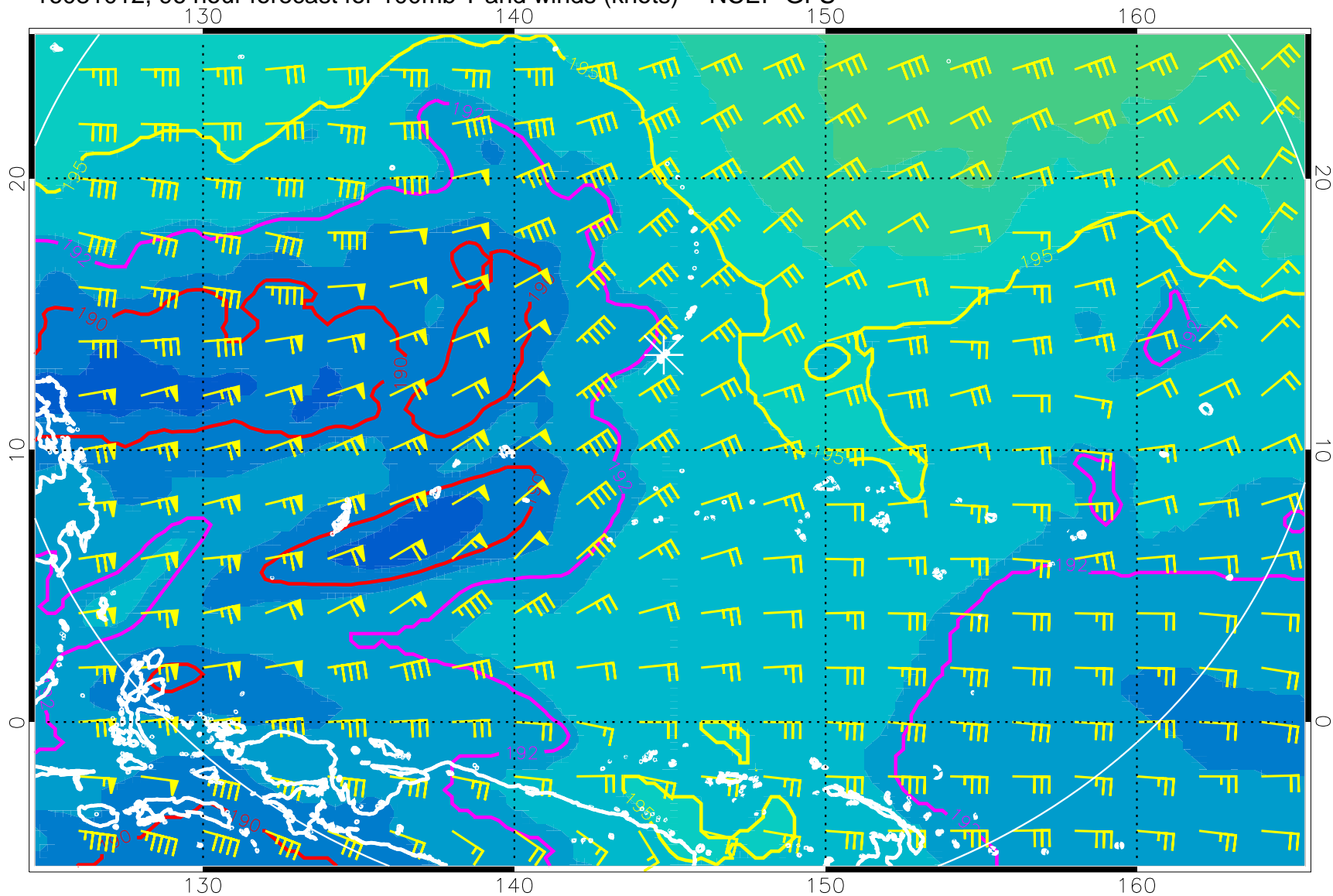
16081012, 96 hour forecast for 100mb T and winds (knots) -- NCEP GFS
