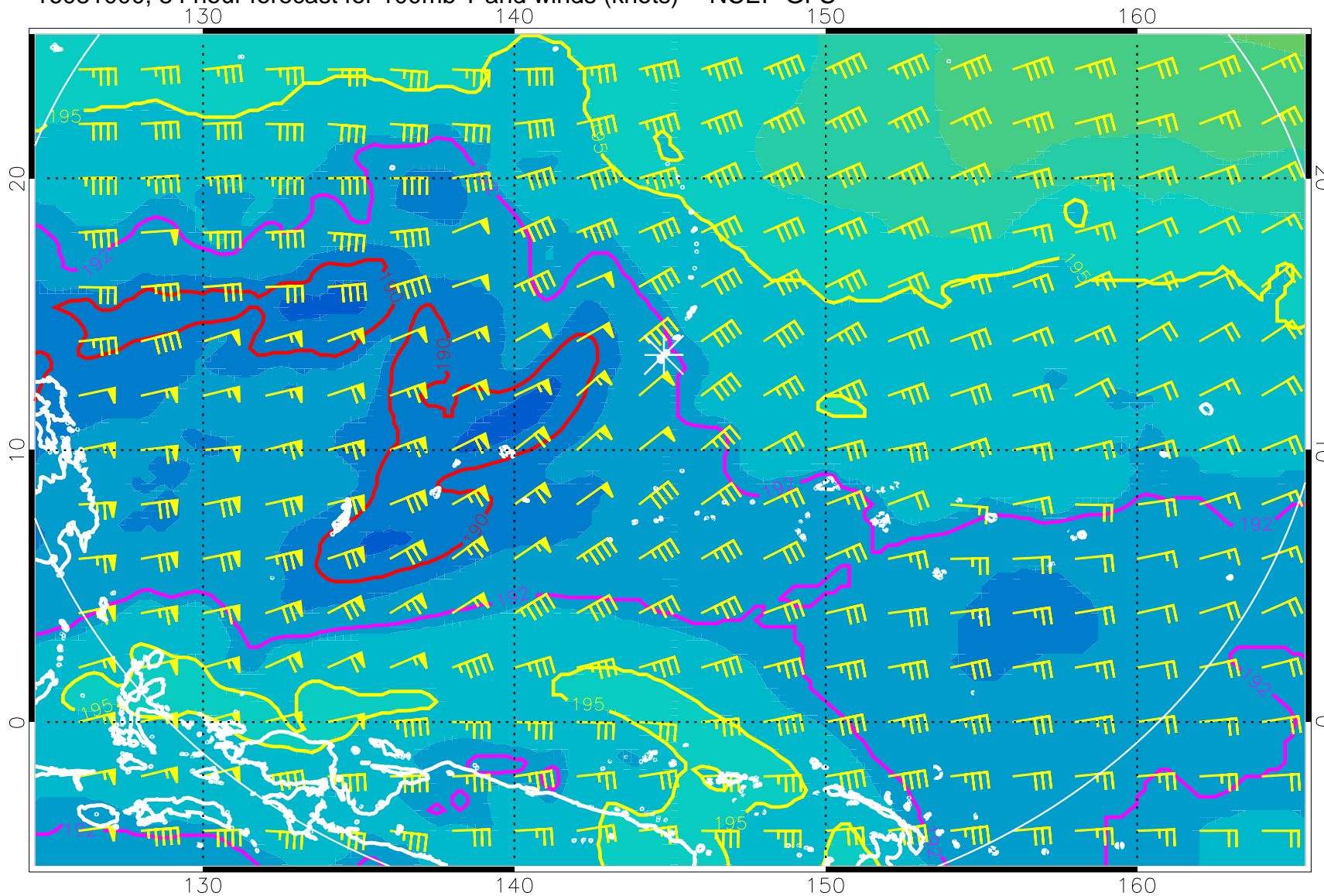
16081000, 84 hour forecast for 100mb T and winds (knots) -- NCEP GFS
