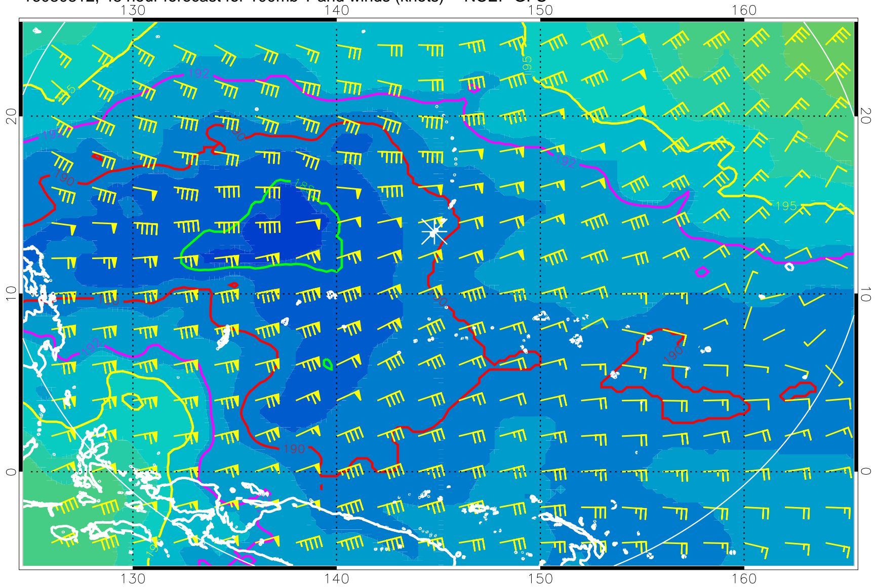
16080812, 48 hour forecast for 100mb T and winds (knots) -- NCEP GFS
