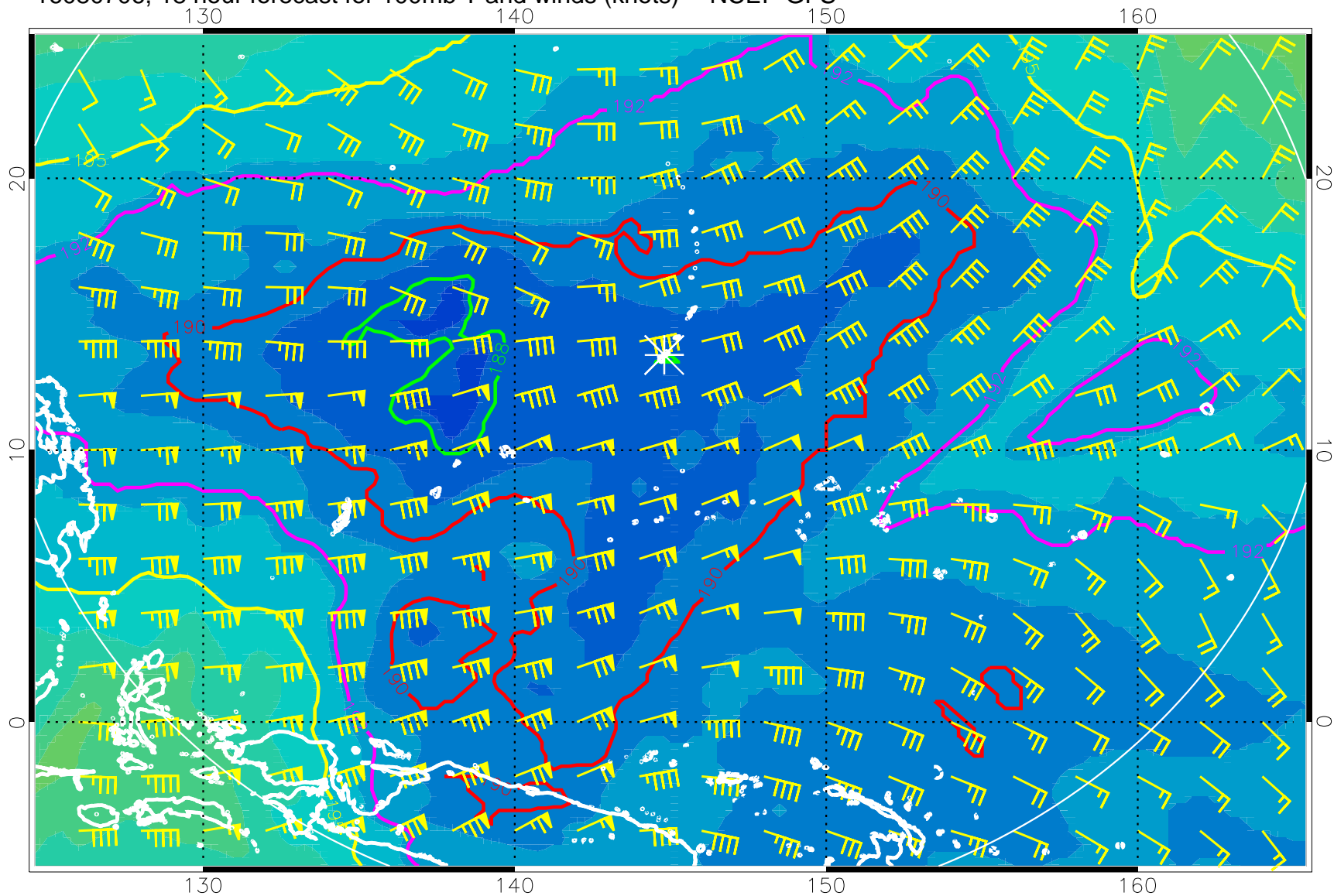
16080706, 18 hour forecast for 100mb T and winds (knots) -- NCEP GFS
