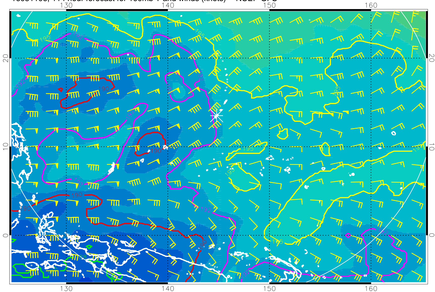
16081106, 114 hour forecast for 100mb T and winds (knots) -- NCEP GFS
