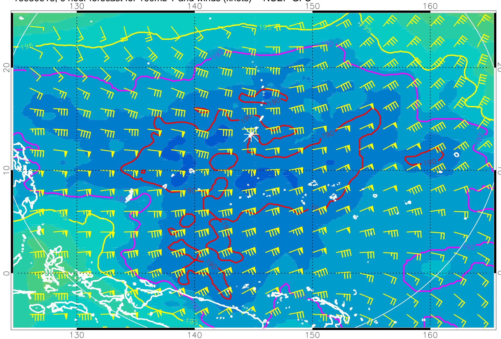
16080618, 6 hour forecast for 100mb T and winds (knots) -- NCEP GFS
