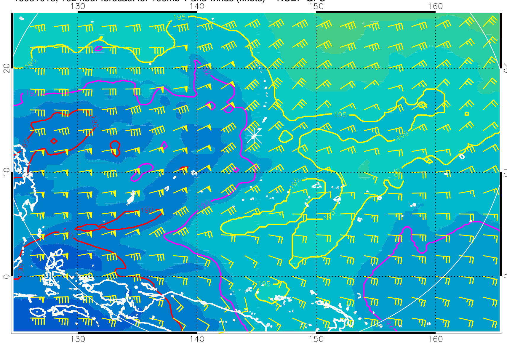
16081018, 102 hour forecast for 100mb T and winds (knots) -- NCEP GFS
