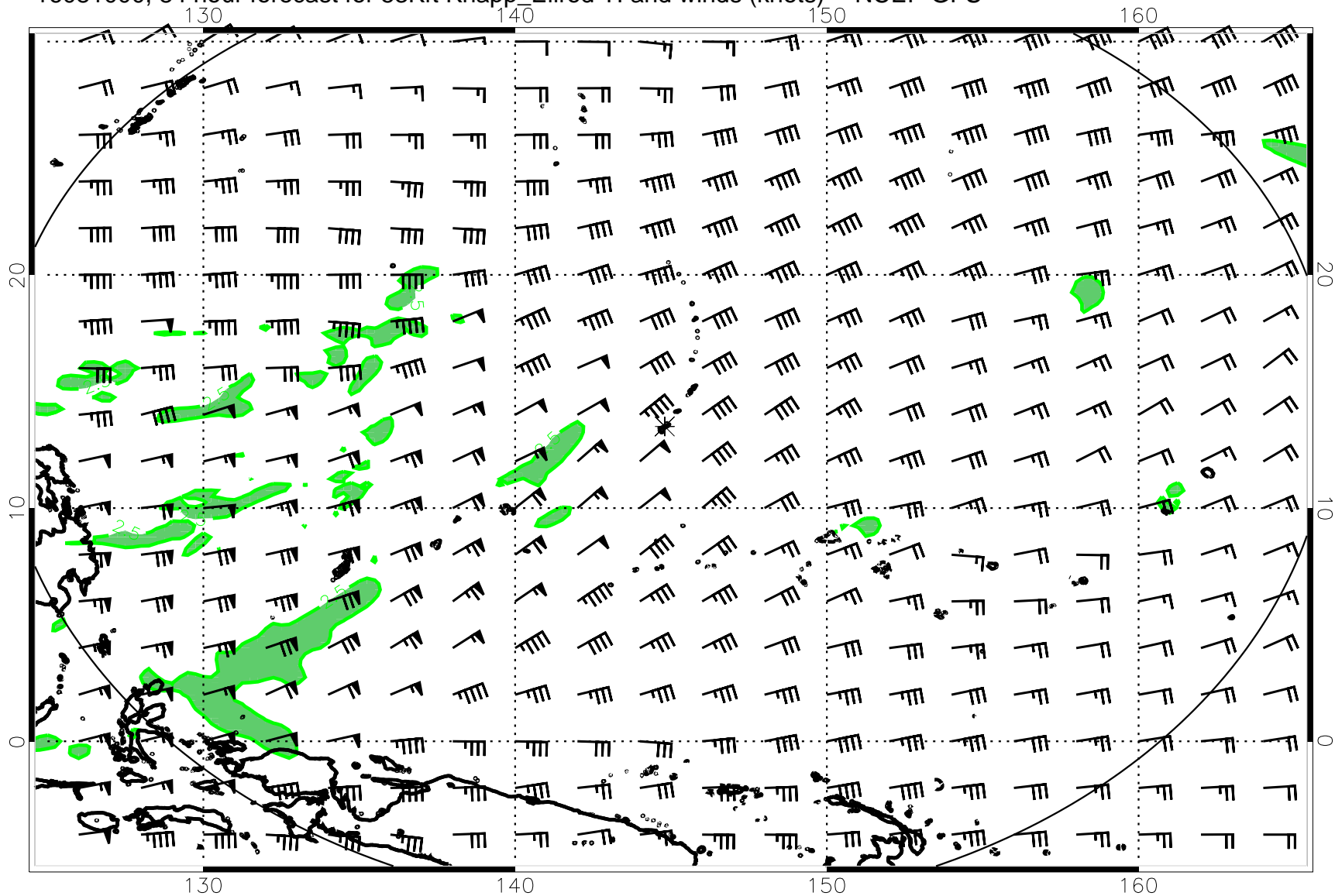
16081000, 84 hour forecast for 53Kft Knapp_Ellrod TI and winds (knots) -- NCEP GFS
