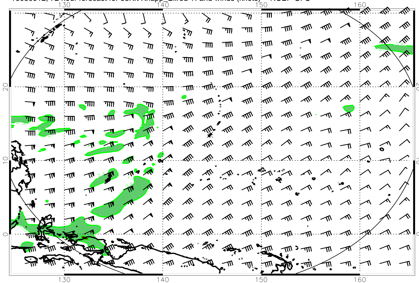
16080912, 72 hour forecast for 53Kft Knapp_Ellrod TI and winds (knots) -- NCEP GFS
