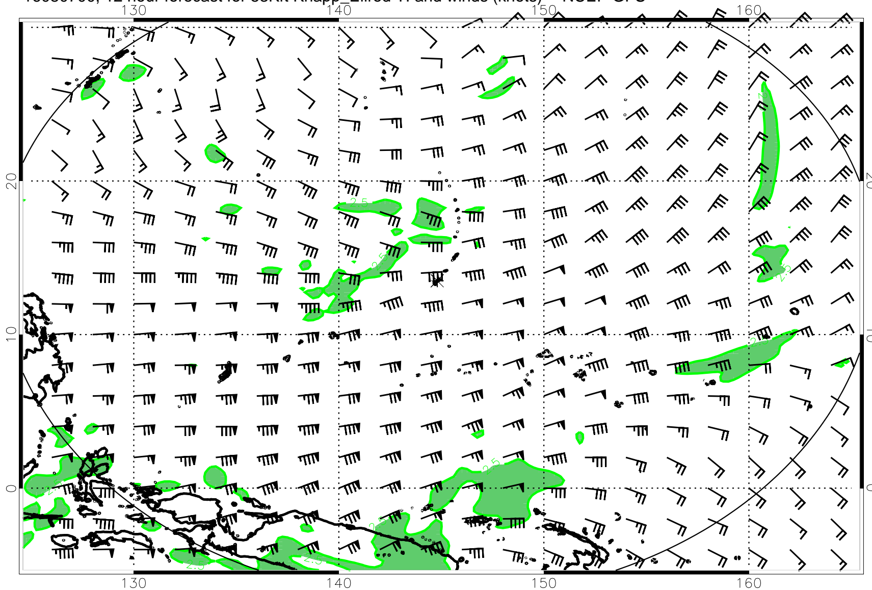
16080700, 12 hour forecast for 53Kft Knapp_Ellrod TI and winds (knots) -- NCEP GFS
