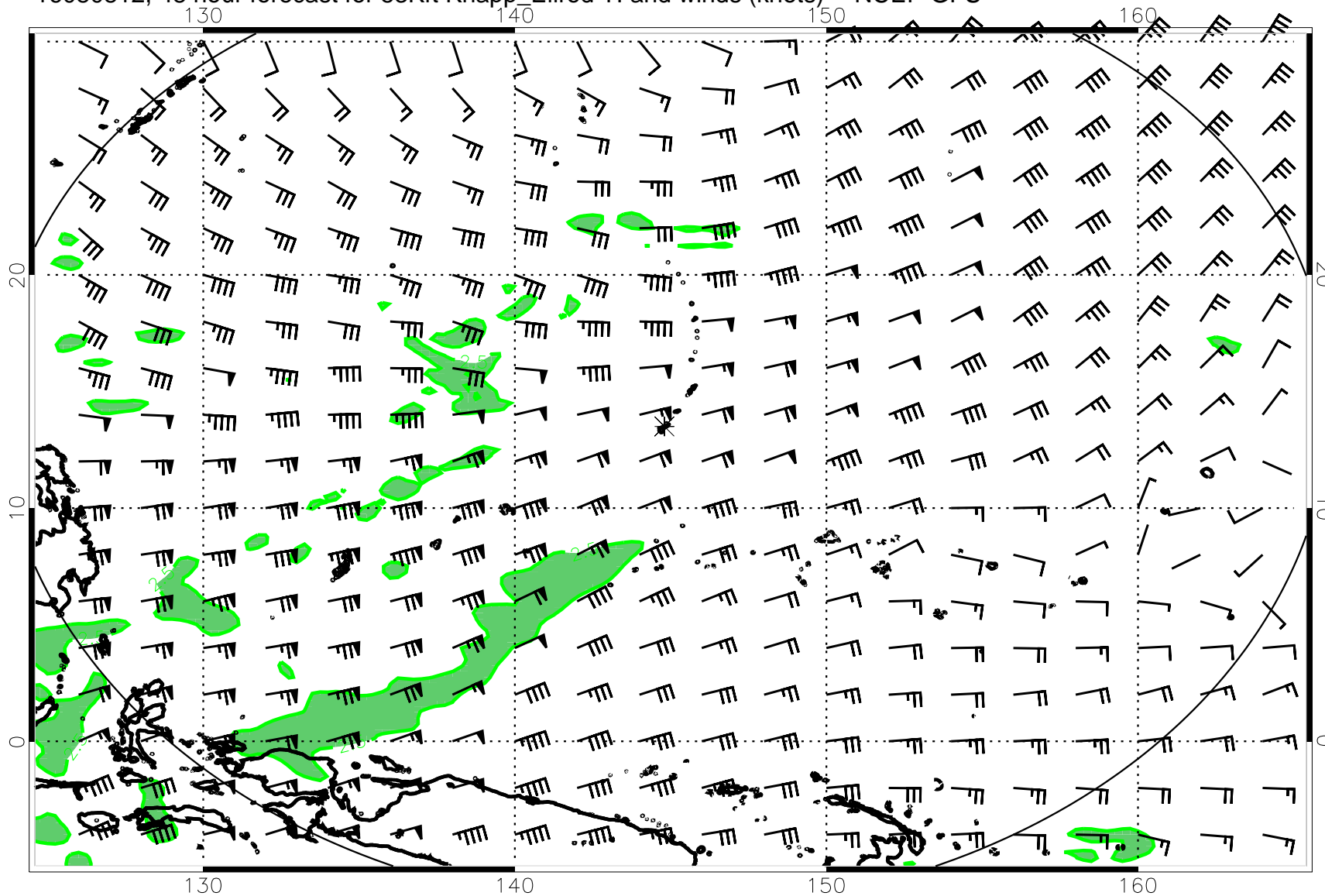
16080812, 48 hour forecast for 53Kft Knapp_Ellrod TI and winds (knots) -- NCEP GFS
