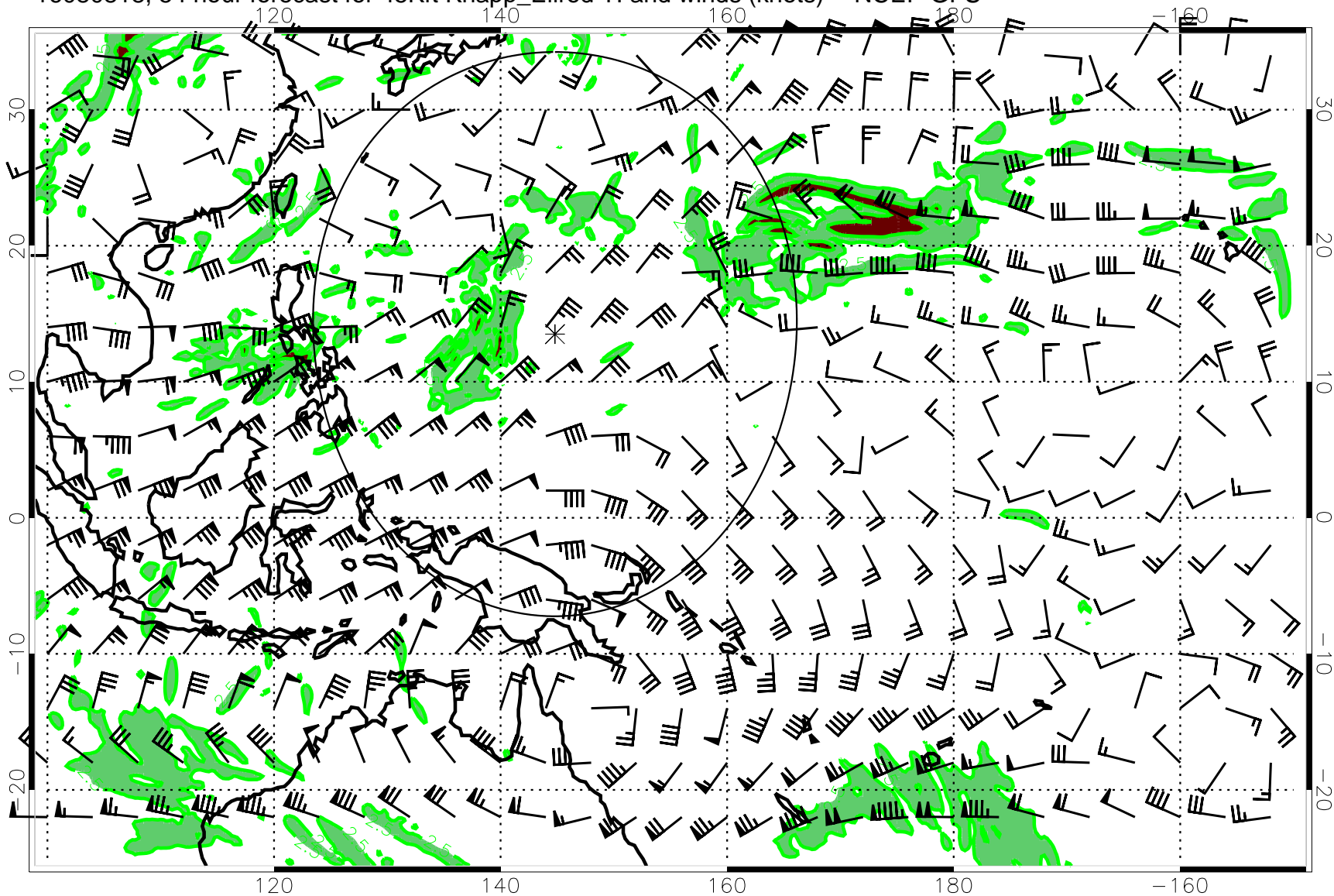
16080818, 54 hour forecast for 45Kft Knapp_Ellrod TI and winds (knots) -- NCEP GFS
