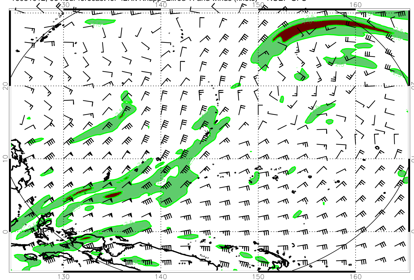
16081012, 96 hour forecast for 42Kft Knapp_Ellrod TI and winds (knots) -- NCEP GFS
