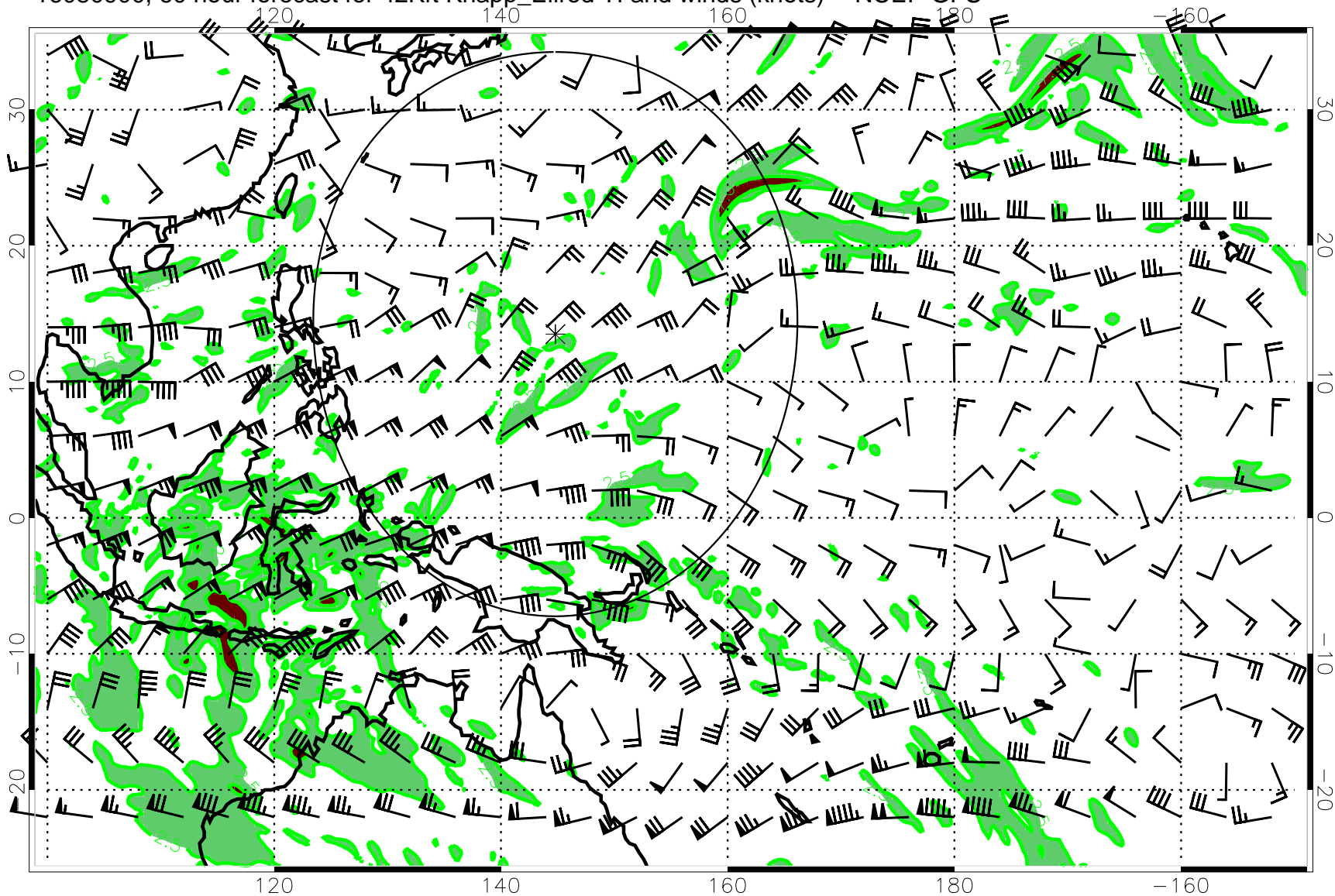
16080900, 60 hour forecast for 42Kft Knapp_Ellrod TI and winds (knots) -- NCEP GFS
