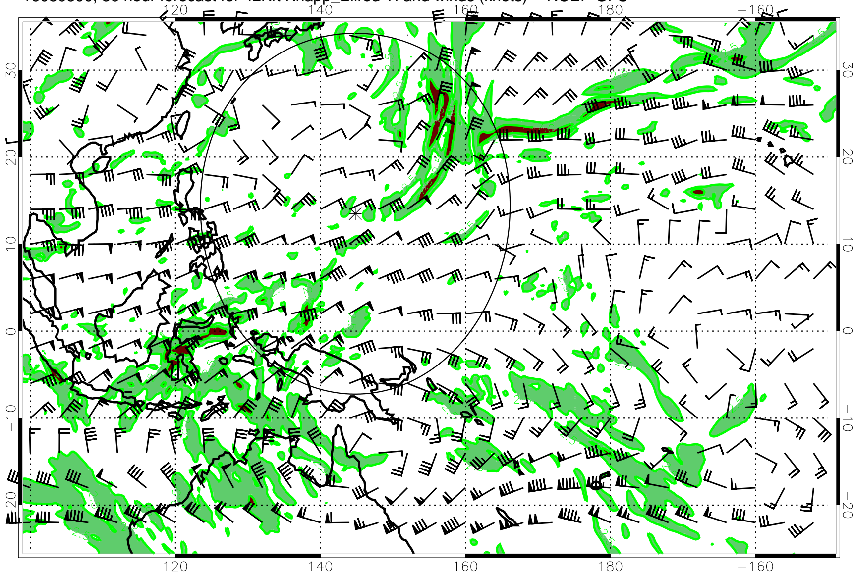
16080800, 36 hour forecast for 42Kft Knapp_Ellrod TI and winds (knots) -- NCEP GFS
