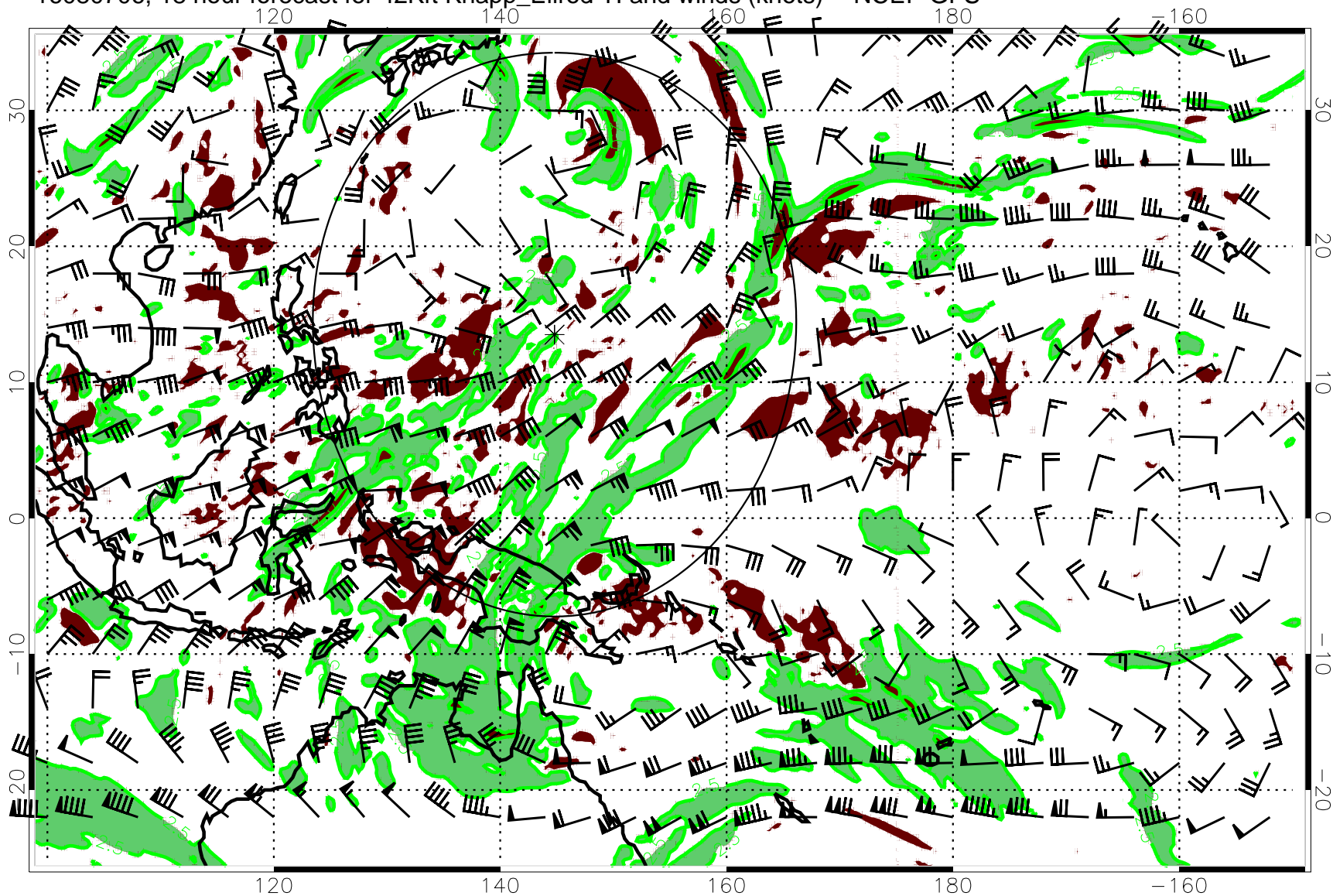
16080706, 18 hour forecast for 42Kft Knapp_Ellrod TI and winds (knots) -- NCEP GFS
