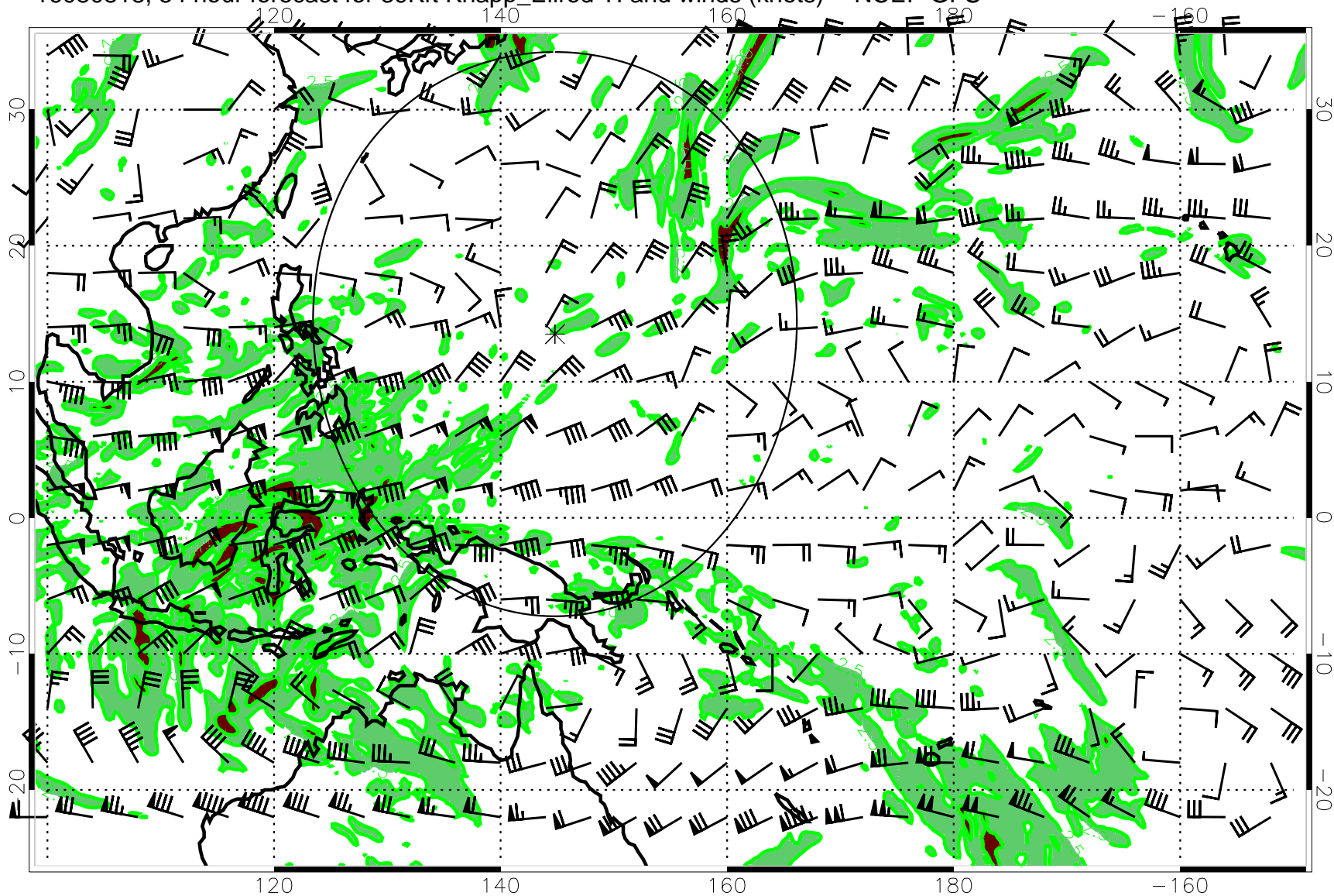
16080818, 54 hour forecast for 39Kft Knapp_Ellrod TI and winds (knots) -- NCEP GFS
