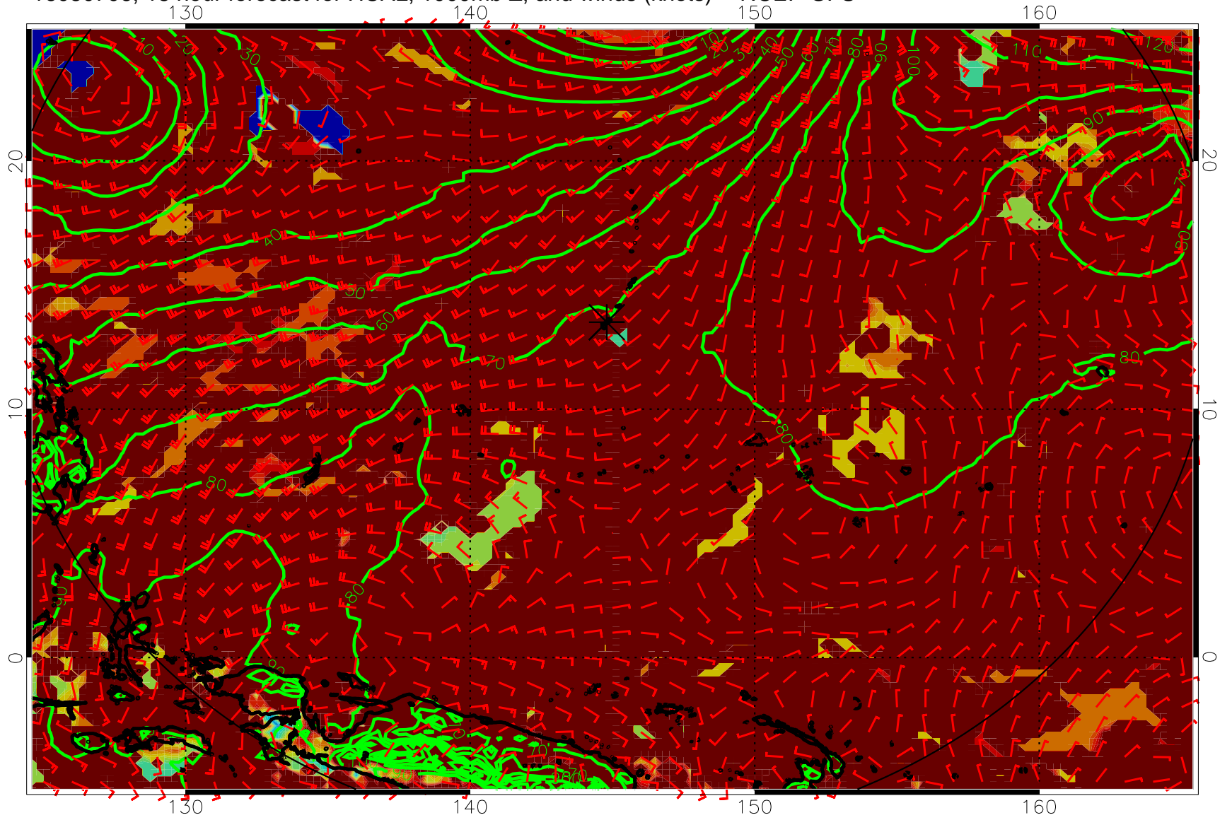
16080706, 18 hour forecast for HCAL, 1000mb Z, and winds (knots) -- NCEP GFS
