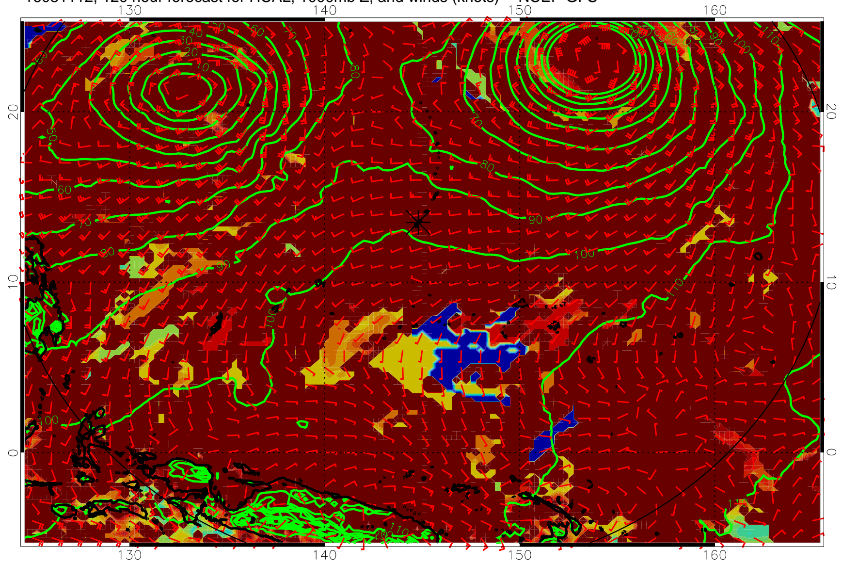
16081112, 120 hour forecast for HCAL, 1000mb Z, and winds (knots) -- NCEP GFS
