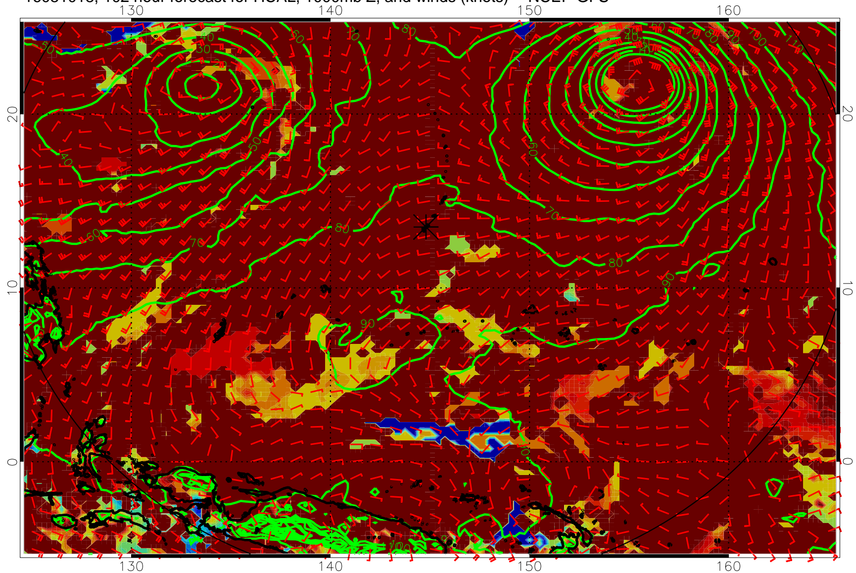
16081018, 102 hour forecast for HCAL, 1000mb Z, and winds (knots) -- NCEP GFS
