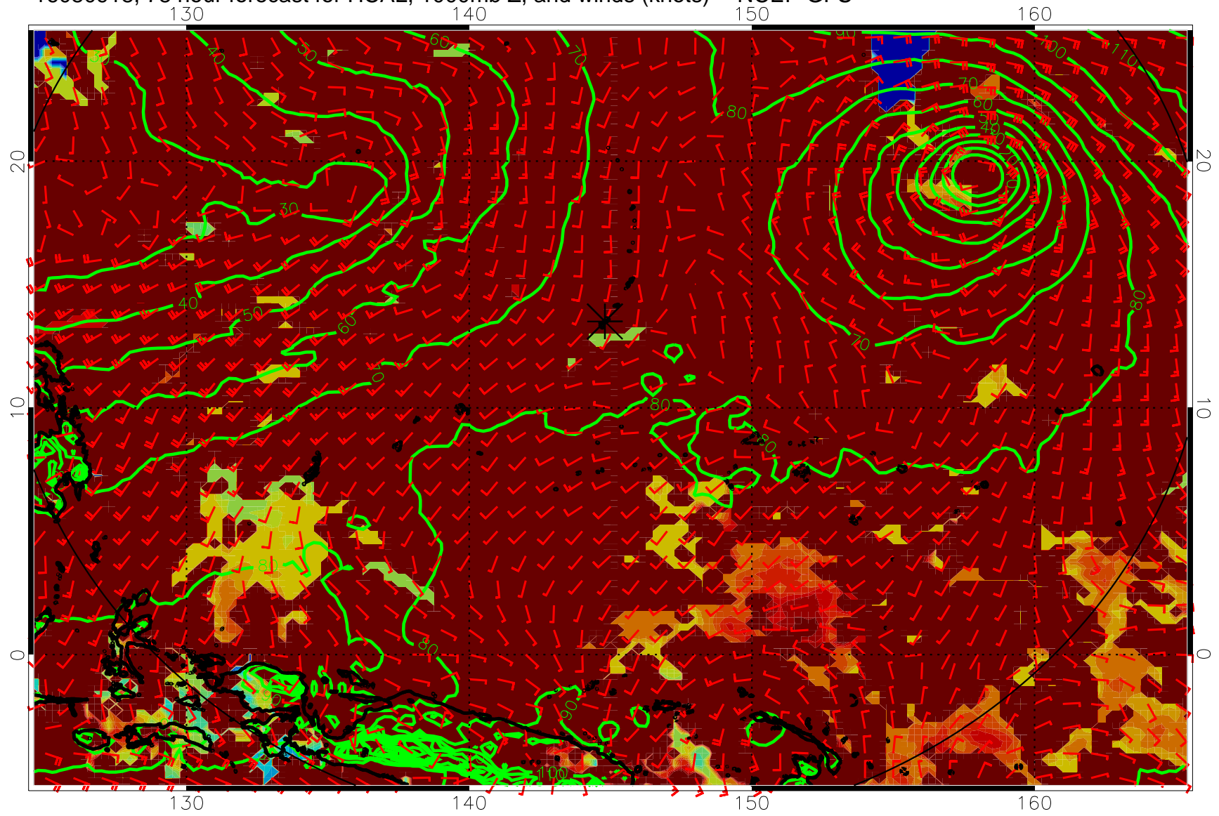
16080918, 78 hour forecast for HCAL, 1000mb Z, and winds (knots) -- NCEP GFS
