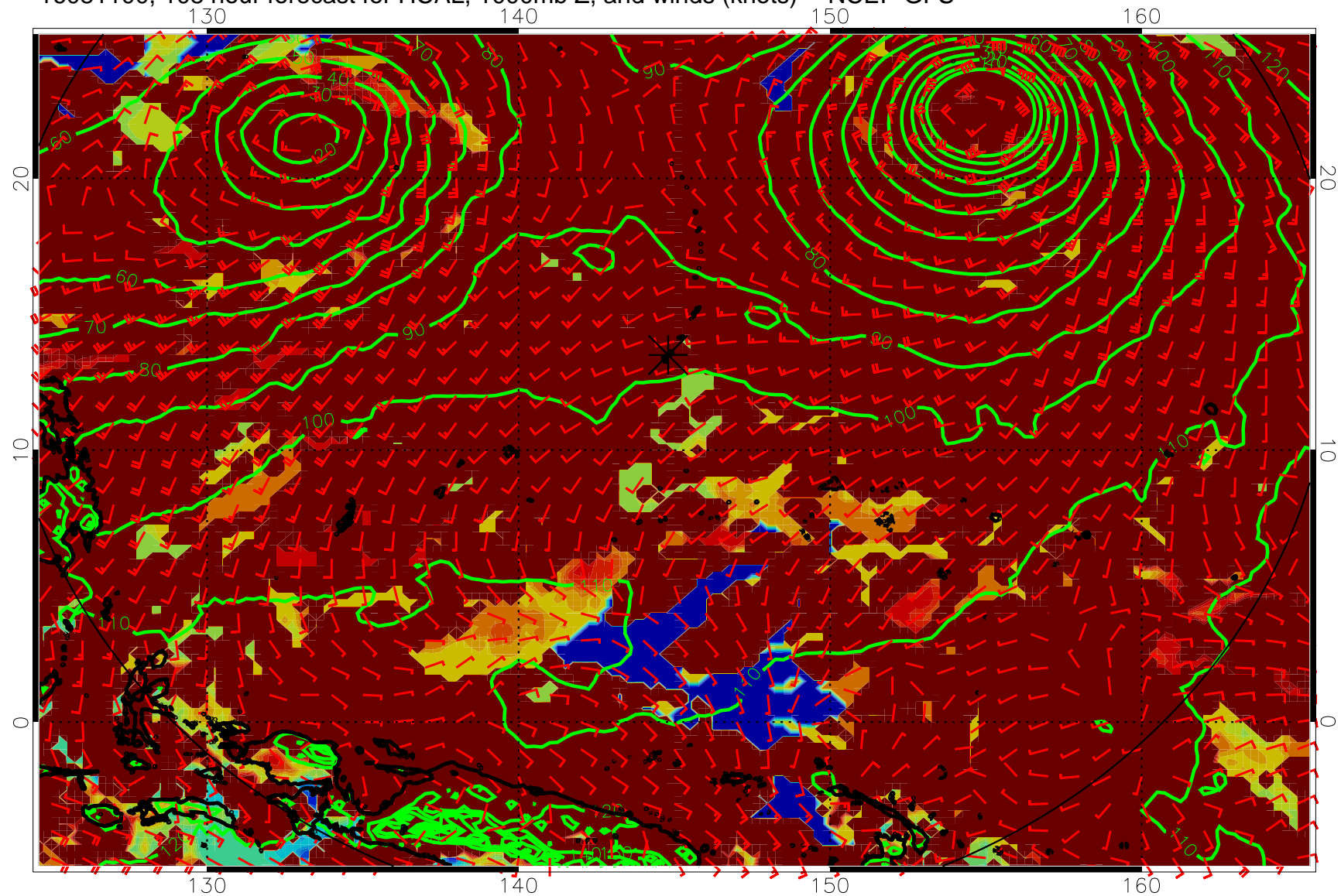
16081100, 108 hour forecast for HCAL, 1000mb Z, and winds (knots) -- NCEP GFS
