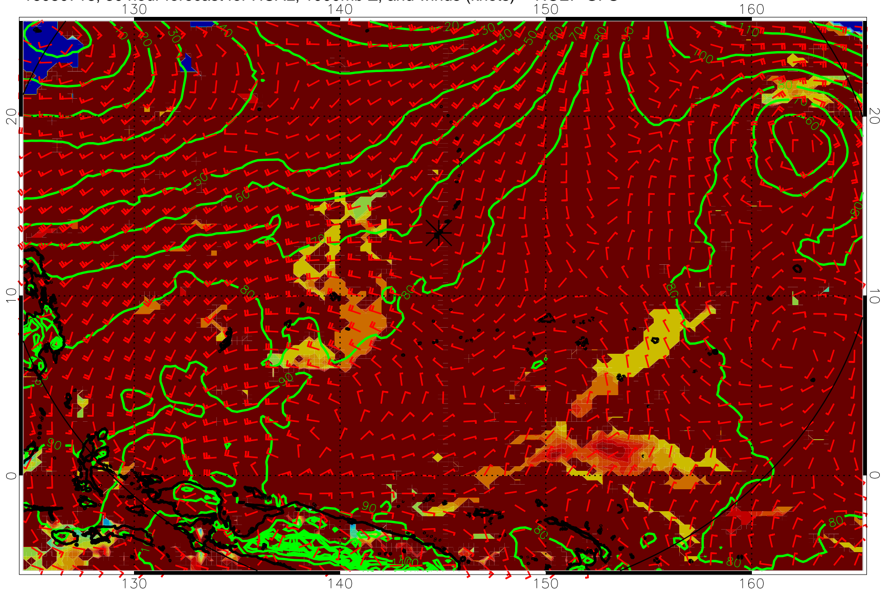
16080718, 30 hour forecast for HCAL, 1000mb Z, and winds (knots) -- NCEP GFS
