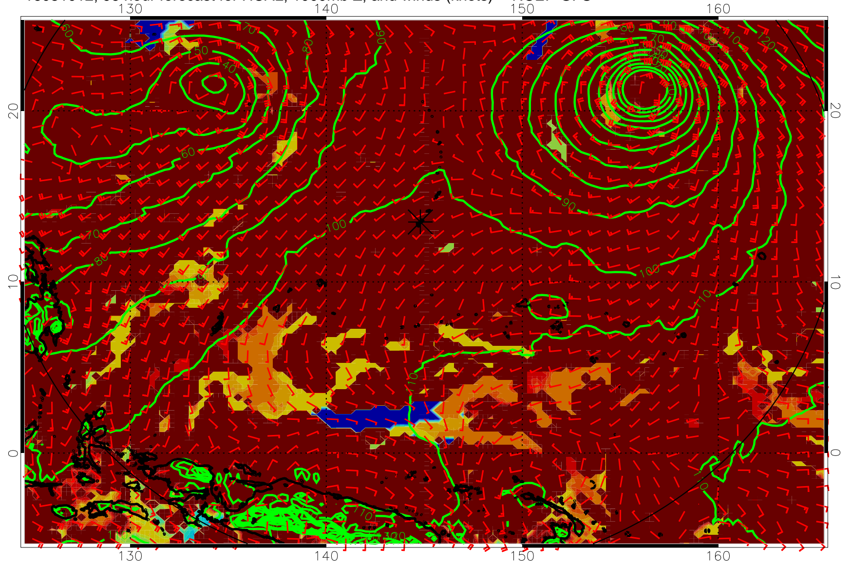
16081012, 96 hour forecast for HCAL, 1000mb Z, and winds (knots) -- NCEP GFS
