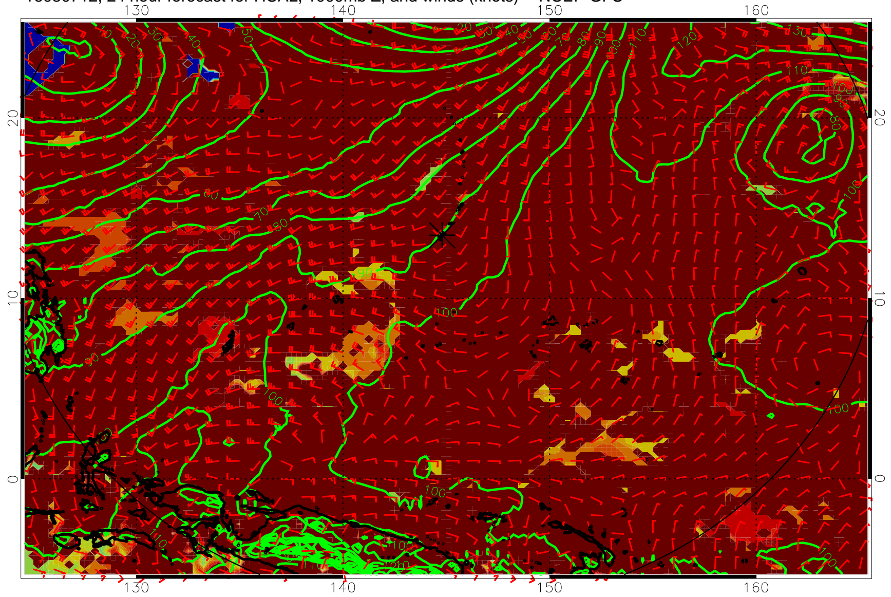
16080712, 24 hour forecast for HCAL, 1000mb Z, and winds (knots) -- NCEP GFS
