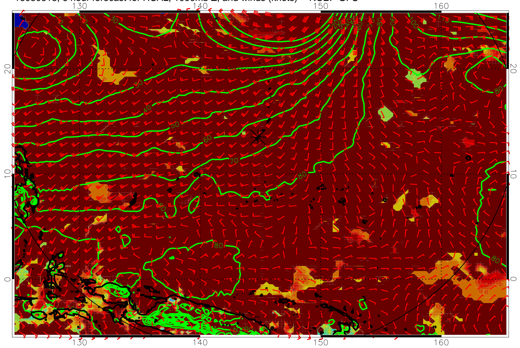
16080618, 6 hour forecast for HCAL, 1000mb Z, and winds (knots) -- NCEP GFS
