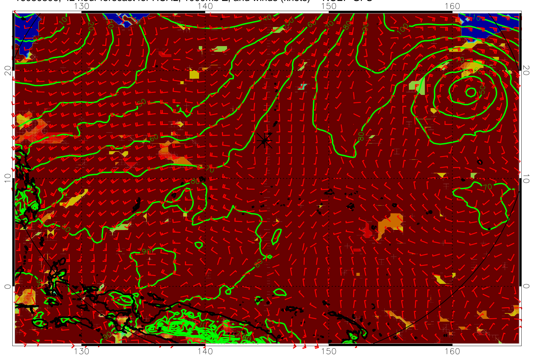
16080806, 42 hour forecast for HCAL, 1000mb Z, and winds (knots) -- NCEP GFS
