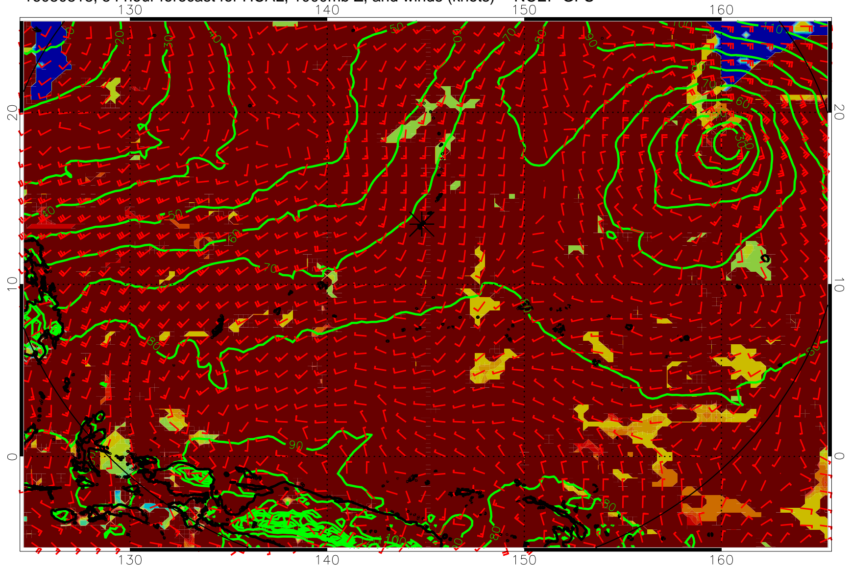
16080818, 54 hour forecast for HCAL, 1000mb Z, and winds (knots) -- NCEP GFS
