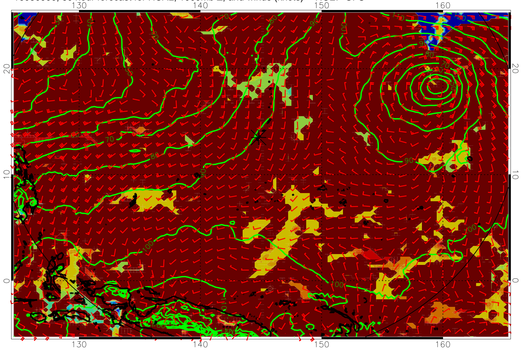
16080900, 60 hour forecast for HCAL, 1000mb Z, and winds (knots) -- NCEP GFS
