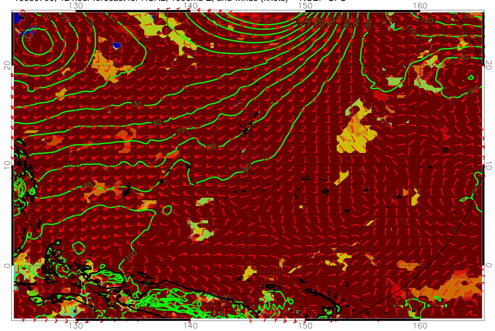
16080700, 12 hour forecast for HCAL, 1000mb Z, and winds (knots) -- NCEP GFS
