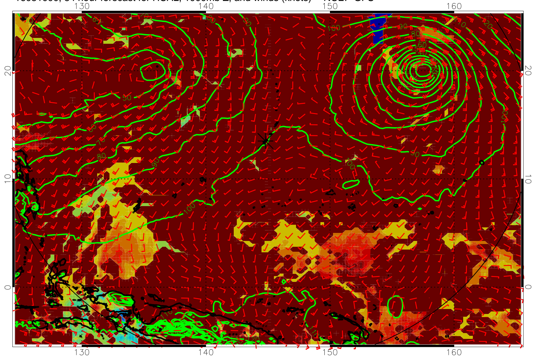
16081000, 84 hour forecast for HCAL, 1000mb Z, and winds (knots) -- NCEP GFS
