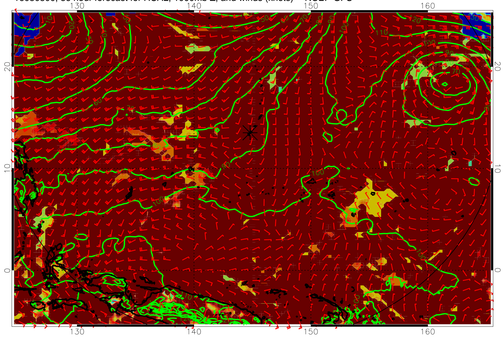
16080800, 36 hour forecast for HCAL, 1000mb Z, and winds (knots) -- NCEP GFS
