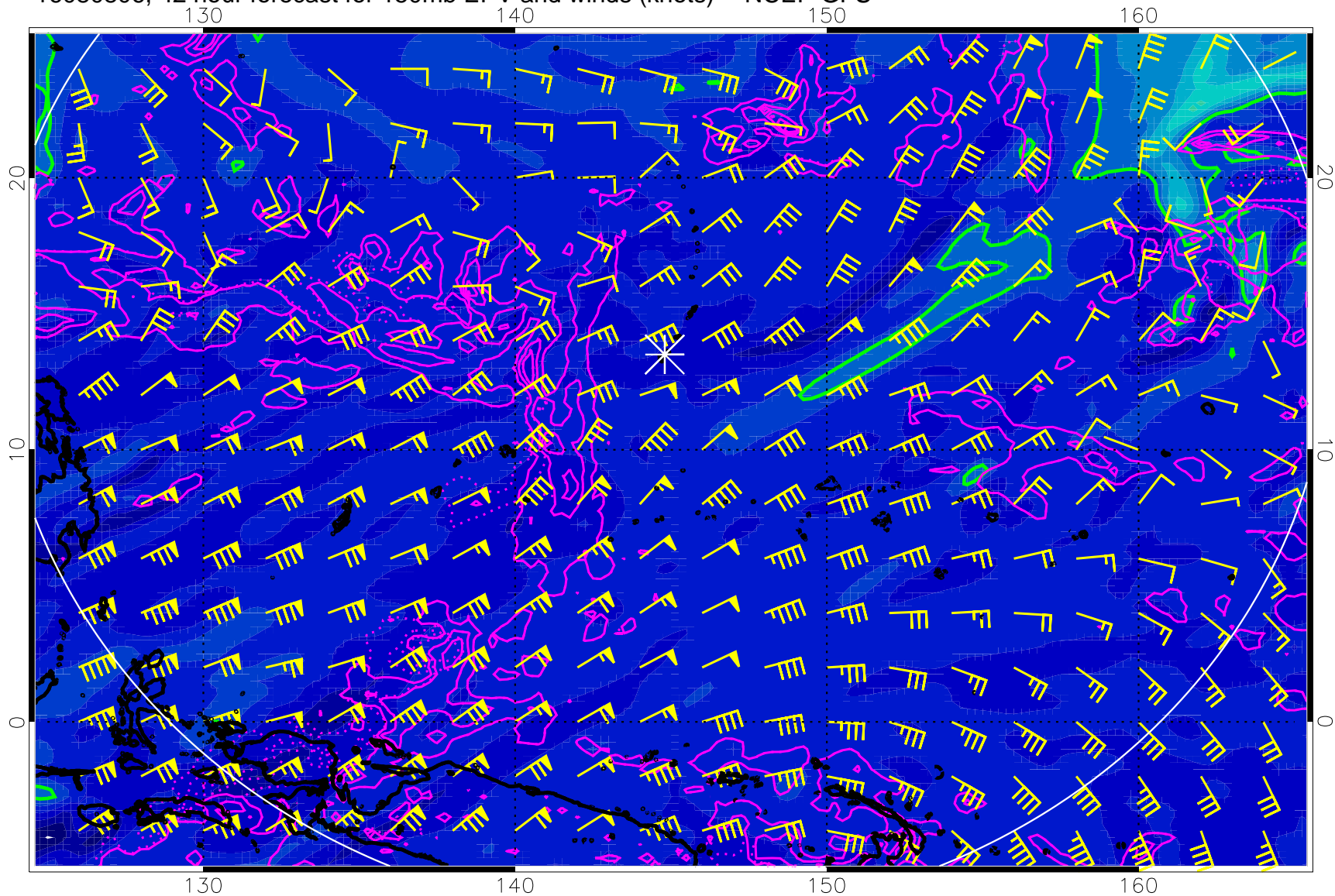
16080806, 42 hour forecast for 150mb EPV and winds (knots) -- NCEP GFS
