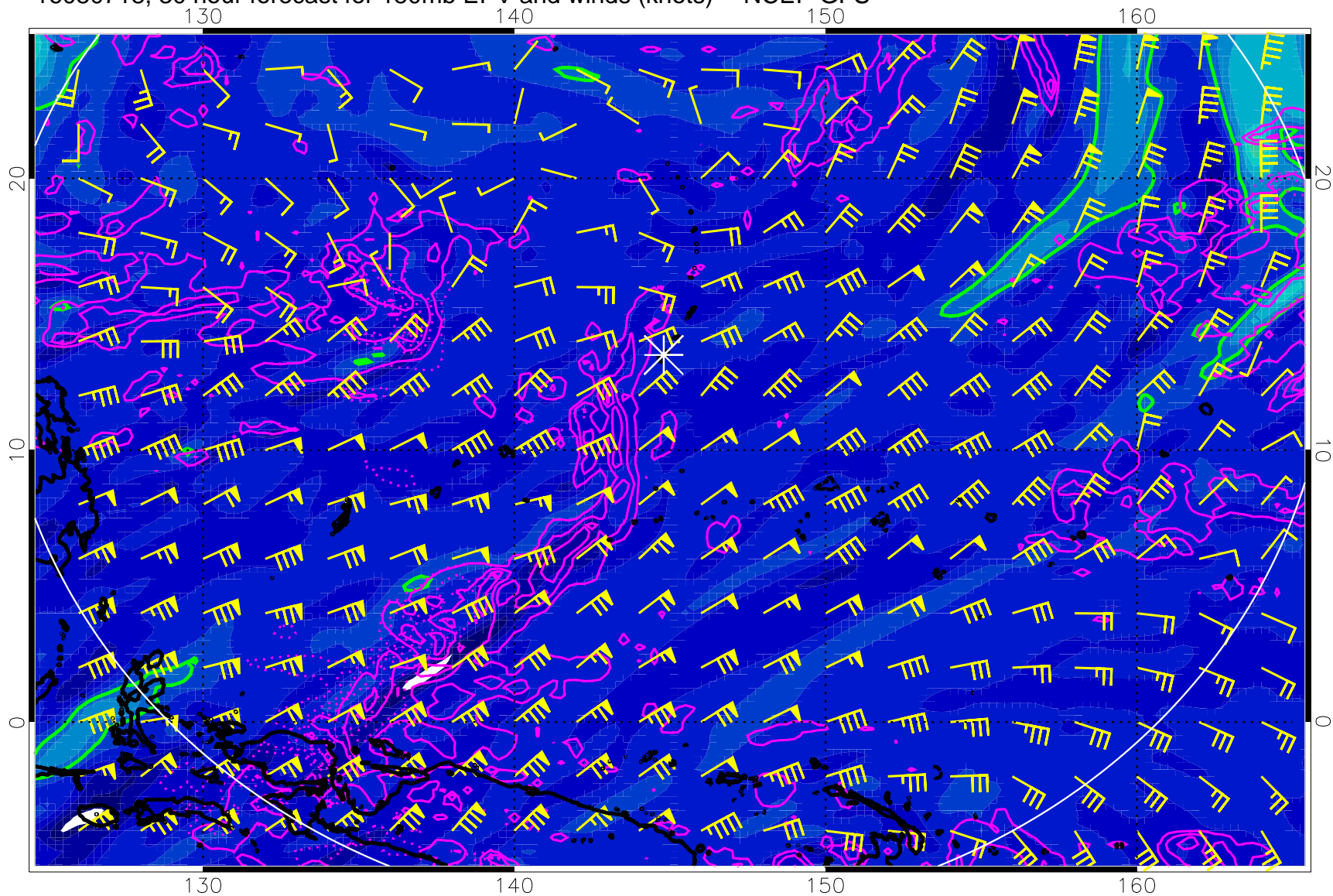
16080718, 30 hour forecast for 150mb EPV and winds (knots) -- NCEP GFS
