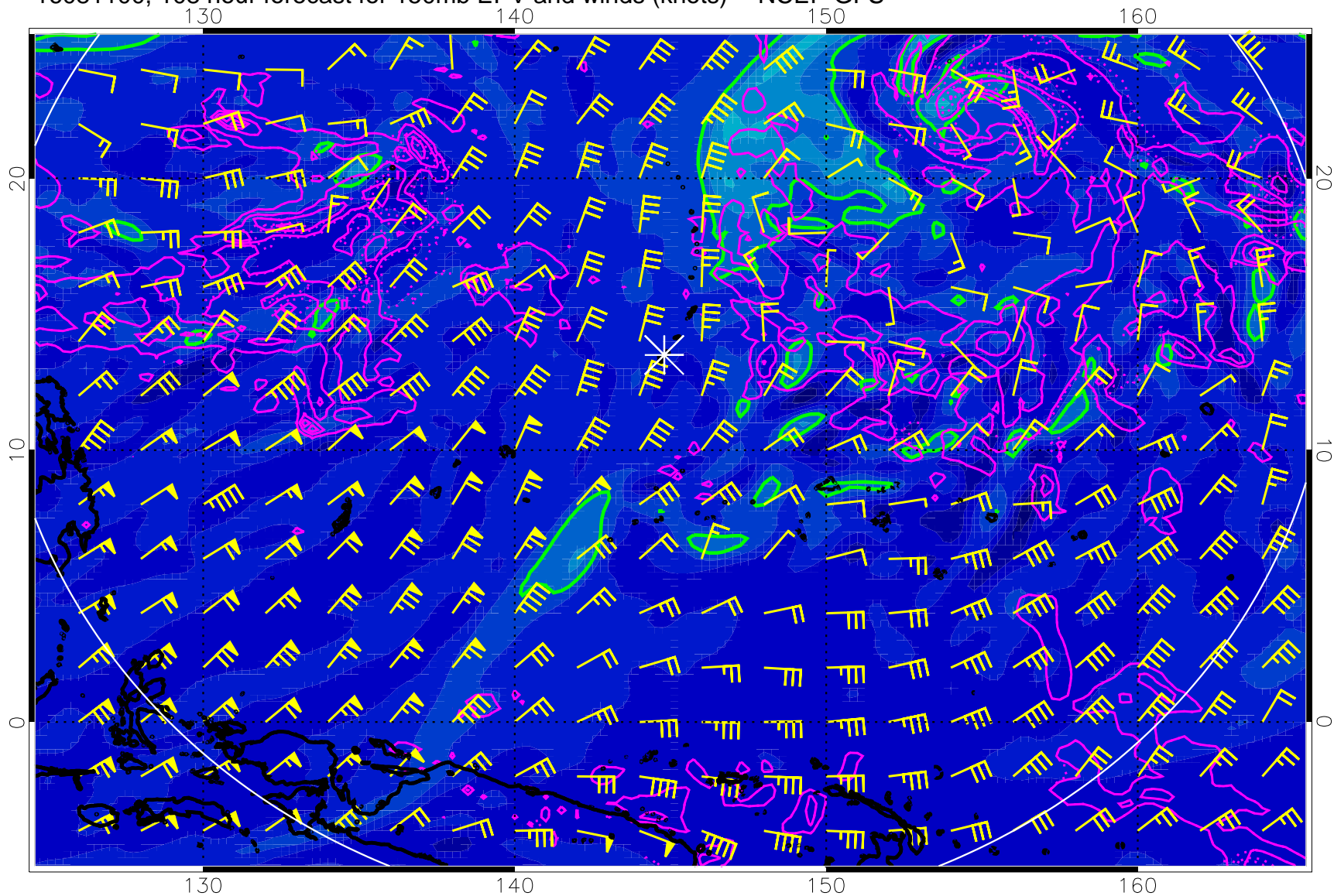
16081100, 108 hour forecast for 150mb EPV and winds (knots) -- NCEP GFS
