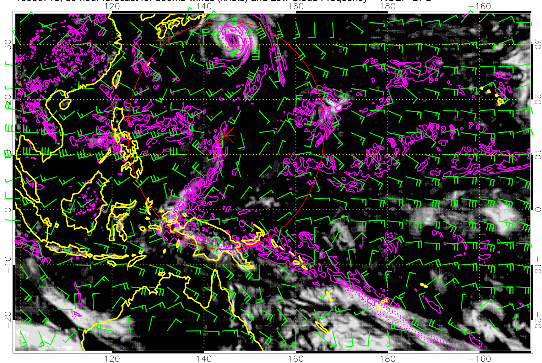
16080718, 30 hour forecast for 850mb winds (knots) and Low Cloud Frequency -- NCEP GFS
