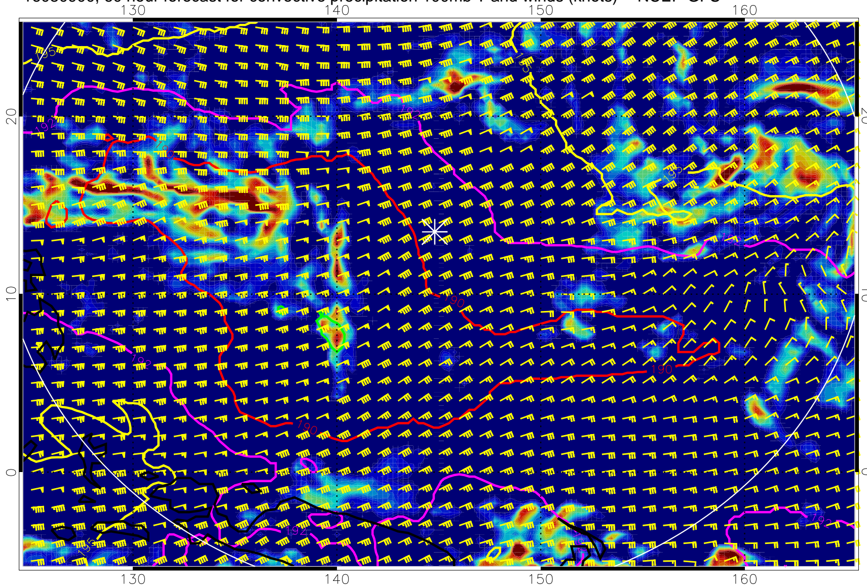
16080900, 60 hour forecast for convective precipitation 100mb T and winds (knots) -- NCEP GFS
