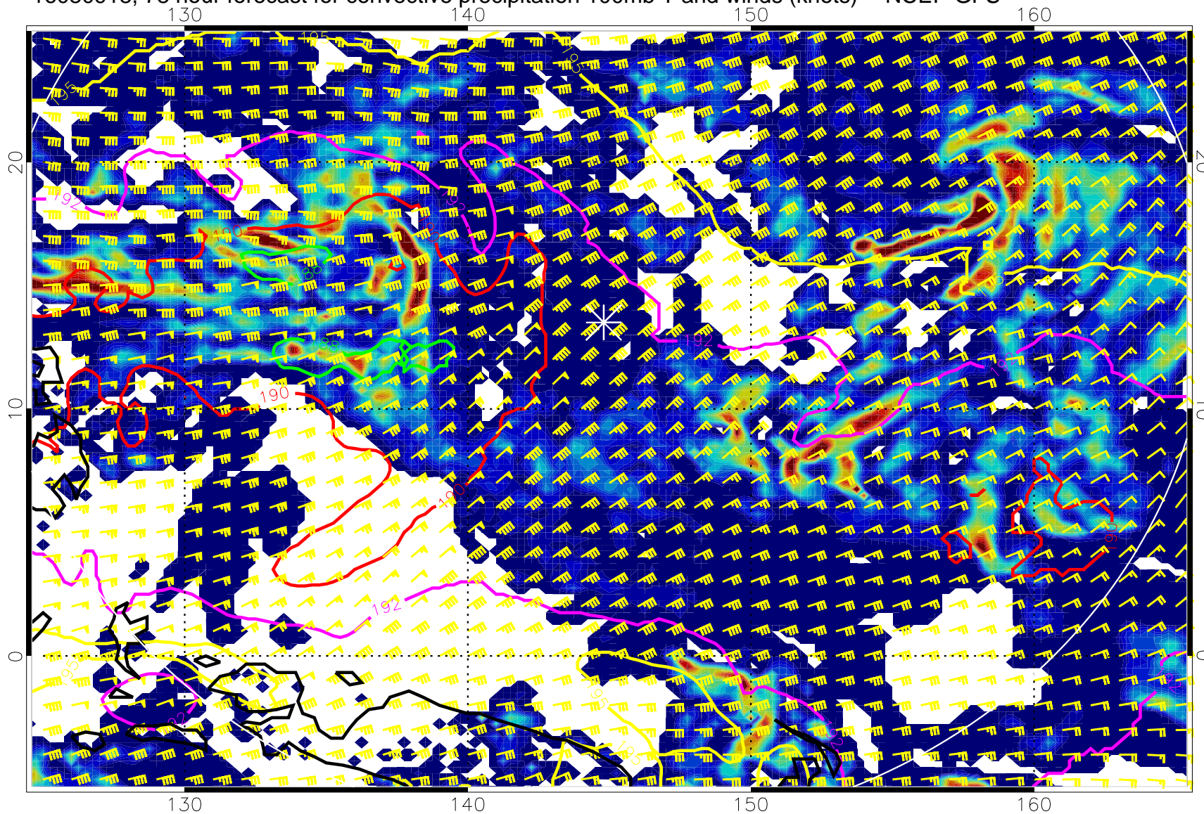
16080918, 78 hour forecast for convective precipitation 100mb T and winds (knots) -- NCEP GFS
