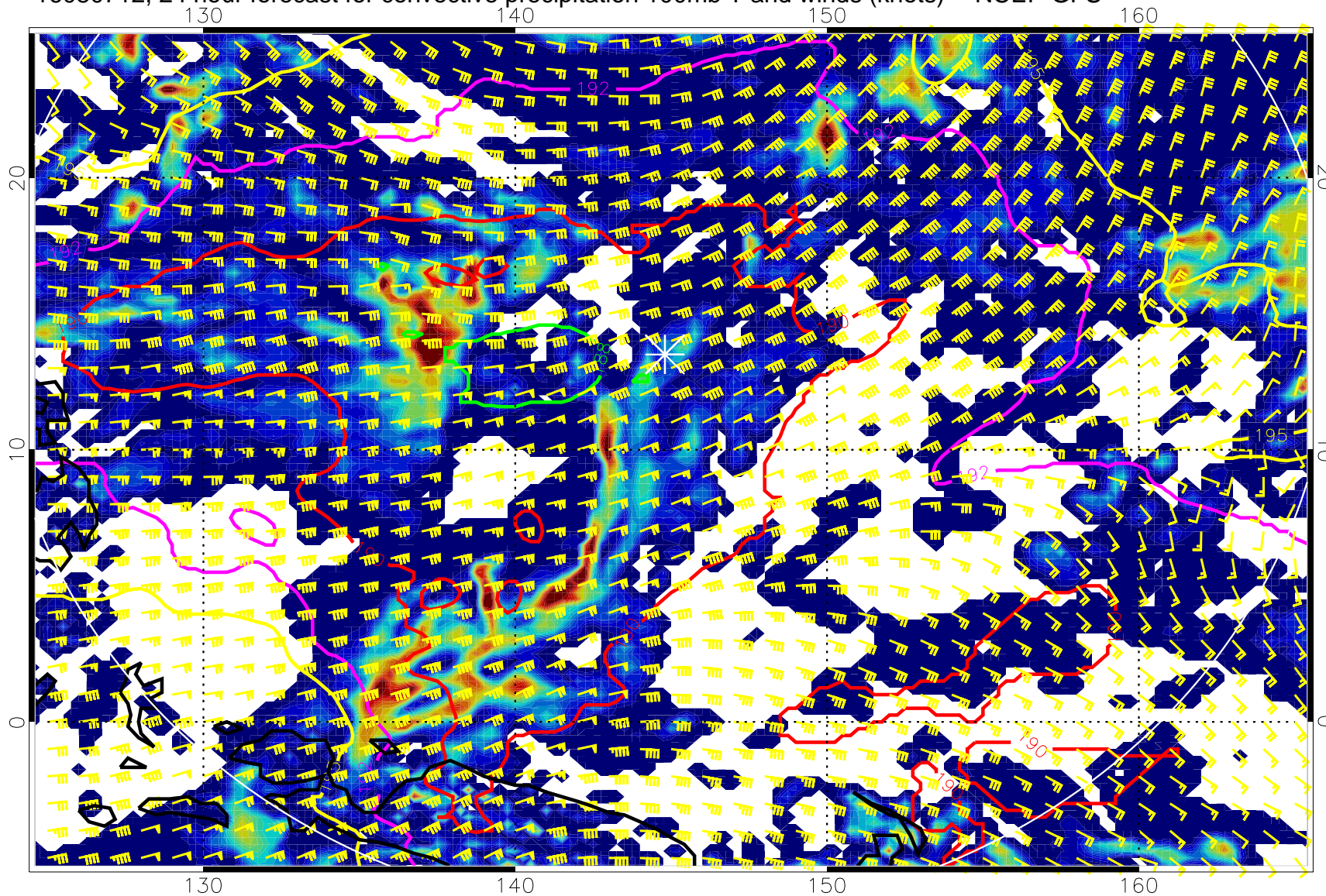
16080712, 24 hour forecast for convective precipitation 100mb T and winds (knots) -- NCEP GFS
