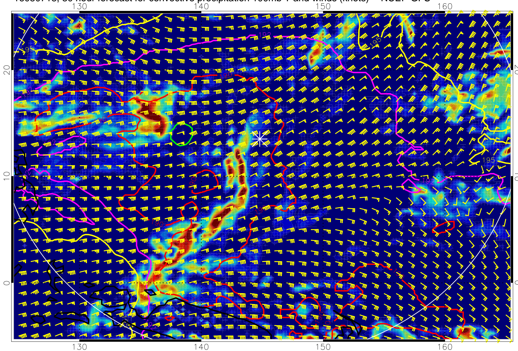
16080718, 30 hour forecast for convective precipitation 100mb T and winds (knots) -- NCEP GFS
