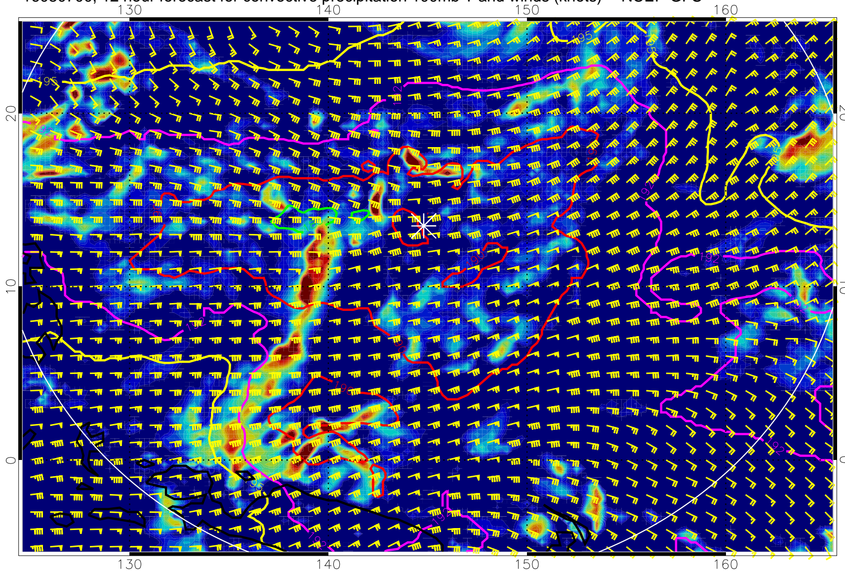
16080700, 12 hour forecast for convective precipitation 100mb T and winds (knots) -- NCEP GFS
