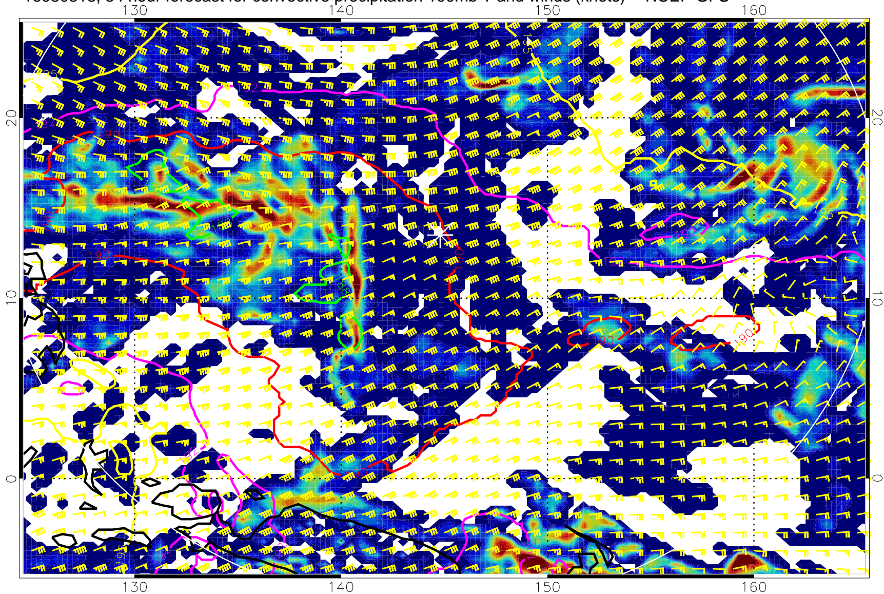
16080818, 54 hour forecast for convective precipitation 100mb T and winds (knots) -- NCEP GFS
