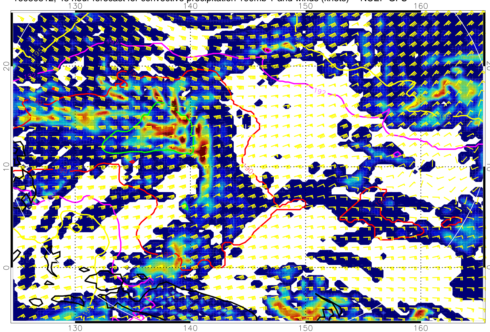
16080812, 48 hour forecast for convective precipitation 100mb T and winds (knots) -- NCEP GFS
