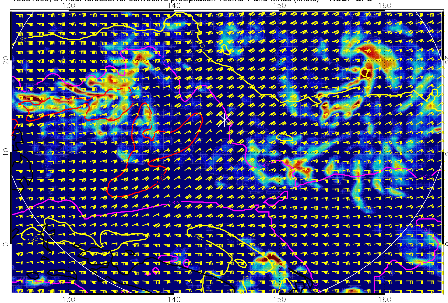
16081000, 84 hour forecast for convective precipitation 100mb T and winds (knots) -- NCEP GFS
