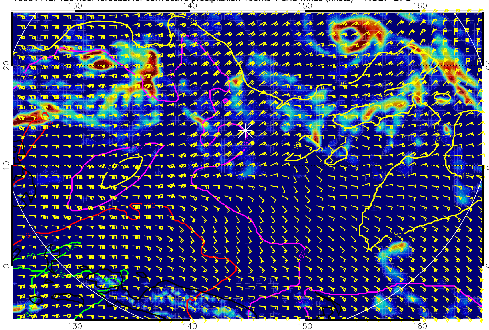
16081112, 120 hour forecast for convective precipitation 100mb T and winds (knots) -- NCEP GFS
