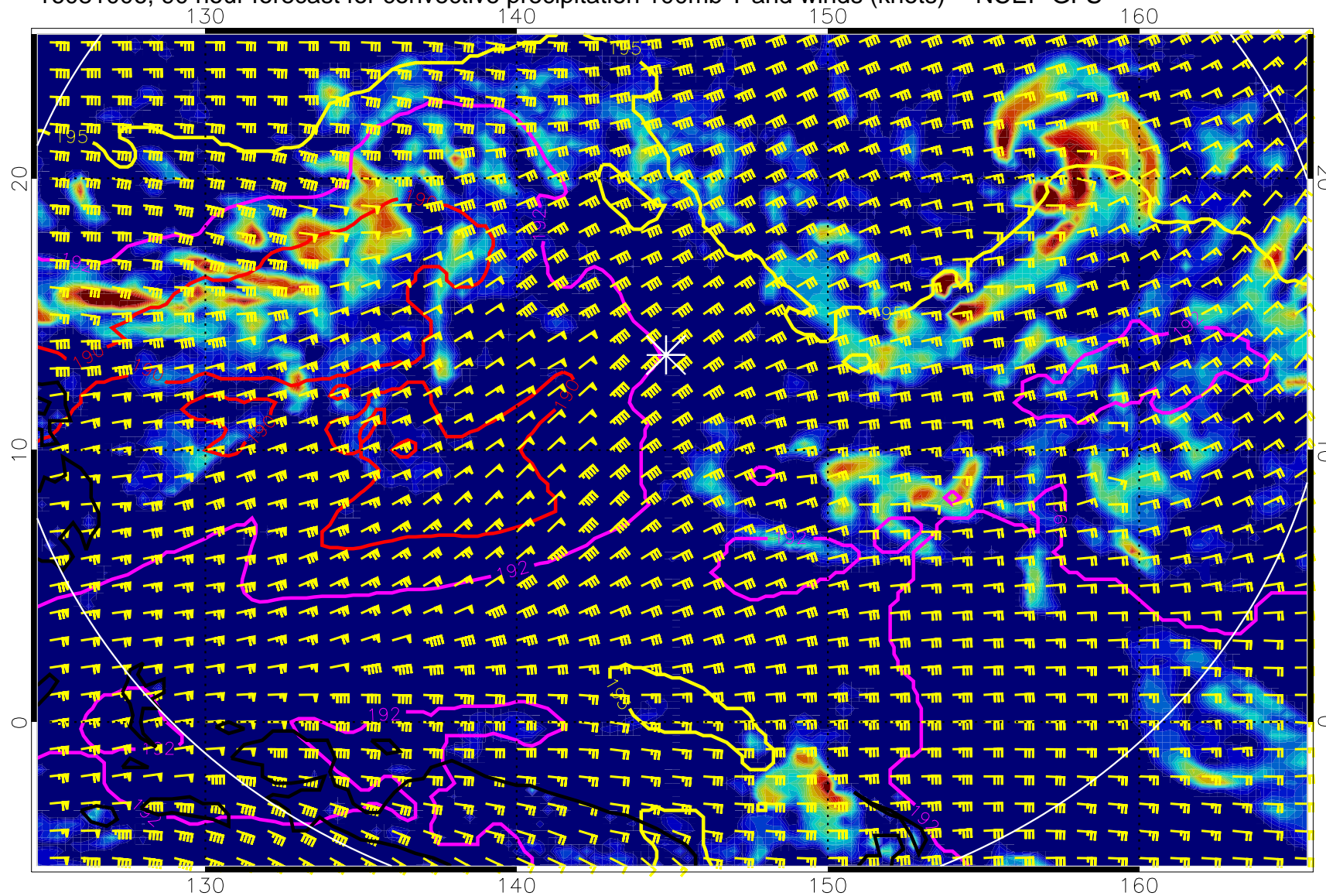
16081006, 90 hour forecast for convective precipitation 100mb T and winds (knots) -- NCEP GFS
