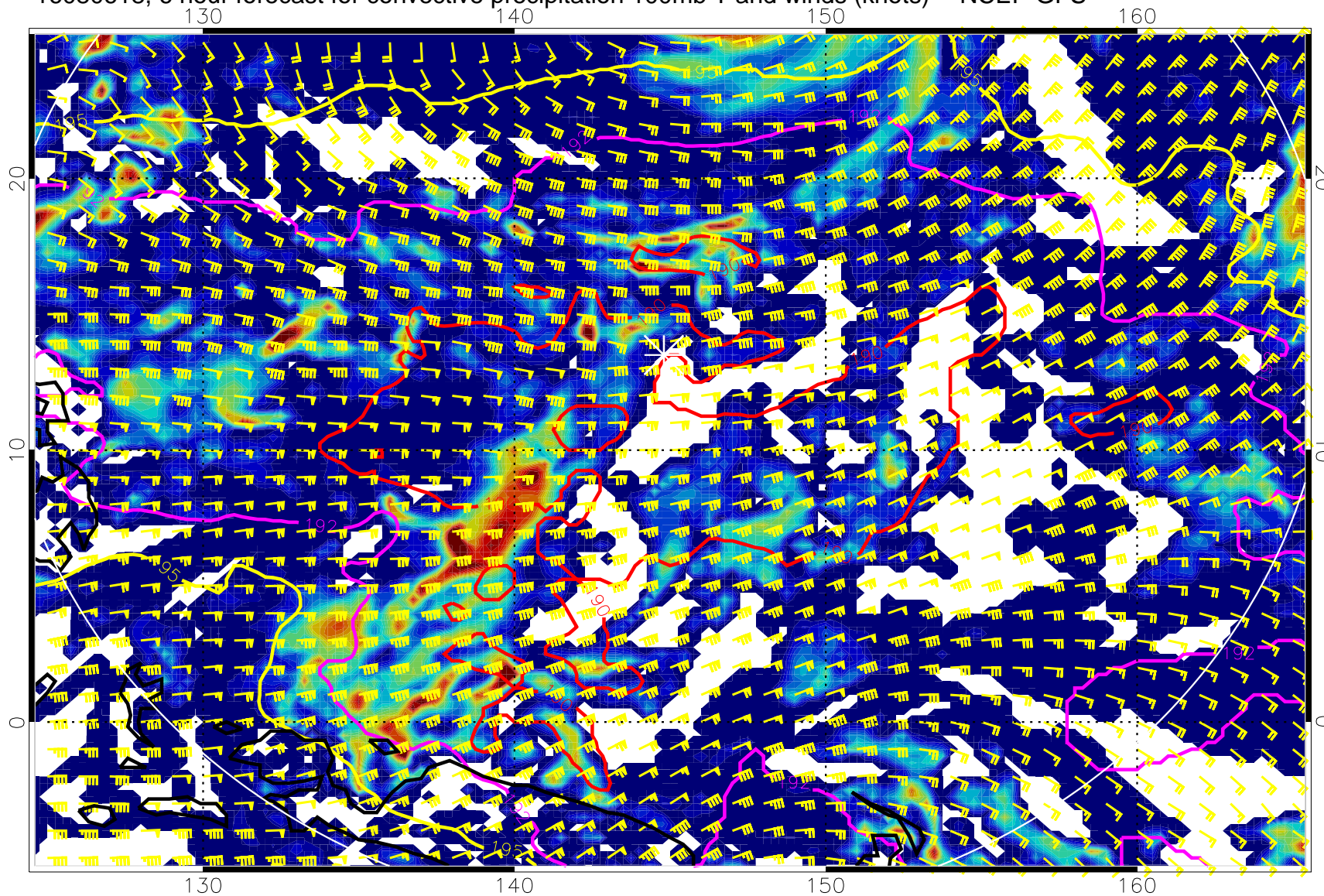
16080618, 6 hour forecast for convective precipitation 100mb T and winds (knots) -- NCEP GFS
