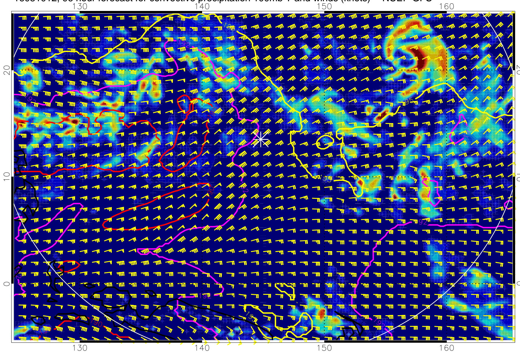
16081012, 96 hour forecast for convective precipitation 100mb T and winds (knots) -- NCEP GFS
