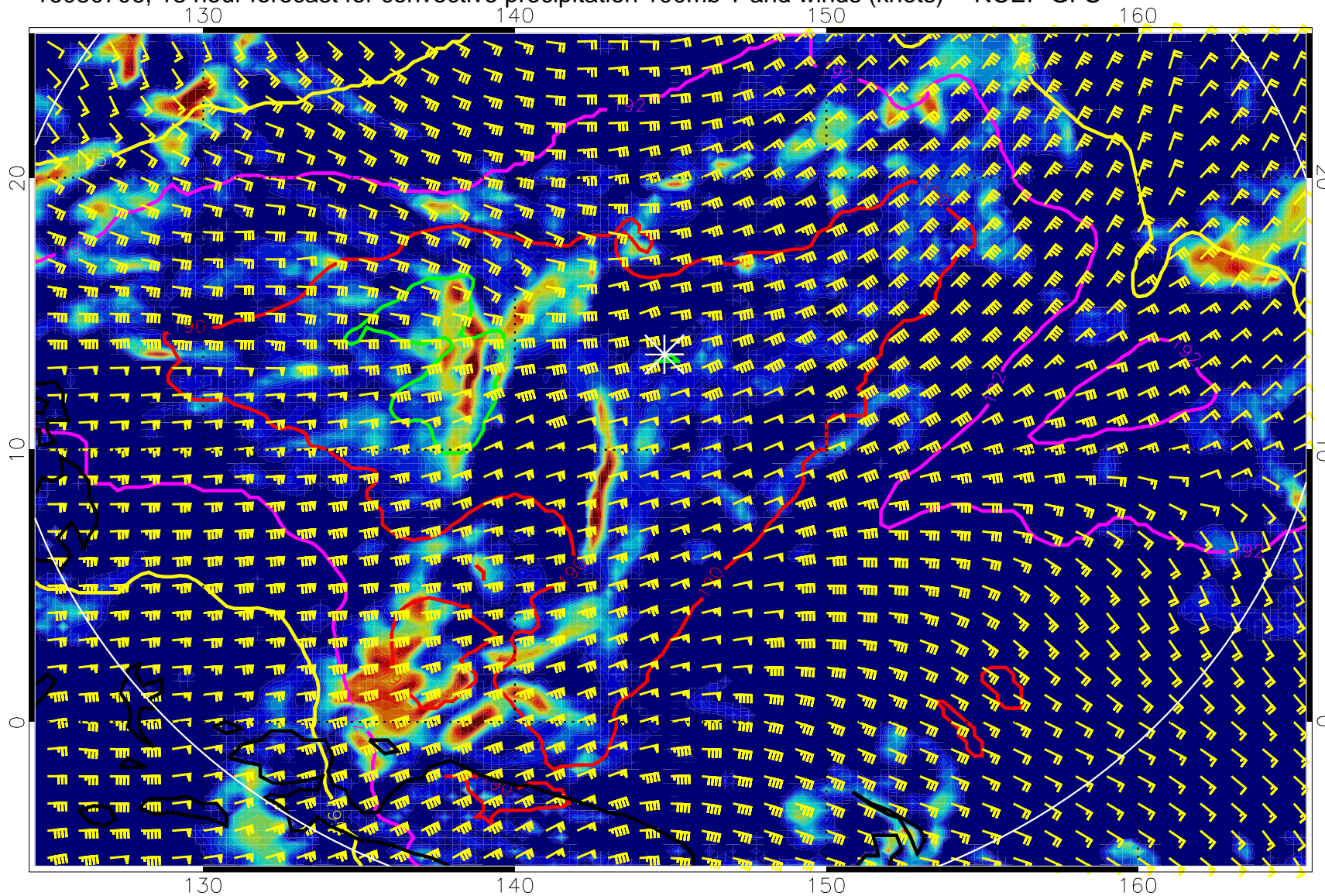
16080706, 18 hour forecast for convective precipitation 100mb T and winds (knots) -- NCEP GFS
