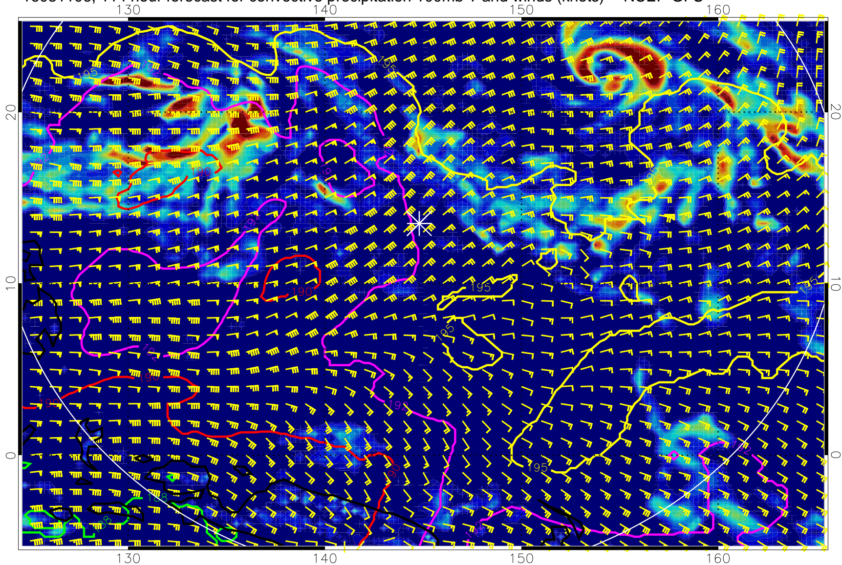
16081106, 114 hour forecast for convective precipitation 100mb T and winds (knots) -- NCEP GFS
