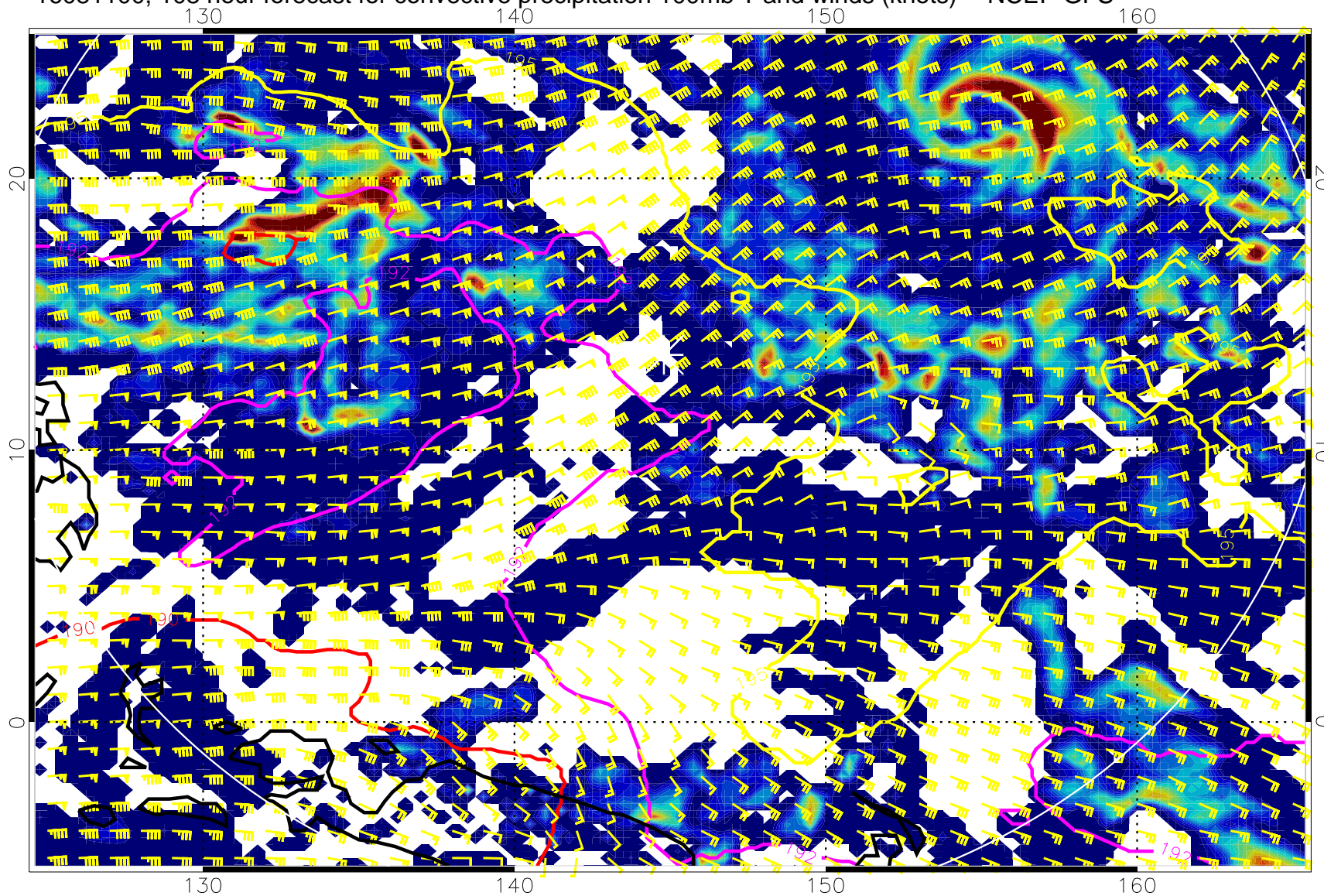
16081100, 108 hour forecast for convective precipitation 100mb T and winds (knots) -- NCEP GFS
