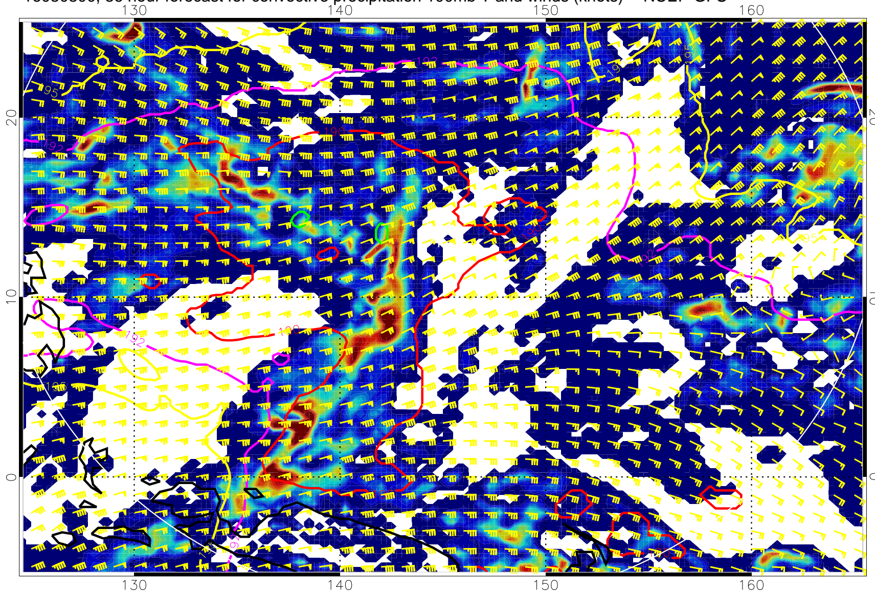
16080800, 36 hour forecast for convective precipitation 100mb T and winds (knots) -- NCEP GFS
