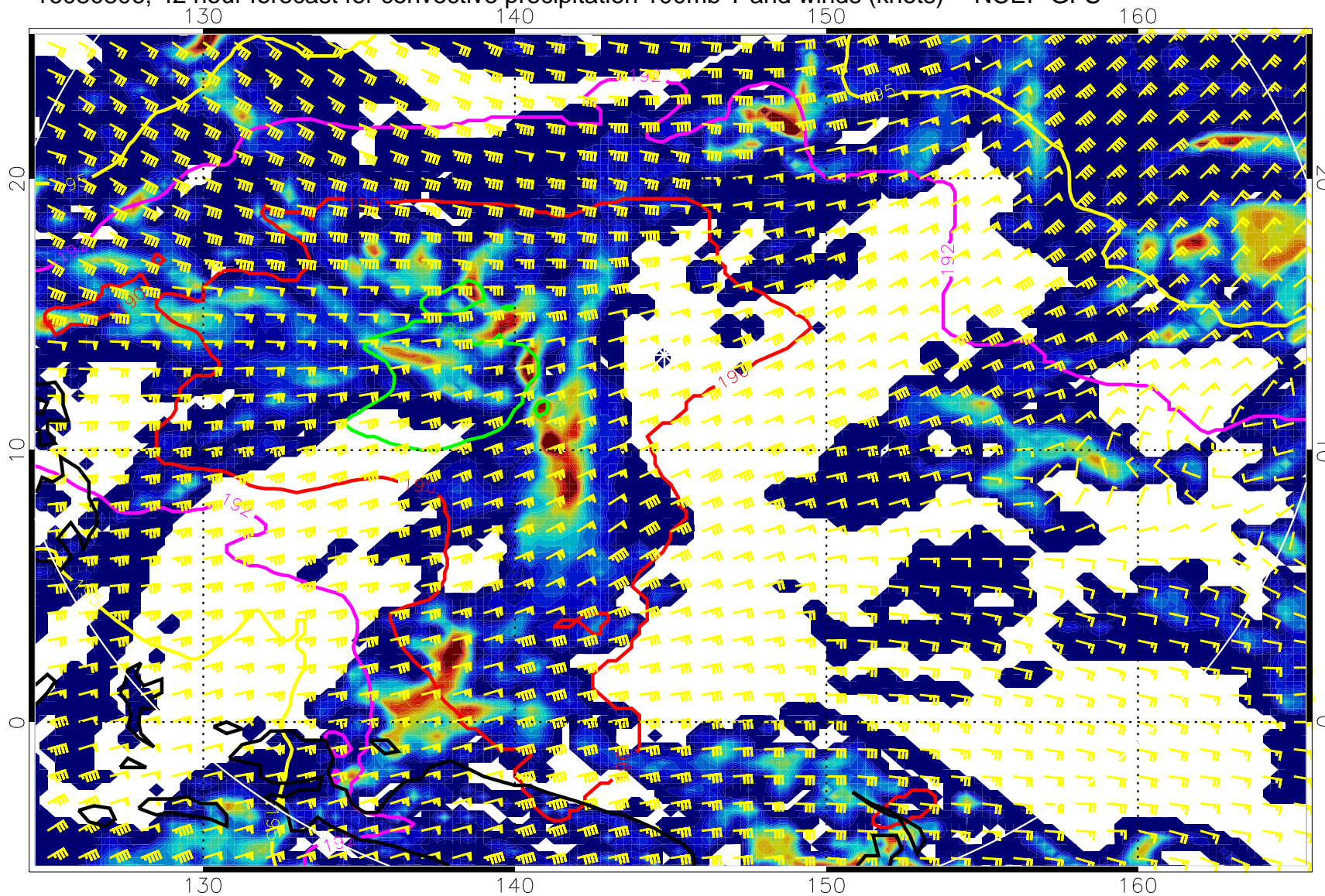
16080806, 42 hour forecast for convective precipitation 100mb T and winds (knots) -- NCEP GFS
