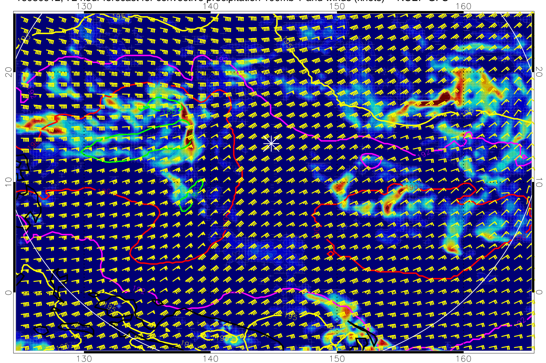
16080912, 72 hour forecast for convective precipitation 100mb T and winds (knots) -- NCEP GFS
