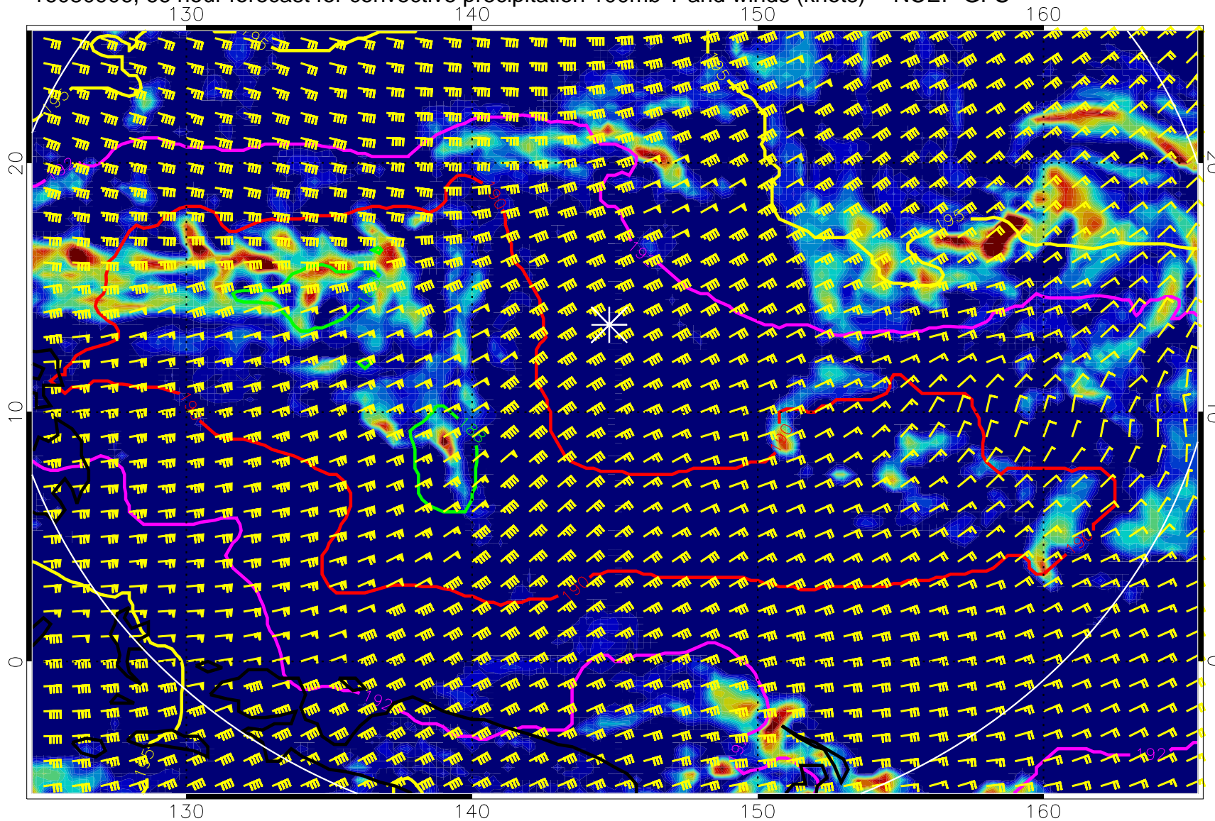
16080906, 66 hour forecast for convective precipitation 100mb T and winds (knots) -- NCEP GFS
