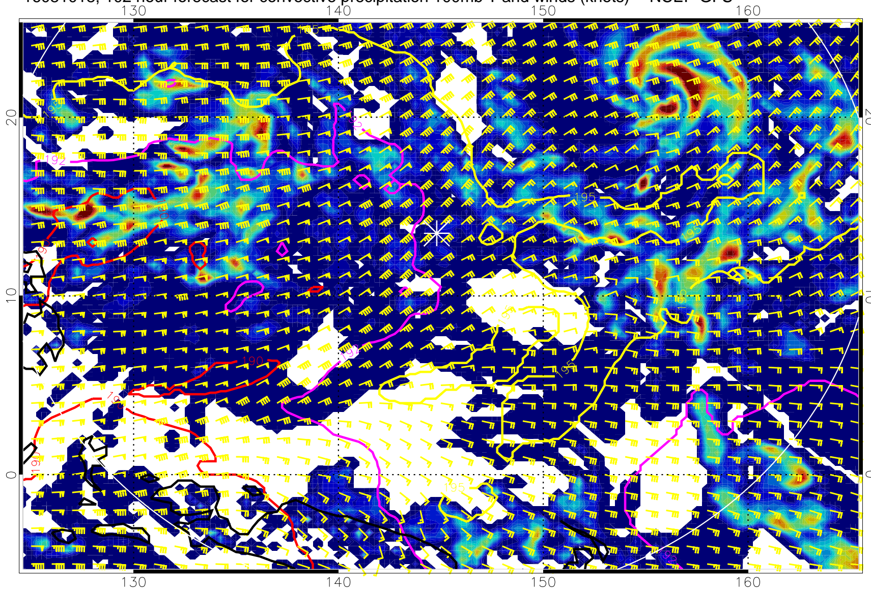
16081018, 102 hour forecast for convective precipitation 100mb T and winds (knots) -- NCEP GFS
