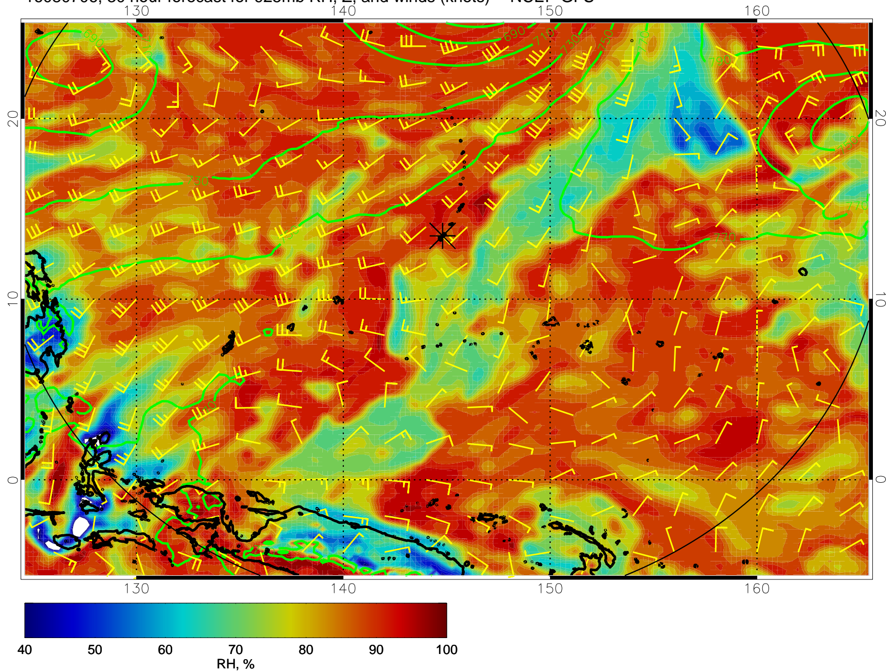
16080706, 30 hour forecast for 925mb RH, Z, and winds (knots) -- NCEP GFS
