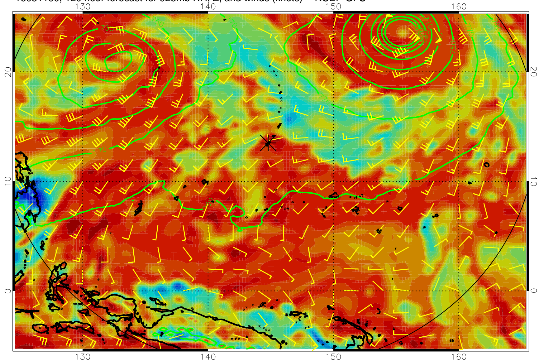
16081100, 120 hour forecast for 925mb RH, Z, and winds (knots) -- NCEP GFS
