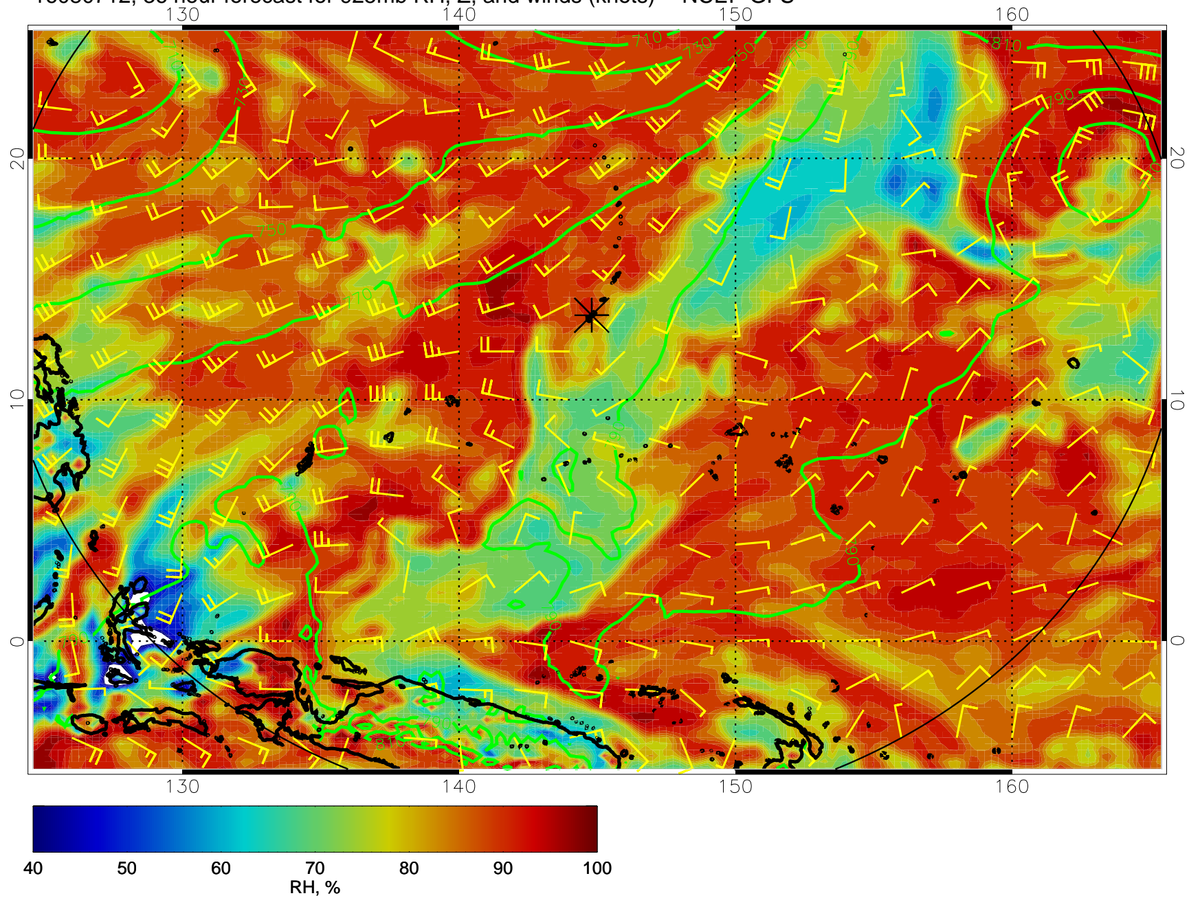
16080712, 36 hour forecast for 925mb RH, Z, and winds (knots) -- NCEP GFS
