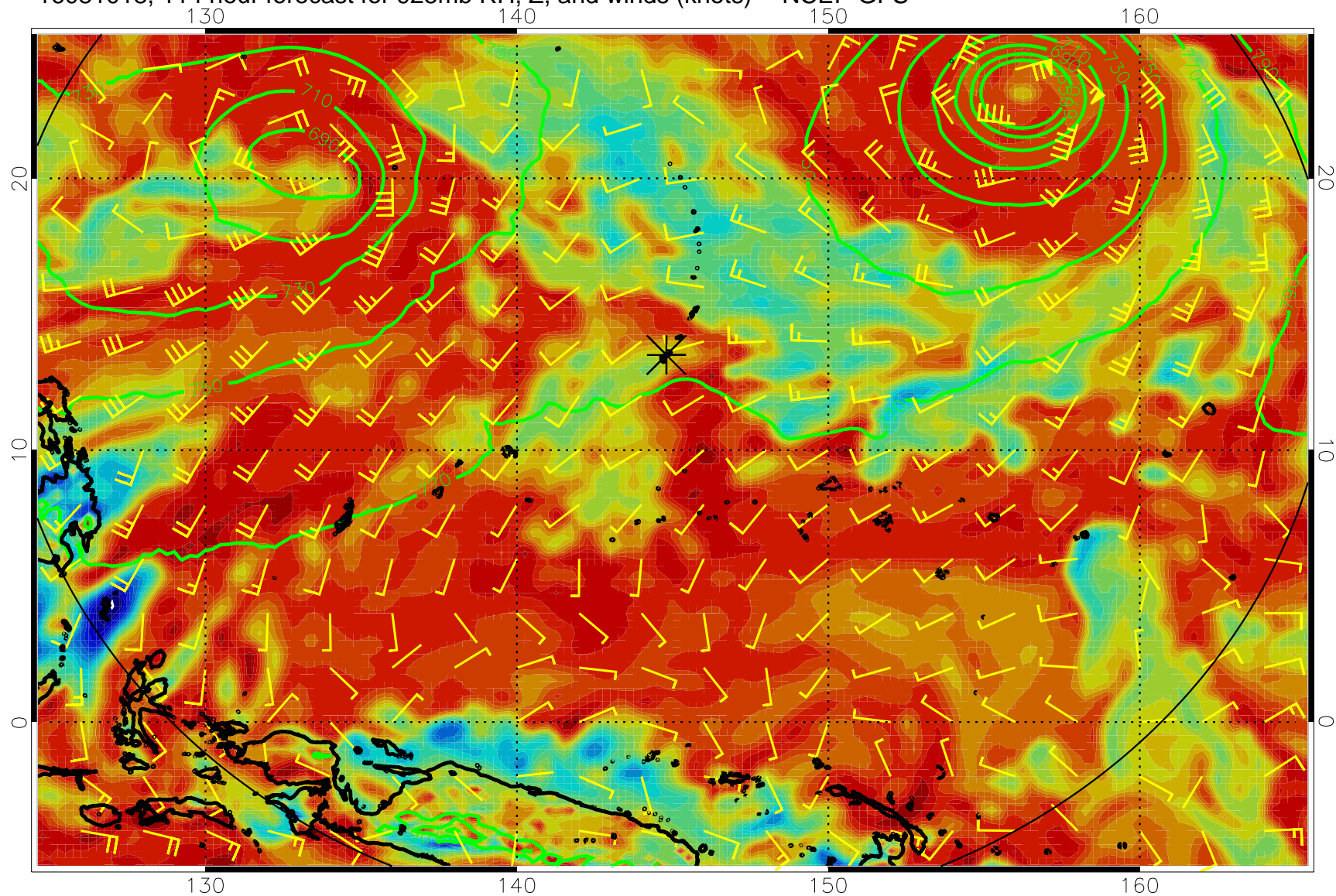
16081018, 114 hour forecast for 925mb RH, Z, and winds (knots) -- NCEP GFS
