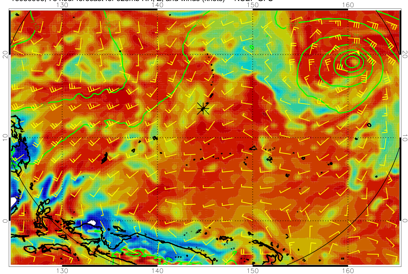
16080906, 78 hour forecast for 925mb RH, Z, and winds (knots) -- NCEP GFS
