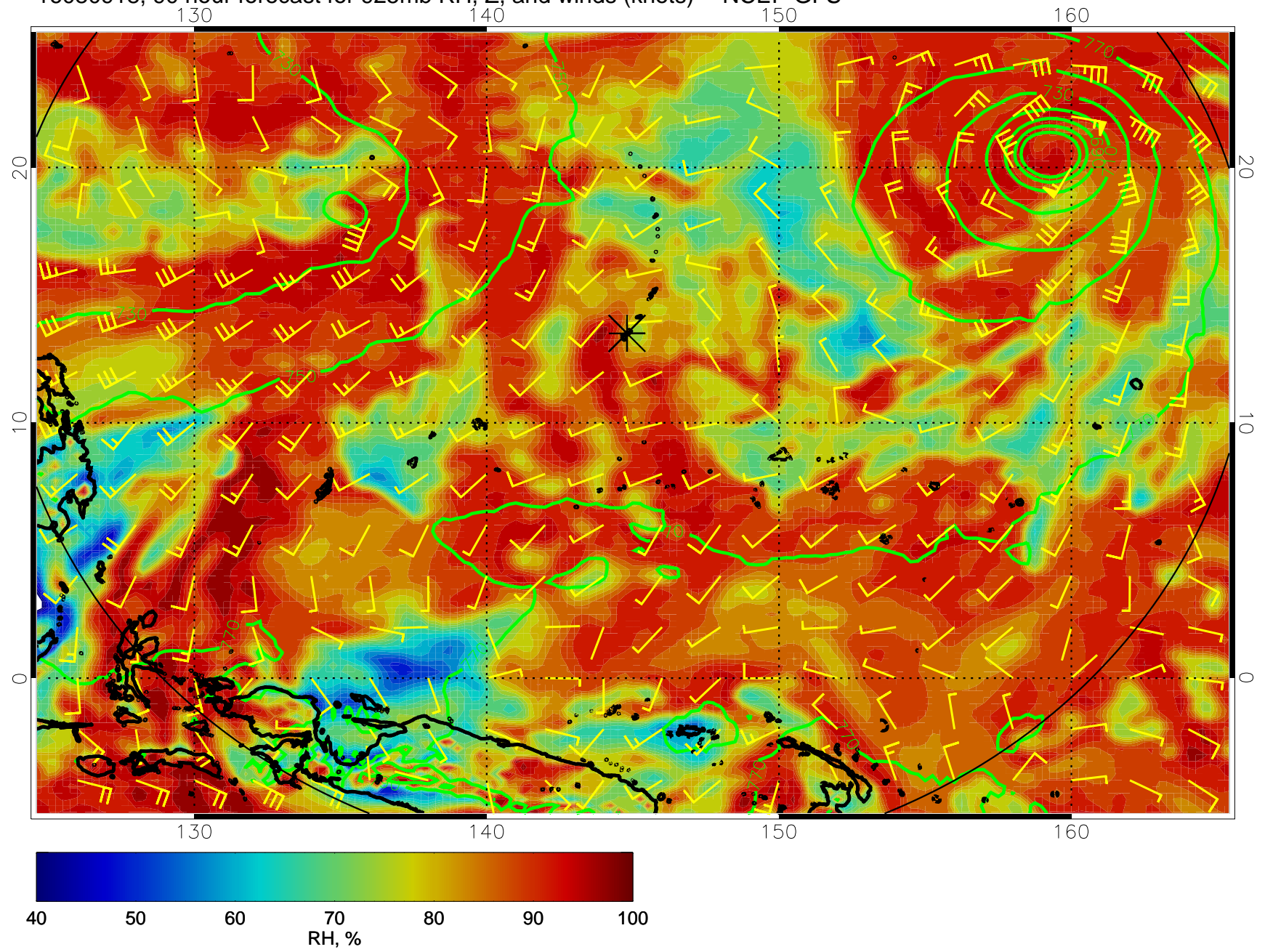
16080918, 90 hour forecast for 925mb RH, Z, and winds (knots) -- NCEP GFS
