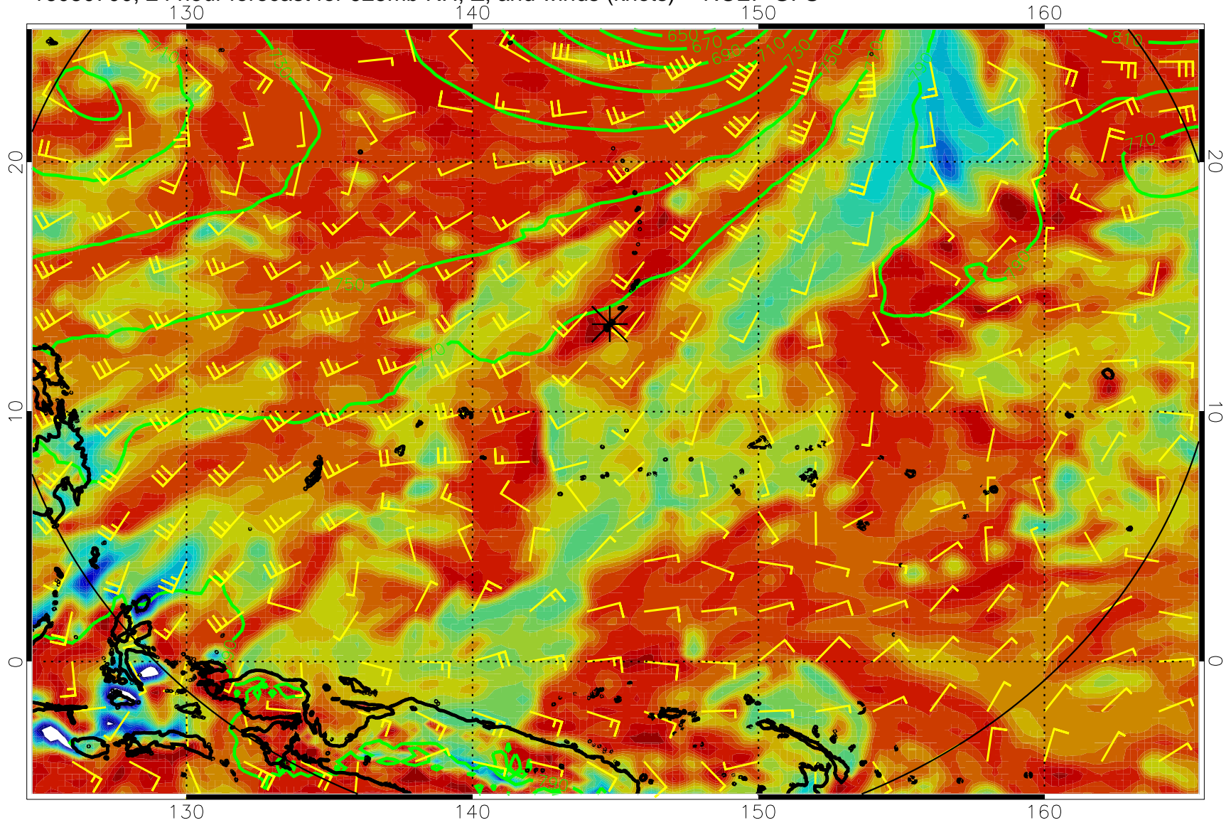
16080700, 24 hour forecast for 925mb RH, Z, and winds (knots) -- NCEP GFS
