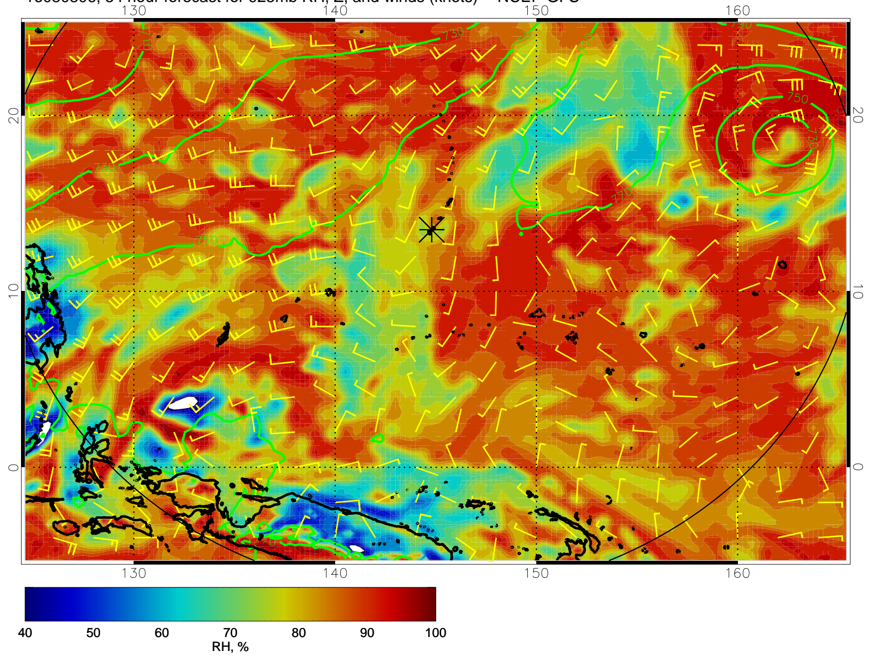
16080806, 54 hour forecast for 925mb RH, Z, and winds (knots) -- NCEP GFS
