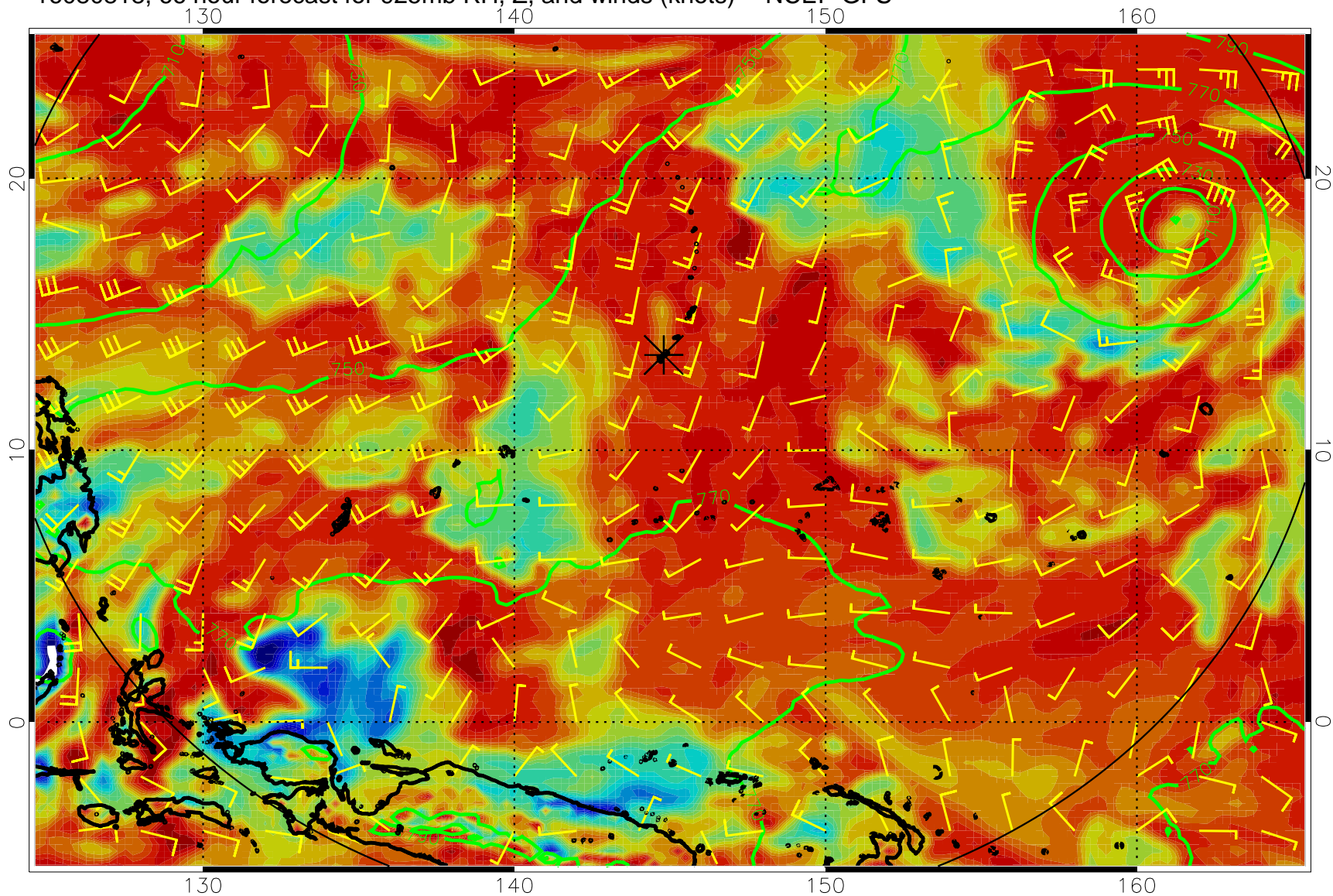
16080818, 66 hour forecast for 925mb RH, Z, and winds (knots) -- NCEP GFS
