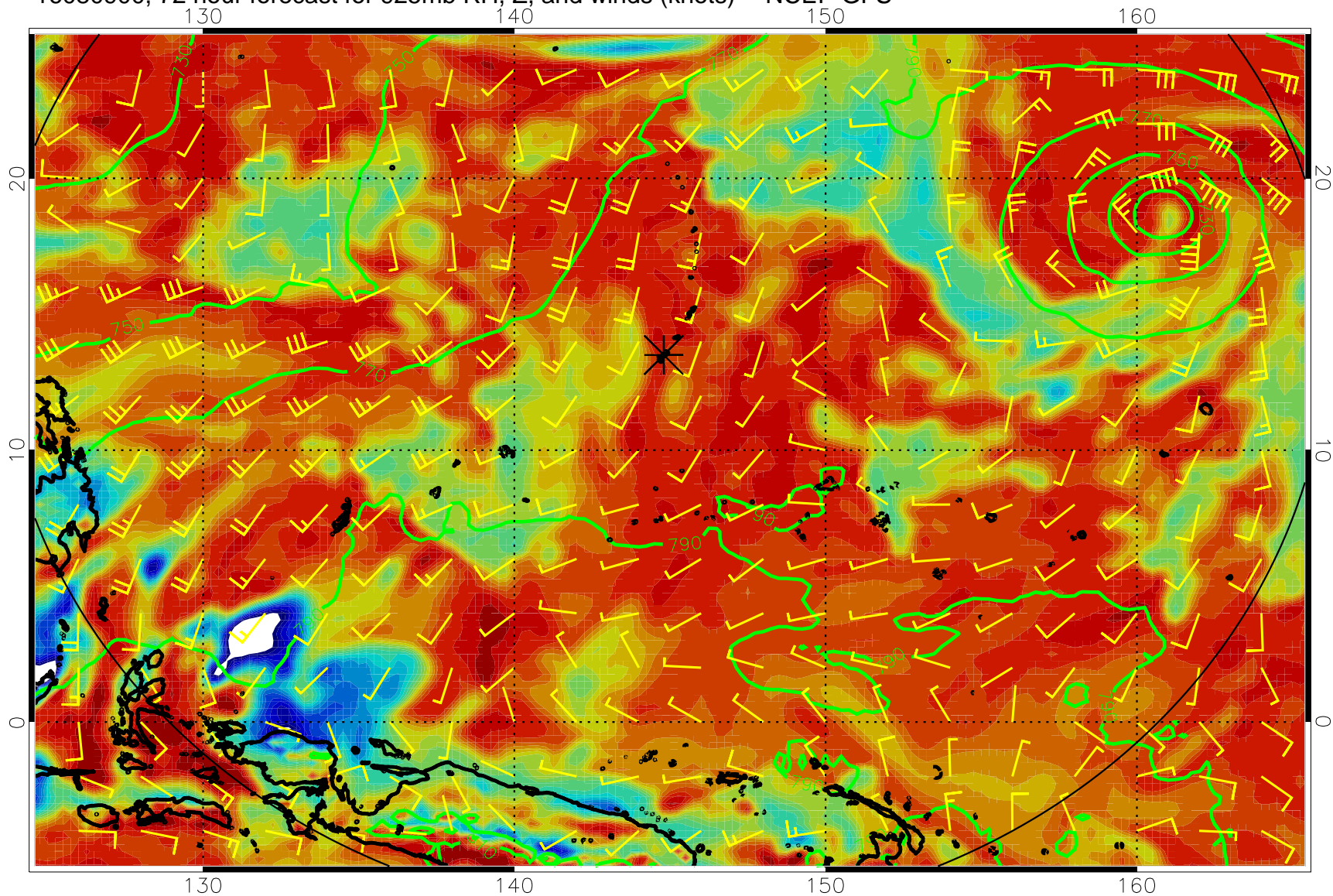
16080900, 72 hour forecast for 925mb RH, Z, and winds (knots) -- NCEP GFS
