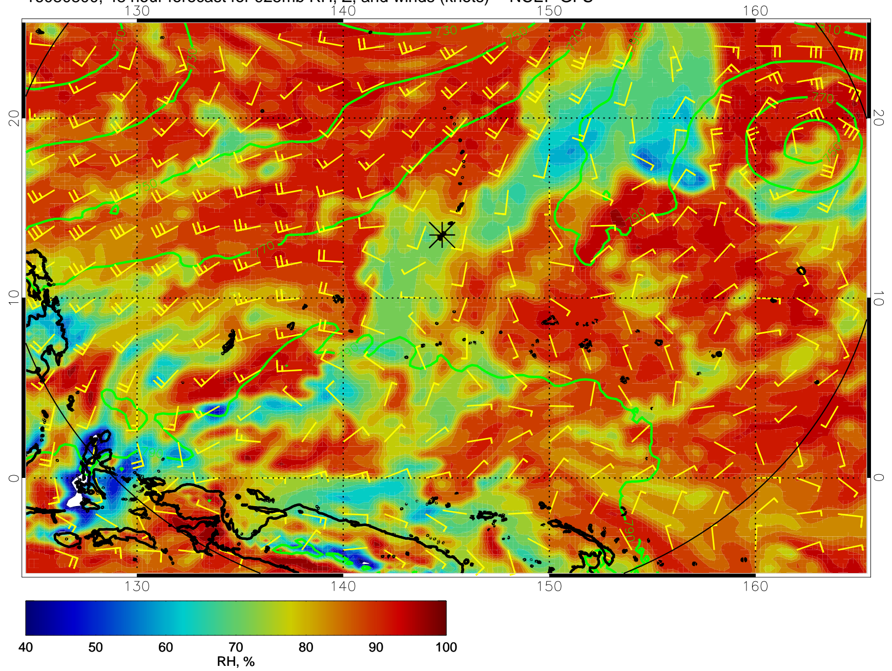
16080800, 48 hour forecast for 925mb RH, Z, and winds (knots) -- NCEP GFS
