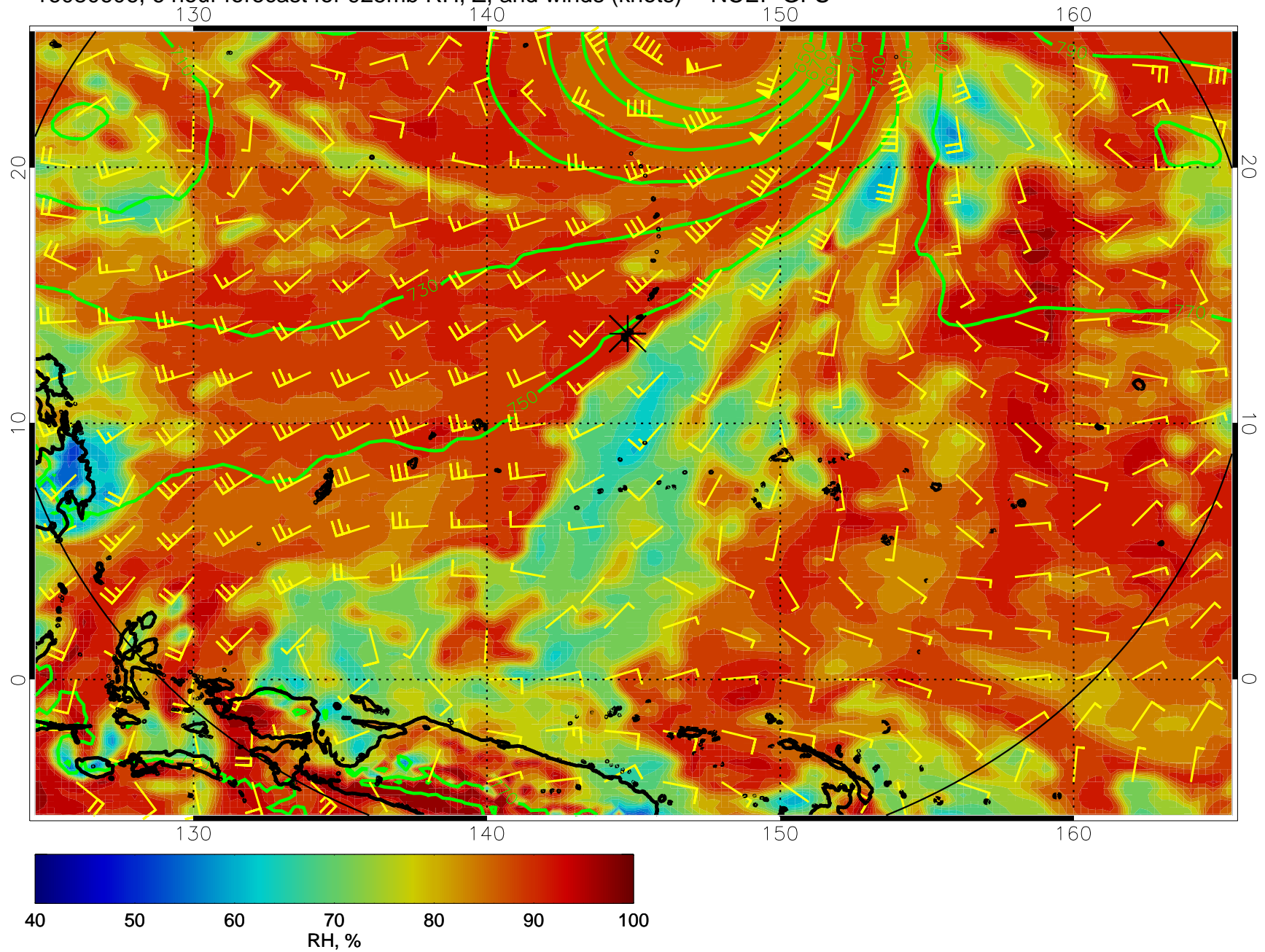
16080606, 6 hour forecast for 925mb RH, Z, and winds (knots) -- NCEP GFS
