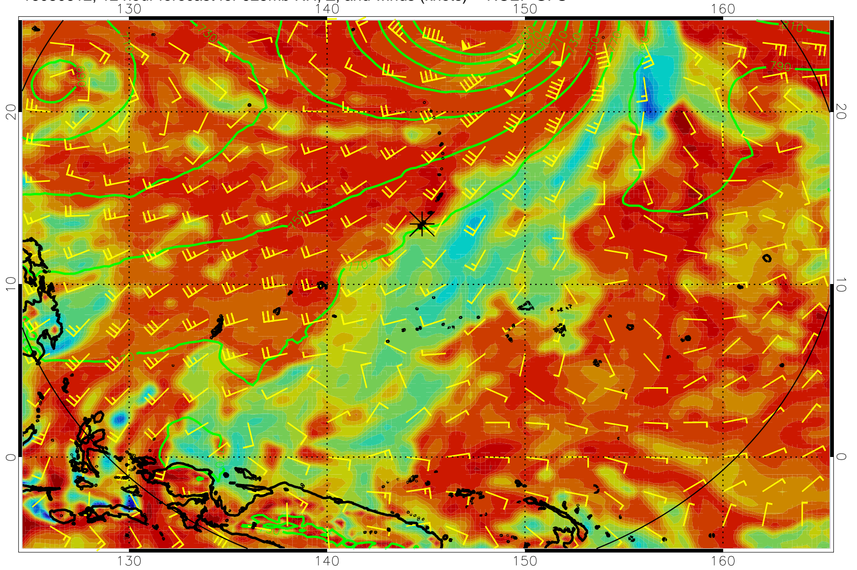
16080612, 12 hour forecast for 925mb RH, Z, and winds (knots) -- NCEP GFS
