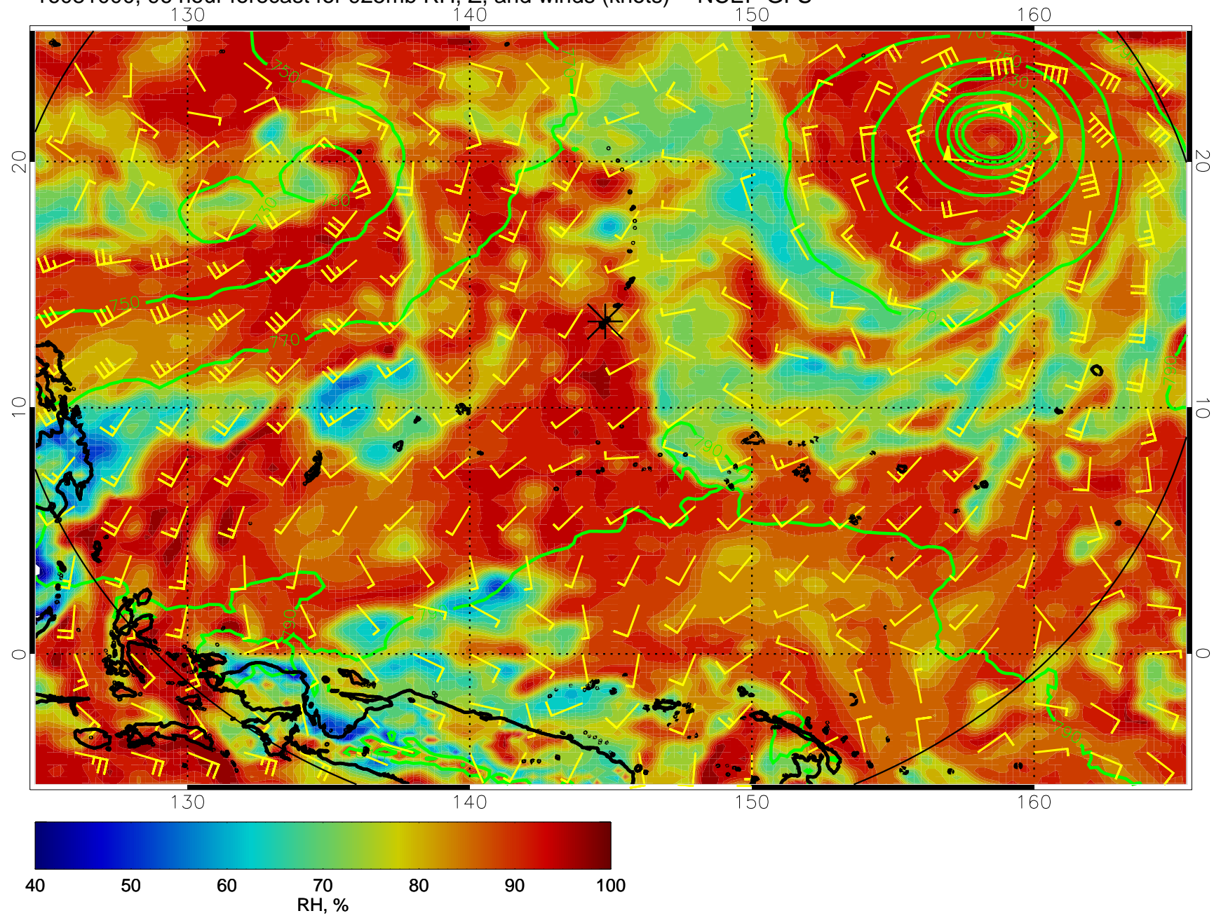
16081000, 96 hour forecast for 925mb RH, Z, and winds (knots) -- NCEP GFS
