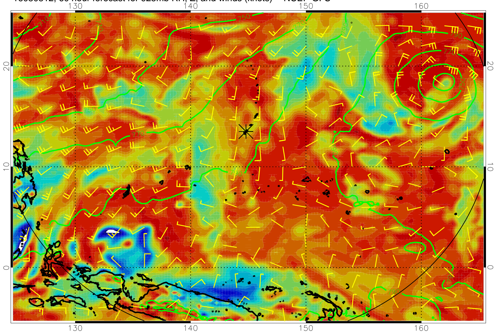
16080812, 60 hour forecast for 925mb RH, Z, and winds (knots) -- NCEP GFS
