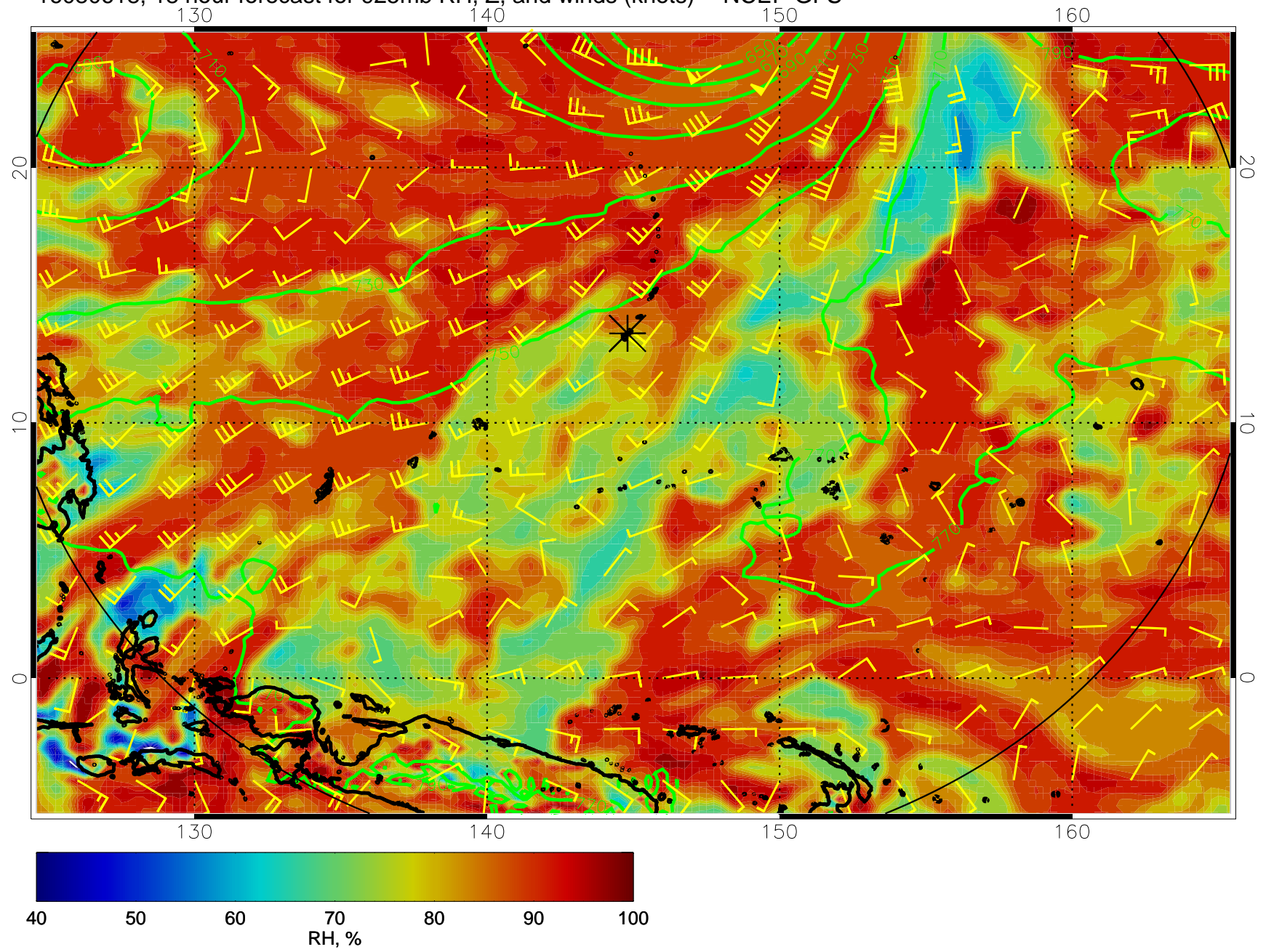
16080618, 18 hour forecast for 925mb RH, Z, and winds (knots) -- NCEP GFS
