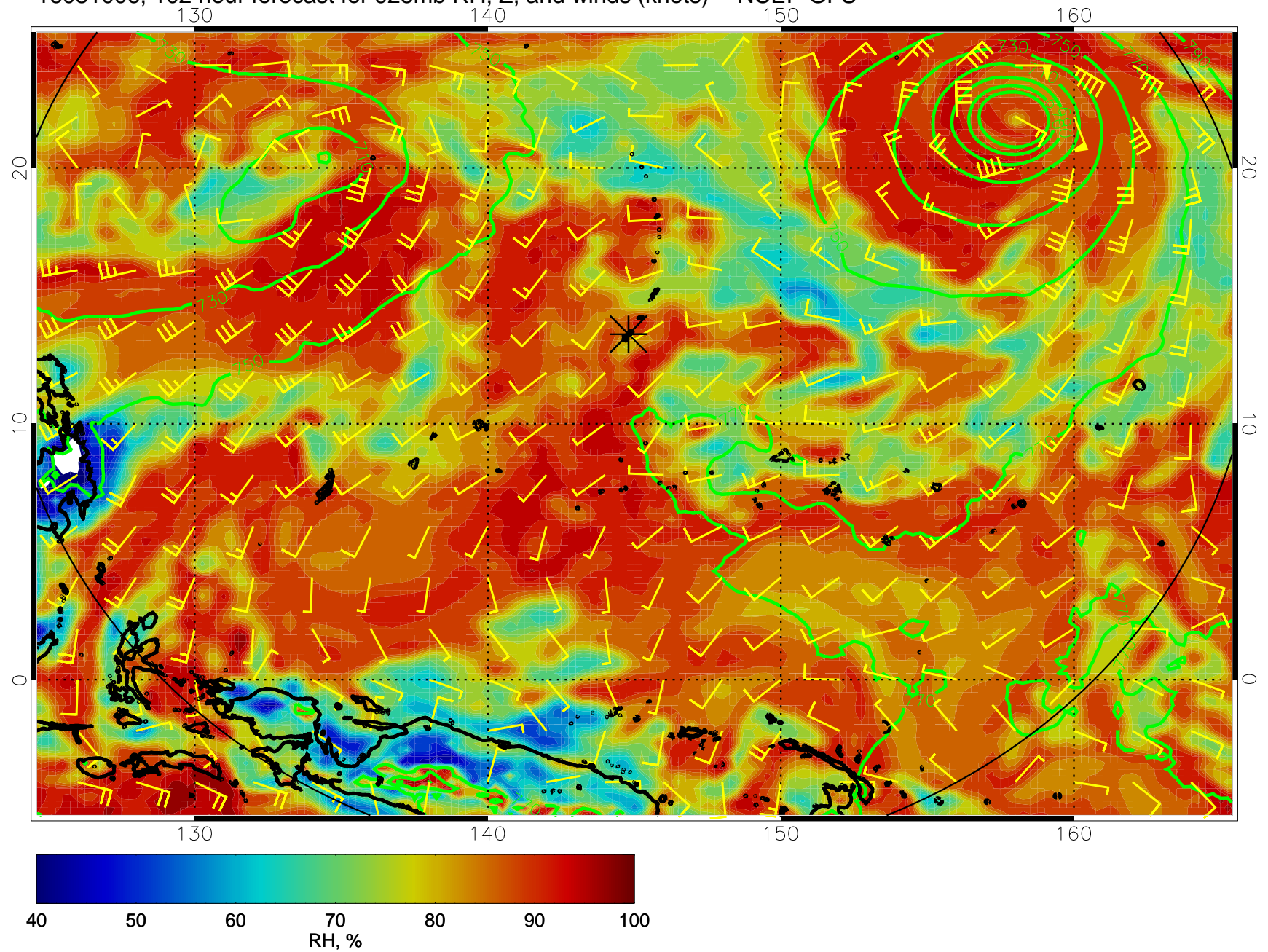
16081006, 102 hour forecast for 925mb RH, Z, and winds (knots) -- NCEP GFS
