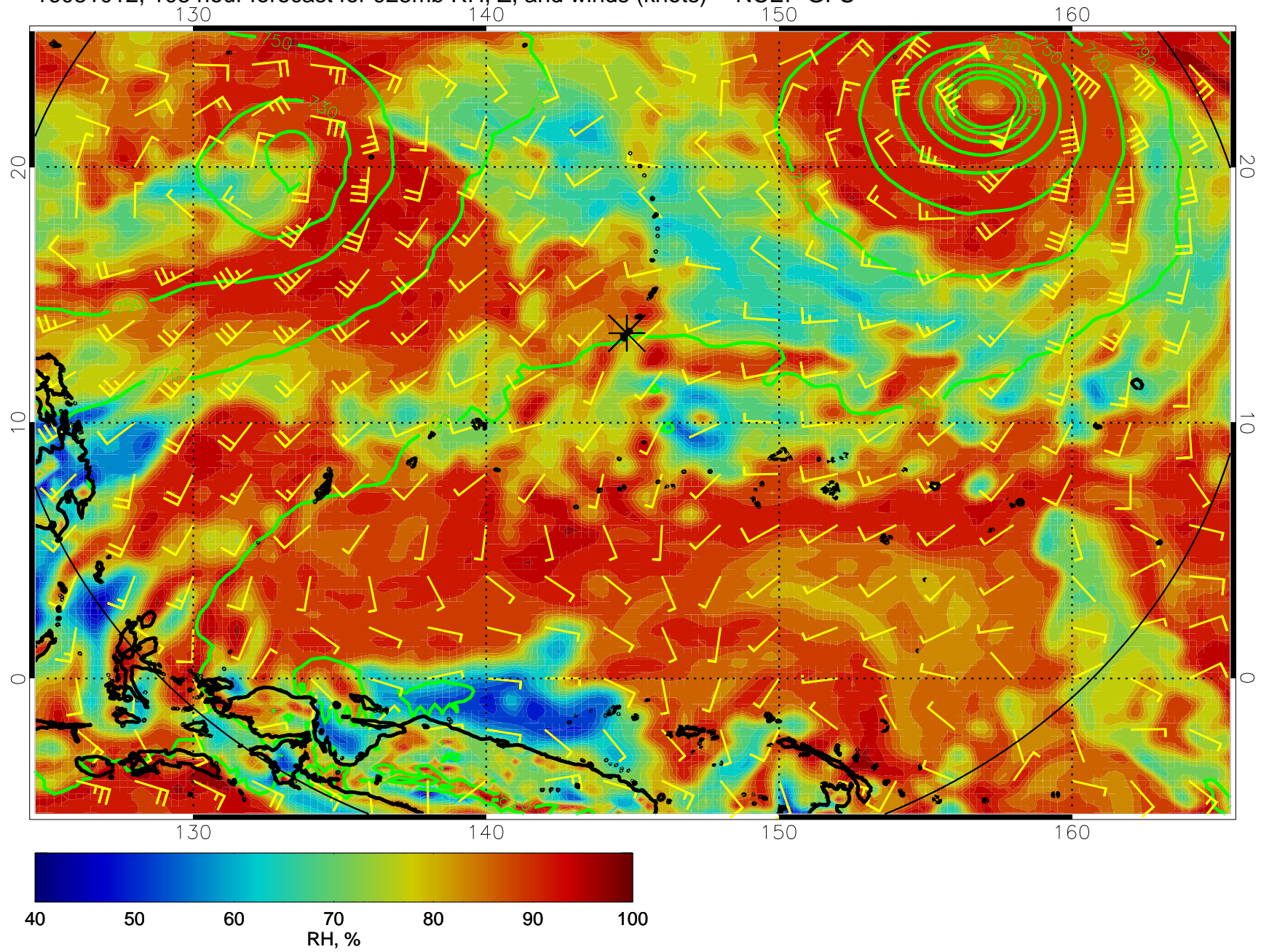
16081012, 108 hour forecast for 925mb RH, Z, and winds (knots) -- NCEP GFS
