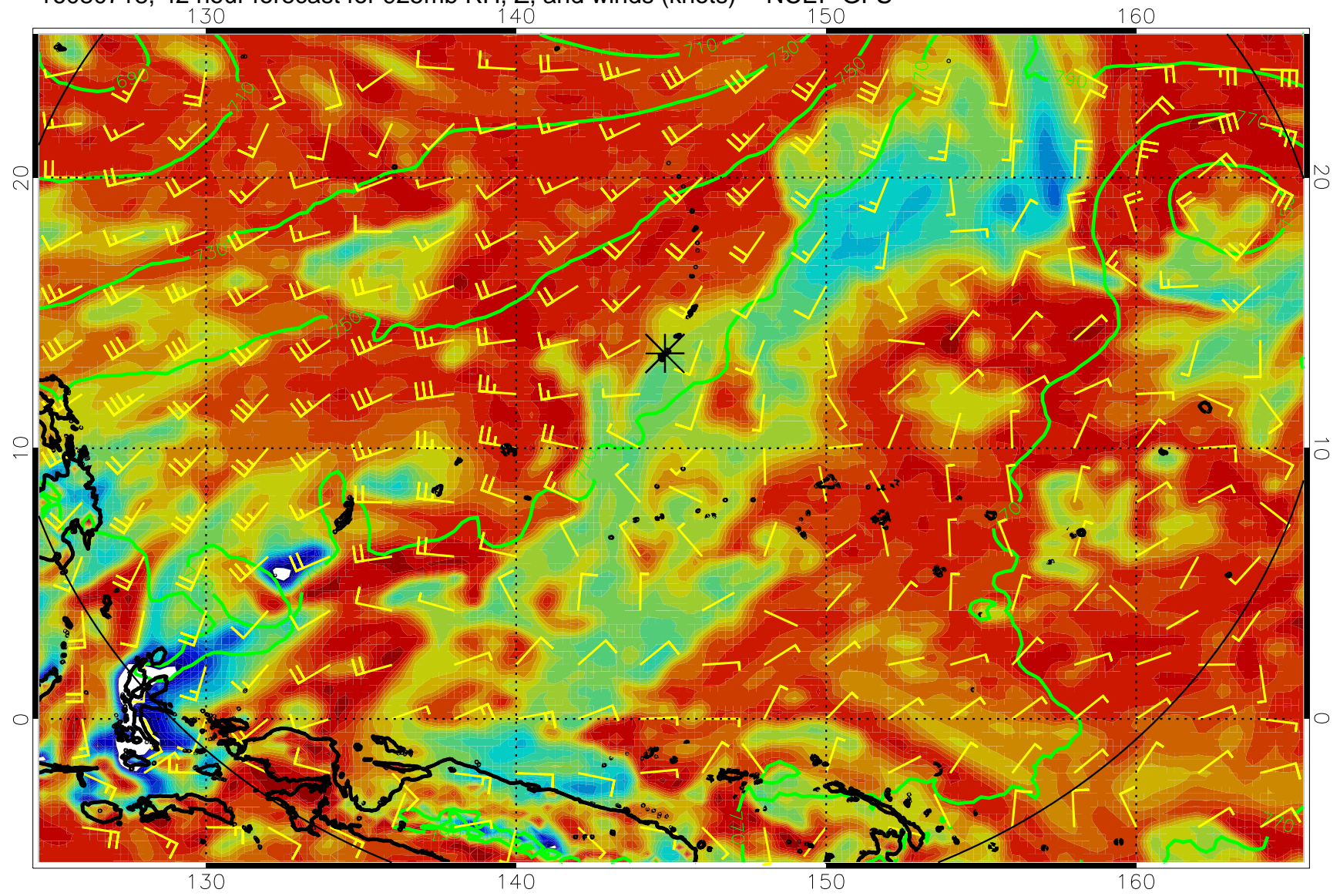
16080718, 42 hour forecast for 925mb RH, Z, and winds (knots) -- NCEP GFS
