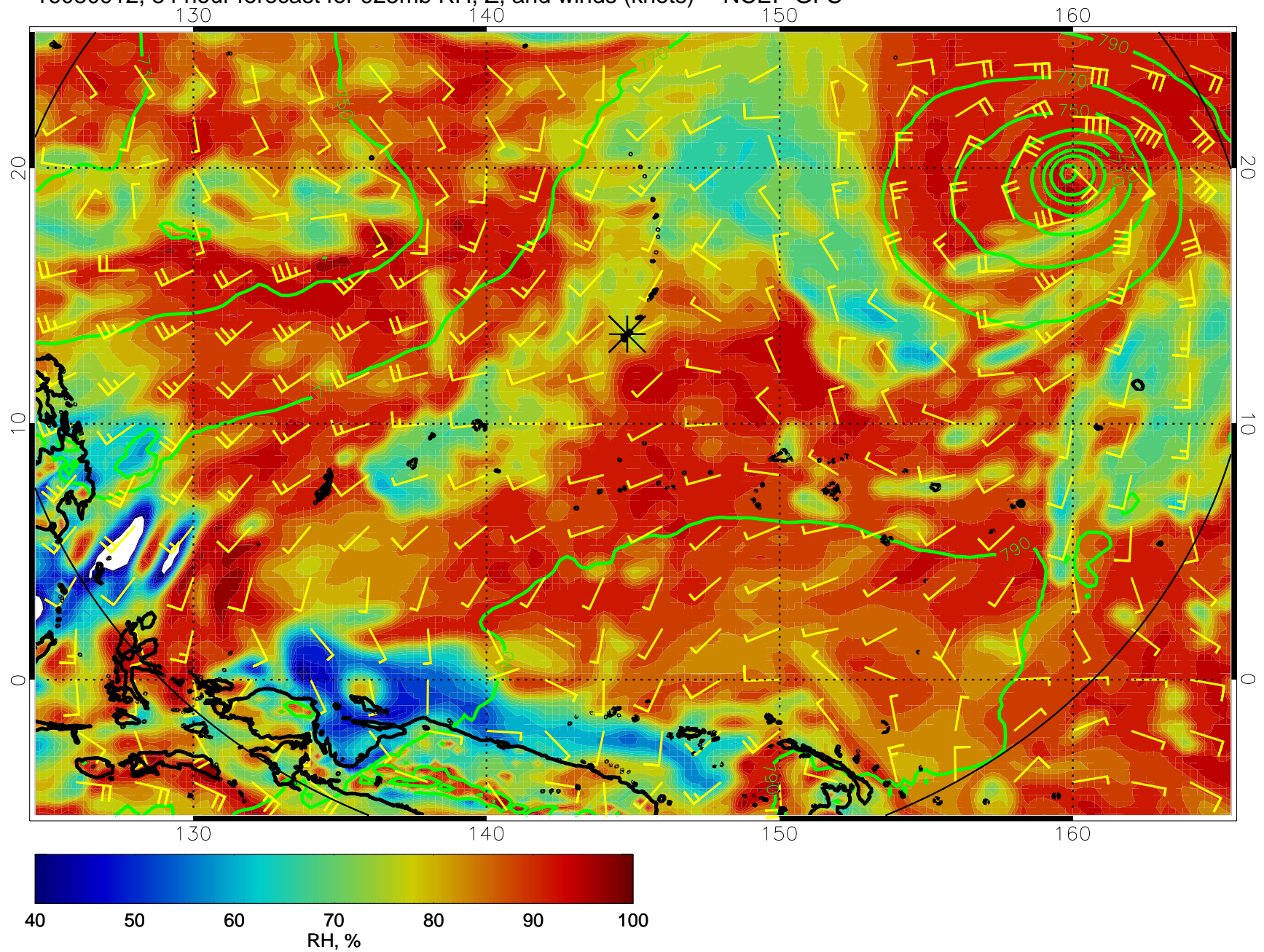
16080912, 84 hour forecast for 925mb RH, Z, and winds (knots) -- NCEP GFS
