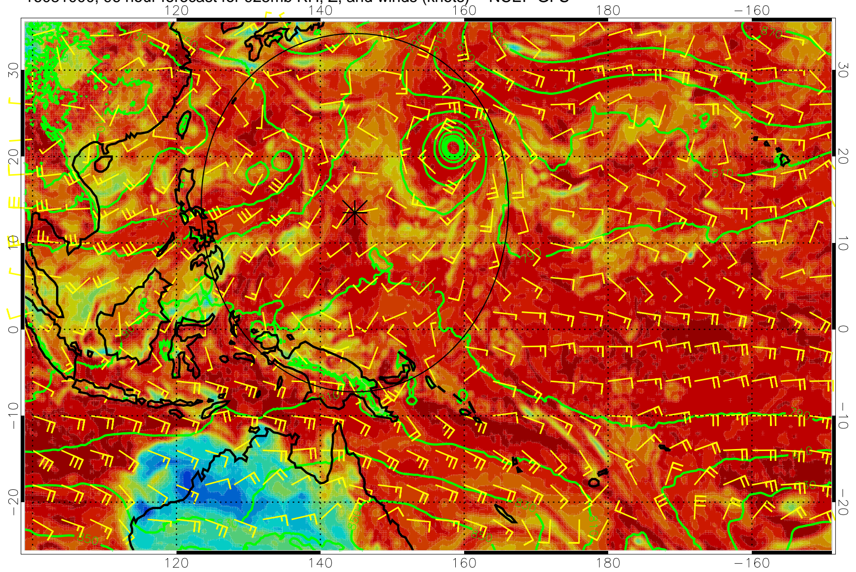
16081000, 96 hour forecast for 925mb RH, Z, and winds (knots) -- NCEP GFS
