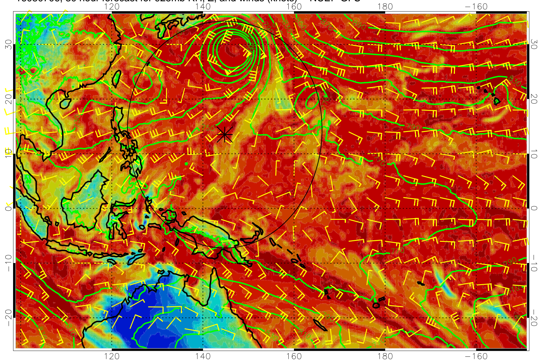
16080706, 30 hour forecast for 925mb RH, Z, and winds (knots) -- NCEP GFS
