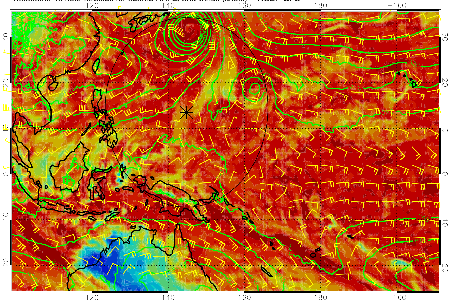
16080800, 48 hour forecast for 925mb RH, Z, and winds (knots) -- NCEP GFS
