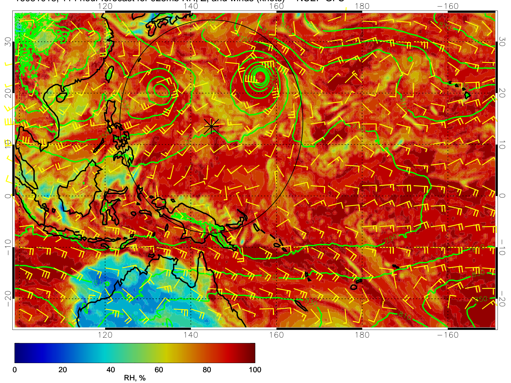
16081018, 114 hour forecast for 925mb RH, Z, and winds (knots) -- NCEP GFS
