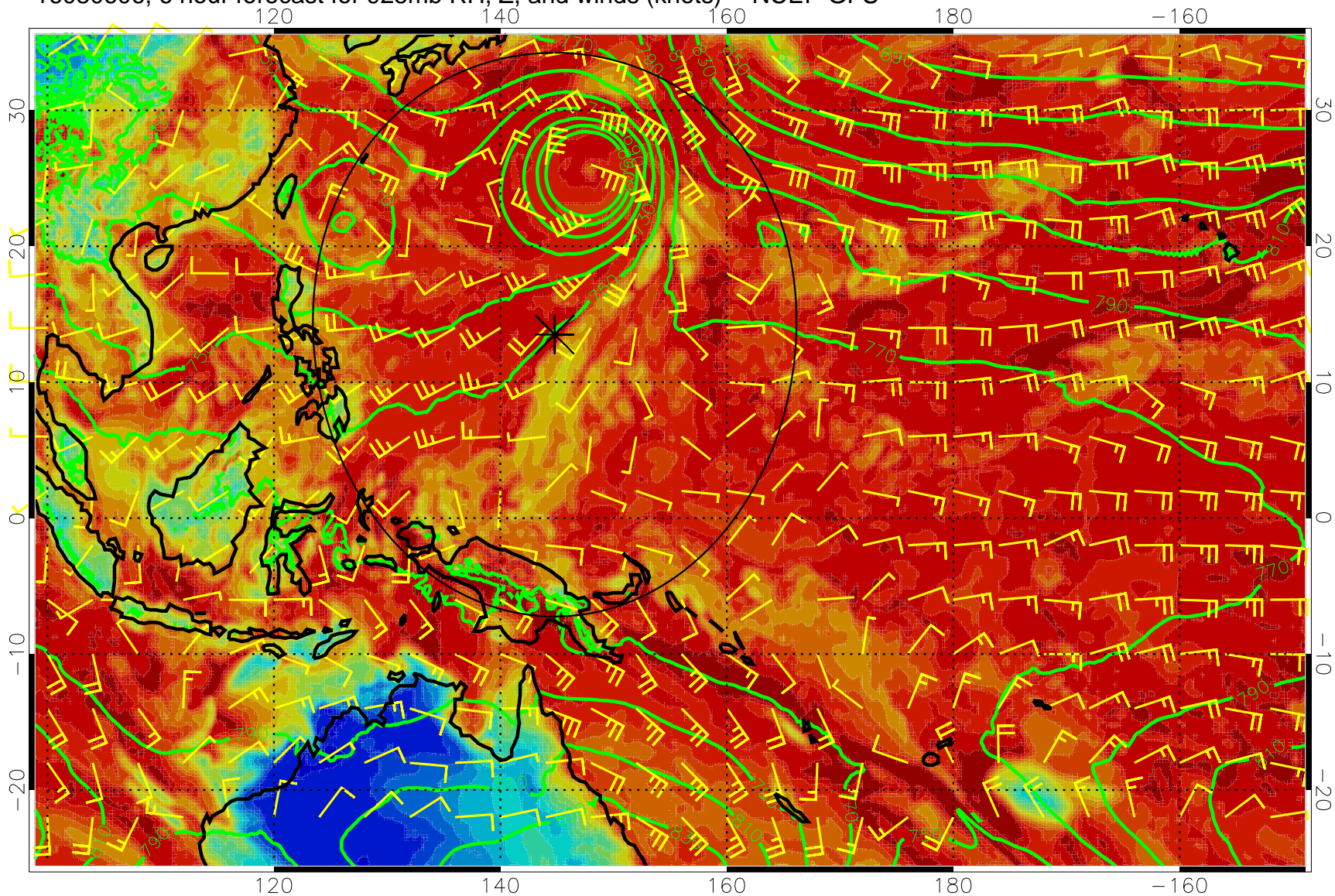
16080606, 6 hour forecast for 925mb RH, Z, and winds (knots) -- NCEP GFS
