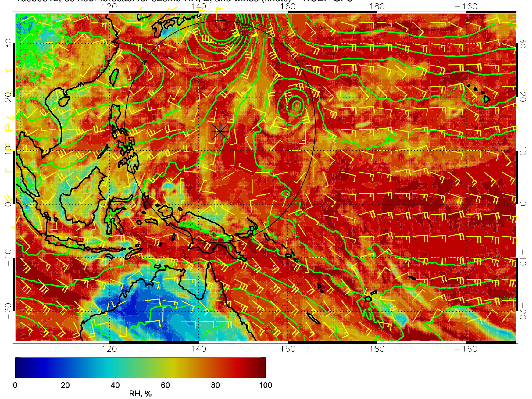
16080812, 60 hour forecast for 925mb RH, Z, and winds (knots) -- NCEP GFS
