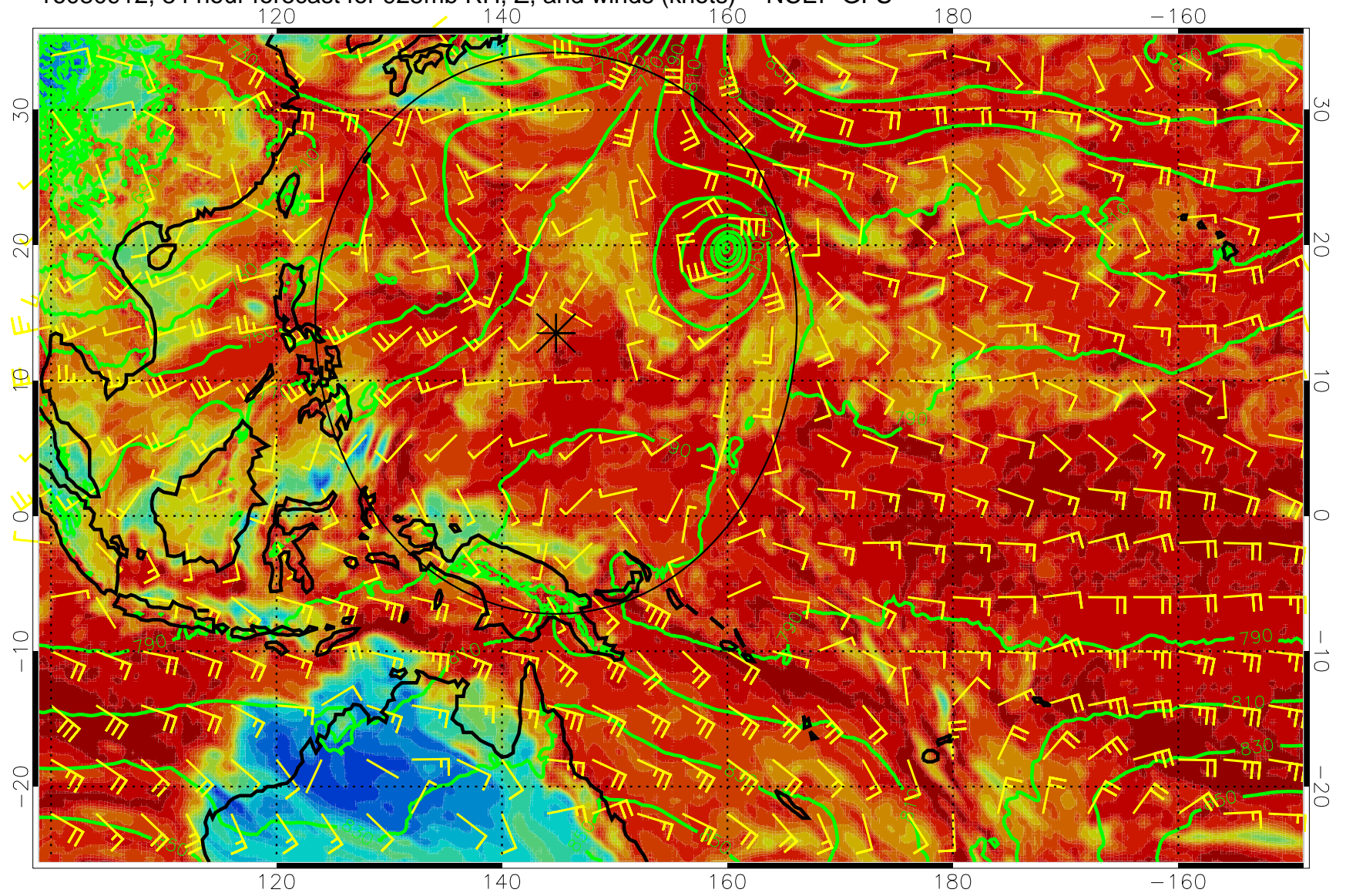
16080912, 84 hour forecast for 925mb RH, Z, and winds (knots) -- NCEP GFS
